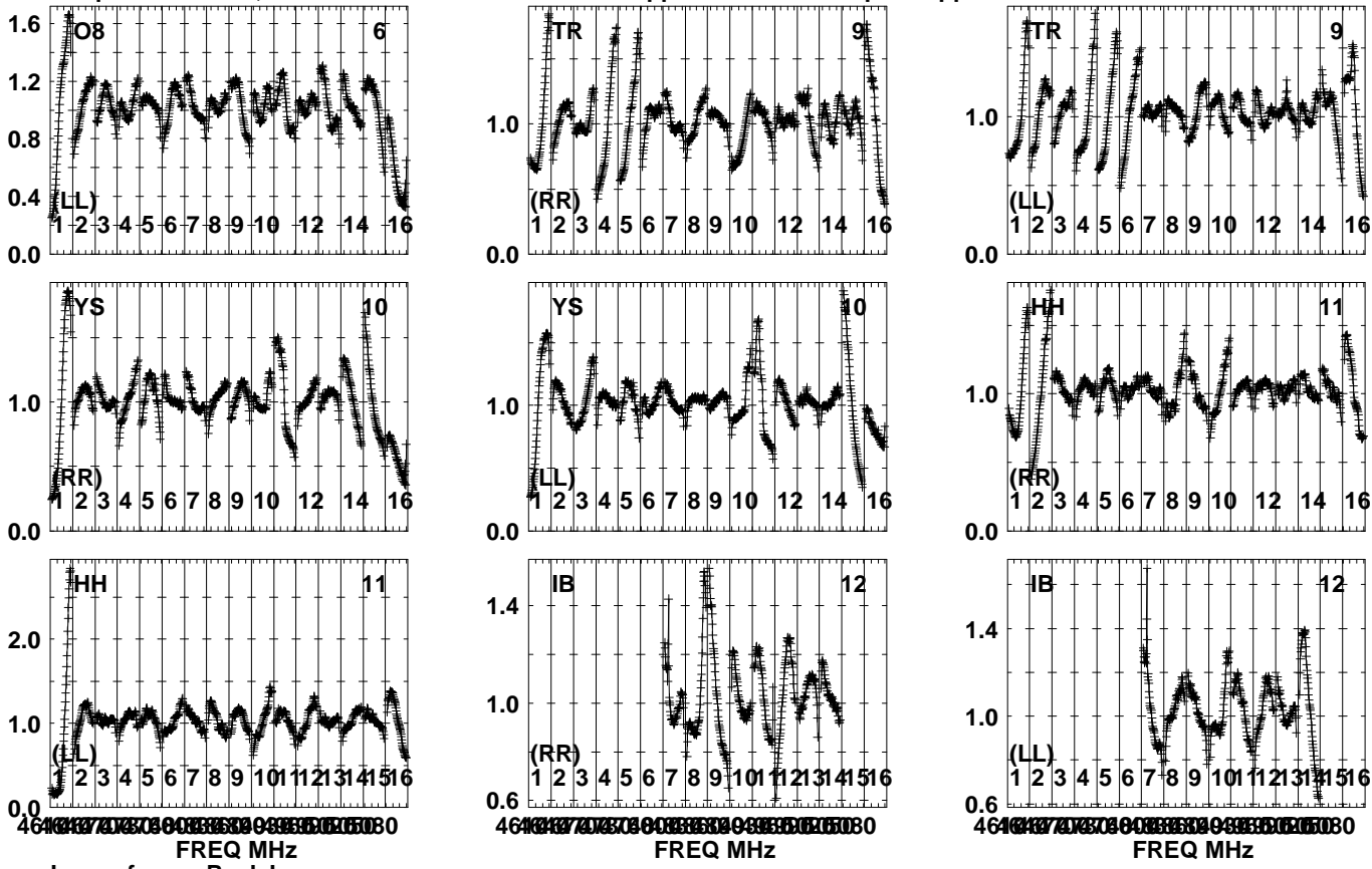
Lower frame: Real Jy Auto-corr total-power spectrum Antenna: * Timerange: 00/13:36:53 to 00/13:37:49
