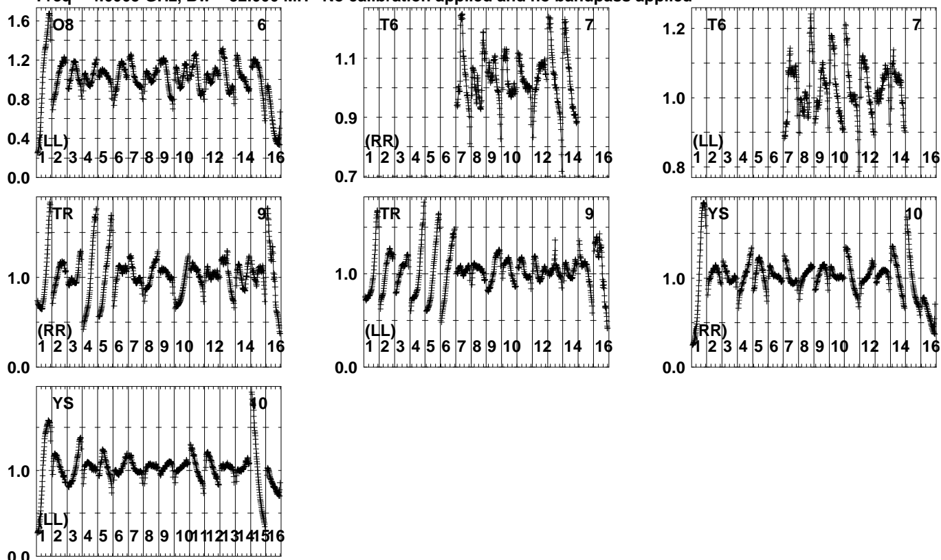
FREQ MHz Lower frame: Real Jy Auto-corr total-power spectrum Antenna: * Timerange: 00/07:07:13 to 00/07:08:09
