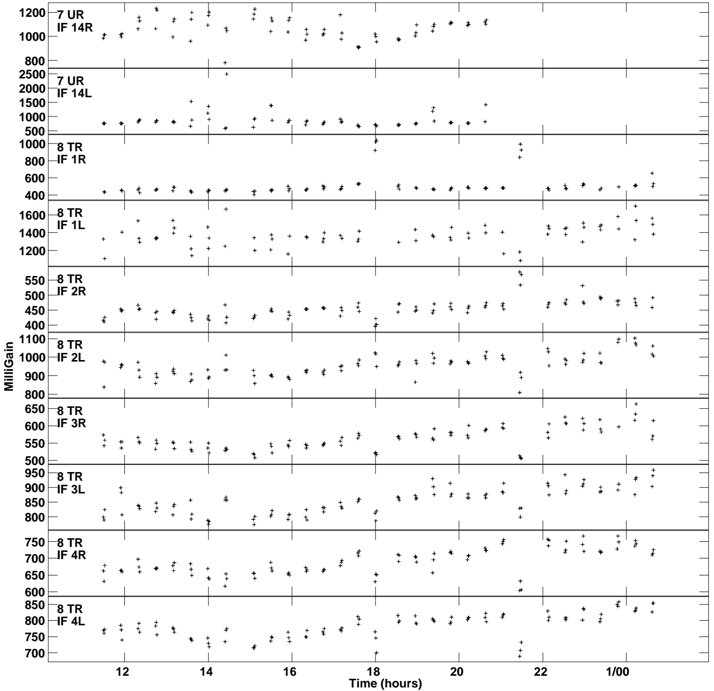
Plot file version 16 created 23-APR-2024 17:58:44 Gain amp vs UTC time for J0518+3306.MULTI.1 SN 1 Rpol & Lpol IF 1 - 16
