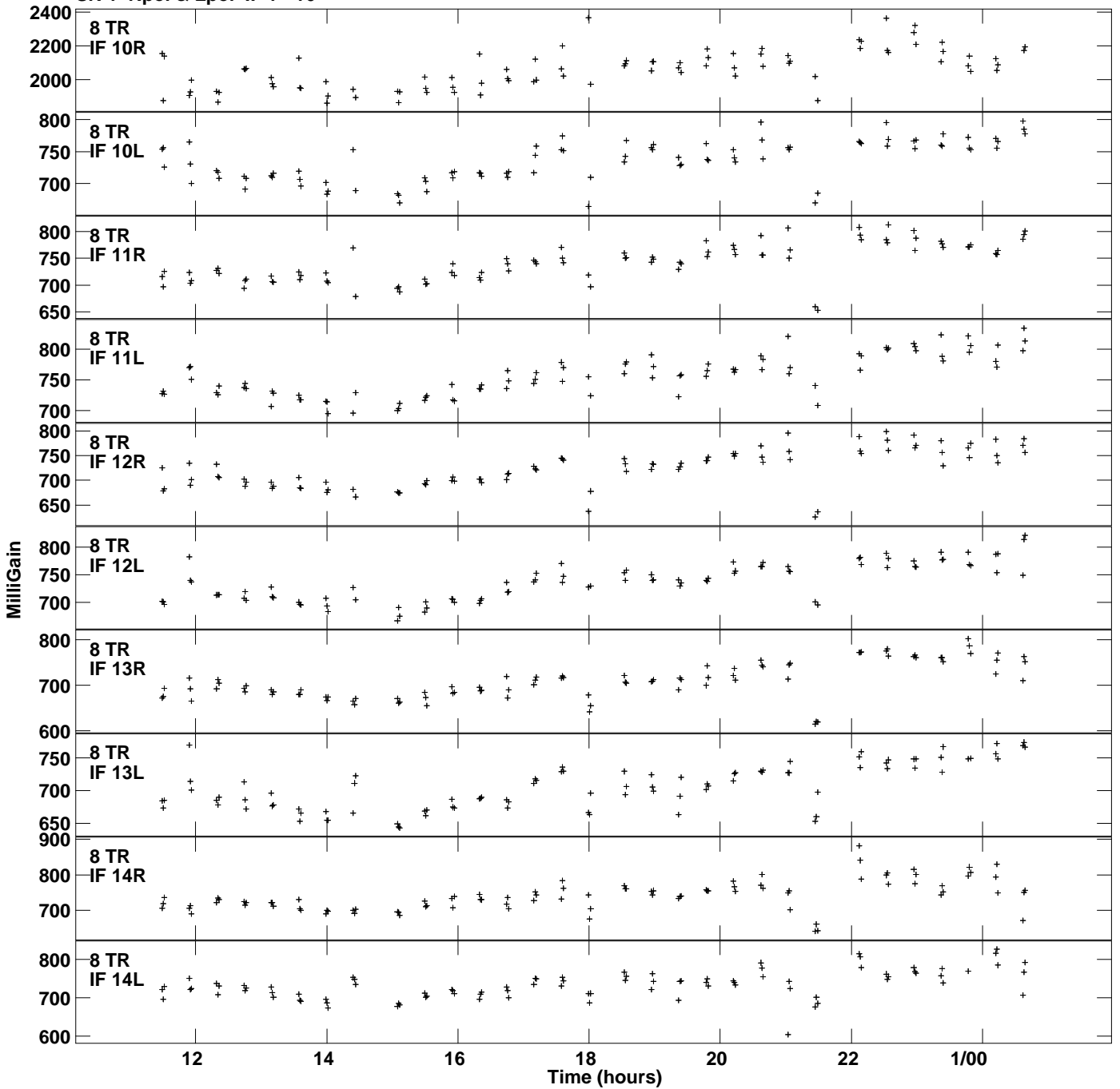
Plot file version 18 created 23-APR-2024 17:58:44 Gain amp vs UTC time for J0518+3306.MULTI.1 SN 1 Rpol & Lpol IF 1 - 16
