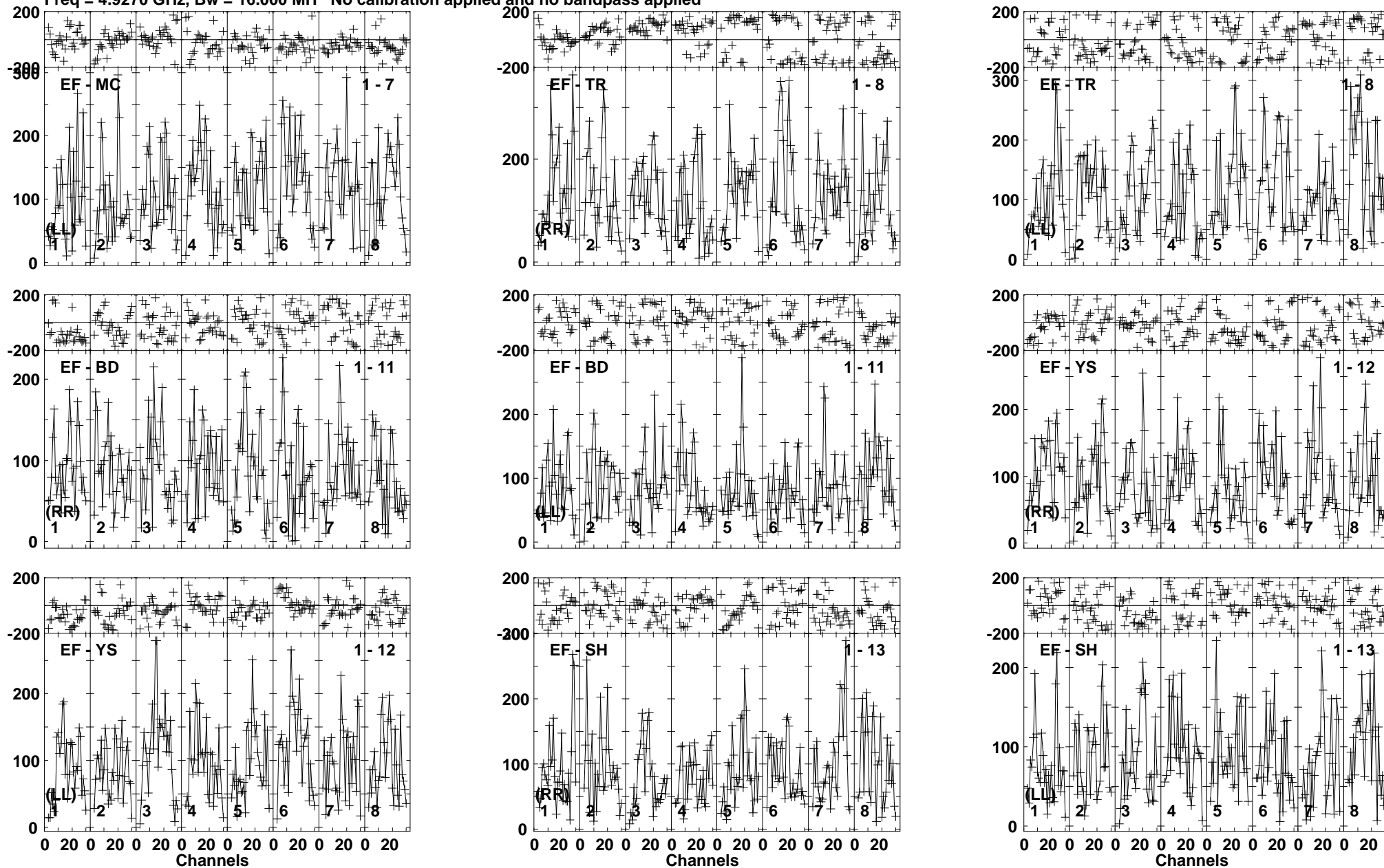
Lower frame: Micro Ampl Jy Top frame: Phas deg Vector averaged cross-power spectrum Baseline: EF (01) - MC (07) Timerange: 00/01:46:05 to 00/01:48:59
