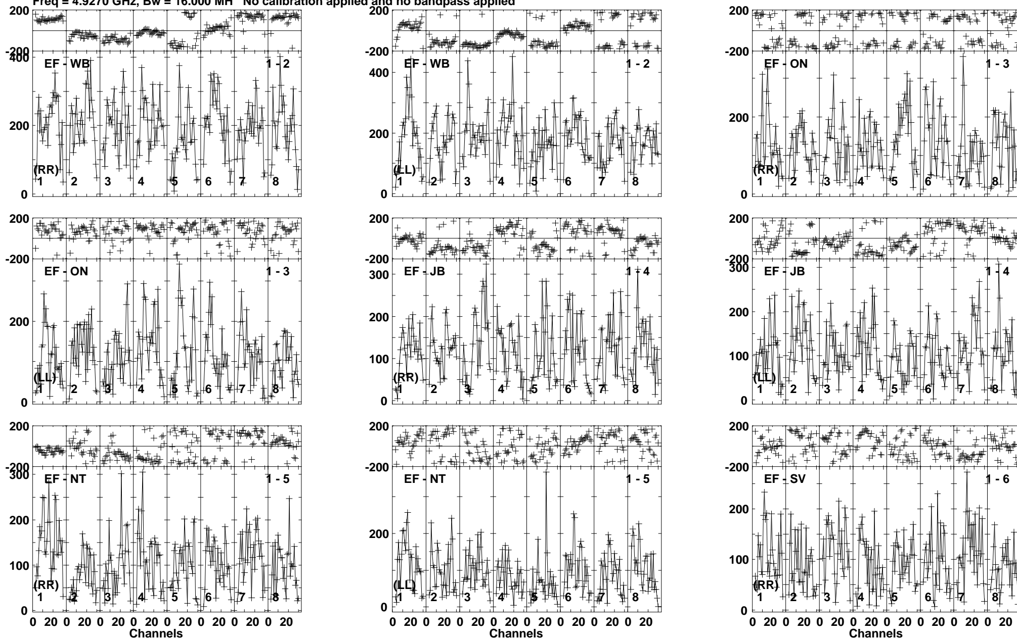
Lower frame: Micro Ampl Jy Top frame: Phas deg Vector averaged cross-power spectrum Baseline: EF (01) - WB (02) Timerange: 00/04:00:35 to 00/04:03:29
