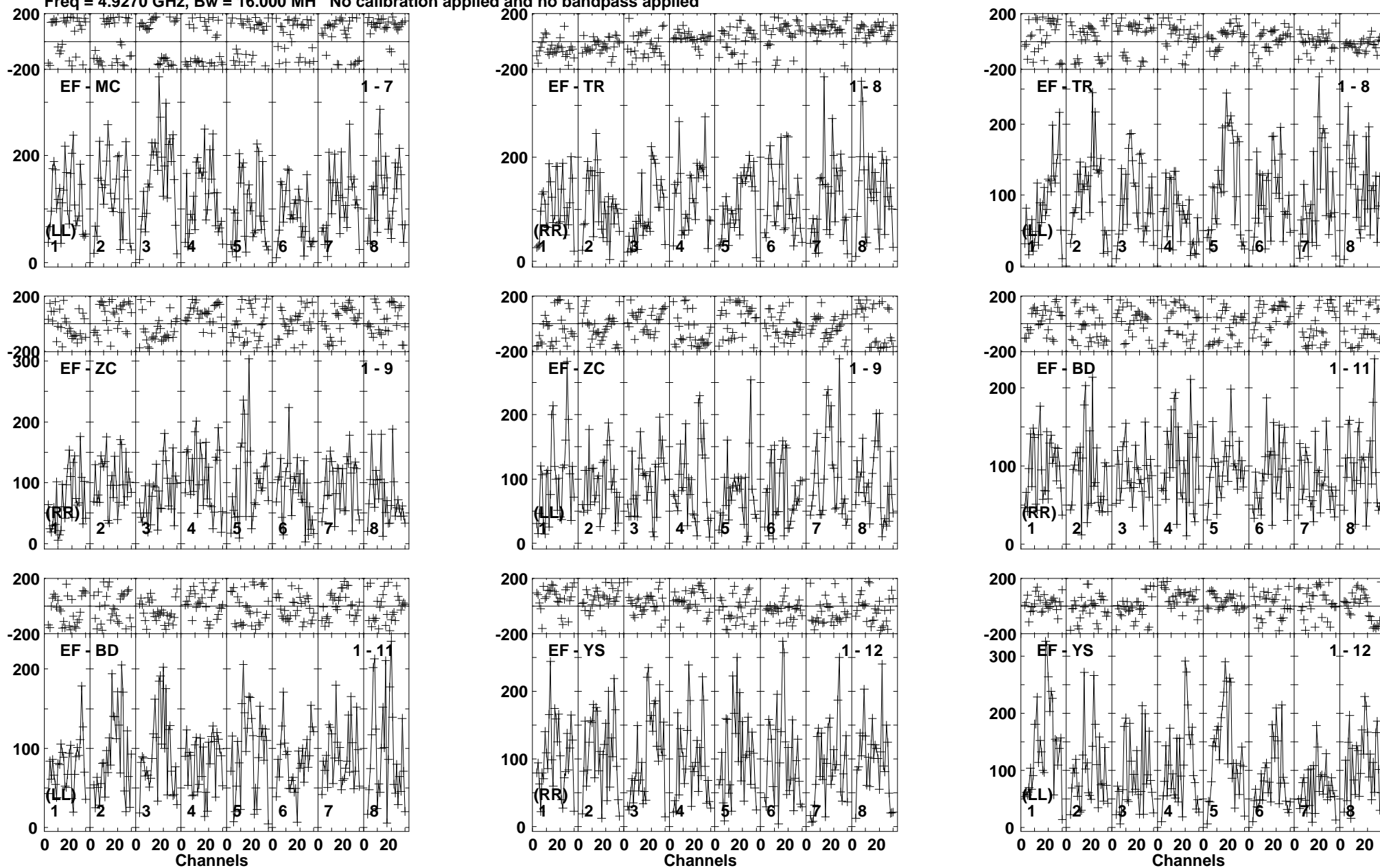
Lower frame: Micro Ampl Jy Top frame: Phas deg Vector averaged cross-power spectrum Baseline: EF (01) - MC (07) Timerange: 00/02:07:05 to 00/02:09:59
