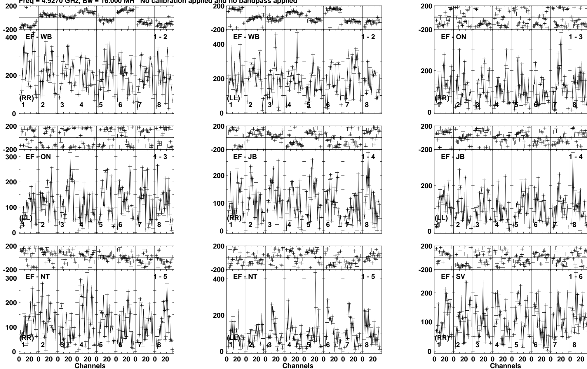
Lower frame: Micro Ampl Jy Top frame: Phas deg Vector averaged cross-power spectrum Baseline: EF (01) - WB (02) Timerange: 00/04:21:35 to 00/04:24:29
