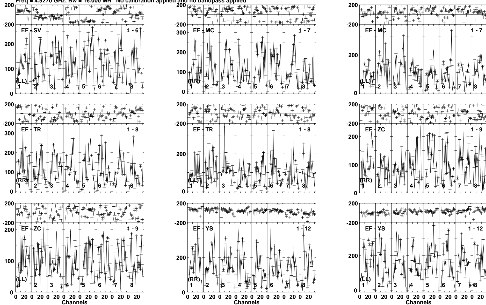
Lower frame: Micro Ampl Jy Top frame: Phas deg Vector averaged cross-power spectrum Baseline: EF (01) - SV (06) Timerange: 00/05:53:05 to 00/05:55:59
