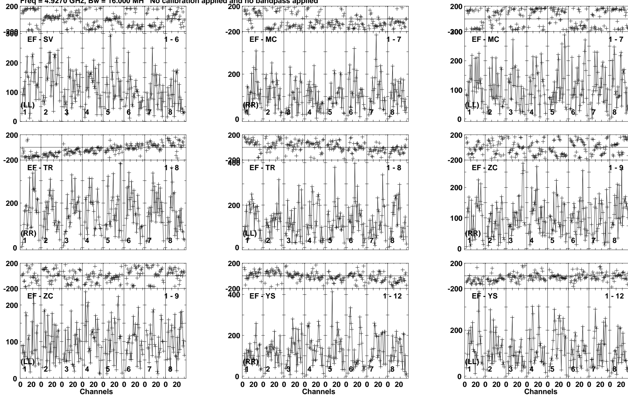
Lower frame: Micro Ampl Jy Top frame: Phas deg Vector averaged cross-power spectrum Baseline: EF (01) - SV (06) Timerange: 00/06:24:35 to 00/06:27:29
