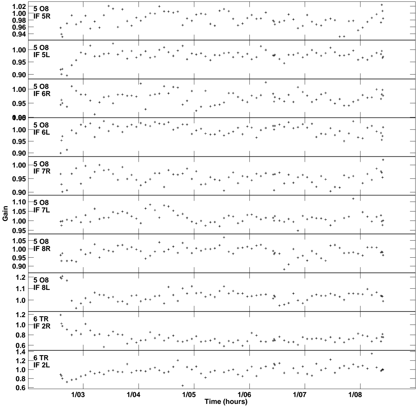
Plot file version 7 created 18-JAN-2016 17:52:54 Gain amp vs UTC time for J1544+3240.MULTI.1 SN 2 Rpol & Lpol IF 1 - 8
