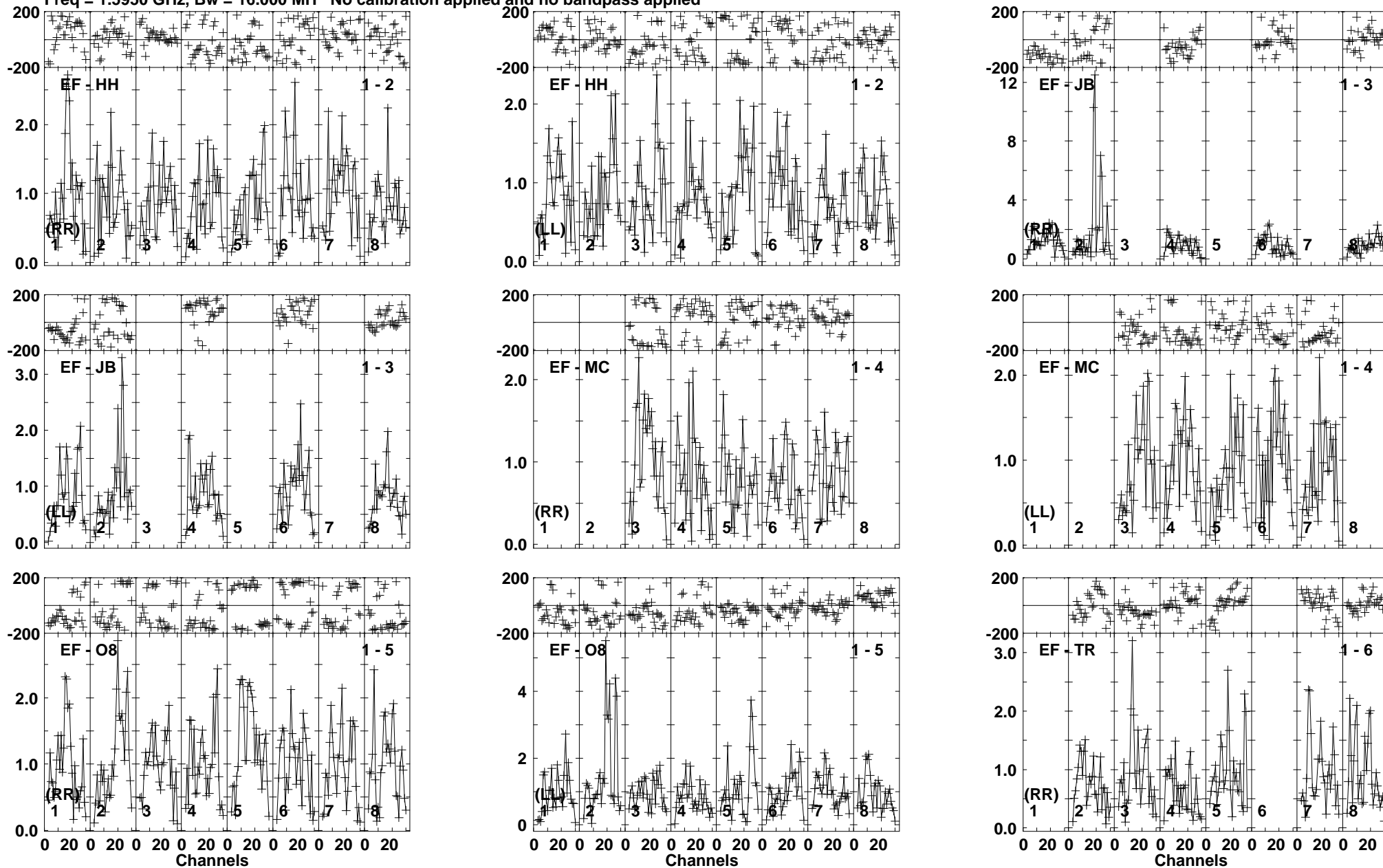
Lower frame: Milli Ampl Jy Top frame: Phas deg Vector averaged cross-power spectrum Baseline: EF (01) - HH (02) Timerange: 00/21:14:56 to 00/21:14:58
