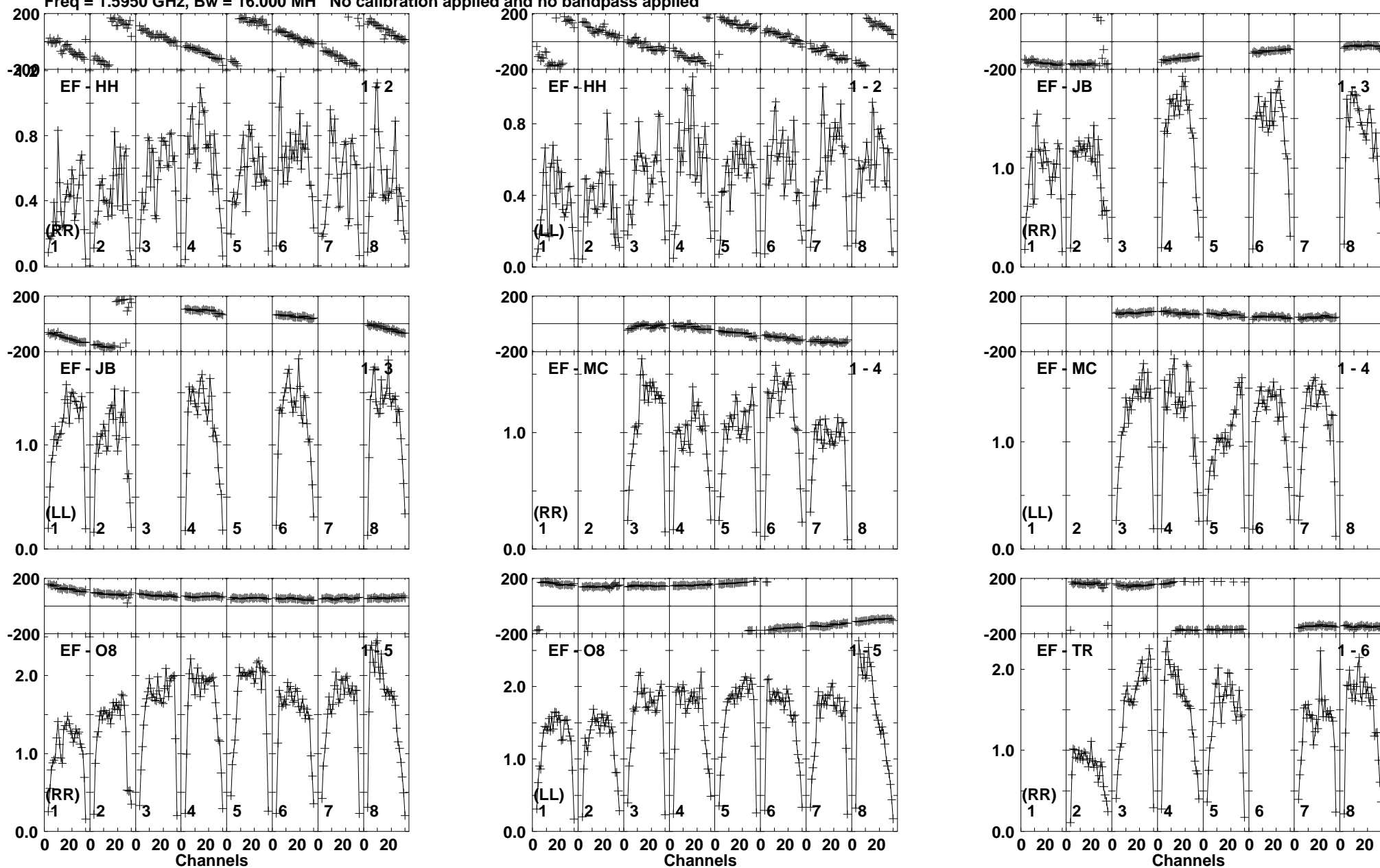
Lower frame: Milli Amply Jy Top frame: Phas deg Vector averaged cross-power spectrum Baseline: EF (01) - HH (02) Timerange: 01/02:51:31 to 01/02:52:59
