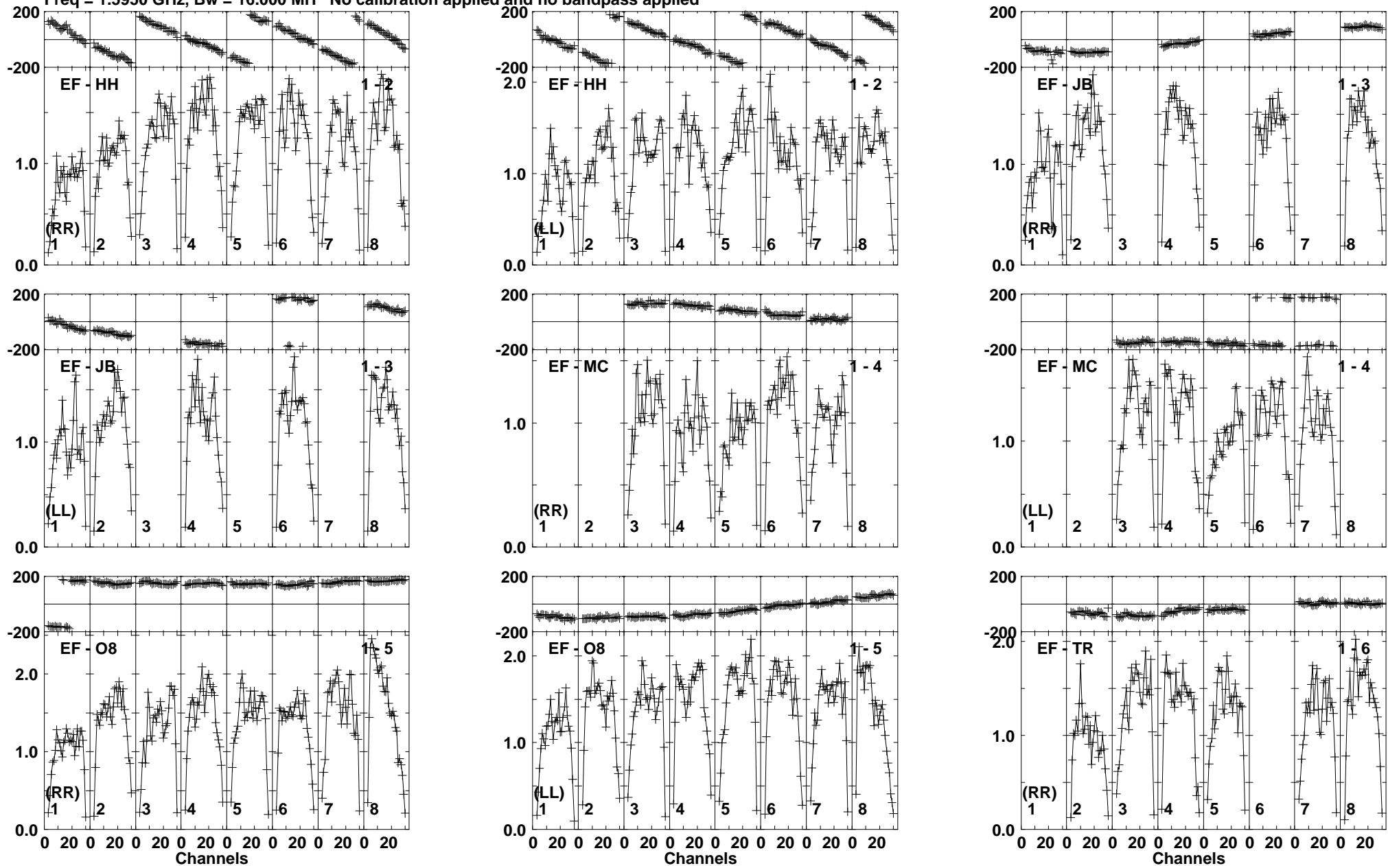
Lower frame: Milli Ampl Jy Top frame: Phas deg Vector averaged cross-power spectrum Baseline: EF (01) - HH (02) Timerange: 01/00:08:31 to 01/00:09:49
