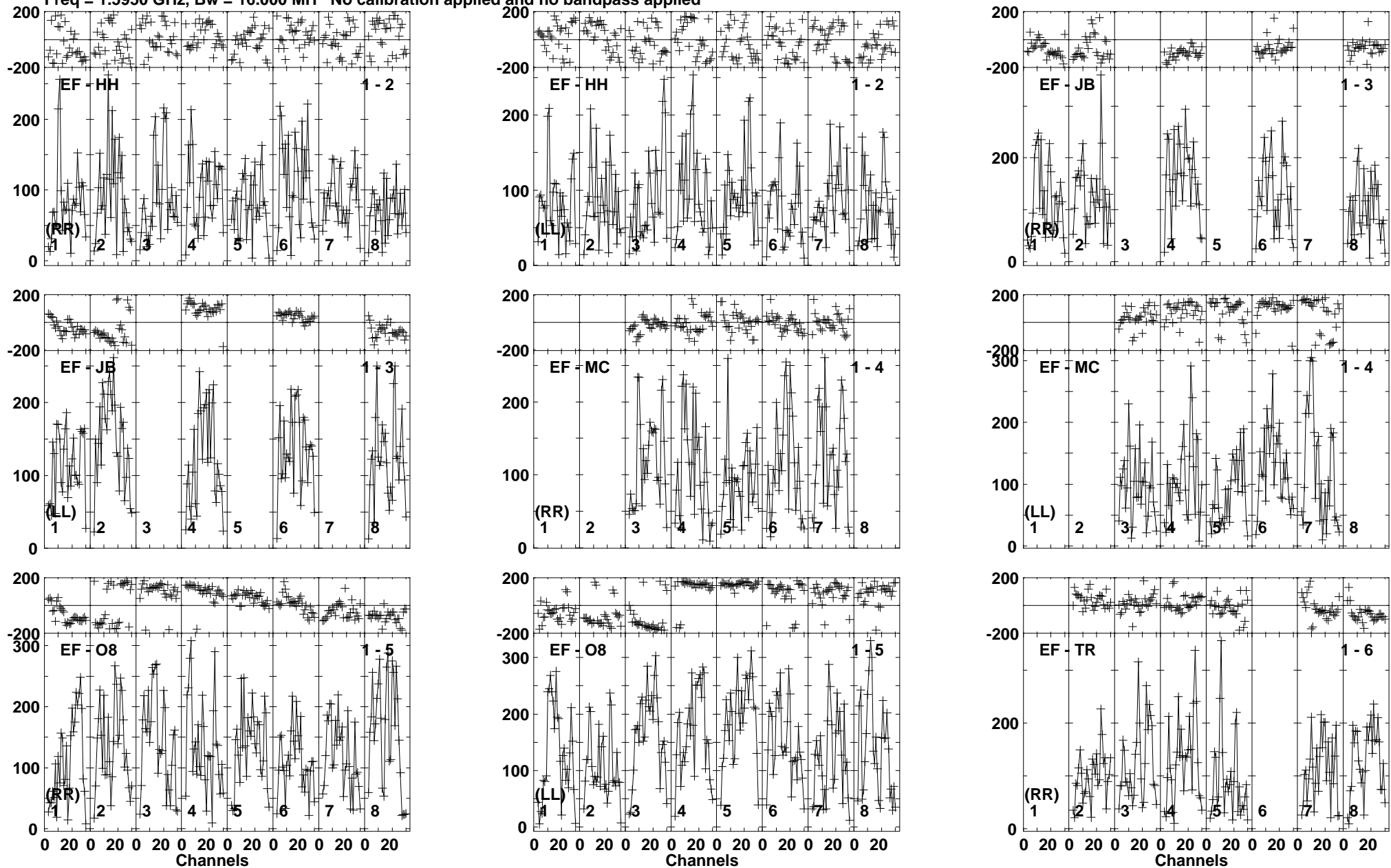
Lower frame: Micro Ampl Jy Top frame: Phas deg Vector averaged cross-power spectrum Baseline: EF (01) - HH (02) Timerange: 01/03:33:01 to 01/03:36:29
