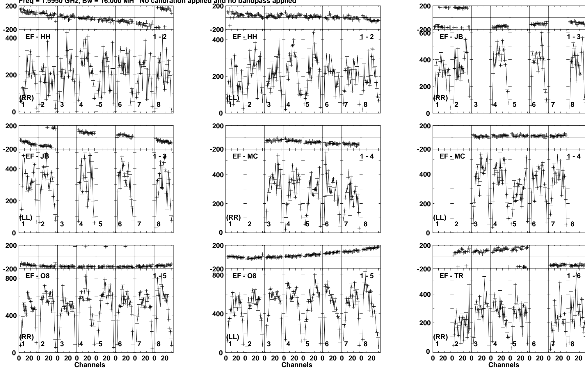
Lower frame: Micro Ampl Jy Top frame: Phas deg Vector averaged cross-power spectrum Baseline: EF (01) - HH (02) Timerange: 01/01:35:01 to 01/01:38:29
