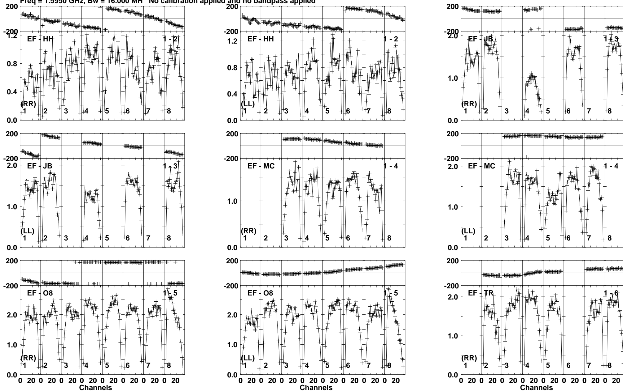
Lower frame: Milli Ampl Jy Top frame: Phas deg Vector averaged cross-power spectrum Baseline: EF (01) - HH (02) Timerange: 01/07:47:11 to 01/07:47:59
