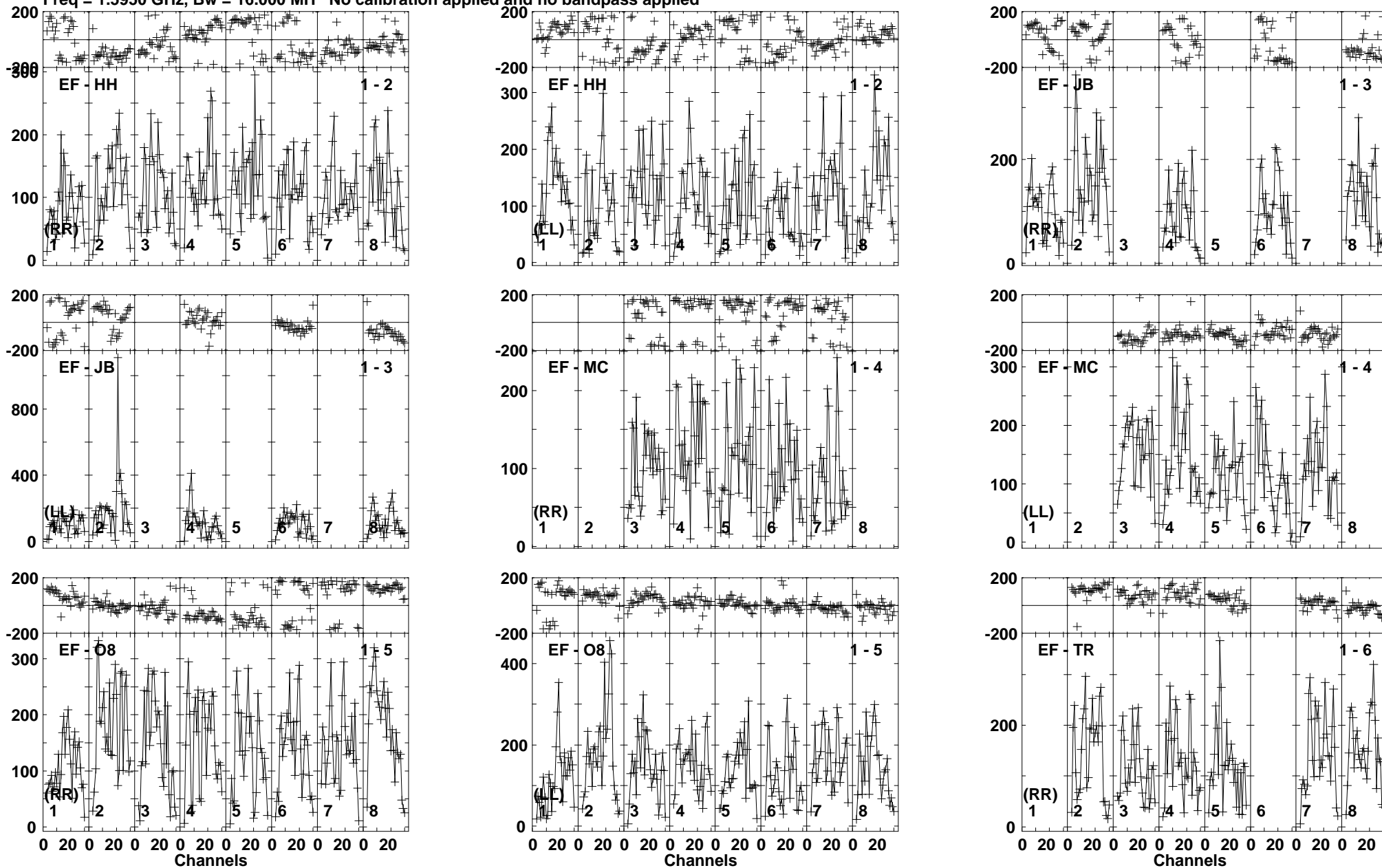
Lower frame: Micro Ampl Jy Top frame: Phas deg Vector averaged cross-power spectrum Baseline: EF (01) - HH (02) Timerange: 01/06:38:01 to 01/06:41:29
