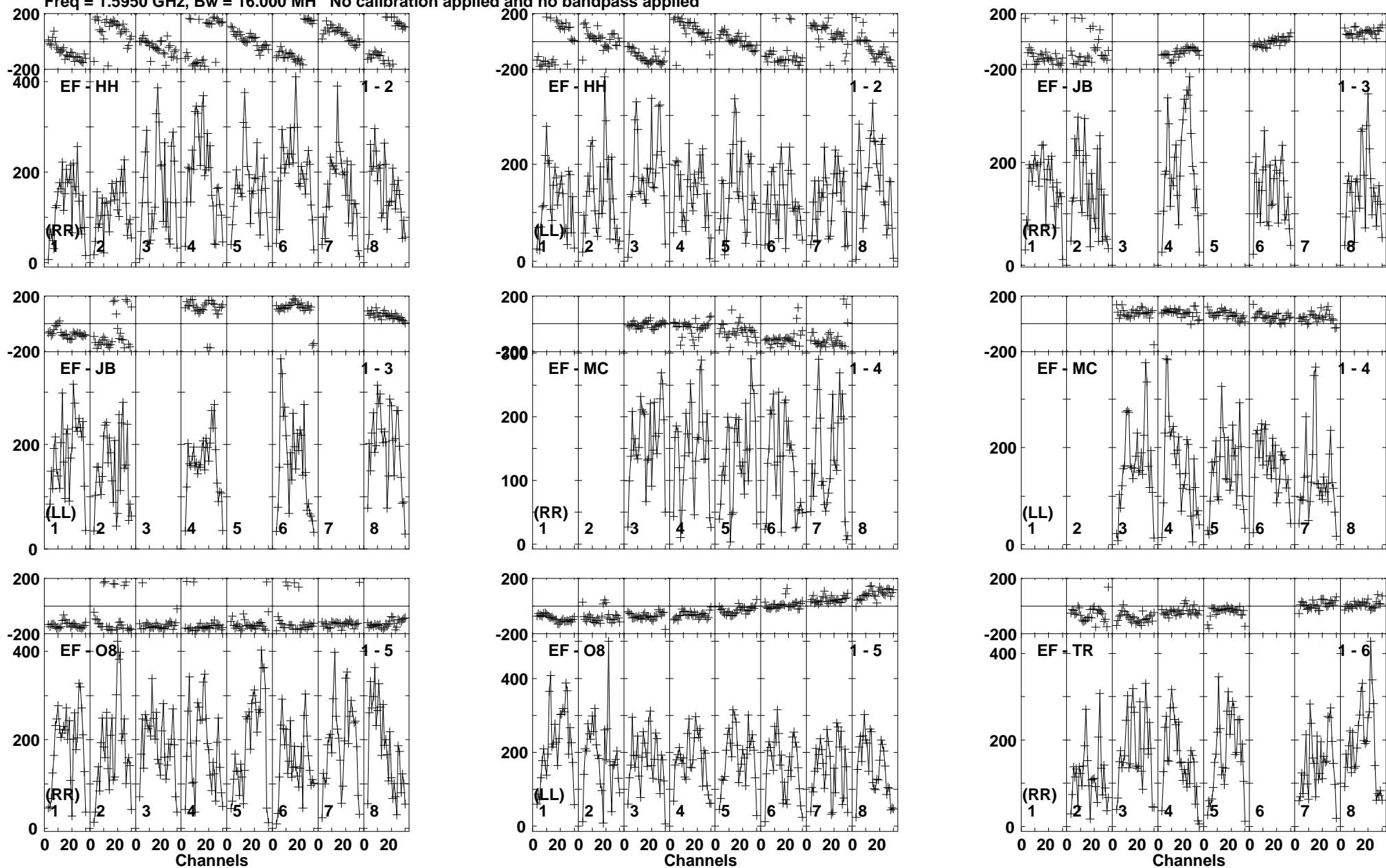
Lower frame: Micro Ampl Jy Top frame: Phas deg Vector averaged cross-power spectrum Baseline: EF (01) - HH (02) Timerange: 00/21:20:01 to 00/21:23:25
