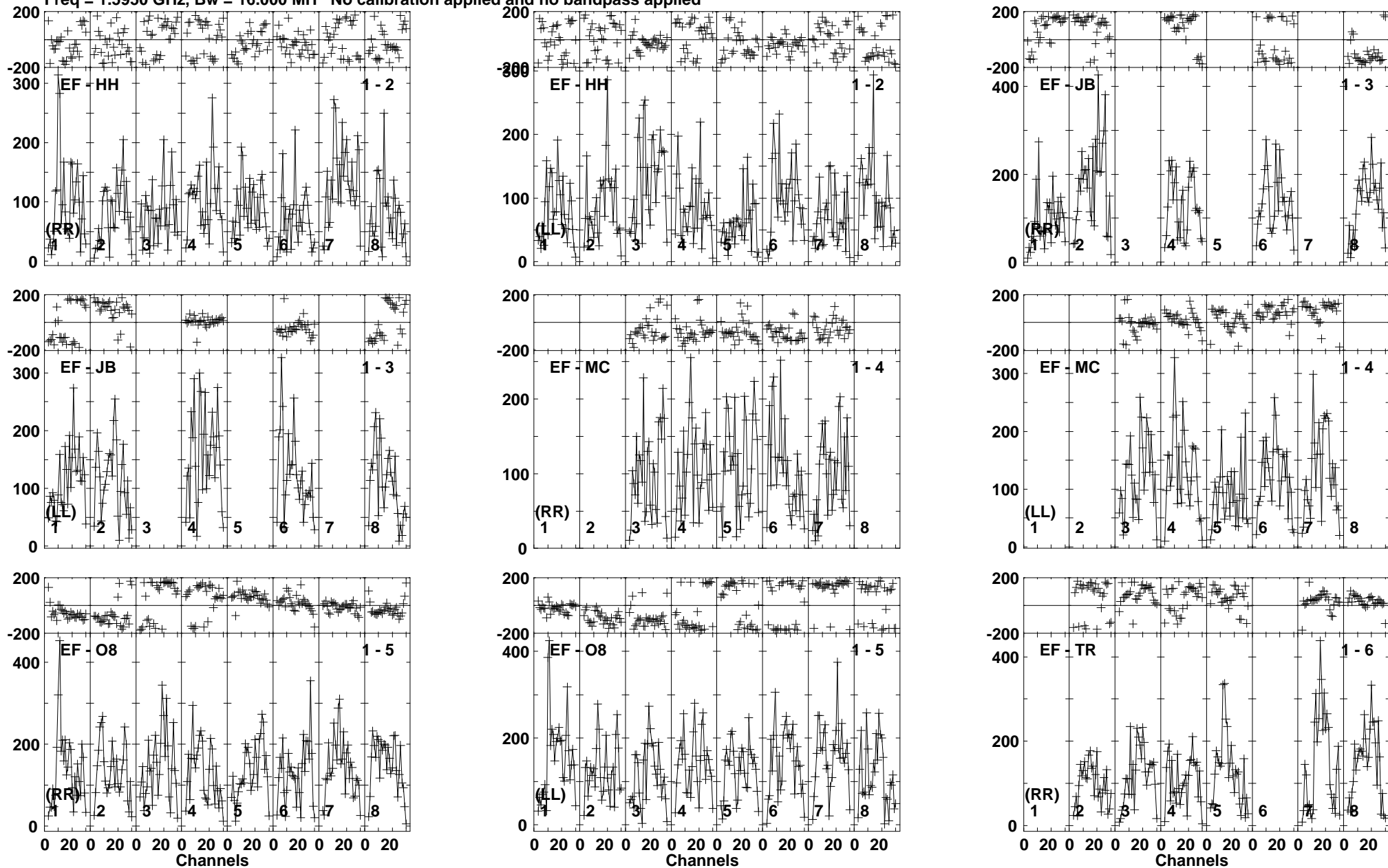
Lower frame: Micro Ampl Jy Top frame: Phas deg Vector averaged cross-power spectrum Baseline: EF (01) - HH (02) Timerange: 01/04:08:01 to 01/04:11:29
