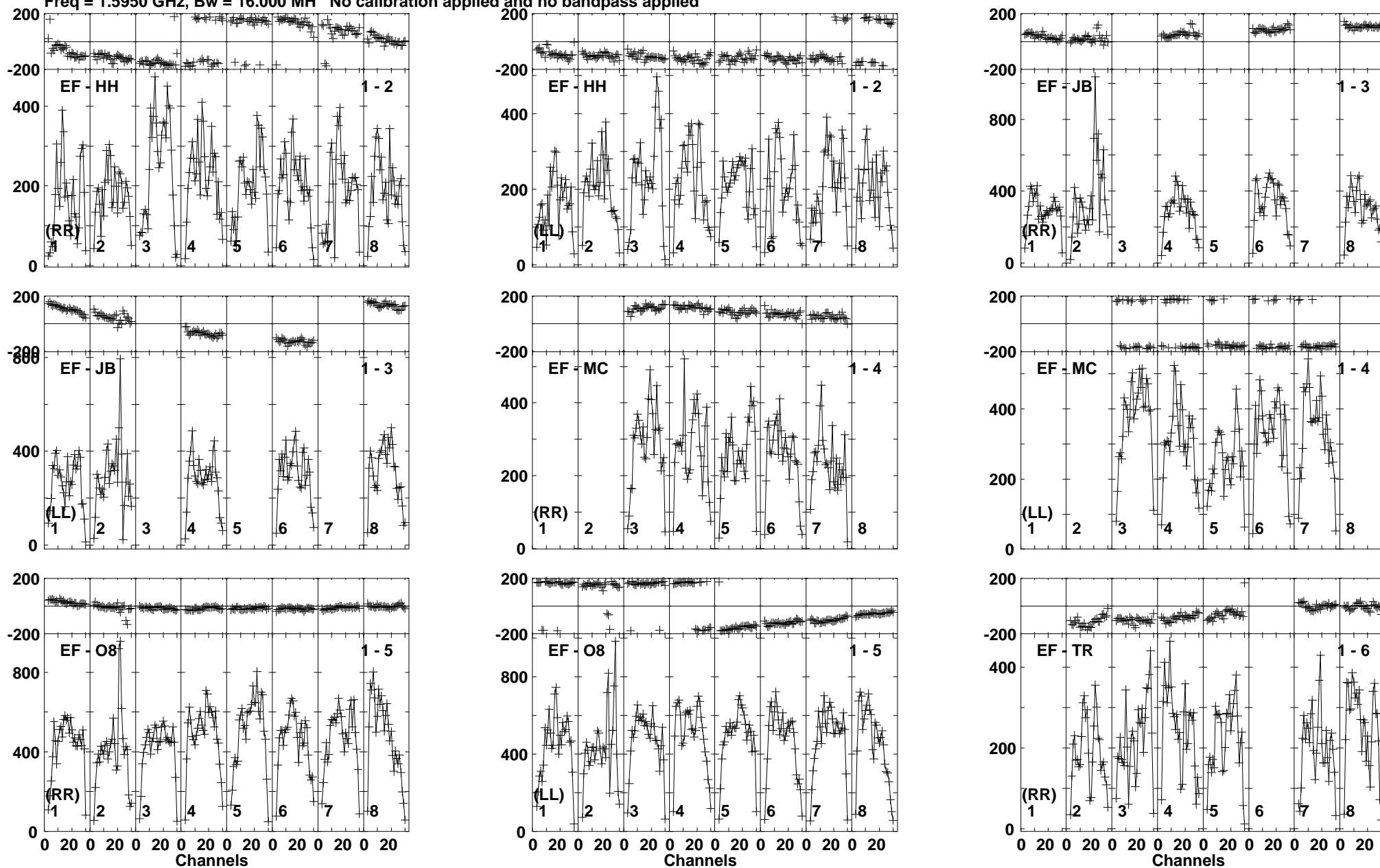
Lower frame: Micro Ampl Jy Top frame: Phas deg Vector averaged cross-power spectrum Baseline: EF (01) - HH (02) Timerange: 01/02:15:01 to 01/02:18:29
