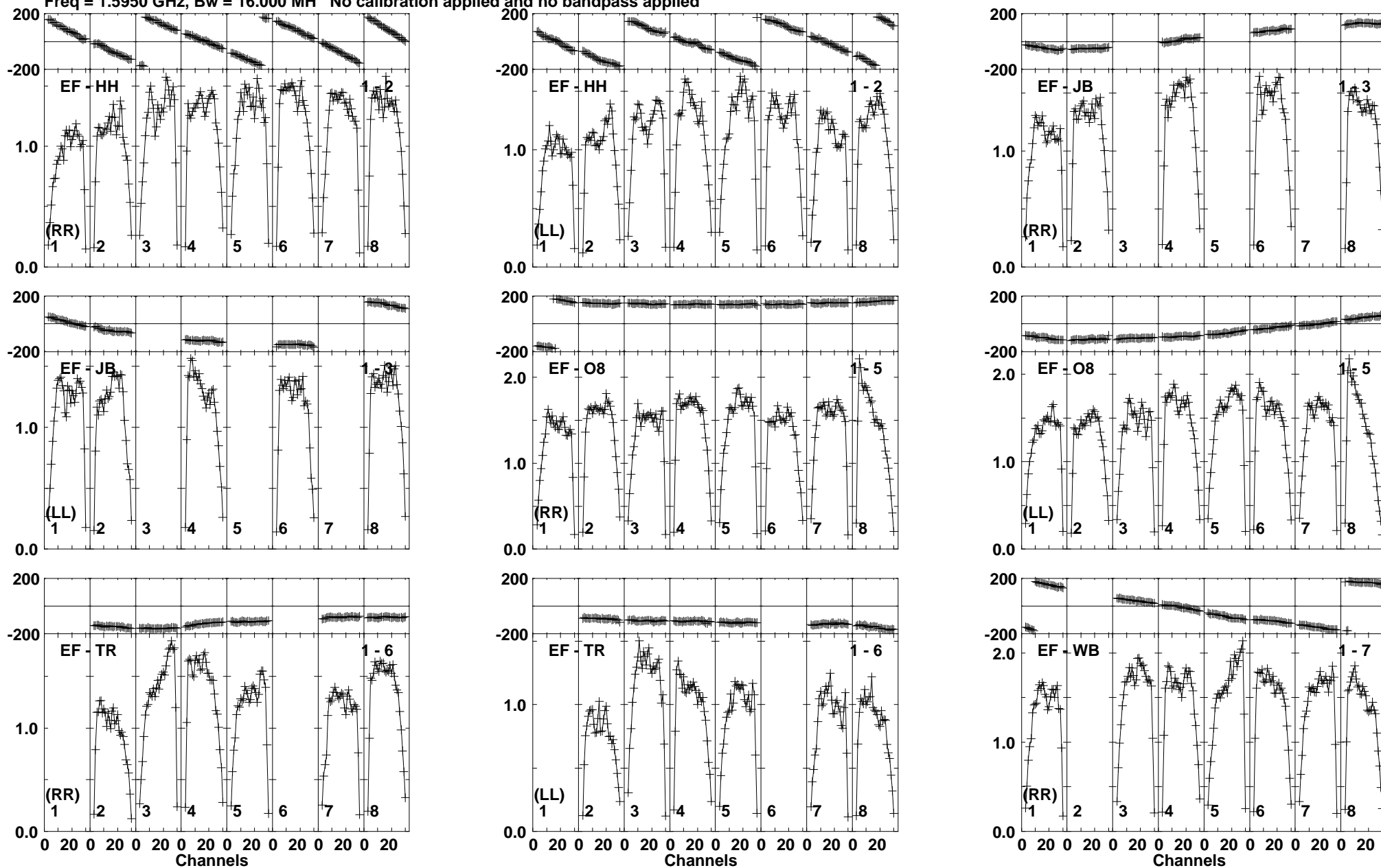
Lower frame: Milli Ampl Jy Top frame: Phas deg Vector averaged cross-power spectrum Baseline: EF (01) - HH (02) Timerange: 00/23:32:01 to 00/23:34:59
