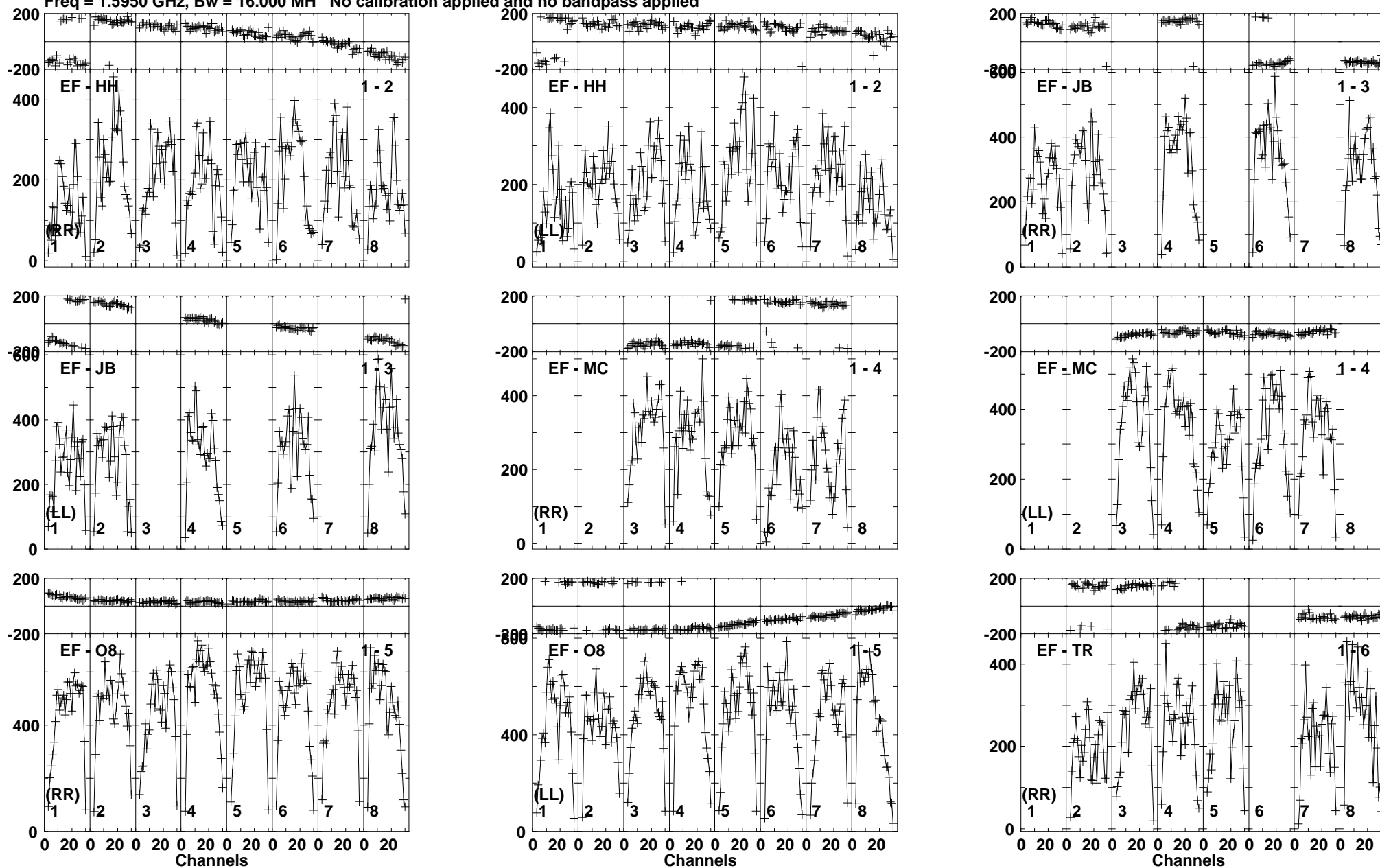
Lower frame: Micro Ampl Jy Top frame: Phas deg Vector averaged cross-power spectrum Baseline: EF (01) - HH (02) Timerange: 01/01:15:01 to 01/01:18:29
