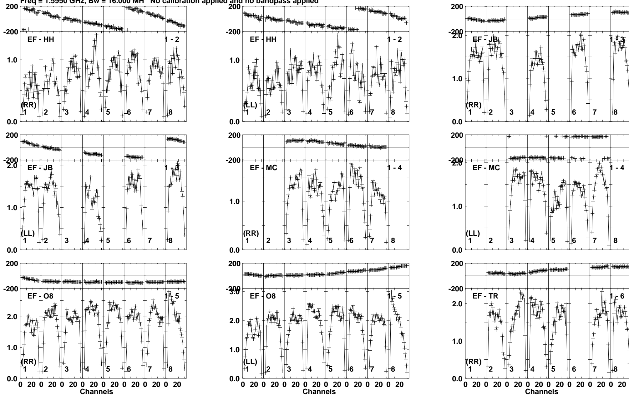
Lower frame: Milli Ampl Jy Top frame: Phas deg Vector averaged cross-power spectrum Baseline: EF (01) - HH (02) Timerange: 01/06:41:31 to 01/06:42:59
