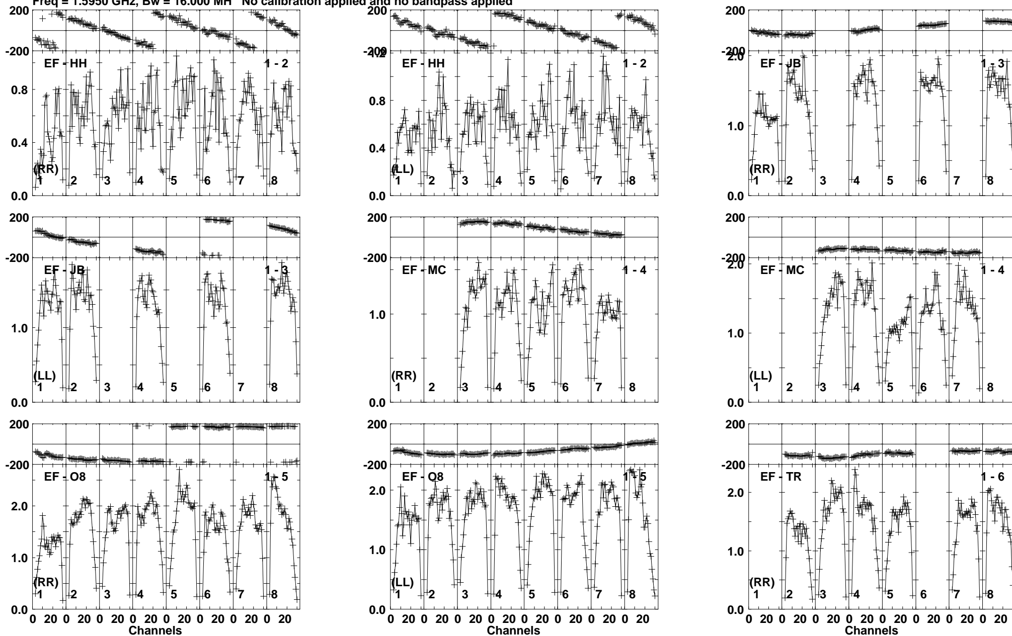
Lower frame: Milli Ampl Jy Top frame: Phas deg Vector averaged cross-power spectrum Baseline: EF (01) - HH (02) Timerange: 01/03:37:11 to 01/03:37:59
