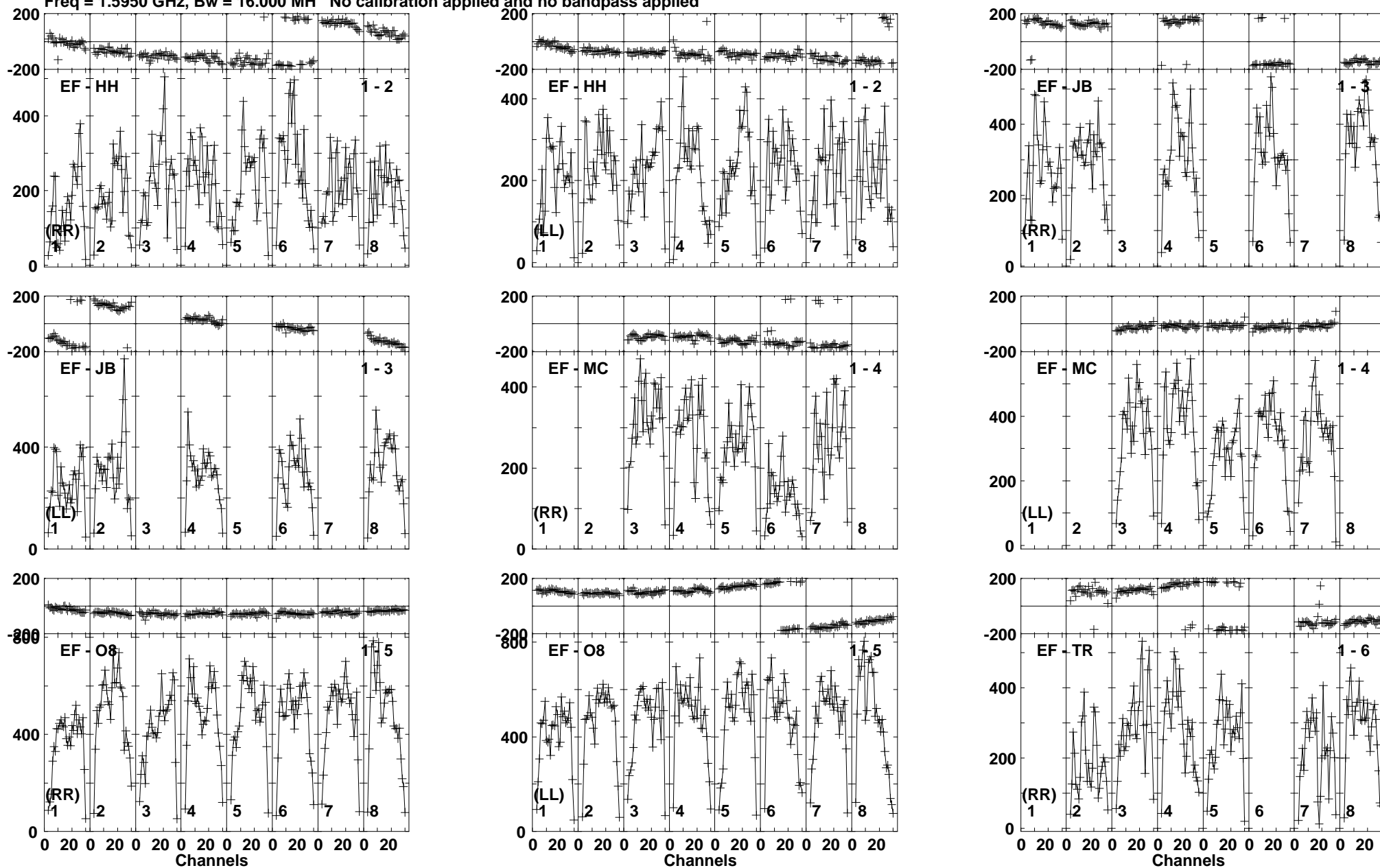
Lower frame: Micro Ampl Jy Top frame: Phas deg Vector averaged cross-power spectrum Baseline: EF (01) - HH (02) Timerange: 01/01:25:01 to 01/01:28:29
