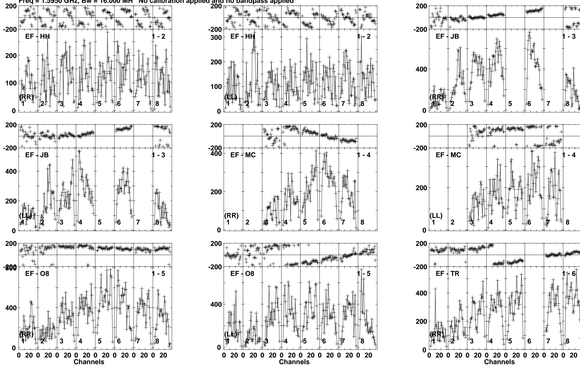
Lower frame: Micro Ampl Jy Top frame: Phas deg Vector averaged cross-power spectrum Baseline: EF (01) - HH (02) Timerange: 01/11:38:01 to 01/11:41:29
