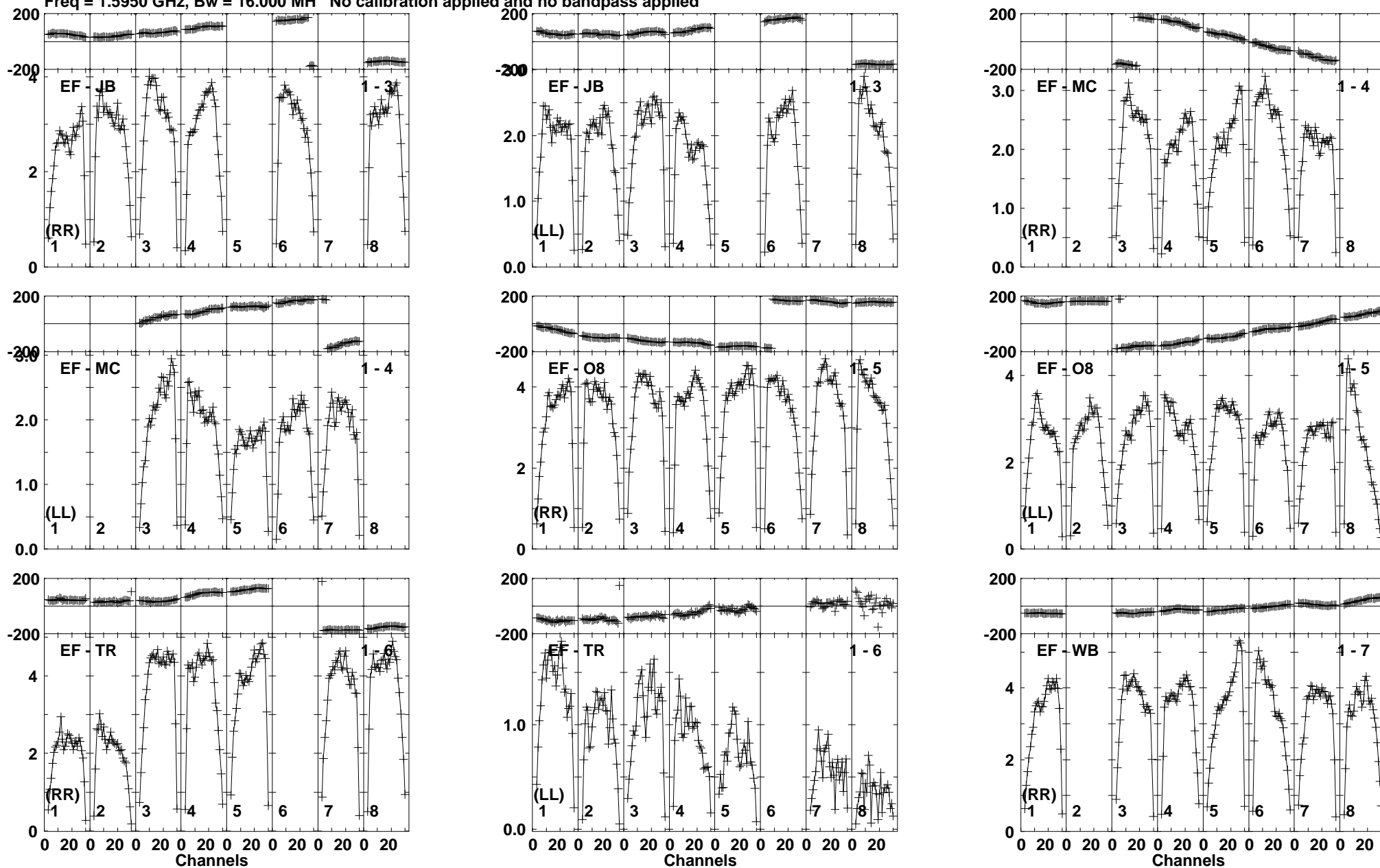
Lower frame: Milli Ampl Jy Top frame: Phas deg Vector averaged cross-power spectrum Baseline: EF (01) - JB (03) Timerange: 01/03:32:51 to 01/03:33:39
