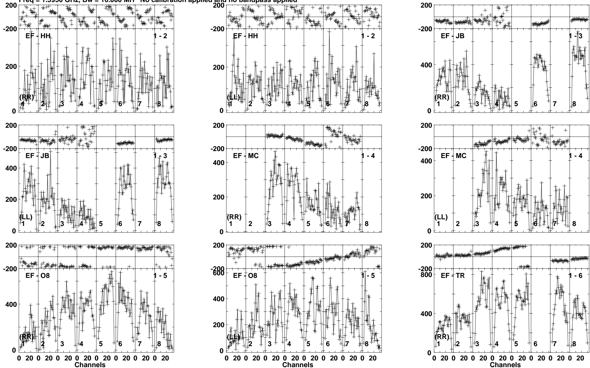
Lower frame: Micro Ampl Jy Top frame: Phas deg Vector averaged cross-power spectrum Baseline: EF (01) - HH (02) Timerange: 01/11:08:01 to 01/11:11:29
