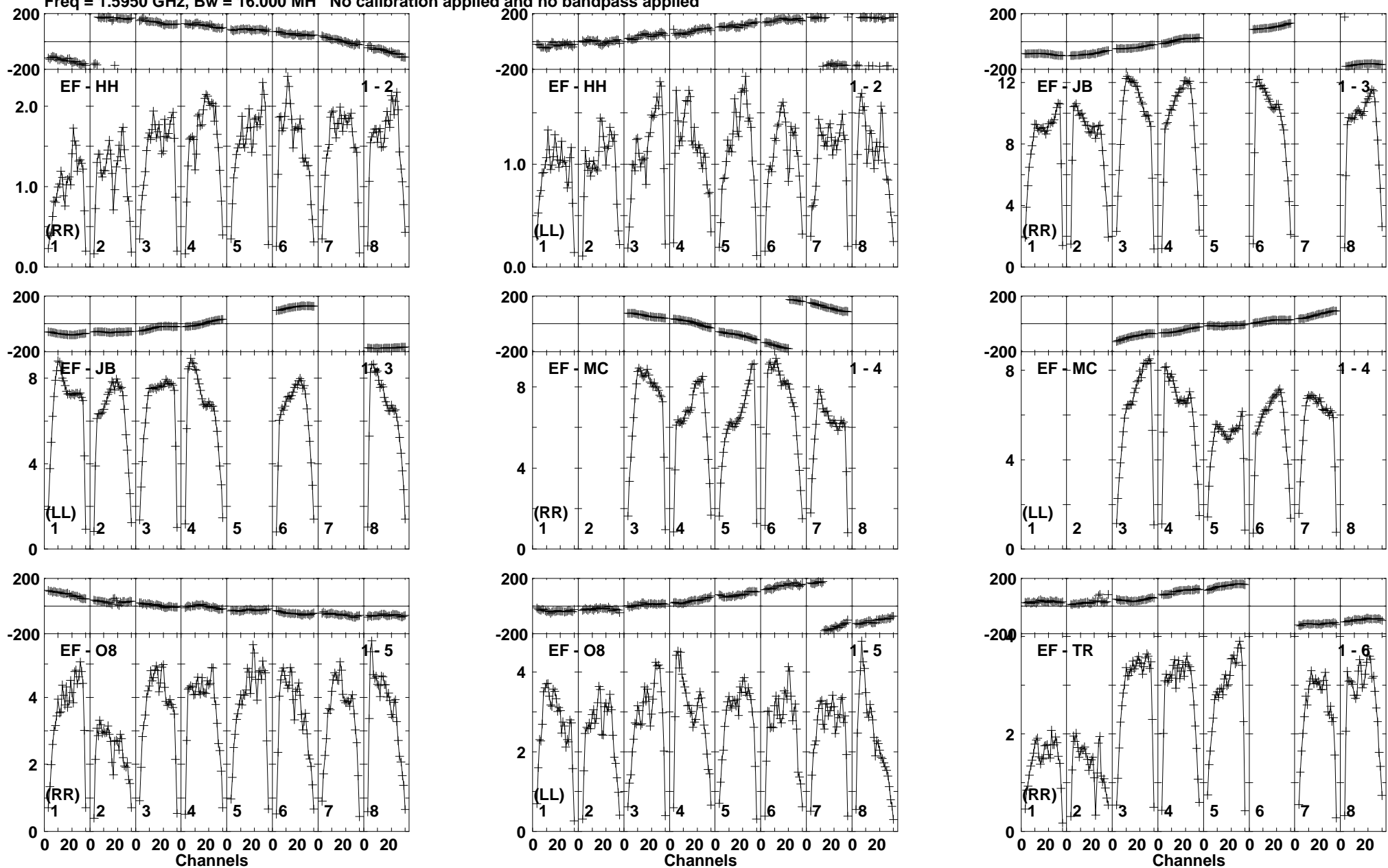
Lower frame: Milli Ampl Jy Top frame: Phas deg Vector averaged cross-power spectrum Baseline: EF (01) - HH (02) Timerange: 01/11:36:31 to 01/11:37:59
