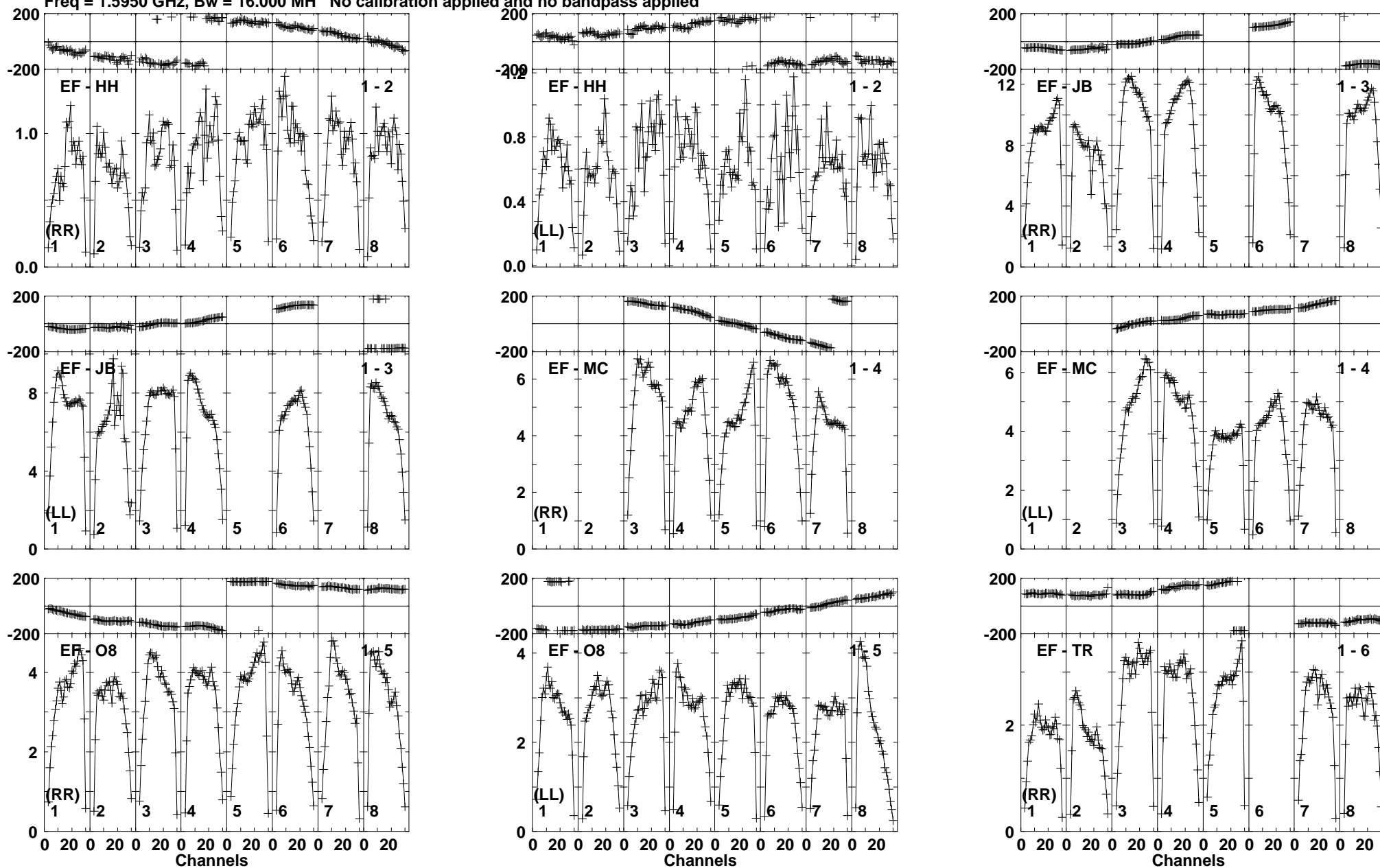
Lower frame: Milli Amp Jy Top frame: Phas deg Vector averaged cross-power spectrum Baseline: EF (01) - HH (02) Timerange: 01/10:26:31 to 01/10:27:59
