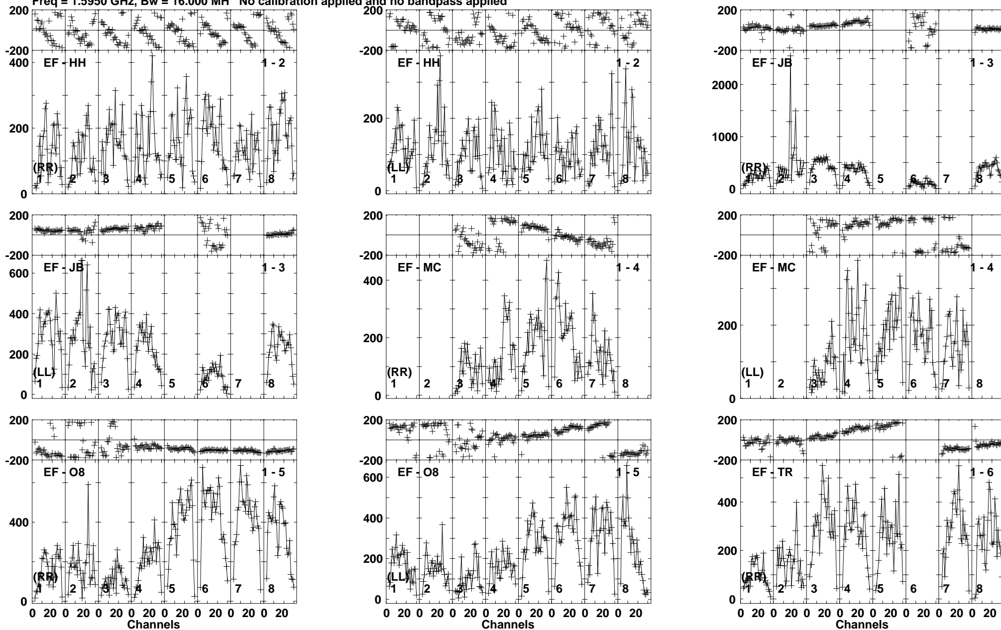
Lower frame: Micro Ampl Jy Top frame: Phas deg Vector averaged cross-power spectrum Baseline: EF (01) - HH (02) Timerange: 01/12:38:01 to 01/12:41:29
