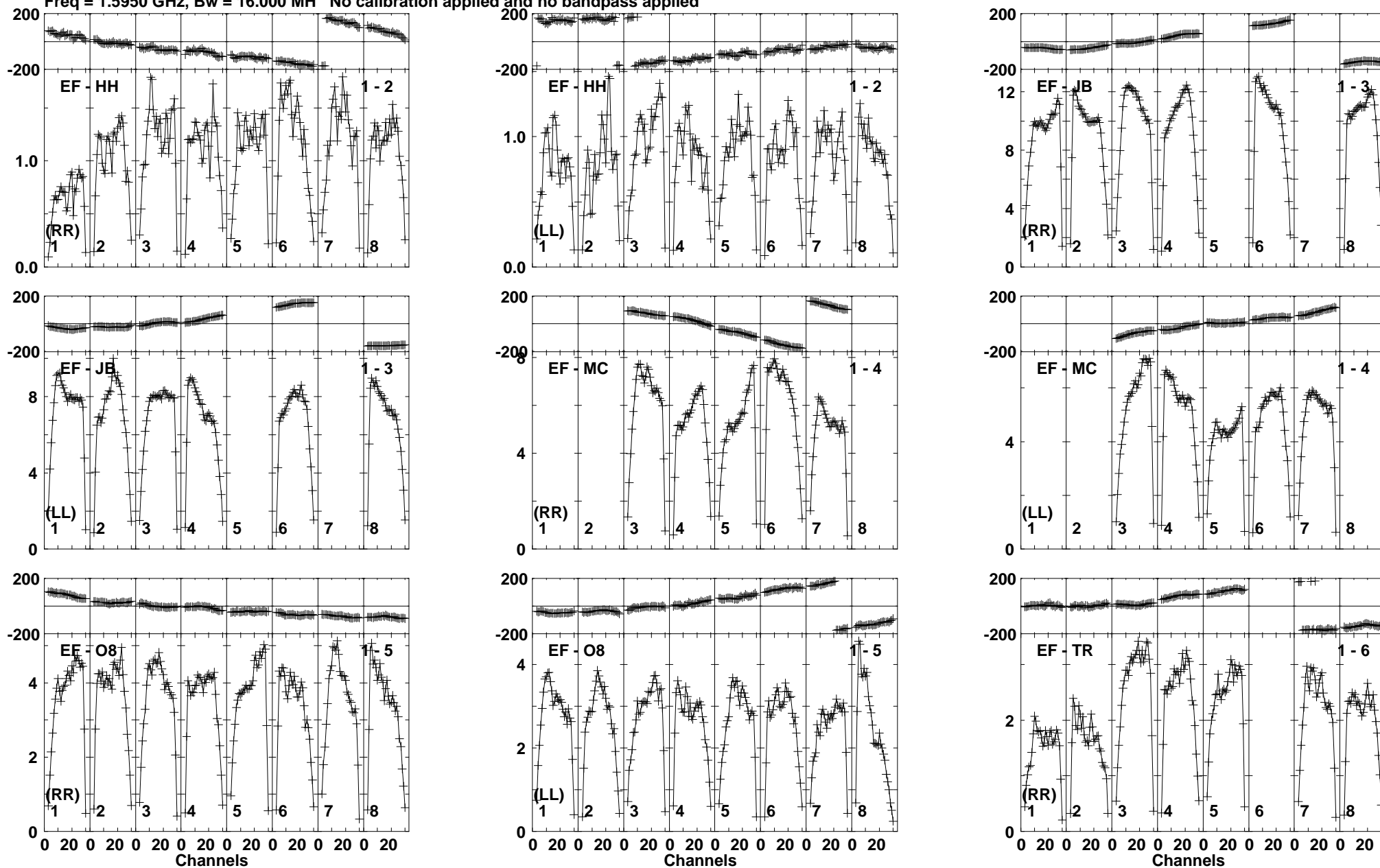
Lower frame: Milli Ampl Jy Top frame: Phas deg Vector averaged cross-power spectrum Baseline: EF (01) - HH (02) Timerange: 01/10:52:11 to 01/10:52:59
