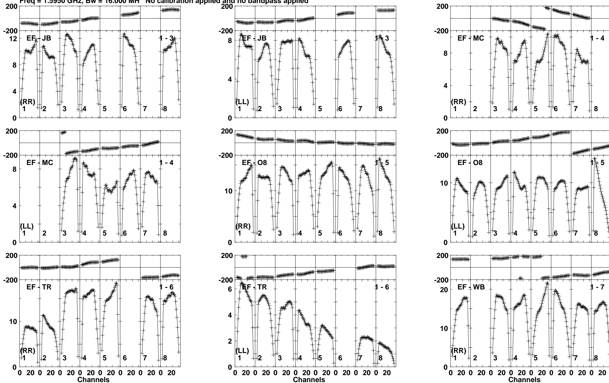
Lower frame: Milli Ampl Jy Top frame: Phas deg Vector averaged cross-power spectrum Baseline: EF (01) - JB (03) Timerange: 01/09:15:41 to 01/09:29:59
