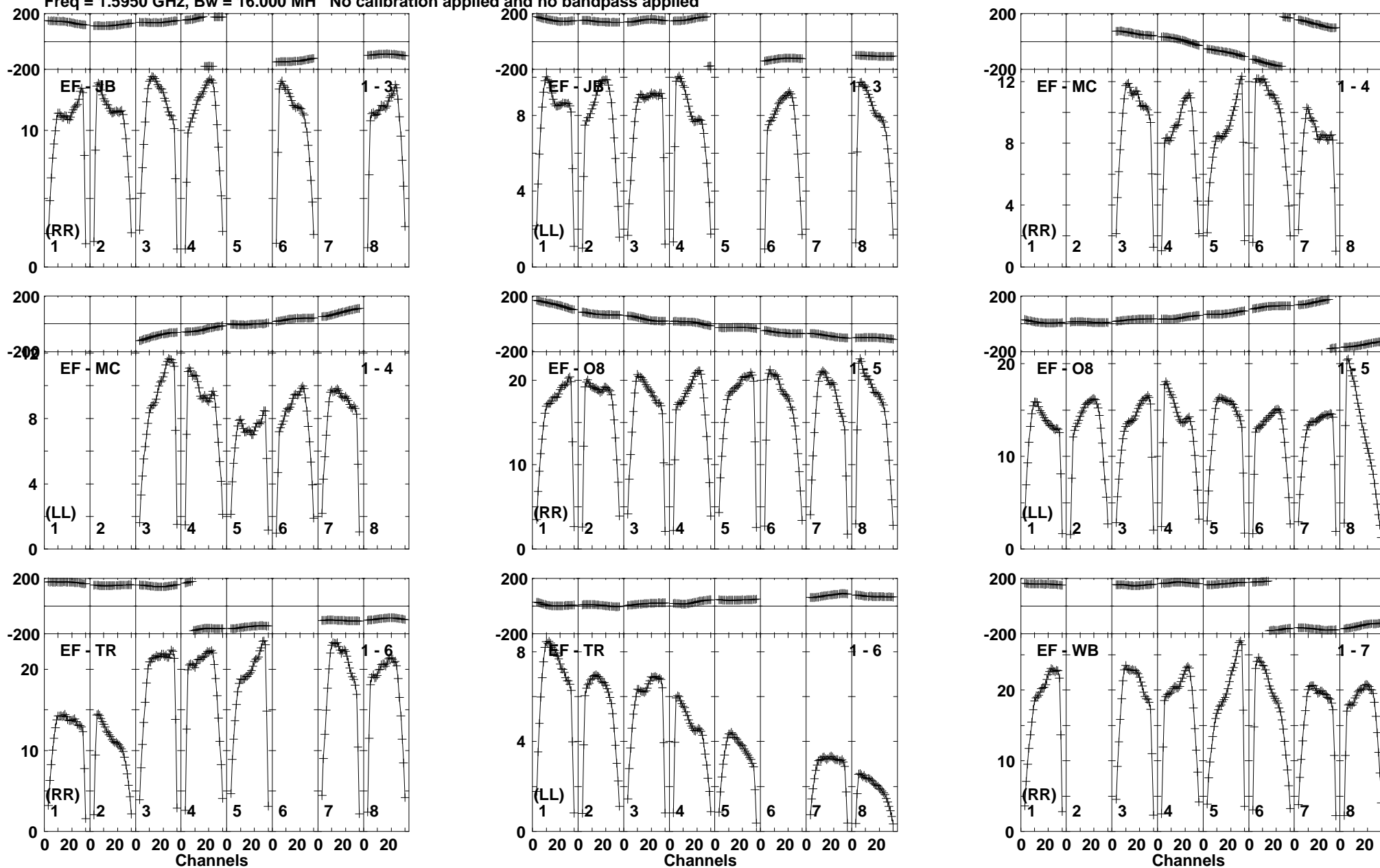
Lower frame: Milli Ampl Jy Top frame: Phas deg Vector averaged cross-power spectrum Baseline: EF (01) - JB (03) Timerange: 01/01:15:41 to 01/01:29:59
