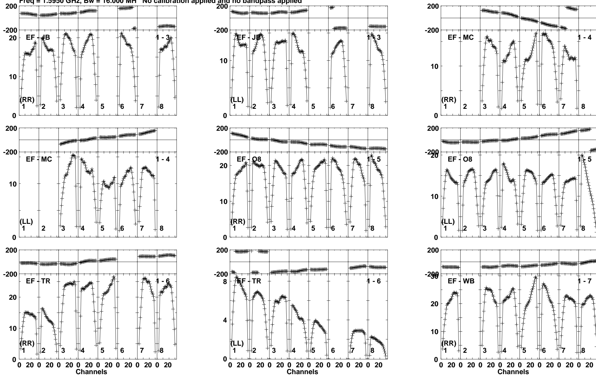
Lower frame: Milli Ampl Jy Top frame: Phas deg Vector averaged cross-power spectrum Baseline: EF (01) - JB (03) Timerange: 01/02:15:41 to 01/02:29:59
