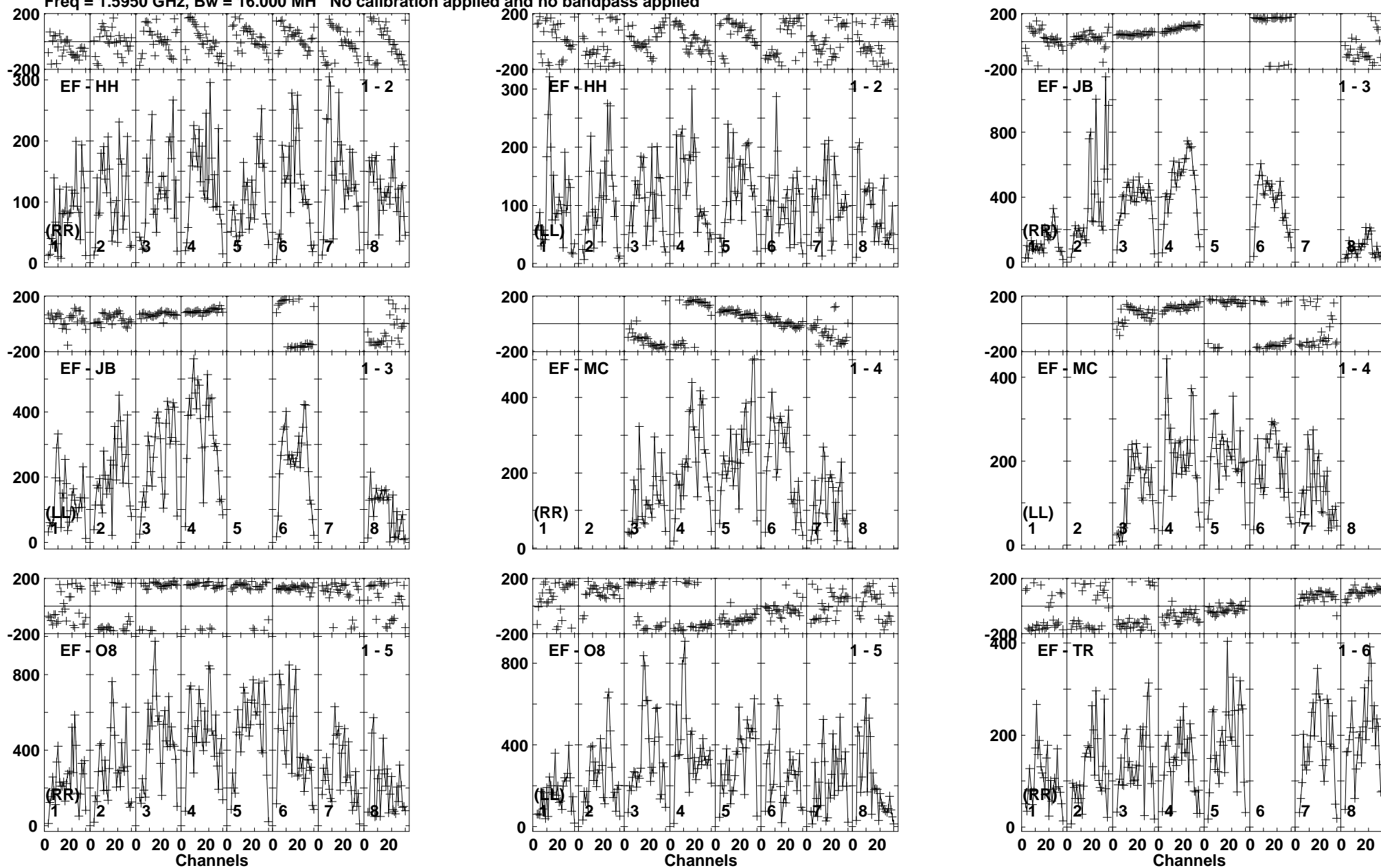
Lower frame: Micro Ampl Jy Top frame: Phas deg Vector averaged cross-power spectrum Baseline: EF (01) - HH (02) Timerange: 01/11:43:01 to 01/11:46:29
