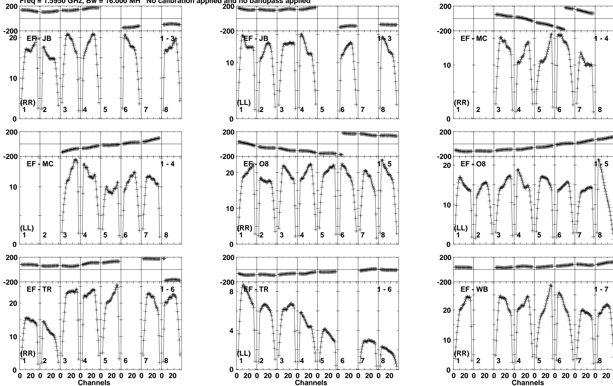
Lower frame: Milli Ampl Jy Top frame: Phas deg Vector averaged cross-power spectrum Baseline: EF (01) - JB (03) Timerange: 01/01:45:41 to 01/01:59:59
