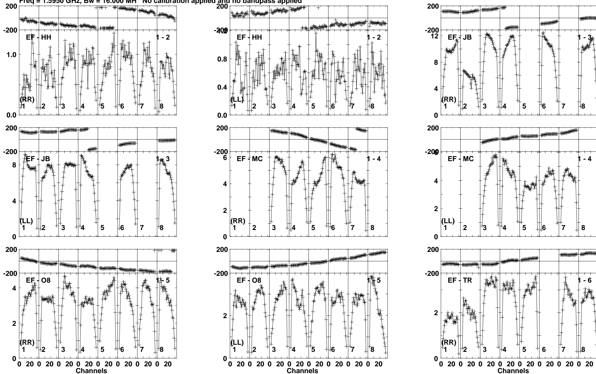
Lower frame: Milli Ampl Jy Top frame: Phas deg Vector averaged cross-power spectrum Baseline: EF (01) - HH (02) Timerange: 01/10:12:11 to 01/10:12:59
