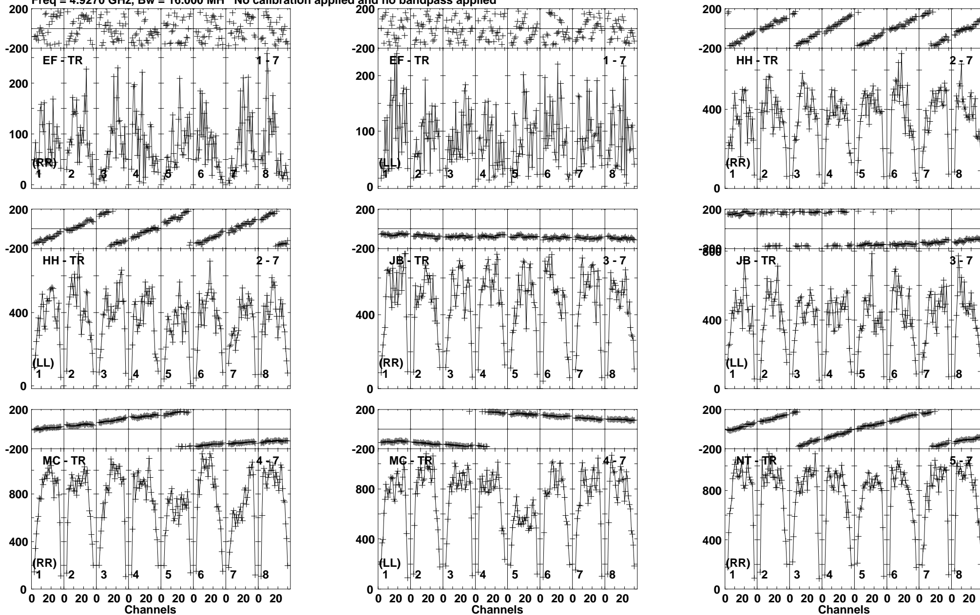
Lower frame: Micro Ampl Jy Top frame: Phas deg Vector averaged cross-power spectrum Baseline: EF (01) - TR (07) Timerange: 00/17:46:12 to 00/17:49:38
