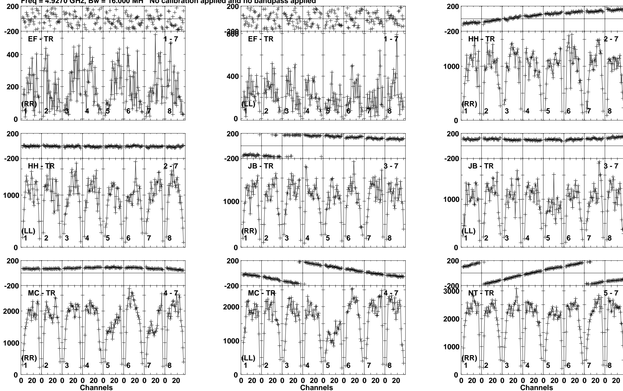
Lower frame: Micro Ampl Jy Top frame: Phas deg Vector averaged cross-power spectrum Baseline: EF (01) - TR (07) Timerange: 01/10:43:31 to 01/10:44:59
