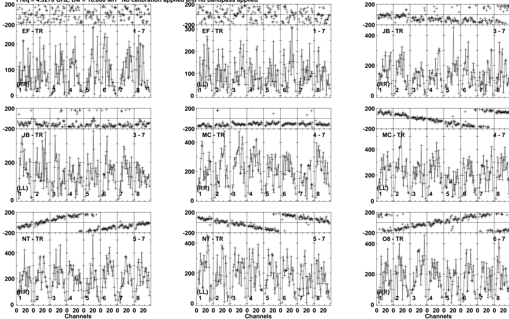
Lower frame: Micro Ampl Jy Top frame: Phas deg Vector averaged cross-power spectrum Baseline: EF (01) - TR (07) Timerange: 01/02:44:01 to 01/02:47:29
