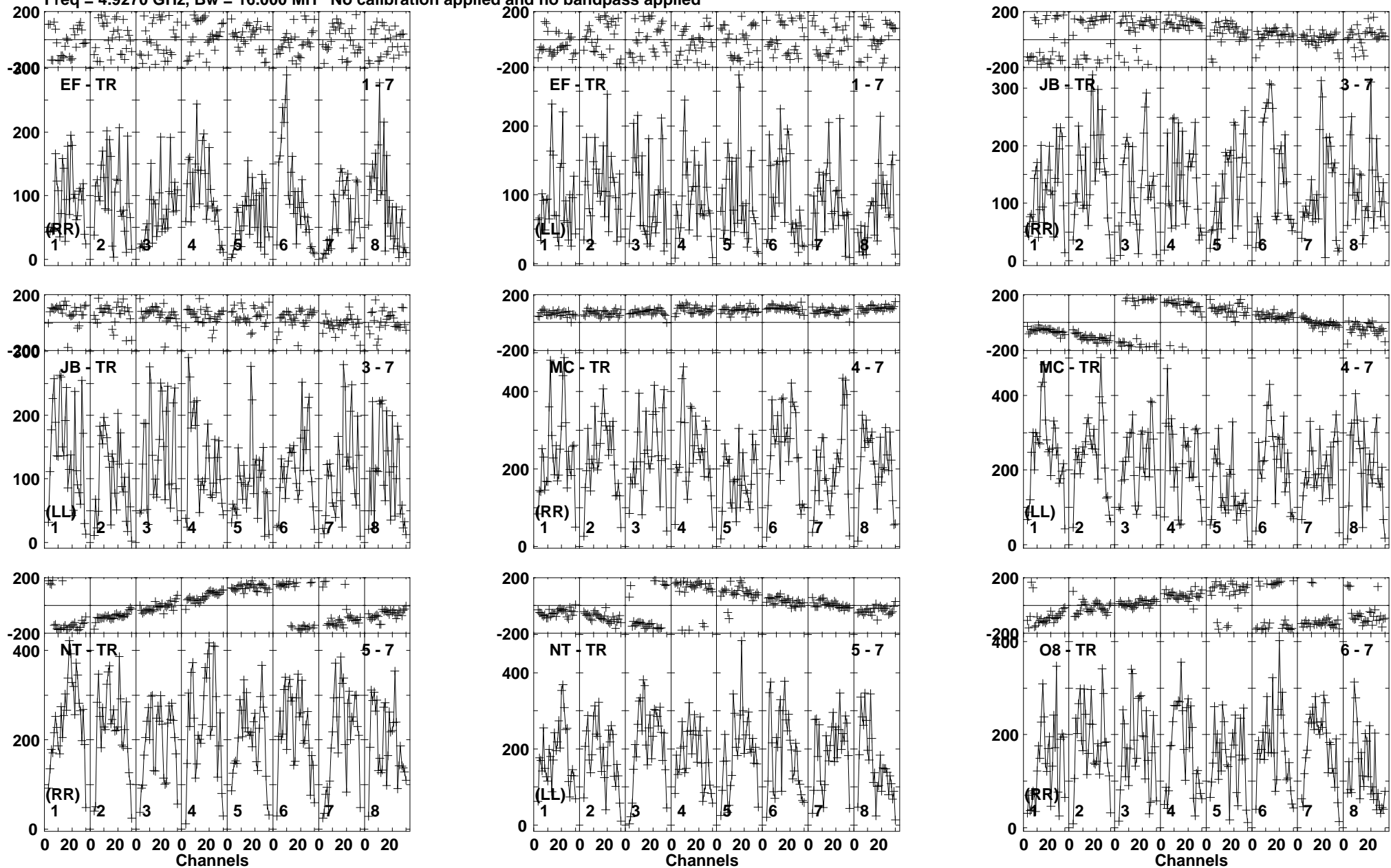
Lower frame: Micro Ampl Jy Top frame: Phas deg Vector averaged cross-power spectrum Baseline: EF (01) - TR (07) Timerange: 01/04:14:01 to 01/04:17:29
