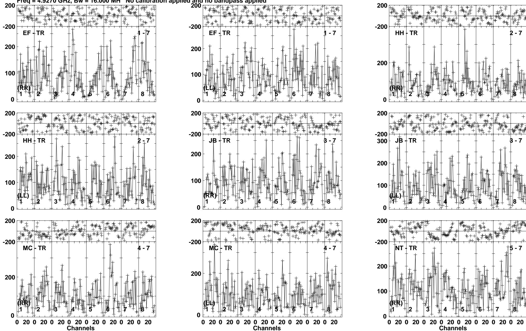
Lower frame: Micro Ampl Jy Top frame: Phas deg Vector averaged cross-power spectrum Baseline: EF (01) - TR (07) Timerange: 01/09:00:01 to 01/09:03:29
