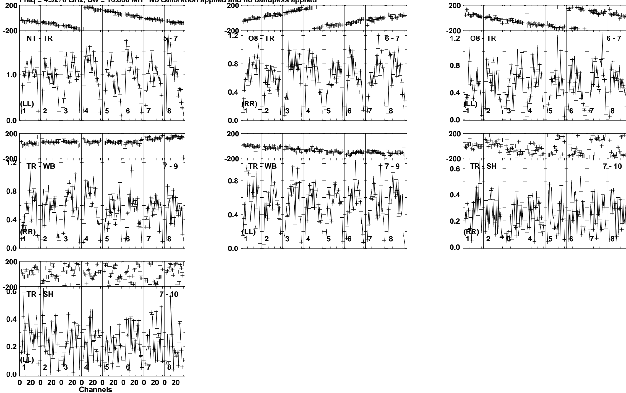
Lower frame: Milli Ampl Jy Top frame: Phas deg Vector averaged cross-power spectrum Baseline: NT (05) - TR (07) Timerange: 00/16:50:52 to 00/16:52:18
