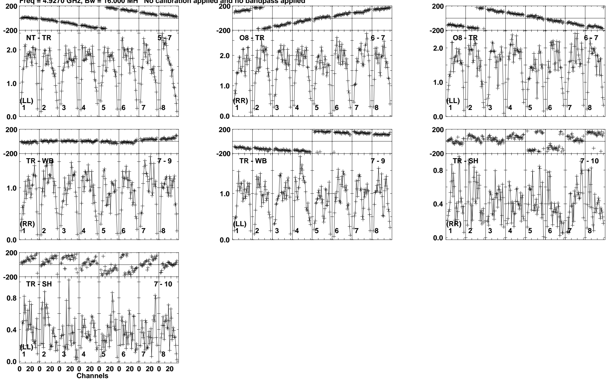
Lower frame: Milli Ampl Jy Top frame: Phas deg Vector averaged cross-power spectrum Baseline: NT (05) - TR (07) Timerange: 01/09:19:11 to 01/09:19:59
