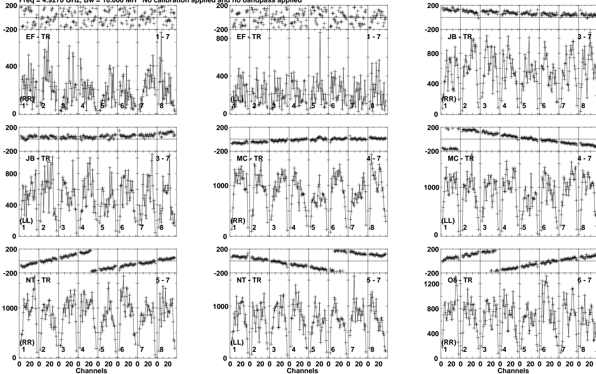
Lower frame: Micro Ampl Jy Top frame: Phas deg Vector averaged cross-power spectrum Baseline: EF (01) - TR (07) Timerange: 01/02:58:11 to 01/02:58:59
