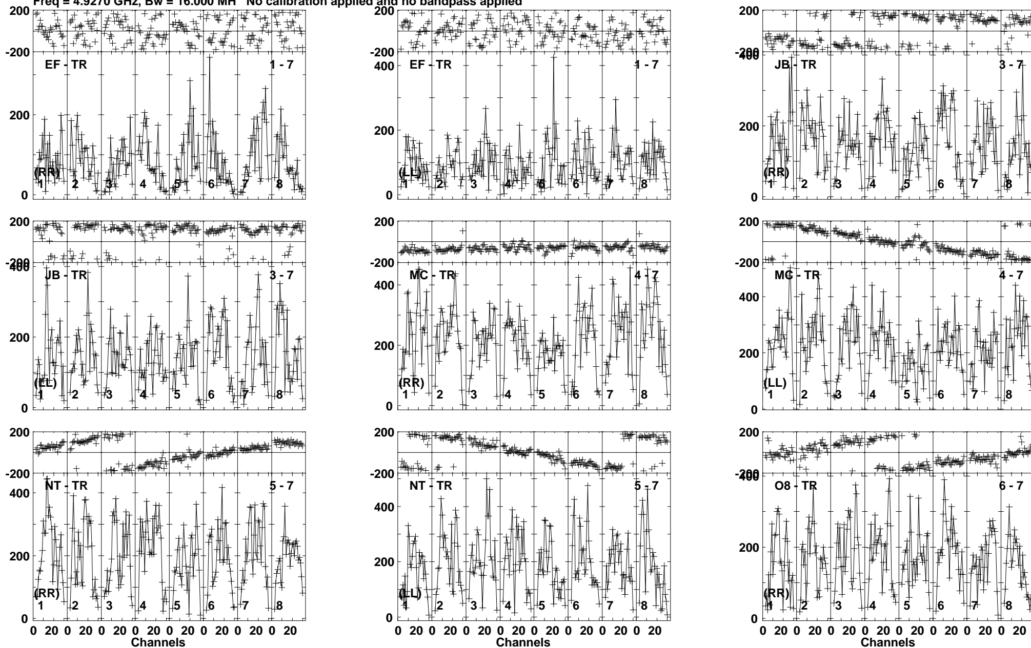
Lower frame: Micro Ampl Jy Top frame: Phas deg Vector averaged cross-power spectrum Baseline: EF (01) - TR (07) Timerange: 01/02:29:01 to 01/02:32:29
