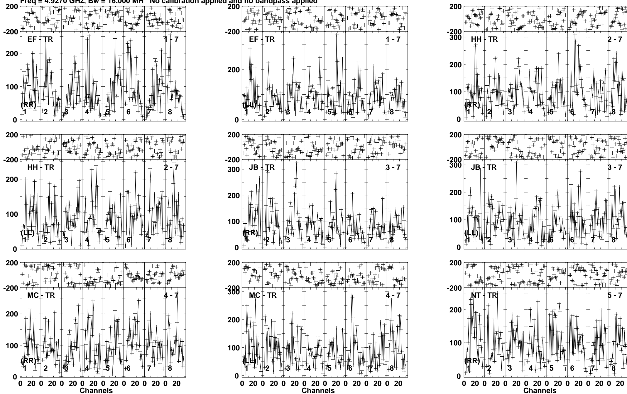
Lower frame: Micro Ampl Jy Top frame: Phas deg Vector averaged cross-power spectrum Baseline: EF (01) - TR (07) Timerange: 01/08:50:01 to 01/08:53:29
