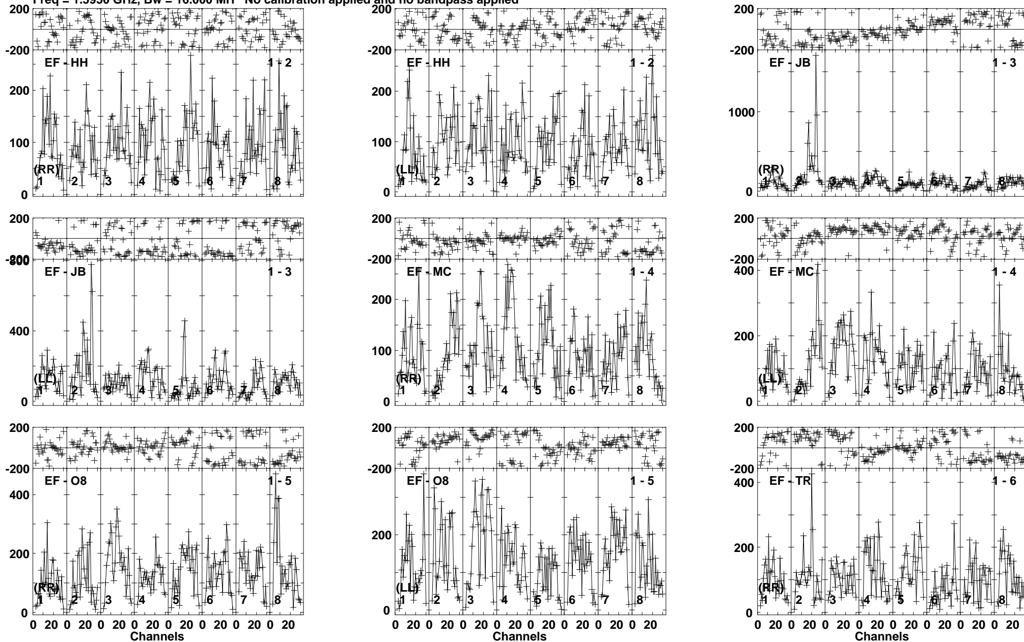
Lower frame: Micro Ampl Jy Top frame: Phas deg Vector averaged cross-power spectrum Baseline: EF (01) - HH (02) Timerange: 00/11:00:01 to 00/11:03:29
