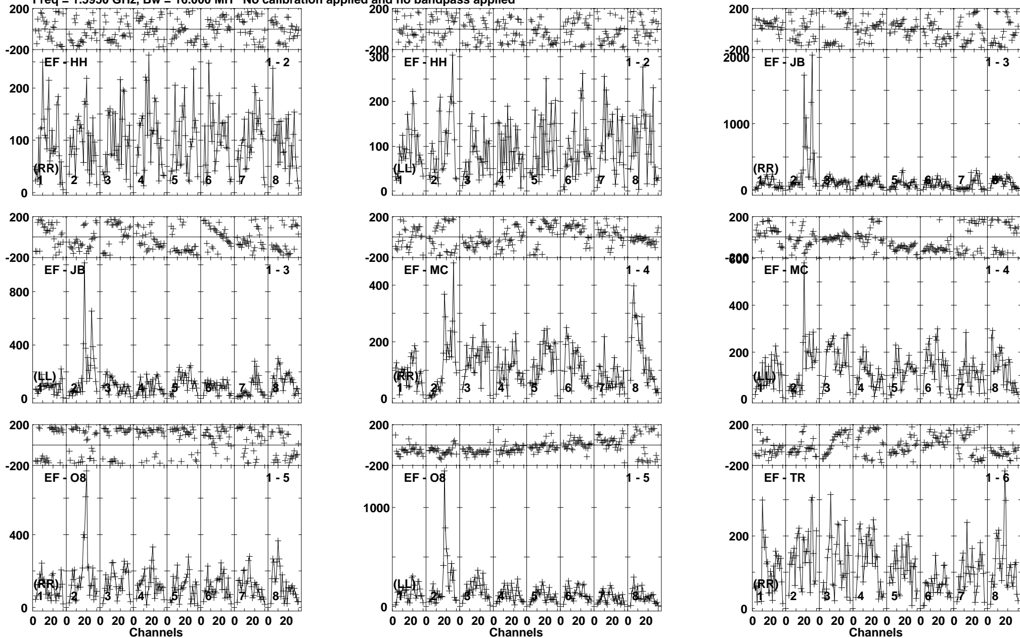
Lower frame: Micro Ampl Jy Top frame: Phas deg Vector averaged cross-power spectrum Baseline: EF (01) - HH (02) Timerange: 00/13:23:31 to 00/13:26:59
