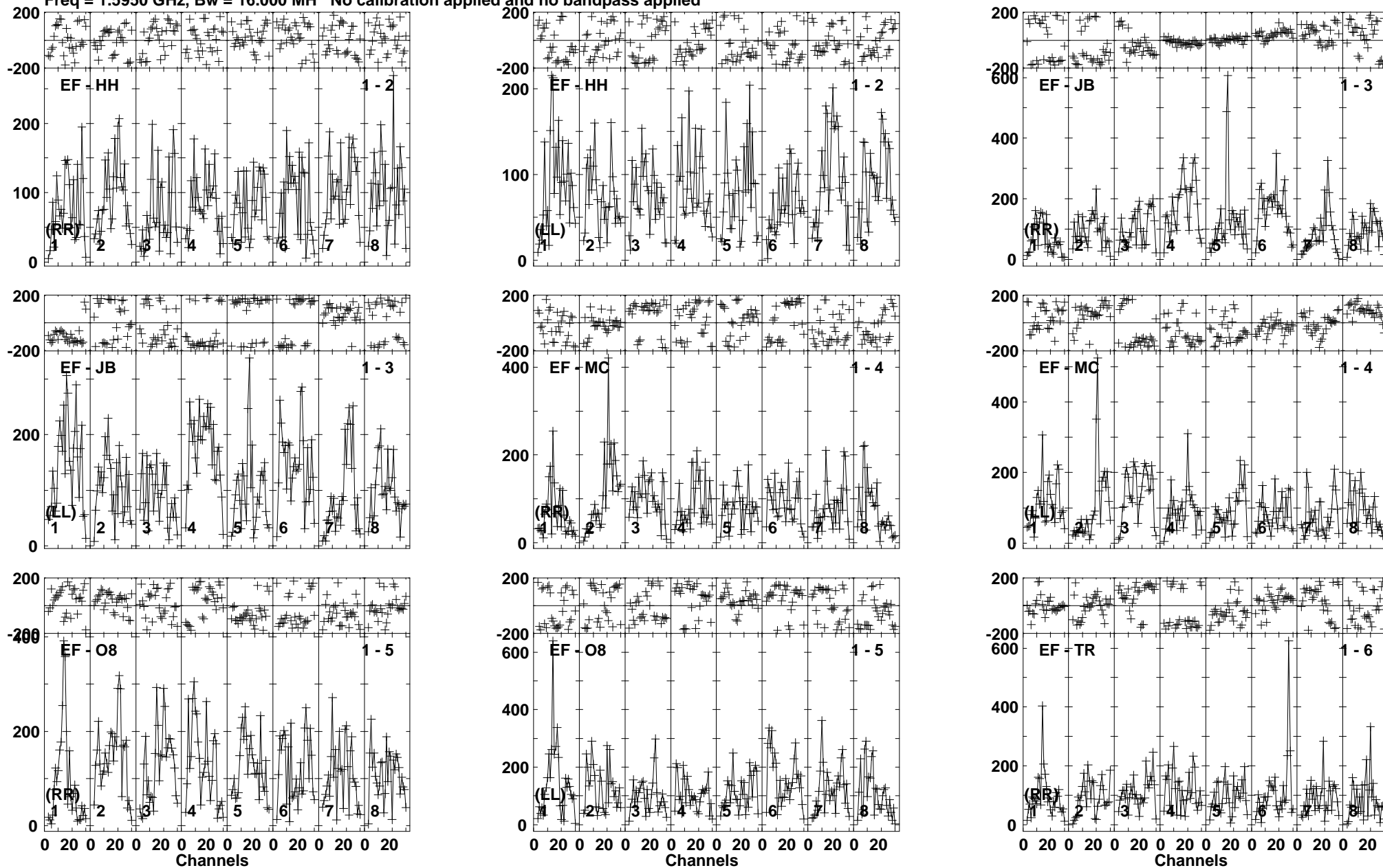
Lower frame: Micro Ampl Jy Top frame: Phas deg Vector averaged cross-power spectrum Baseline: EF (01) - HH (02) Timerange: 00/10:55:01 to 00/10:58:29
