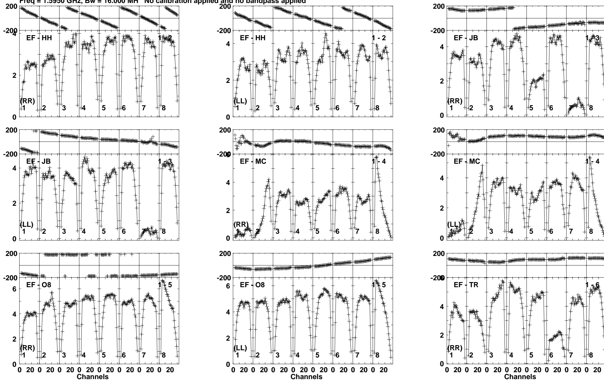
Lower frame: Milli Ampl Jy Top frame: Phas deg Vector averaged cross-power spectrum Baseline: EF (01) - HH (02) Timerange: 00/13:12:41 to 00/13:13:29
