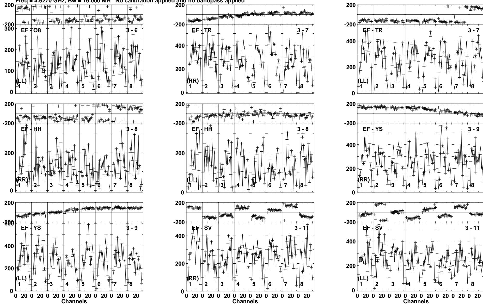
Lower frame: Micro Ampl Jy Top frame: Phas deg Vector averaged cross-power spectrum Baseline: EF (03) - O8 (06) Timerange: 00/09:28:11 to 00/09:31:49
