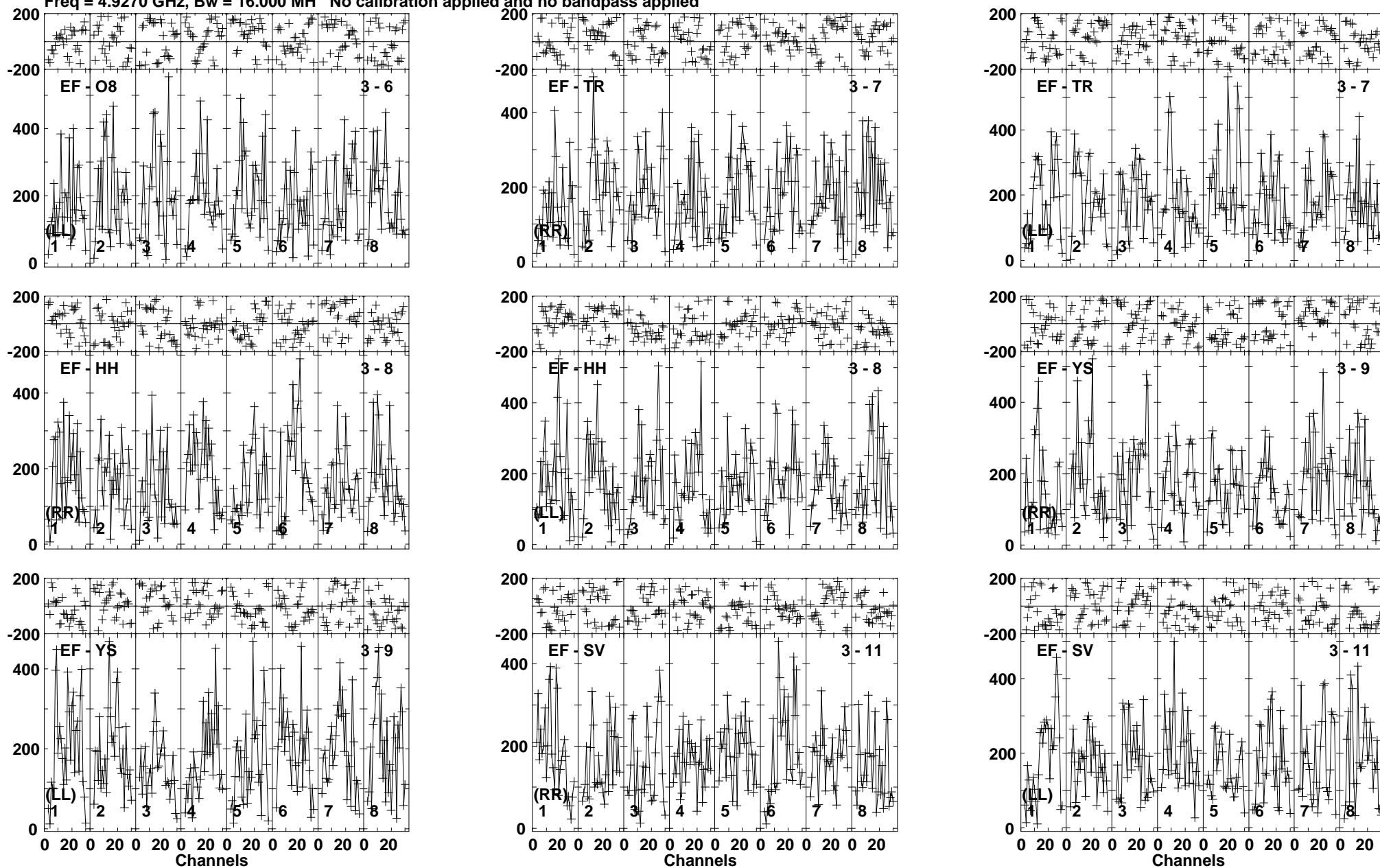
Lower frame: Micro Ampl Jy Top frame: Phas deg Vector averaged cross-power spectrum Baseline: EF (03) - O8 (06) Timerange: 00/09:34:11 to 00/09:37:39
