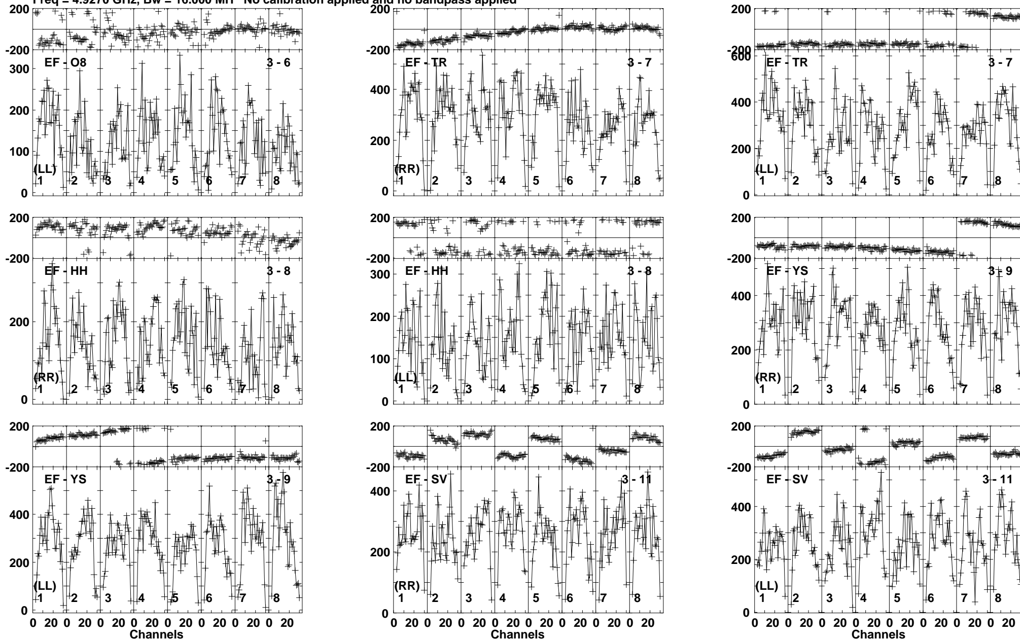
Lower frame: Micro Ampl Jy Top frame: Phas deg Vector averaged cross-power spectrum Baseline: EF (03) - O8 (06) Timerange: 00/09:51:31 to 00/09:55:19
