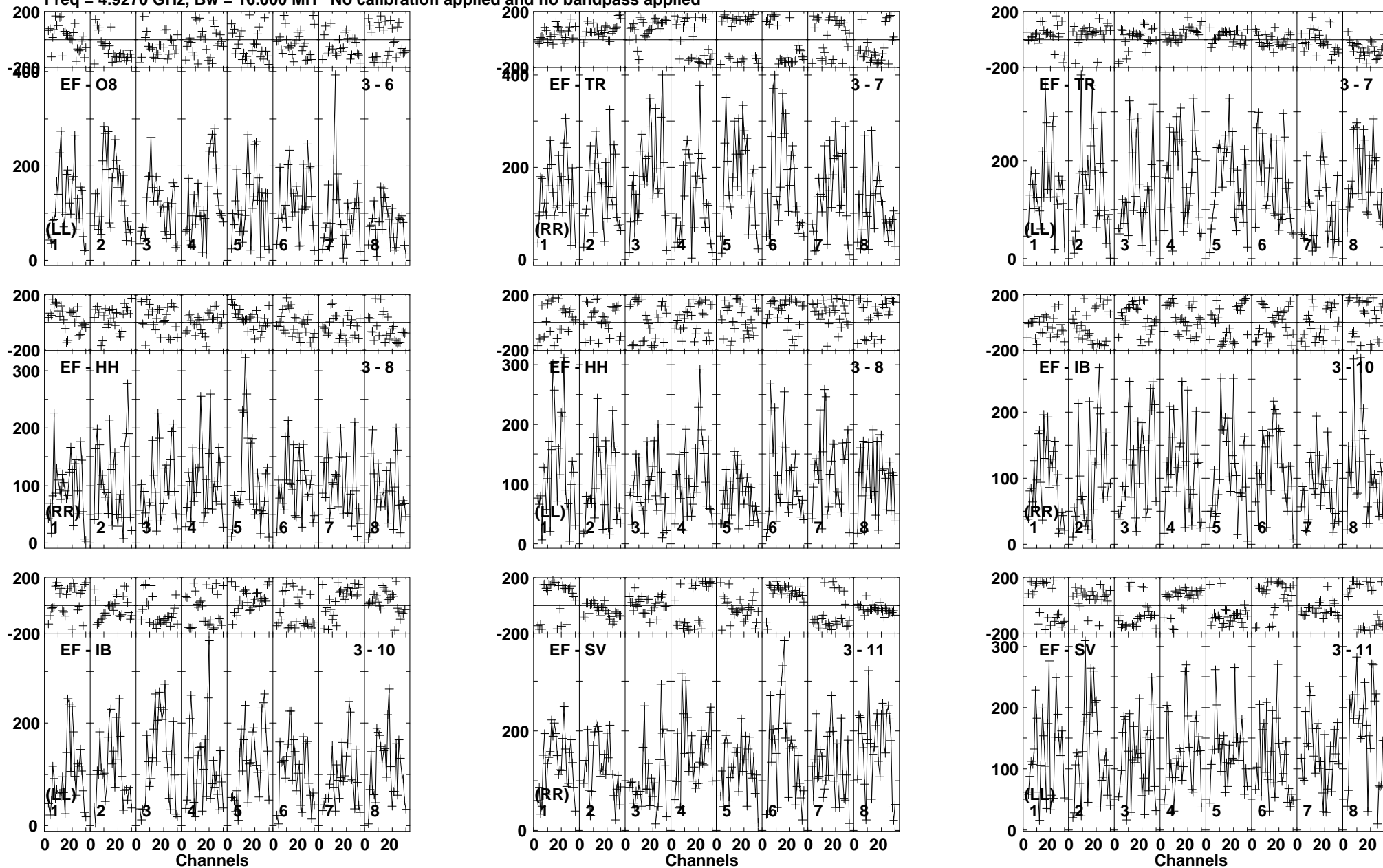
Lower frame: Micro Ampl Jy Top frame: Phas deg Vector averaged cross-power spectrum Baseline: EF (03) - O8 (06) Timerange: 00/08:02:31 to 00/08:05:59
