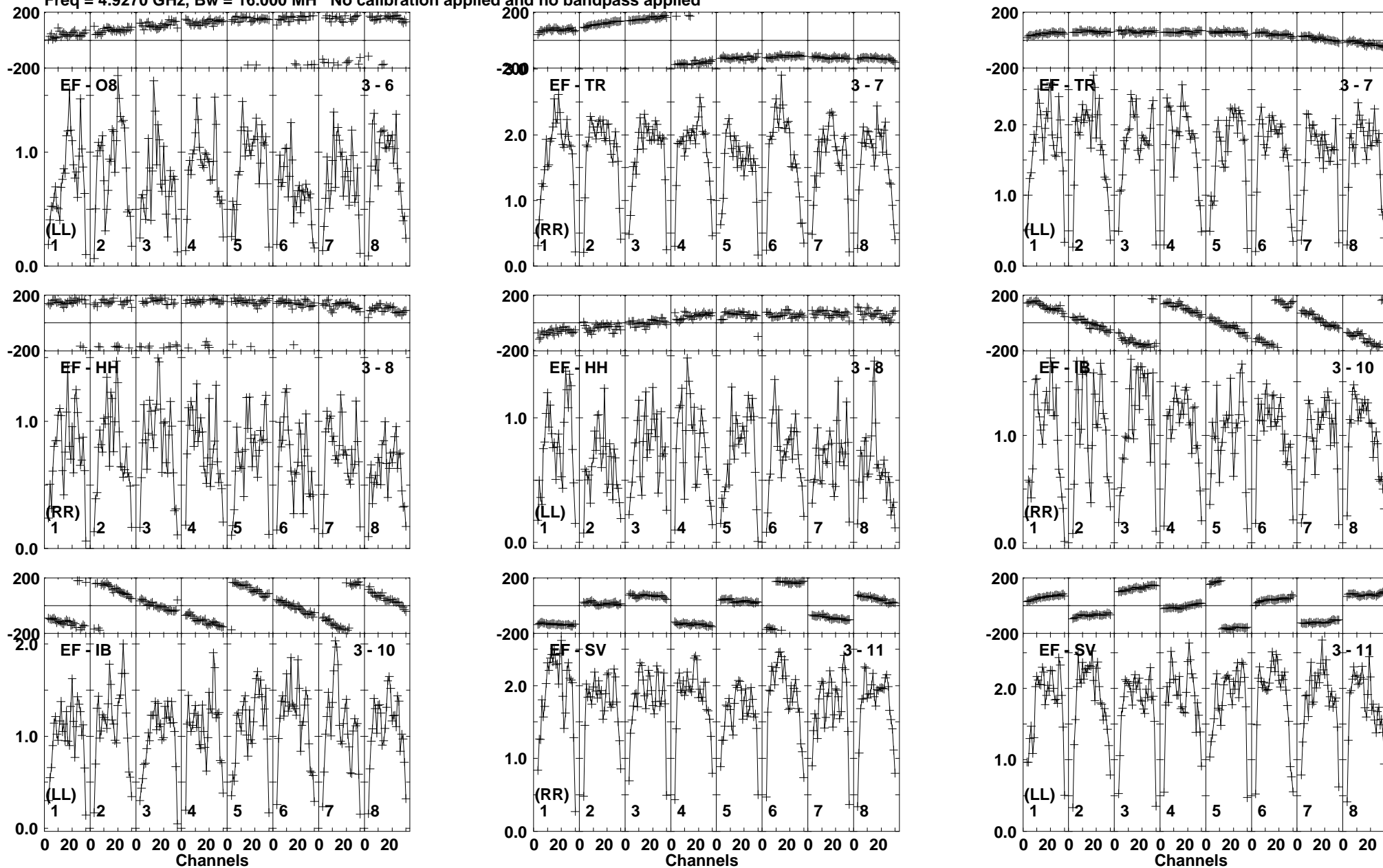
Lower frame: Milli Ampl Jy Top frame: Phas deg Vector averaged cross-power spectrum Baseline: EF (03) - O8 (06) Timerange: 00/14:47:51 to 00/14:49:19
