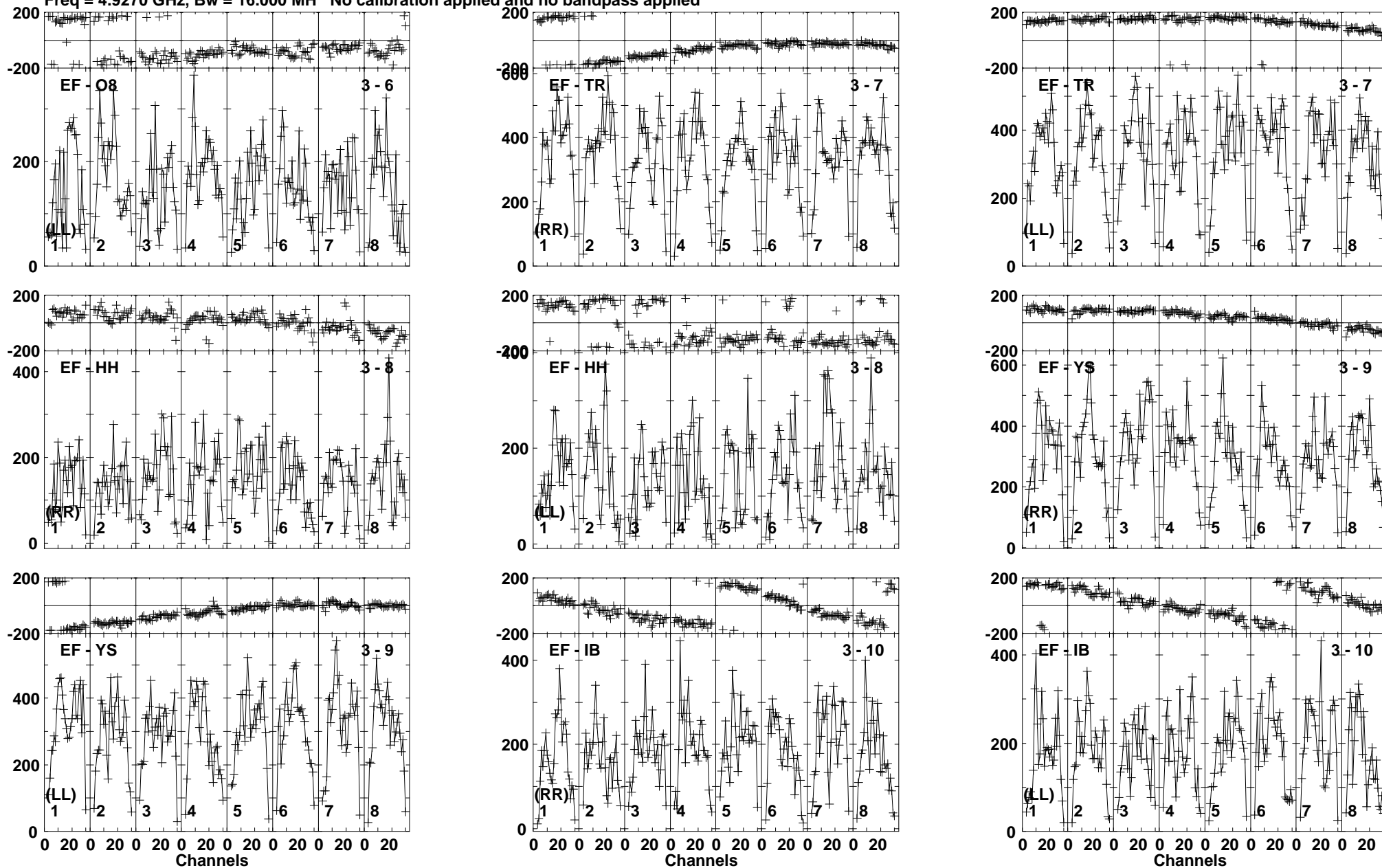
Lower frame: Micro Ampl Jy Top frame: Phas deg Vector averaged cross-power spectrum Baseline: EF (03) - O8 (06) Timerange: 00/13:21:51 to 00/13:25:19
