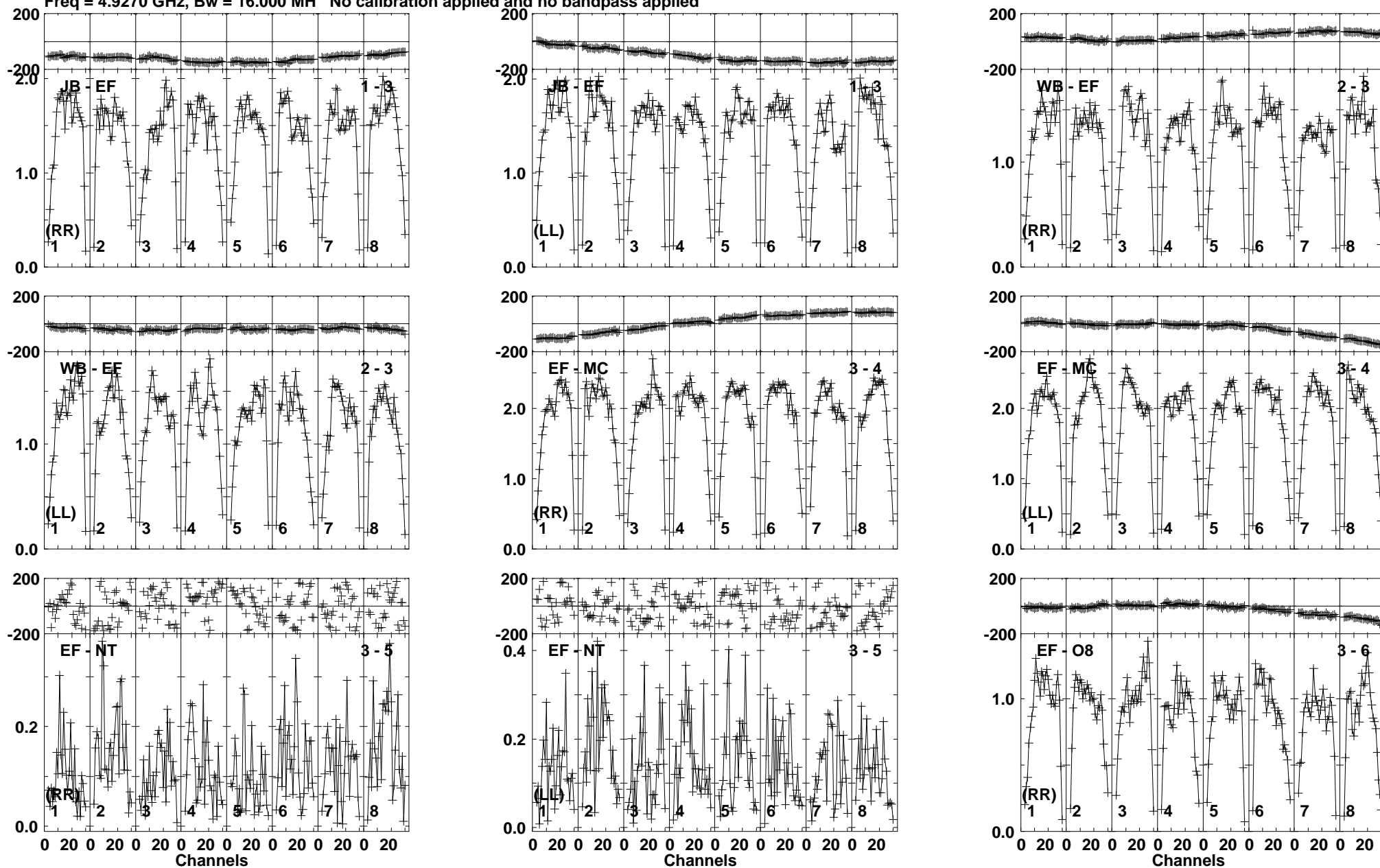
Lower frame: Milli Ampl Jy Top frame: Phas deg Vector averaged cross-power spectrum Baseline: JB (01) - EF (03) Timerange: 00/10:46:51 to 00/10:48:19
