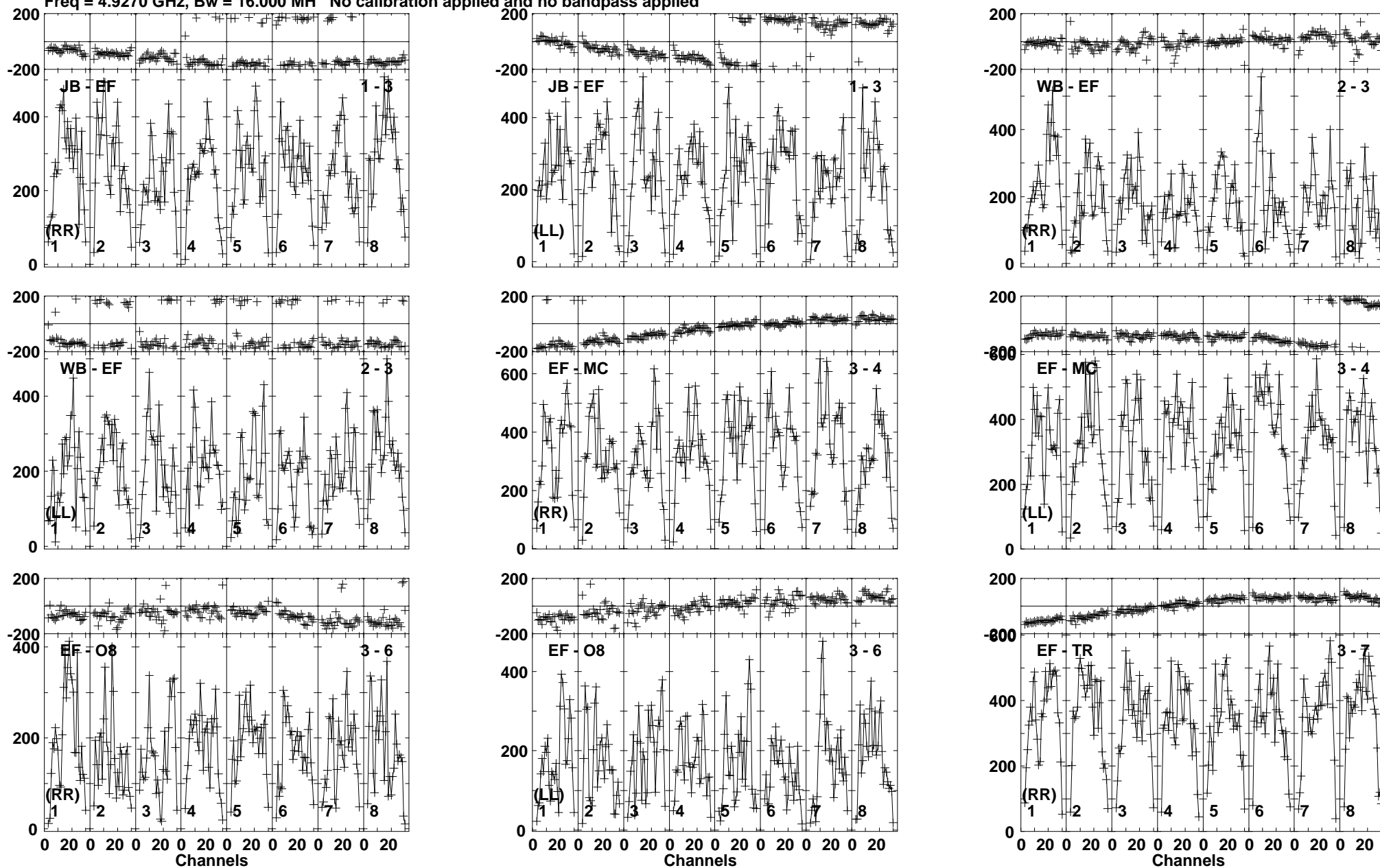
Lower frame: Micro Ampl Jy Top frame: Phas deg Vector averaged cross-power spectrum Baseline: JB (01) - EF (03) Timerange: 00/12:44:51 to 00/12:48:39
