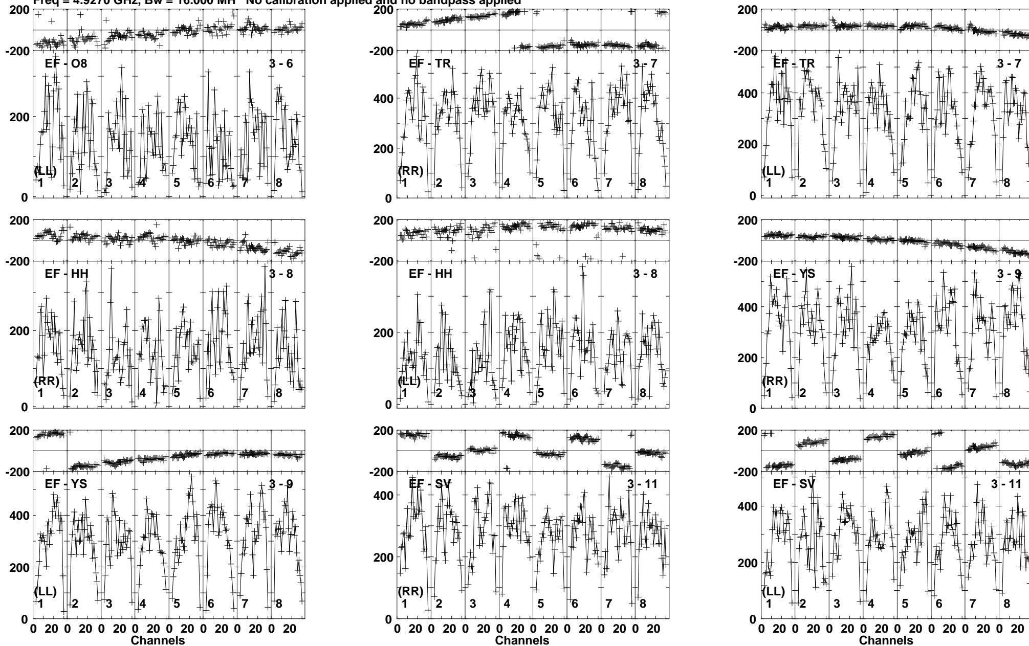
Lower frame: Micro Ampl Jy Top frame: Phas deg Vector averaged cross-power spectrum Baseline: EF (03) - O8 (06) Timerange: 00/11:19:01 to 00/11:22:49
