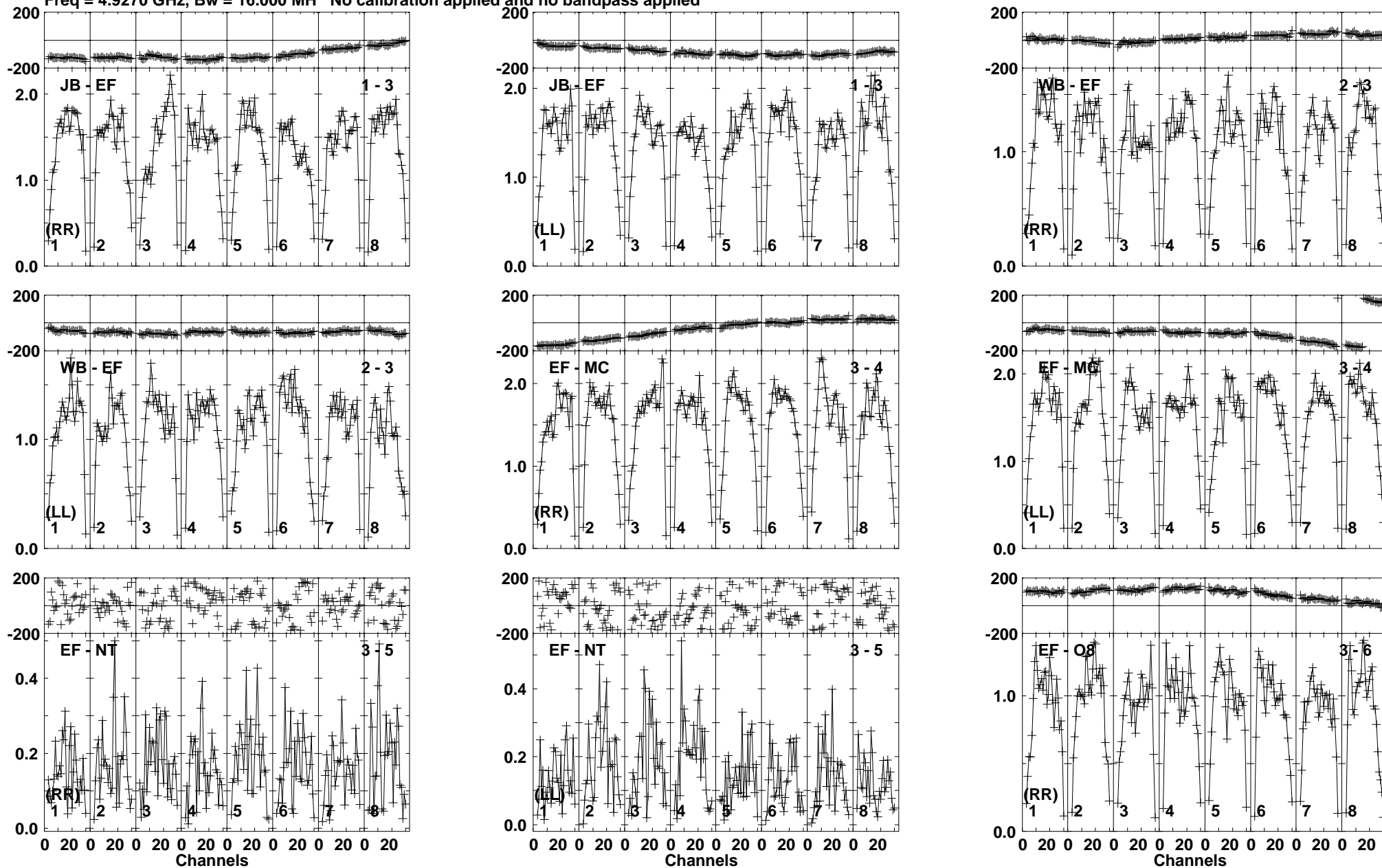
Lower frame: Milli Ampl Jy Top frame: Phas deg Vector averaged cross-power spectrum Baseline: JB (01) - EF (03) Timerange: 00/09:25:21 to 00/09:26:49
