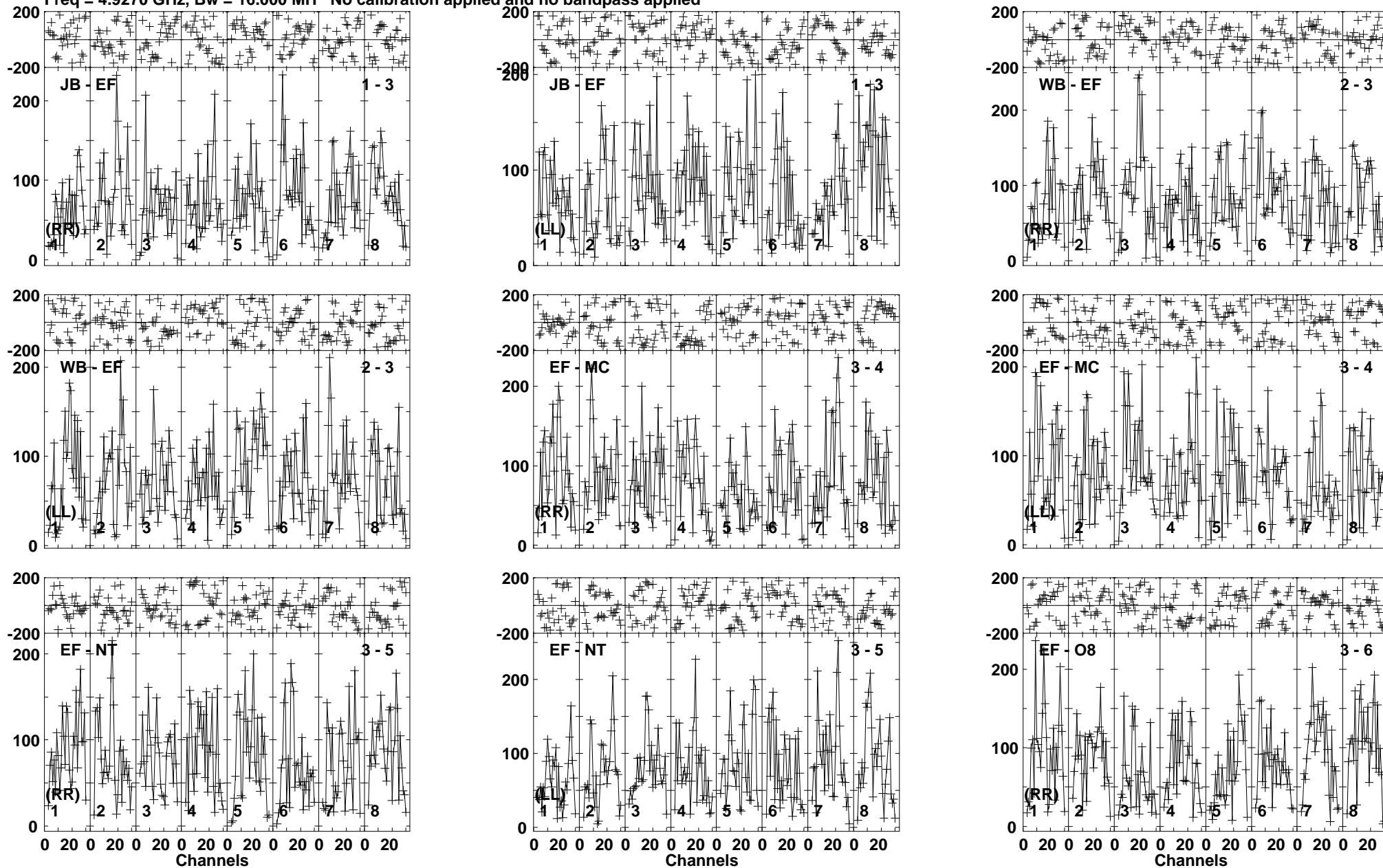
Lower frame: Micro Ampl Jy Top frame: Phas deg Vector averaged cross-power spectrum Baseline: JB (01) - EF (03) Timerange: 00/07:44:01 to 00/07:47:39
