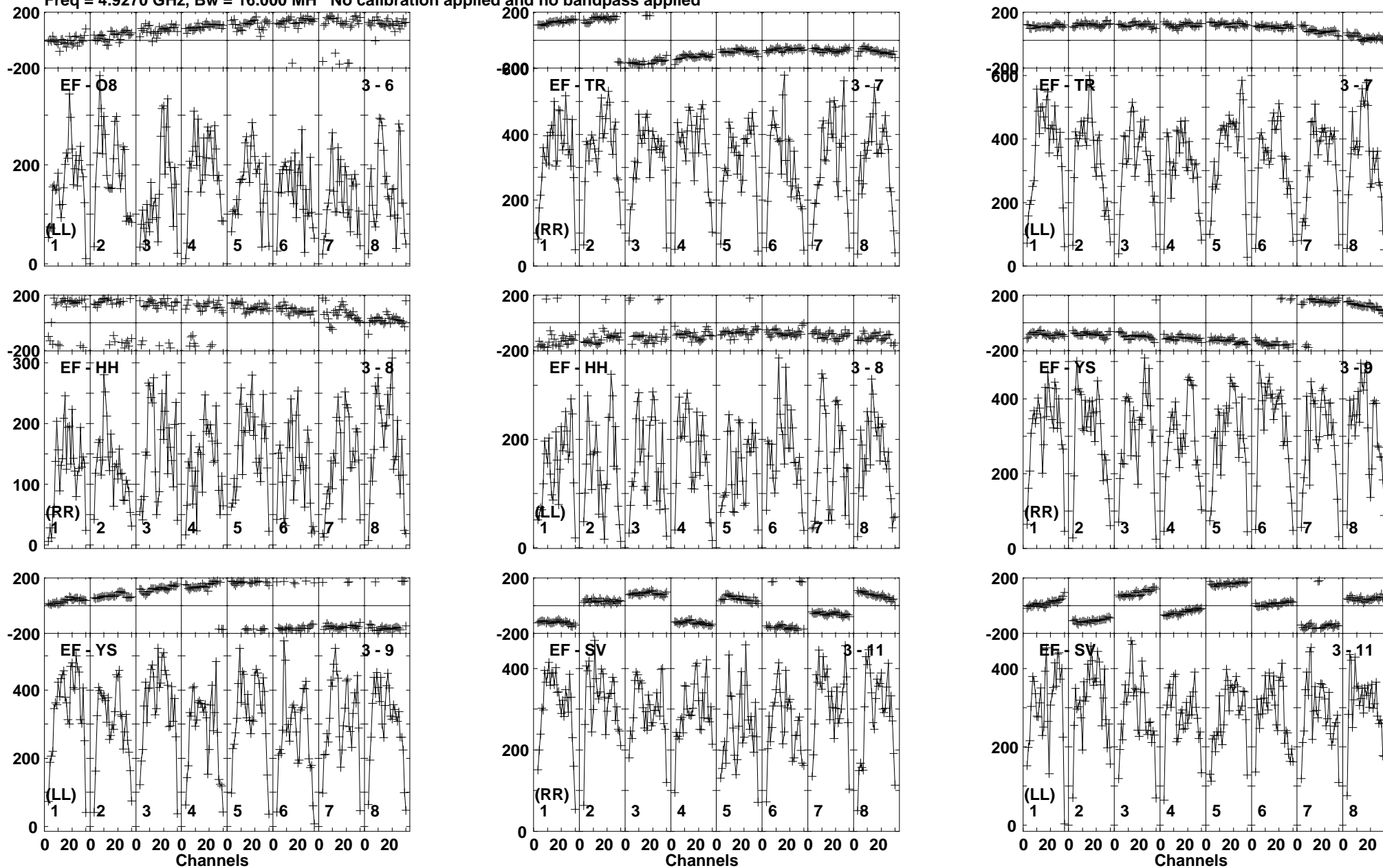
Lower frame: Micro Ampl Jy Top frame: Phas deg Vector averaged cross-power spectrum Baseline: EF (03) - O8 (06) Timerange: 00/12:04:11 to 00/12:07:59
