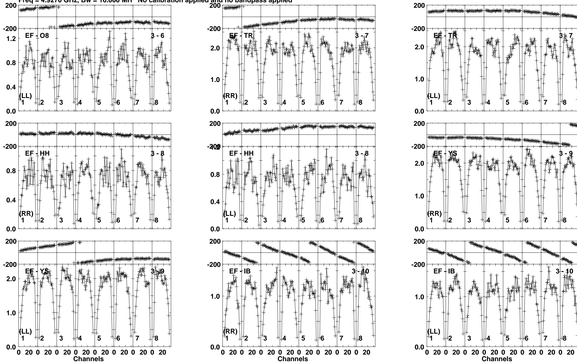
Lower frame: Milli Ampl Jy Top frame: Phas deg Vector averaged cross-power spectrum Baseline: EF (03) - O8 (06) Timerange: 00/13:13:21 to 00/13:14:49
