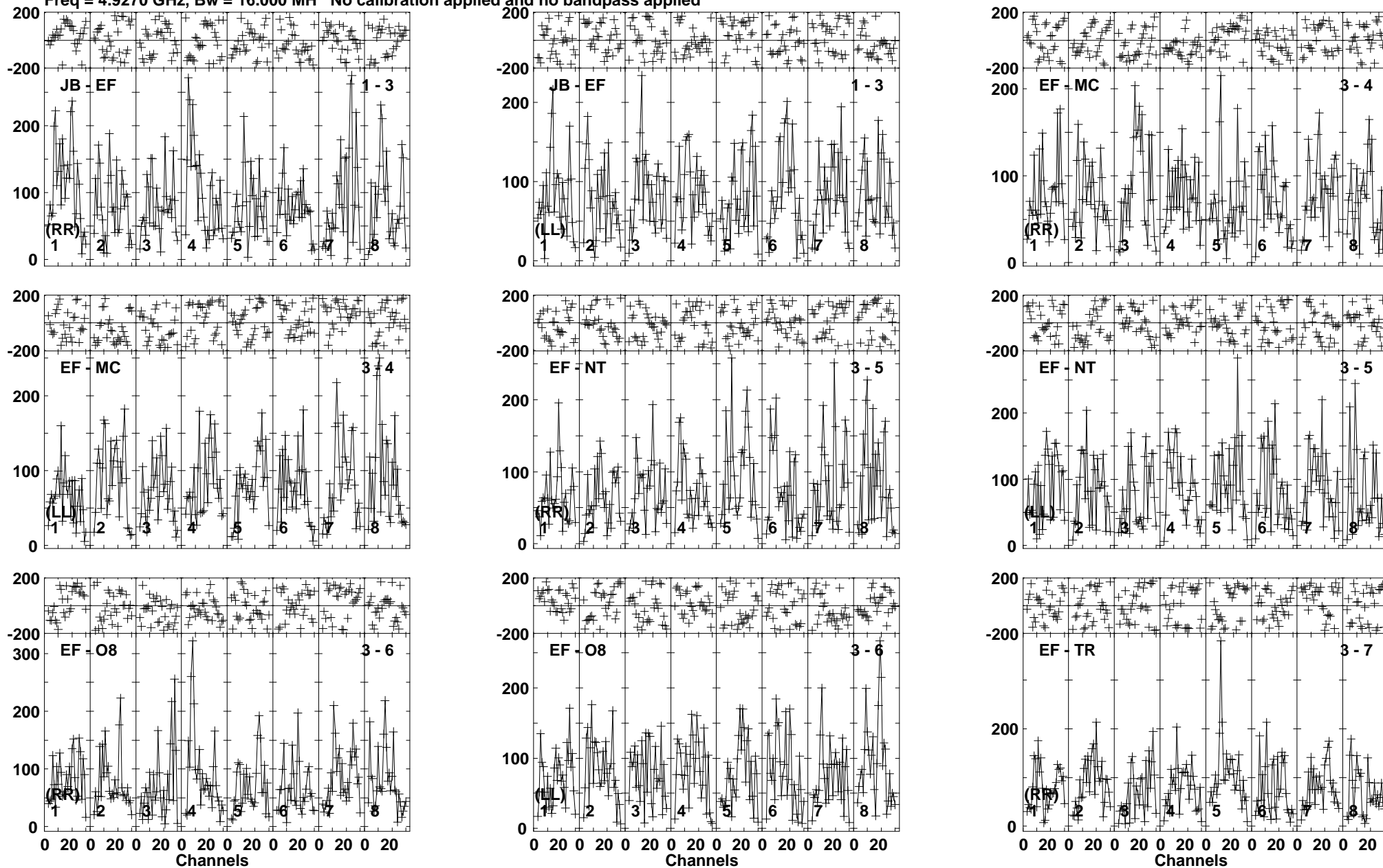
Lower frame: Micro Ampl Jy Top frame: Phas deg Vector averaged cross-power spectrum Baseline: JB (01) - EF (03) Timerange: 00/07:26:31 to 00/07:30:09
