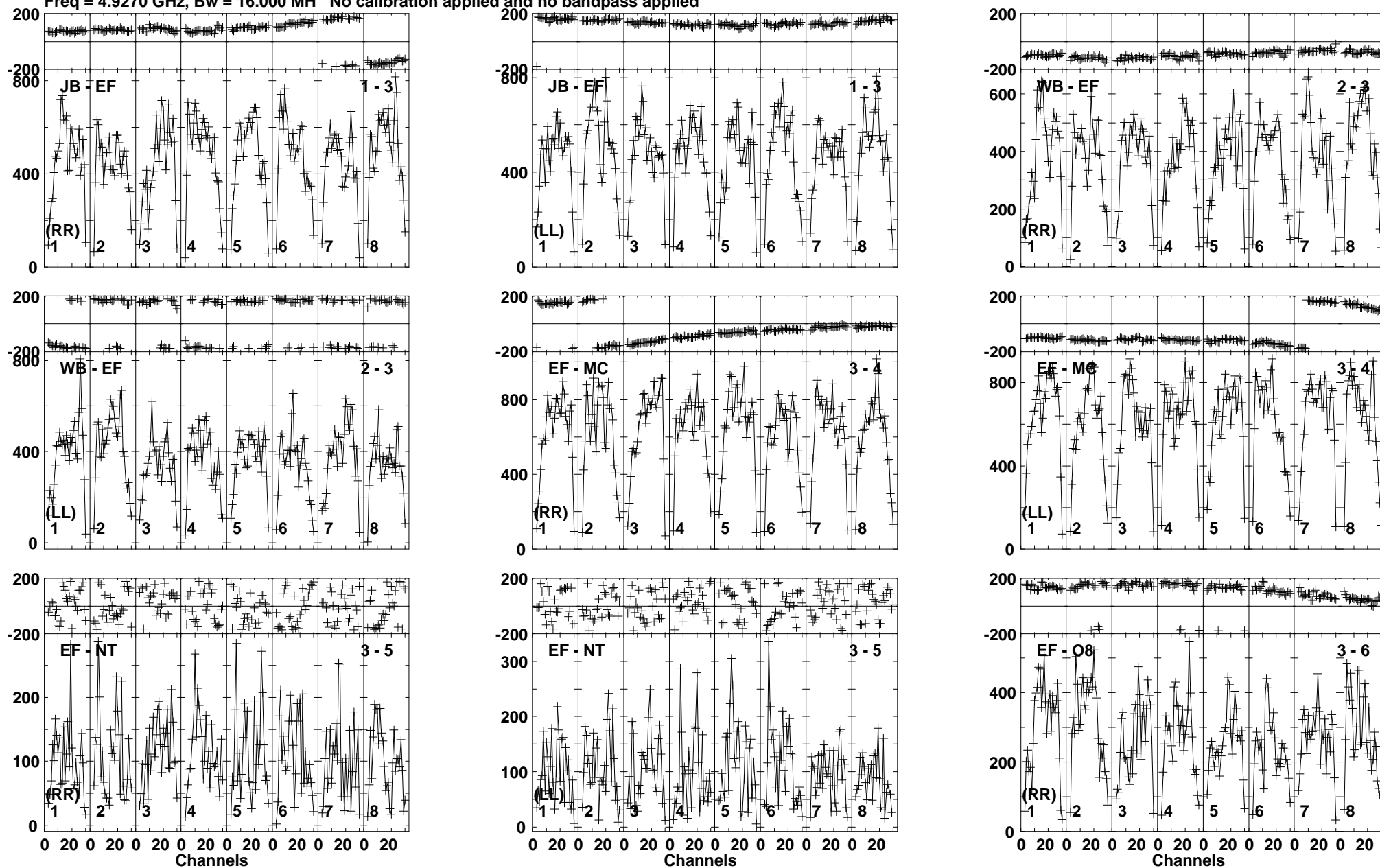
Lower frame: Micro Ampl Jy Top frame: Phas deg Vector averaged cross-power spectrum Baseline: JB (01) - EF (03) Timerange: 00/08:41:11 to 00/08:44:39
