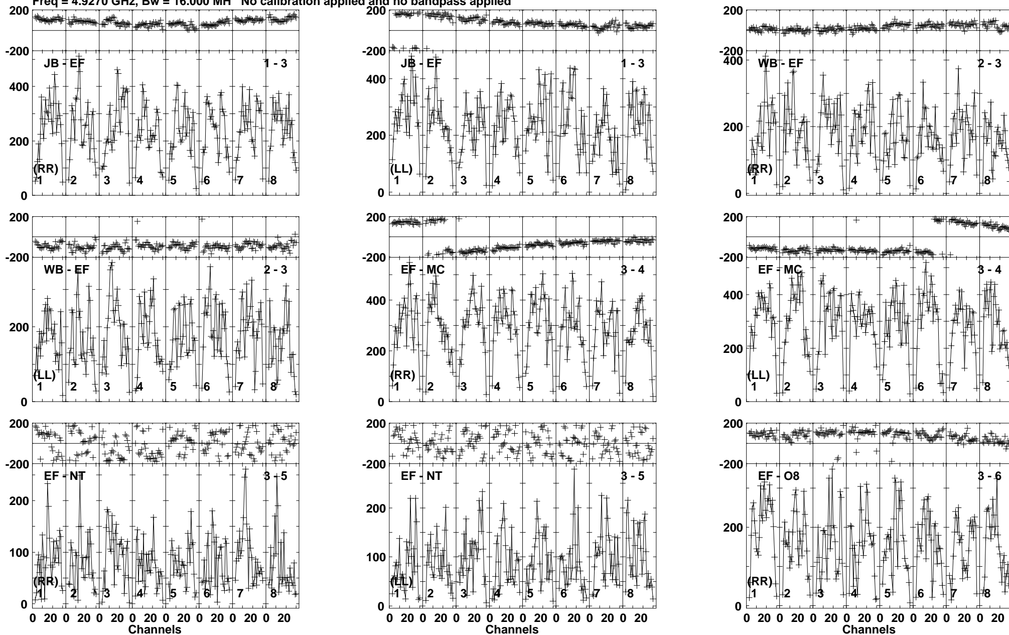
Lower frame: Micro Ampl Jy Top frame: Phas deg Vector averaged cross-power spectrum Baseline: JB (01) - EF (03) Timerange: 00/10:50:01 to 00/10:53:49
