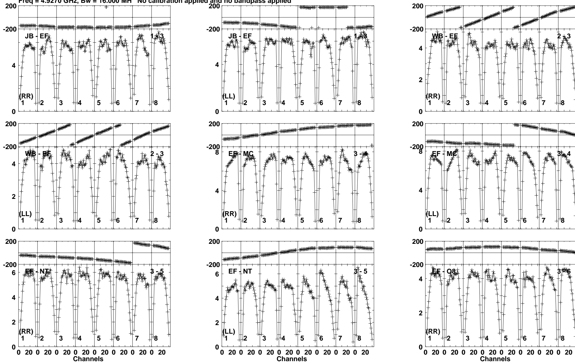
Lower frame: Milli Ampl Jy Top frame: Phas deg Vector averaged cross-power spectrum Baseline: JB (01) - EF (03) Timerange: 00/04:14:51 to 00/04:16:19
