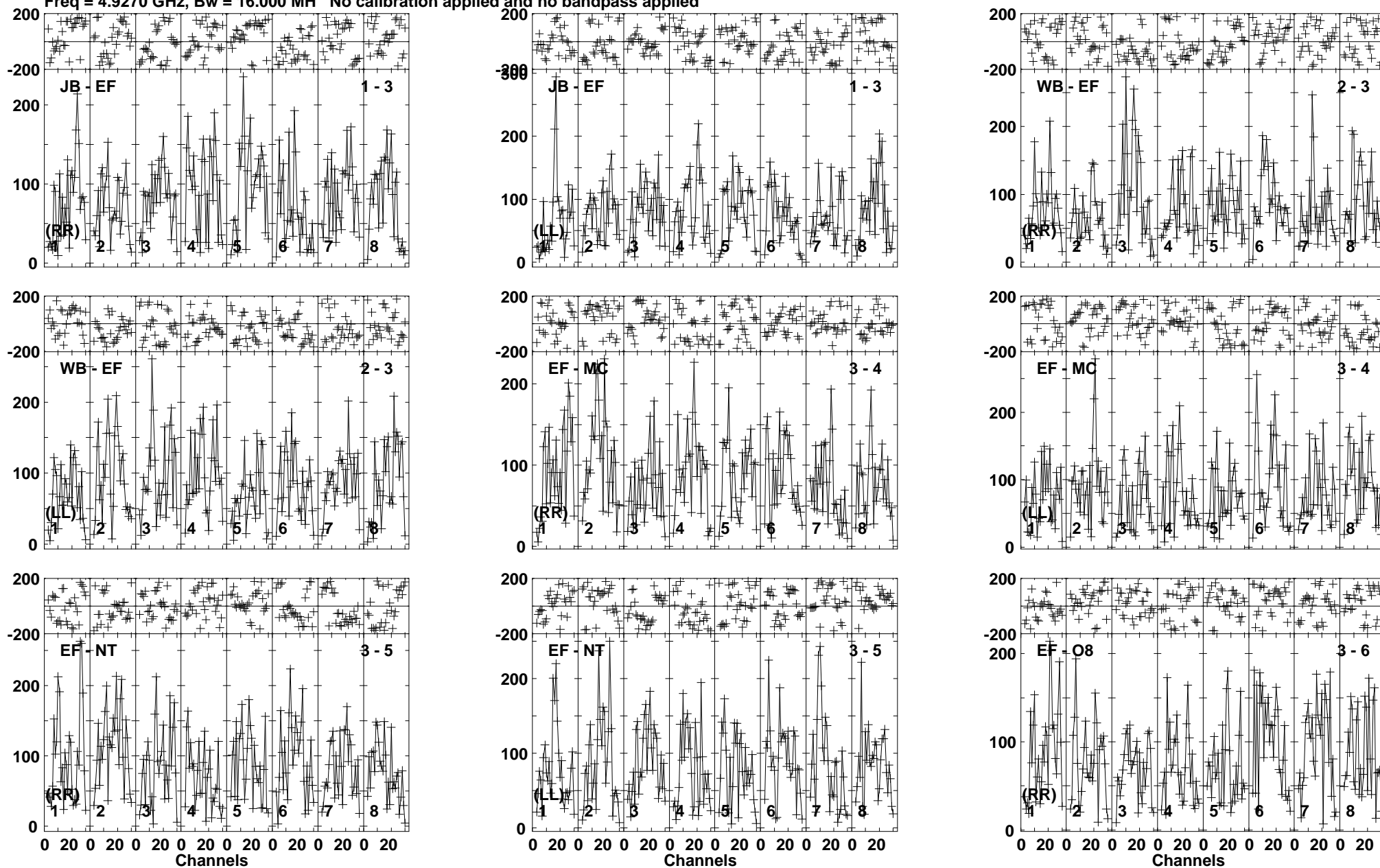
Lower frame: Micro Ampl Jy Top frame: Phas deg Vector averaged cross-power spectrum Baseline: JB (01) - EF (03) Timerange: 00/03:53:41 to 00/03:57:39
