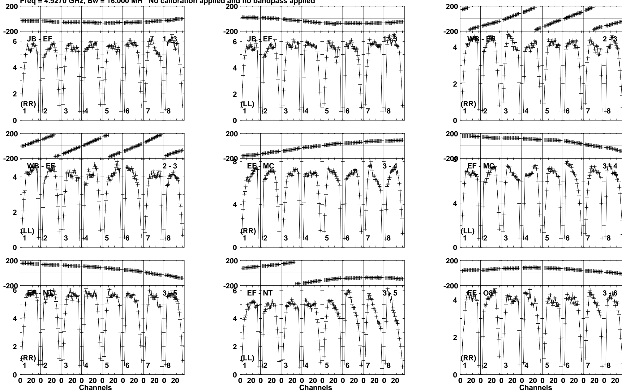
Lower frame: Milli Ampl Jy Top frame: Phas deg Vector averaged cross-power spectrum Baseline: JB (01) - EF (03) Timerange: 00/03:13:01 to 00/03:14:09
