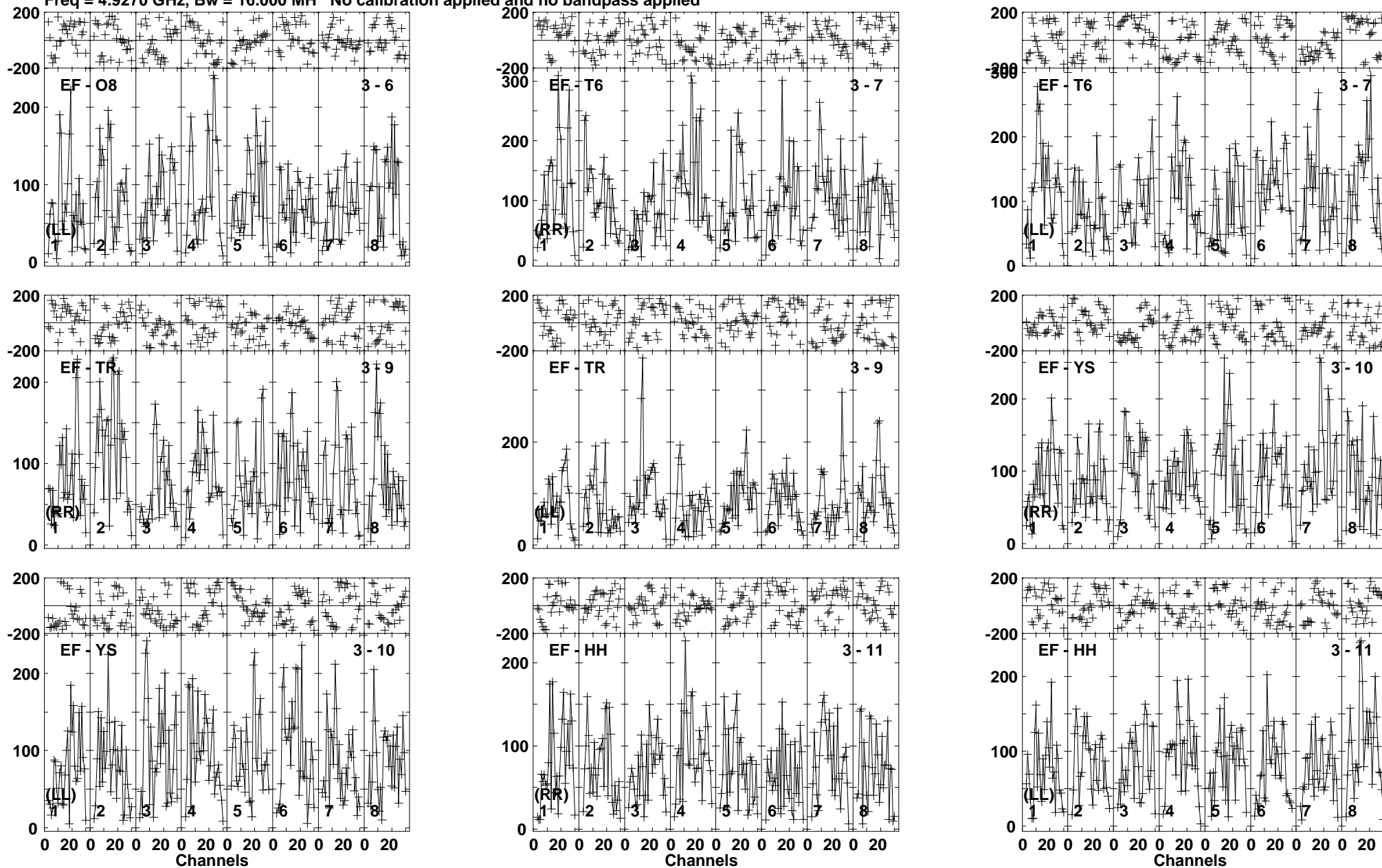
Lower frame: Micro Ampl Jy Top frame: Phas deg Vector averaged cross-power spectrum Baseline: EF (03) - O8 (06) Timerange: 00/03:48:11 to 00/03:52:09
