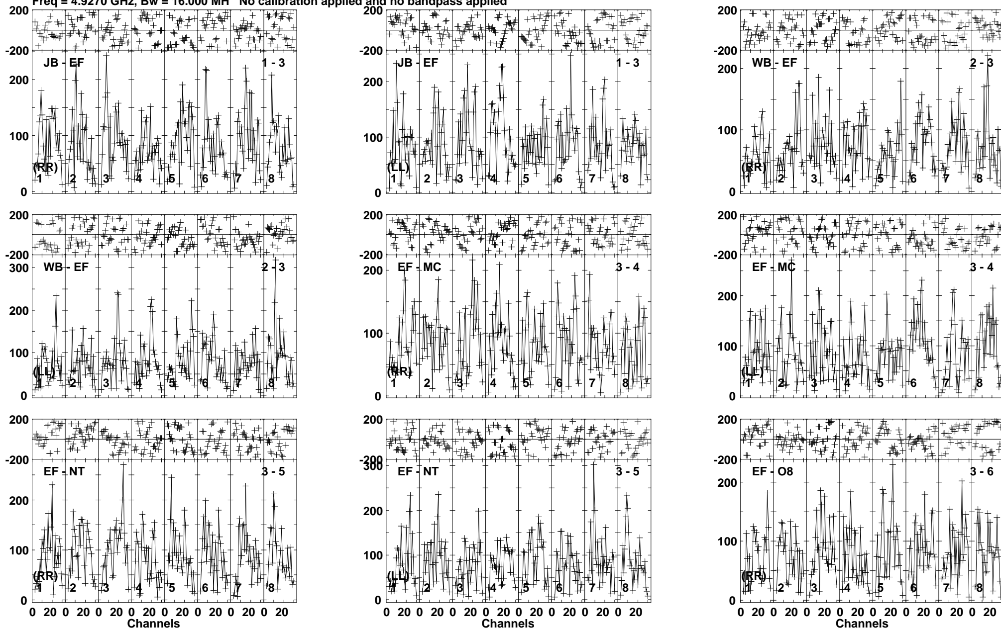
Lower frame: Micro Ampl Jy Top frame: Phas deg Vector averaged cross-power spectrum Baseline: JB (01) - EF (03) Timerange: 00/02:34:21 to 00/02:38:19
