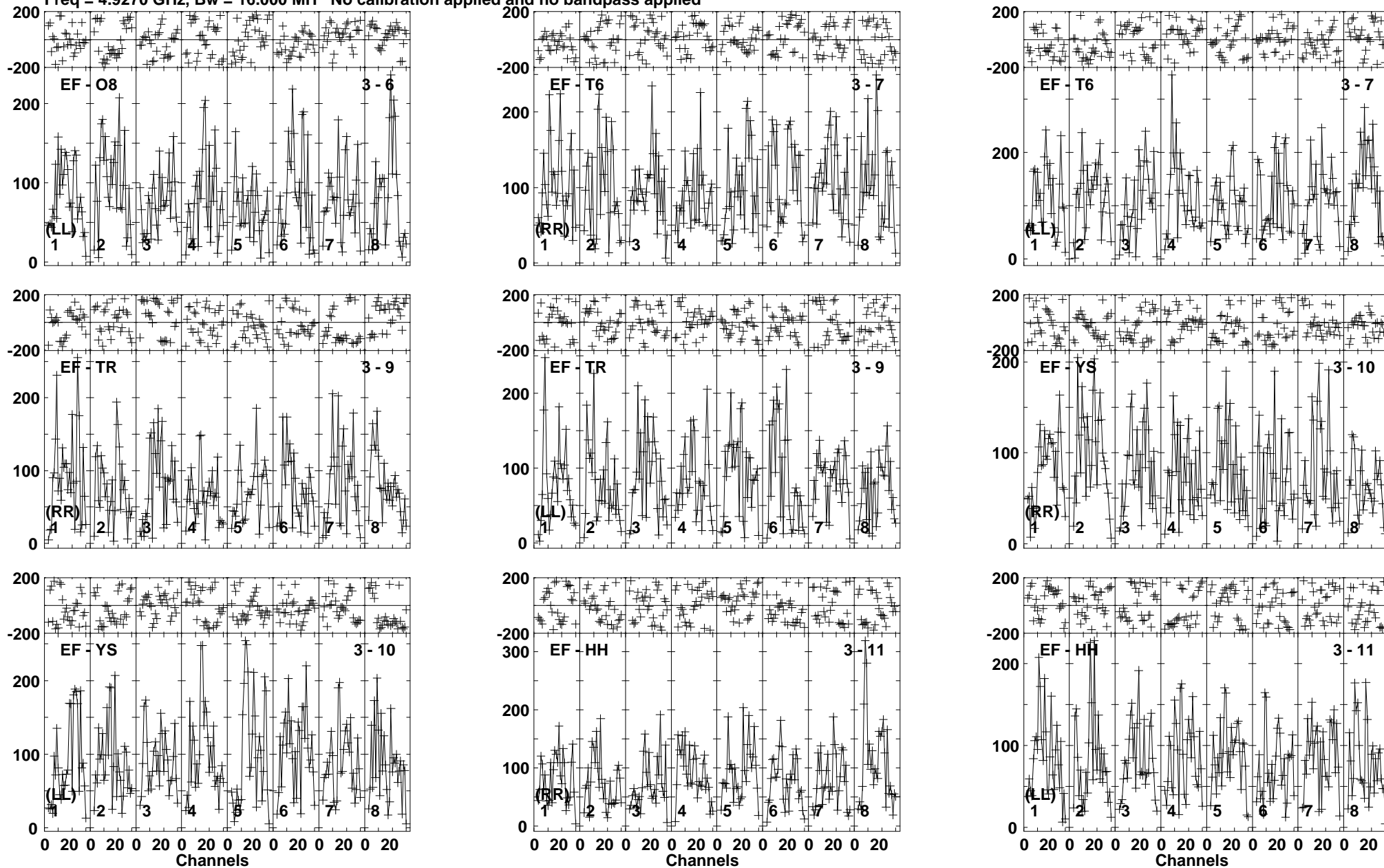
Lower frame: Micro Ampl Jy Top frame: Phas deg Vector averaged cross-power spectrum Baseline: EF (03) - O8 (06) Timerange: 00/02:51:31 to 00/02:55:29
