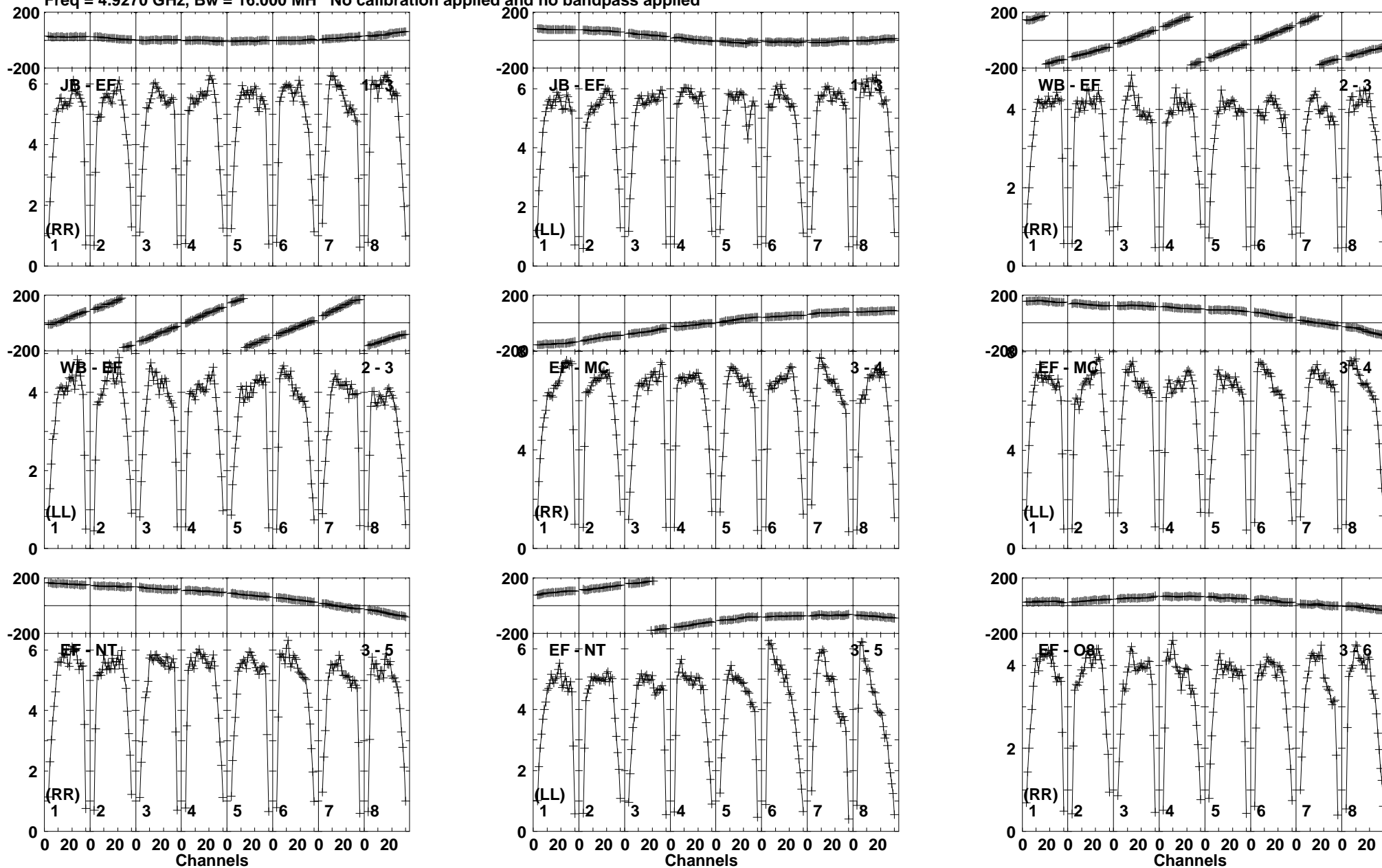
Lower frame: Milli Ampl Jy Top frame: Phas deg Vector averaged cross-power spectrum Baseline: JB (01) - EF (03) Timerange: 00/03:18:11 to 00/03:19:39
