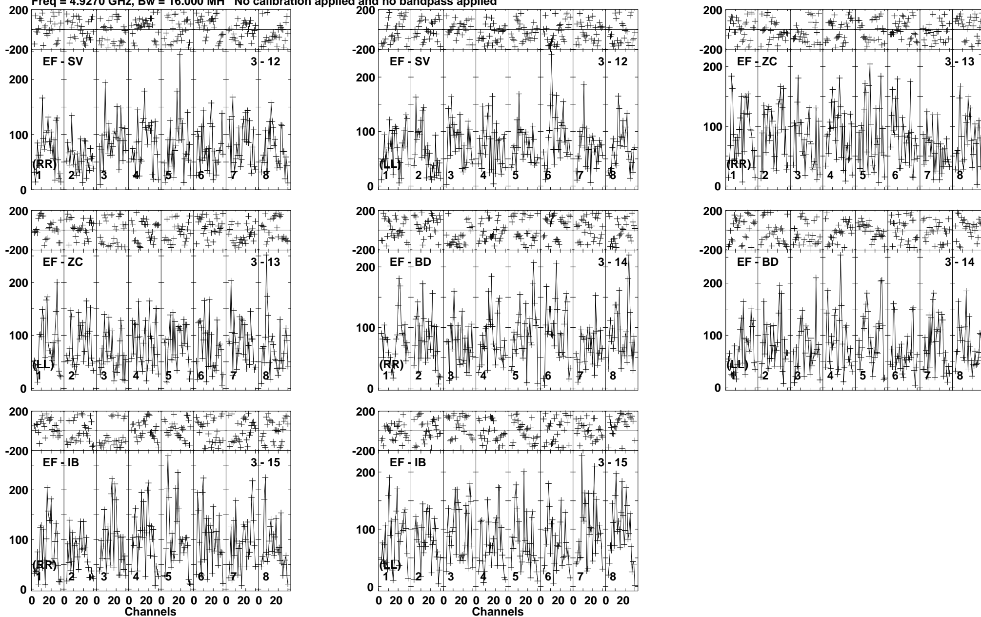
Lower frame: Micro Ampl Jy Top frame: Phas deg Vector averaged cross-power spectrum Baseline: EF (03) - SV (12) Timerange: 00/03:08:21 to 00/03:12:19
