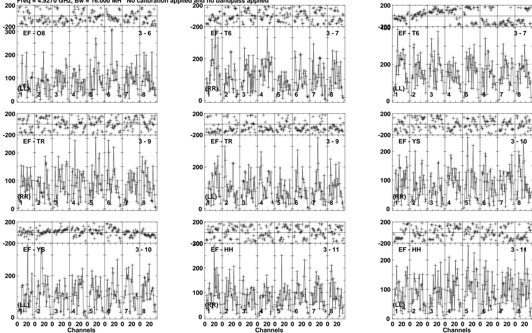
Lower frame: Micro Ampl Jy Top frame: Phas deg Vector averaged cross-power spectrum Baseline: EF (03) - O8 (06) Timerange: 00/02:45:41 to 00/02:49:39
