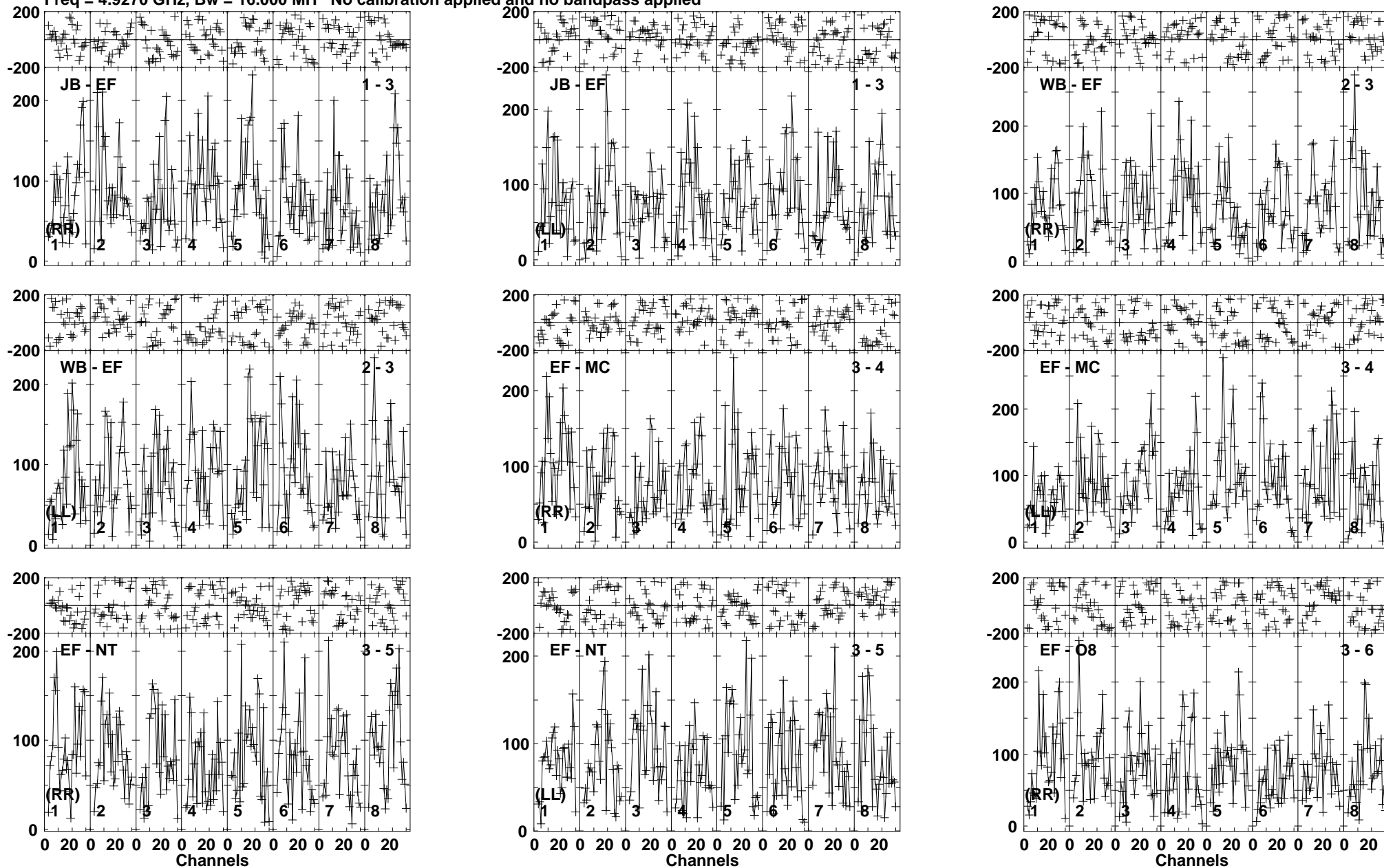
Lower frame: Micro Ampl Jy Top frame: Phas deg Vector averaged cross-power spectrum Baseline: JB (01) - EF (03) Timerange: 00/04:10:51 to 00/04:14:49
