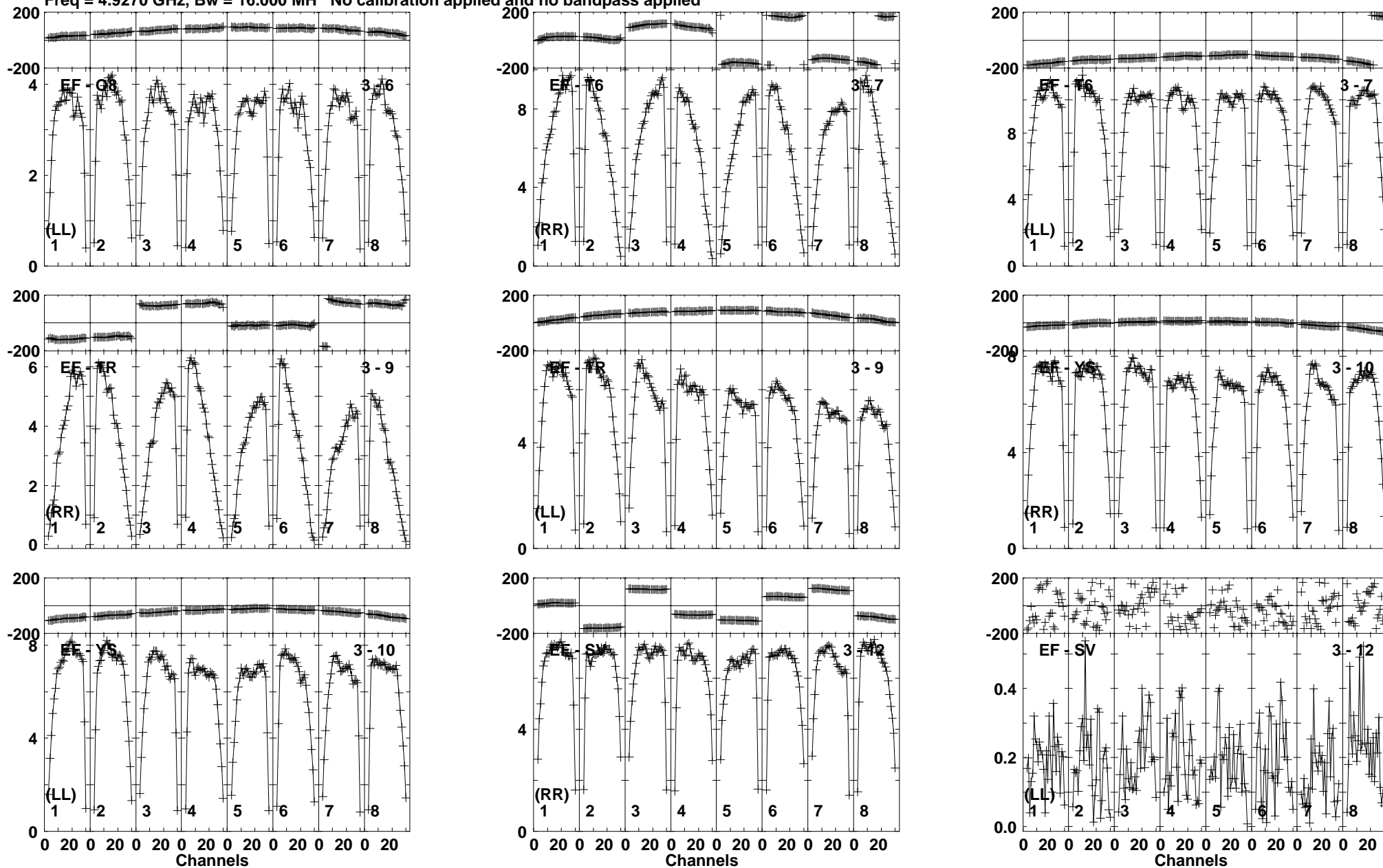
Lower frame: Milli Ampl Jy Top frame: Phas deg Vector averaged cross-power spectrum Baseline: EF (03) - O8 (06) Timerange: 00/02:10:11 to 00/02:11:39
