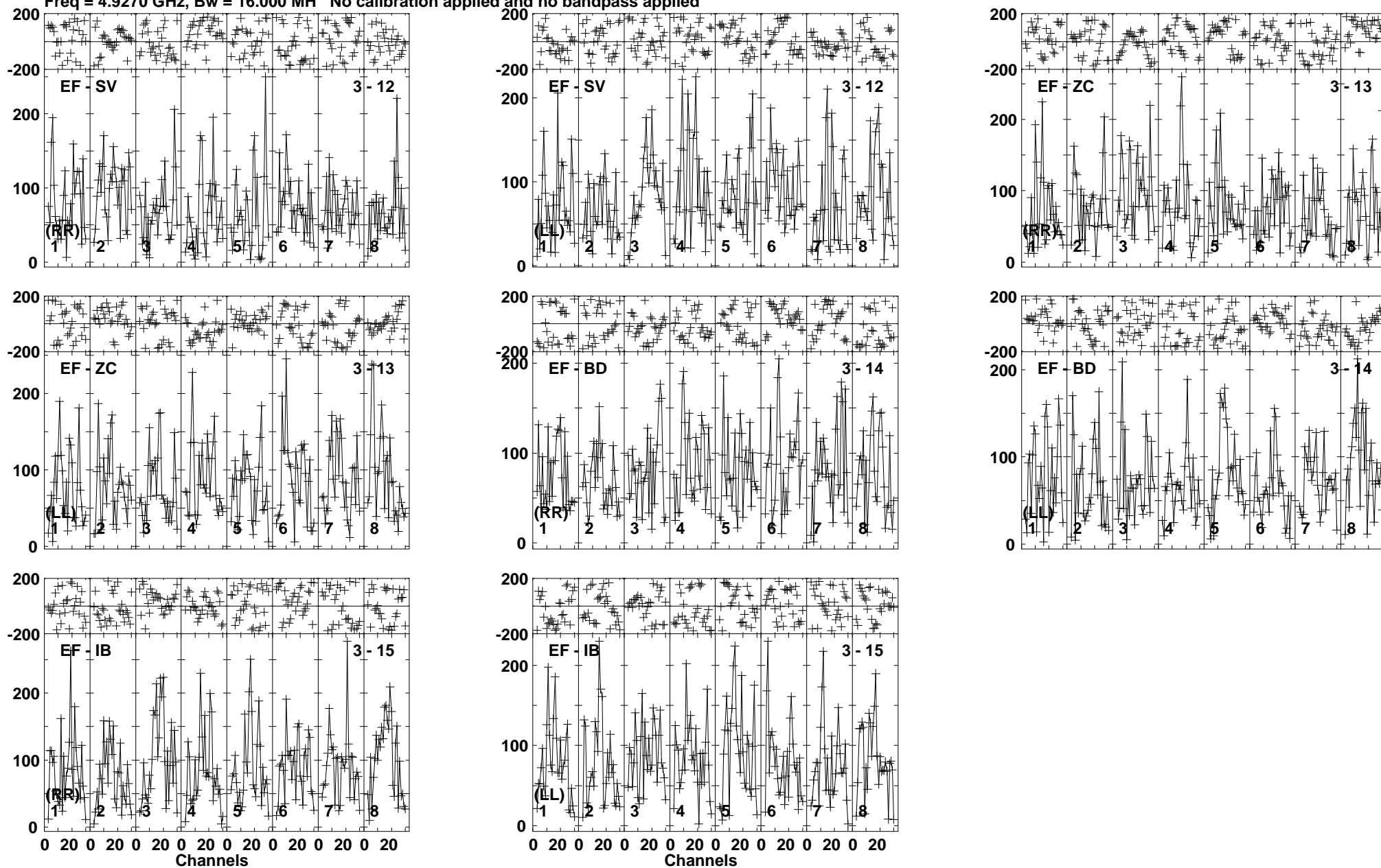
Lower frame: Micro Ampl Jy Top frame: Phas deg Vector averaged cross-power spectrum Baseline: EF (03) - SV (12) Timerange: 00/02:17:31 to 00/02:21:29
