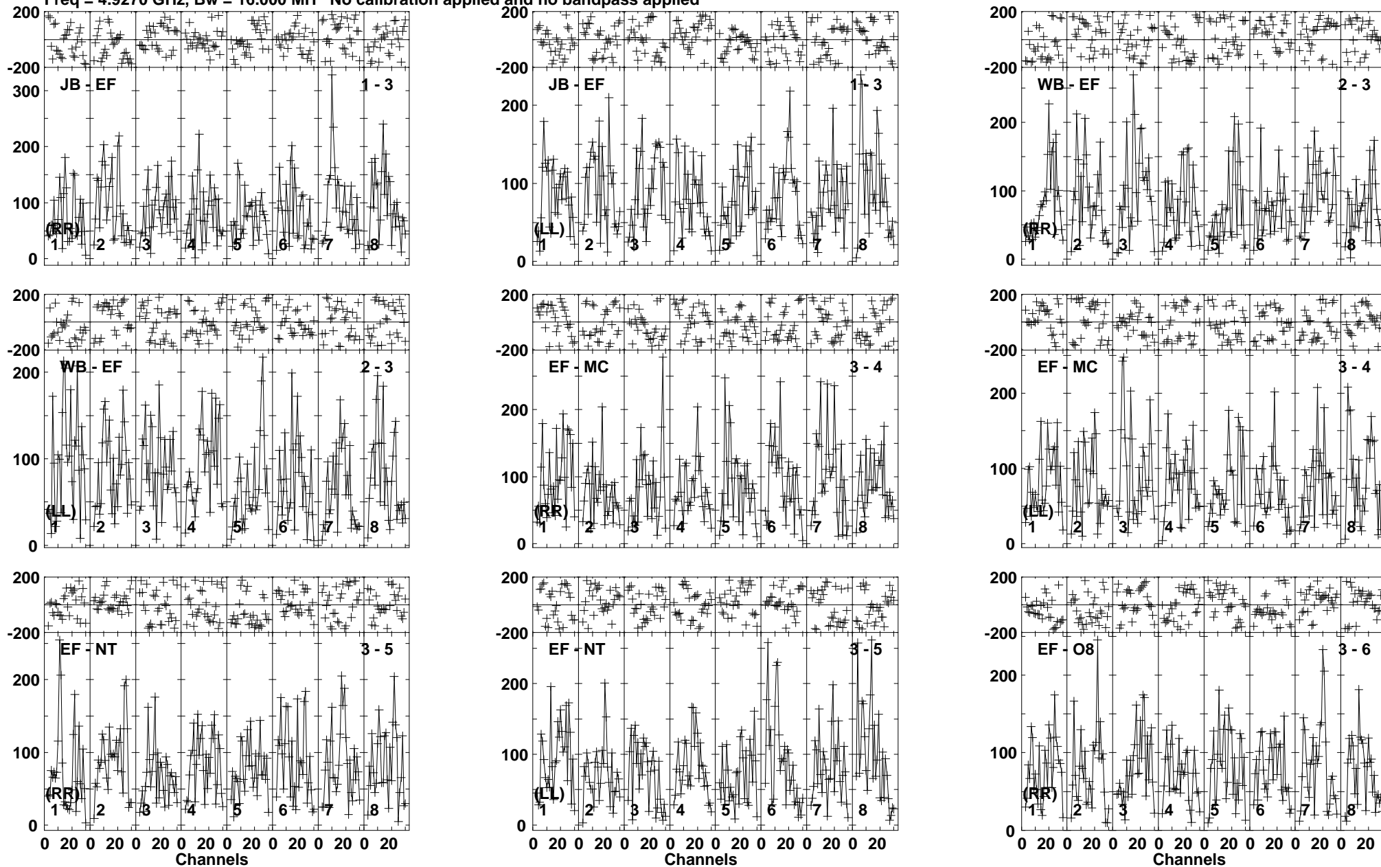
Lower frame: Micro Ampl Jy Top frame: Phas deg Vector averaged cross-power spectrum Baseline: JB (01) - EF (03) Timerange: 00/03:36:51 to 00/03:40:49
