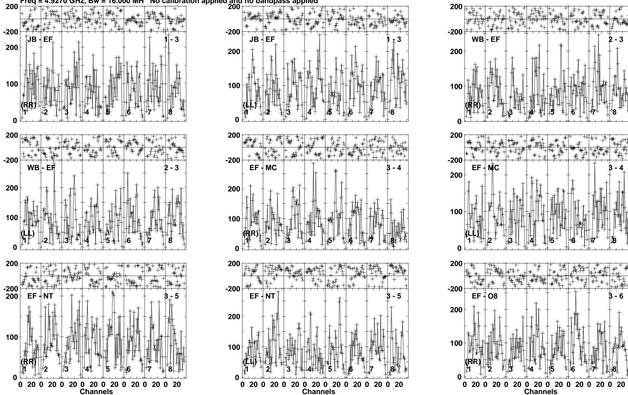
Lower frame: Micro Ampl Jy Top frame: Phas deg Vector averaged cross-power spectrum Baseline: JB (01) - EF (03) Timerange: 00/02:40:11 to 00/02:44:09
