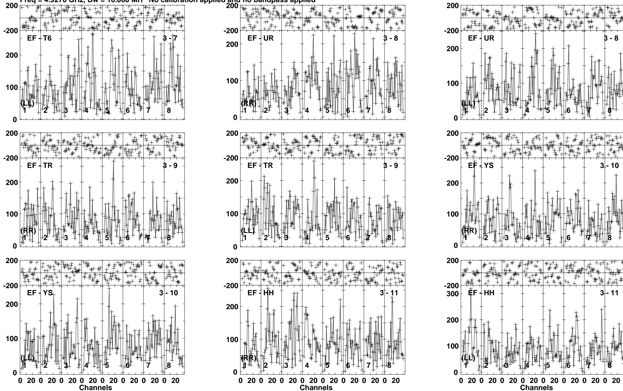
Lower frame: Micro Ampl Jy Top frame: Phas deg Vector averaged cross-power spectrum Baseline: EF (03) - T6 (07) Timerange: 00/09:27:01 to 00/09:30:59
