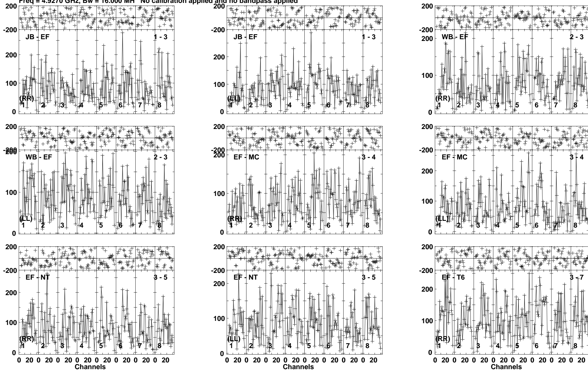
Lower frame: Micro Ampl Jy Top frame: Phas deg Vector averaged cross-power spectrum Baseline: JB (01) - EF (03) Timerange: 00/10:35:01 to 00/10:38:59
