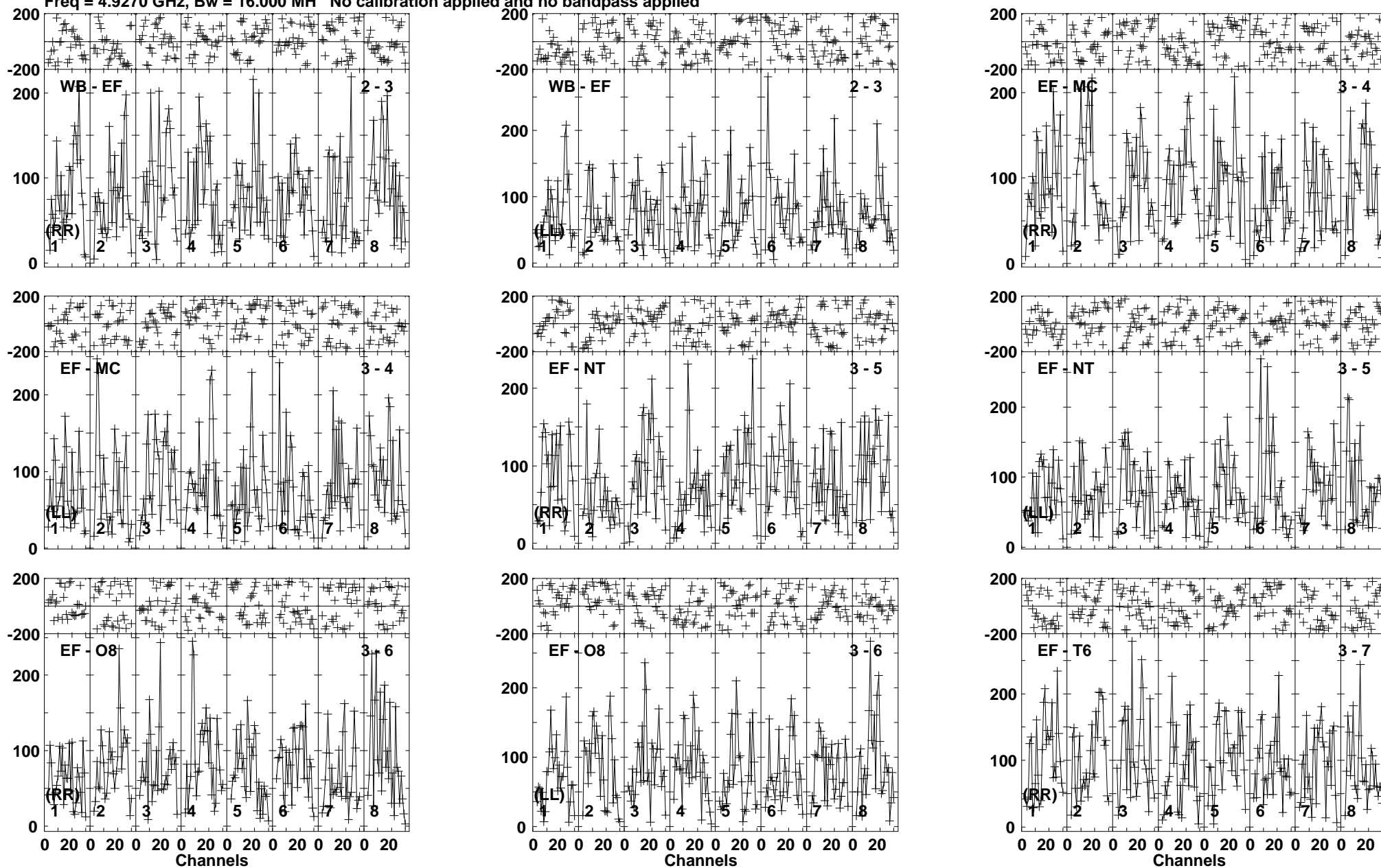
Lower frame: Micro Ampl Jy Top frame: Phas deg Vector averaged cross-power spectrum Baseline: WB (02) - EF (03) Timerange: 00/21:18:11 to 00/21:22:09
