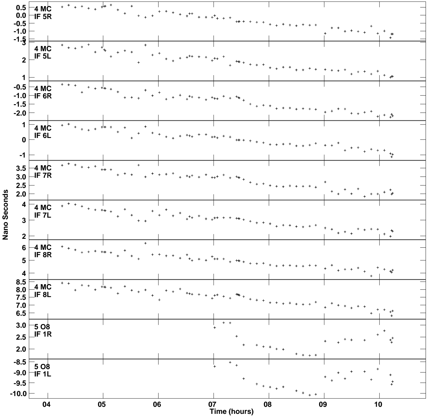
Plot file version 5 created 20-JAN-2020 15:48:19 Delay vs UTC time for EC070D.UVDATA.1 SN 2 Rpol & Lpol IF 1 - 8
