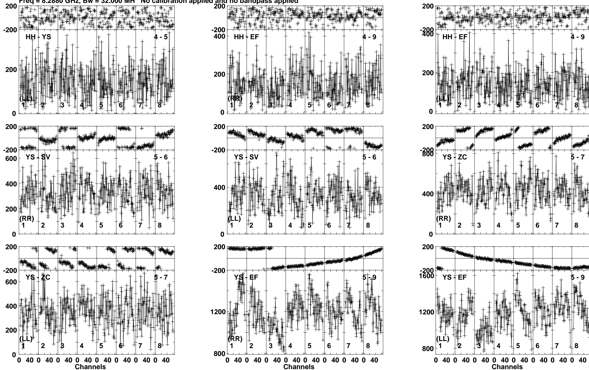
Lower frame: Micro Ampl Jy Top frame: Phas deg Vector averaged cross-power spectrum Baseline: HH (04) - YS (05) Timerange: 00/06:16:53 to 00/06:17:53
