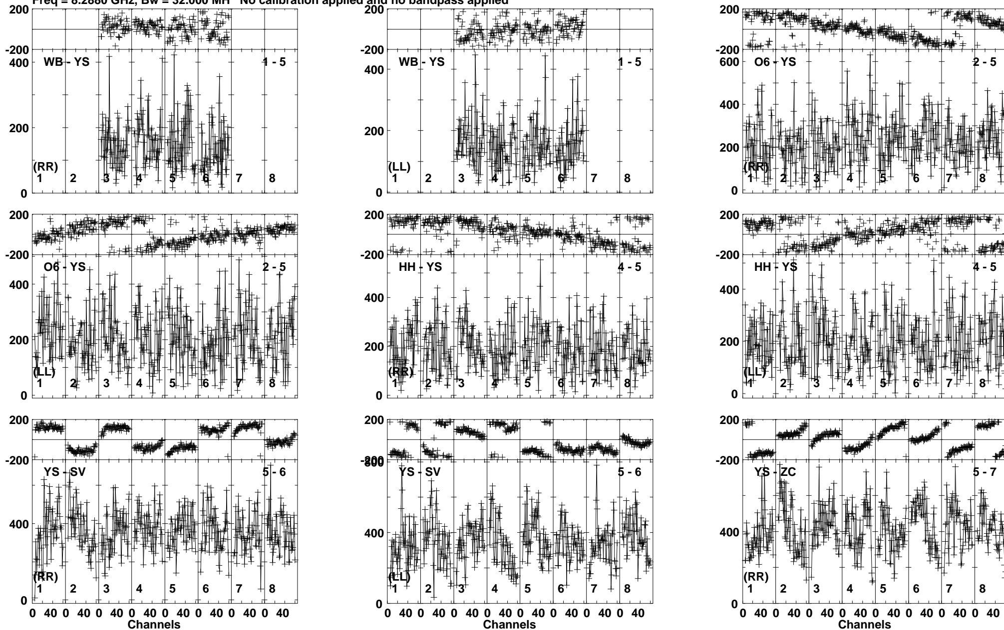
Lower frame: Micro Ampl Jy Top frame: Phas deg Vector averaged cross-power spectrum Baseline: WB (01) - YS (05) Timerange: 00/04:28:04 to 00/04:29:04
