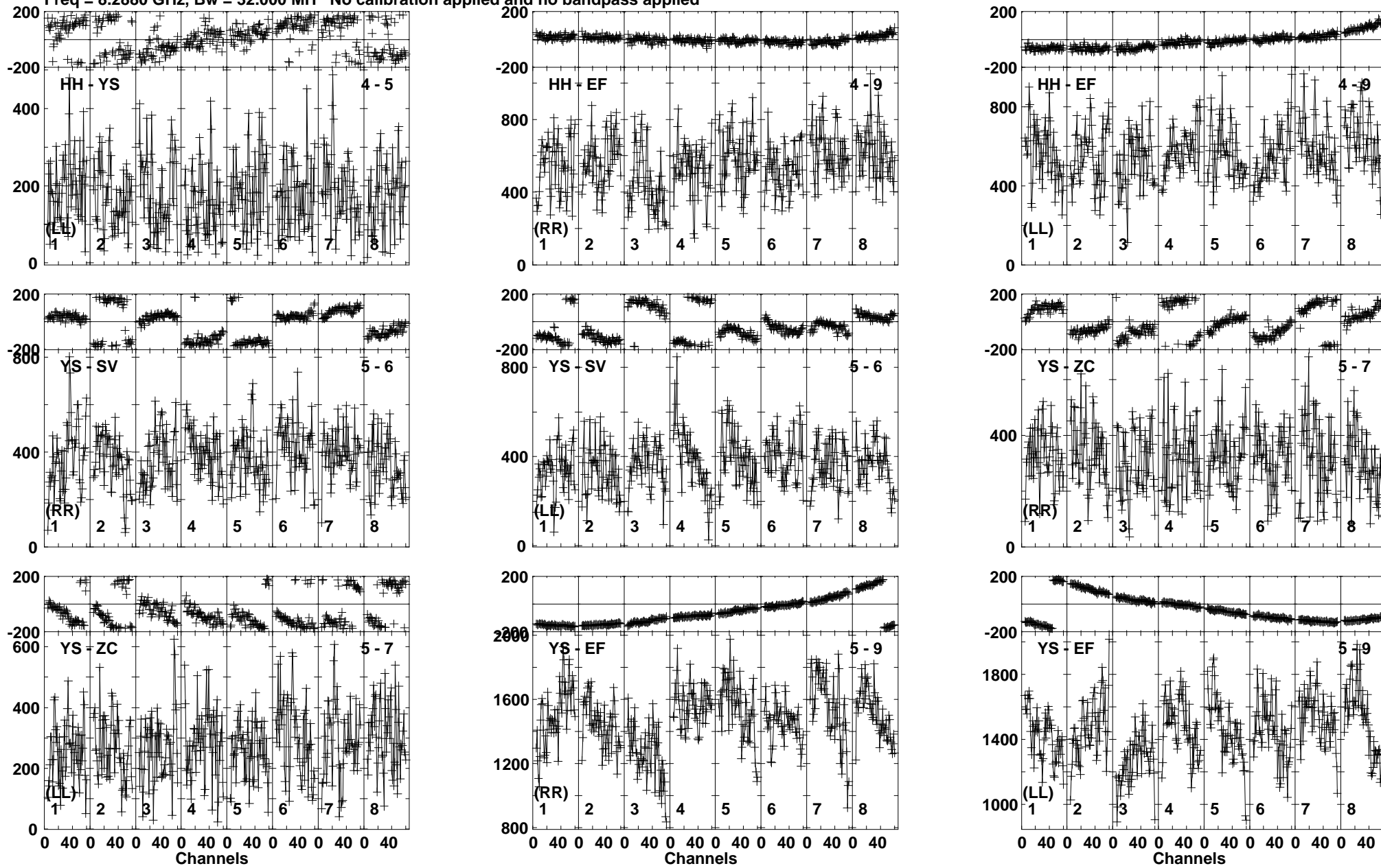
Lower frame: Micro Ampl Jy Top frame: Phas deg Vector averaged cross-power spectrum Baseline: HH (04) - YS (05) Timerange: 00/06:47:21 to 00/06:48:19
