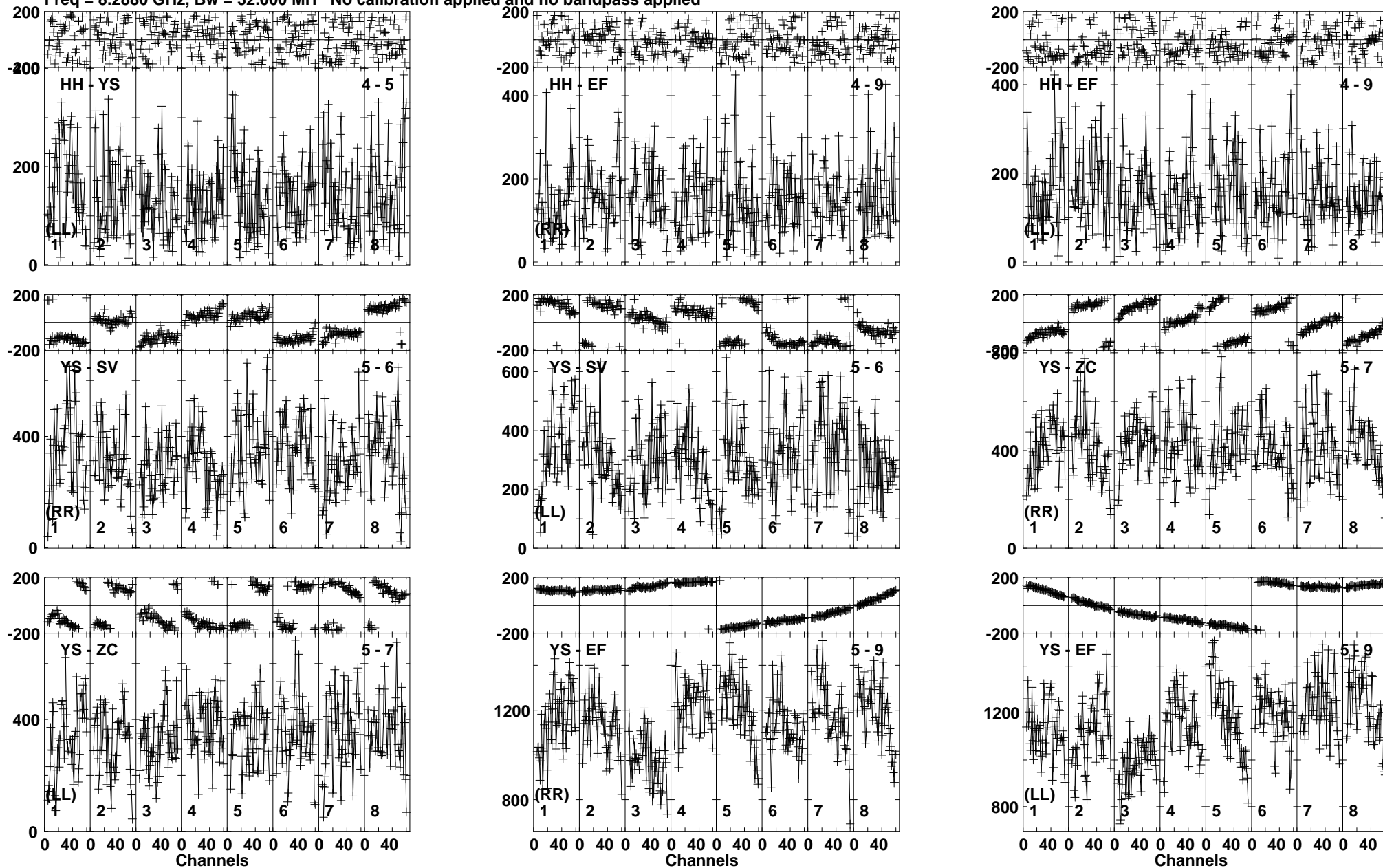
Lower frame: Micro Ampl Jy Top frame: Phas deg Vector average cross-power spectrum Baseline: HH (04) - YS (05) Timerange: 00/06:09:34 to 00/06:10:33
