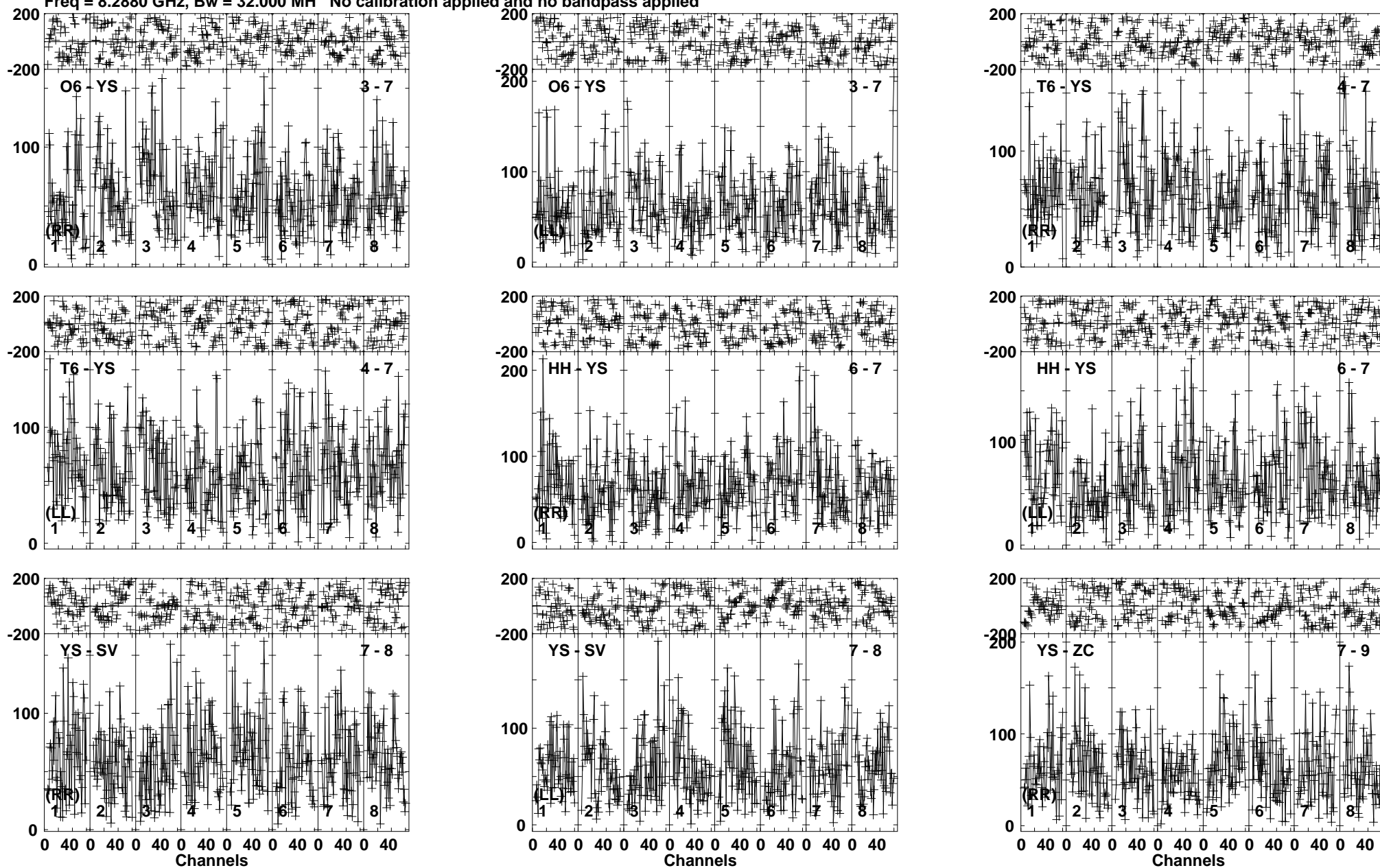
Lower frame: Micro Ampl Jy Top frame: Phas deg Vector averaged cross-power spectrum Baseline: O6 (03) - YS (07) Timerange: 00/15:20:12 to 00/15:25:11
