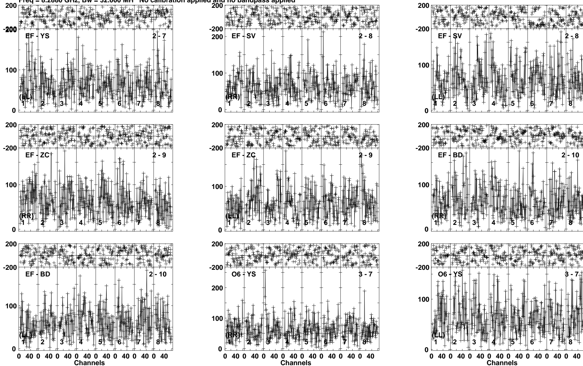
Lower frame: Micro Ampl Jy Top frame: Phas deg Vector averaged cross-power spectrum Baseline: EF (02) - YS (07) Timerange: 00/13:34:38 to 00/13:39:24
