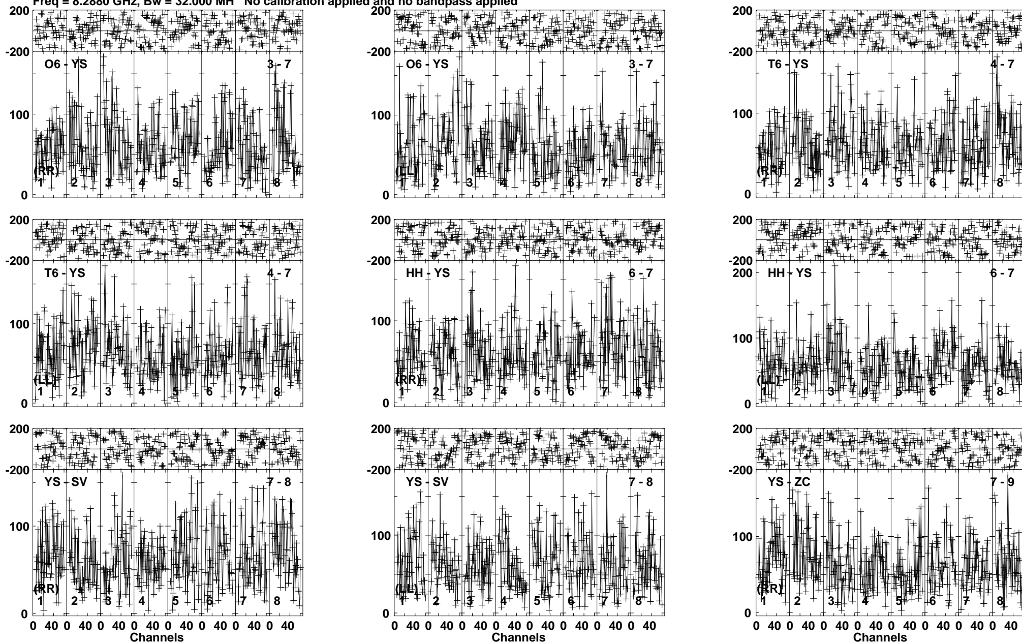
Lower frame: Micro Ampl Jy Top frame: Phas deg Vector averaged cross-power spectrum Baseline: O6 (03) - YS (07) Timerange: 00/14:43:33 to 00/14:48:32
