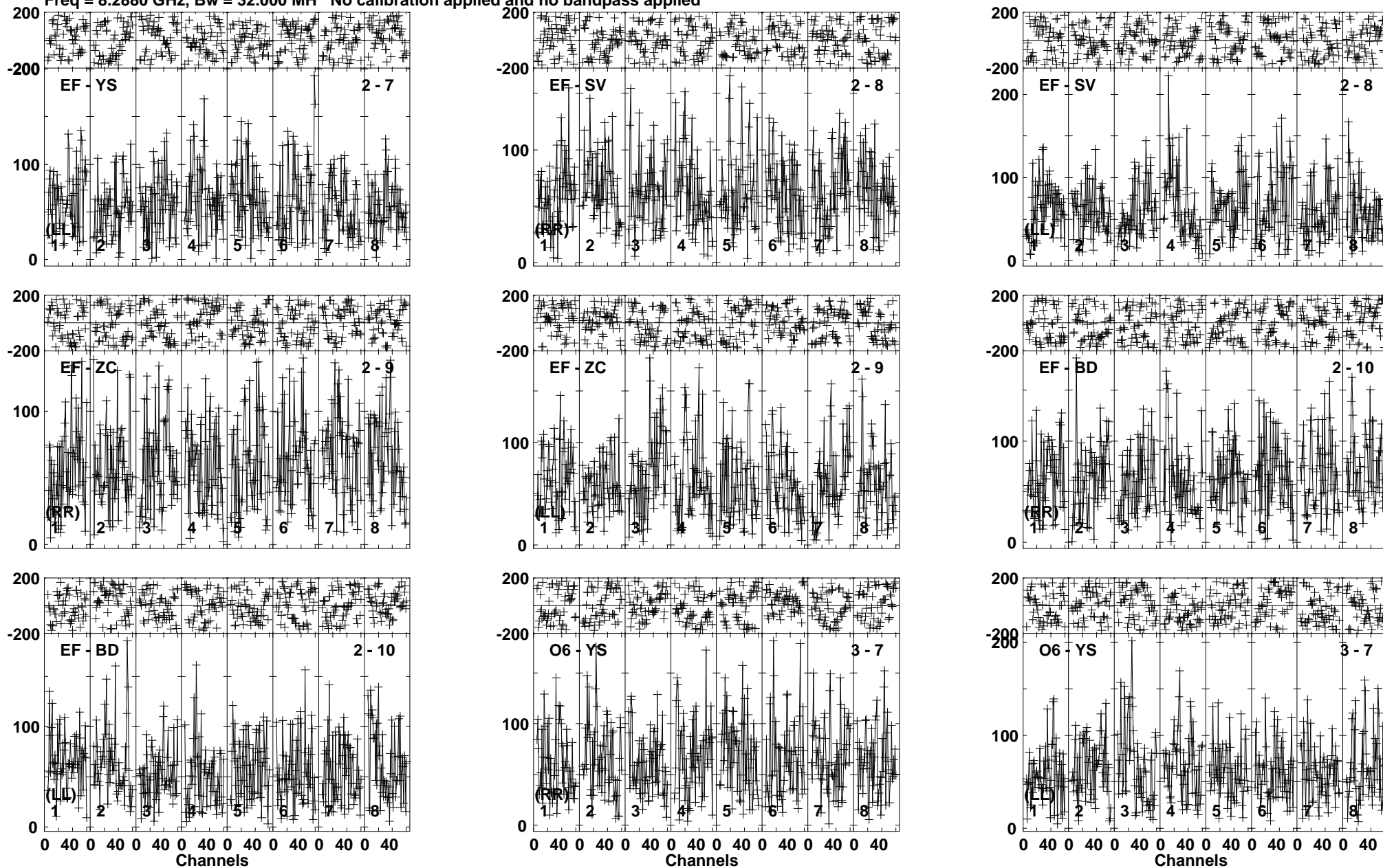
Lower frame: Micro Ampl Jy Top frame: Phas deg Vector averaged cross-power spectrum Baseline: EF (02) - YS (07) Timerange: 00/14:11:52 to 00/14:16:40
