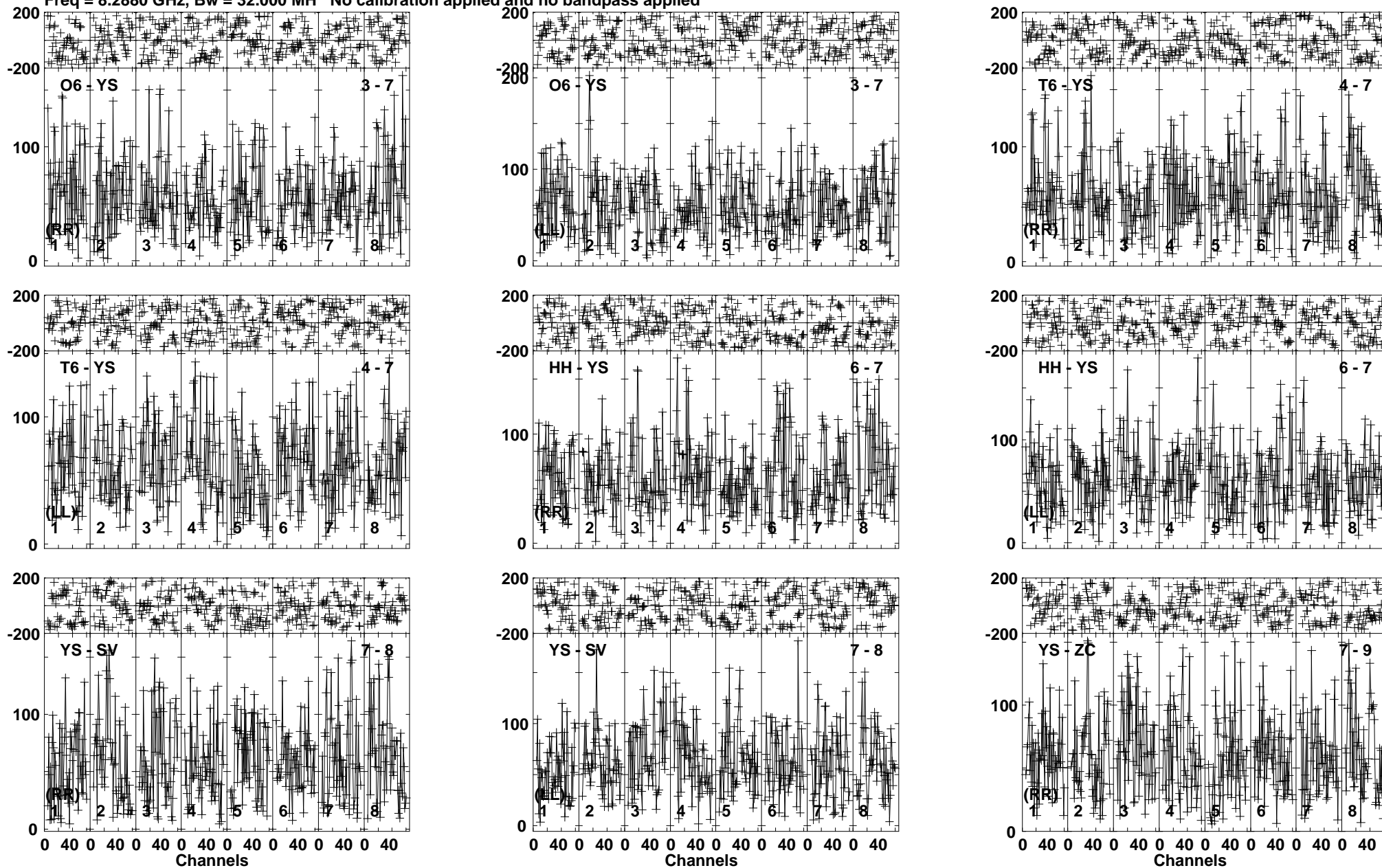
Lower frame: Micro Ampl Jy Top frame: Phas deg Vector averaged cross-power spectrum Baseline: O6 (03) - YS (07) Timerange: 00/15:34:52 to 00/15:39:51
