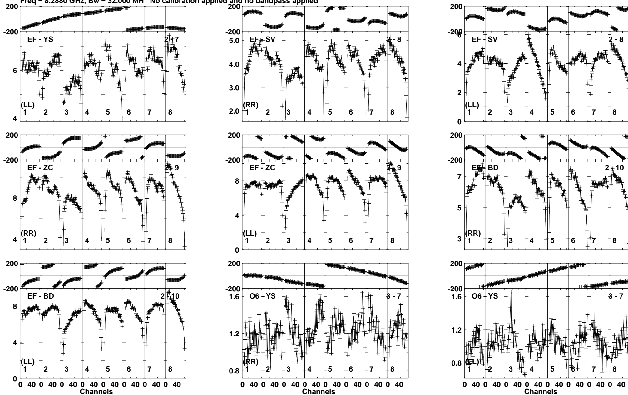
Lower frame: Milli Ampl Jy Top frame: Phas deg Vector averaged cross-power spectrum Baseline: EF (02) - YS (07) Timerange: 00:13:10:22 to 00:13:11:20
