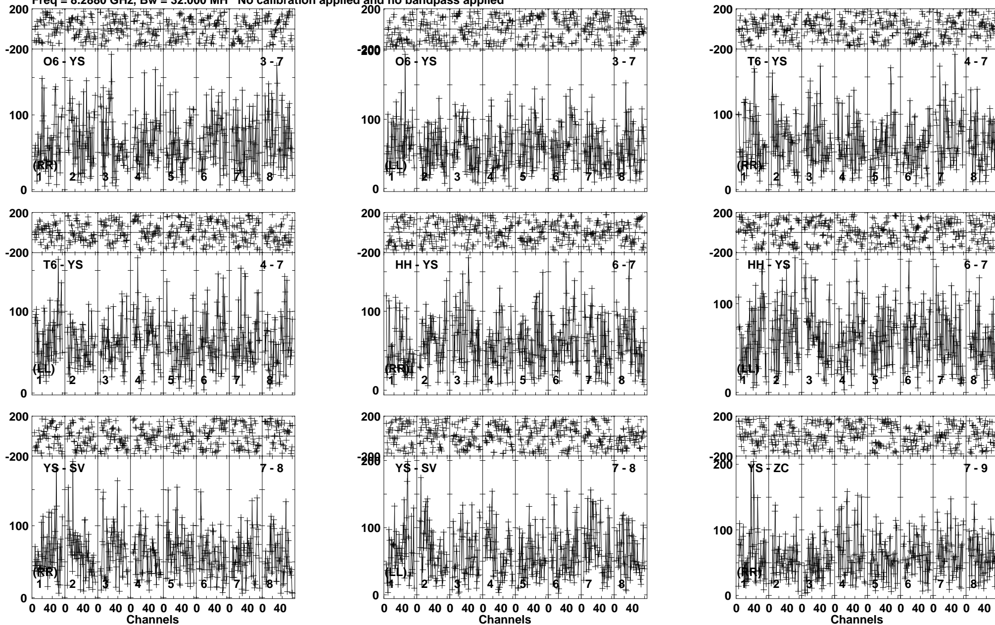
Lower frame: Micro Ampl Jy Top frame: Phas deg Vector averaged cross-power spectrum Baseline: O6 (03) - YS (07) Timerange: 00/15:05:33 to 00/15:10:32
