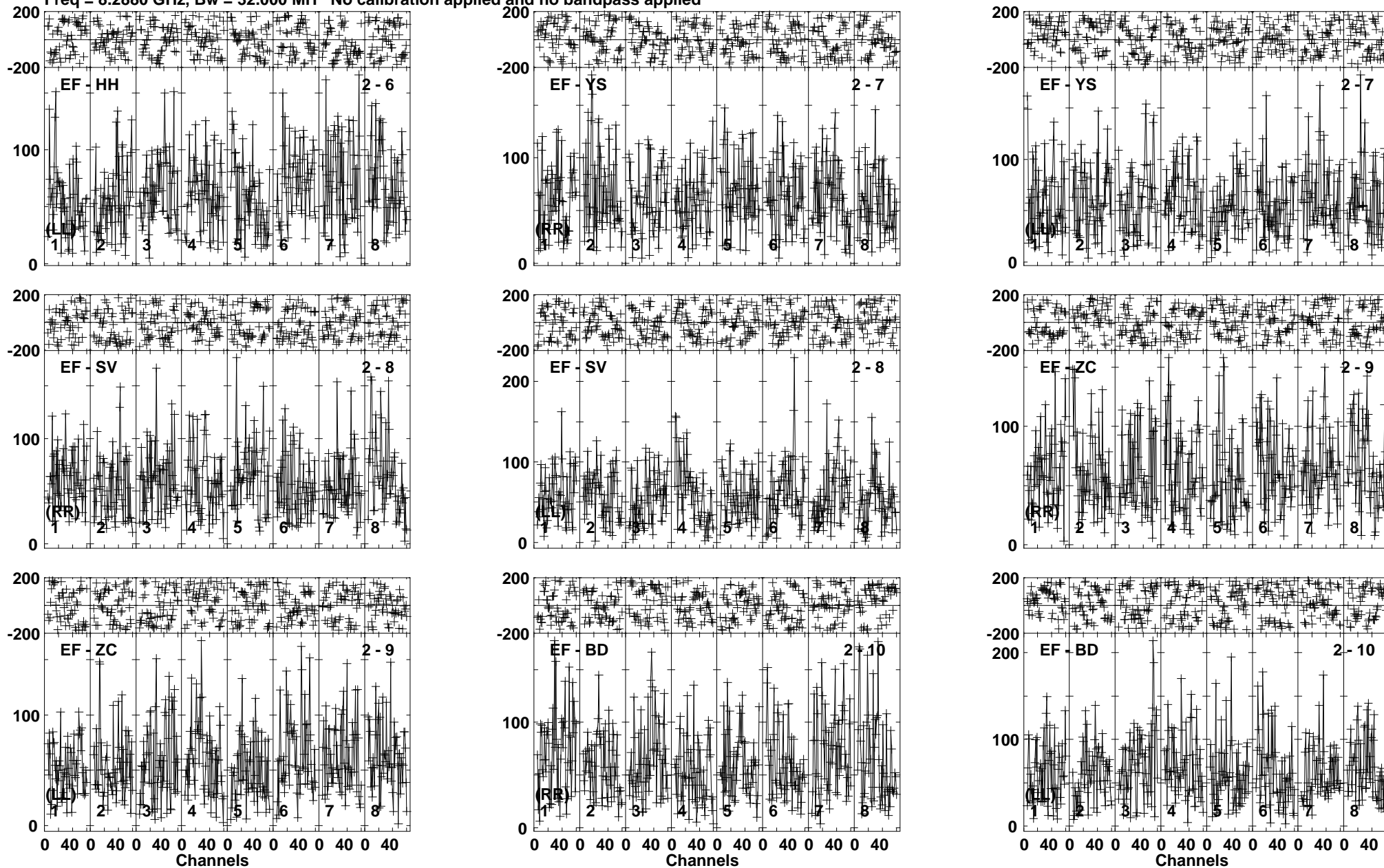
Lower frame: Micro Ampl Jy Top frame: Phas deg Vector averaged cross-power spectrum Baseline: EF (02) - HH (06) Timerange: 00/14:58:13 to 00/15:03:12
