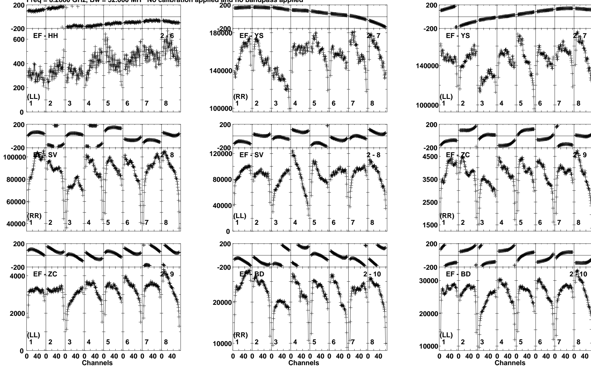
Lower frame: Micro Ampl Jy Top frame: Phas deg Vector averaged cross-power spectrum Baseline: EF (02) - HH (06) Timerange: 00/11:59:50 to 00/12:04:49
