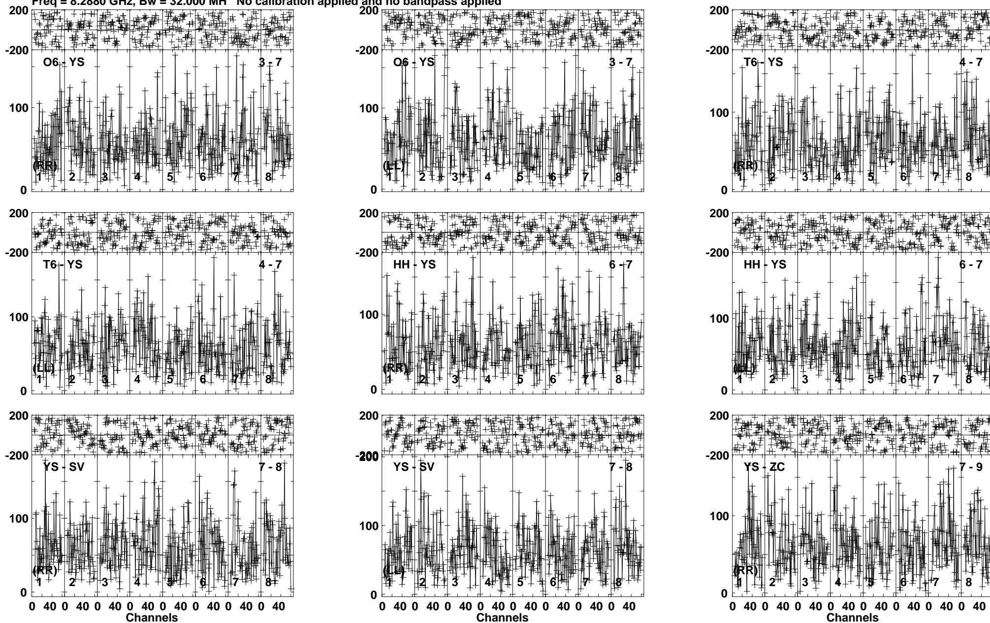
Lower frame: Micro Ampl Jy Top frame: Phas deg Vector averaged cross-power spectrum Baseline: O6 (03) - YS (07) Timerange: 00/14:50:52 to 00/14:55:51
