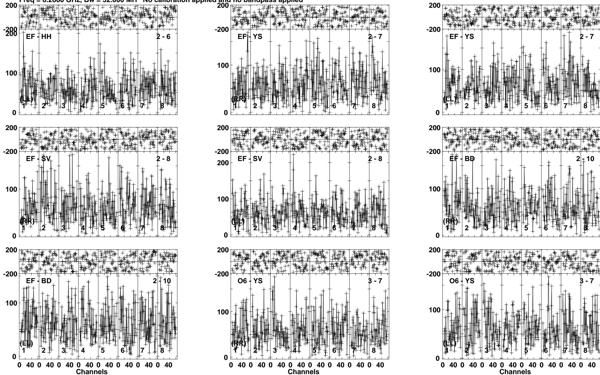
Lower frame: Micro Ampl Jy Top frame: Phas deg Vector averaged cross-power spectrum Baseline: EF (02) - HH (06) Timerange: 00/06:52:36 to 00/06:57:34
