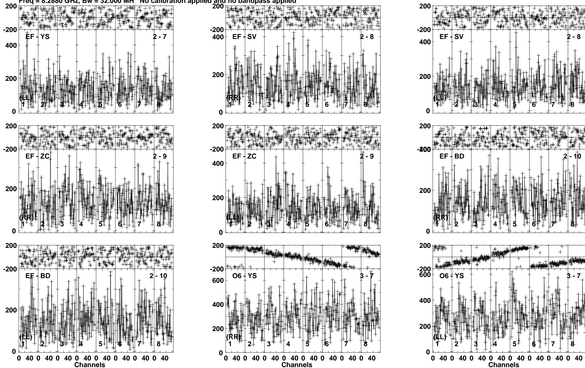
Lower frame: Micro Ampl Jy Top frame: Phas deg Vector averaged cross-power spectrum Baseline: EF (02) - YS (07) Timerange: 00/08:37:20 to 00/08:38:19
