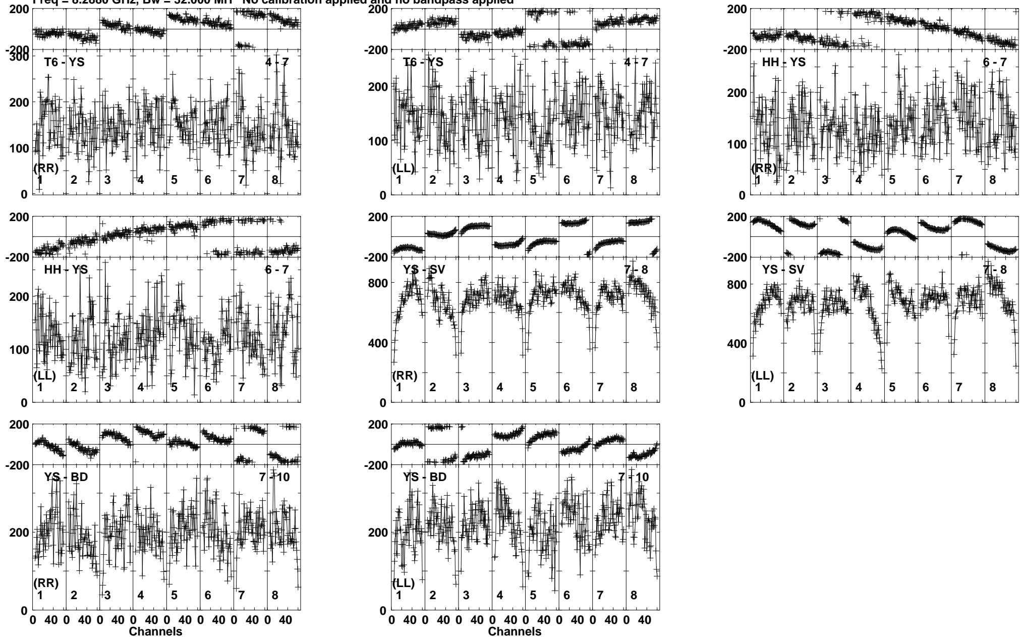
Lower frame: Micro Ampl Jy Top frame: Phas deg Vector averaged cross-power spectrum Baseline: T6 (04) - YS (07) Timerange: 00/06:37:36 to 00/06:42:34
