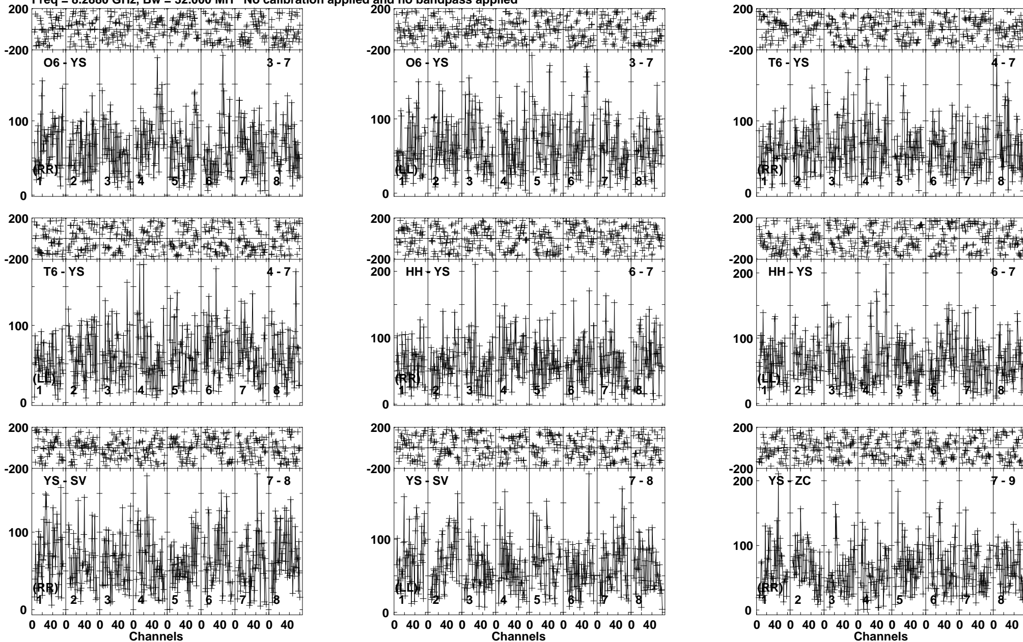
Lower frame: Micro Ampl Jy Top frame: Phas deg Vector averaged cross-power spectrum Baseline: O6 (03) - YS (07) Timerange: 00/05:51:06 to 00/05:55:49
