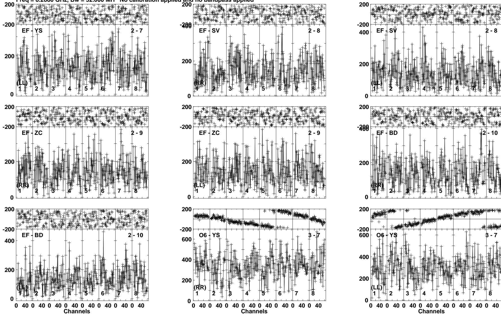
Lower frame: Micro Ampl Jy Top frame: Phas deg Vector averaged cross-power spectrum Baseline: EF (02) - YS (07) Timerange: 00/08:22:39 to 00/08:23:38
