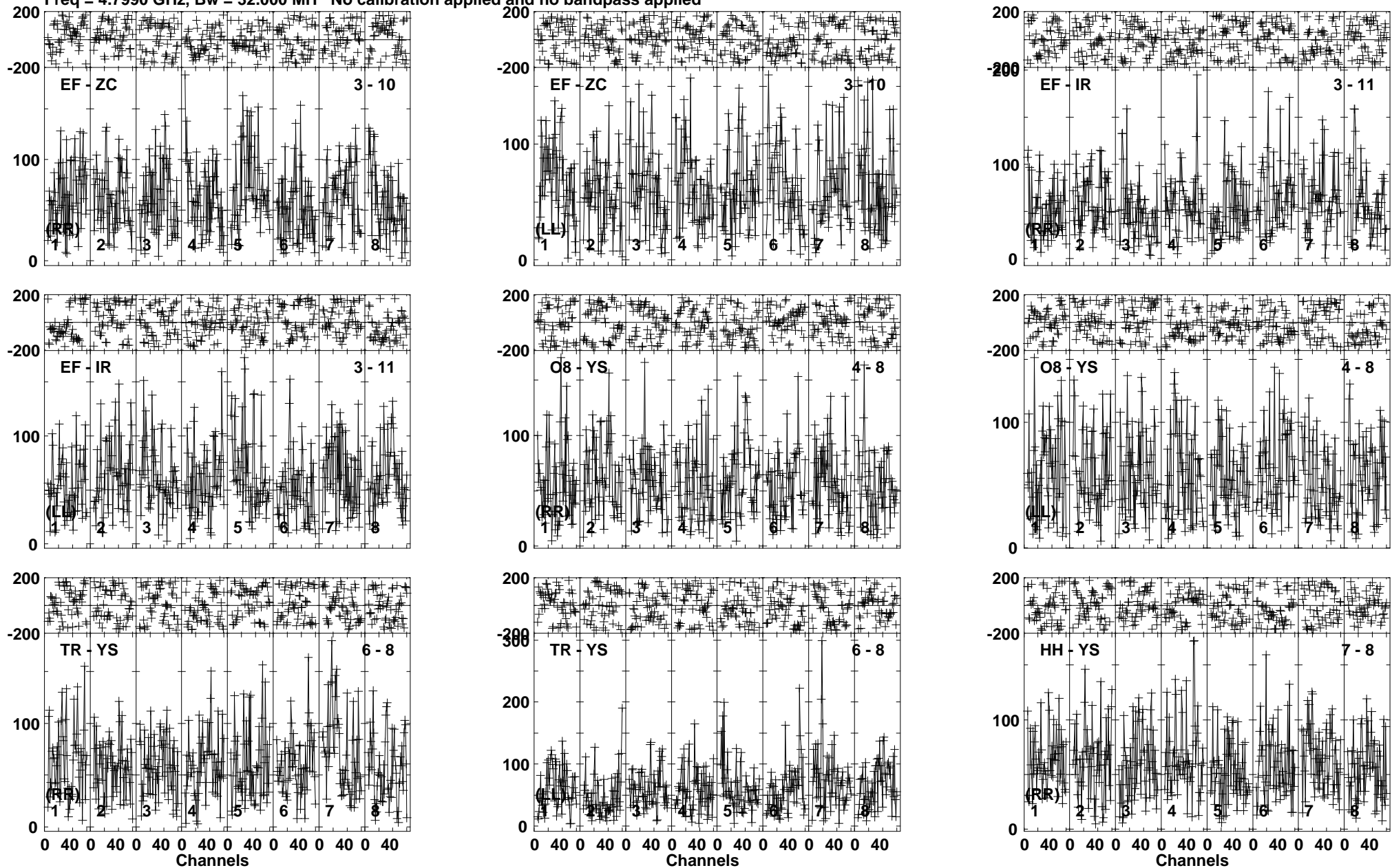
Lower frame: Micro Ampl Jy Top frame: Phas deg Vector averaged cross-power spectrum Baseline: EF (03) - ZC (10) Timerange: 00/04:37:25 to 00/04:42:24
