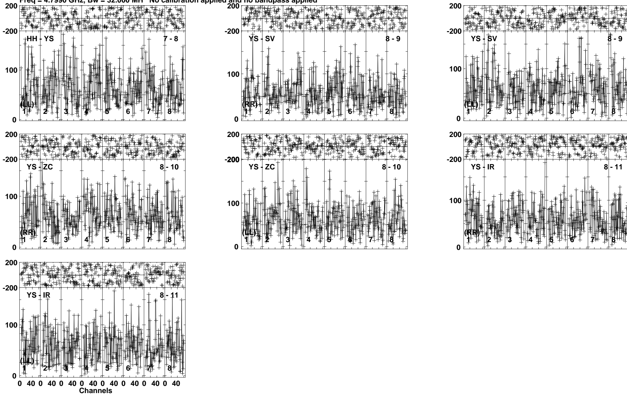
Lower frame: Micro Ampl Jy Top frame: Phas deg Vector averaged cross-power spectrum Baseline: HH (07) - YS (08) Timerange: 00/05:48:36 to 00/05:53:35
