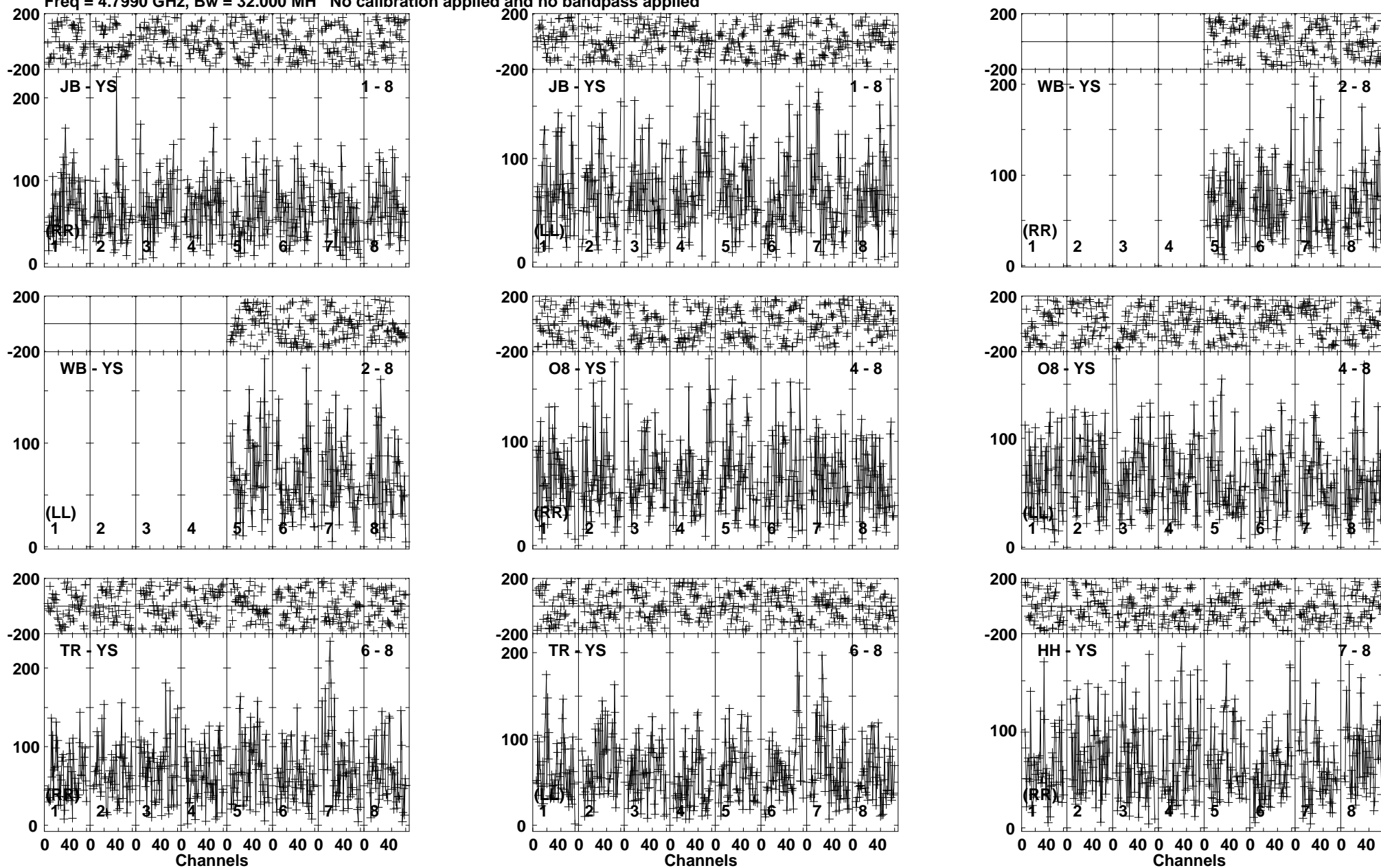
Lower frame: Micro Ampl Jy Top frame: Phas deg Vector averaged cross-power spectrum Baseline: JB (01) - YS (08) Timerange: 00/06:26:56 to 00/06:31:20
