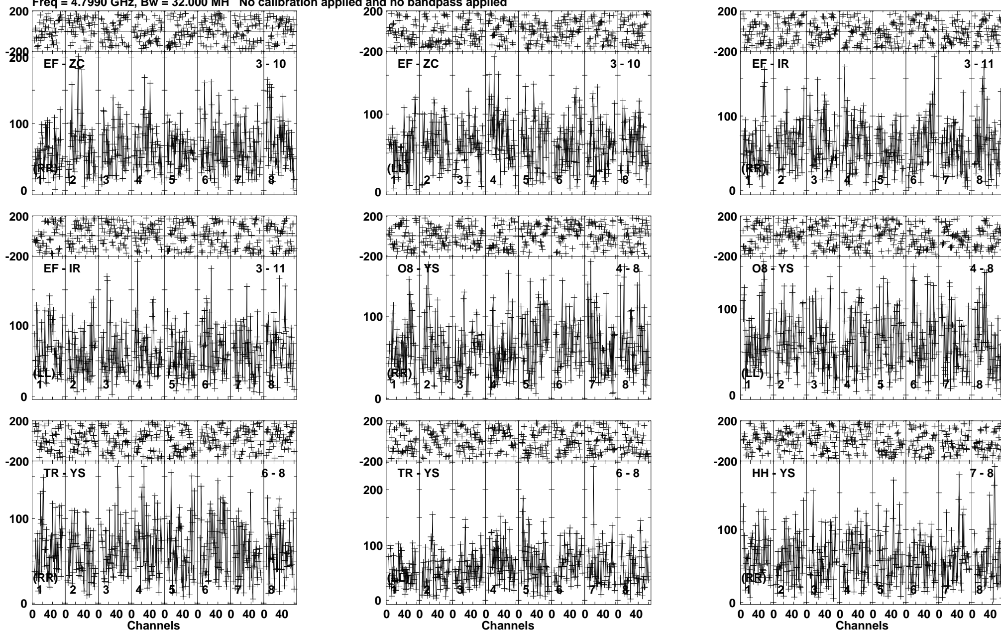
Lower frame: Micro Ampl Jy Top frame: Phas deg Vector averaged cross-power spectrum Baseline: EF (03) - ZC (10) Timerange: 00/05:15:46 to 00/05:20:45
