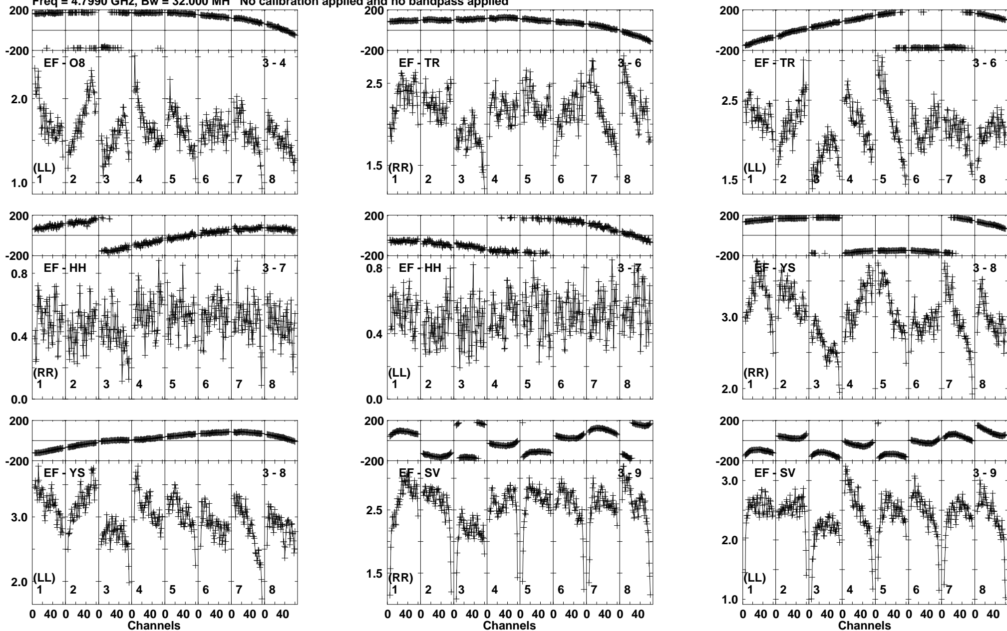
Lower frame: Milli Ampl Jy Top frame: Phas deg Vector averaged cross-power spectrum Baseline: EF (03) - O8 (04) Timerange: 00/07:08:40 to 00/07:09:40
