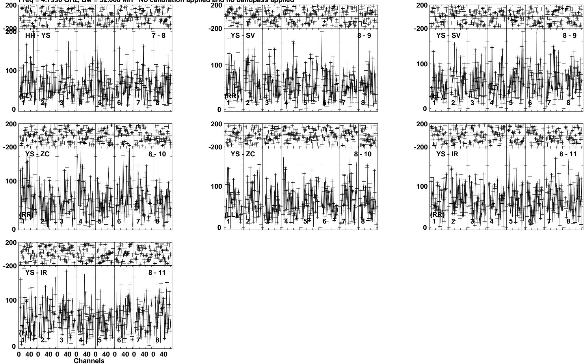
Lower frame: Micro Ampl Jy Top frame: Phas deg Vector averaged cross-power spectrum Baseline: HH (07) - YS (08) Timerange: 00/04:37:25 to 00/04:42:24
