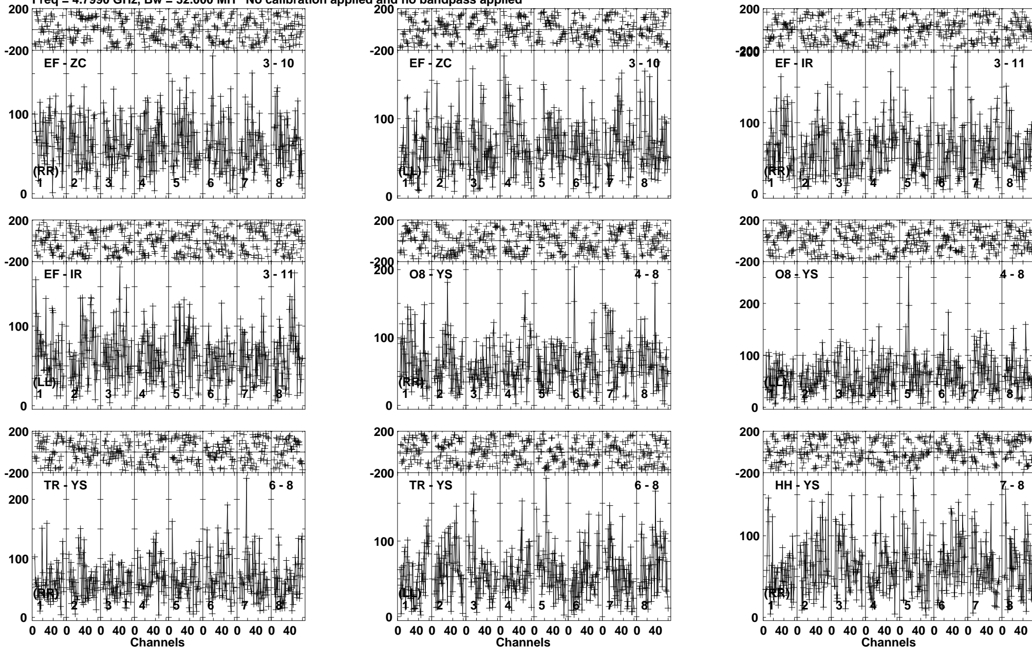
Lower frame: Micro Ampl Jy Top frame: Phas deg Vector averaged cross-power spectrum Baseline: EF (03) - ZC (10) Timerange: 00/07:10:21 to 00/07:15:20
