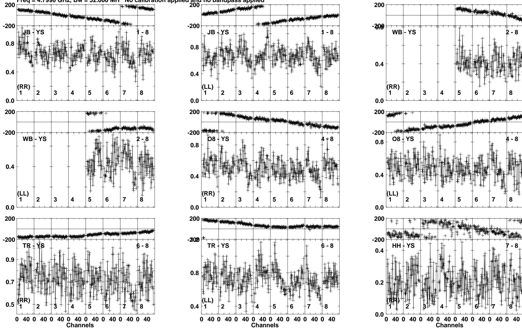
Lower frame: Milli Ampl Jy Top frame: Phas deg Vector averaged cross-power spectrum Baseline: JB (01) - YS (08) Timerange: 00/06:25:16 to 00/06:26:14
