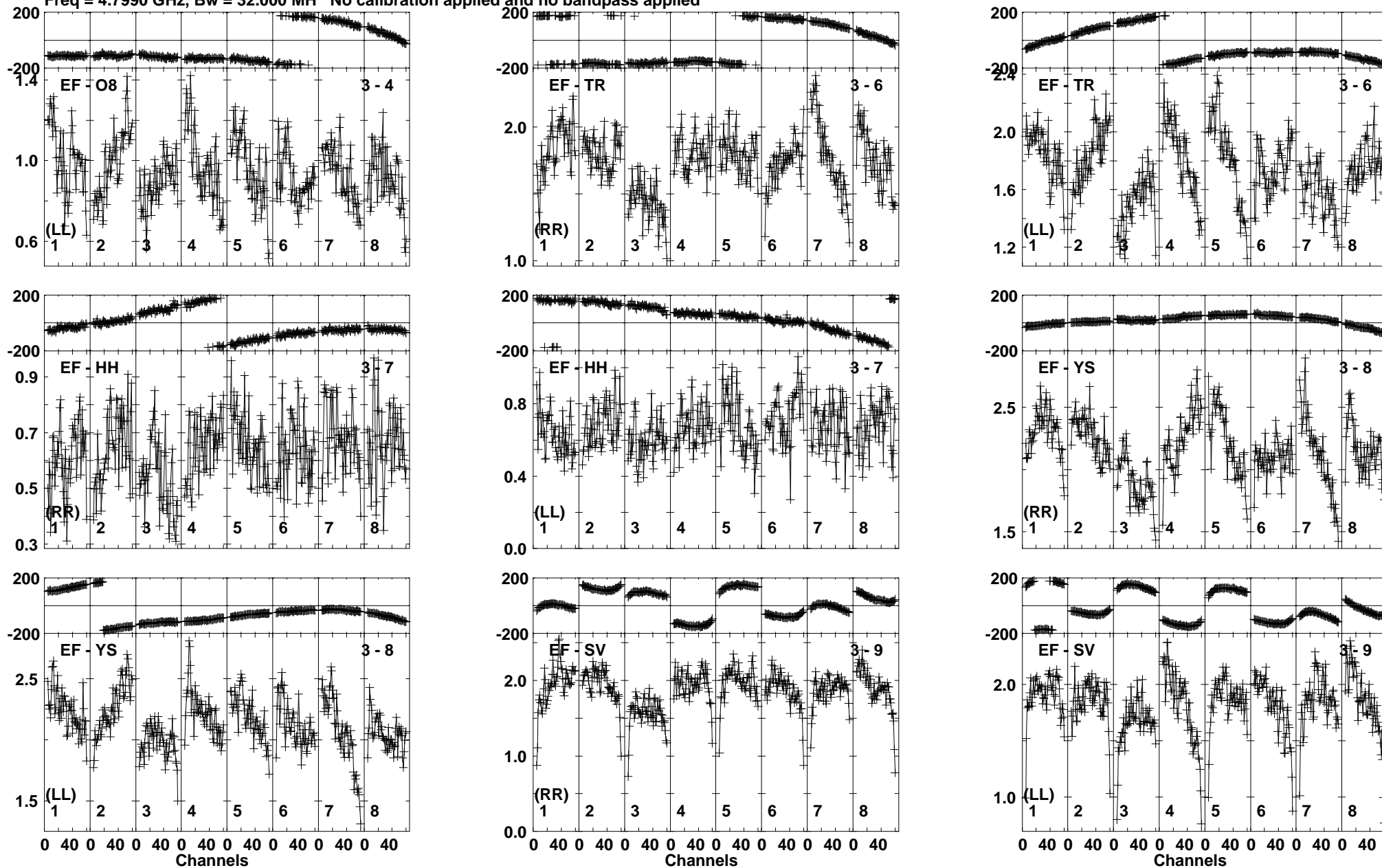
Lower frame: Milli Ampl Jy Top frame: Phas deg Vector averaged cross-power spectrum Baseline: EF (03) - O8 (04) Timerange: 00/04:12:04 to 00/04:13:02
