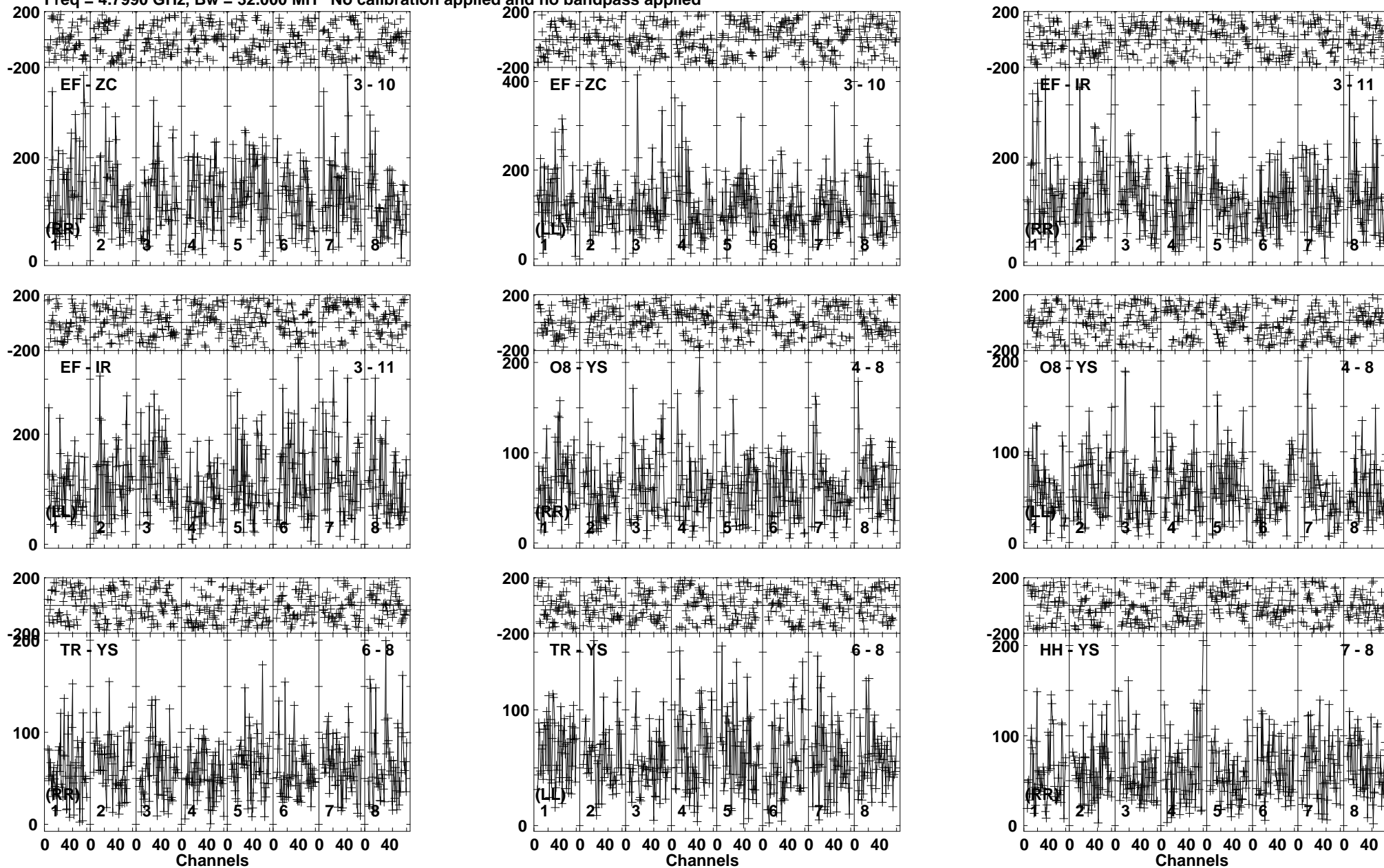
Lower frame: Micro Ampl Jy Top frame: Phas deg Vector averaged cross-power spectrum Baseline: EF (03) - ZC (10) Timerange: 00/05:33:15 to 00/05:38:14
