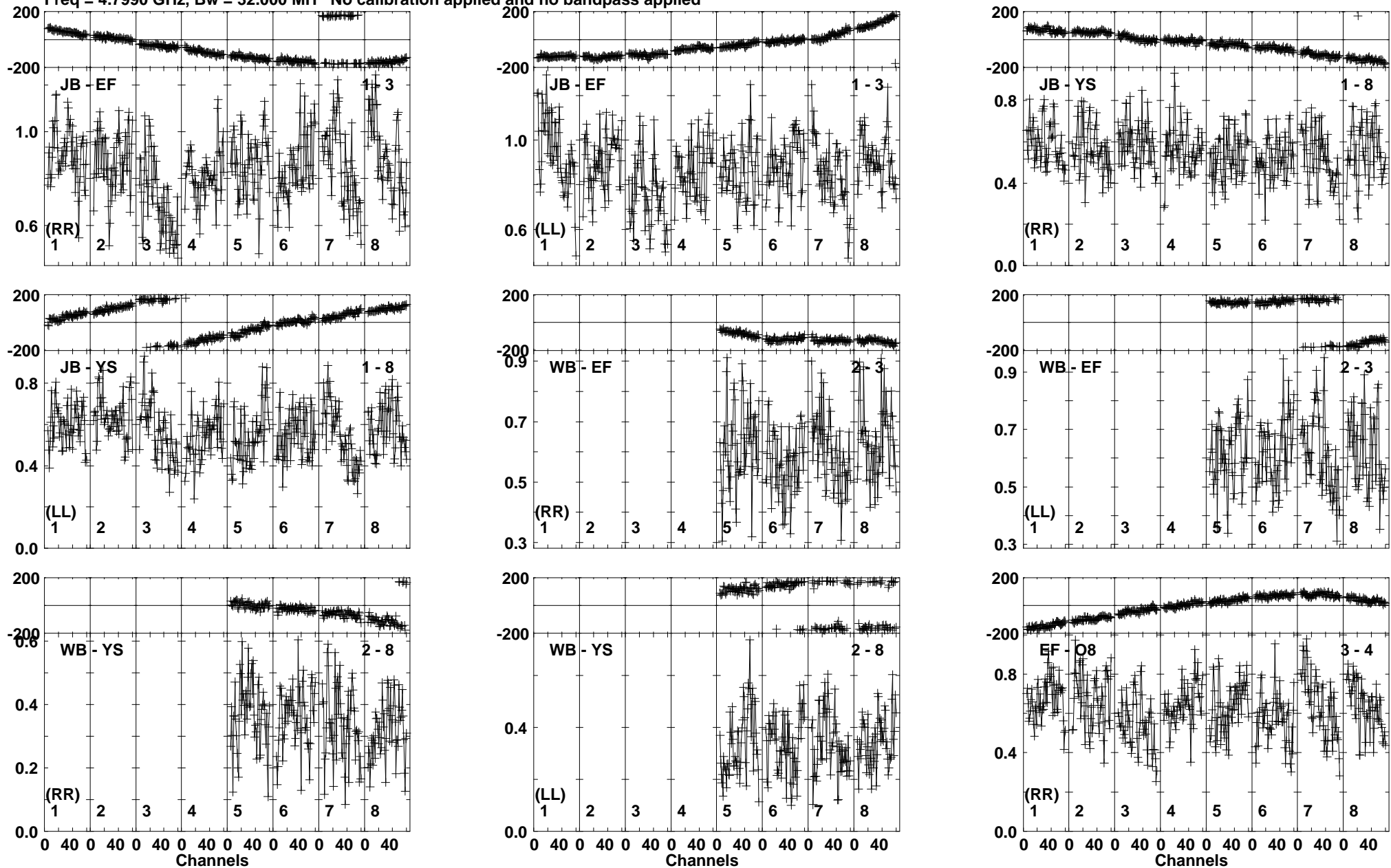
Lower frame: Milli Ampl Jy Top frame: Phas deg Vector averaged cross-power spectrum Baseline: JB (01) - EF (03) Timerange: 00/03:43:55 to 00/03:44:54
