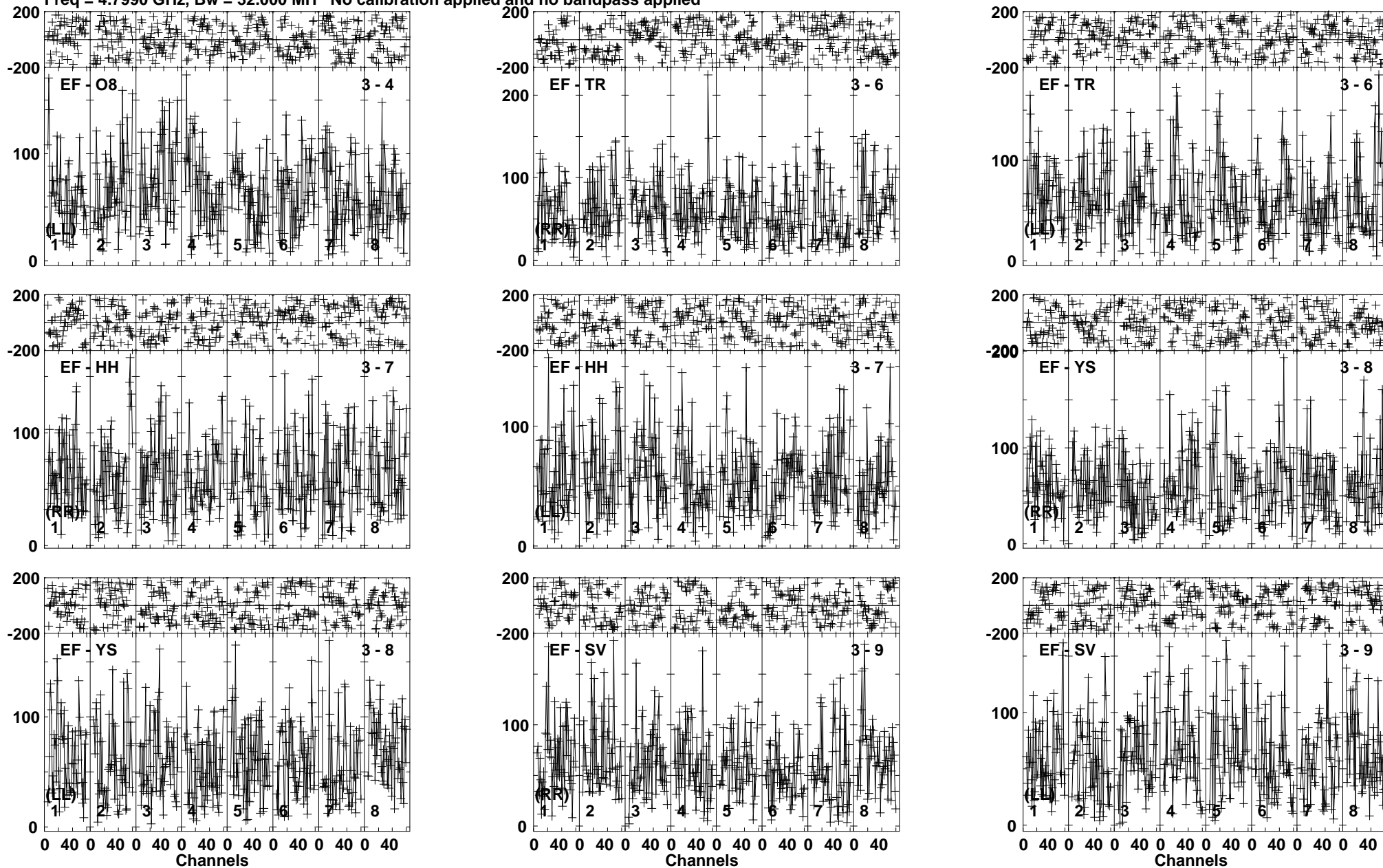
Lower frame: Micro Ampl Jy Top frame: Phas deg Vector averaged cross-power spectrum Baseline: EF (03) - O8 (04) Timerange: 00/06:48:20 to 00/06:53:19
