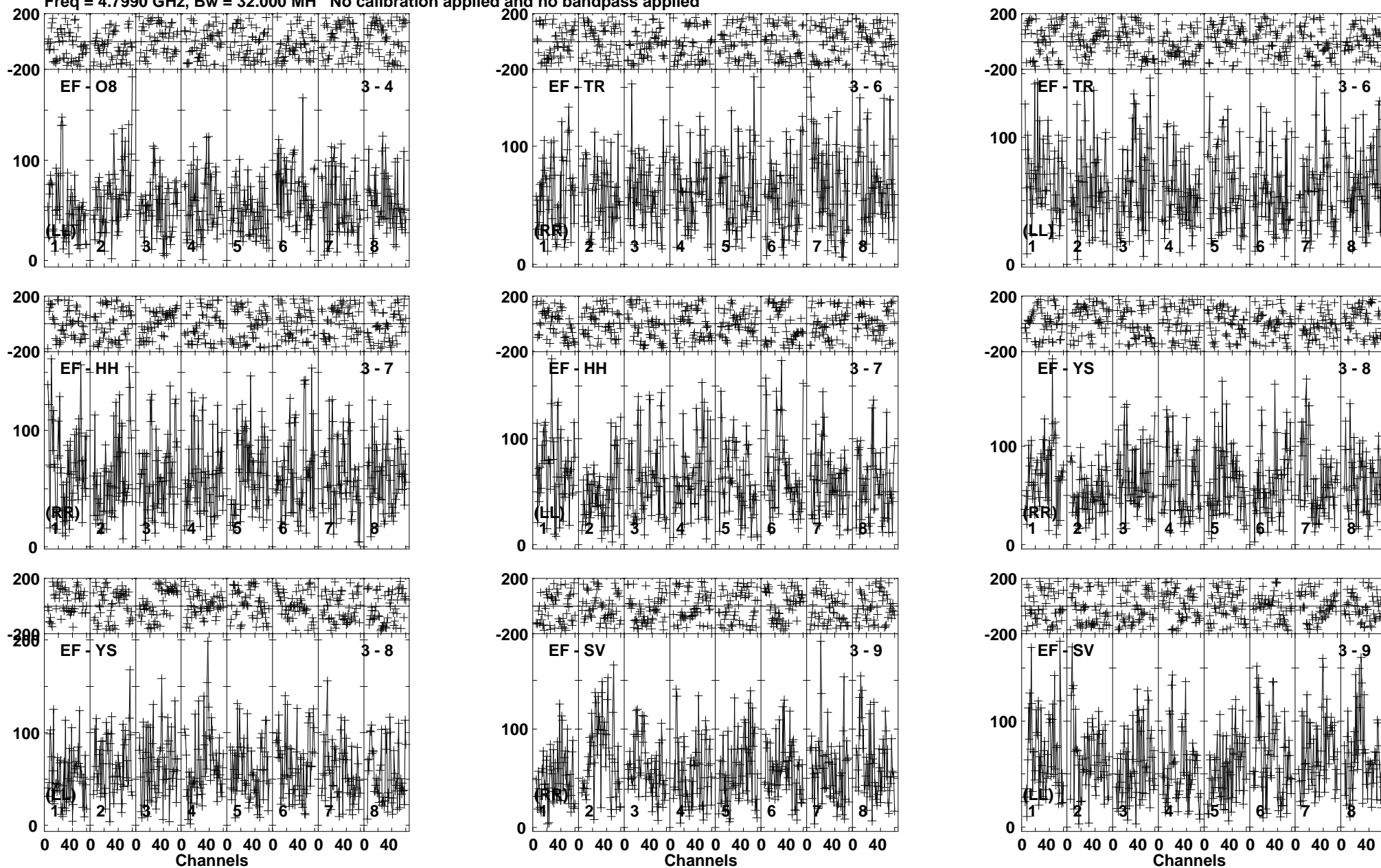
Lower frame: Micro Ampl Jy Top frame: Phas deg Vector averaged cross-power spectrum Baseline: EF (03) - O8 (04) Timerange: 00/05:56:16 to 00/06:01:15
