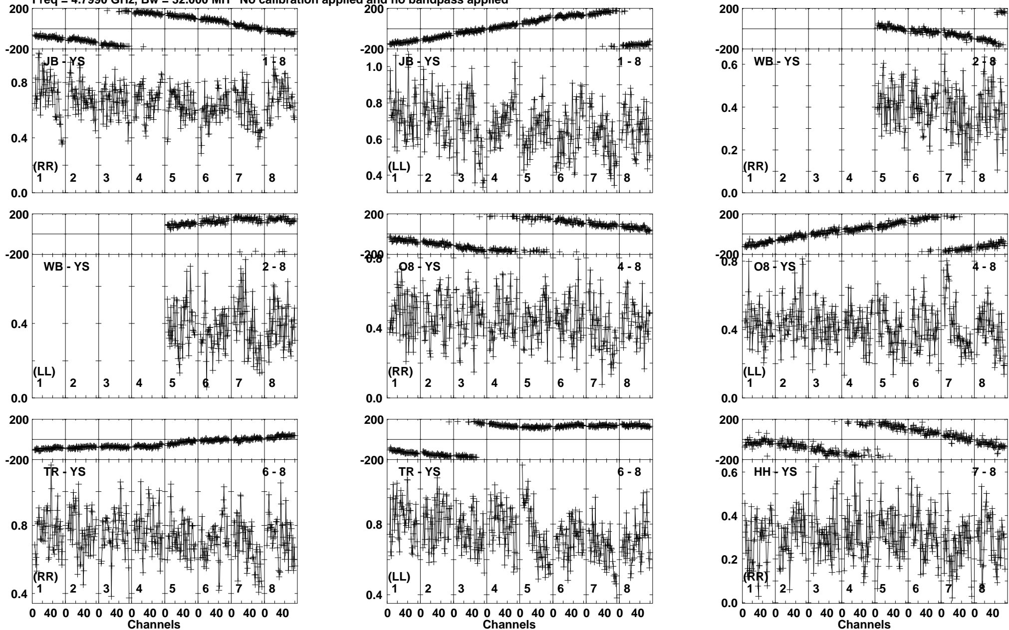
Lower frame: Milli Ampl Jy Top frame: Phas deg Vector averaged cross-power spectrum Baseline: JB (01) - YS (08) Timerange: 00/04:43:15 to 00/04:44:14
