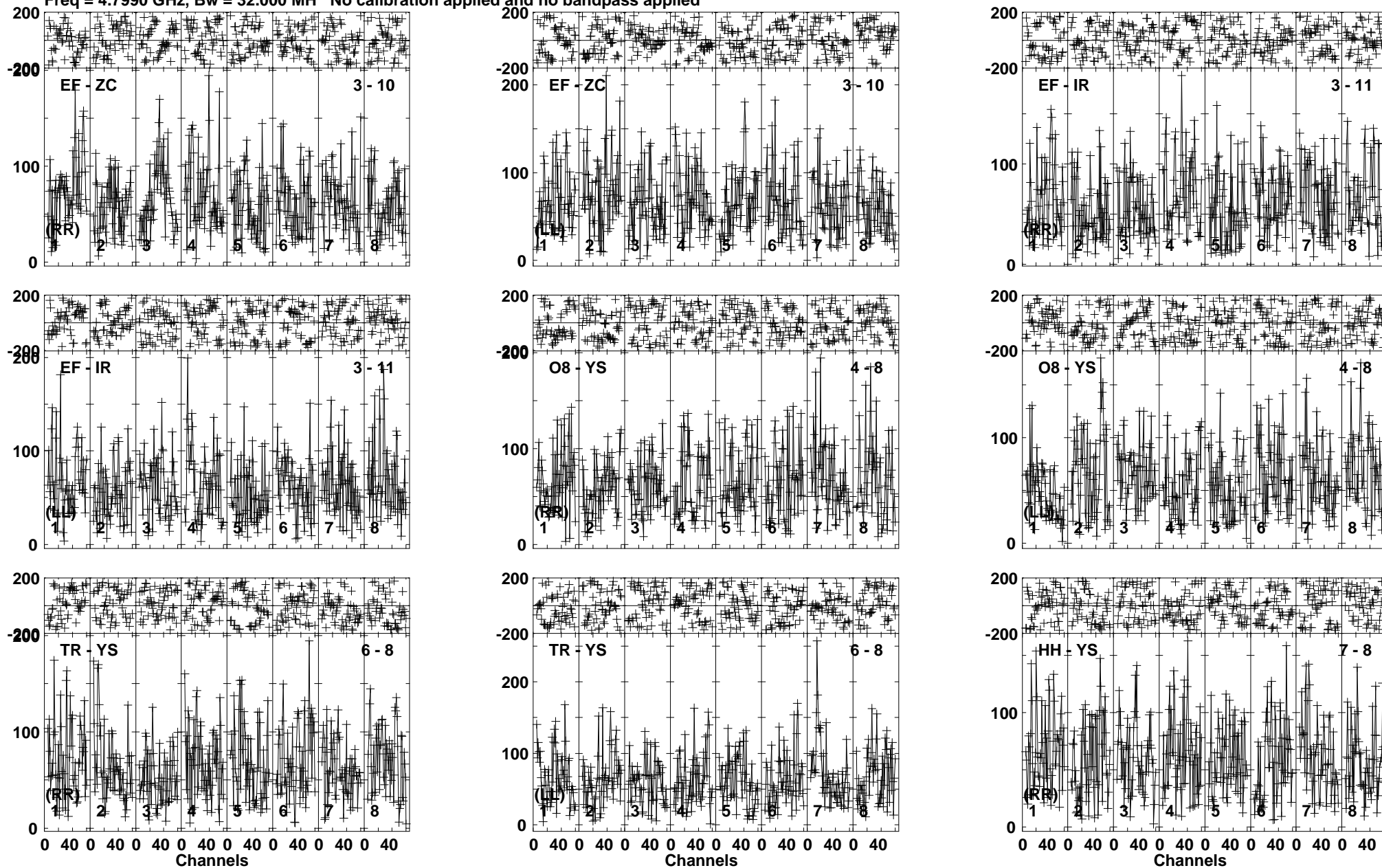
Lower frame: Micro Ampl Jy Top frame: Phas deg Vector averaged cross-power spectrum Baseline: EF (03) - ZC (10) Timerange: 00/04:13:54 to 00/04:18:27
