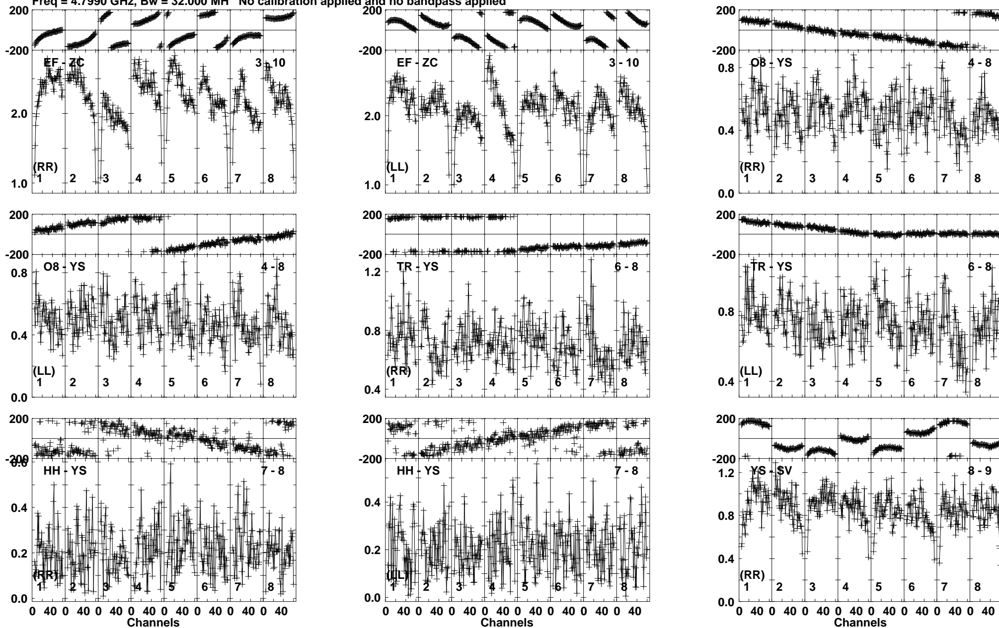
Lower frame: Milli Ampl Jy Top frame: Phas deg Vector averaged cross-power spectrum Baseline: EF (03) - ZC (10) Timerange: 00/06:39:20 to 00/06:40:20
