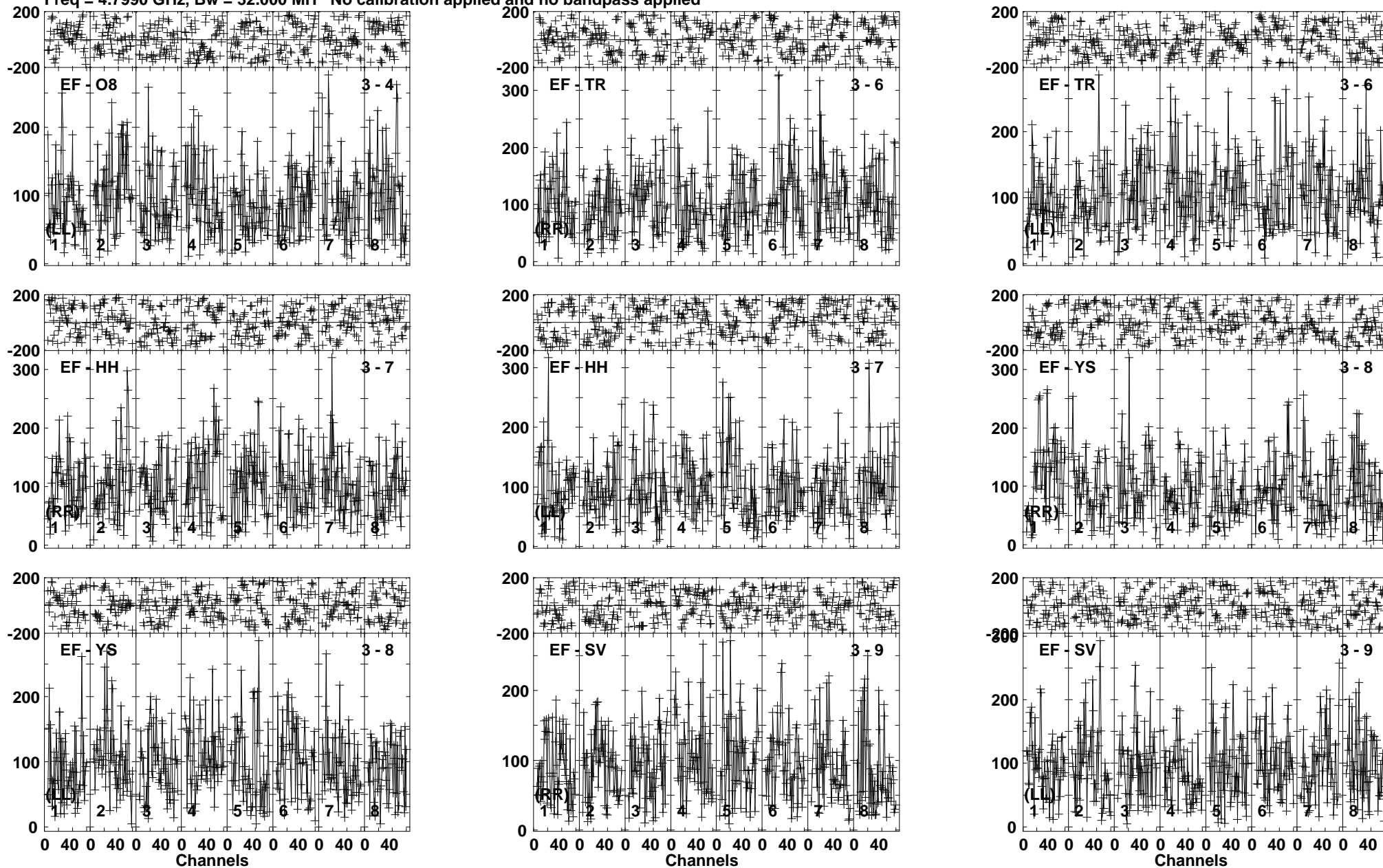
Lower frame: Micro Ampl Jy Top frame: Phas deg Vector averaged cross-power spectrum Baseline: EF (03) - O8 (04) Timerange: 00/05:25:07 to 00/05:27:08
