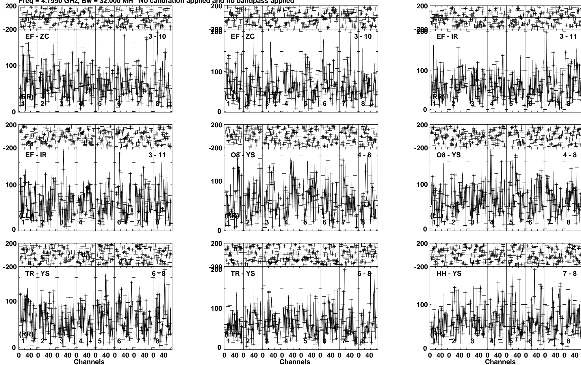
Lower frame: Micro Ampl Jy Top frame: Phas deg Vector averaged cross-power spectrum Baseline: EF (03) - ZC (10) Timerange: 00/06:48:20 to 00/06:53:19
