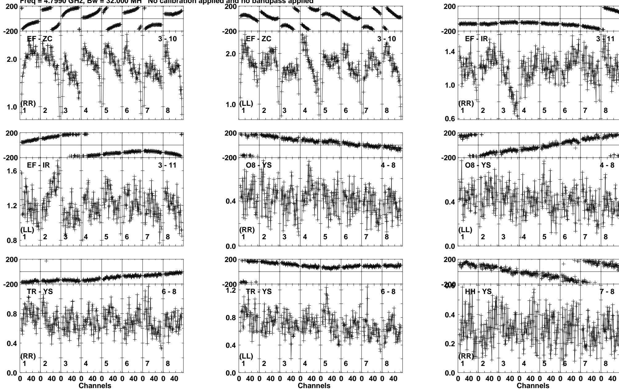
Lower frame: Milli Ampl Jy Top frame: Phas deg Vector averaged cross-power spectrum Baseline: EF (03) - ZC (10) Timerange: 00/04:19:07 to 00/04:20:05
