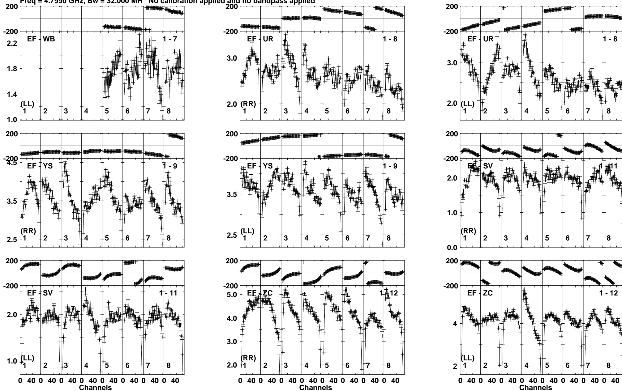
Lower frame: Milli Ampl Jy Top frame: Phas deg Vector averaged cross-power spectrum Baseline: EF (01) - WB (07) Timerange: 00/01:03:56 to 00/01:05:14
