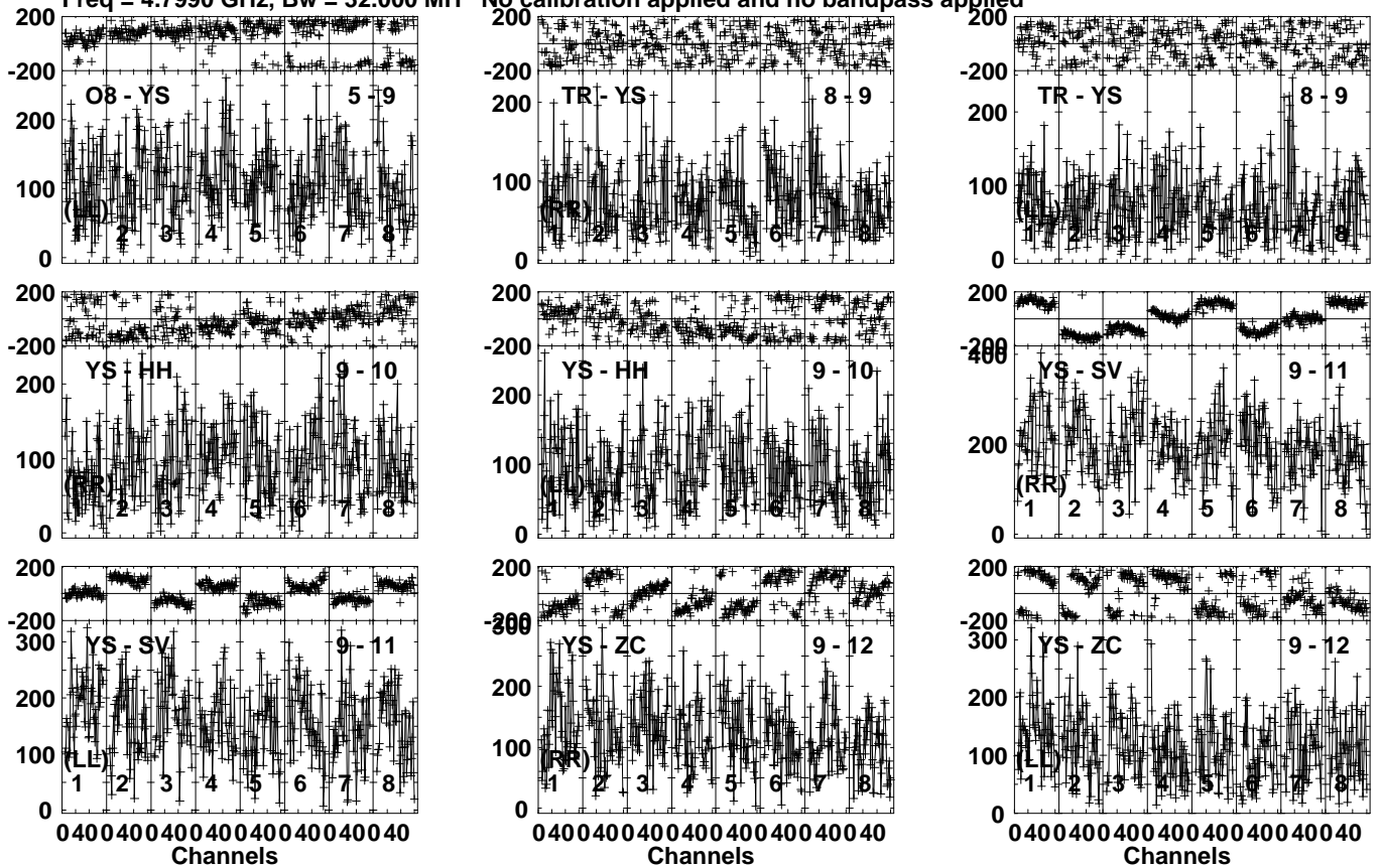
Lower frame: Micro Ampl Jy Top frame: Phas deg Vector averaged cross-power spectrum Several baselines displayed Timerange: 00/21:24:31 to 00/21:28:09
