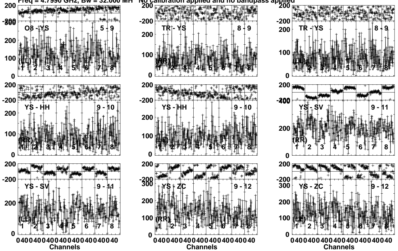
Lower frame: Micro Ampl Jy Top frame: Phas deg Vector averaged cross-power spectrum Several baselines displayed Timerange: 00/21:40:31 to 00/21:44:09
