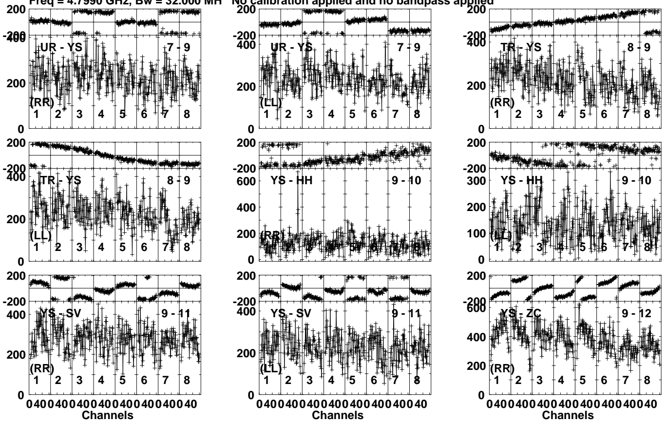
Lower frame: Micro Ampl Jy Top frame: Phas deg Vector averaged cross-power spectrum Several baselines displayed Timerange: 00/20:16:11 to 00/20:19:59
