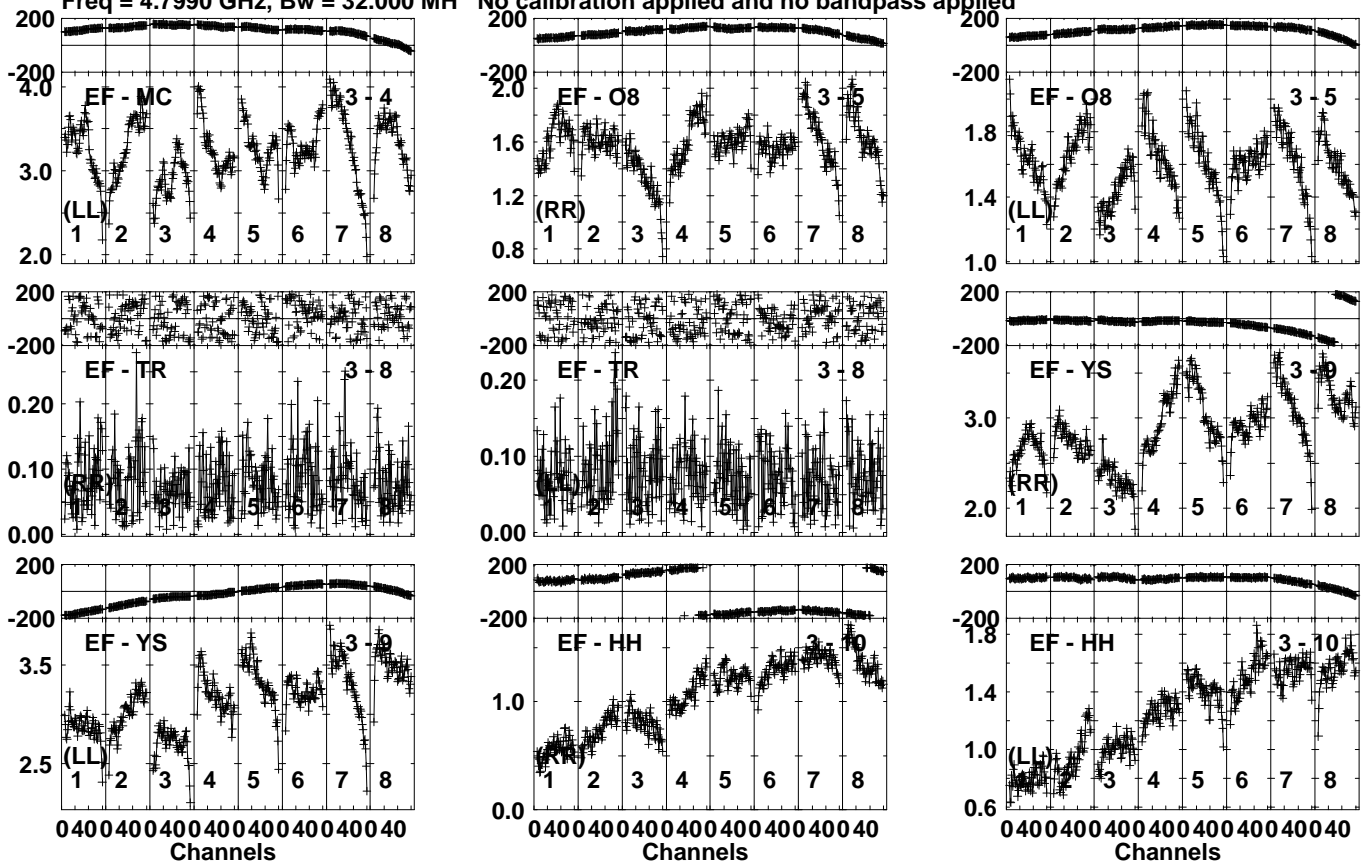
Lower frame: Milli Ampl Jy Top frame: Phas deg Vector averaged cross-power spectrum Several baselines displayed Timerange: 00/22:24:41 to 00/22:28:19
