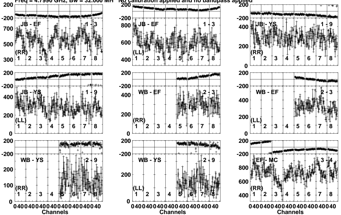
Lower frame: Micro Ampl Jy Top frame: Phas deg Vector averaged cross-power spectrum Several baselines displayed Timerange: 00/20:33:11 to 00/20:36:59
