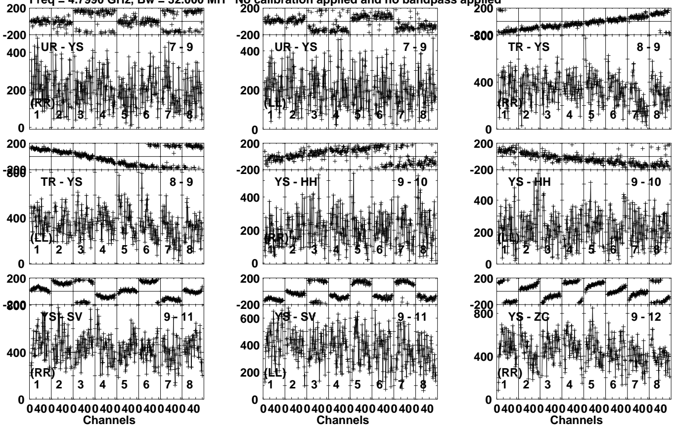
Lower frame: Micro Ampl Jy Top frame: Phas deg Vector averaged cross-power spectrum Several baselines displayed Timerange: 00/18:35:01 to 00/18:36:09
