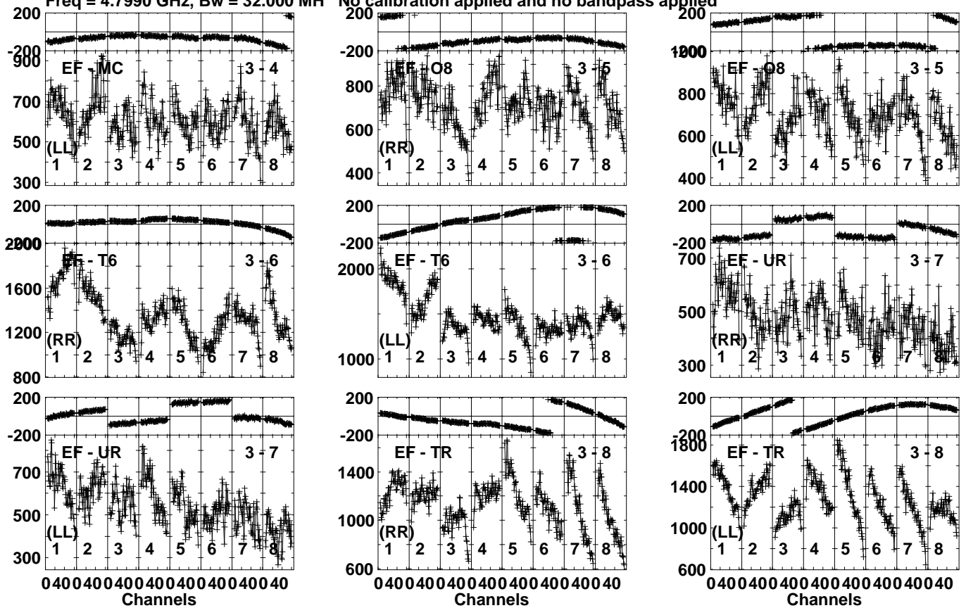
Lower frame: Micro Ampl Jy Top frame: Phas deg Vector averaged cross-power spectrum Several baselines displayed Timerange: 00/18:50:03 to 00/18:53:39
