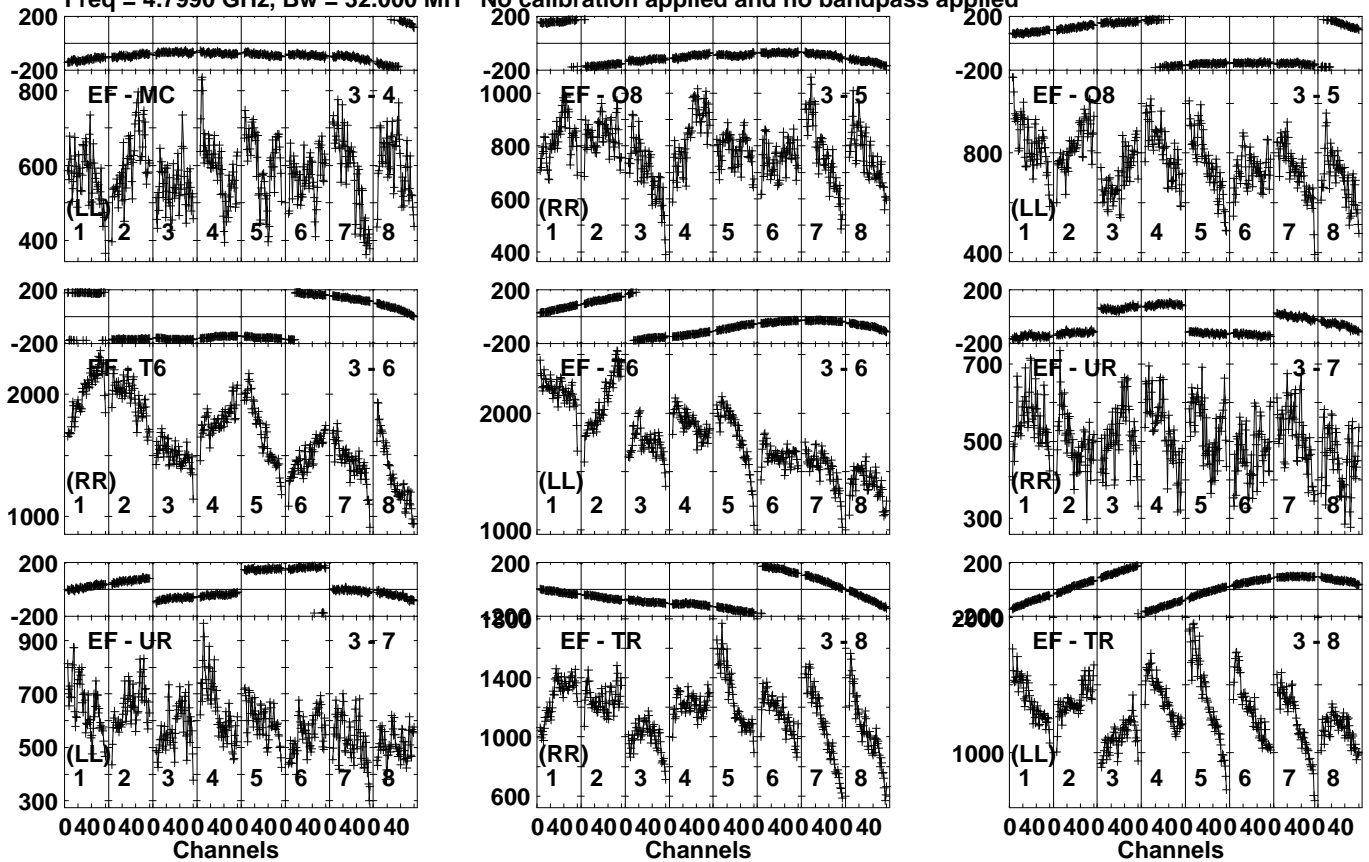
Lower frame: Micro Ampl Jy Top frame: Phas deg Vector averaged cross-power spectrum Several baselines displayed Timerange: 00/19:00:41 to 00/19:04:19
