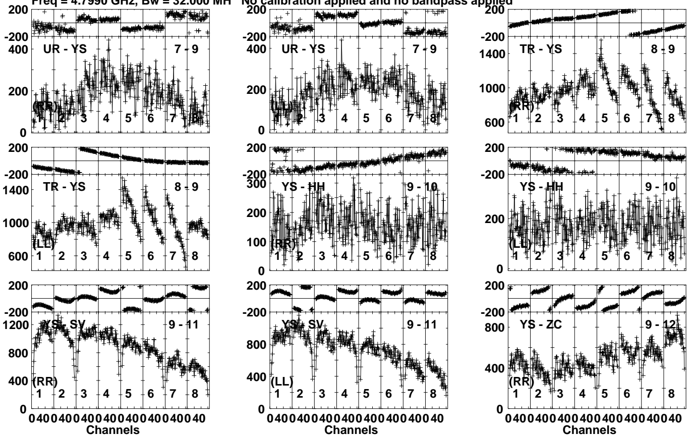
Lower frame: Micro Ampl Jy Top frame: Phas deg Vector averaged cross-power spectrum Several baselines displayed Timerange: 00/19:29:01 to 00/19:32:29
