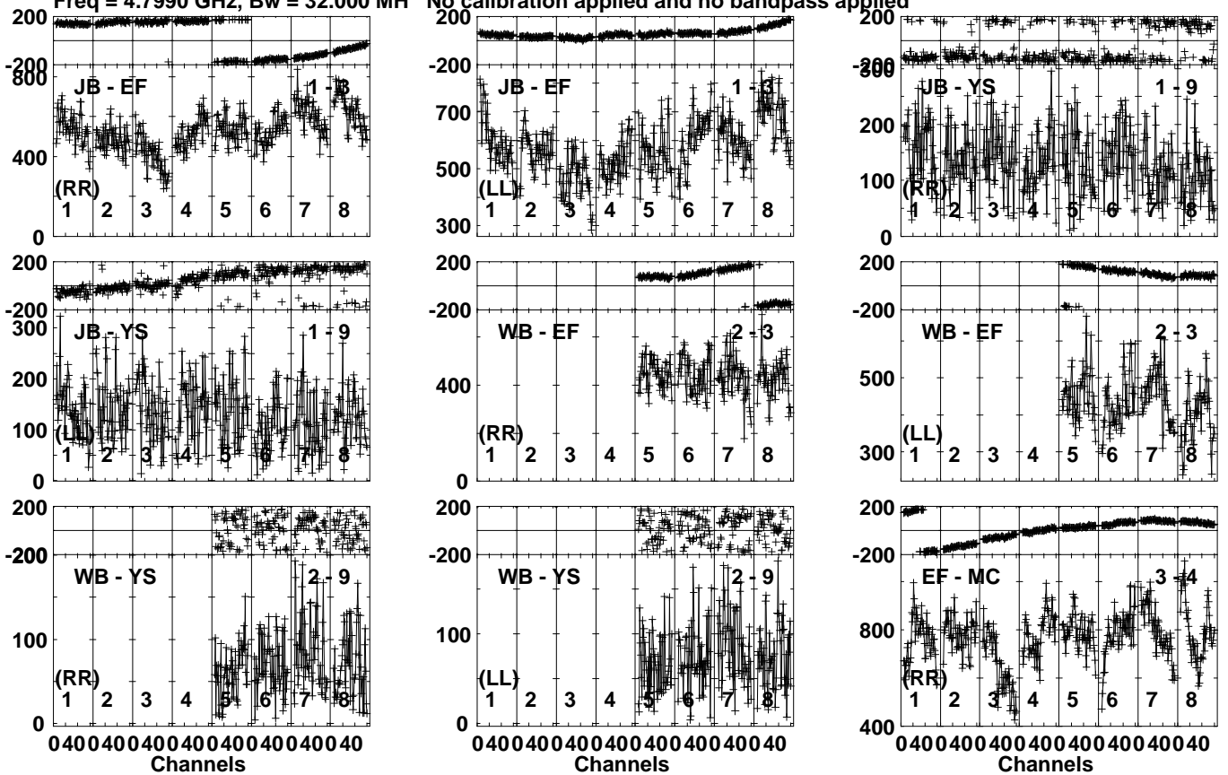
Lower frame: Micro Ampl Jy Top frame: Phas deg Vector averaged cross-power spectrum Several baselines displayed Timerange: 00:17:41:53 to 00:17:45:39
