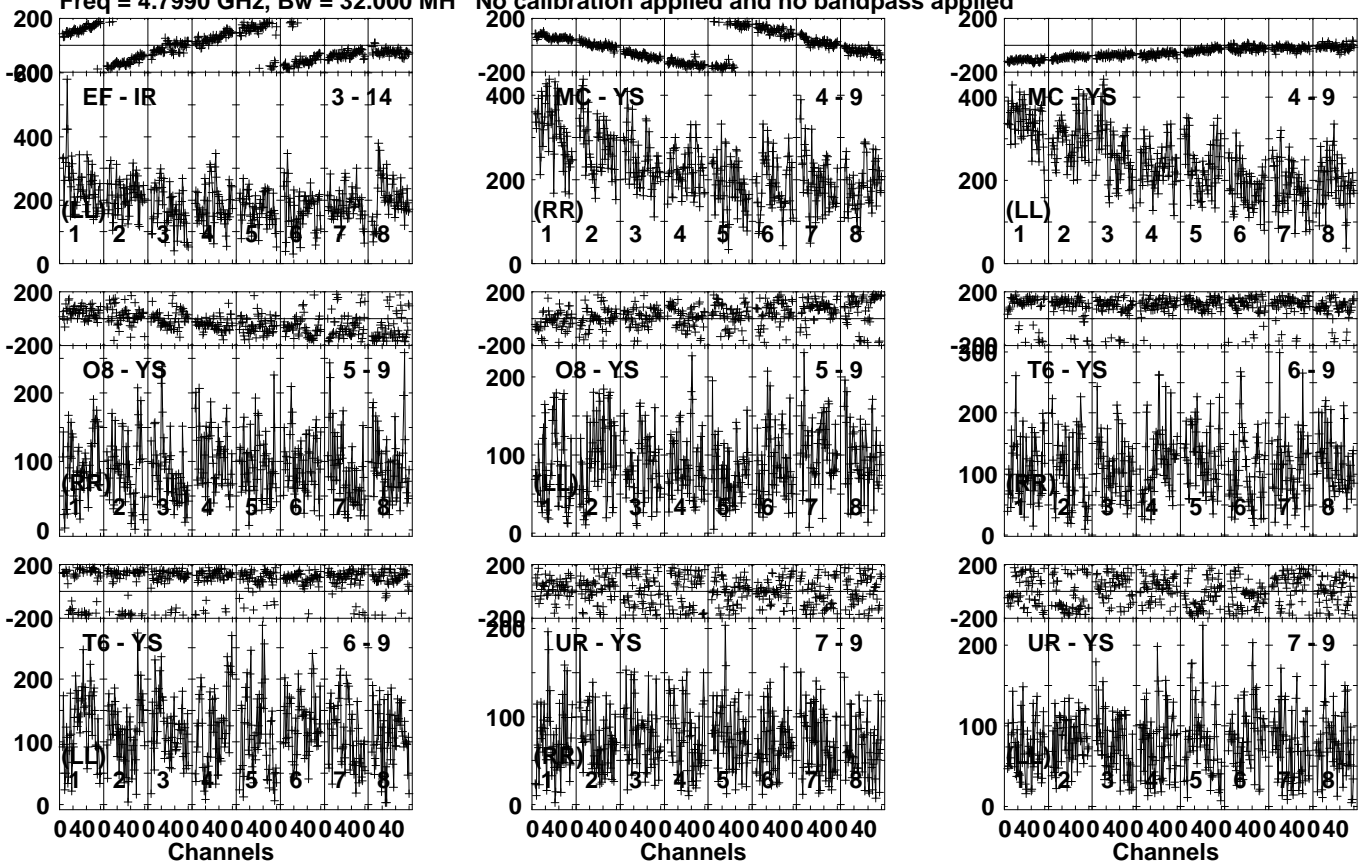
Lower frame: Micro Ampl Jy Top frame: Phas deg Vector averaged cross-power spectrum Several baselines displayed Timerange: 00/18:04:31 to 00/18:08:19
