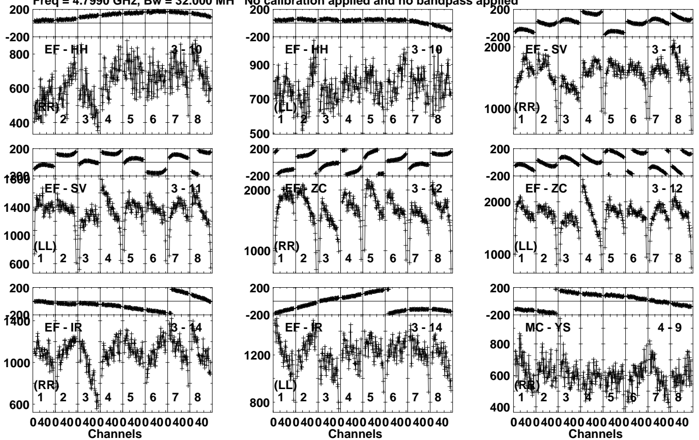
Lower frame: Micro Ampl Jy Top frame: Phas deg Vector averaged cross-power spectrum Several baselines displayed Timerange: 00/20:49:31 to 00/20:53:09
