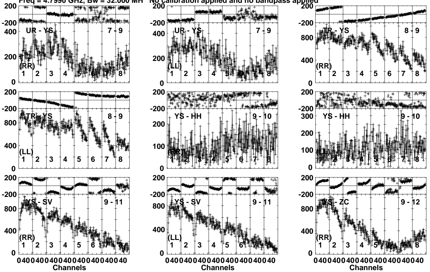
Lower frame: Micro Ampl Jy Top frame: Phas deg Vector averaged cross-power spectrum Several baselines displayed Timerange: 00/18:25:31 to 00/18:29:09
