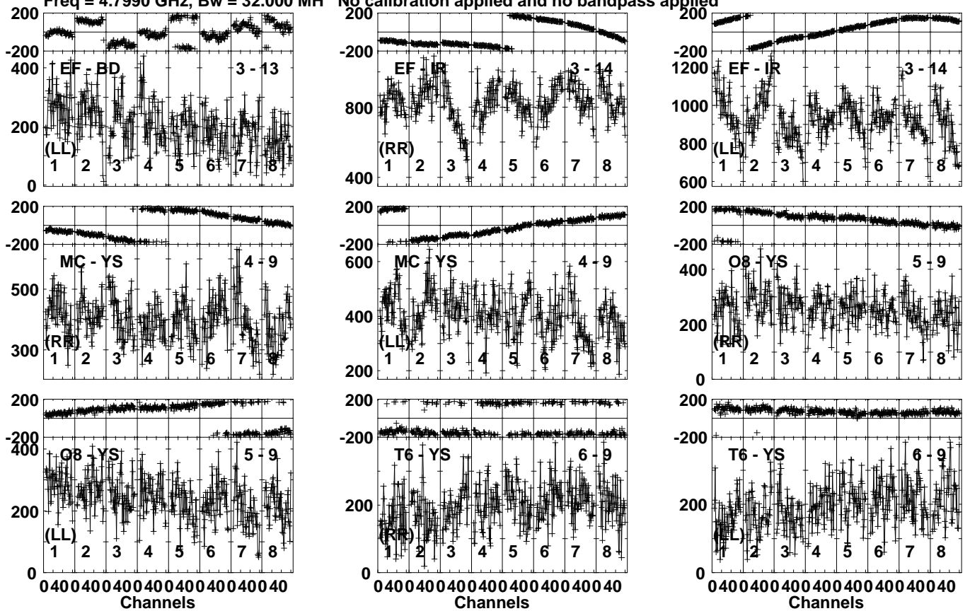
Lower frame: Micro Ampl Jy Top frame: Phas deg Vector averaged cross-power spectrum Several baselines displayed Timerange: 00/20:02:21 to 00/20:05:59
