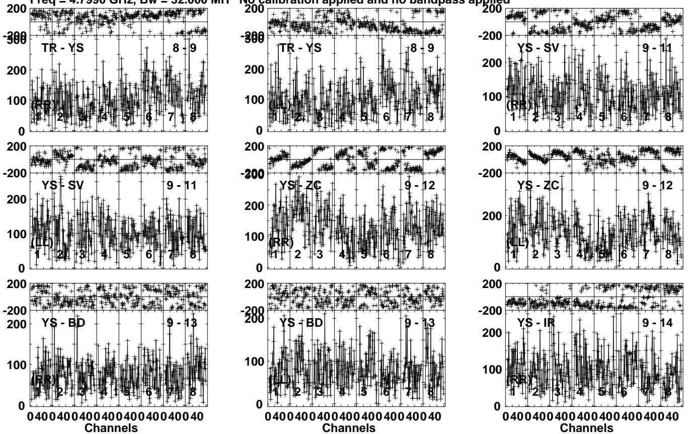
Lower frame: Micro Ampl Jy Top frame: Phas deg Vector averaged cross-power spectrum Several baselines displayed Timerange: 00/17:53:11 to 00/17:56:59
