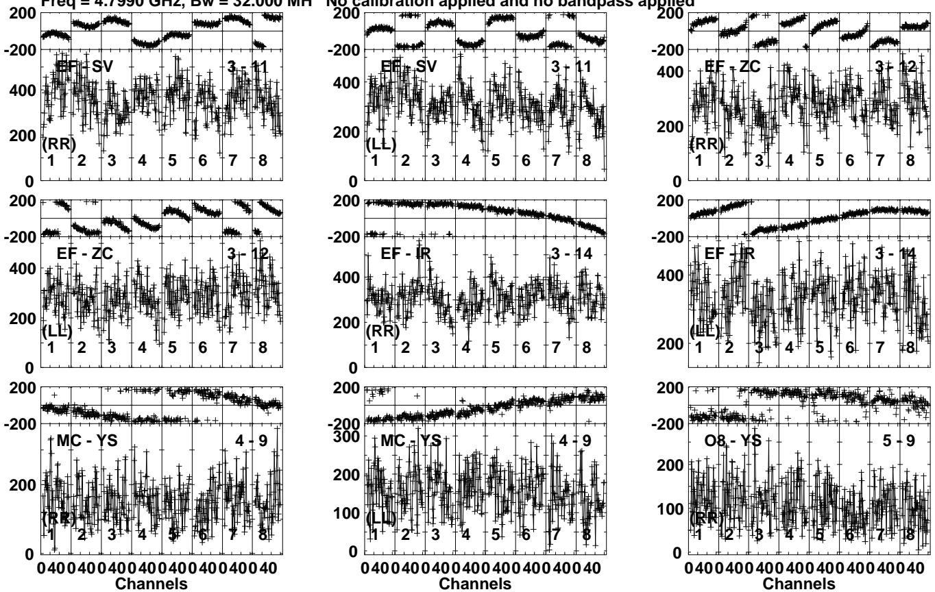
Lower frame: Micro Ampl Jy Top frame: Phas deg Vector averaged cross-power spectrum Several baselines displayed Timerange: 00/21:19:11 to 00/21:22:49
