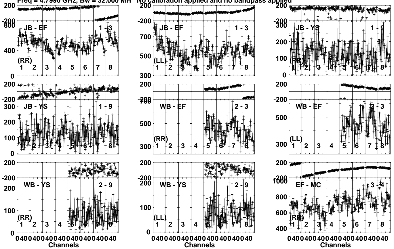
Lower frame: Micro Ampl Jy Top frame: Phas deg Vector averaged cross-power spectrum Several baselines displayed Timerange: 00/17:36:11 to 00/17:39:59
