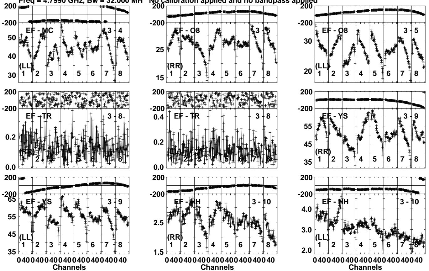
Lower frame: Milli Ampl Jy Top frame: Phas deg Vector averaged cross-power spectrum Several baselines displayed Timerange: 00/21:22:51 to 00/21:24:29
