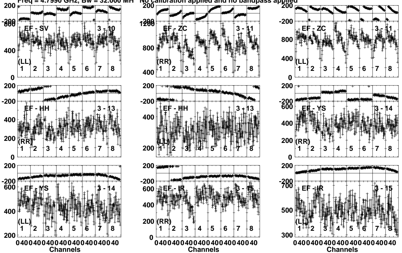
Lower frame: Micro Ampl Jy Top frame: Phas deg Vector averaged cross-power spectrum Several baselines displayed Timerange: 00/06:13:51 to 00/06:17:19
