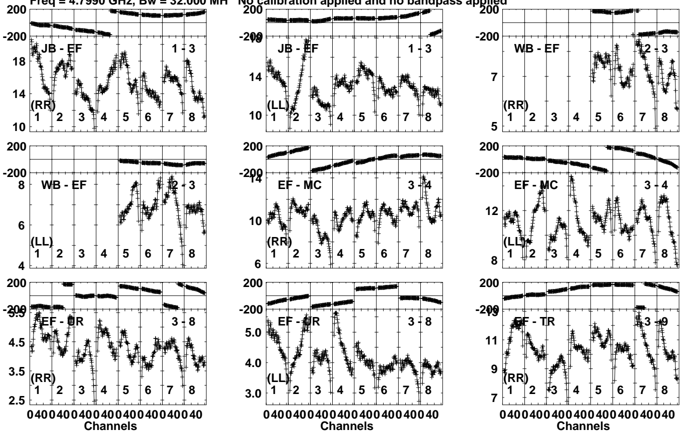
Lower frame: Milli Ampl Jy Top frame: Phas deg Vector averaged cross-power spectrum Several baselines displayed Timerange: 00/05:15:51 to 00/05:18:49
