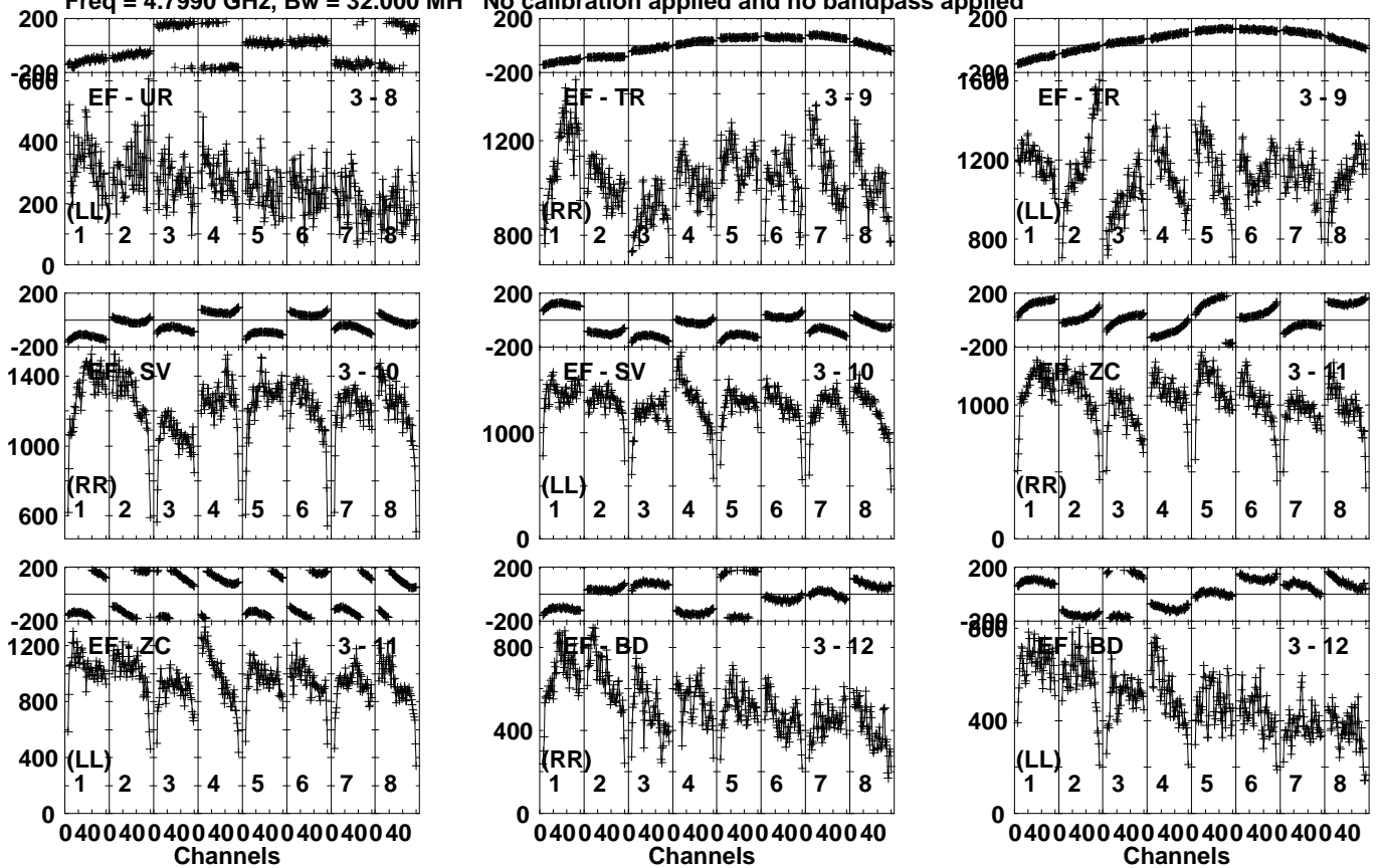
Lower frame: Micro Ampl Jy Top frame: Phas deg Vector averaged cross-power spectrum Several baselines displayed Timerange: 00/05:06:21 to 00/05:09:49
