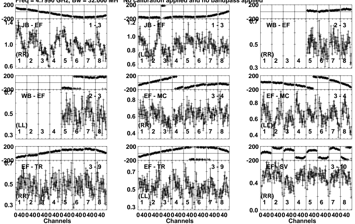
Lower frame: Milli Ampl Jy Top frame: Phas deg Vector averaged cross-power spectrum Several baselines displayed Timerange: 00/05:58:51 to 00/06:02:19
