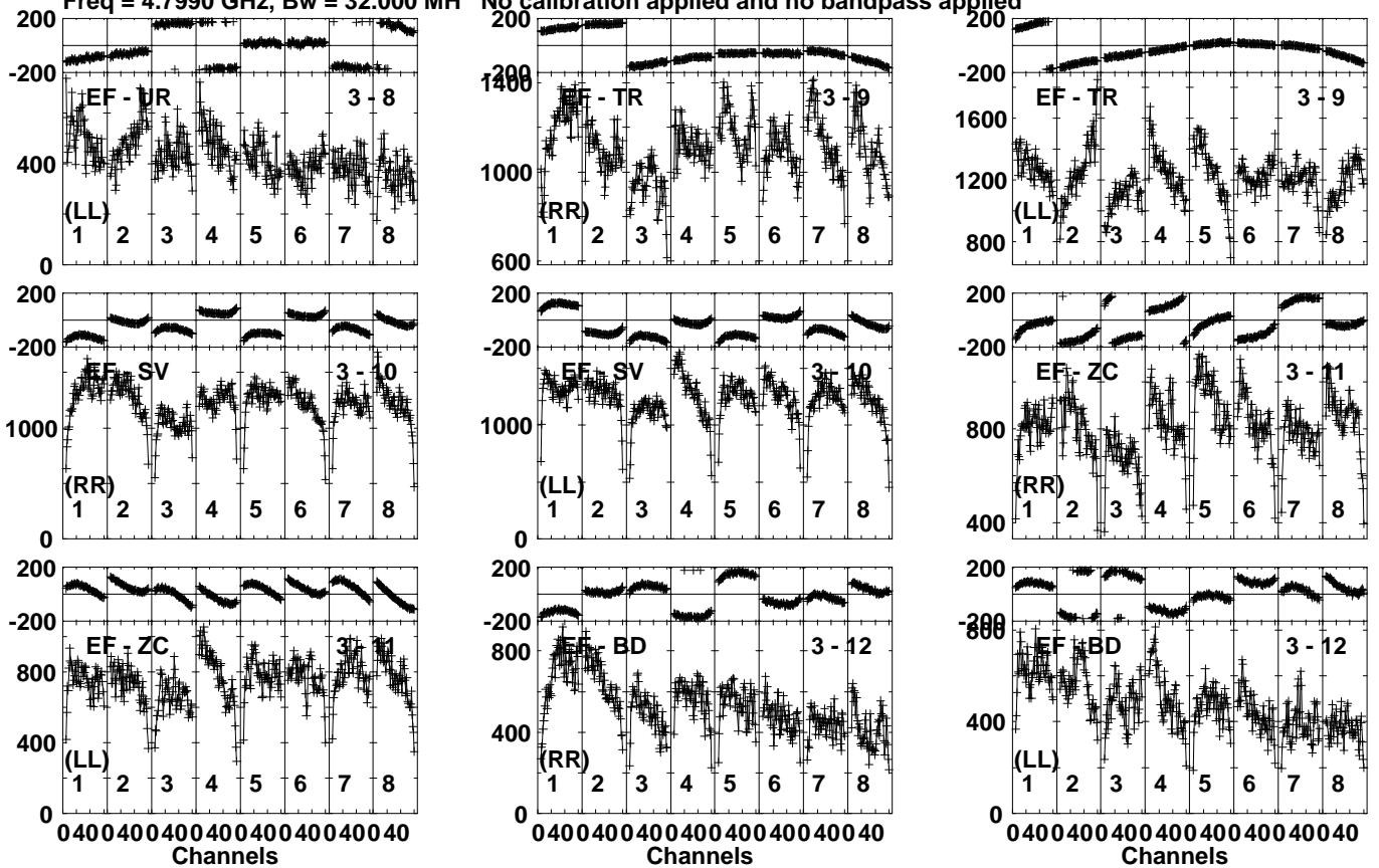
Lower frame: Micro Ampl Jy Top frame: Phas deg Vector averaged cross-power spectrum Several baselines displayed Timerange: 00/04:41:21 to 00/04:44:49
