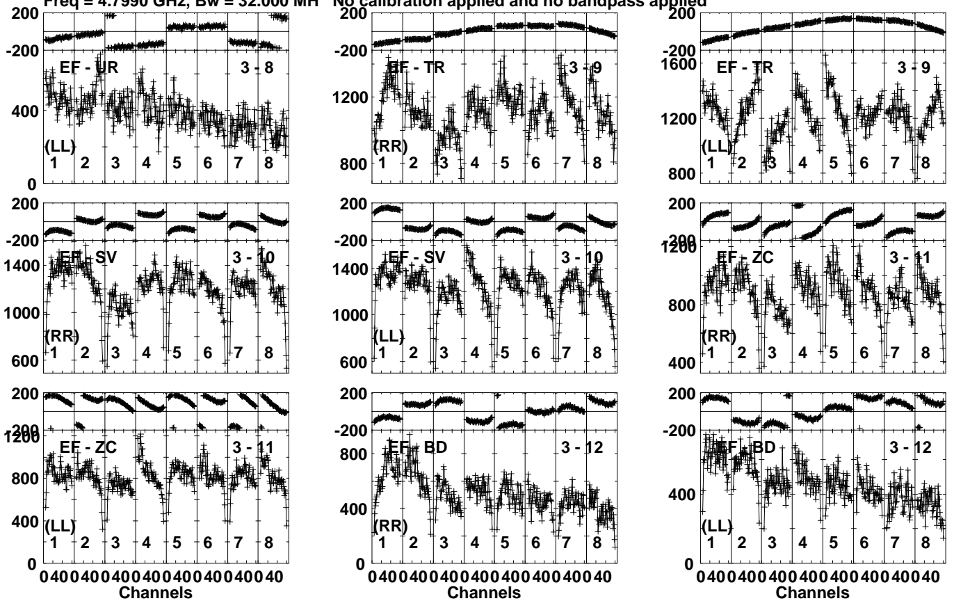
Lower frame: Micro Ampl Jy Top frame: Phas deg Vector averaged cross-power spectrum Several baselines displayed Timerange: 00/04:51:23 to 00/04:54:49
