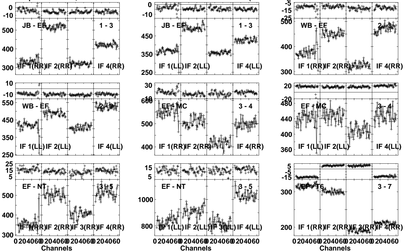
Lower frame: Milli Ampl Jy Top frame: Phas deg Vector averaged cross-power spectrum Several baselines displayed Timerange: 00/13:23:31 to 00/13:24:59
