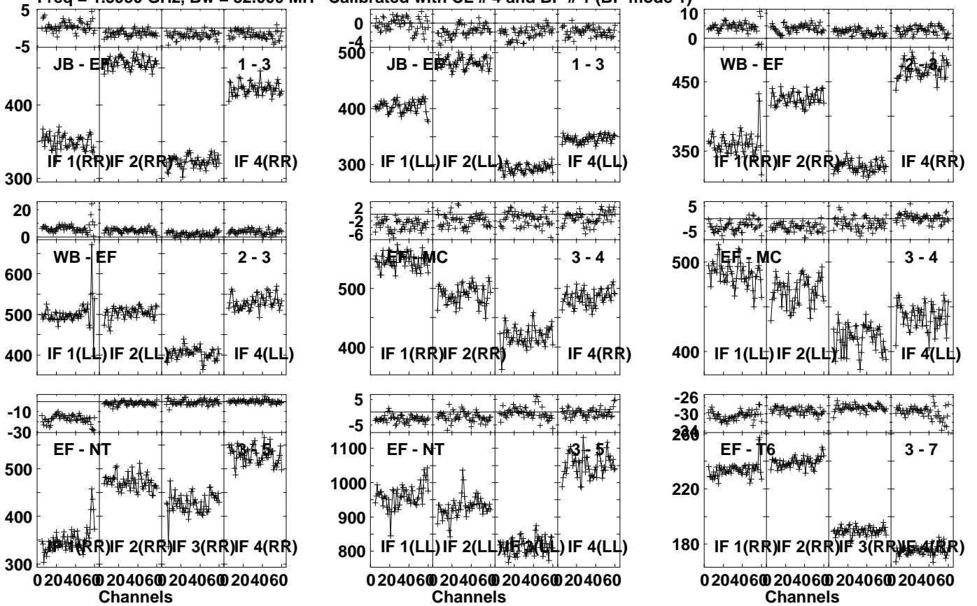
Lower frame: Milli Ampl Jy Top frame: Phas deg Vector averaged cross-power spectrum Several baselines displayed Timerange: 00/13:18:31 to 00/13:19:59
