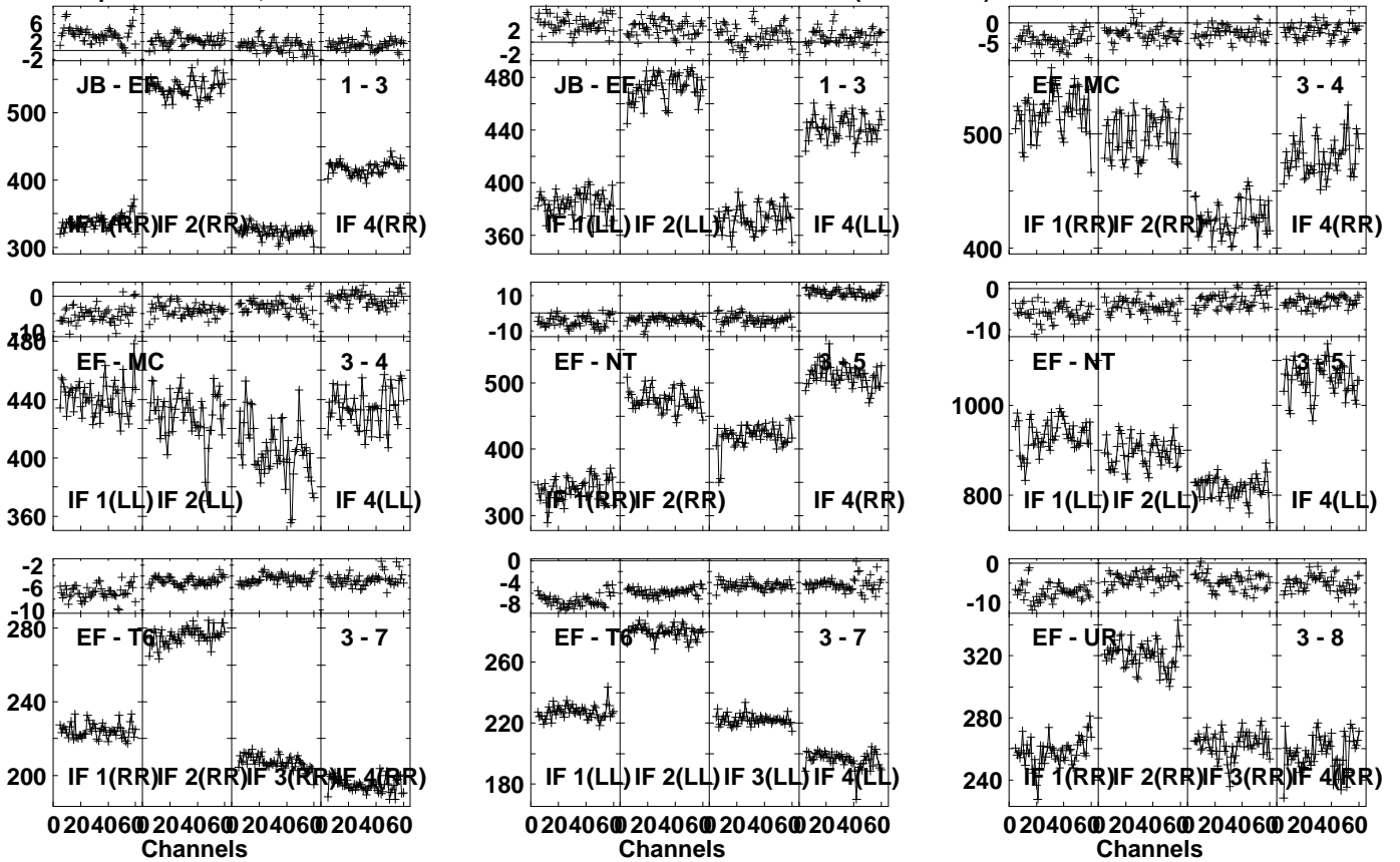
Lower frame: Milli Ampl Jy Top frame: Phas deg Vector averaged cross-power spectrum Several baselines displayed Timerange: 00/11:23:01 to 00/11:24:29
