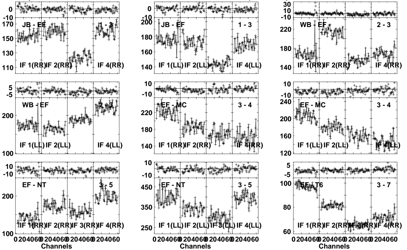
Lower frame: Milli Ampl Jy Top frame: Phas deg Vector averaged cross-power spectrum Several baselines displayed Timerange: 00/19:57:01 to 00/19:58:29
