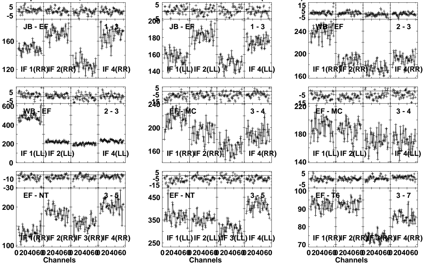
Lower frame: Milli Ampl Jy Top frame: Phas deg Vector averaged cross-power spectrum Several baselines displayed Timerange: 00:19:07:01 to 00:19:08:29
