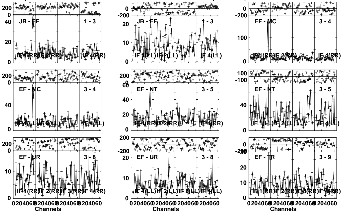
Lower frame: Milli Ampl Jy Top frame: Phas deg Vector averaged cross-power spectrum Several baselines displayed Timerange: 00/13:04:01 to 00/13:07:29
