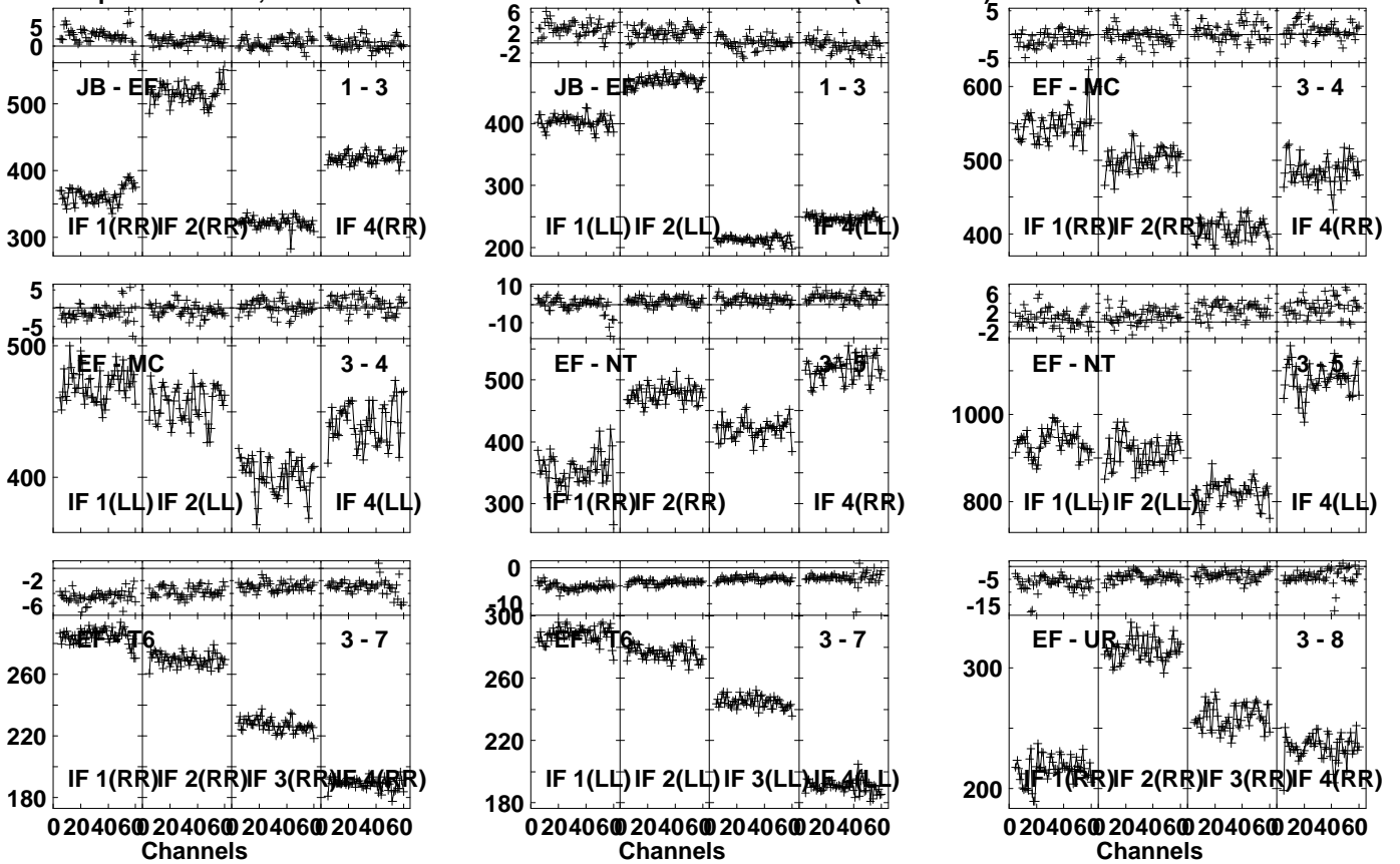
Lower frame: Milli Ampl Jy Top frame: Phas deg Vector averaged cross-power spectrum Several baselines displayed Timerange: 00/11:12:31 to 00/11:13:59
