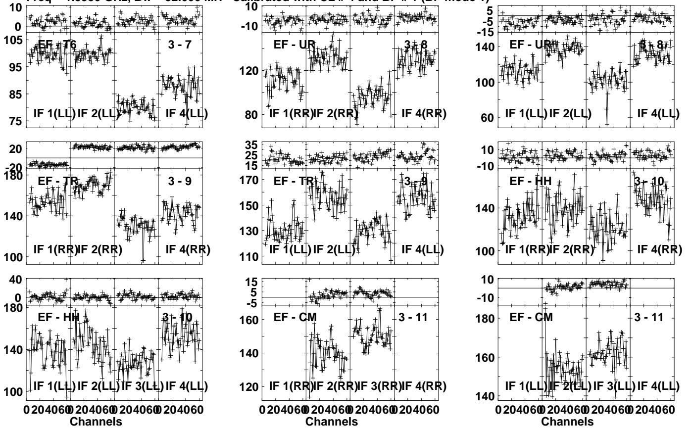
Lower frame: Milli Ampl Jy Top frame: Phas deg Vector averaged cross-power spectrum Several baselines displayed Timerange: 00/18:14:31 to 00/18:15:59
