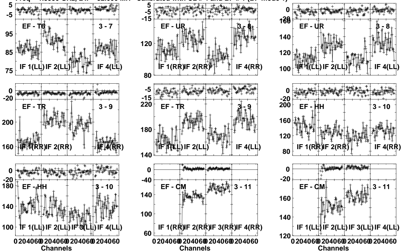
Lower frame: Milli Ampl Jy Top frame: Phas deg Vector averaged cross-power spectrum Several baselines displayed Timerange: 00/19:22:31 to 00/19:23:59
