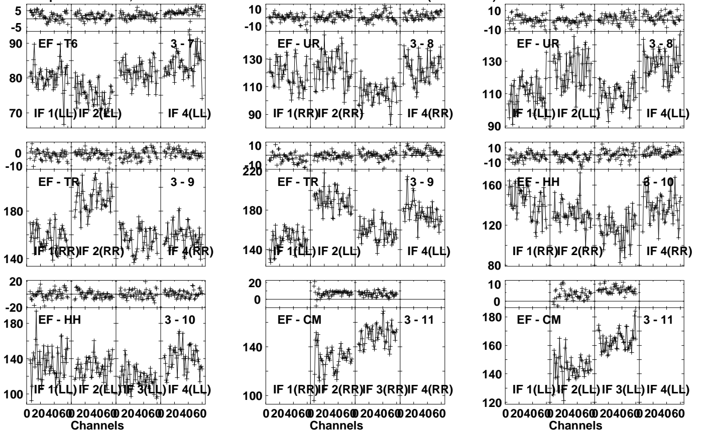
Lower frame: Milli Ampl Jy Top frame: Phas deg Vector averaged cross-power spectrum Several baselines displayed Timerange: 00/19:33:01 to 00/19:34:29
