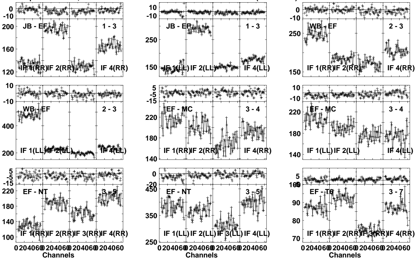
Lower frame: Milli Ampl Jy Top frame: Phas deg Vector averaged cross-power spectrum Several baselines displayed Timerange: 00:18:46:01 to 00:18:47:29
