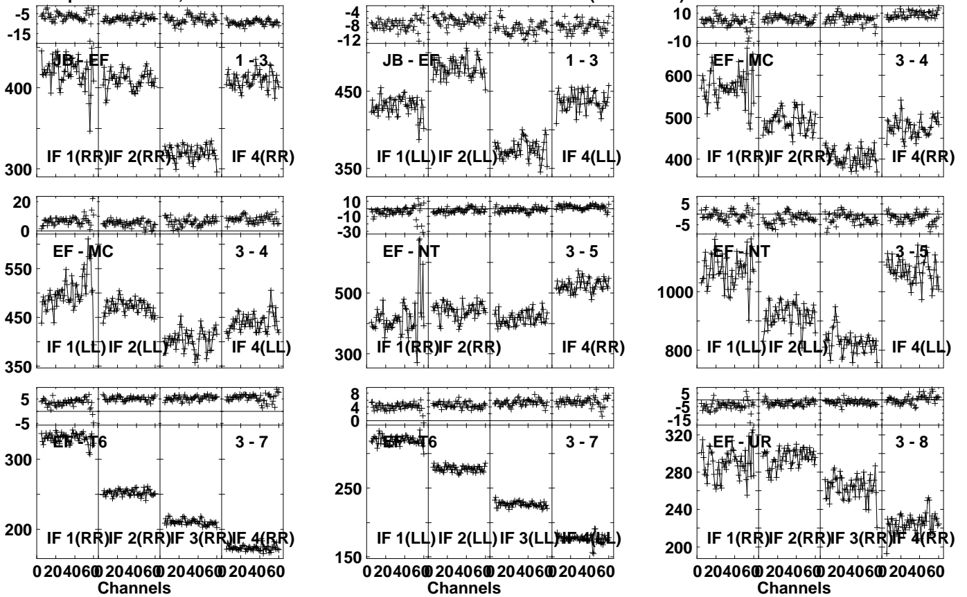
Lower frame: Milli Ampl Jy Top frame: Phas deg Vector averaged cross-power spectrum Several baselines displayed Timerange: 00/11:17:31 to 00/11:18:59
