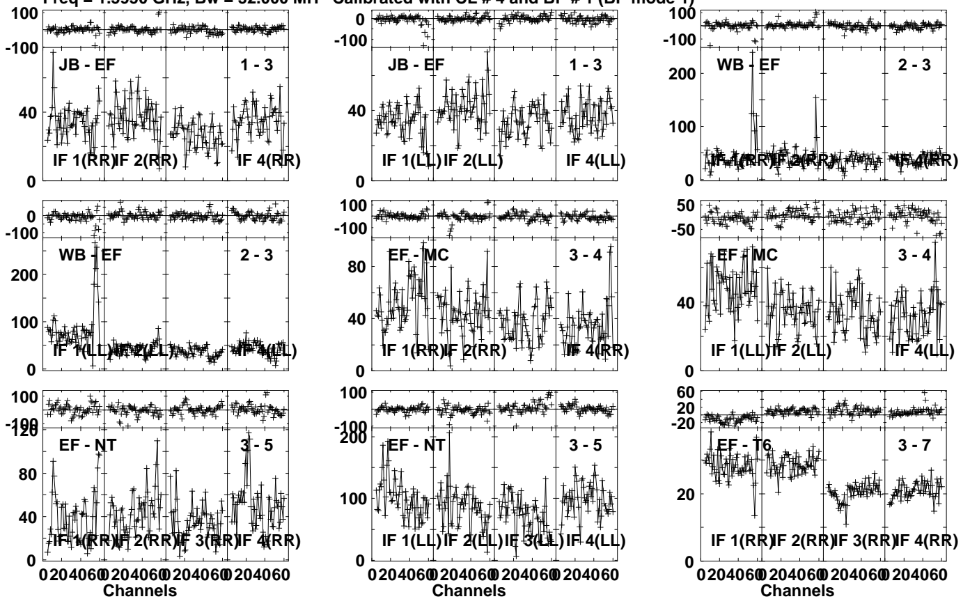
Lower frame: Milli Ampl Jy Top frame: Phas deg Vector averaged cross-power spectrum Several baselines displayed Timerange: 00/17:18:31 to 00/17:19:59
