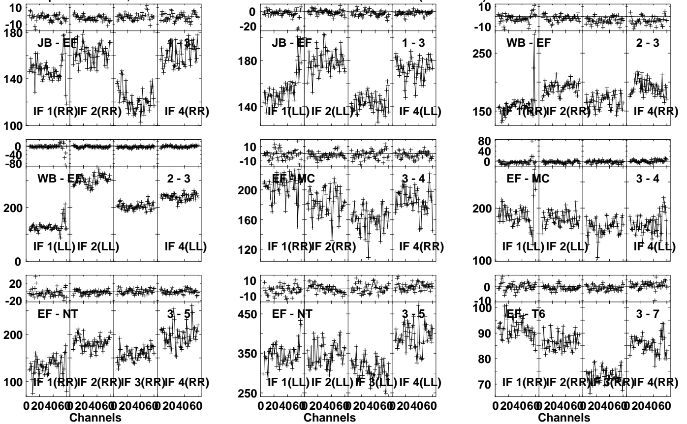
Lower frame: Milli Ampl Jy Top frame: Phas deg Vector averaged cross-power spectrum Several baselines displayed Timerange: 00/19:51:31 to 00/19:52:59
