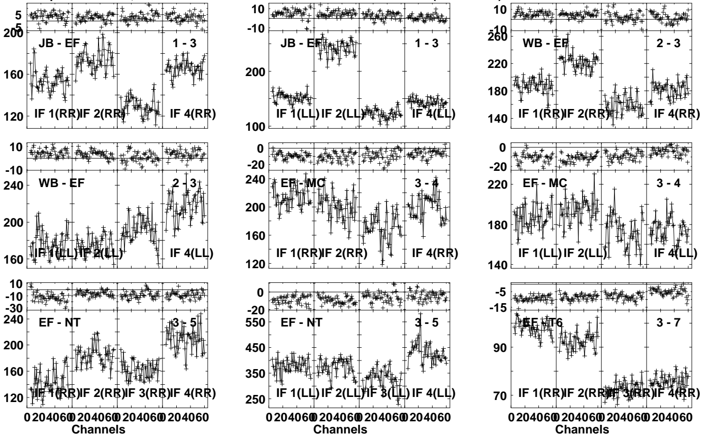
Lower frame: Milli Ampl Jy Top frame: Phas deg Vector averaged cross-power spectrum Several baselines displayed Timerange: 00:18:30:01 to 00:18:31:29
