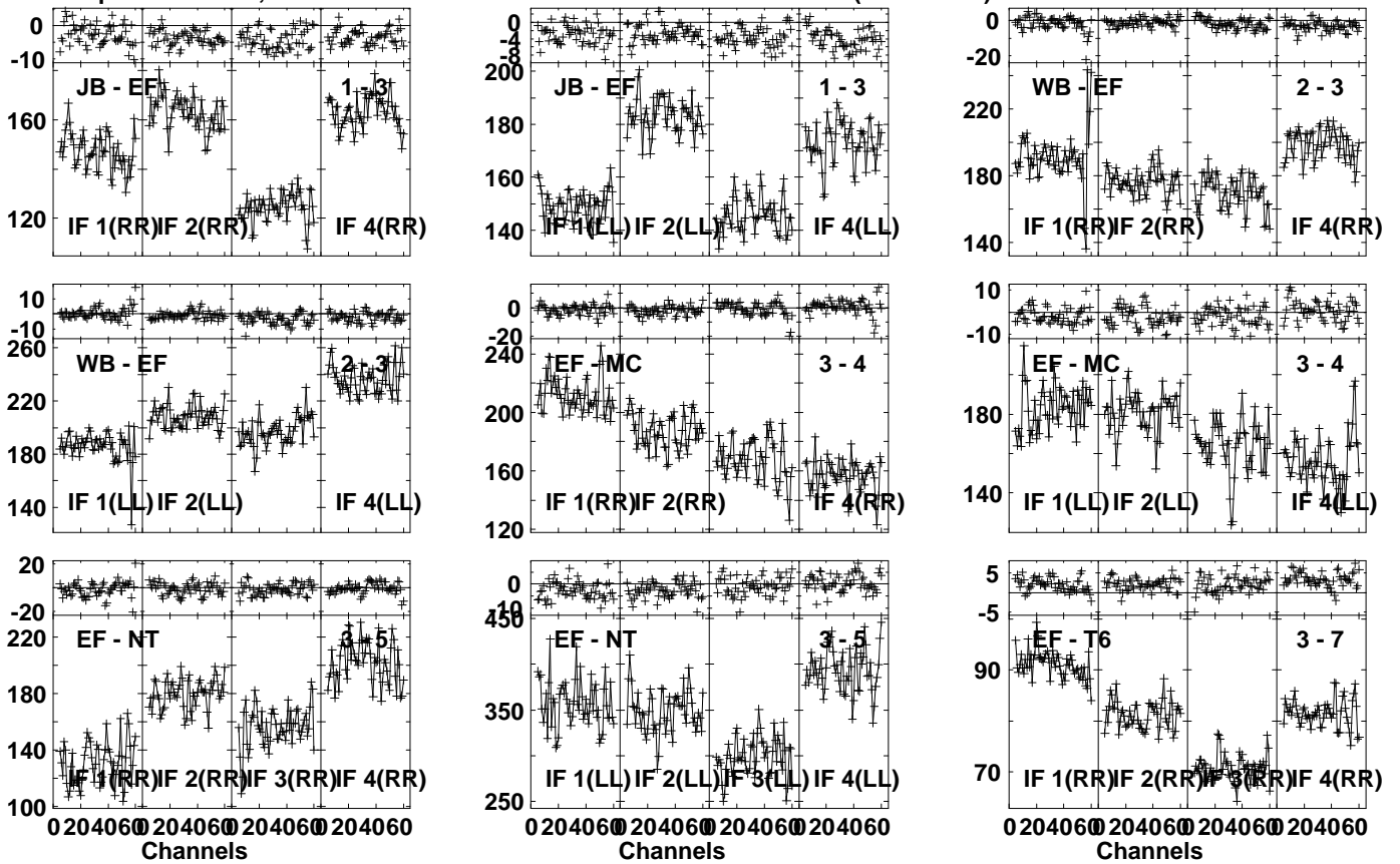
Lower frame: Milli Ampl Jy Top frame: Phas deg Vector averaged cross-power spectrum Several baselines displayed Timerange: 00:19:38:31 to 00:19:39:59
