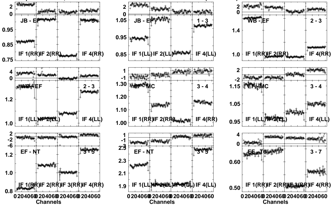
Lower frame: Ampl Jy Top frame: Phas deg Vector averaged cross-power spectrum Several baselines displayed Timerange: 00/13:44:31 to 00/13:49:29
