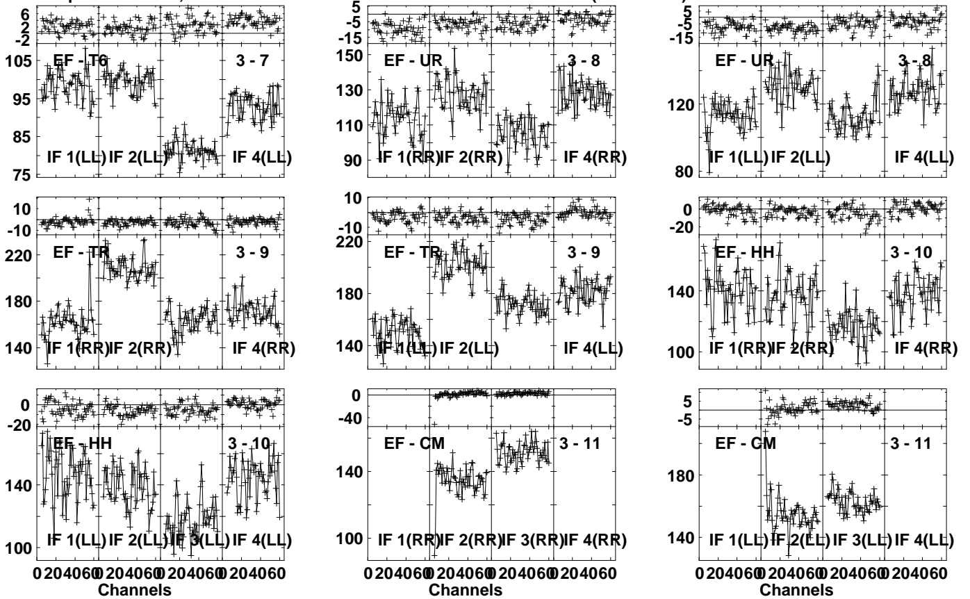
Lower frame: Milli Ampl Jy Top frame: Phas deg Vector averaged cross-power spectrum Several baselines displayed Timerange: 00:19:01:31 to 00:19:02:59
