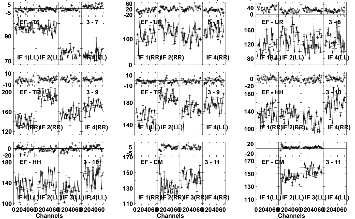
Lower frame: Milli Ampl Jy Top frame: Phas deg Vector averaged cross-power spectrum Several baselines displayed Timerange: 00/17:26:31 to 00/17:29:29
