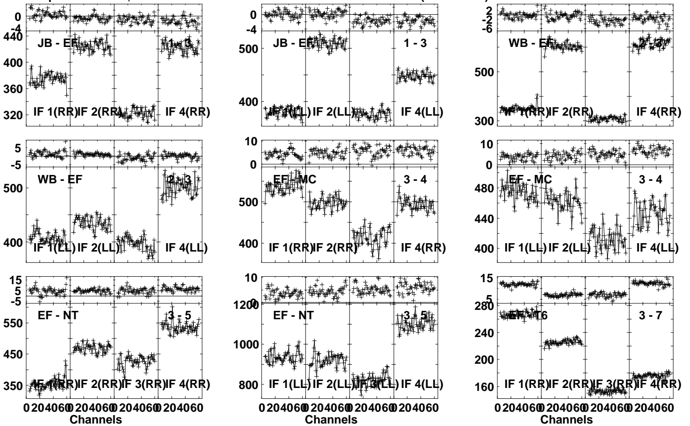
Lower frame: Milli Ampl Jy Top frame: Phas deg Vector averaged cross-power spectrum Several baselines displayed Timerange: 00/13:29:01 to 00/13:30:29
