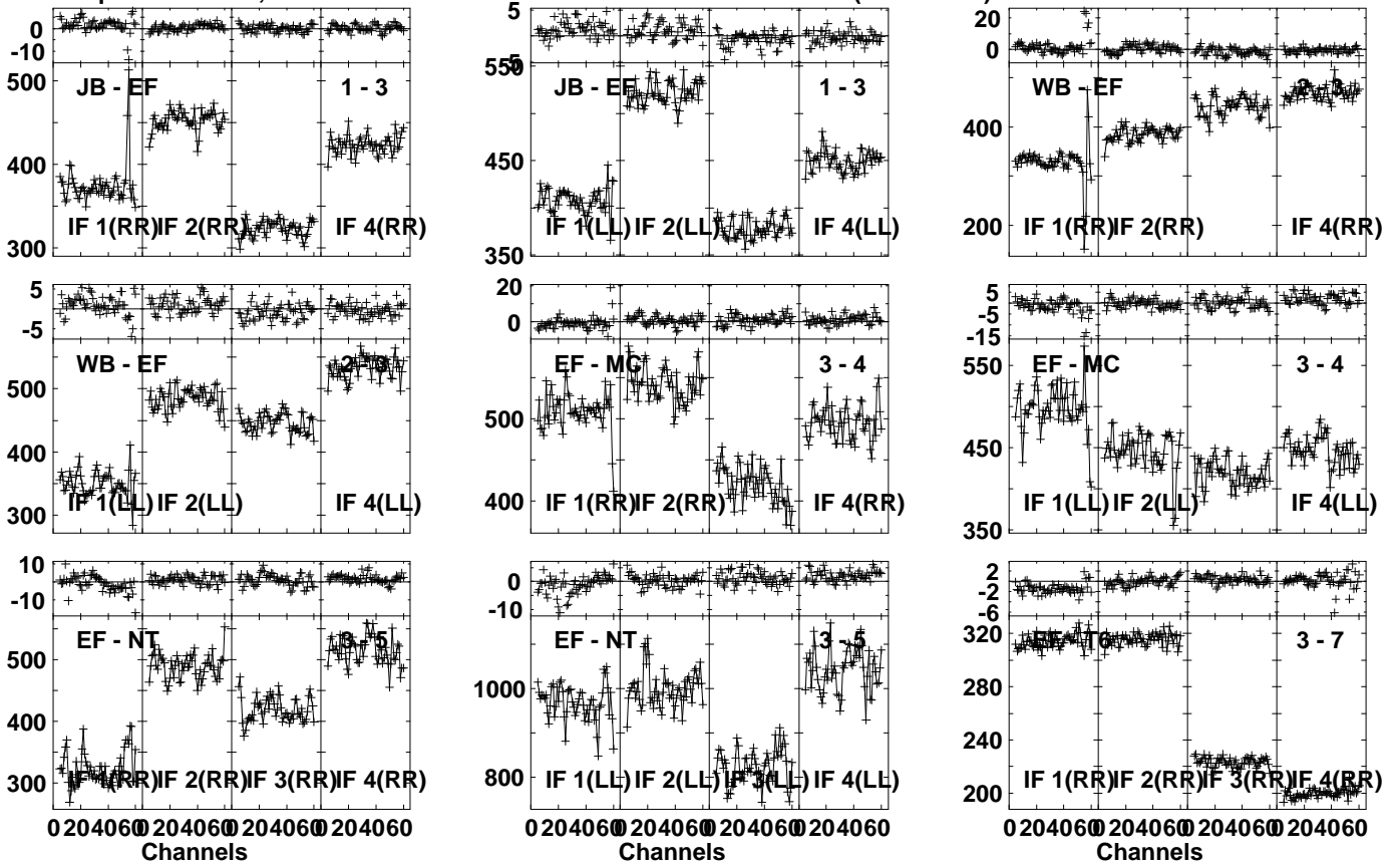
Lower frame: Milli Ampl Jy Top frame: Phas deg Vector averaged cross-power spectrum Several baselines displayed Timerange: 00/13:41:31 to 00/13:42:59
