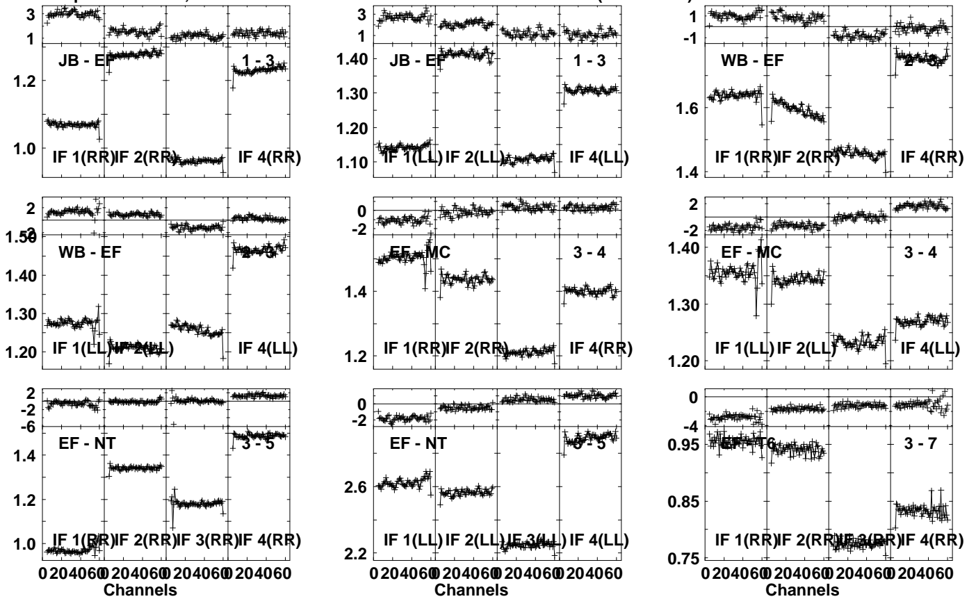
Lower frame: Ampl Jy Top frame: Phas deg Vector averaged cross-power spectrum Several baselines displayed Timerange: 00/15:44:01 to 00/15:48:59
