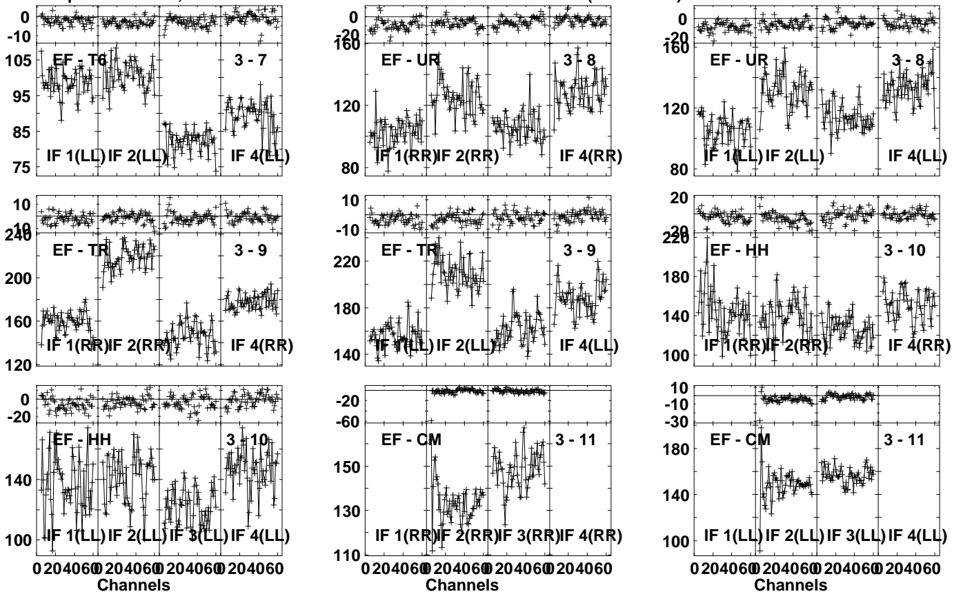
Lower frame: Milli Ampl Jy Top frame: Phas deg Vector averaged cross-power spectrum Several baselines displayed Timerange: 00/17:58:31 to 00/17:59:59
