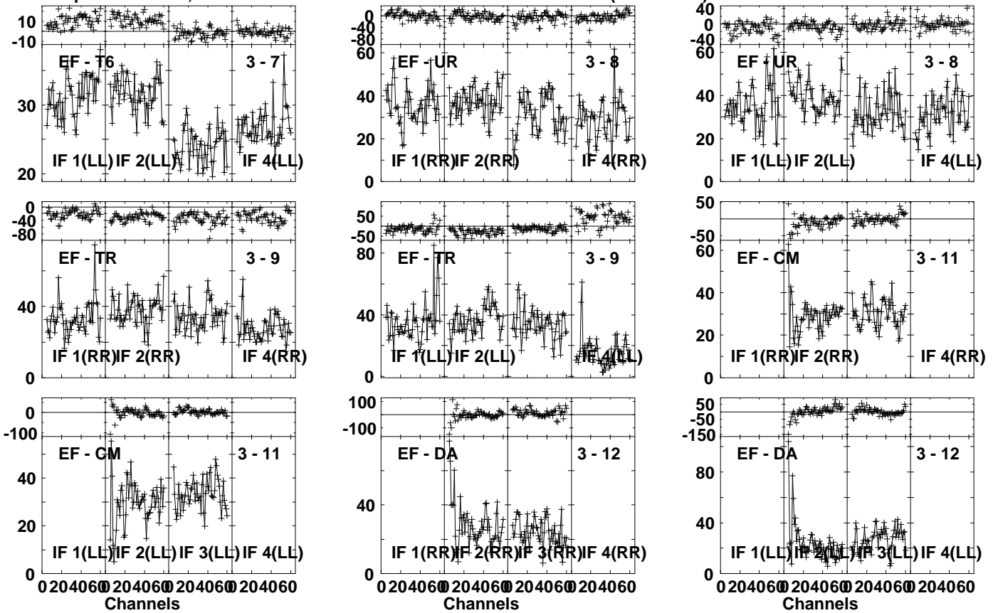
Lower frame: Milli Ampl Jy Top frame: Phas deg Vector averaged cross-power spectrum Several baselines displayed Timerange: 00:16:32:01 to 00:16:33:29
