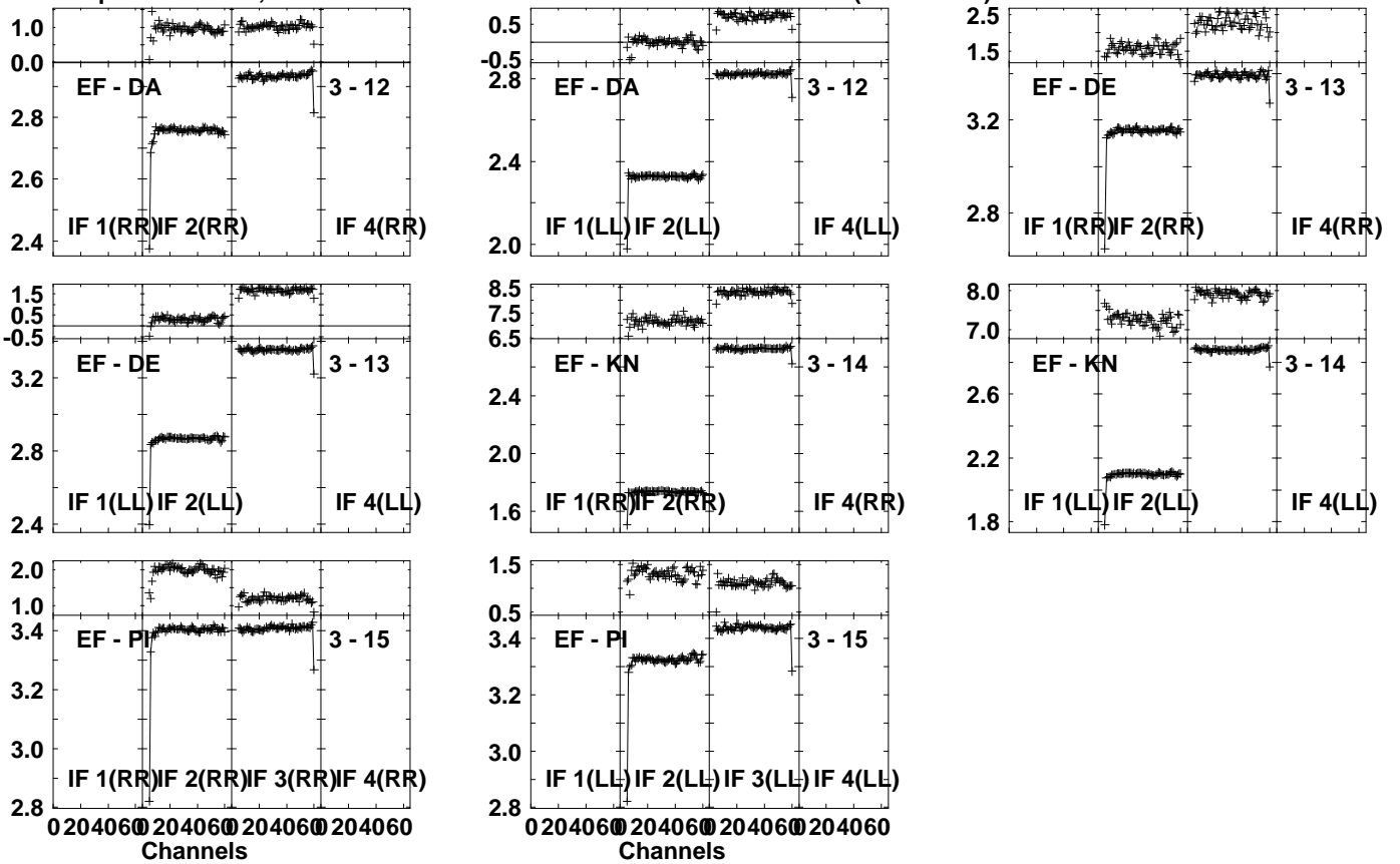
Lower frame: Ampl Jy Top frame: Phas deg Vector averaged cross-power spectrum Several baselines displayed Timerange: 00/19:41:01 to 00/19:45:59
