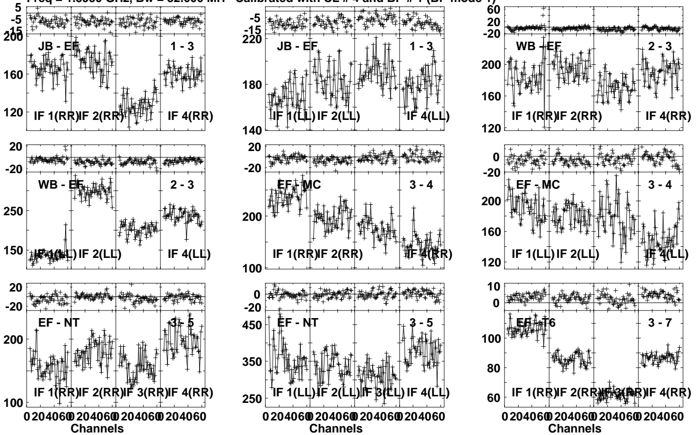
Lower frame: Milli Ampl Jy Top frame: Phas deg Vector averaged cross-power spectrum Several baselines displayed Timerange: 00:19:46:31 to 00:19:47:59
