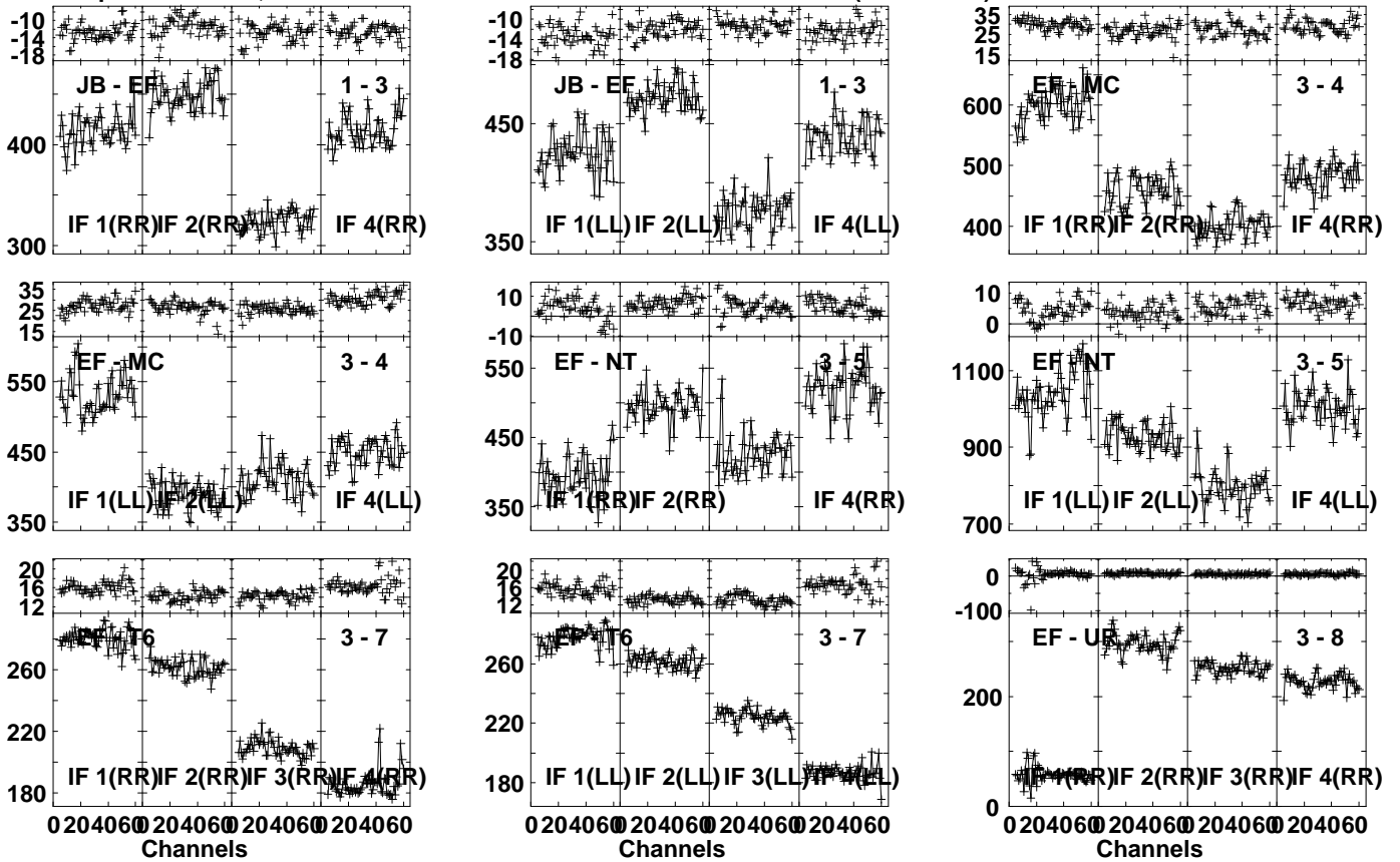
Lower frame: Milli Ampl Jy Top frame: Phas deg Vector averaged cross-power spectrum Several baselines displayed Timerange: 00/10:56:31 to 00/10:57:59
