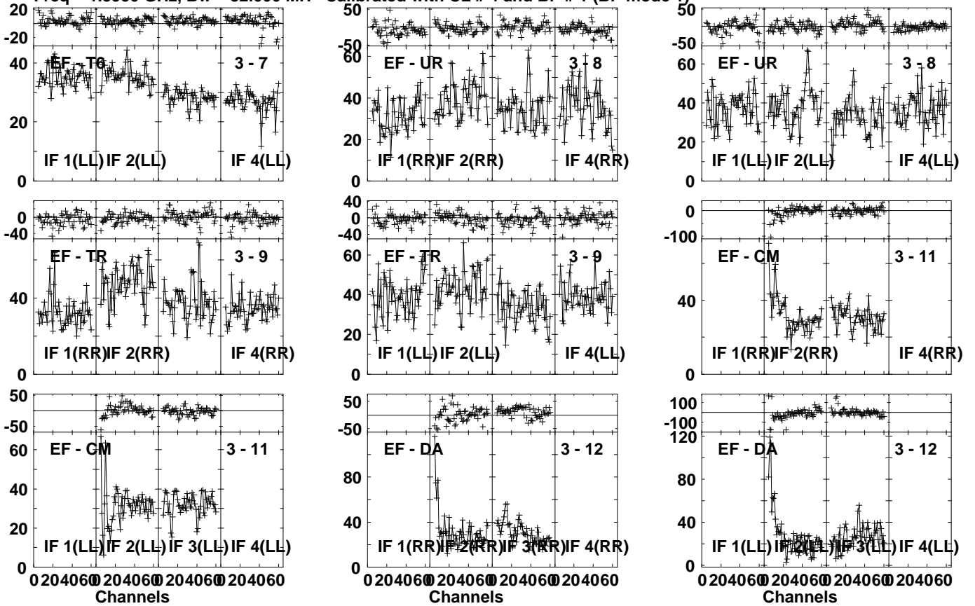
Lower frame: Milli Ampl Jy Top frame: Phas deg Vector averaged cross-power spectrum Several baselines displayed Timerange: 00/15:09:31 to 00/15:10:59
