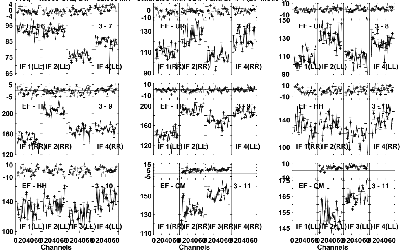
Lower frame: Milli Ampl Jy Top frame: Phas deg Vector averaged cross-power spectrum Several baselines displayed Timerange: 00/19:17:31 to 00/19:18:59
