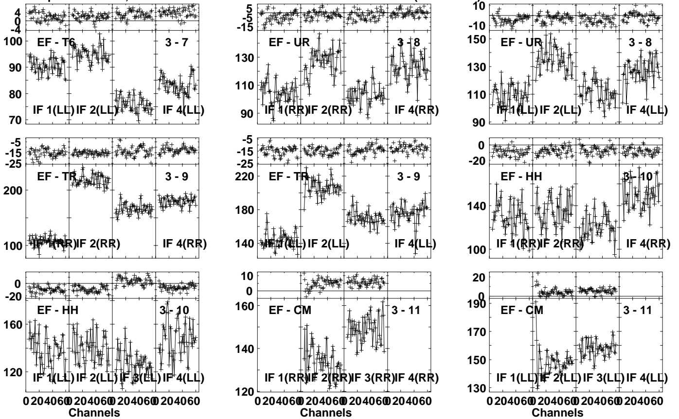
Lower frame: Milli Ampl Jy Top frame: Phas deg Vector averaged cross-power spectrum Several baselines displayed Timerange: 00/17:43:01 to 00/17:44:29
