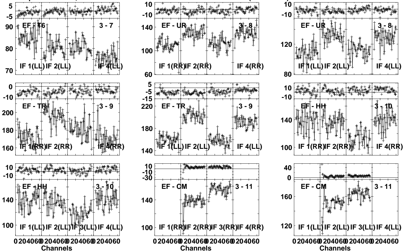
Lower frame: Milli Ampl Jy Top frame: Phas deg Vector averaged cross-power spectrum Several baselines displayed Timerange: 00/20:28:31 to 00/20:29:59
