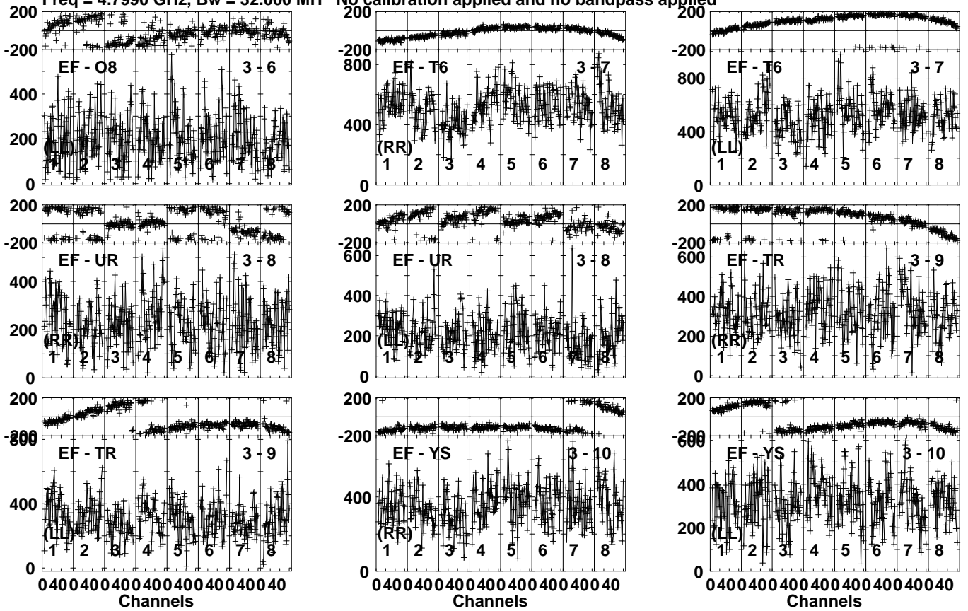
Lower frame: Micro Ampl Jy Top frame: Phas deg Vector averaged cross-power spectrum Several baselines displayed Timerange: 00:16:53:01 to 00:16:54:29
