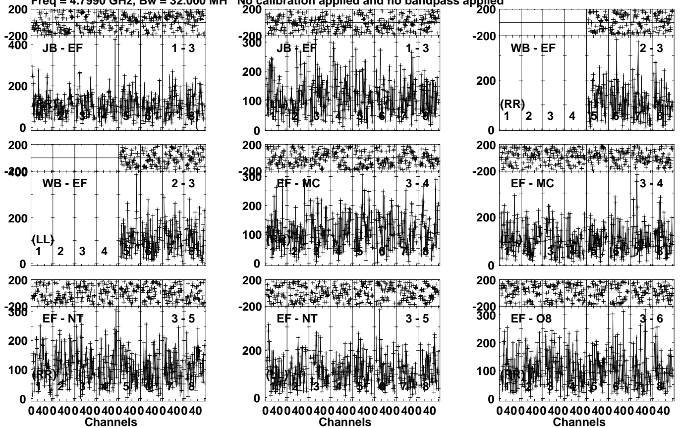
Lower frame: Micro Ampl Jy Top frame: Phas deg Vector averaged cross-power spectrum Several baselines displayed Timerange: 00/13:30:33 to 00/13:32:59
