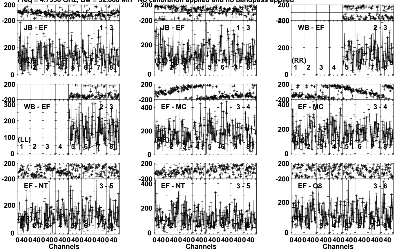
Lower frame: Micro Ampl Jy Top frame: Phas deg Vector averaged cross-power spectrum Several baselines displayed Timerange: 00/16:54:31 to 00/16:56:59
