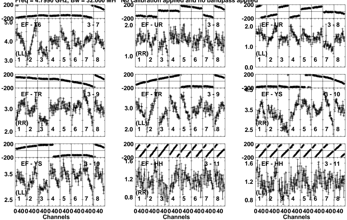
Lower frame: Milli Ampl Jy Top frame: Phas deg Vector averaged cross-power spectrum Several baselines displayed Timerange: 00/19:46:31 to 00/19:47:59
