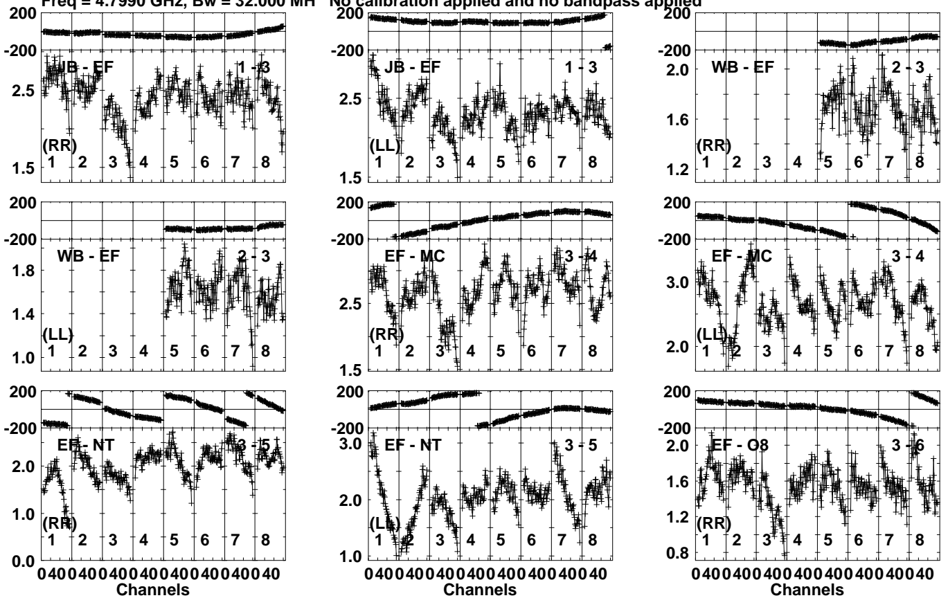
Lower frame: Milli Ampl Jy Top frame: Phas deg Vector averaged cross-power spectrum Several baselines displayed Timerange: 00/19:01:31 to 00/19:02:59
