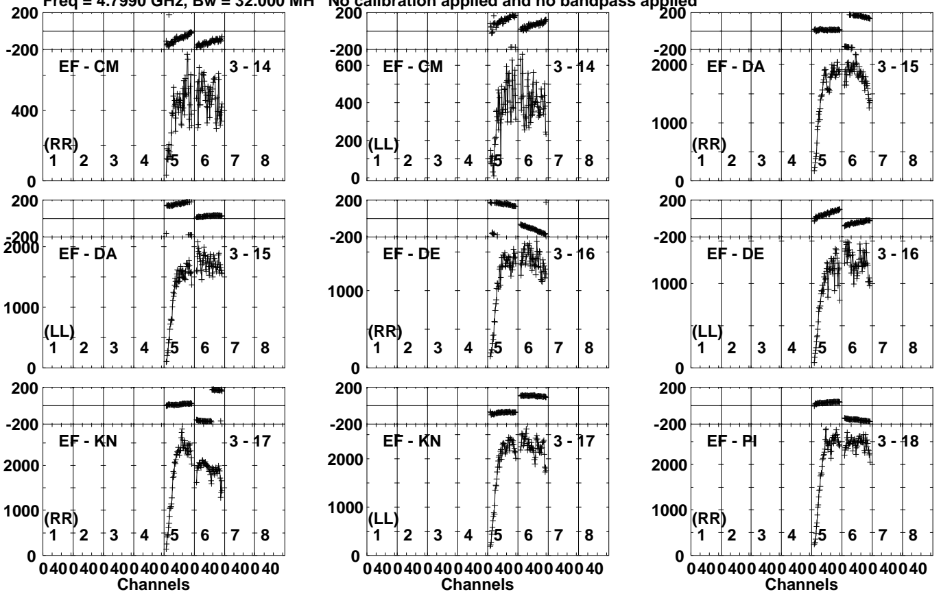
Lower frame: Micro Ampl Jy Top frame: Phas deg Vector averaged cross-power spectrum Several baselines displayed Timerange: 00/13:29:01 to 00/13:30:29
