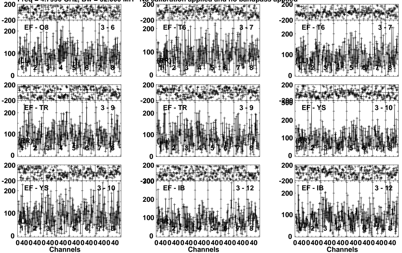
Lower frame: Micro Ampl Jy Top frame: Phas deg Vector averaged cross-power spectrum Several baselines displayed Timerange: 00/12:53:31 to 00/12:56:59
