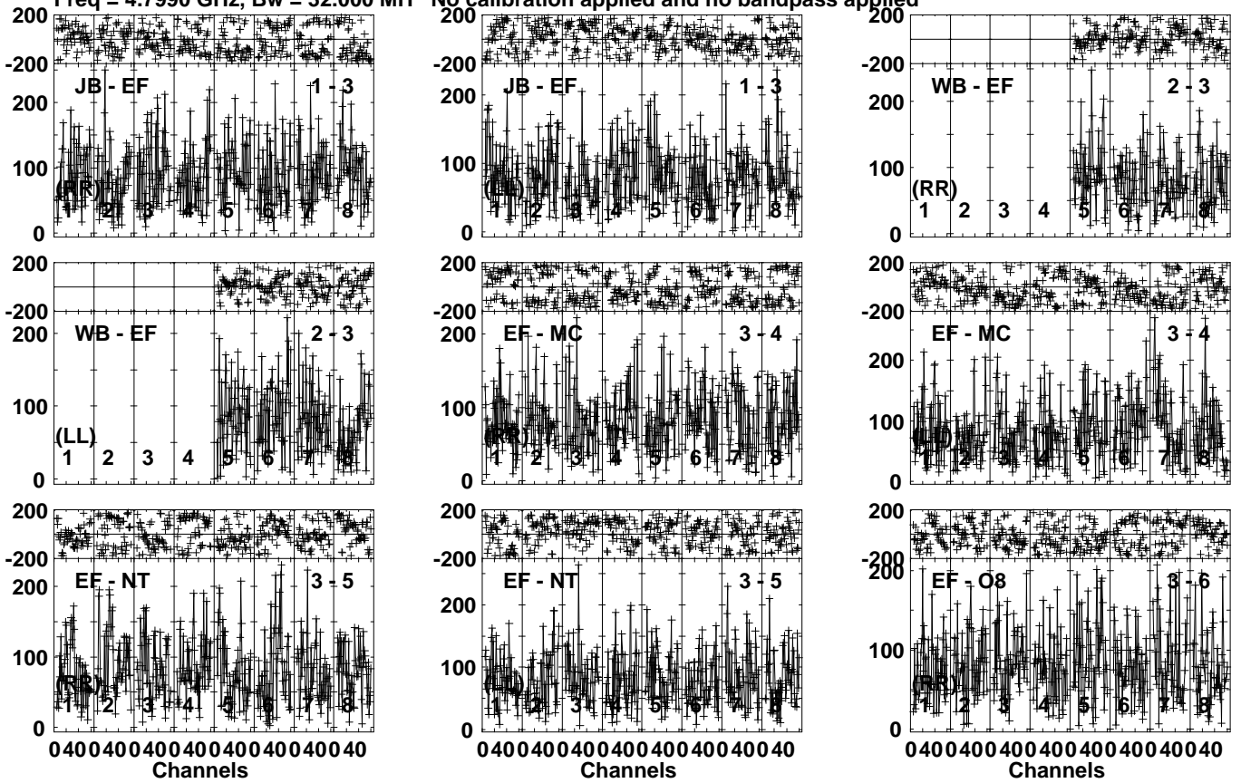
Lower frame: Micro Ampl Jy Top frame: Phas deg Vector averaged cross-power spectrum Several baselines displayed Timerange: 00/20:19:31 to 00/20:22:59
