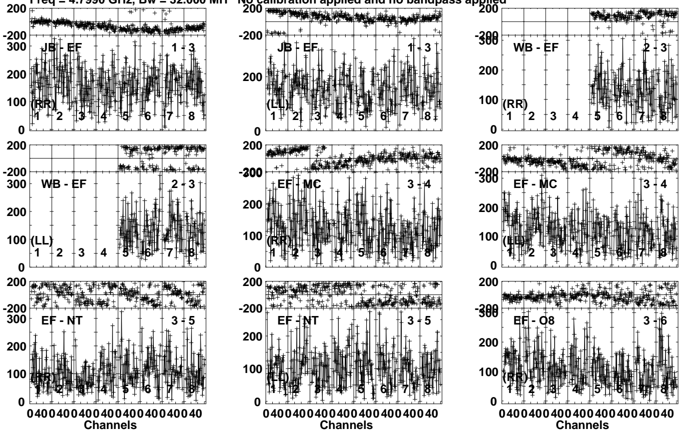
Lower frame: Micro Ampl Jy Top frame: Phas deg Vector averaged cross-power spectrum Several baselines displayed Timerange: 00/16:07:01 to 00/16:10:29
