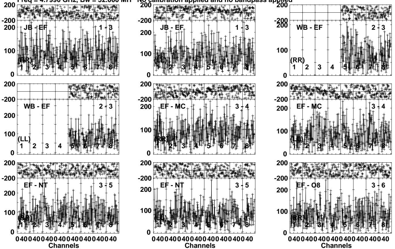
Lower frame: Micro Ampl Jy Top frame: Phas deg Vector averaged cross-power spectrum Several baselines displayed Timerange: 00/18:00:01 to 00/18:03:29
