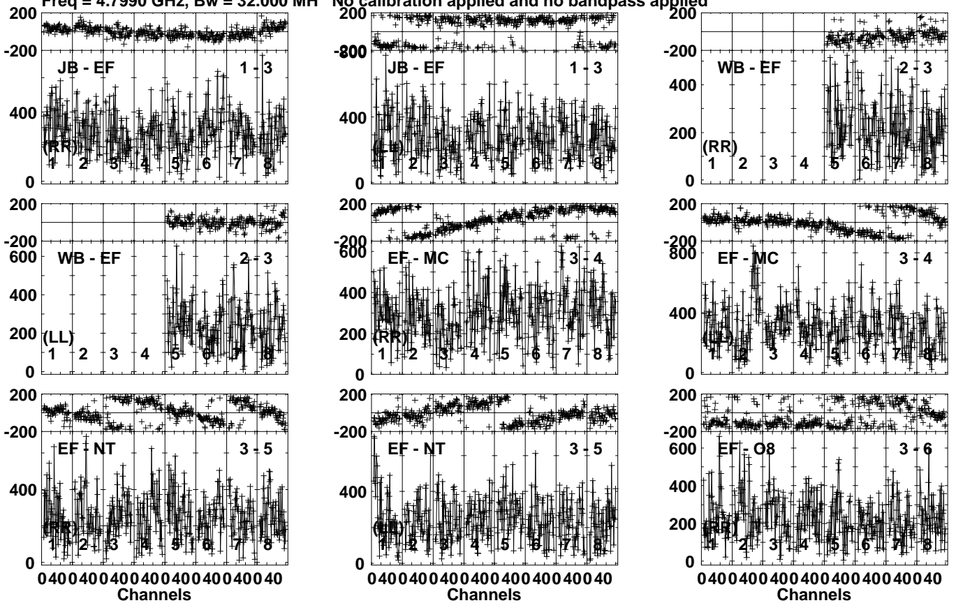
Lower frame: Micro Ampl Jy Top frame: Phas deg Vector averaged cross-power spectrum Several baselines displayed Timerange: 00/16:26:31 to 00/16:27:59
