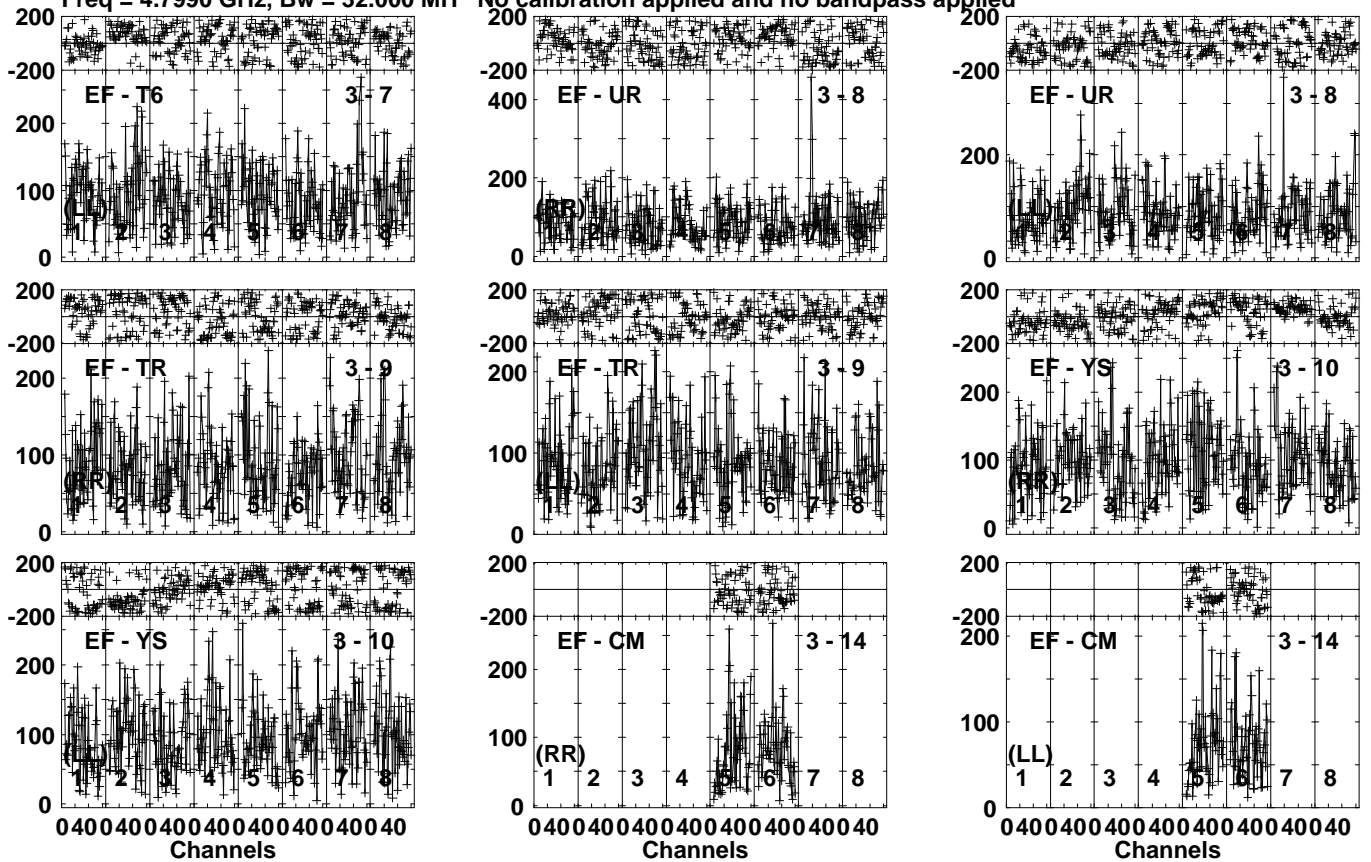
Lower frame: Micro Ampl Jy Top frame: Phas deg Vector averaged cross-power spectrum Several baselines displayed Timerange: 00/10:32:03 to 00/10:35:29
