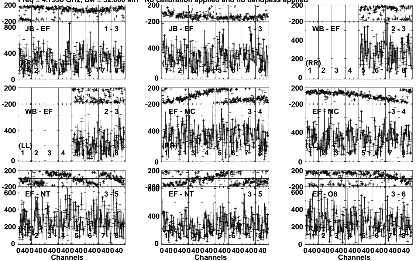
Lower frame: Micro Ampl Jy Top frame: Phas deg Vector averaged cross-power spectrum Several baselines displayed Timerange: 00/15:14:31 to 00/15:15:59
