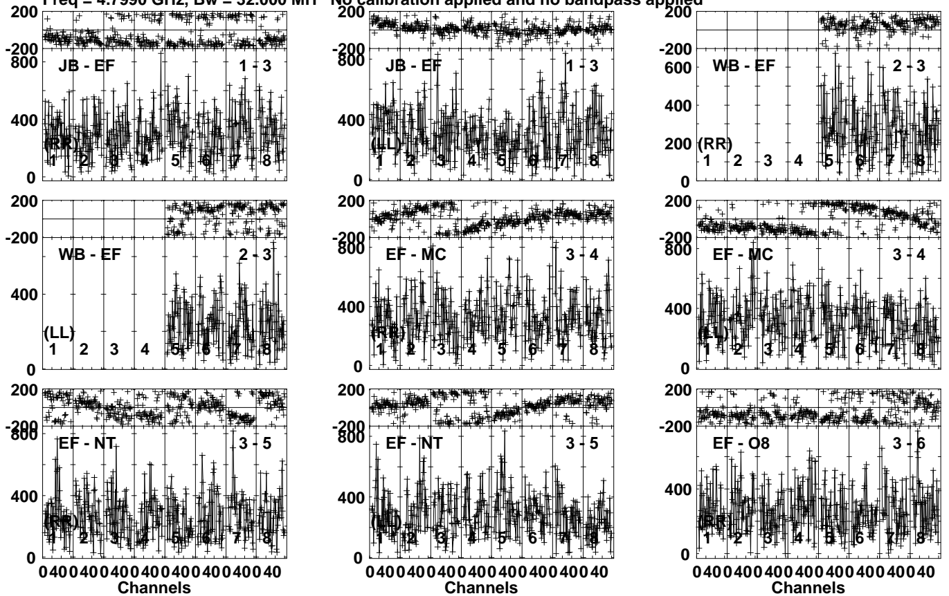
Lower frame: Micro Ampl Jy Top frame: Phas deg Vector averaged cross-power spectrum Several baselines displayed Timerange: 00/15:55:01 to 00/15:56:29
