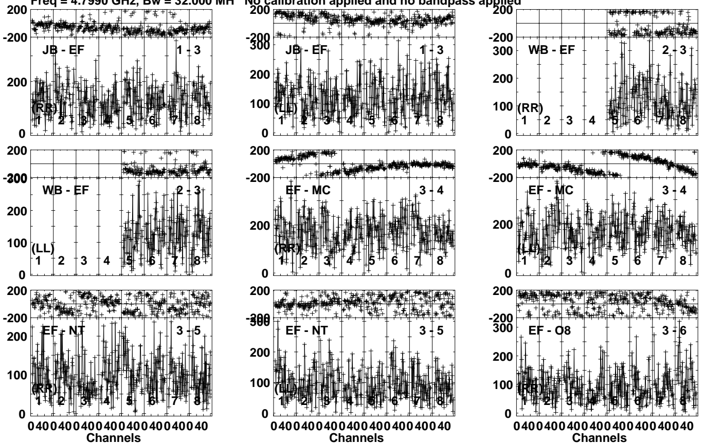
Lower frame: Micro Ampl Jy Top frame: Phas deg Vector averaged cross-power spectrum Several baselines displayed Timerange: 00:16:49:01 to 00:16:52:29
