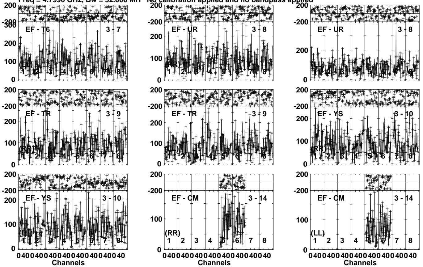
Lower frame: Micro Ampl Jy Top frame: Phas deg Vector averaged cross-power spectrum Several baselines displayed Timerange: 00/11:14:01 to 00/11:17:29
