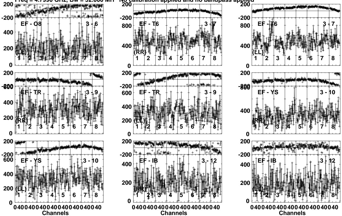
Lower frame: Micro Ampl Jy Top frame: Phas deg Vector averaged cross-power spectrum Several baselines displayed Timerange: 00/15:41:01 to 00/15:42:29
