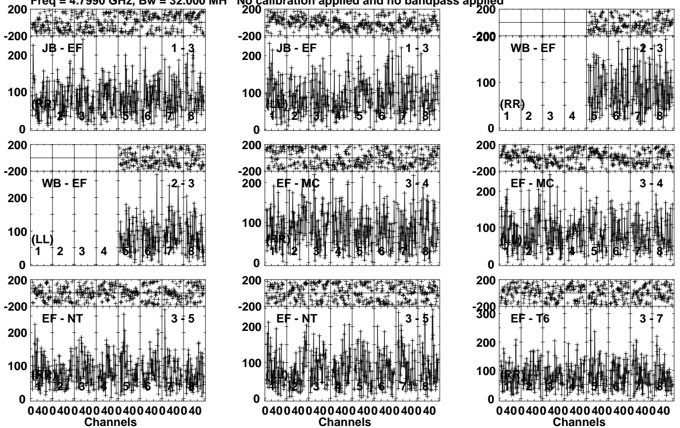
Lower frame: Micro Ampl Jy Top frame: Phas deg Vector averaged cross-power spectrum Several baselines displayed Timerange: 00/19:48:01 to 00/19:51:29
