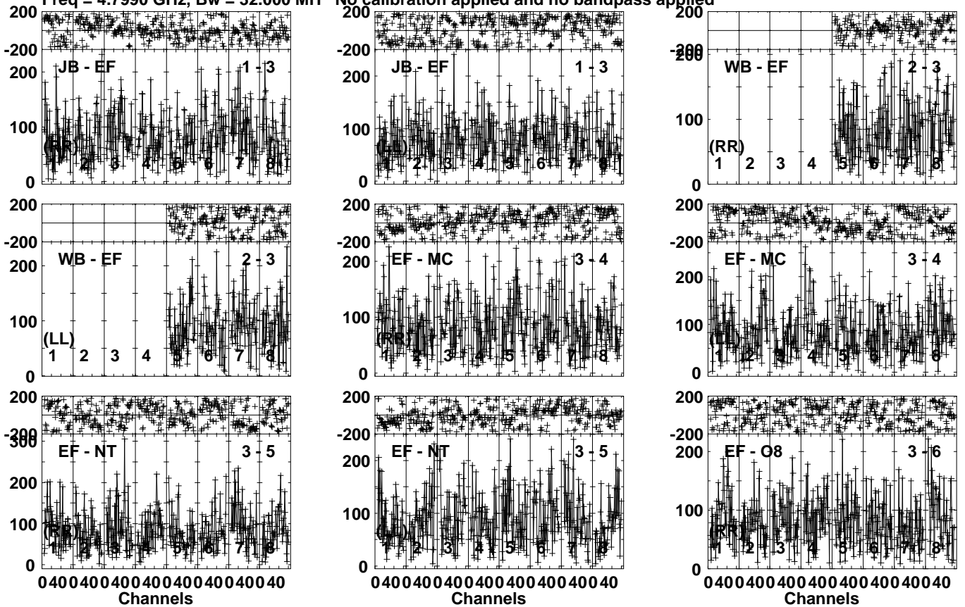
Lower frame: Micro Ampl Jy Top frame: Phas deg Vector averaged cross-power spectrum Several baselines displayed Timerange: 00/18:10:31 to 00/18:13:59
