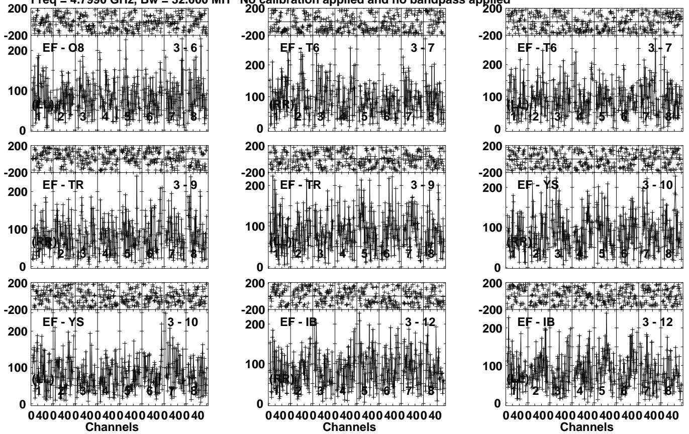
Lower frame: Micro Ampl Jy Top frame: Phas deg Vector averaged cross-power spectrum Several baselines displayed Timerange: 00/12:59:01 to 00/13:02:29
