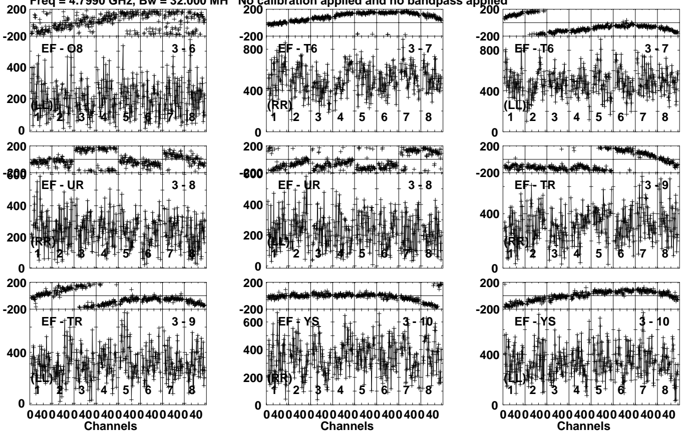
Lower frame: Micro Ampl Jy Top frame: Phas deg Vector averaged cross-power spectrum Several baselines displayed Timerange: 00/17:18:31 to 00/17:19:59
