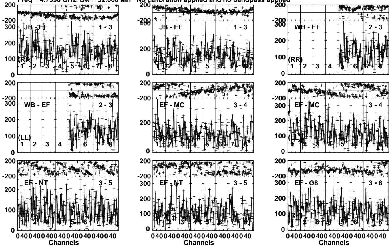
Lower frame: Micro Ampl Jy Top frame: Phas deg Vector averaged cross-power spectrum Several baselines displayed Timerange: 00/16:02:01 to 00/16:05:29
