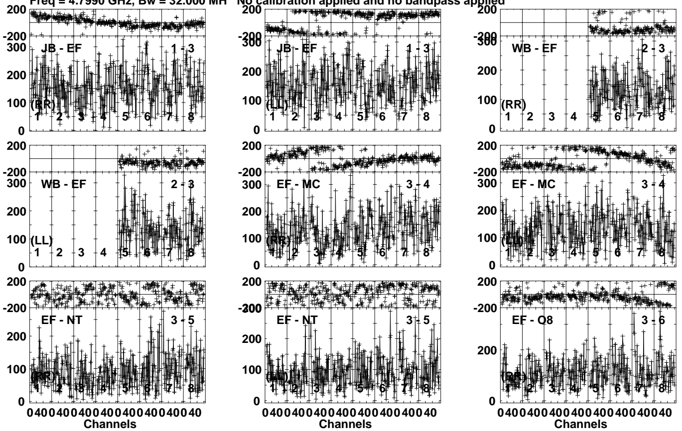
Lower frame: Micro Ampl Jy Top frame: Phas deg Vector averaged cross-power spectrum Several baselines displayed Timerange: 00/15:16:01 to 00/15:19:29
