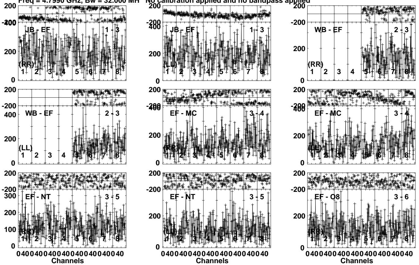
Lower frame: Micro Ampl Jy Top frame: Phas deg Vector averaged cross-power spectrum Several baselines displayed Timerange: 00/17:20:01 to 00/17:22:29
