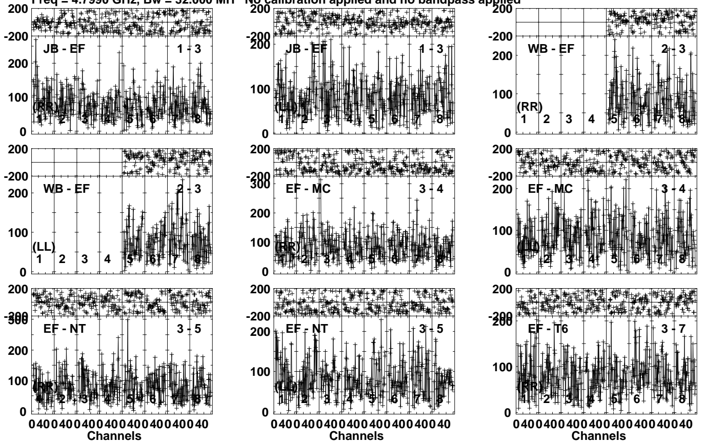
Lower frame: Micro Ampl Jy Top frame: Phas deg Vector averaged cross-power spectrum Several baselines displayed Timerange: 00/19:24:03 to 00/19:27:29
