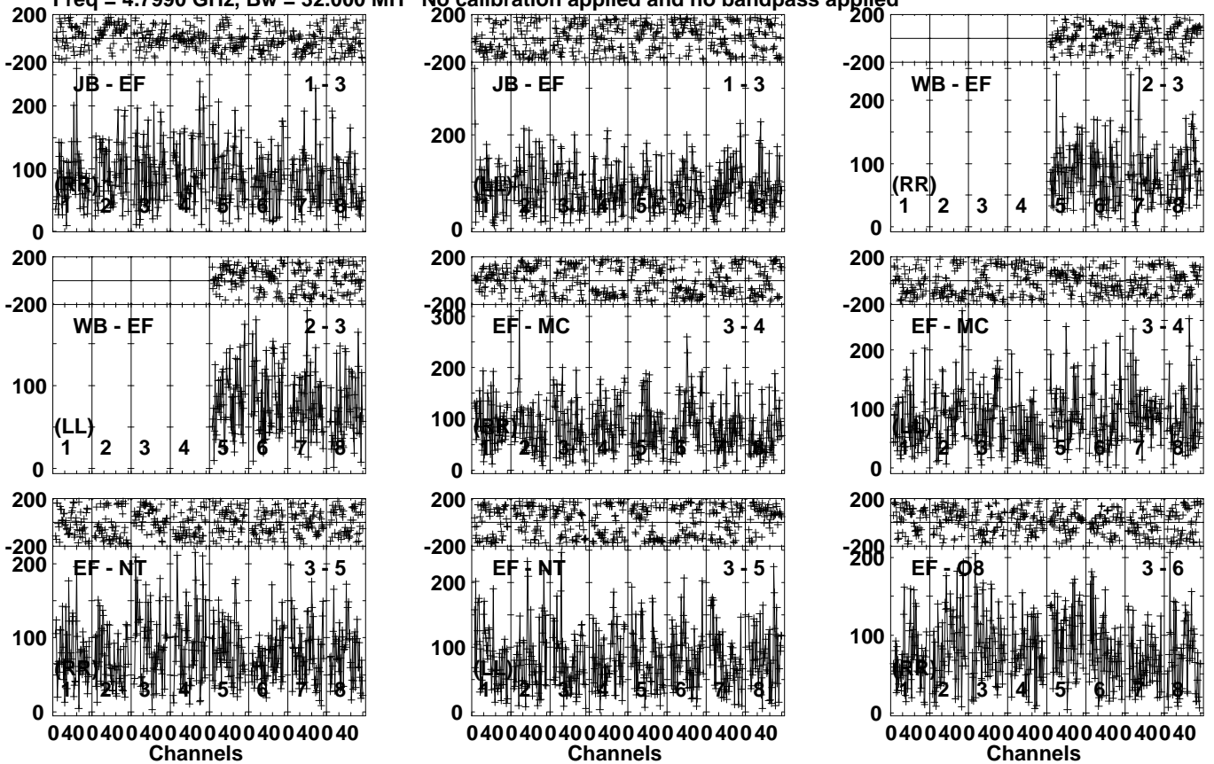
Lower frame: Micro Ampl Jy Top frame: Phas deg Vector averaged cross-power spectrum Several baselines displayed Timerange: 00/18:58:01 to 00/19:01:29
