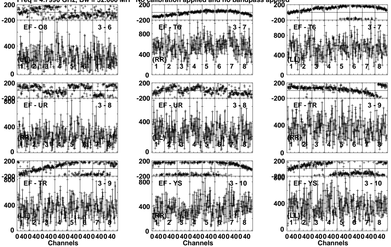
Lower frame: Micro Ampl Jy Top frame: Phas deg Vector averaged cross-power spectrum Several baselines displayed Timerange: 00/16:57:01 to 00/16:58:29
