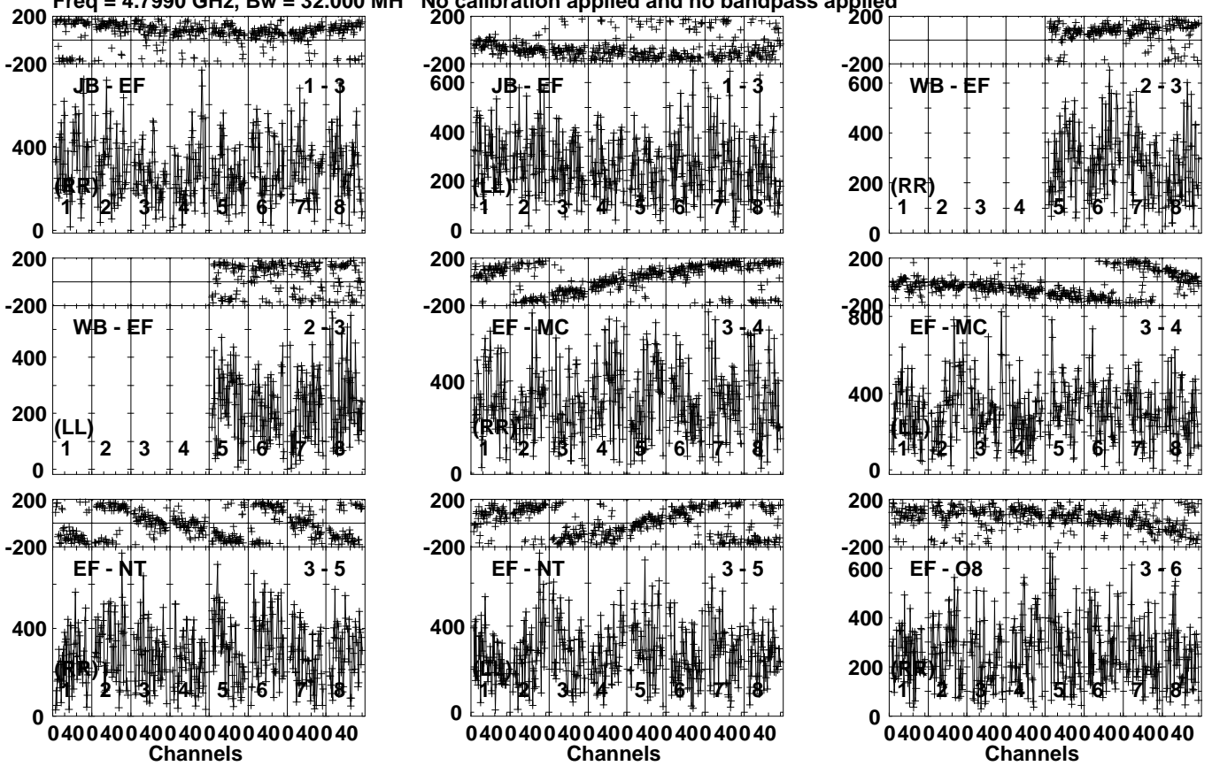
Lower frame: Micro Ampl Jy Top frame: Phas deg Vector averaged cross-power spectrum Several baselines displayed Timerange: 00/15:25:01 to 00/15:26:29
