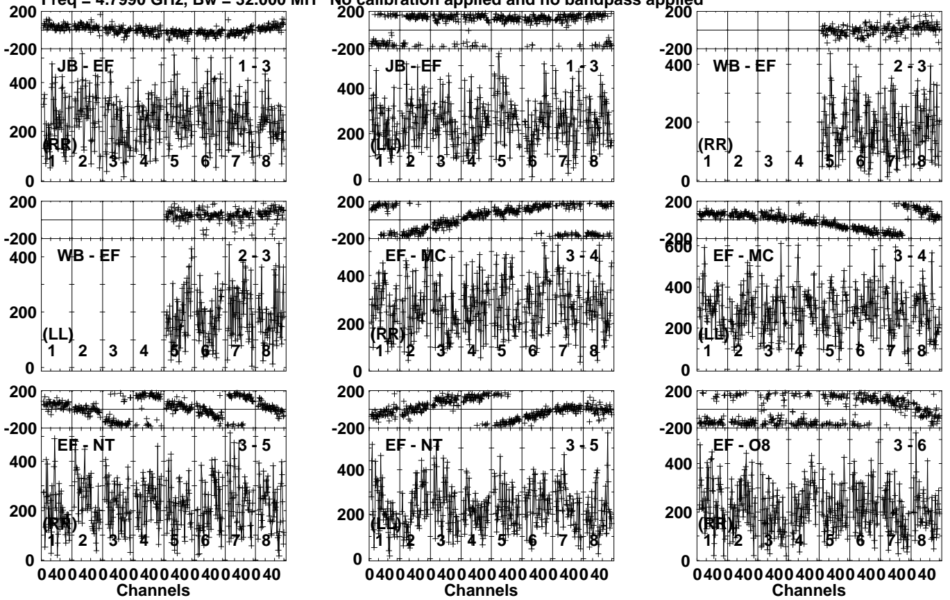
Lower frame: Micro Ampl Jy Top frame: Phas deg Vector averaged cross-power spectrum Several baselines displayed Timerange: 00/16:21:31 to 00/16:22:59
