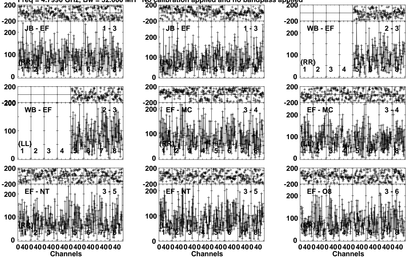
Lower frame: Micro Ampl Jy Top frame: Phas deg Vector averaged cross-power spectrum Several baselines displayed Timerange: 00/20:24:31 to 00/20:27:59
