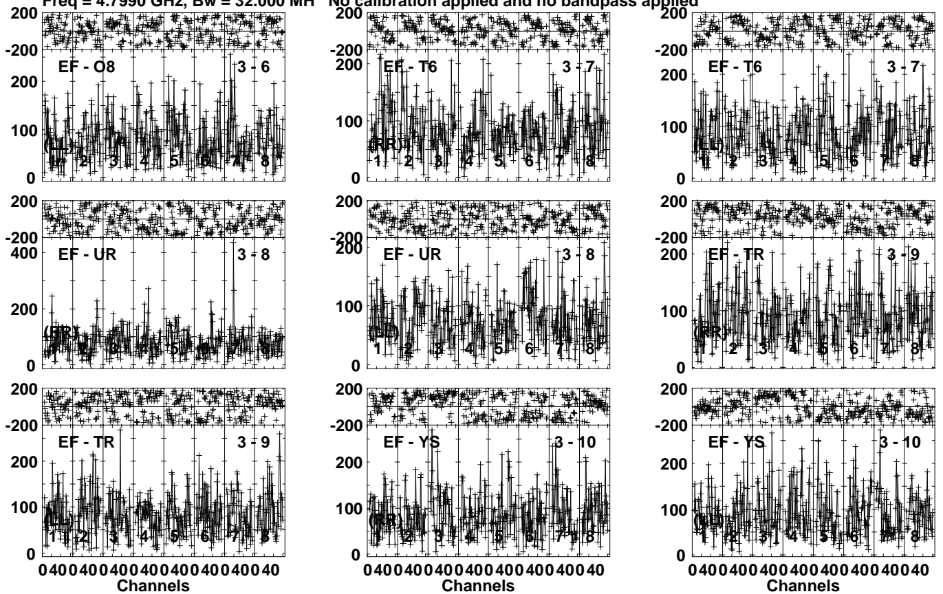
Lower frame: Micro Ampl Jy Top frame: Phas deg Vector averaged cross-power spectrum Several baselines displayed Timerange: 00/17:39:01 to 00/17:42:29
