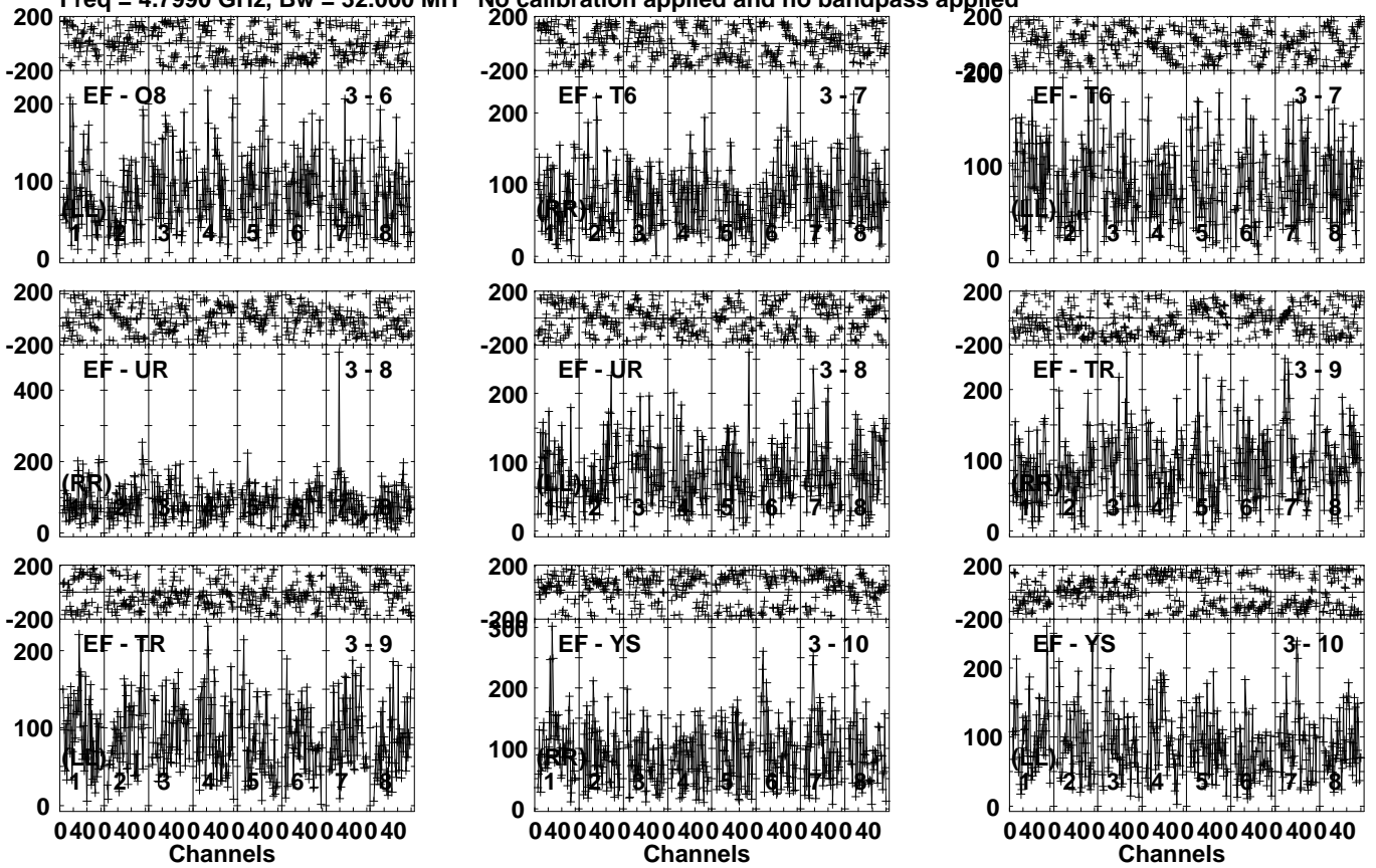
Lower frame: Micro Ampl Jy Top frame: Phas deg Vector averaged cross-power spectrum Several baselines displayed Timerange: 00/18:21:01 to 00/18:24:29
