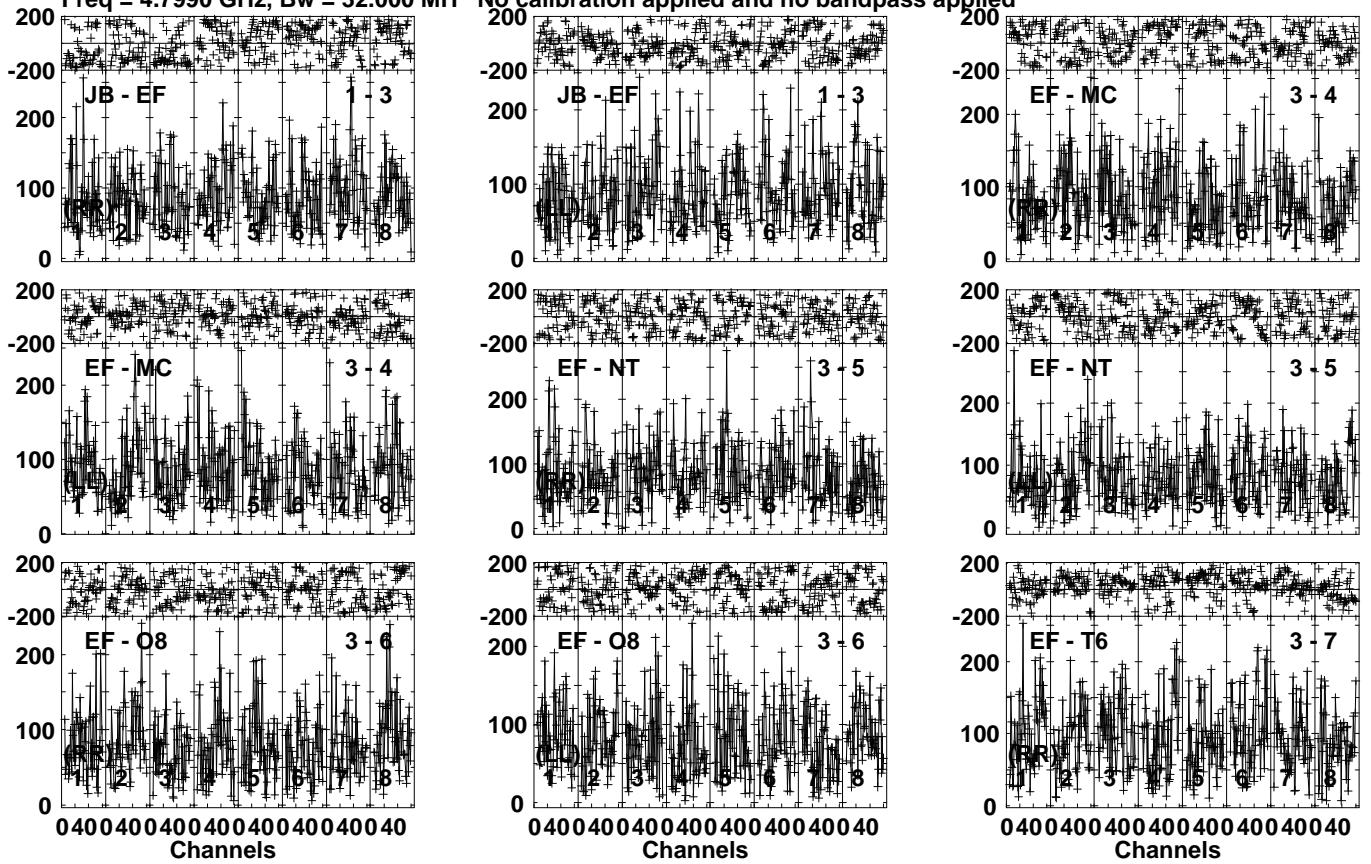
Lower frame: Micro Ampl Jy Top frame: Phas deg Vector averaged cross-power spectrum Several baselines displayed Timerange: 00/11:45:31 to 00/11:48:59
