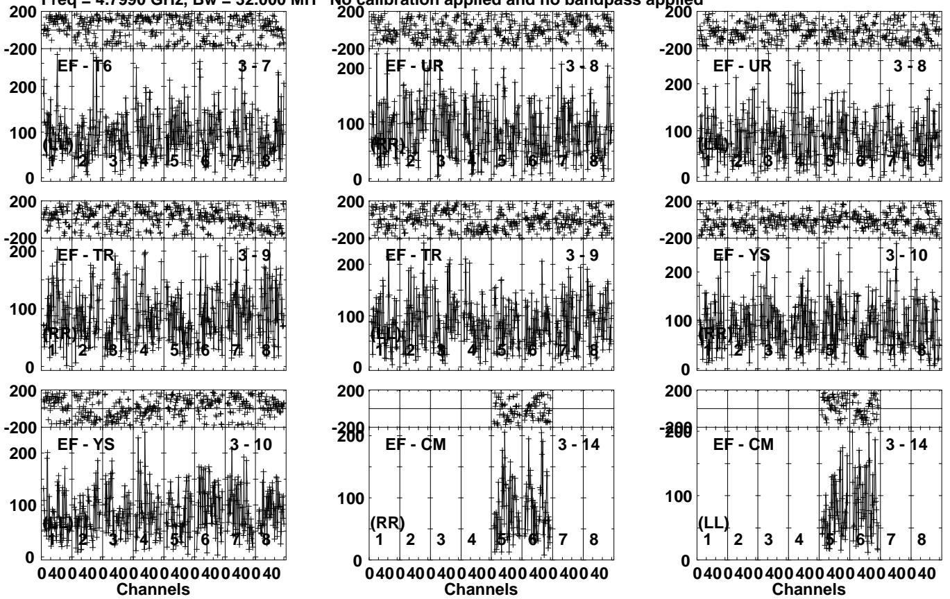
Lower frame: Micro Ampl Jy Top frame: Phas deg Vector averaged cross-power spectrum Several baselines displayed Timerange: 00/11:29:33 to 00/11:32:59
