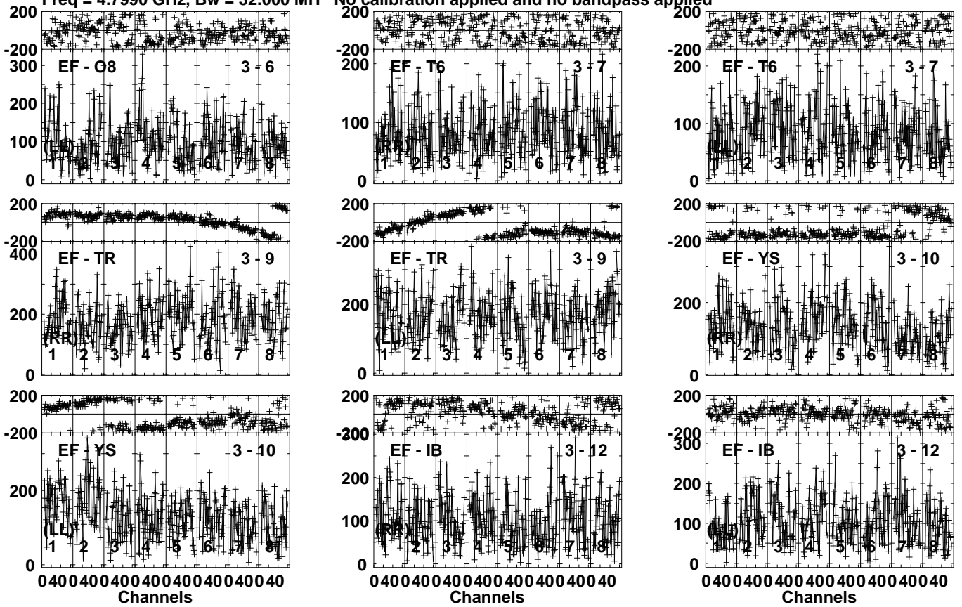
Lower frame: Micro Ampl Jy Top frame: Phas deg Vector averaged cross-power spectrum Several baselines displayed Timerange: 00/14:34:01 to 00/14:37:29
