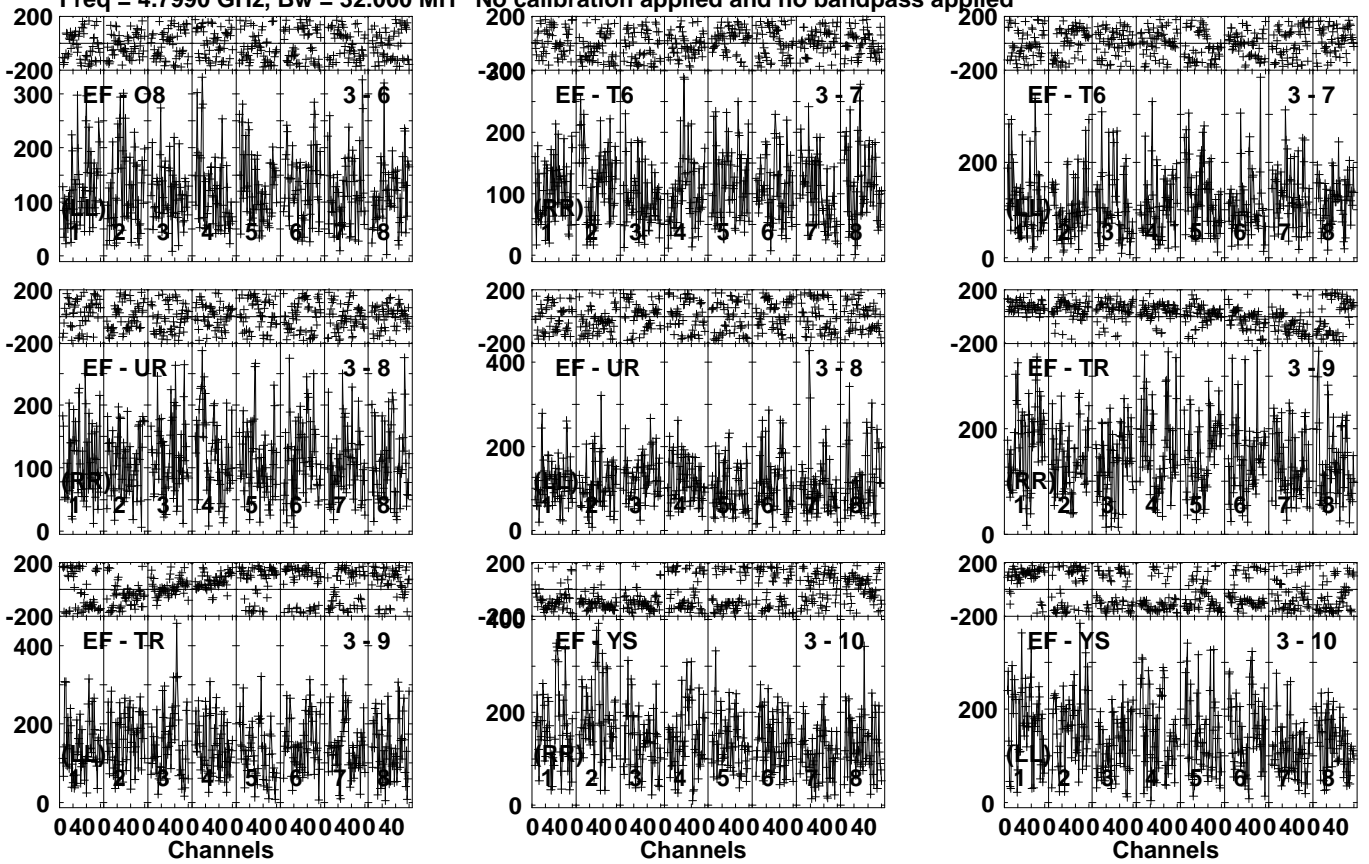
Lower frame: Micro Ampl Jy Top frame: Phas deg Vector averaged cross-power spectrum Several baselines displayed Timerange: 00/17:11:33 to 00/17:13:59
