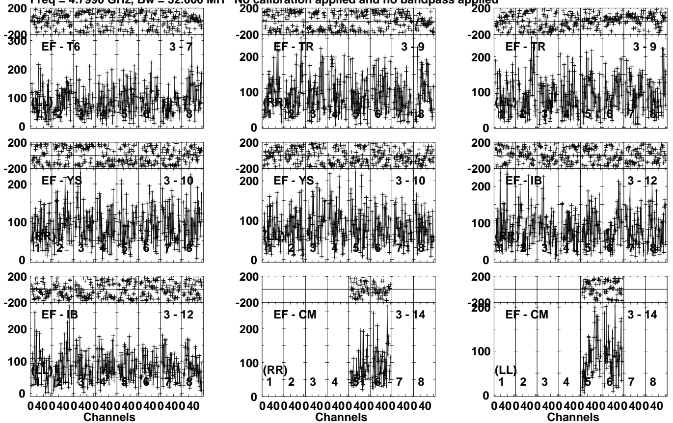
Lower frame: Micro Ampl Jy Top frame: Phas deg Vector averaged cross-power spectrum Several baselines displayed Timerange: 00/12:43:03 to 00/12:46:29
