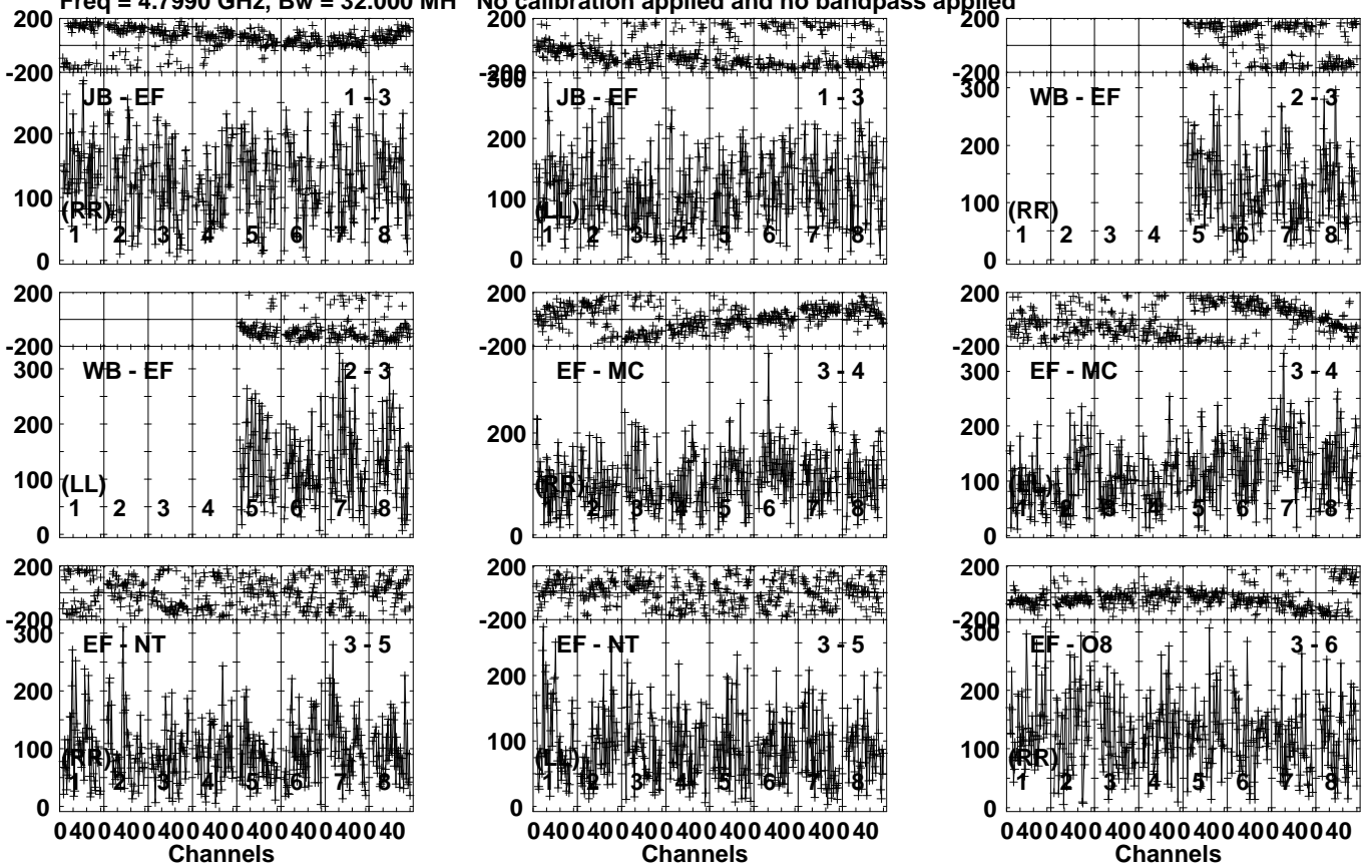
Lower frame: Micro Ampl Jy Top frame: Phas deg Vector averaged cross-power spectrum Several baselines displayed Timerange: 00/15:37:01 to 00/15:40:29
