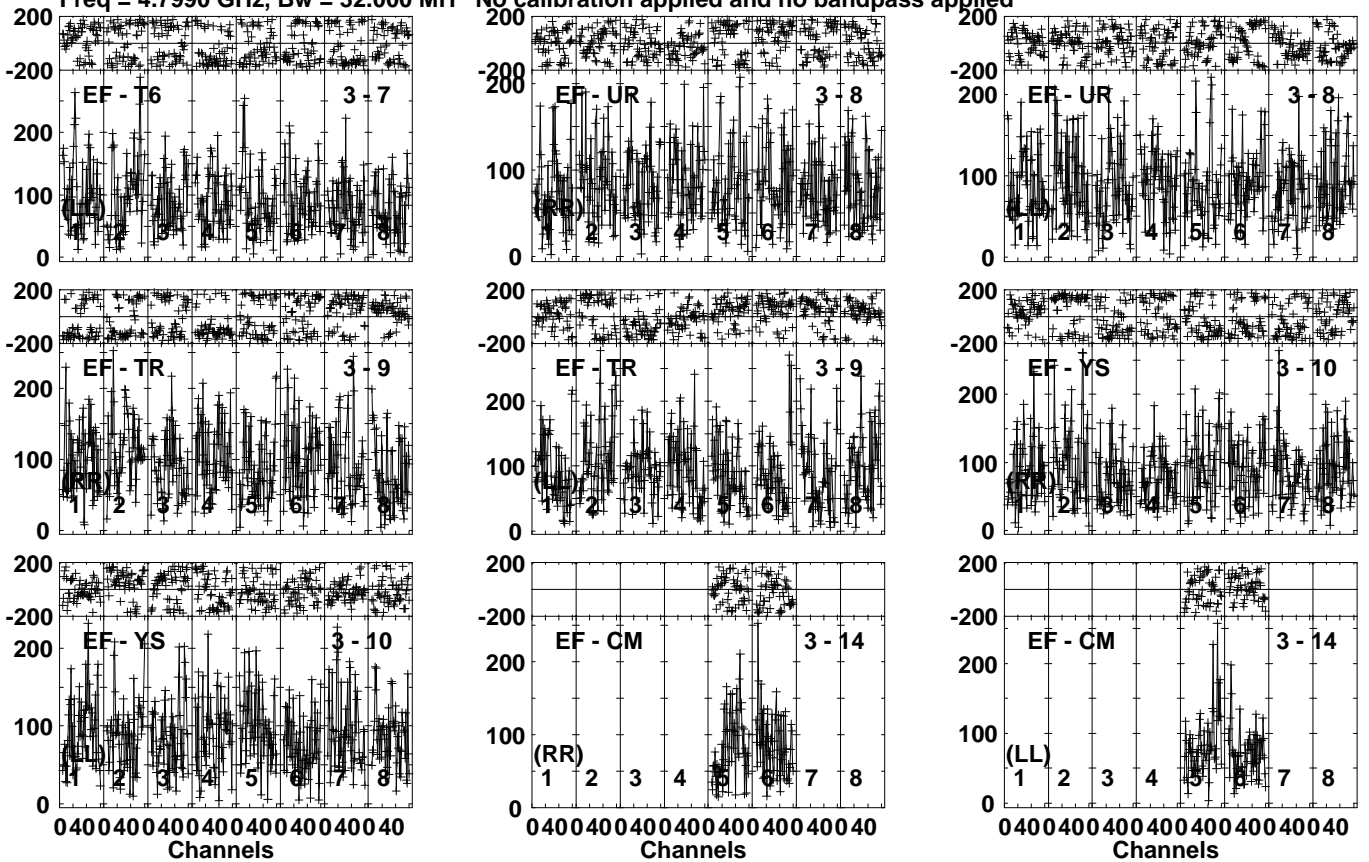
Lower frame: Micro Ampl Jy Top frame: Phas deg Vector averaged cross-power spectrum Several baselines displayed Timerange: 00/11:19:03 to 00/11:22:29
