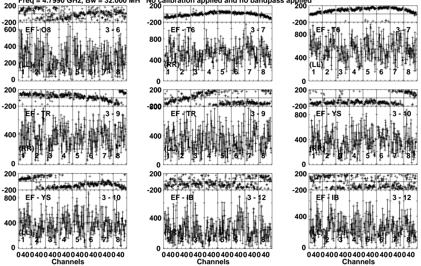
Lower frame: Micro Ampl Jy Top frame: Phas deg Vector averaged cross-power spectrum Several baselines displayed Timerange: 00/16:05:31 to 00/16:06:59
