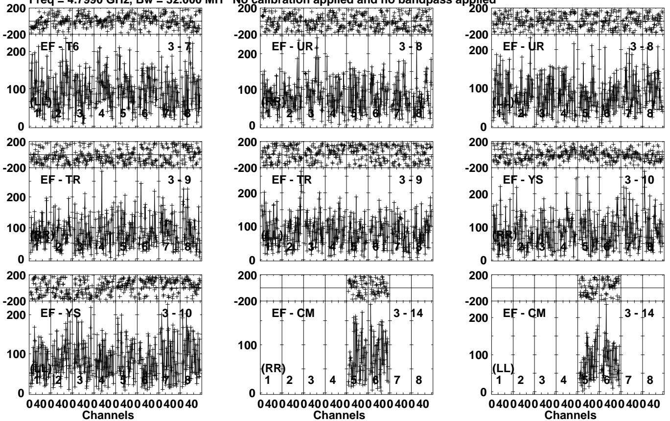
Lower frame: Micro Ampl Jy Top frame: Phas deg Vector averaged cross-power spectrum Several baselines displayed Timerange: 00/11:50:33 to 00/11:53:59
