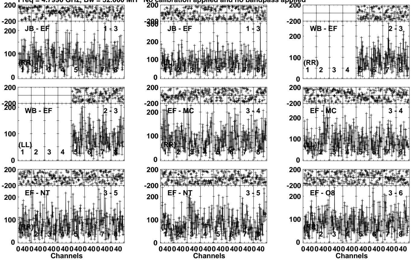
Lower frame: Micro Ampl Jy Top frame: Phas deg Vector averaged cross-power spectrum Several baselines displayed Timerange: 00/17:55:01 to 00/17:58:29
