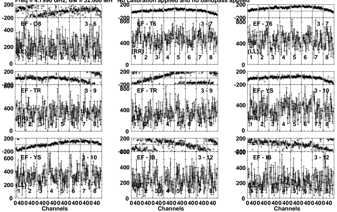
Lower frame: Micro Ampl Jy Top frame: Phas deg Vector averaged cross-power spectrum Several baselines displayed Timerange: 00/14:22:01 to 00/14:23:29
