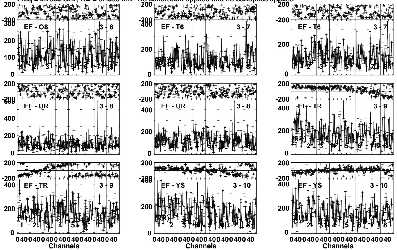
Lower frame: Micro Ampl Jy Top frame: Phas deg Vector averaged cross-power spectrum Several baselines displayed Timerange: 00/17:03:01 to 00/17:05:29
