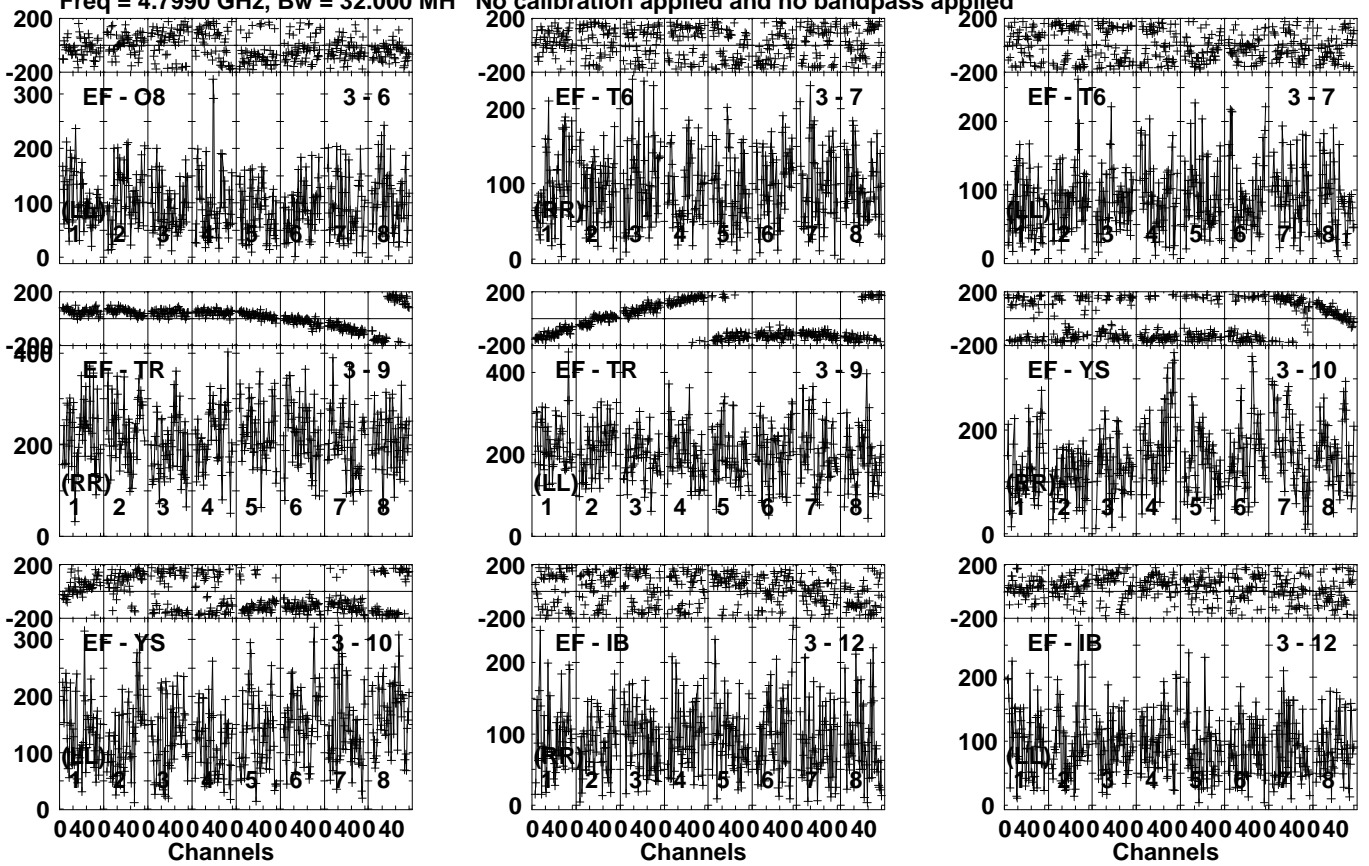
Lower frame: Micro Ampl Jy Top frame: Phas deg Vector averaged cross-power spectrum Several baselines displayed Timerange: 00/14:55:01 to 00/14:58:29
