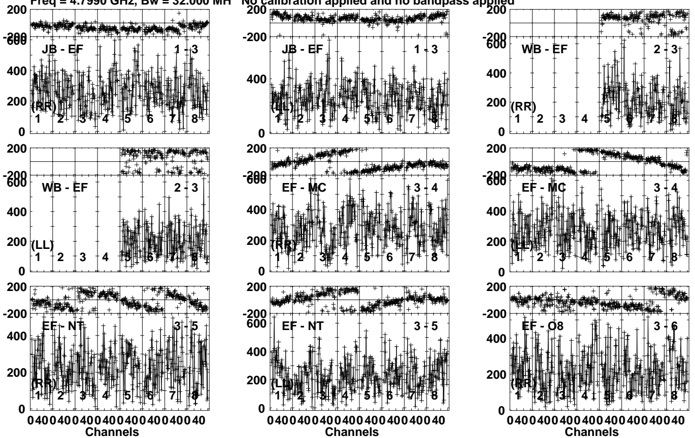
Lower frame: Micro Ampl Jy Top frame: Phas deg Vector averaged cross-power spectrum Several baselines displayed Timerange: 00/17:23:01 to 00/17:24:29
