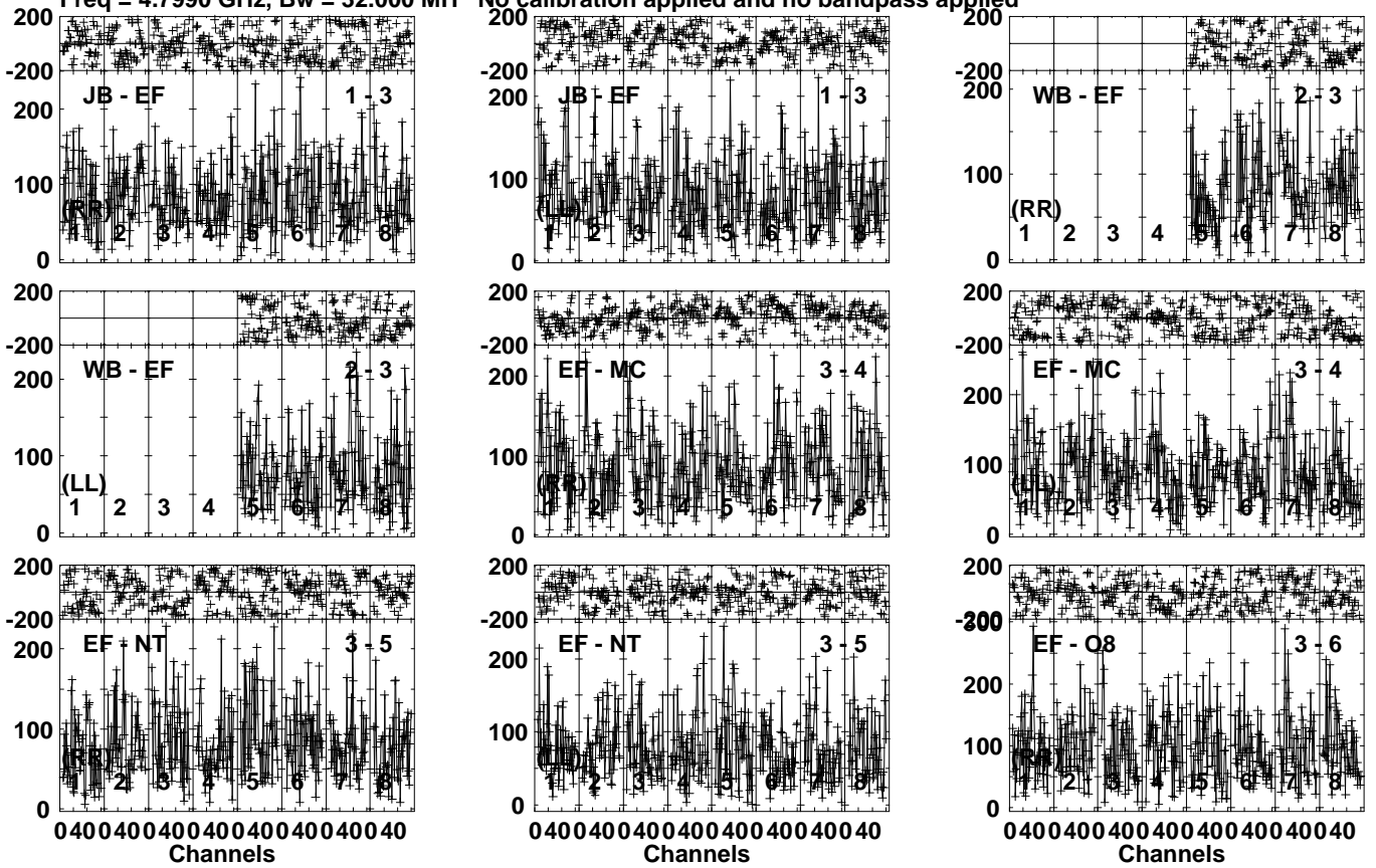
Lower frame: Micro Ampl Jy Top frame: Phas deg Vector averaged cross-power spectrum Several baselines displayed Timerange: 00/19:13:31 to 00/19:16:59
