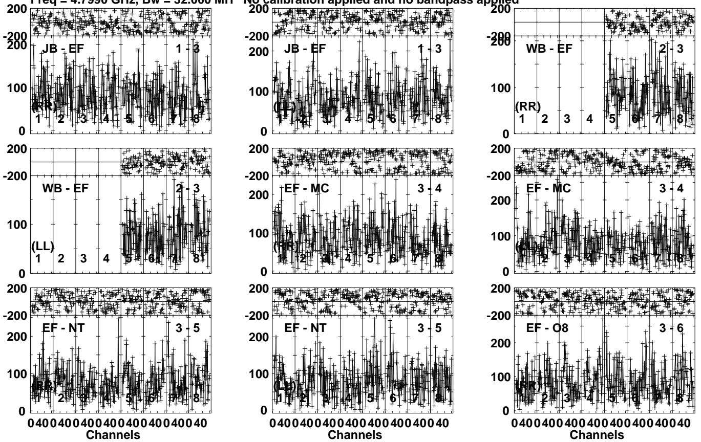
Lower frame: Micro Ampl Jy Top frame: Phas deg Vector averaged cross-power spectrum Several baselines displayed Timerange: 00/19:03:01 to 00/19:06:29
