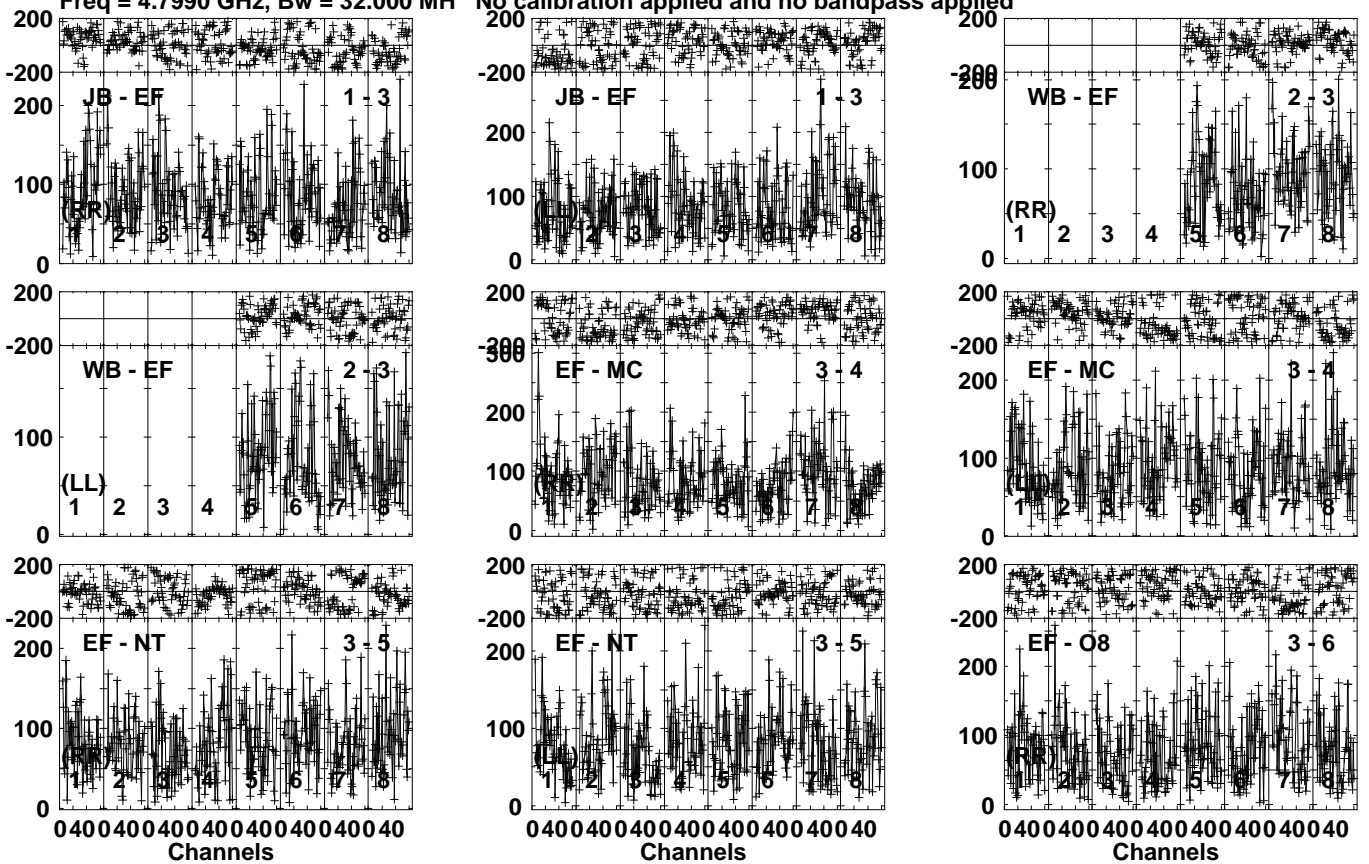
Lower frame: Micro Ampl Jy Top frame: Phas deg Vector averaged cross-power spectrum Several baselines displayed Timerange: 00/18:16:01 to 00/18:19:29
