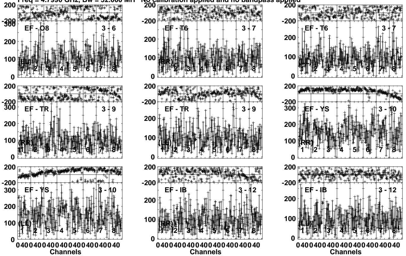
Lower frame: Micro Ampl Jy Top frame: Phas deg Vector averaged cross-power spectrum Several baselines displayed Timerange: 00/15:11:01 to 00/15:14:29
