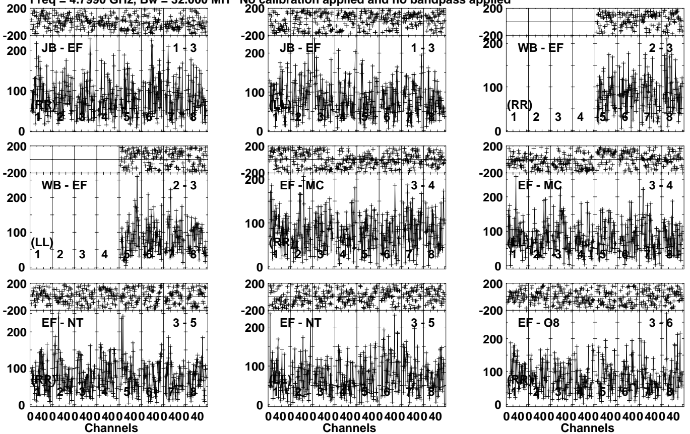
Lower frame: Micro Ampl Jy Top frame: Phas deg Vector averaged cross-power spectrum Several baselines displayed Timerange: 00/17:34:01 to 00/17:37:29
