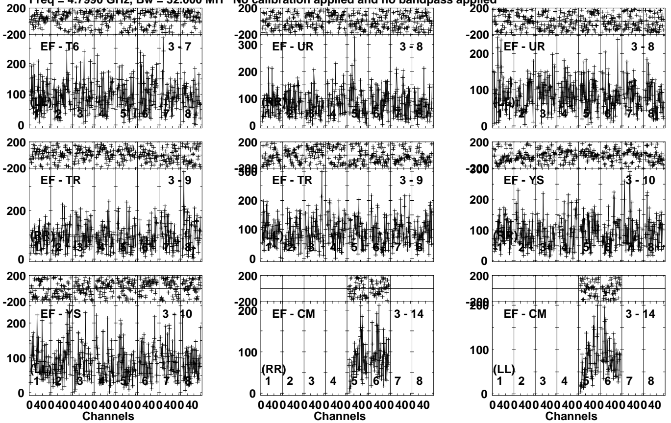
Lower frame: Micro Ampl Jy Top frame: Phas deg Vector averaged cross-power spectrum Several baselines displayed Timerange: 00/11:35:01 to 00/11:38:29
