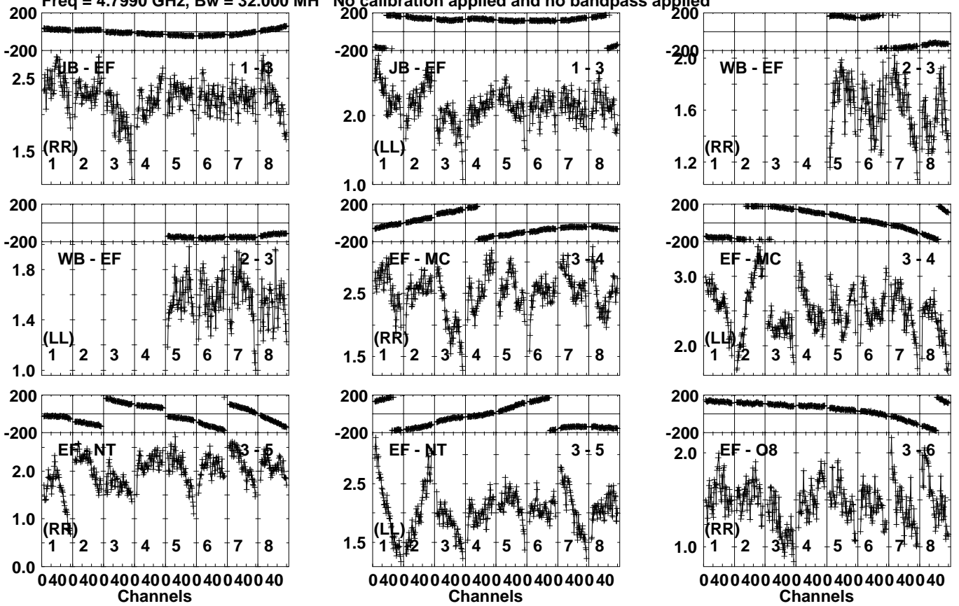
Lower frame: Milli Ampl Jy Top frame: Phas deg Vector averaged cross-power spectrum Several baselines displayed Timerange: 00/17:48:01 to 00/17:49:29
