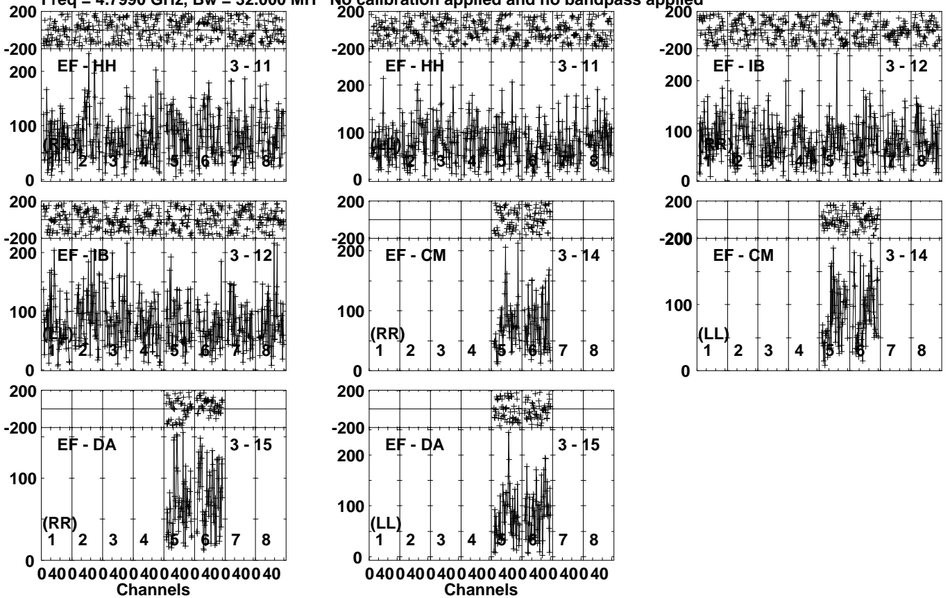
Lower frame: Micro Ampl Jy Top frame: Phas deg Vector averaged cross-power spectrum Several baselines displayed Timerange: 00/18:42:01 to 00/18:45:29
