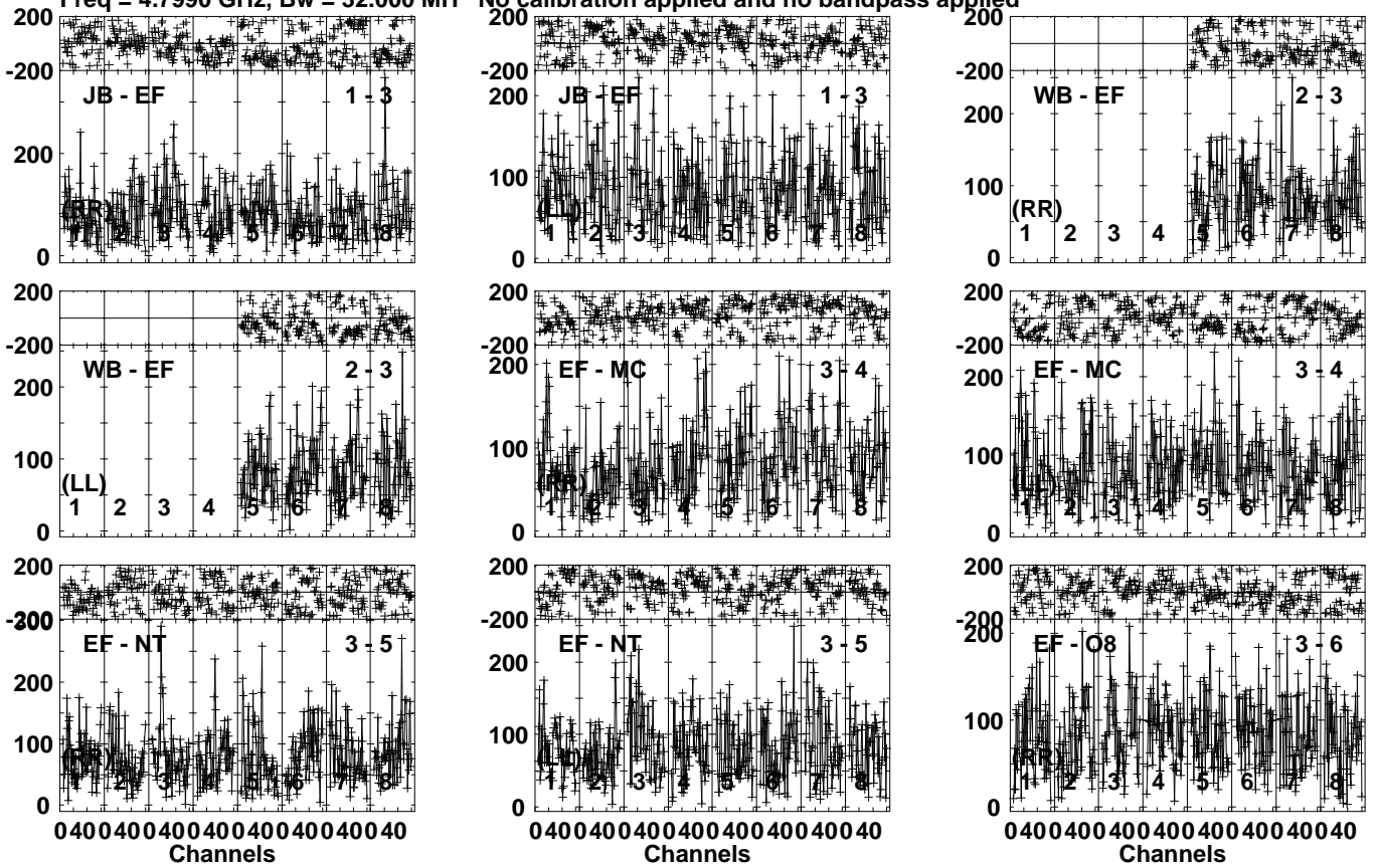
Lower frame: Micro Ampl Jy Top frame: Phas deg Vector averaged cross-power spectrum Several baselines displayed Timerange: 00/19:08:31 to 00/19:11:59
