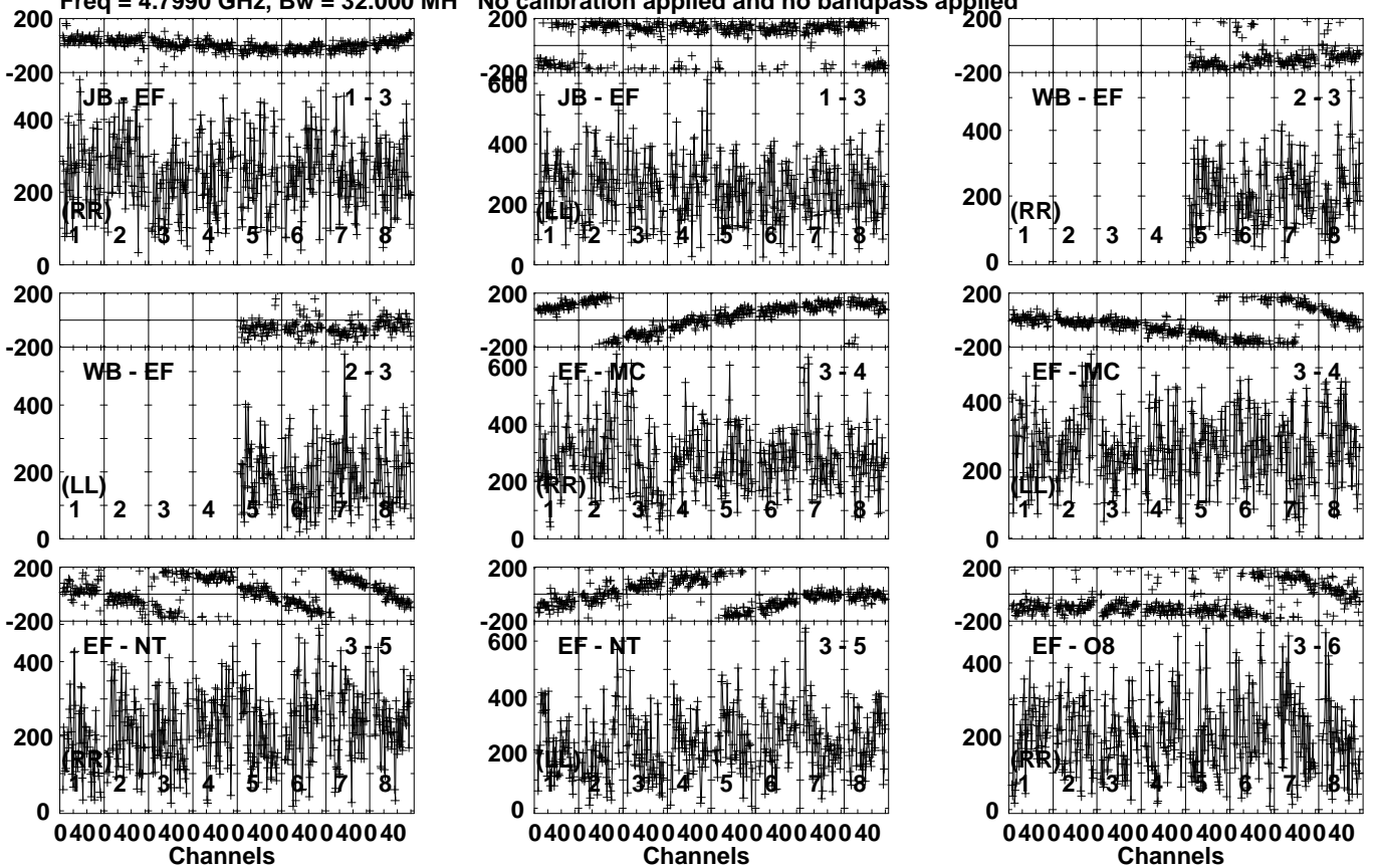
Lower frame: Micro Ampl Jy Top frame: Phas deg Vector averaged cross-power spectrum Several baselines displayed Timerange: 00:16:32:01 to 00:16:33:29
