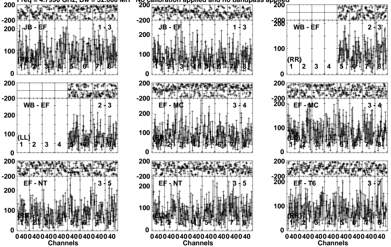
Lower frame: Micro Ampl Jy Top frame: Phas deg Vector averaged cross-power spectrum Several baselines displayed Timerange: 00/19:53:01 to 00/19:56:29
