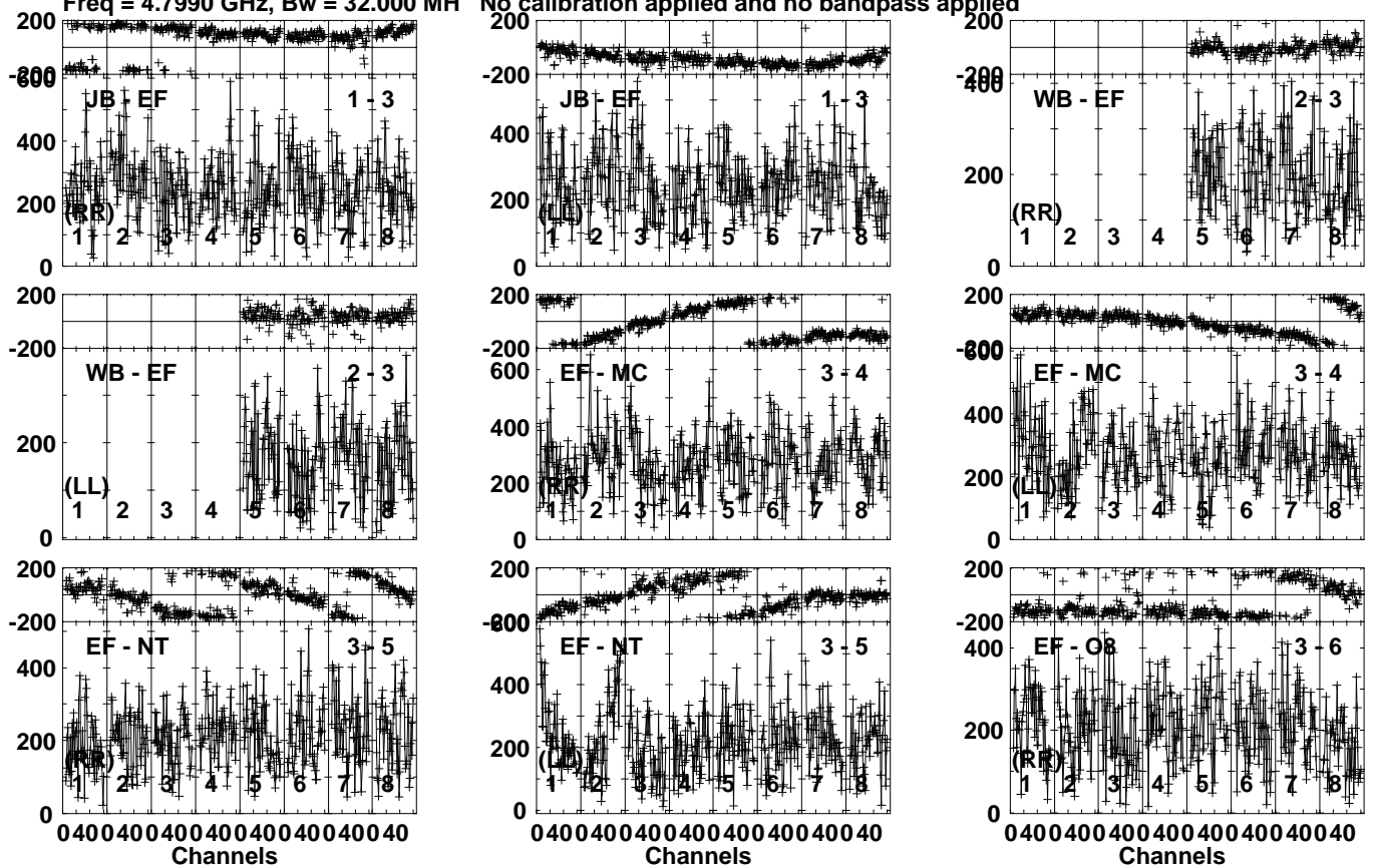
Lower frame: Micro Ampl Jy Top frame: Phas deg Vector averaged cross-power spectrum Several baselines displayed Timerange: 00/14:17:01 to 00/14:18:29
