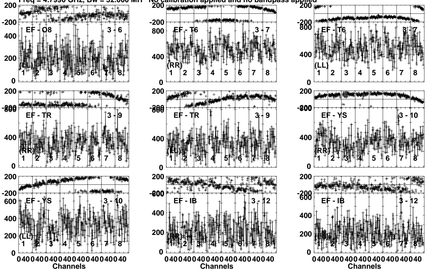
Lower frame: Micro Ampl Jy Top frame: Phas deg Vector averaged cross-power spectrum Several baselines displayed Timerange: 00/14:32:31 to 00/14:33:59
