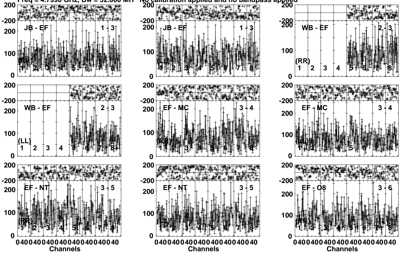
Lower frame: Micro Ampl Jy Top frame: Phas deg Vector averaged cross-power spectrum Several baselines displayed Timerange: 00/18:26:31 to 00/18:29:59
