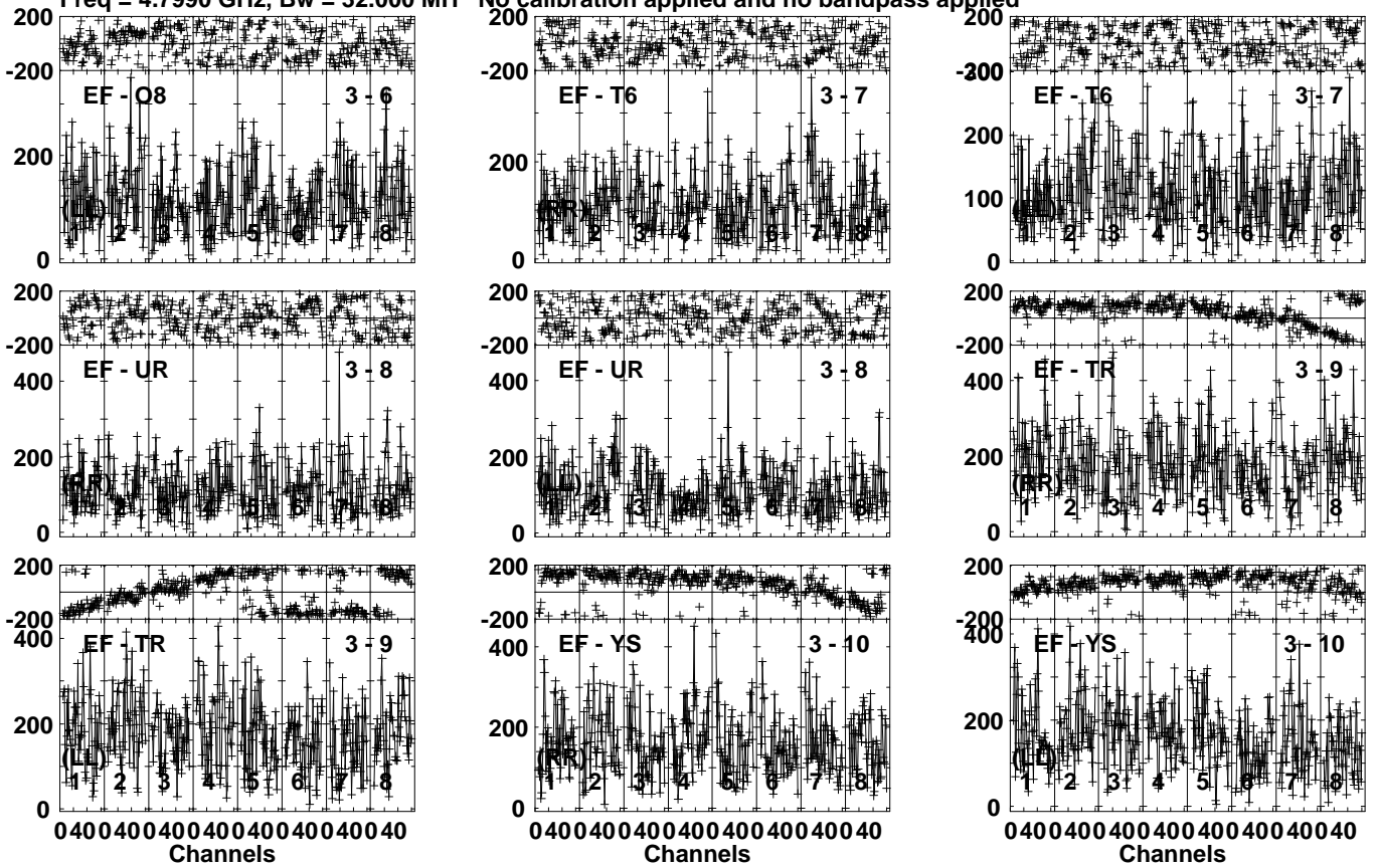
Lower frame: Micro Ampl Jy Top frame: Phas deg Vector averaged cross-power spectrum Several baselines displayed Timerange: 00/16:58:31 to 00/17:00:59
