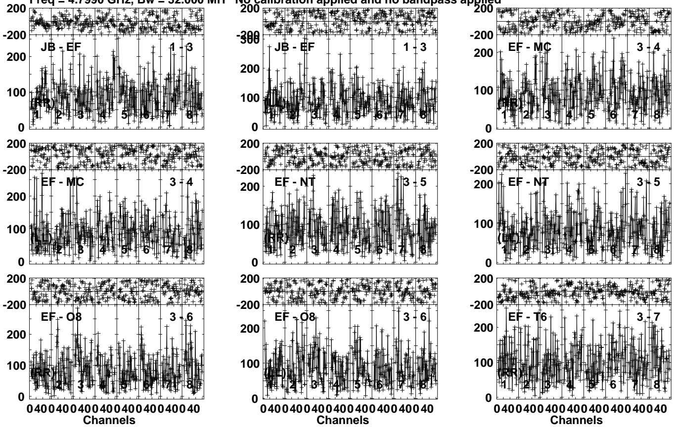
Lower frame: Micro Ampl Jy Top frame: Phas deg Vector averaged cross-power spectrum Several baselines displayed Timerange: 00/10:47:33 to 00/10:50:59
