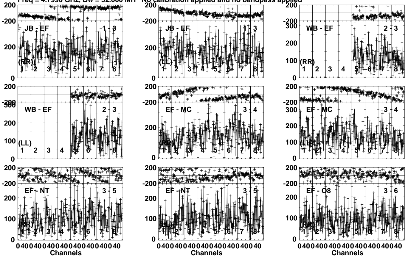
Lower frame: Micro Ampl Jy Top frame: Phas deg Vector averaged cross-power spectrum Several baselines displayed Timerange: 00/15:00:31 to 00/15:03:59
