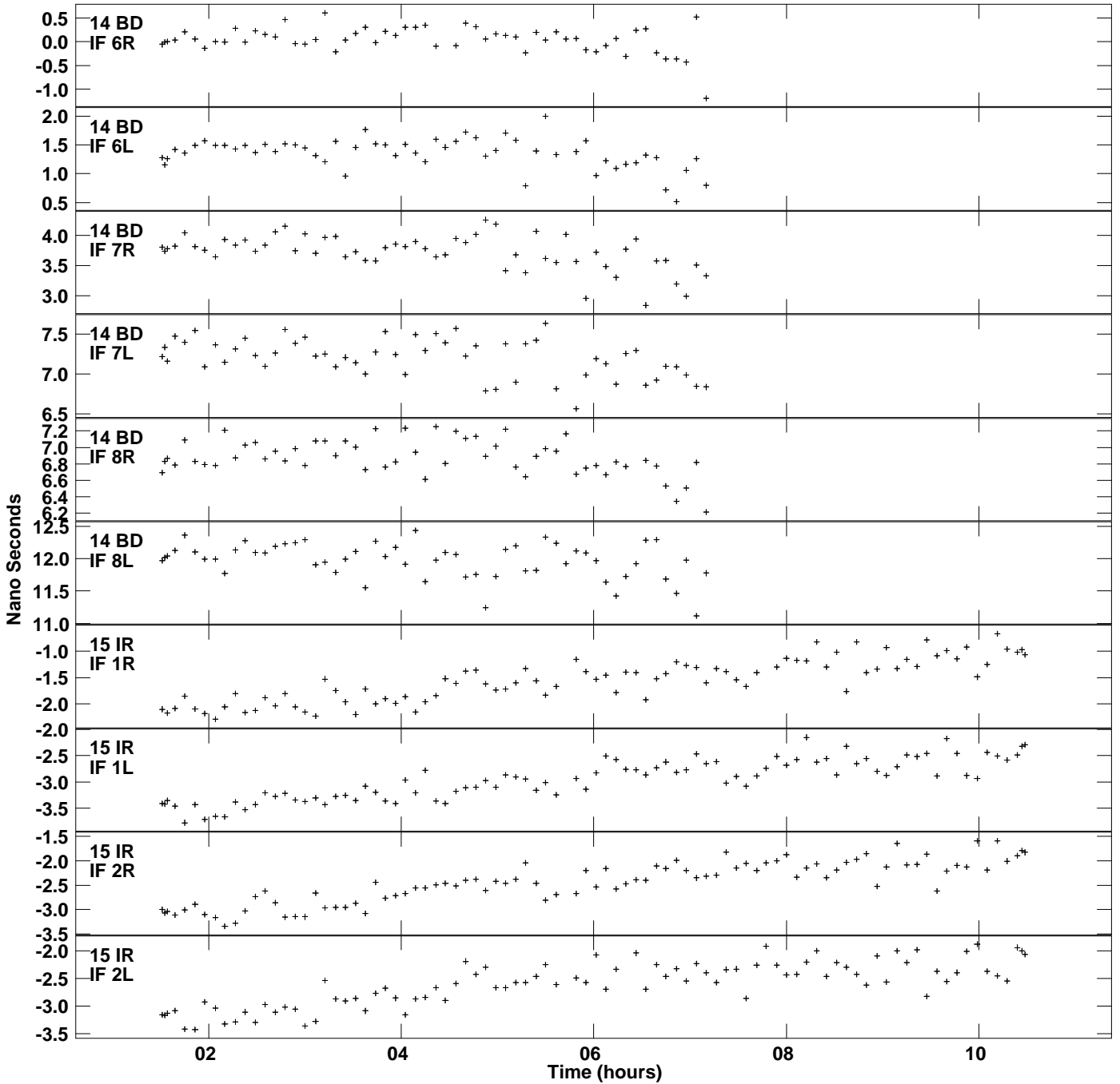
Plot file version 22 created 15-NOV-2021 12:32:48 Delay vs UTC time for EC077B.UVDATA.1 SN 3 Rpol & Lpol IF 1 - 8
