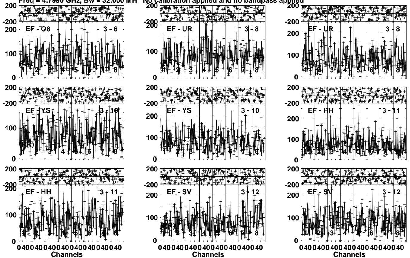
Lower frame: Micro Ampl Jy Top frame: Phas deg Vector averaged cross-power spectrum Several baselines displayed Timerange: 01/01:06:01 to 01/01:09:19
