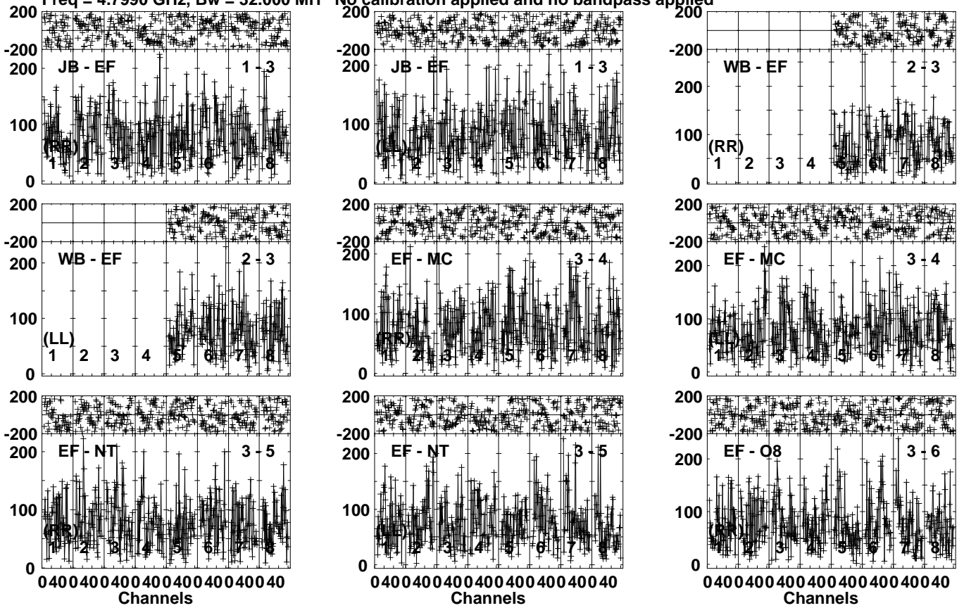
Lower frame: Micro Ampl Jy Top frame: Phas deg Vector averaged cross-power spectrum Several baselines displayed Timerange: 01/01:49:51 to 01/01:53:59
