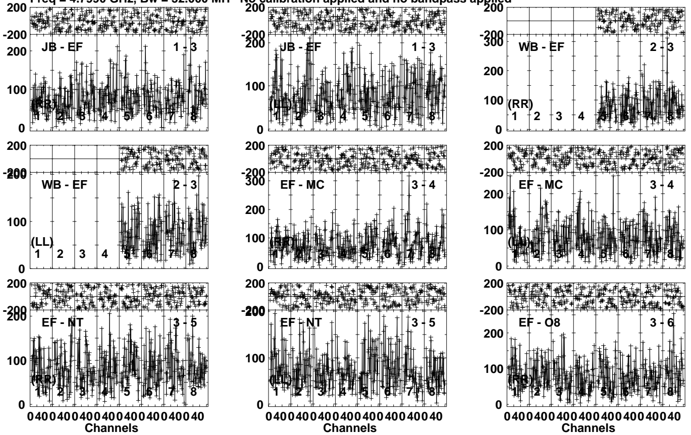
Lower frame: Micro Ampl Jy Top frame: Phas deg Vector averaged cross-power spectrum Several baselines displayed Timerange: 00/20:36:31 to 00/20:39:49
