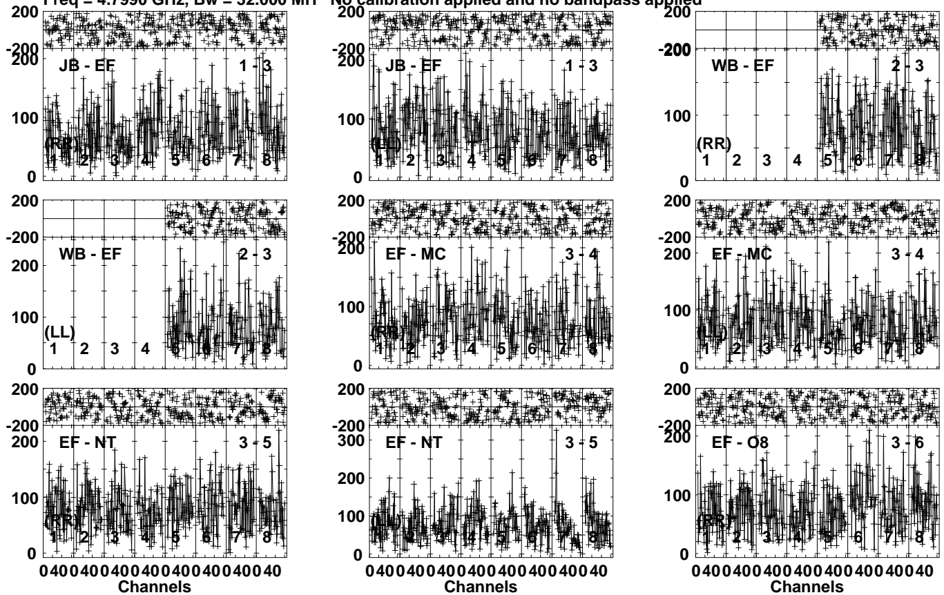
Lower frame: Micro Ampl Jy Top frame: Phas deg Vector averaged cross-power spectrum Several baselines displayed Timerange: 00/22:37:21 to 00/22:41:29
