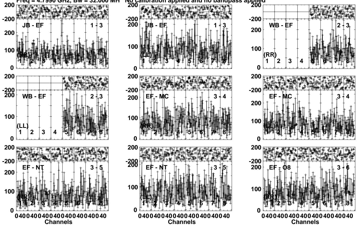
Lower frame: Micro Ampl Jy Top frame: Phas deg Vector averaged cross-power spectrum Several baselines displayed Timerange: 01/00:27:31 to 01/00:30:49
