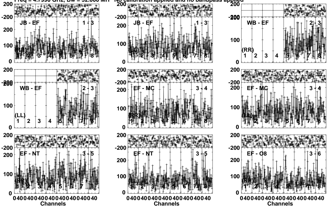
Lower frame: Micro Ampl Jy Top frame: Phas deg Vector averaged cross-power spectrum Several baselines displayed Timerange: 01/01:11:21 to 01/01:15:29
