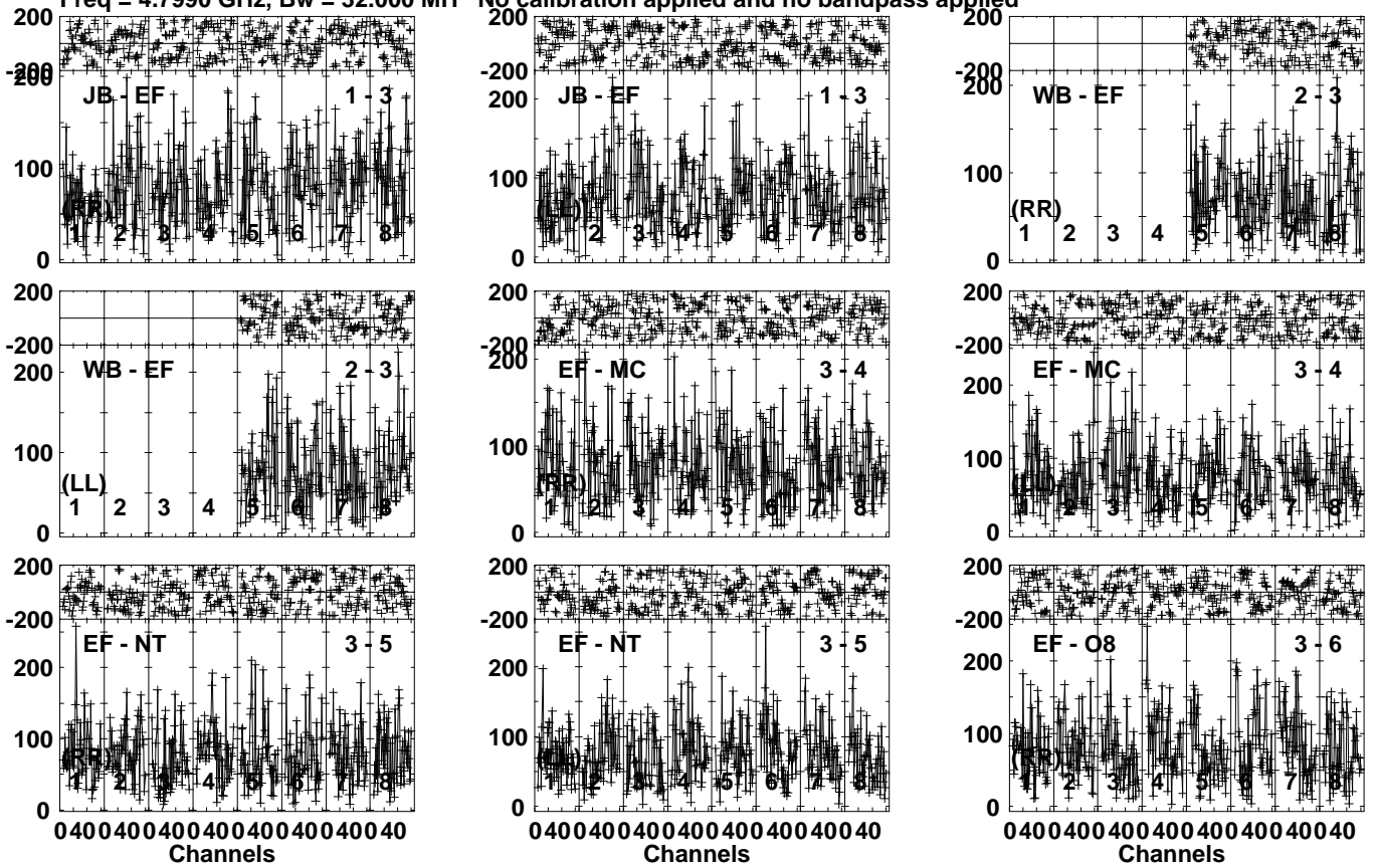
Lower frame: Micro Ampl Jy Top frame: Phas deg Vector averaged cross-power spectrum Several baselines displayed Timerange: 00/21:58:51 to 00/22:02:59
