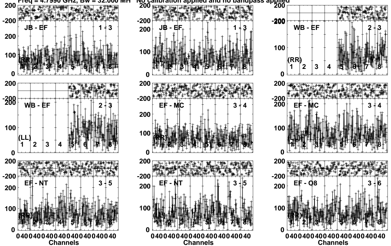
Lower frame: Micro Ampl Jy Top frame: Phas deg Vector averaged cross-power spectrum Several baselines displayed Timerange: 00/20:16:11 to 00/20:20:19
