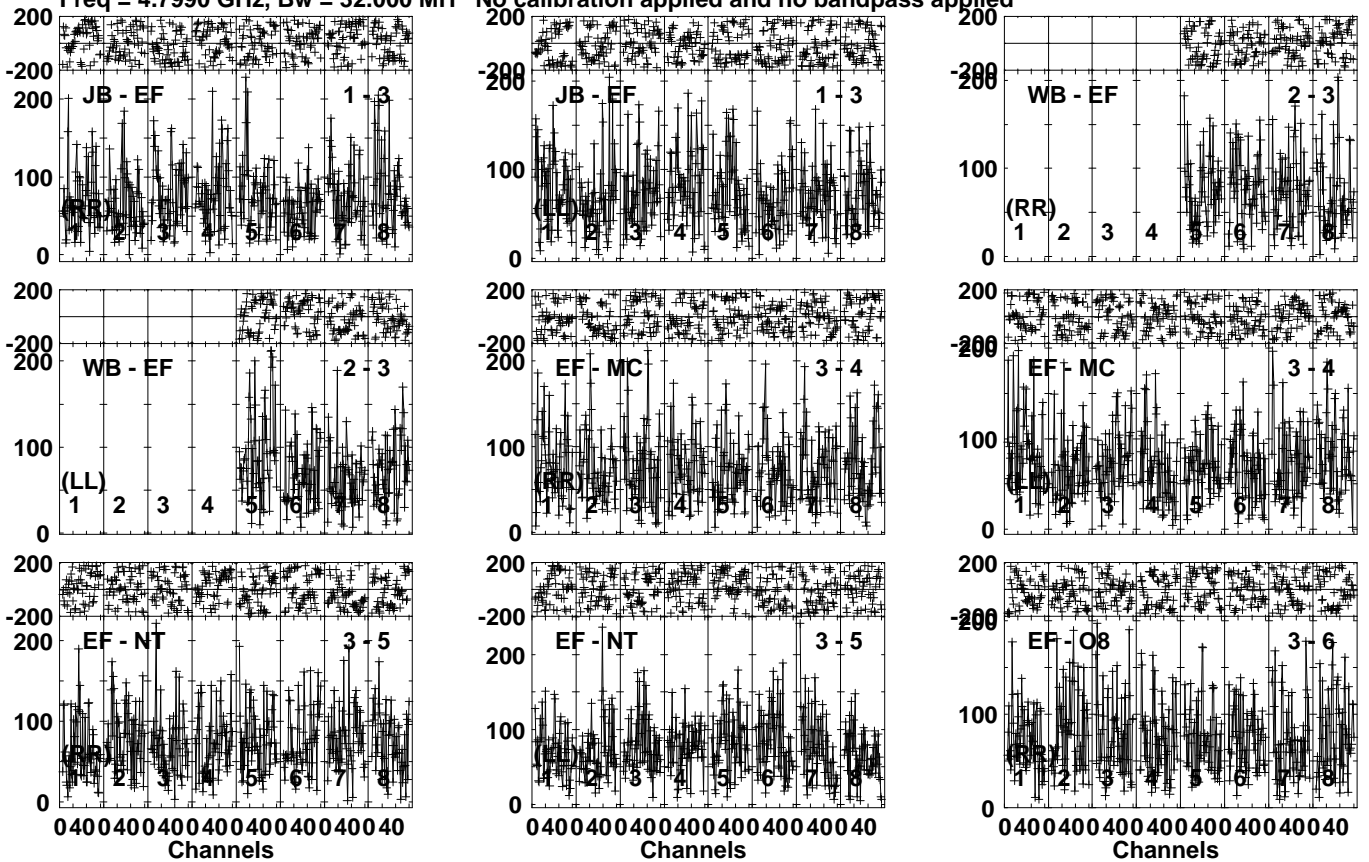
Lower frame: Micro Ampl Jy Top frame: Phas deg Vector averaged cross-power spectrum Several baselines displayed Timerange: 00/22:24:31 to 00/22:28:39
