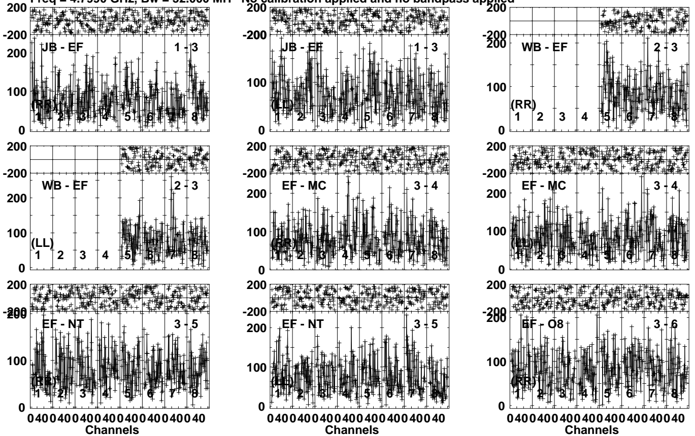
Lower frame: Micro Ampl Jy Top frame: Phas deg Vector averaged cross-power spectrum Several baselines displayed Timerange: 00/23:03:01 to 00/23:07:09
