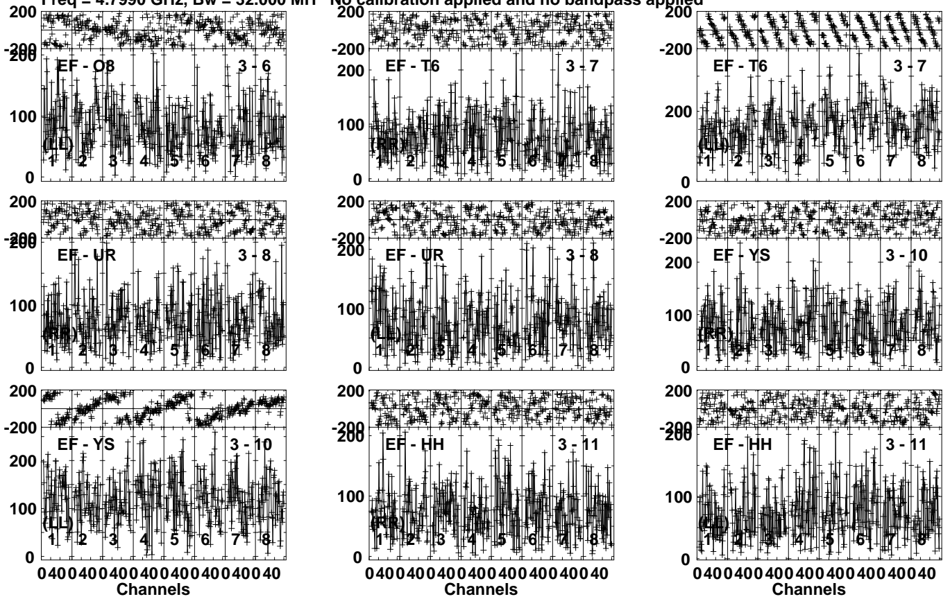
Lower frame: Micro Ampl Jy Top frame: Phas deg Vector averaged cross-power spectrum Several baselines displayed Timerange: 00/21:15:01 to 00/21:18:19
