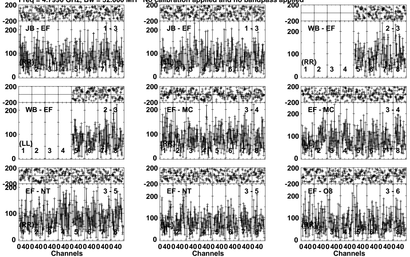
Lower frame: Micro Ampl Jy Top frame: Phas deg Vector averaged cross-power spectrum Several baselines displayed Timerange: 01/00:53:11 to 01/00:56:29
