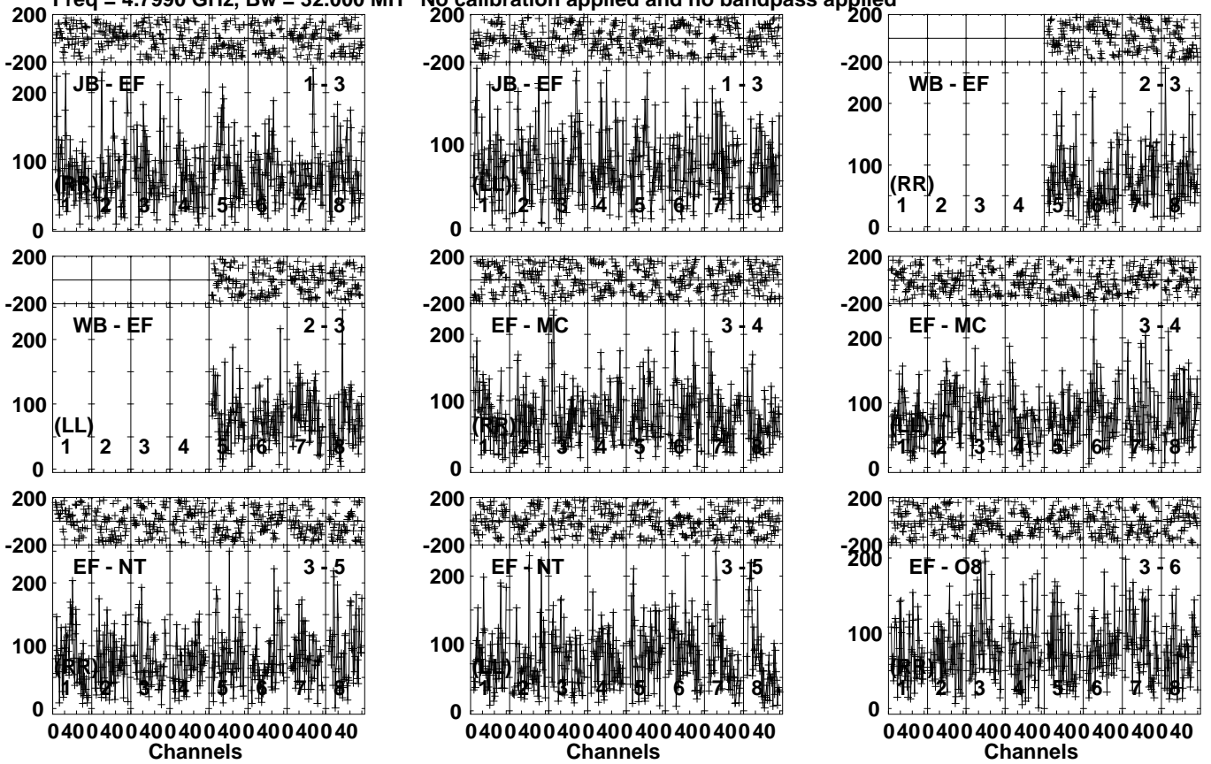
Lower frame: Micro Ampl Jy Top frame: Phas deg Vector averaged cross-power spectrum Several baselines displayed Timerange: 00/21:33:11 to 00/21:37:19
