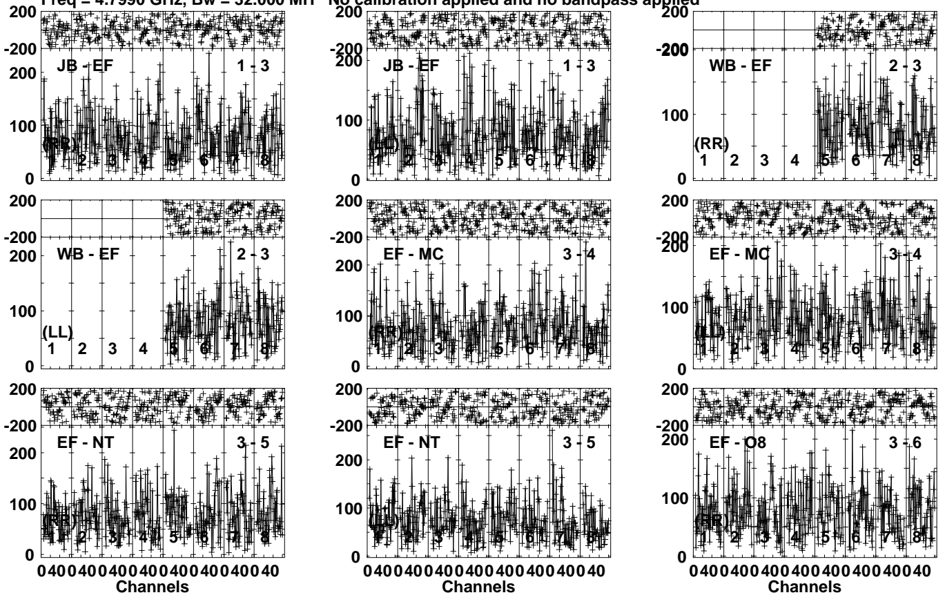
Lower frame: Micro Ampl Jy Top frame: Phas deg Vector averaged cross-power spectrum Several baselines displayed Timerange: 00/23:41:31 to 00/23:45:39
