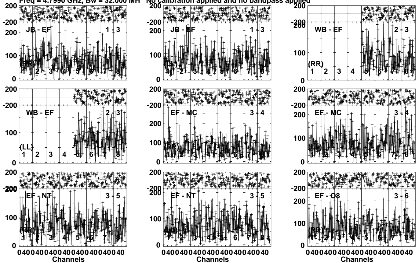
Lower frame: Micro Ampl Jy Top frame: Phas deg Vector averaged cross-power spectrum Several baselines displayed Timerange: 00/21:27:51 to 00/21:31:09
