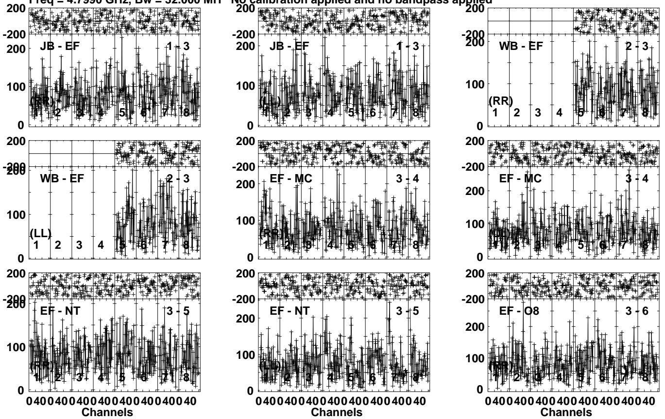
Lower frame: Micro Ampl Jy Top frame: Phas deg Vector averaged cross-power spectrum Several baselines displayed Timerange: 00/20:49:21 to 00/20:52:39
