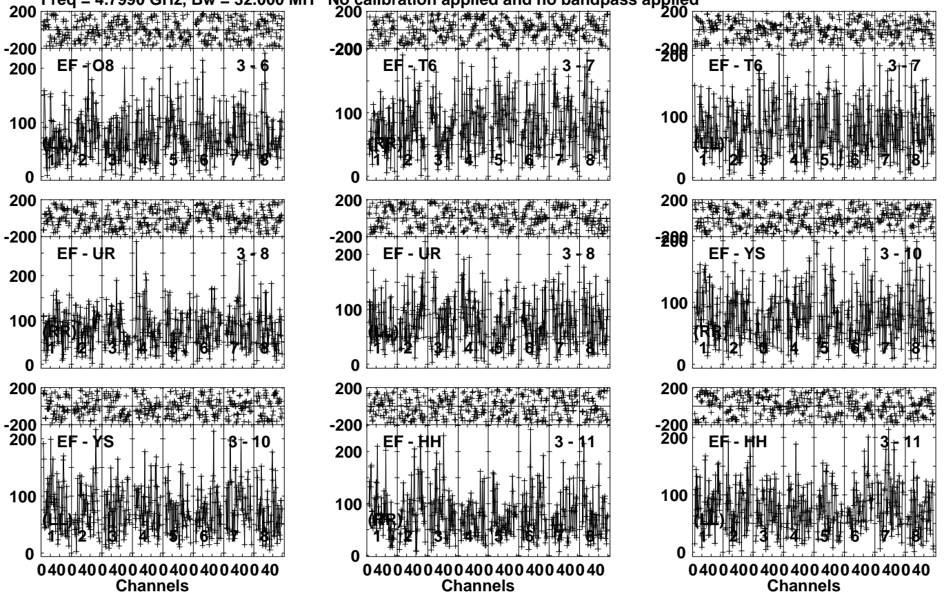
Lower frame: Micro Ampl Jy Top frame: Phas deg Vector averaged cross-power spectrum Several baselines displayed Timerange: 00/21:53:31 to 00/21:56:49
