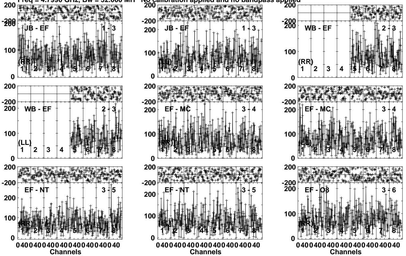
Lower frame: Micro Ampl Jy Top frame: Phas deg Vector averaged cross-power spectrum Several baselines displayed Timerange: 00/20:10:51 to 00/20:14:09
