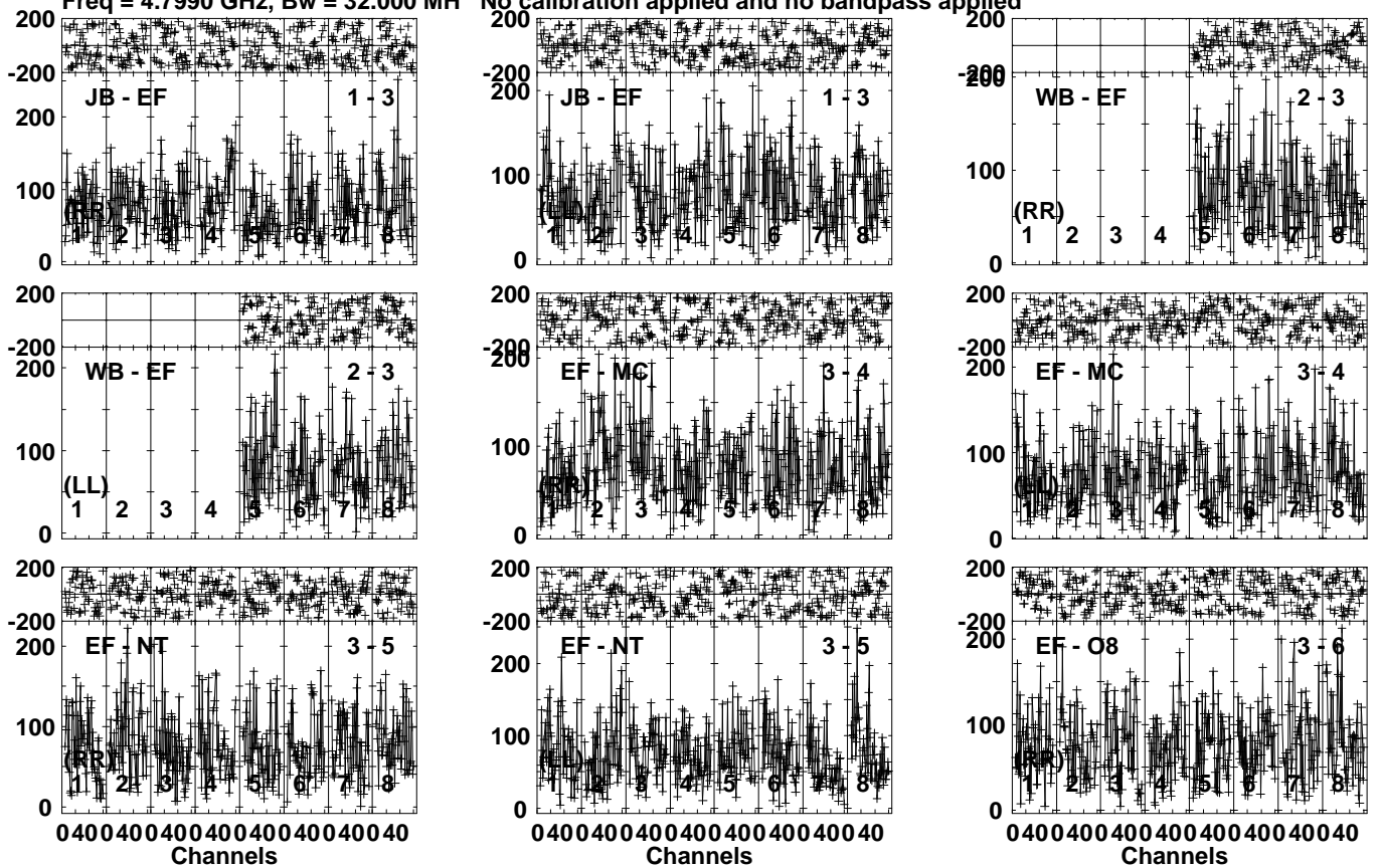
Lower frame: Micro Ampl Jy Top frame: Phas deg Vector averaged cross-power spectrum Several baselines displayed Timerange: 00/20:23:41 to 00/20:26:59
