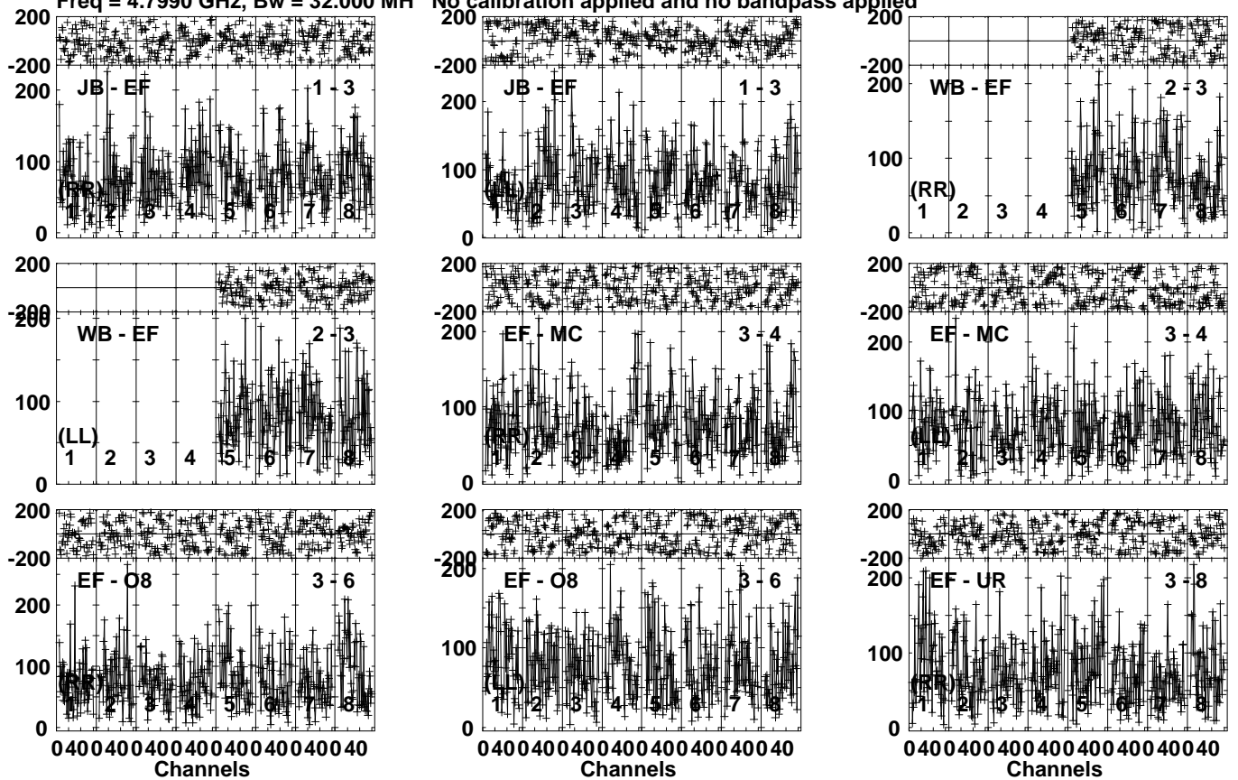
Lower frame: Micro Ampl Jy Top frame: Phas deg Vector averaged cross-power spectrum Several baselines displayed Timerange: 01/00:01:51 to 01/00:05:09
