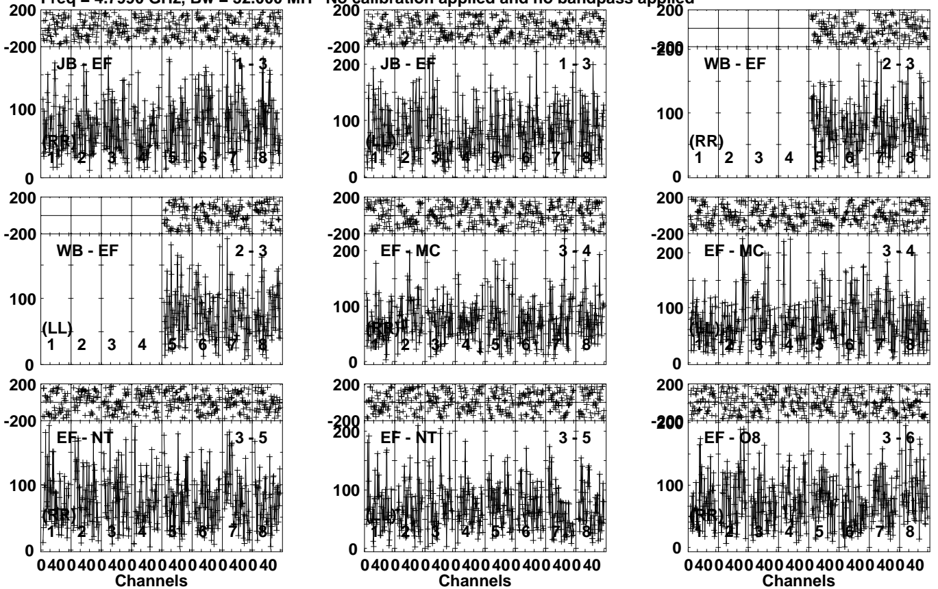
Lower frame: Micro Ampl Jy Top frame: Phas deg Vector averaged cross-power spectrum Several baselines displayed Timerange: 00/22:11:41 to 00/22:15:49
