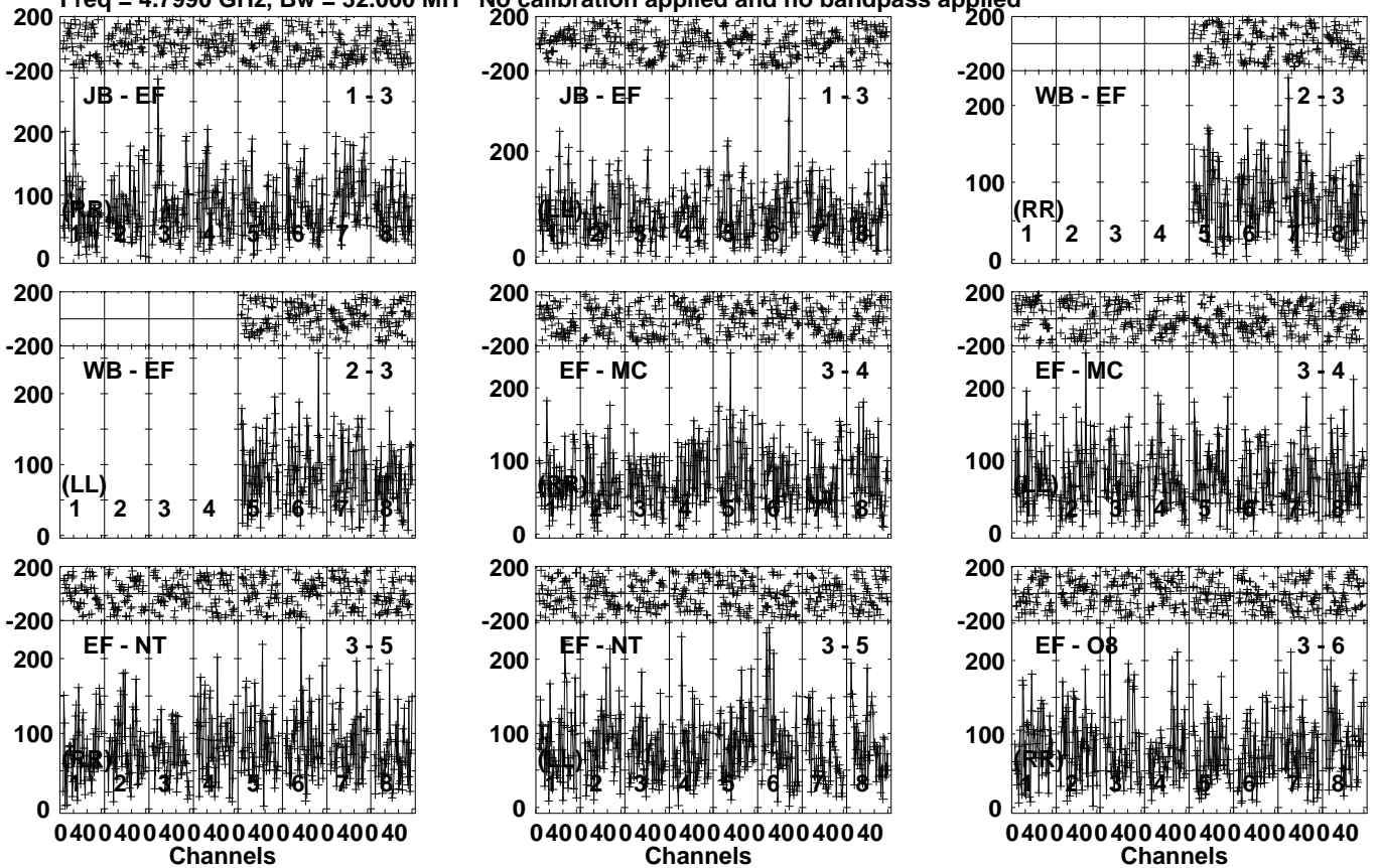
Lower frame: Micro Ampl Jy Top frame: Phas deg Vector averaged cross-power spectrum Several baselines displayed Timerange: 00/22:57:41 to 00/23:00:59
