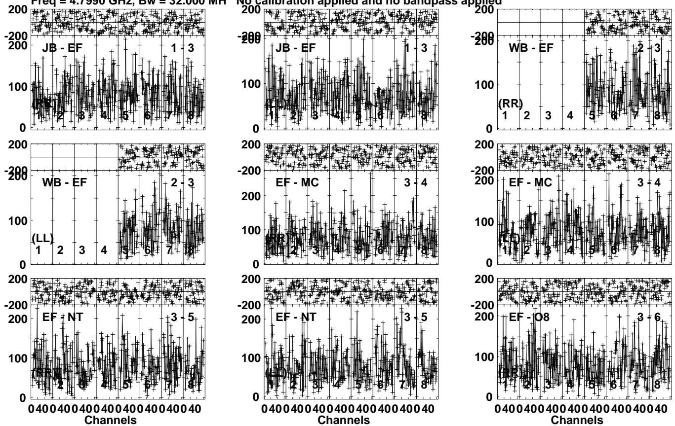
Lower frame: Micro Ampl Jy Top frame: Phas deg Vector averaged cross-power spectrum Several baselines displayed Timerange: 01/01:31:41 to 01/01:34:59
