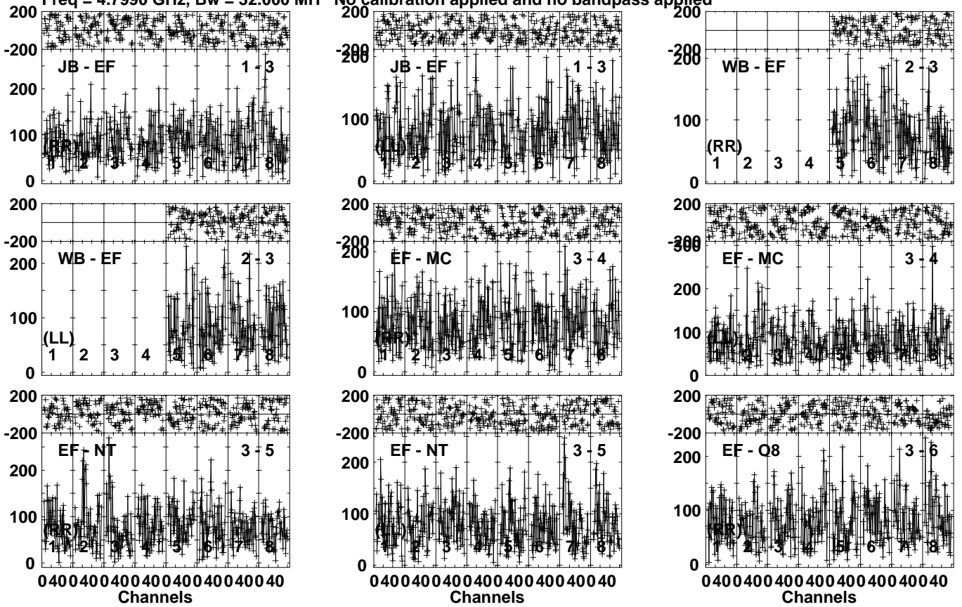
Lower frame: Micro Ampl Jy Top frame: Phas deg Vector averaged cross-power spectrum Several baselines displayed Timerange: 01/00:14:41 to 01/00:17:59
