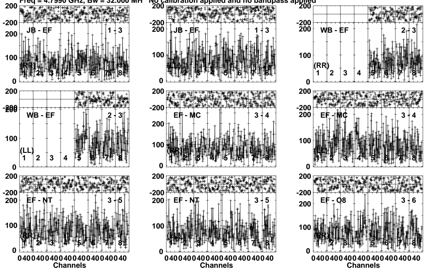
Lower frame: Micro Ampl Jy Top frame: Phas deg Vector averaged cross-power spectrum Several baselines displayed Timerange: 00/23:10:31 to 00/23:13:49
