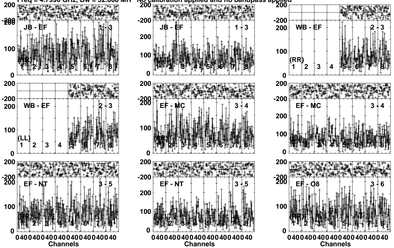
Lower frame: Micro Ampl Jy Top frame: Phas deg Vector averaged cross-power spectrum Several baselines displayed Timerange: 00/21:20:21 to 00/21:24:29
