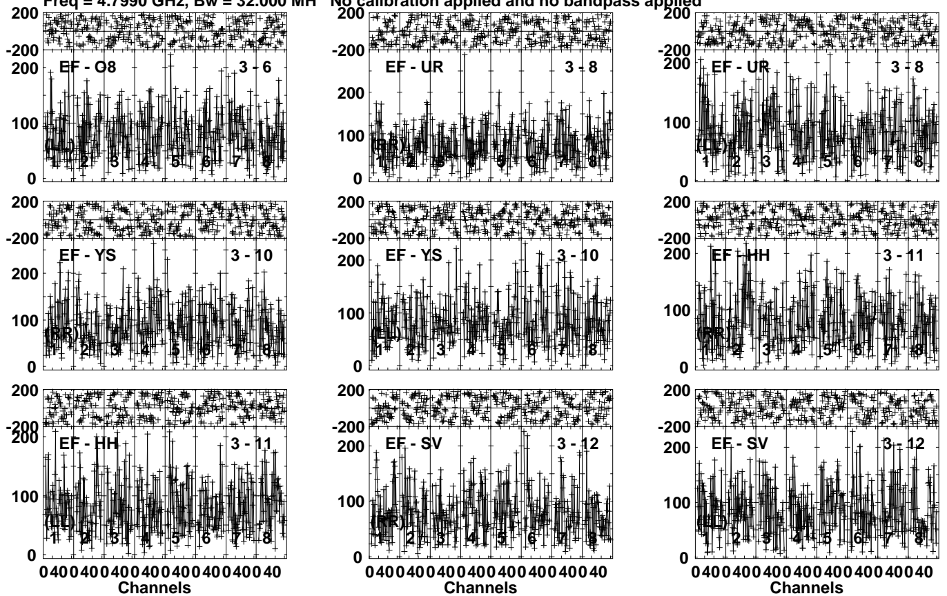
Lower frame: Micro Ampl Jy Top frame: Phas deg Vector averaged cross-power spectrum Several baselines displayed Timerange: 01/00:40:21 to 01/00:43:39
