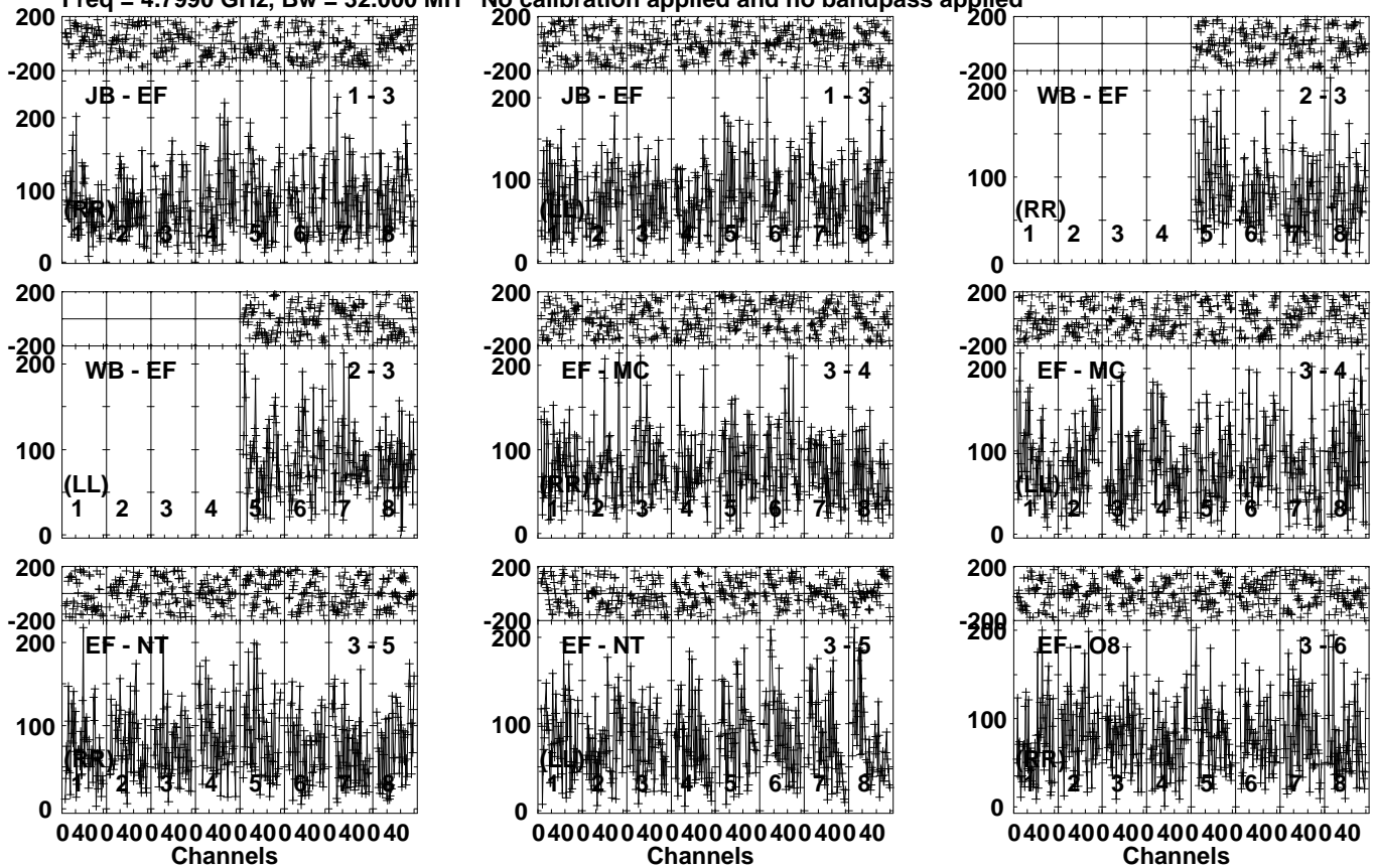
Lower frame: Micro Ampl Jy Top frame: Phas deg Vector averaged cross-power spectrum Several baselines displayed Timerange: 00/20:54:41 to 00/20:58:49
