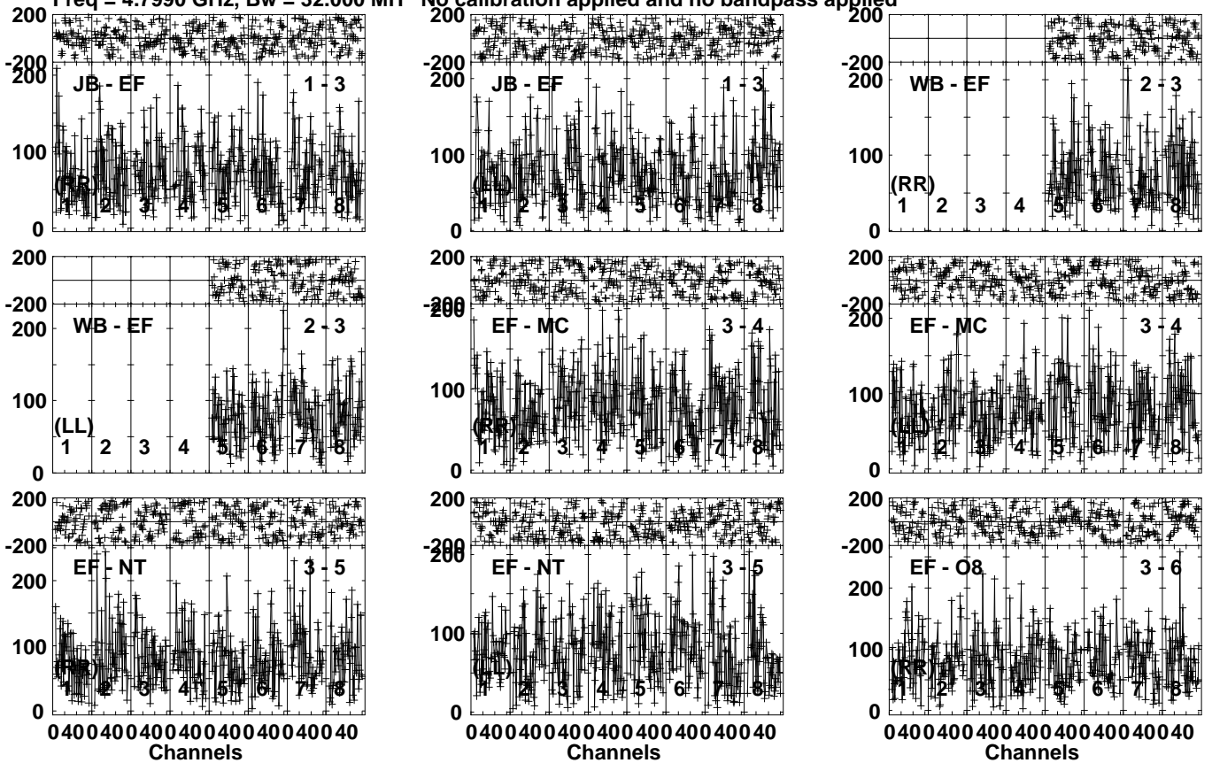
Lower frame: Micro Ampl Jy Top frame: Phas deg Vector averaged cross-power spectrum Several baselines displayed Timerange: 00/20:41:51 to 00/20:45:59
