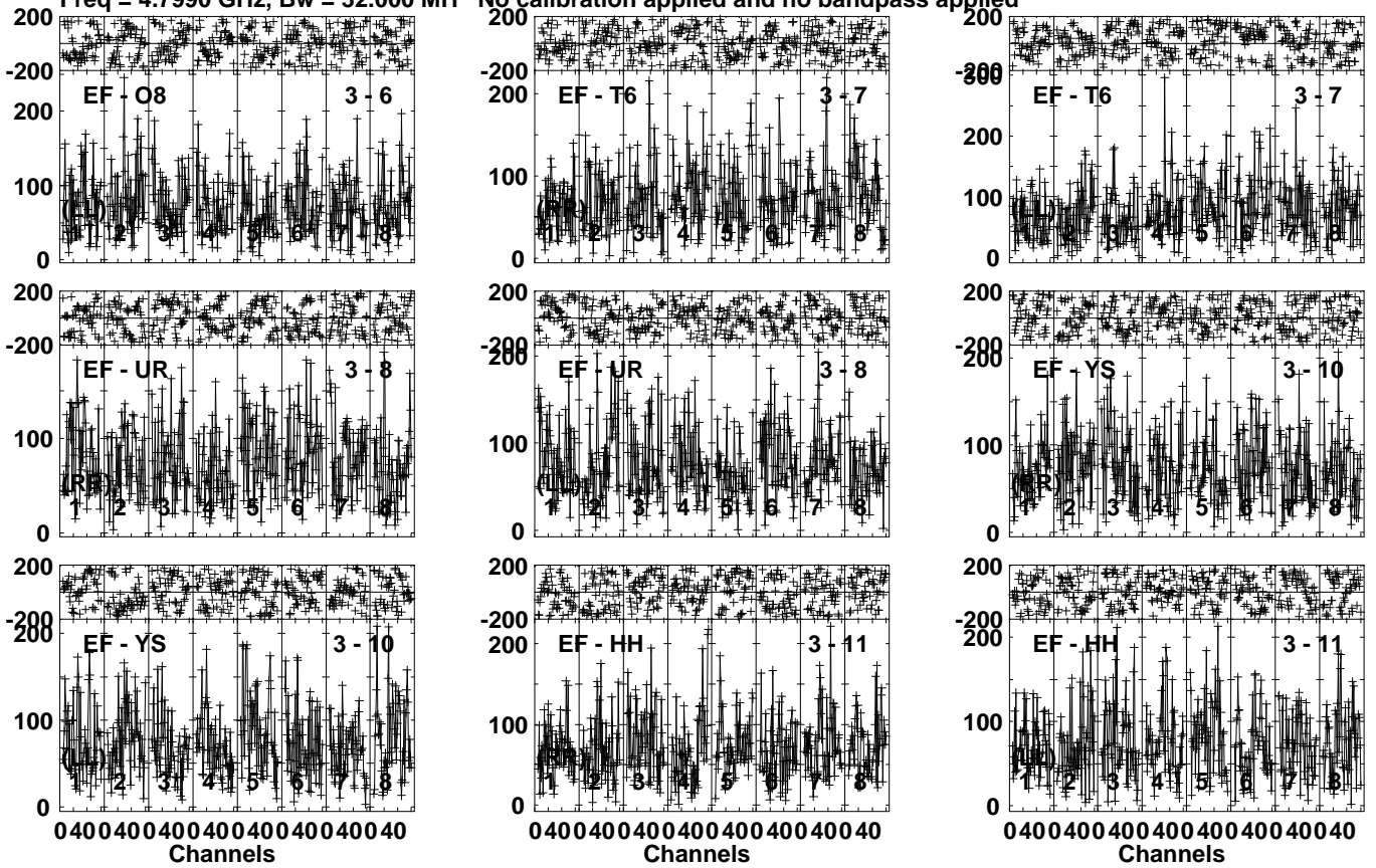
Lower frame: Micro Ampl Jy Top frame: Phas deg Vector averaged cross-power spectrum Several baselines displayed Timerange: 00/22:19:11 to 00/22:22:29
