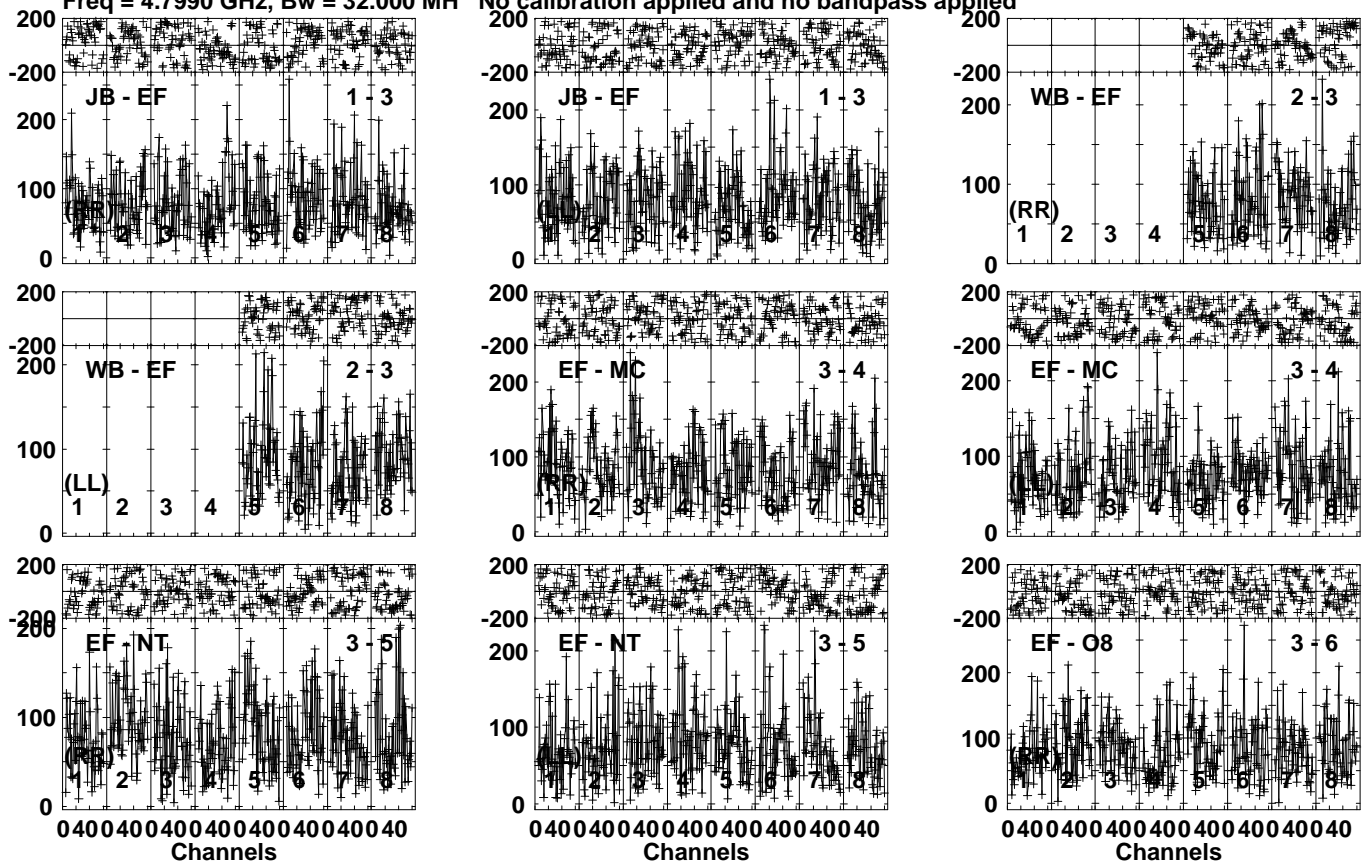
Lower frame: Micro Ampl Jy Top frame: Phas deg Vector averaged cross-power spectrum Several baselines displayed Timerange: 01/00:32:51 to 01/00:36:59
