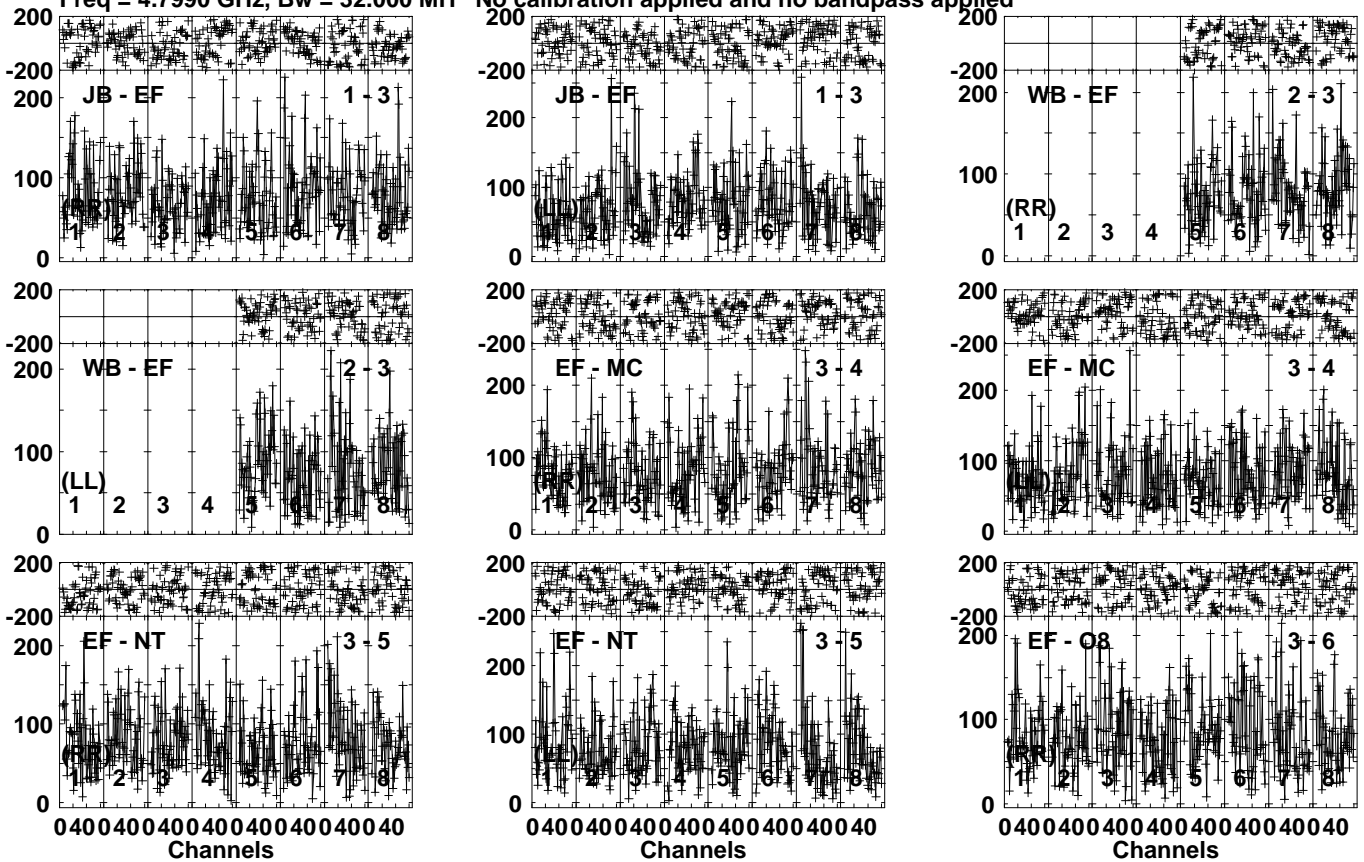
Lower frame: Micro Ampl Jy Top frame: Phas deg Vector averaged cross-power spectrum Several baselines displayed Timerange: 01/00:58:31 to 01/01:02:39
