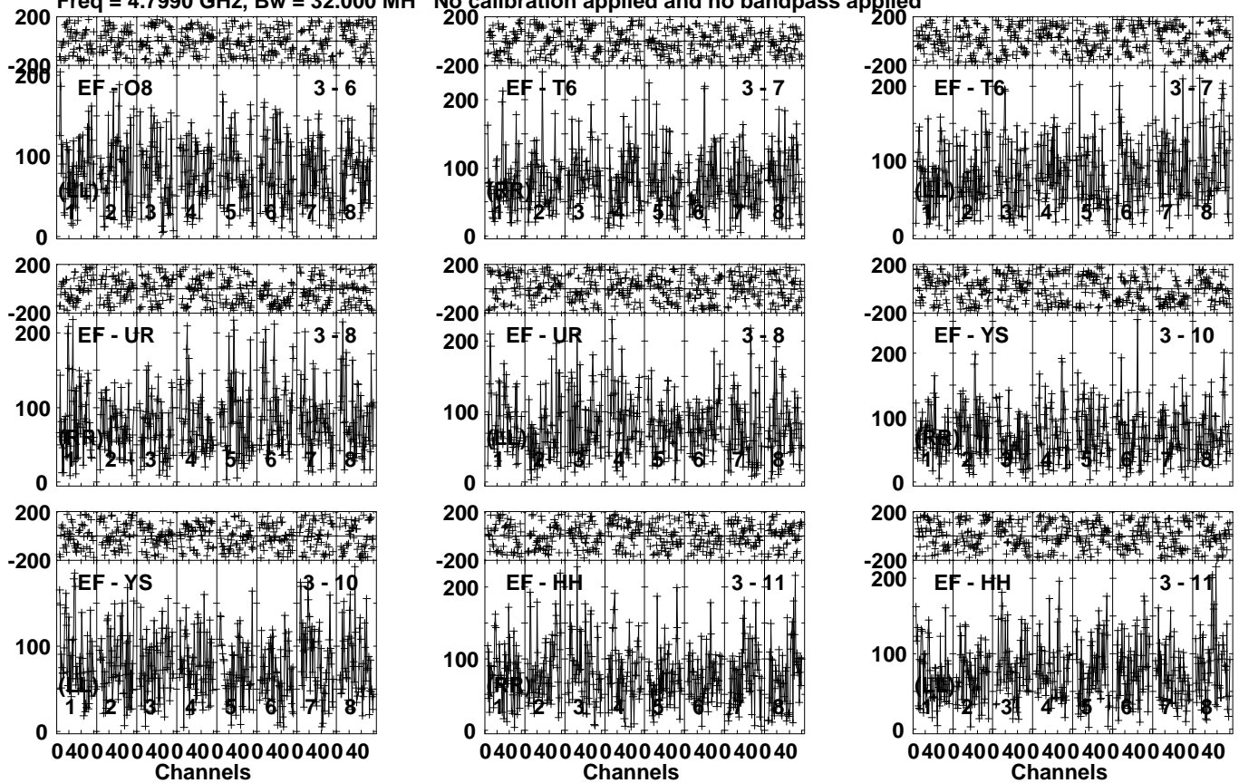
Lower frame: Micro Ampl Jy Top frame: Phas deg Vector averaged cross-power spectrum Several baselines displayed Timerange: 00/20:29:01 to 00/20:33:09
