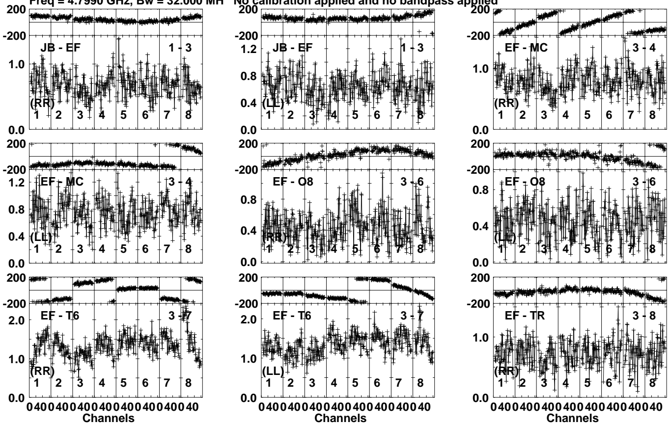
Lower frame: Milli Ampl Jy Top frame: Phas deg Vector averaged cross-power spectrum Several baselines displayed Timerange: 00/12:30:31 to 00/12:31:09
