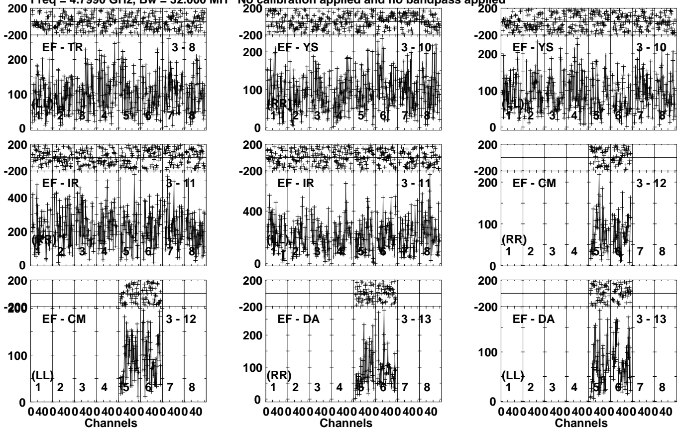
Lower frame: Micro Ampl Jy Top frame: Phas deg Vector averaged cross-power spectrum Several baselines displayed Timerange: 00/11:20:21 to 00/11:22:59
