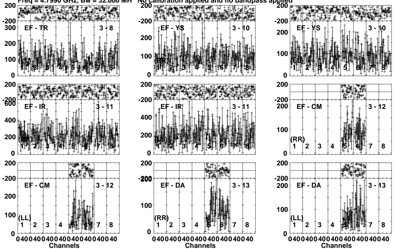
Lower frame: Micro Ampl Jy Top frame: Phas deg Vector averaged cross-power spectrum Several baselines displayed Timerange: 00/11:39:01 to 00/11:41:39
