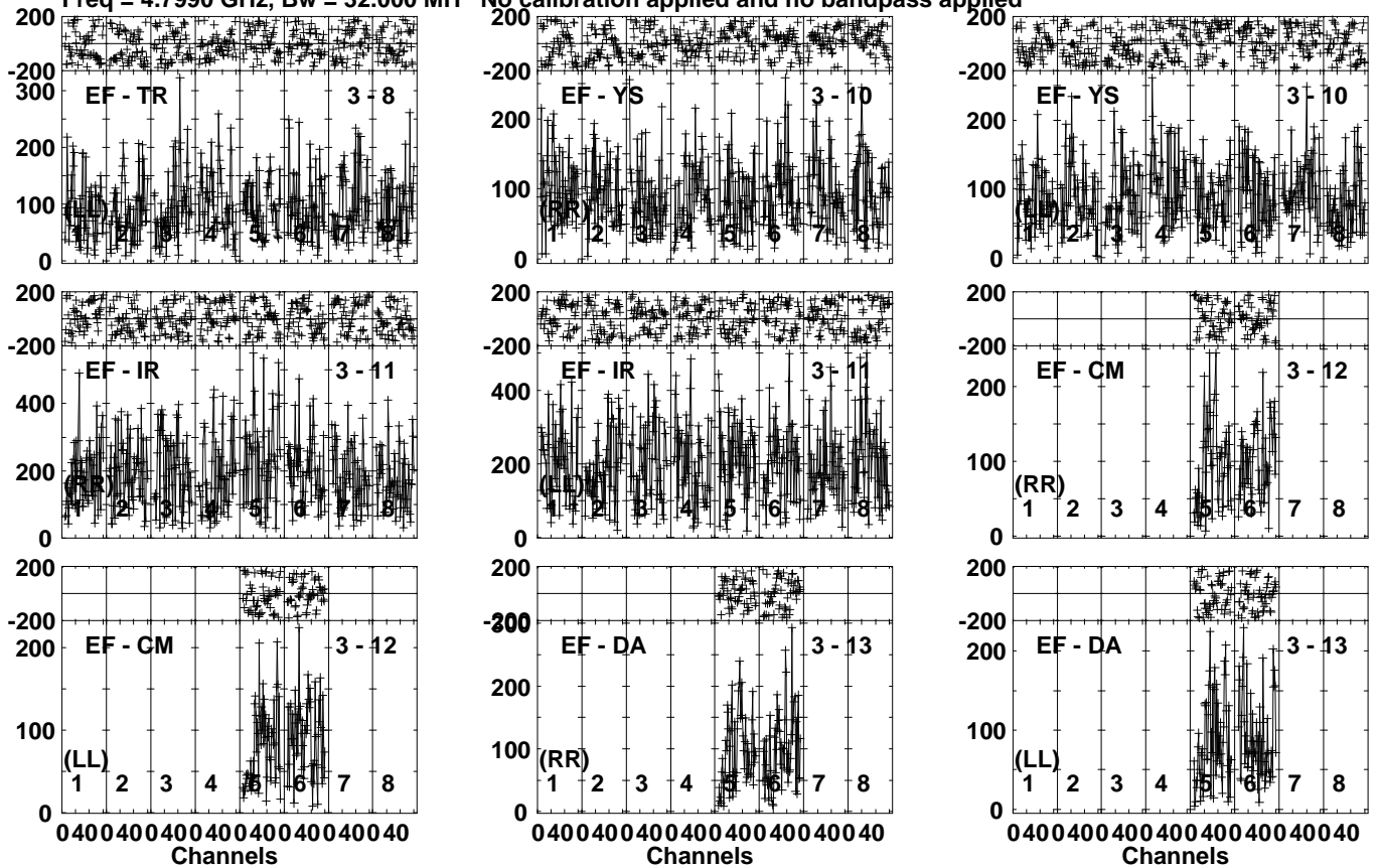
Lower frame: Micro Ampl Jy Top frame: Phas deg Vector averaged cross-power spectrum Several baselines displayed Timerange: 00/12:38:41 to 00/12:41:19
