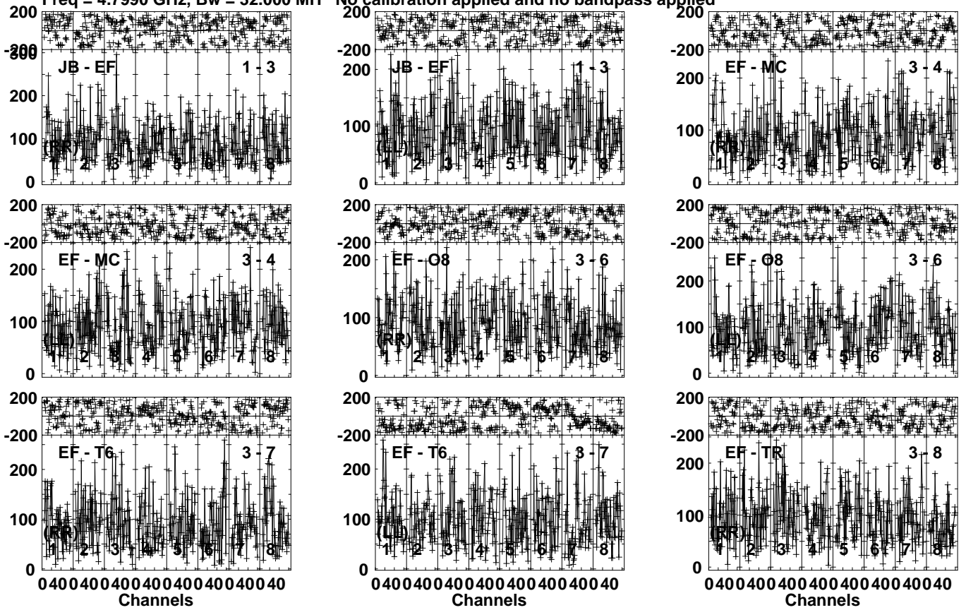
Lower frame: Micro Ampl Jy Top frame: Phas deg Vector averaged cross-power spectrum Several baselines displayed Timerange: 00/11:50:11 to 00/11:52:49
