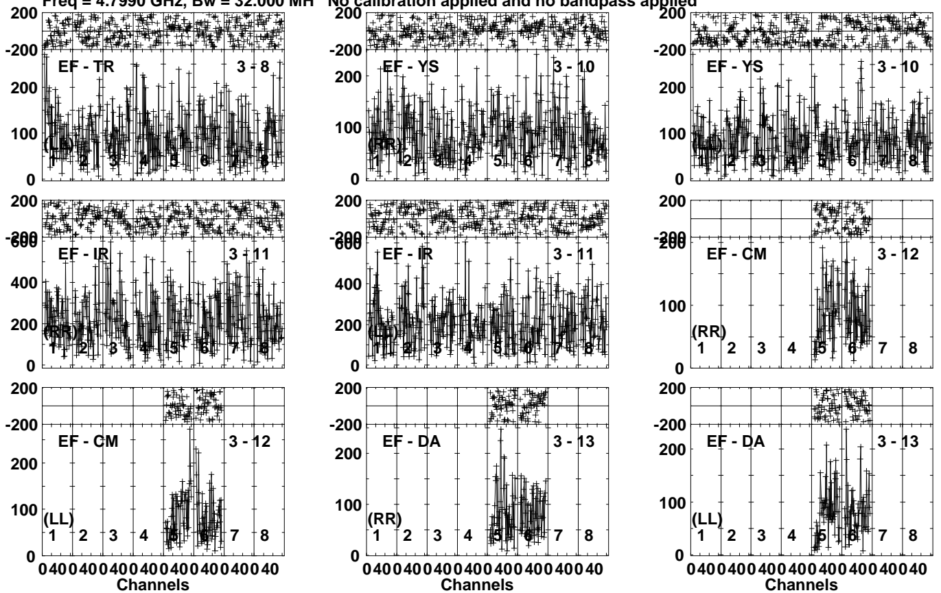
Lower frame: Micro Ampl Jy Top frame: Phas deg Vector averaged cross-power spectrum Several baselines displayed Timerange: 00/12:42:31 to 00/12:45:09
