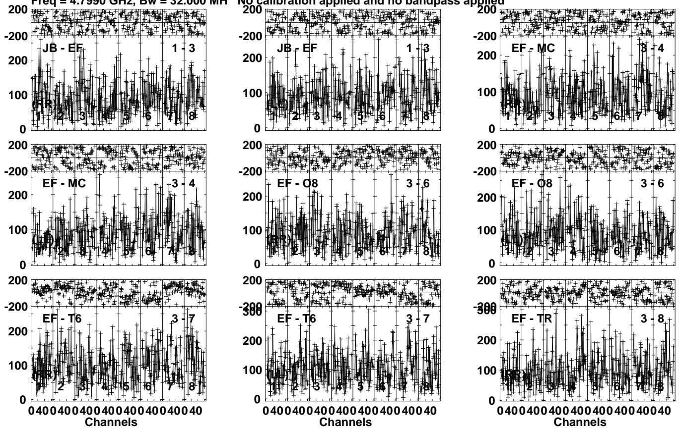
Lower frame: Micro Ampl Jy Top frame: Phas deg Vector averaged cross-power spectrum Several baselines displayed Timerange: 00/12:12:41 to 00/12:15:19
