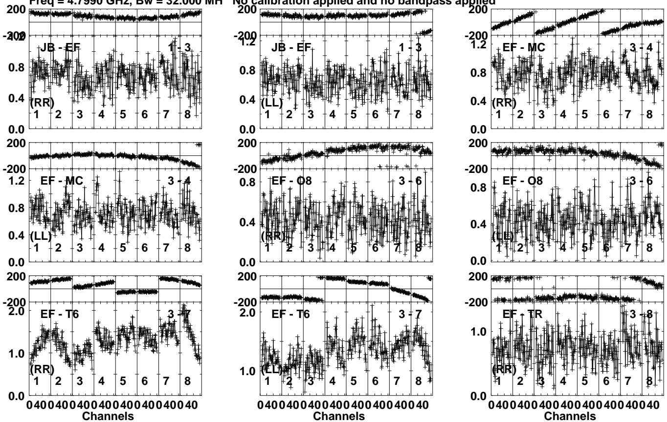
Lower frame: Milli Ampl Jy Top frame: Phas deg Vector averaged cross-power spectrum Several baselines displayed Timerange: 00/12:04:21 to 00/12:04:59
