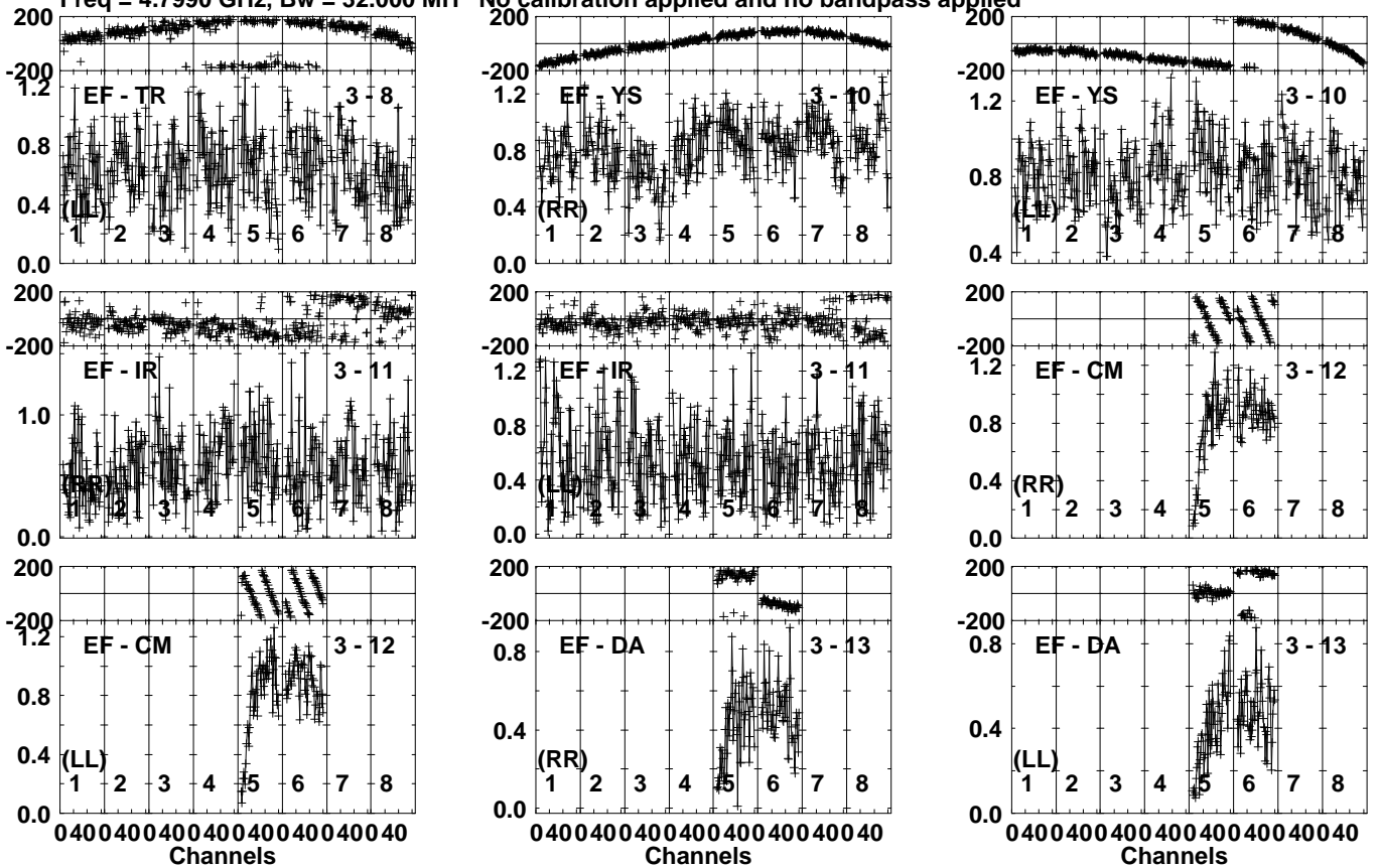
Lower frame: Milli Ampl Jy Top frame: Phas deg Vector averaged cross-power spectrum Several baselines displayed Timerange: 00/11:53:11 to 00/11:53:49
