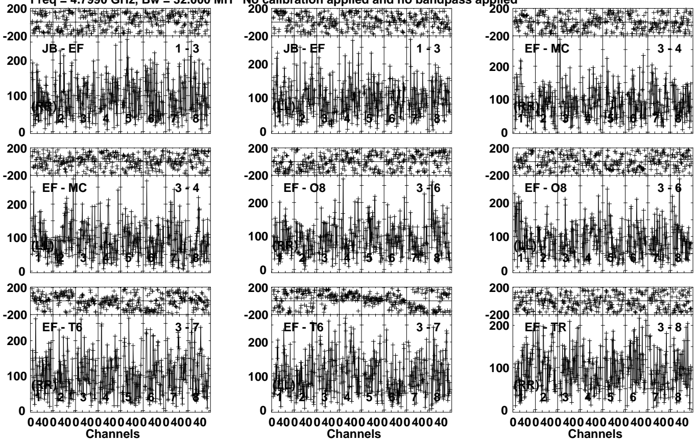
Lower frame: Micro Ampl Jy Top frame: Phas deg Vector averaged cross-power spectrum Several baselines displayed Timerange: 00/12:35:01 to 00/12:37:39
