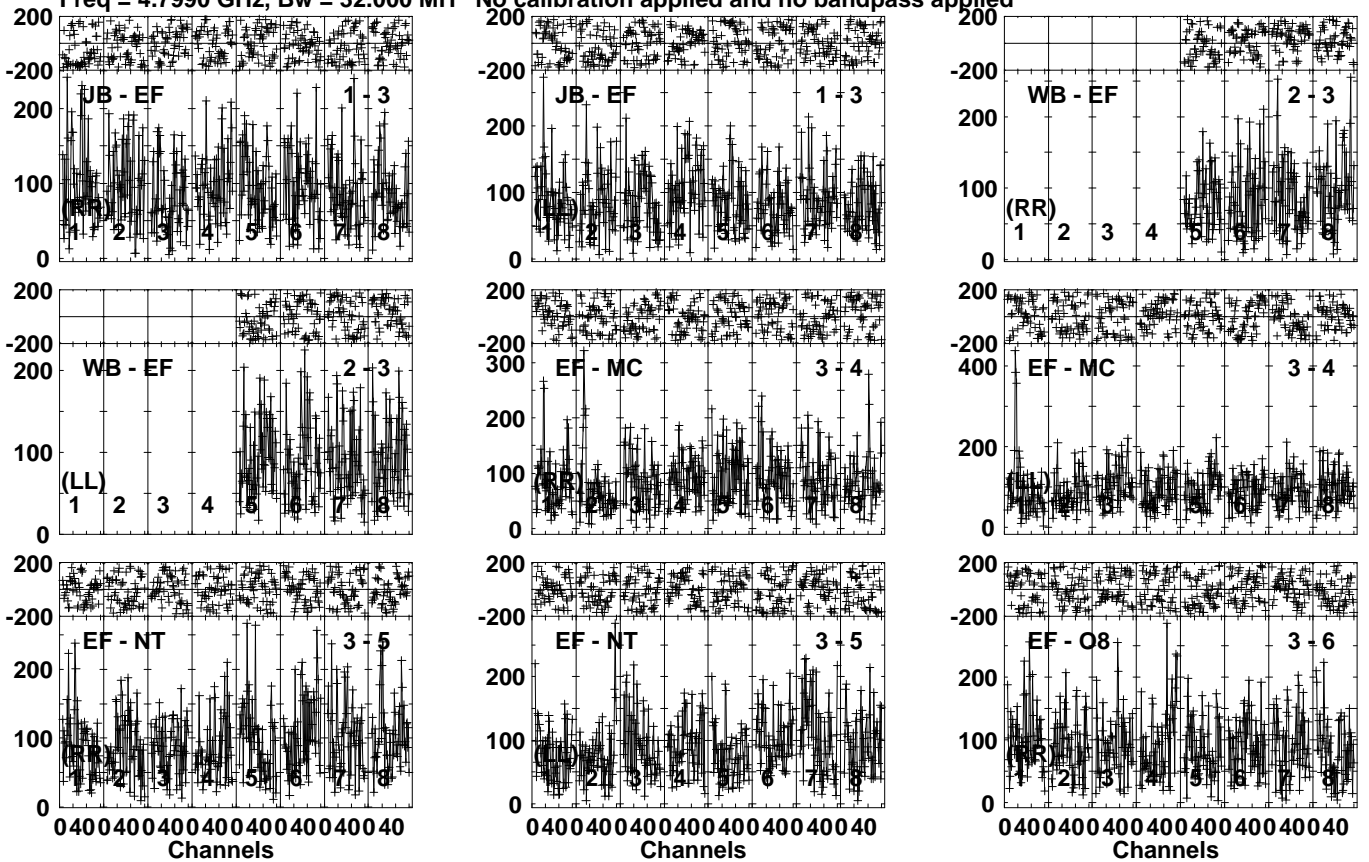
Lower frame: Micro Ampl Jy Top frame: Phas deg Vector averaged cross-power spectrum Several baselines displayed Timerange: 00/22:36:01 to 00/22:38:59
