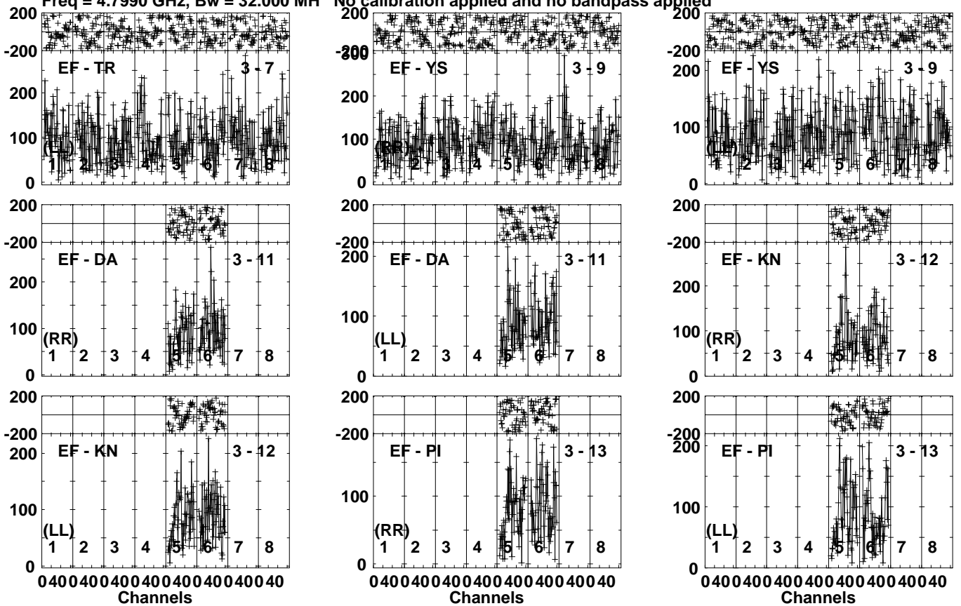
Lower frame: Micro Ampl Jy Top frame: Phas deg Vector averaged cross-power spectrum Several baselines displayed Timerange: 01/05:11:41 to 01/05:14:39
