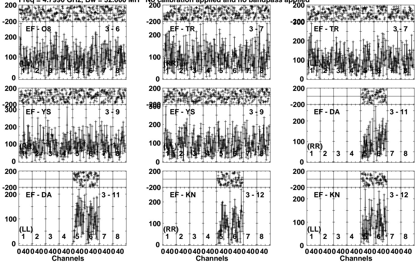
Lower frame: Micro Ampl Jy Top frame: Phas deg Vector averaged cross-power spectrum Several baselines displayed Timerange: 00/22:52:41 to 00/22:55:39
