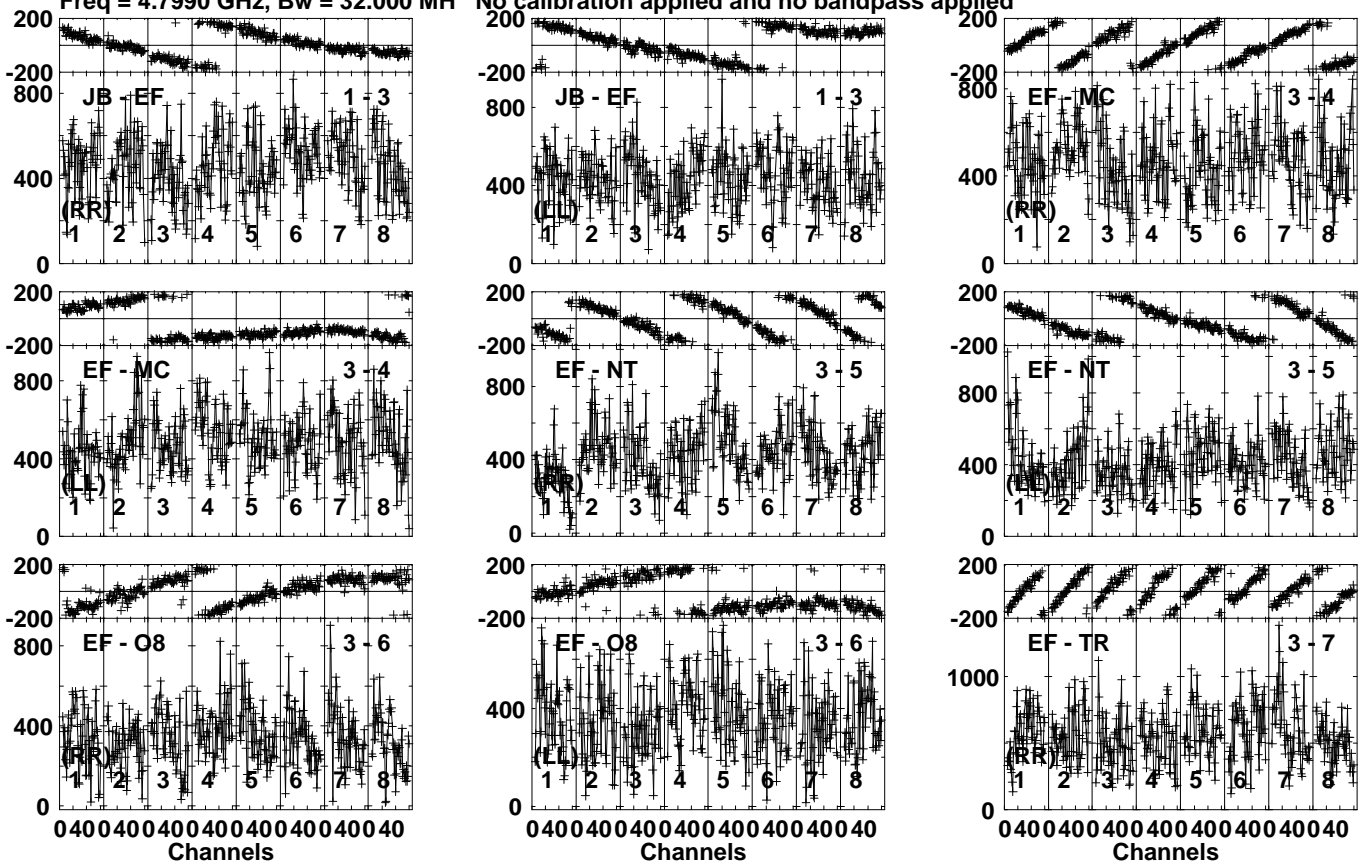
Lower frame: Micro Ampl Jy Top frame: Phas deg Vector averaged cross-power spectrum Several baselines displayed Timerange: 01/05:19:11 to 01/05:19:49
