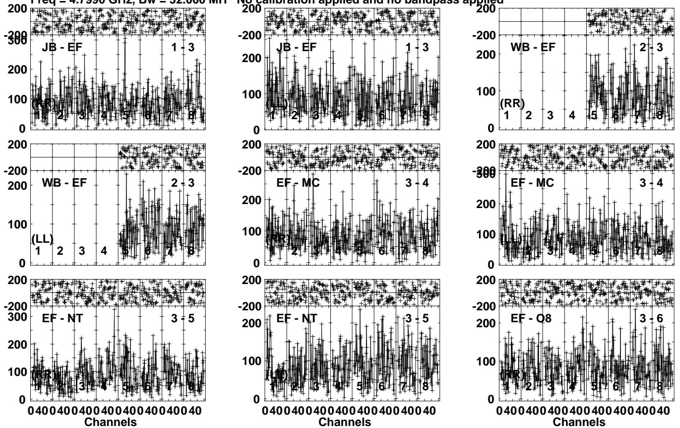
Lower frame: Micro Ampl Jy Top frame: Phas deg Vector averaged cross-power spectrum Several baselines displayed Timerange: 01/00:38:11 to 01/00:41:09
