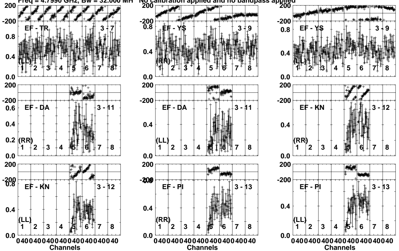
Lower frame: Milli Ampl Jy Top frame: Phas deg Vector averaged cross-power spectrum Several baselines displayed Timerange: 01/05:07:01 to 01/05:07:39
