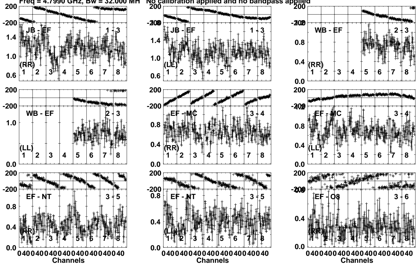
Lower frame: Milli Ampl Jy Top frame: Phas deg Vector averaged cross-power spectrum Several baselines displayed Timerange: 01/03:48:01 to 01/03:49:19
