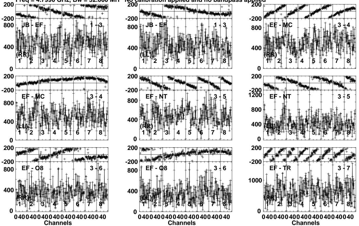
Lower frame: Micro Ampl Jy Top frame: Phas deg Vector averaged cross-power spectrum Several baselines displayed Timerange: 01/04:58:31 to 01/04:59:29
