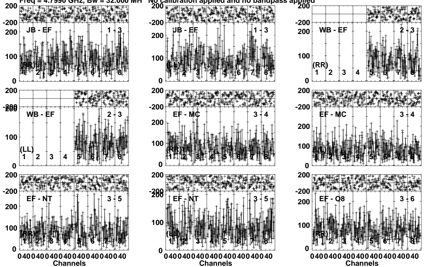
Lower frame: Micro Ampl Jy Top frame: Phas deg Vector averaged cross-power spectrum Several baselines displayed Timerange: 00/23:35:51 to 00/23:39:19
