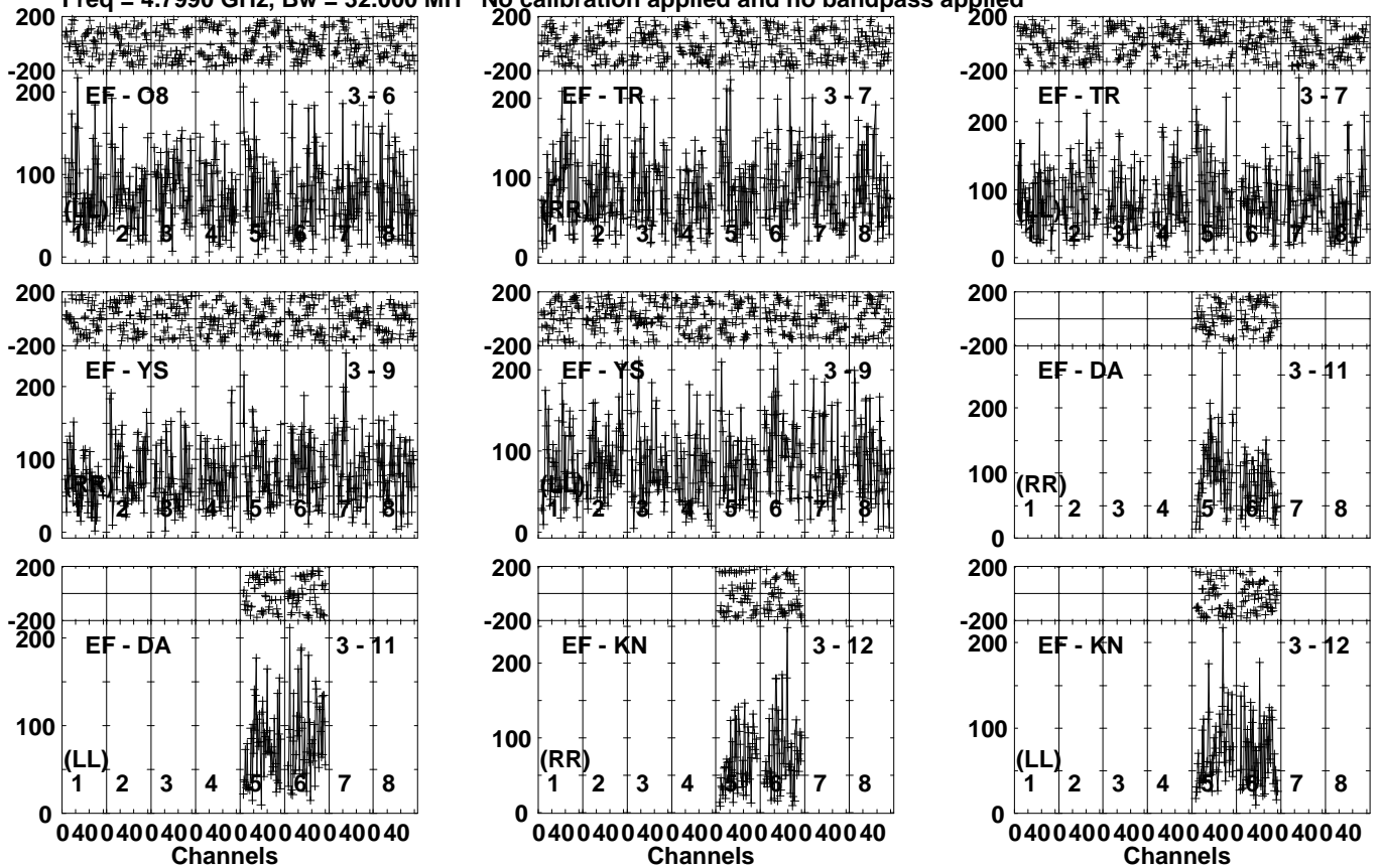
Lower frame: Micro Ampl Jy Top frame: Phas deg Vector averaged cross-power spectrum Several baselines displayed Timerange: 01/00:25:11 to 01/00:28:39
