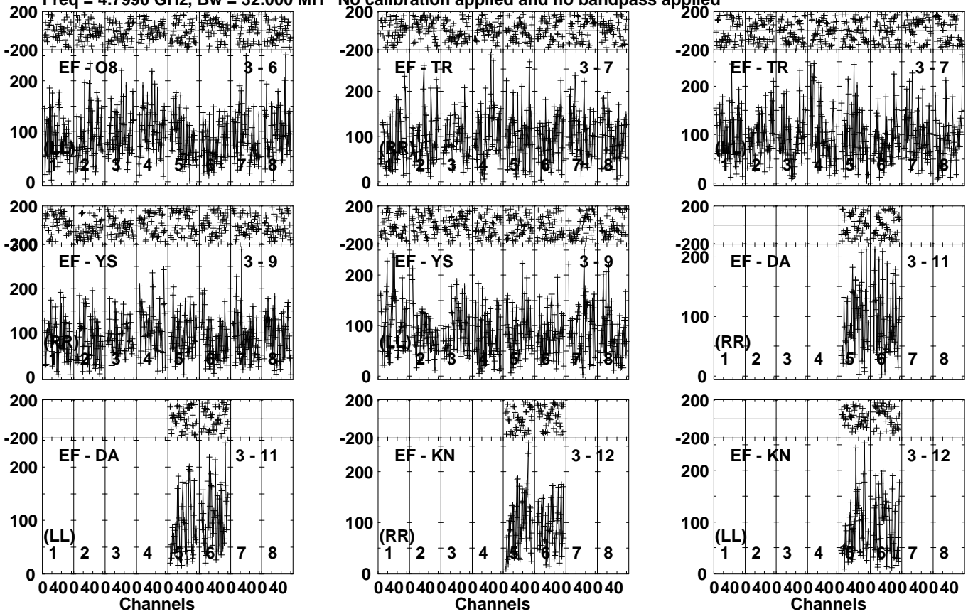
Lower frame: Micro Ampl Jy Top frame: Phas deg Vector averaged cross-power spectrum Several baselines displayed Timerange: 01/02:22:01 to 01/02:24:59
