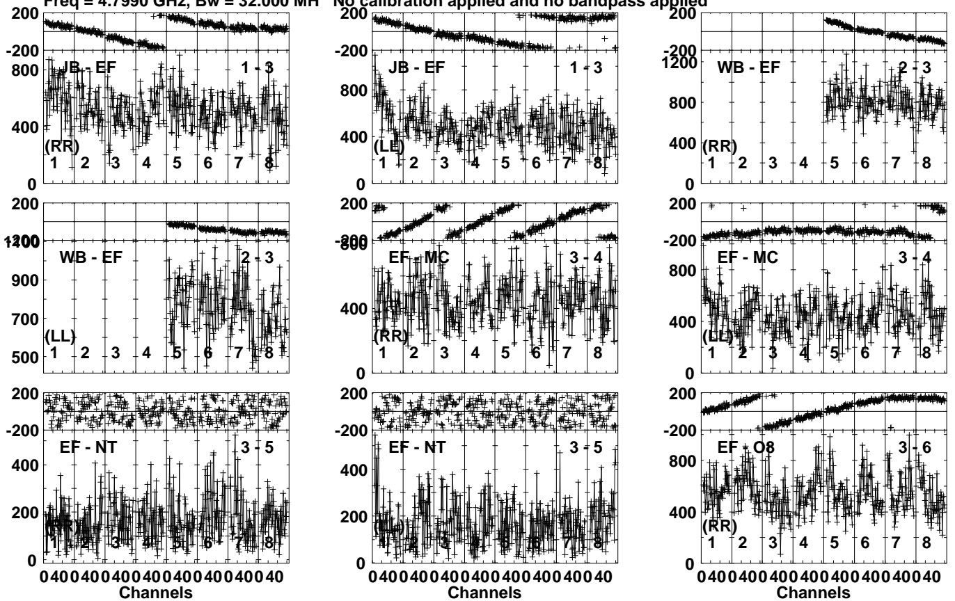
Lower frame: Micro Ampl Jy Top frame: Phas deg Vector averaged cross-power spectrum Several baselines displayed Timerange: 01/00:04:01 to 01/00:05:29
