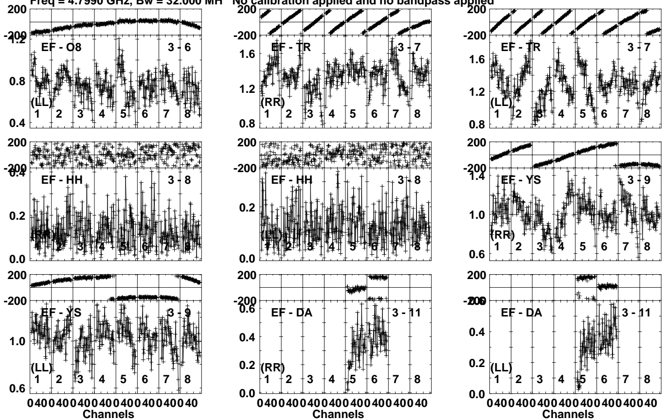
Lower frame: Milli Ampl Jy Top frame: Phas deg Vector averaged cross-power spectrum Several baselines displayed Timerange: 00/23:14:01 to 00/23:15:59
