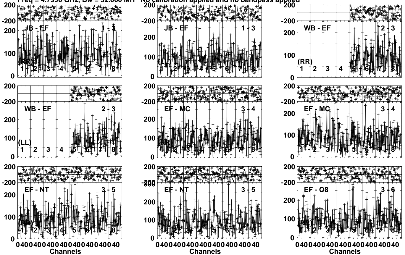
Lower frame: Micro Ampl Jy Top frame: Phas deg Vector averaged cross-power spectrum Several baselines displayed Timerange: 01/01:10:41 to 01/01:13:39
