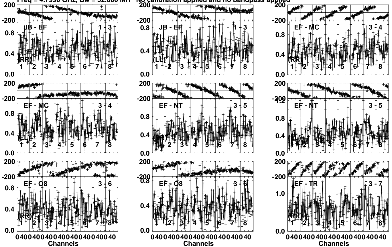
Lower frame: Milli Ampl Jy Top frame: Phas deg Vector averaged cross-power spectrum Several baselines displayed Timerange: 01/05:22:51 to 01/05:23:49
