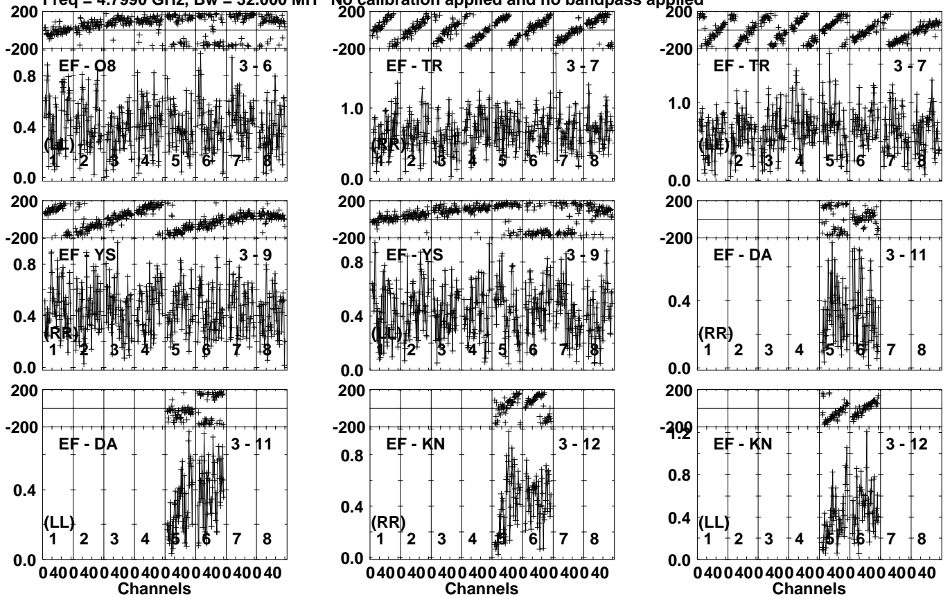
Lower frame: Milli Ampl Jy Top frame: Phas deg Vector averaged cross-power spectrum Several baselines displayed Timerange: 01/01:09:41 to 01/01:10:39
