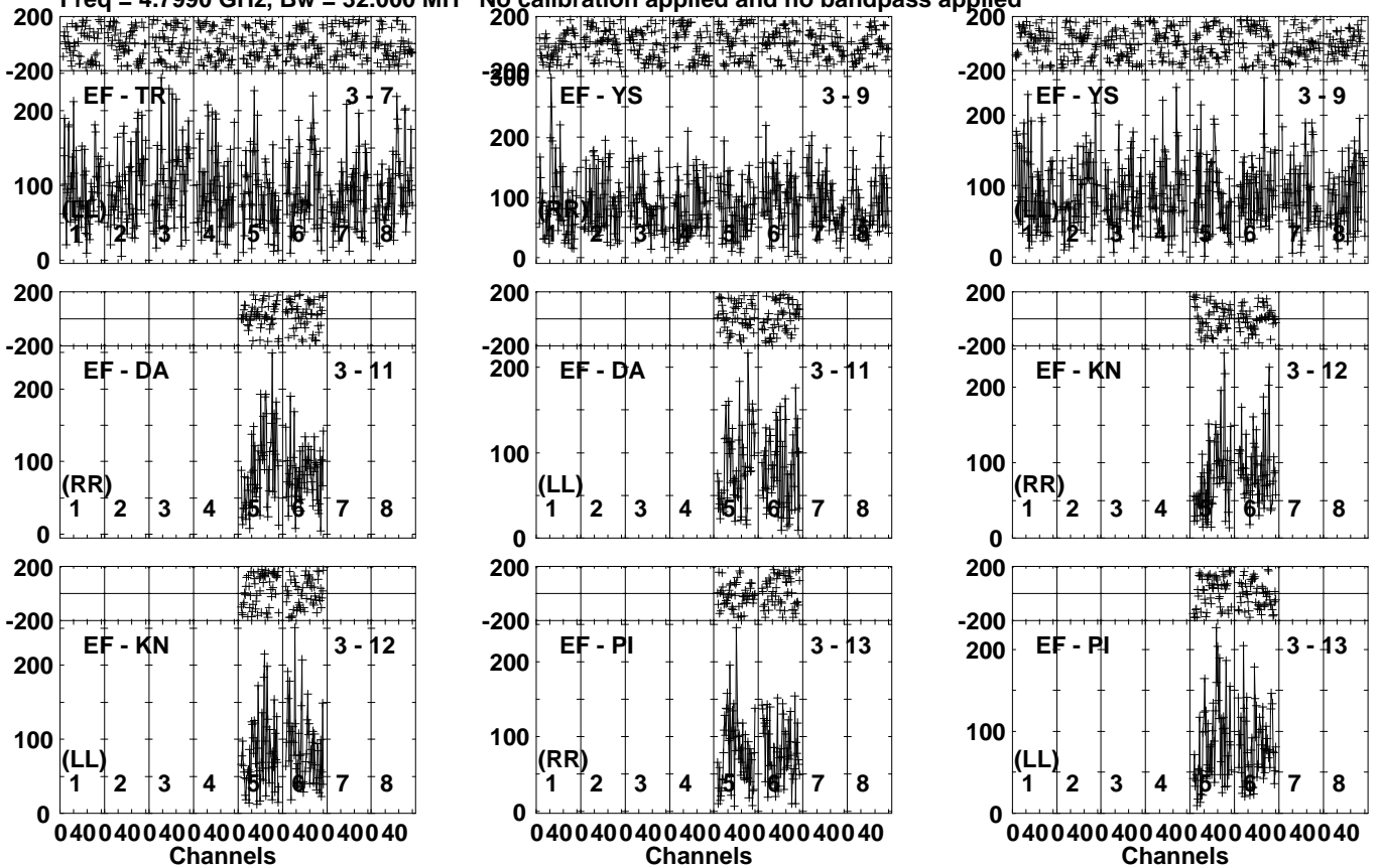
Lower frame: Micro Ampl Jy Top frame: Phas deg Vector averaged cross-power spectrum Several baselines displayed Timerange: 01/05:32:01 to 01/05:34:59
