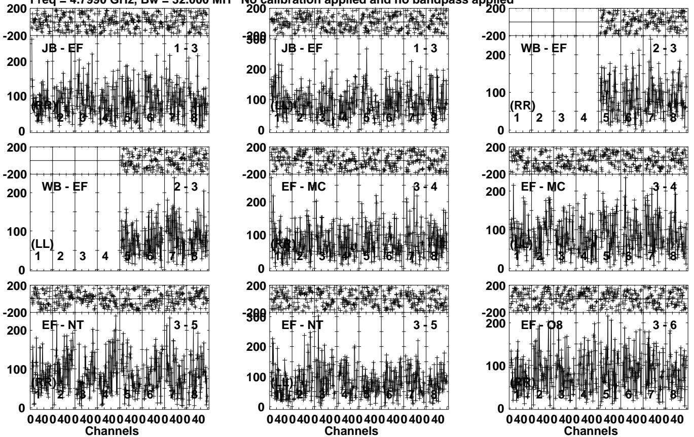
Lower frame: Micro Ampl Jy Top frame: Phas deg Vector averaged cross-power spectrum Several baselines displayed Timerange: 01/03:59:01 to 01/04:02:29
