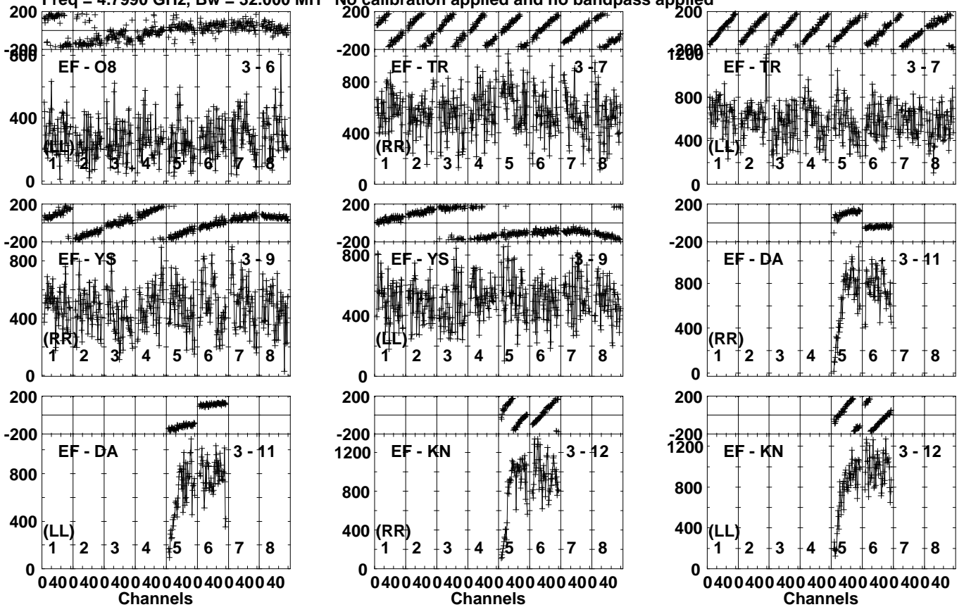
Lower frame: Micro Ampl Jy Top frame: Phas deg Vector averaged cross-power spectrum Several baselines displayed Timerange: 01/03:48:01 to 01/03:49:19
