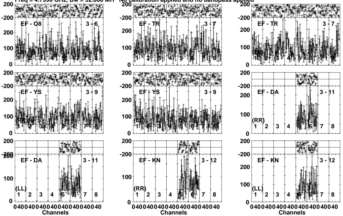
Lower frame: Micro Ampl Jy Top frame: Phas deg Vector averaged cross-power spectrum Several baselines displayed Timerange: 01/01:53:01 to 01/01:55:59
