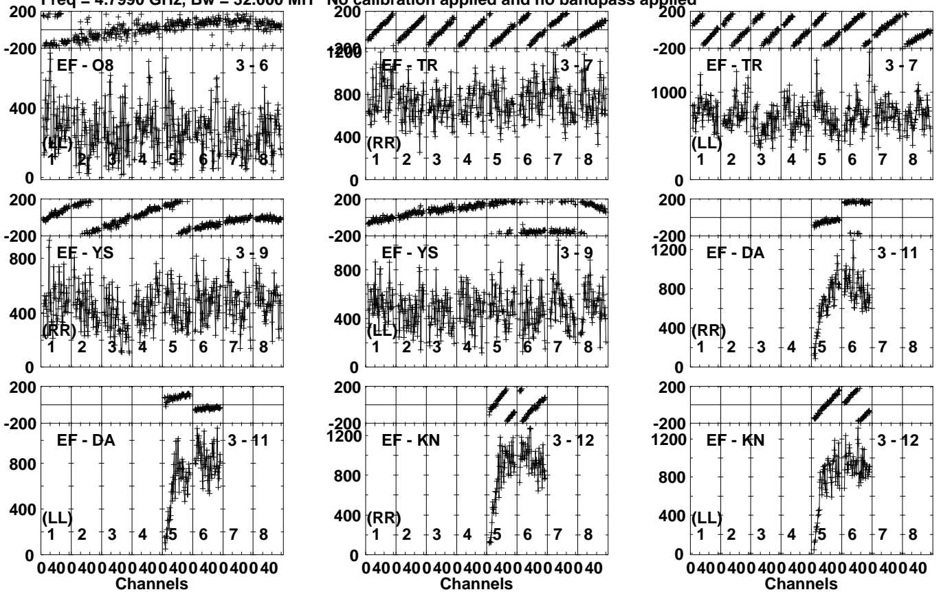
Lower frame: Micro Ampl Jy Top frame: Phas deg Vector averaged cross-power spectrum Several baselines displayed Timerange: 01/03:33:31 to 01/03:34:49
