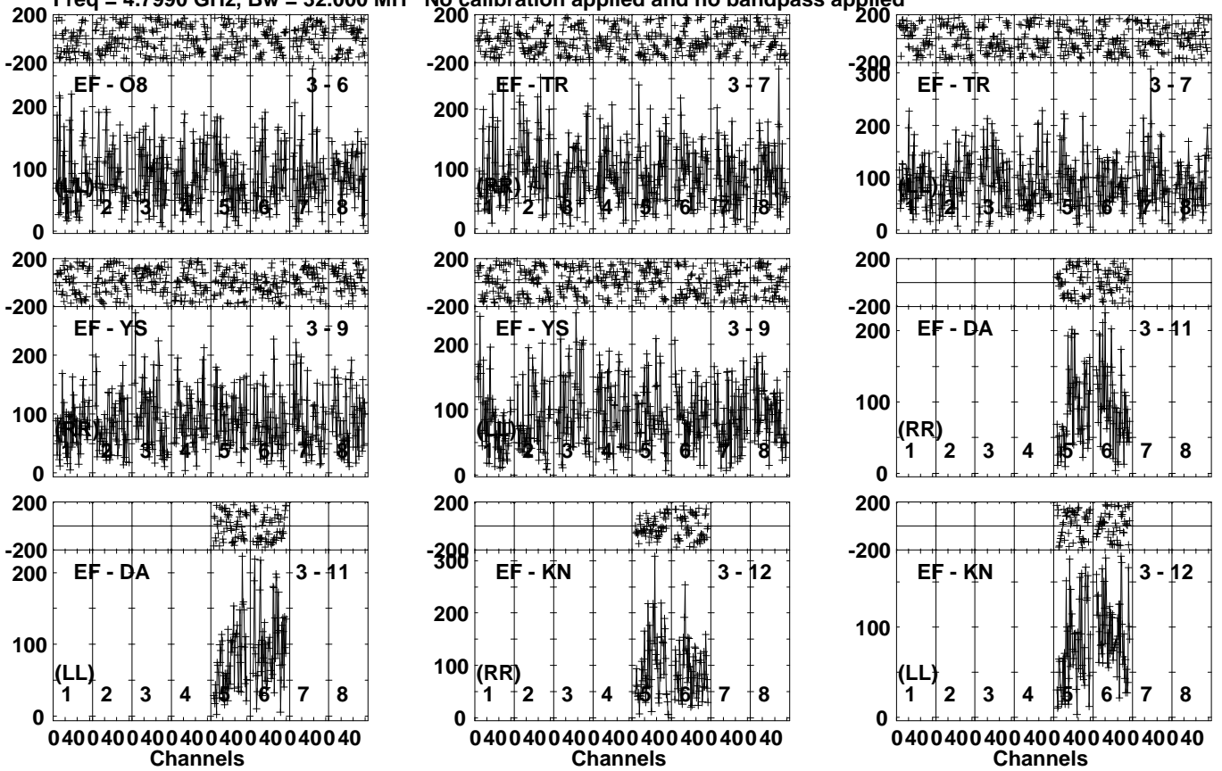
Lower frame: Micro Ampl Jy Top frame: Phas deg Vector averaged cross-power spectrum Several baselines displayed Timerange: 01/02:09:41 to 01/02:12:39
