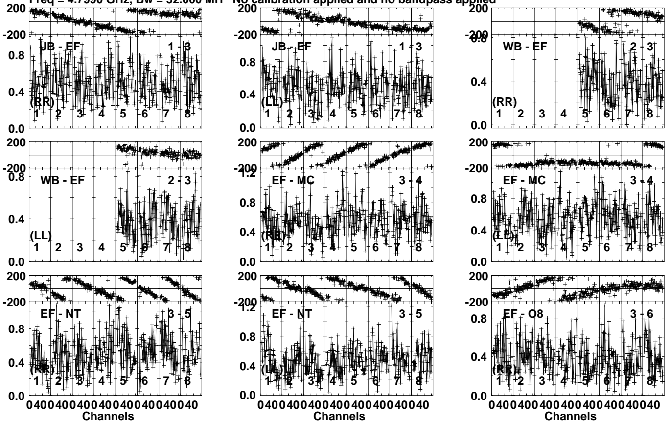
Lower frame: Milli Ampl Jy Top frame: Phas deg Vector averaged cross-power spectrum Several baselines displayed Timerange: 01/00:37:11 to 01/00:38:09
