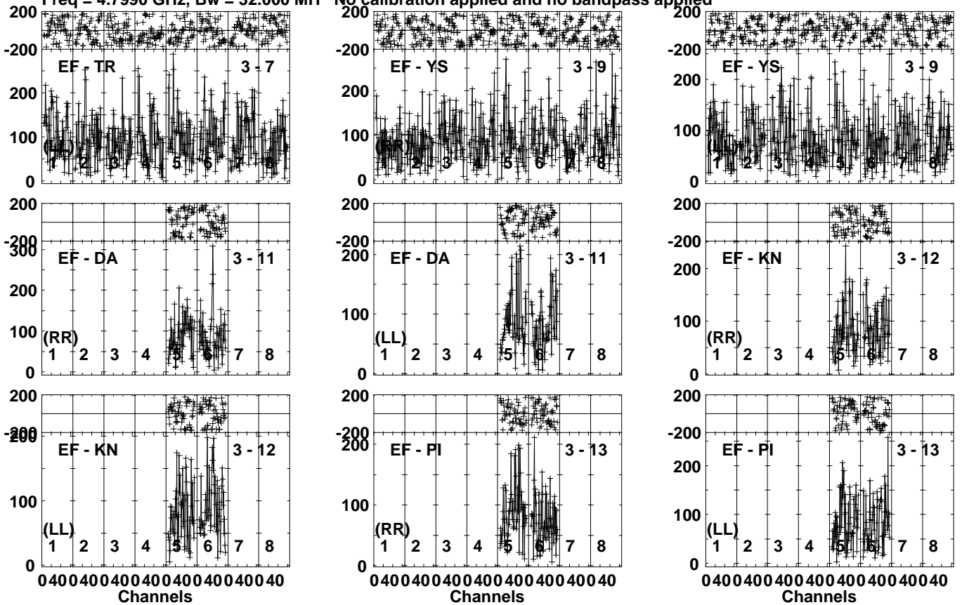
Lower frame: Micro Ampl Jy Top frame: Phas deg Vector averaged cross-power spectrum Several baselines displayed Timerange: 01/05:40:01 to 01/05:42:59
