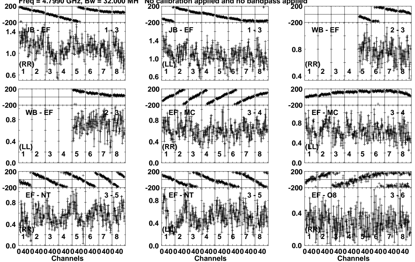
Lower frame: Milli Ampl Jy Top frame: Phas deg Vector averaged cross-power spectrum Several baselines displayed Timerange: 01/03:19:01 to 01/03:20:19
