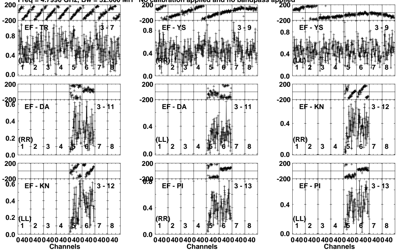
Lower frame: Milli Ampl Jy Top frame: Phas deg Vector averaged cross-power spectrum Several baselines displayed Timerange: 01/05:19:11 to 01/05:19:49
