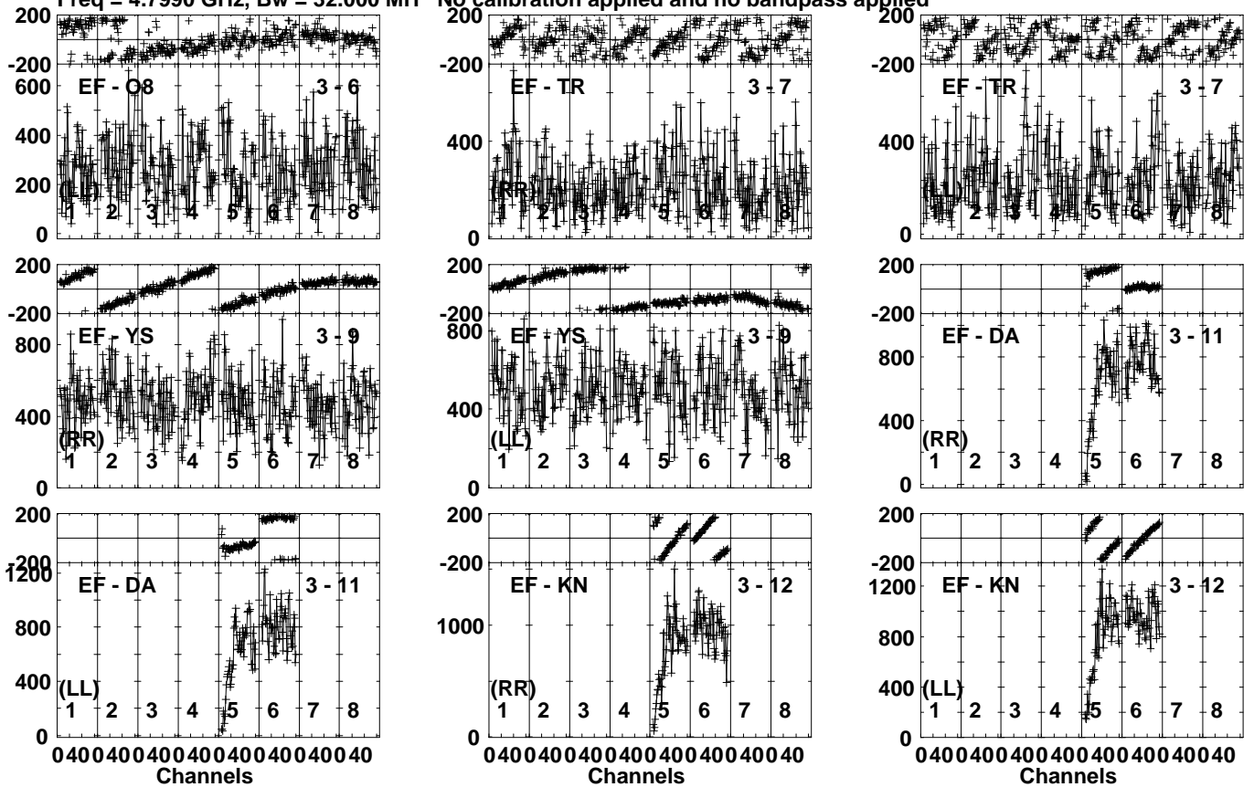
Lower frame: Micro Ampl Jy Top frame: Phas deg Vector averaged cross-power spectrum Several baselines displayed Timerange: 01/03:52:51 to 01/03:54:09
