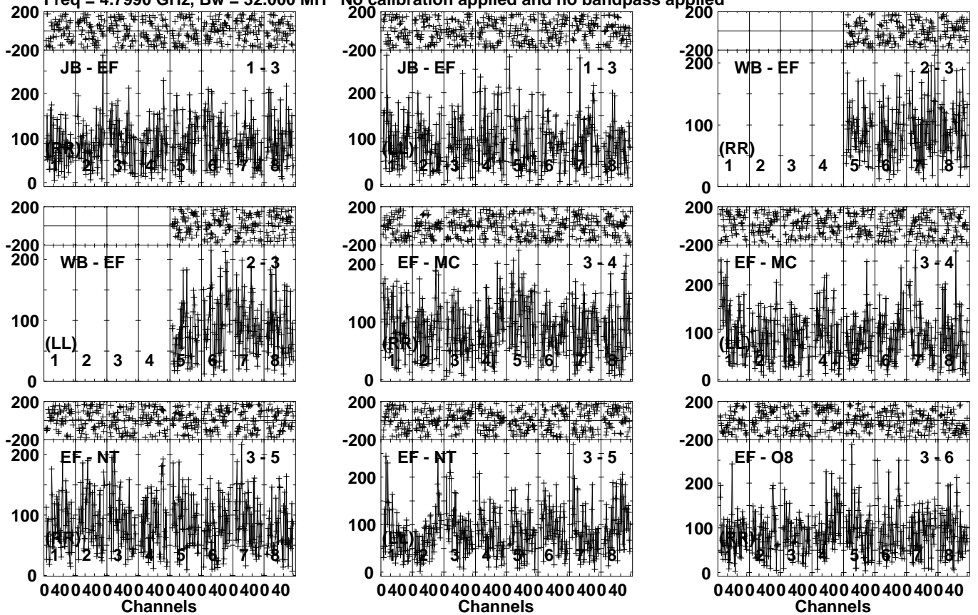
Lower frame: Micro Ampl Jy Top frame: Phas deg Vector averaged cross-power spectrum Several baselines displayed Timerange: 01/02:50:41 to 01/02:53:39
