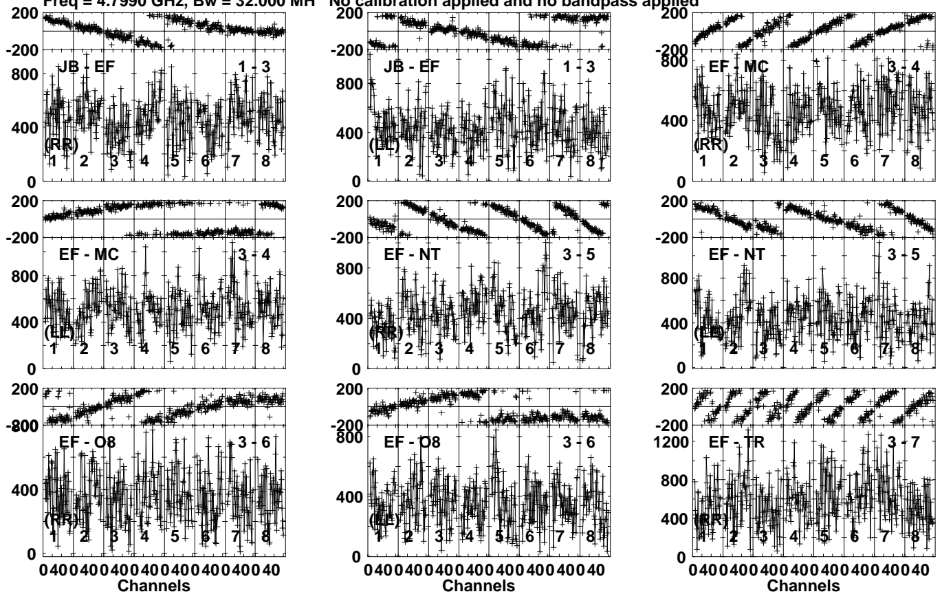
Lower frame: Micro Ampl Jy Top frame: Phas deg Vector averaged cross-power spectrum Several baselines displayed Timerange: 01/05:14:41 to 01/05:15:39
