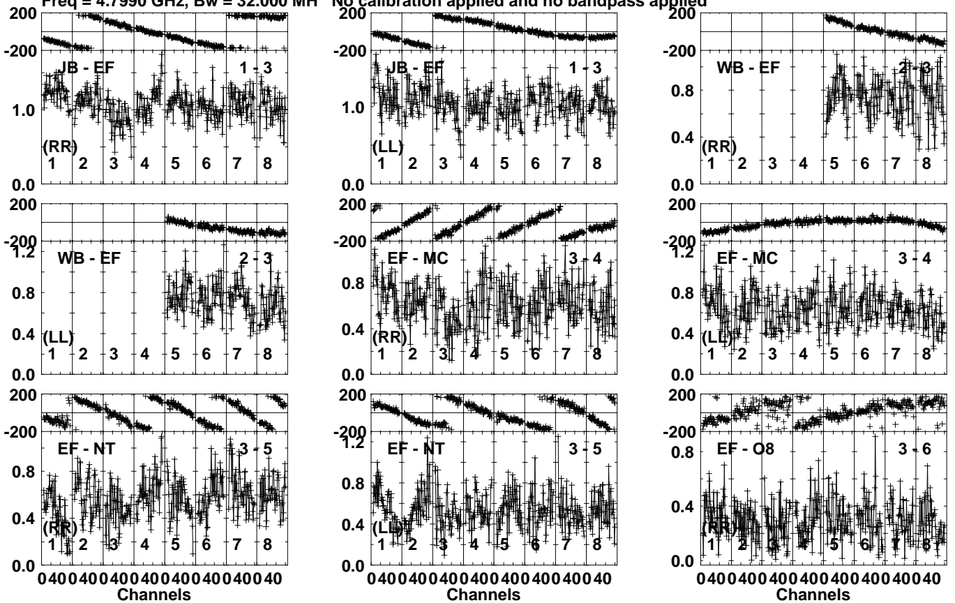
Lower frame: Milli Ampl Jy Top frame: Phas deg Vector averaged cross-power spectrum Several baselines displayed Timerange: 01/03:09:21 to 01/03:10:39
