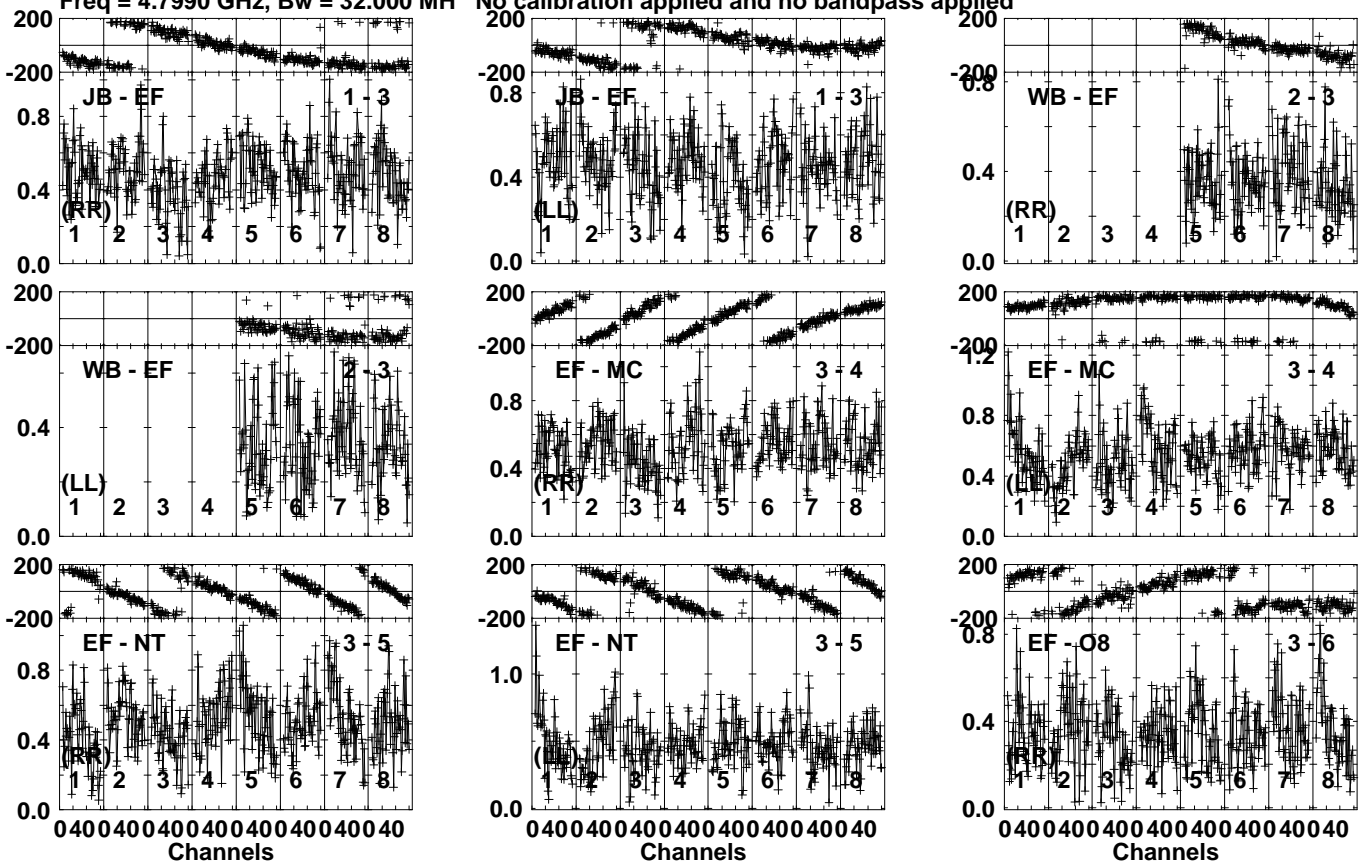
Lower frame: Milli Ampl Jy Top frame: Phas deg Vector averaged cross-power spectrum Several baselines displayed Timerange: 01/01:06:01 to 01/01:06:39
