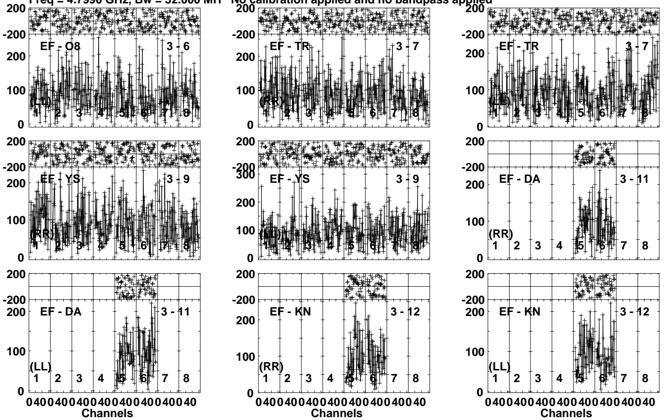
Lower frame: Micro Ampl Jy Top frame: Phas deg Vector averaged cross-power spectrum Several baselines displayed Timerange: 00/22:28:01 to 00/22:30:59
