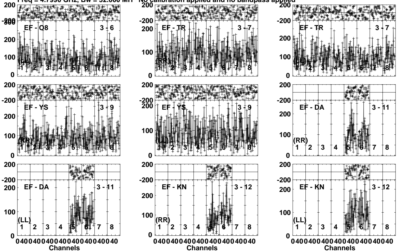
Lower frame: Micro Ampl Jy Top frame: Phas deg Vector averaged cross-power spectrum Several baselines displayed Timerange: 00/22:40:21 to 00/22:43:19
