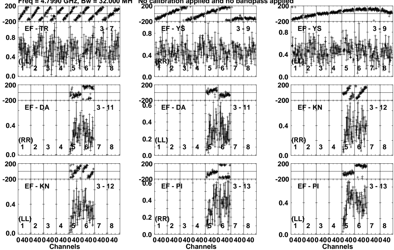
Lower frame: Milli Ampl Jy Top frame: Phas deg Vector averaged cross-power spectrum Several baselines displayed Timerange: 01/05:31:21 to 01/05:31:59
