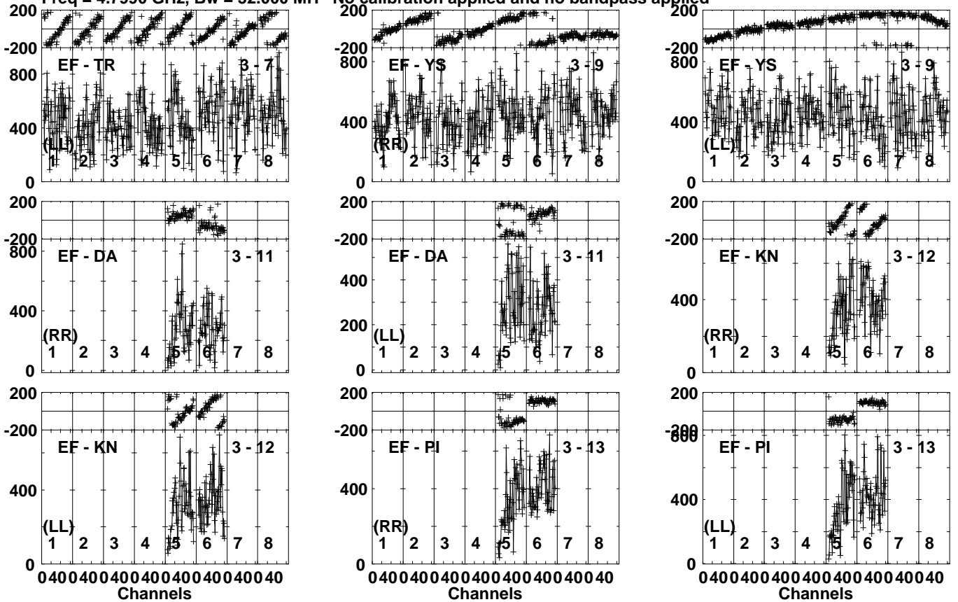
Lower frame: Micro Ampl Jy Top frame: Phas deg Vector averaged cross-power spectrum Several baselines displayed Timerange: 01/04:42:41 to 01/04:43:19
