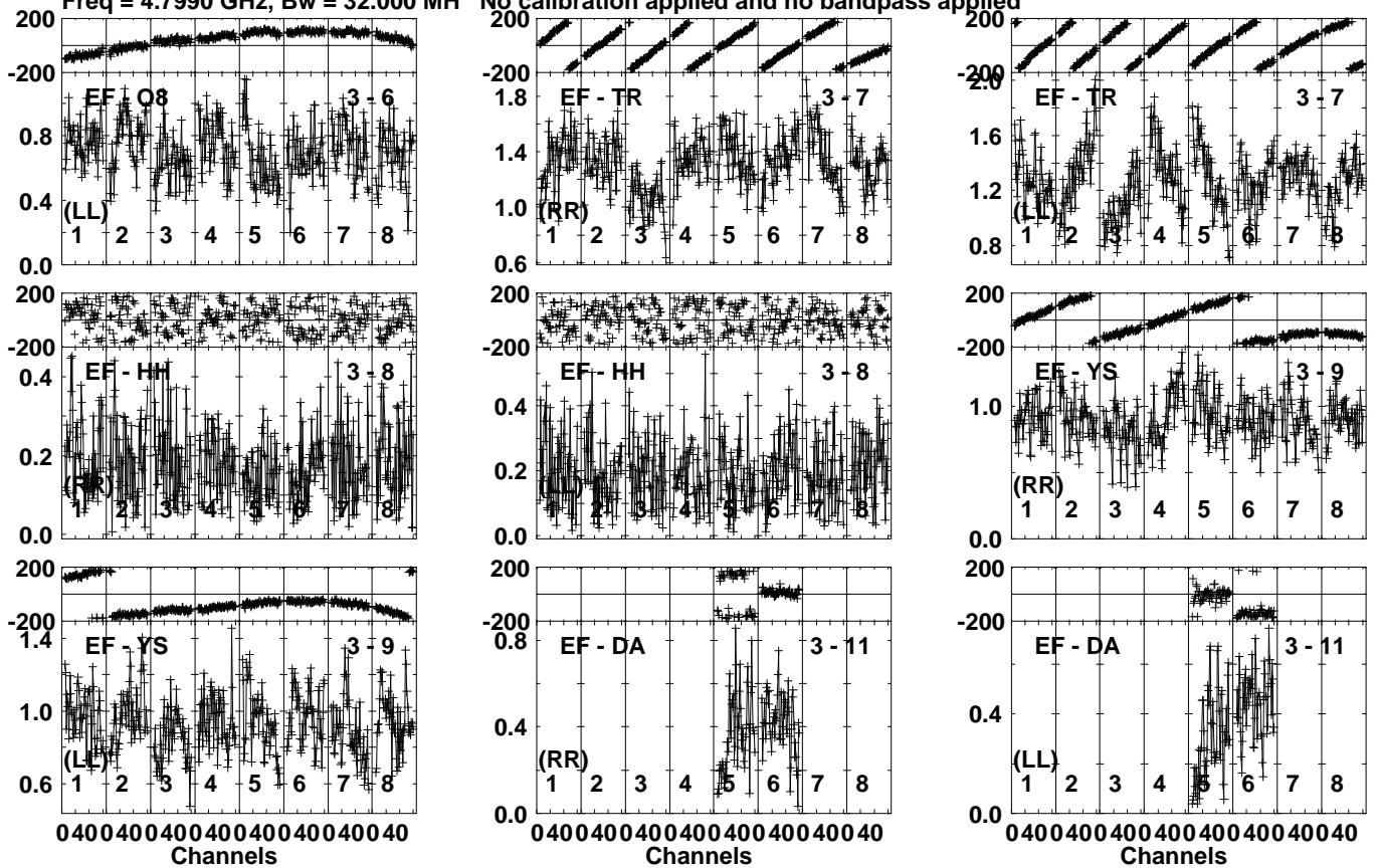
Lower frame: Milli Ampl Jy Top frame: Phas deg Vector averaged cross-power spectrum Several baselines displayed Timerange: 00/23:29:21 to 00/23:30:49
