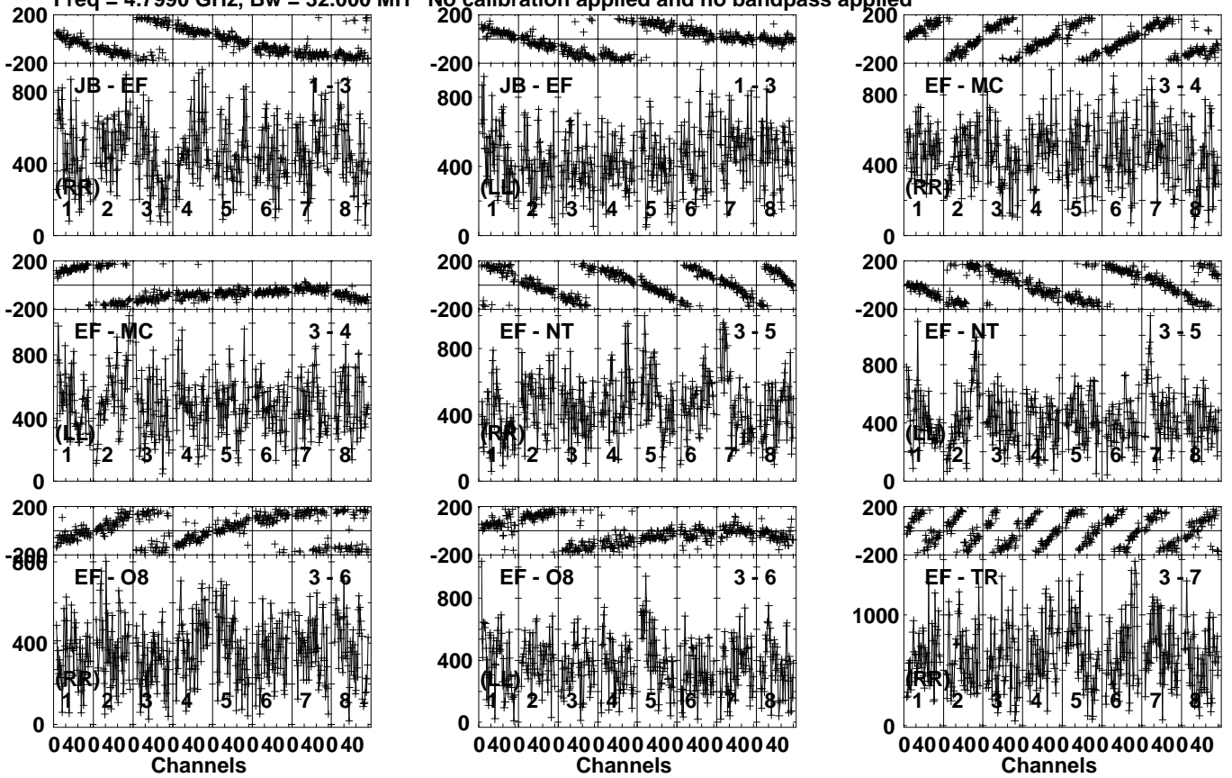
Lower frame: Micro Ampl Jy Top frame: Phas deg Vector averaged cross-power spectrum Several baselines displayed Timerange: 01/05:26:51 to 01/05:27:49
