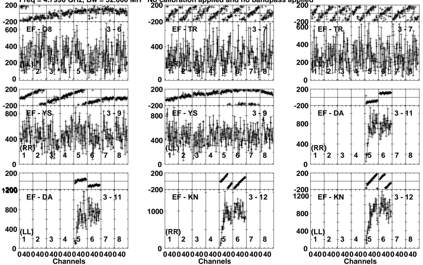
Lower frame: Micro Ampl Jy Top frame: Phas deg Vector averaged cross-power spectrum Several baselines displayed Timerange: 01/03:29:11 to 01/03:29:59
