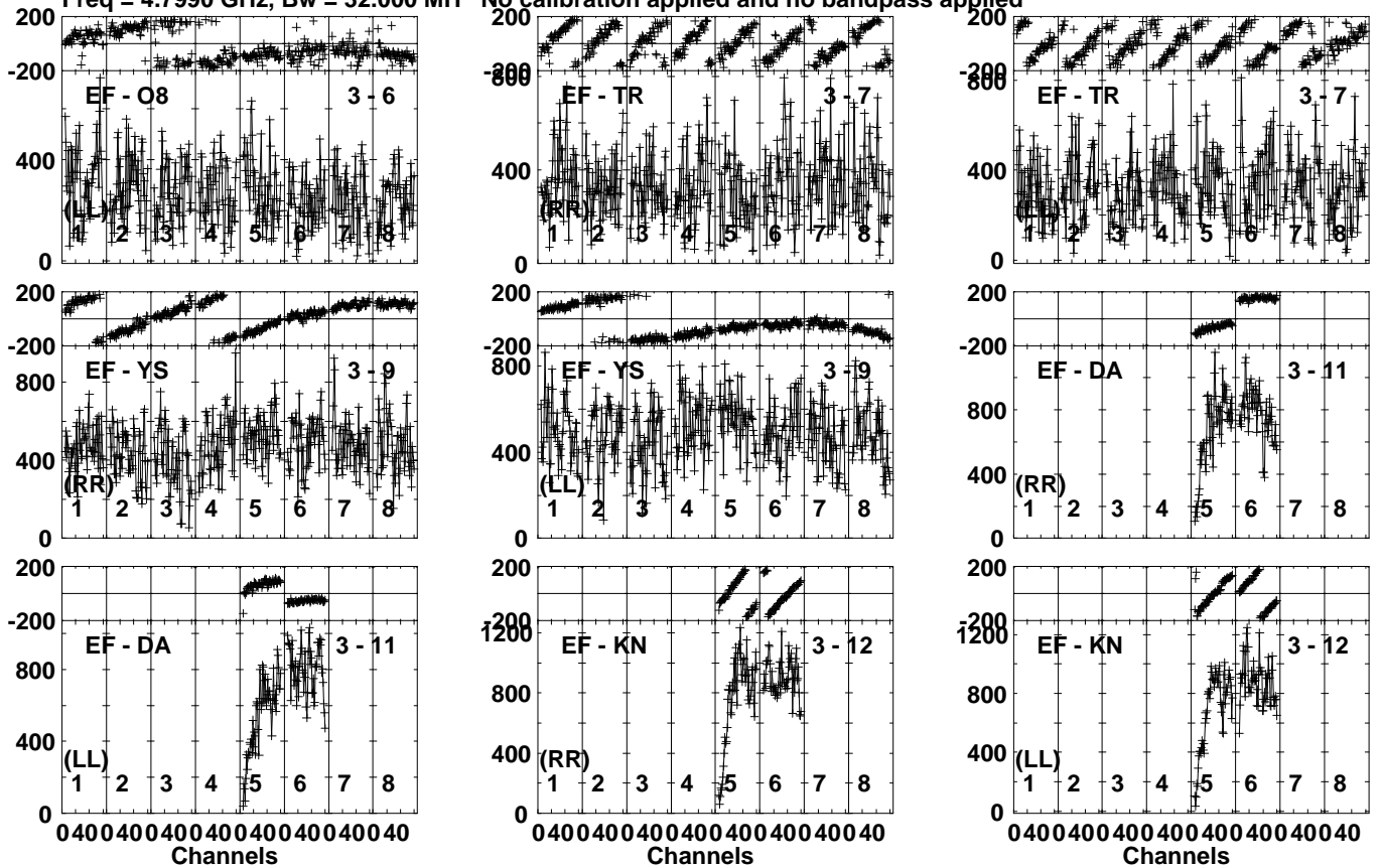
Lower frame: Micro Ampl Jy Top frame: Phas deg Vector averaged cross-power spectrum Several baselines displayed Timerange: 01/04:02:31 to 01/04:03:49
