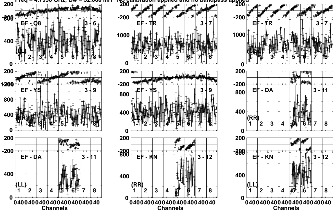
Lower frame: Micro Ampl Jy Top frame: Phas deg Vector averaged cross-power spectrum Several baselines displayed Timerange: 01/00:49:21 to 01/00:50:19
