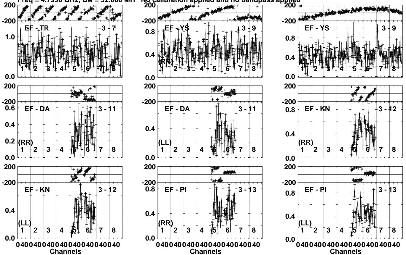
Lower frame: Milli Ampl Jy Top frame: Phas deg Vector averaged cross-power spectrum Several baselines displayed Timerange: 01/04:38:11 to 01/04:39:09
