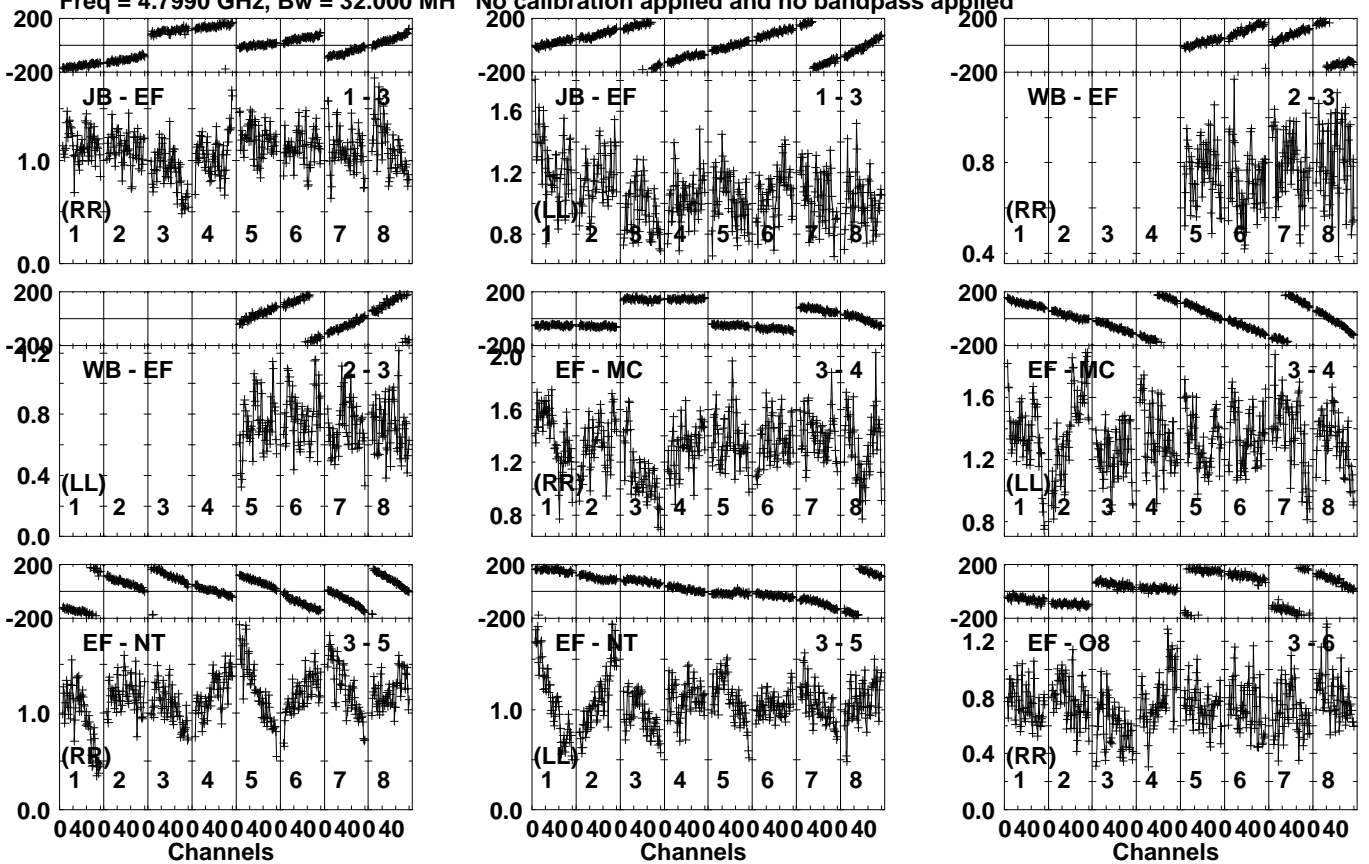
Lower frame: Milli Ampl Jy Top frame: Phas deg Vector averaged cross-power spectrum Several baselines displayed Timerange: 00/07:34:31 to 00/07:35:19
