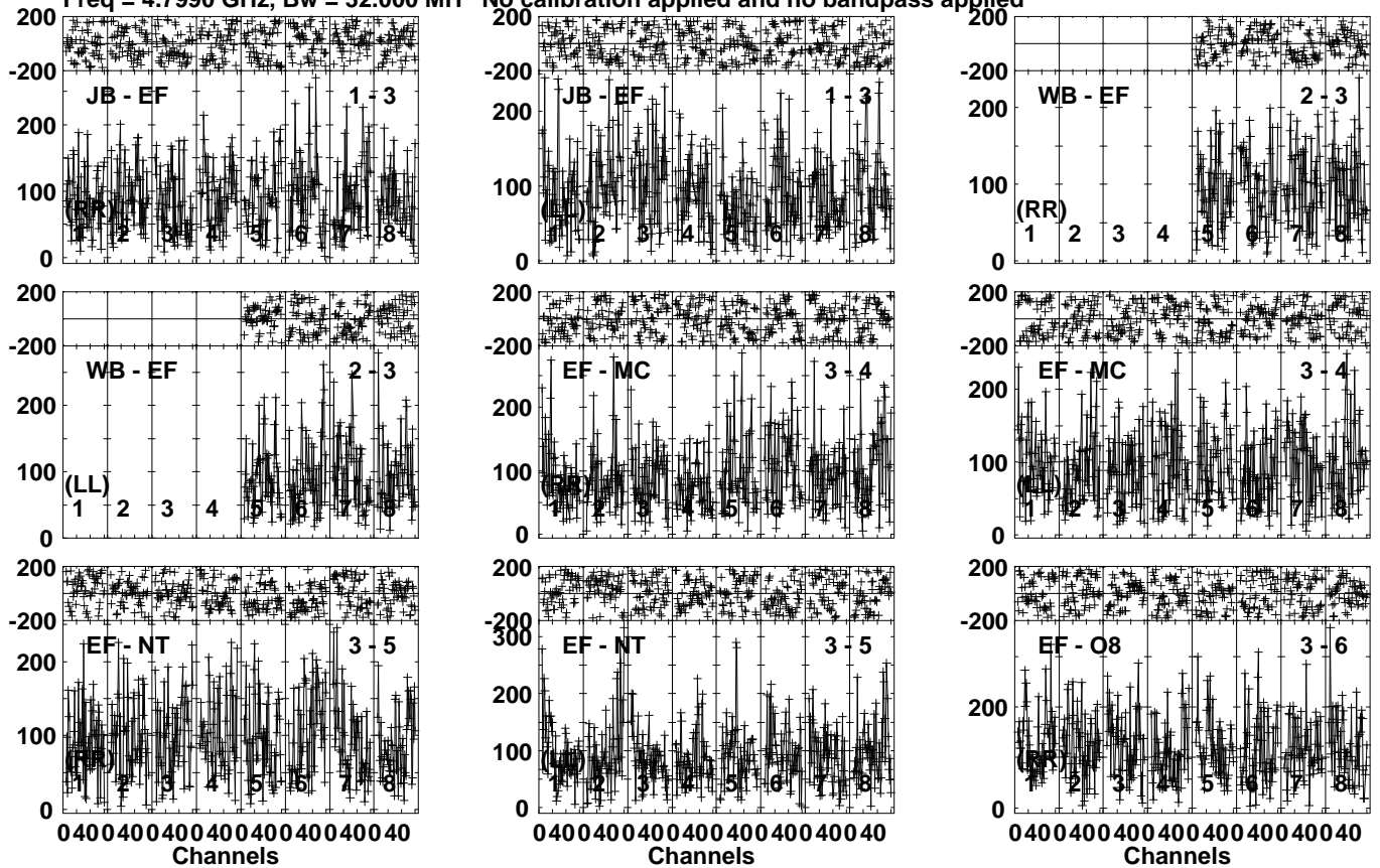
Lower frame: Micro Ampl Jy Top frame: Phas deg Vector averaged cross-power spectrum Several baselines displayed Timerange: 00/12:56:11 to 00/12:59:09
