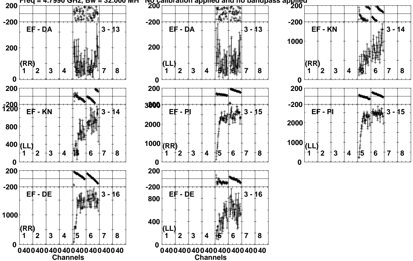
Lower frame: Micro Ampl Jy Top frame: Phas deg Vector averaged cross-power spectrum Several baselines displayed Timerange: 00/12:55:21 to 00/12:56:09
