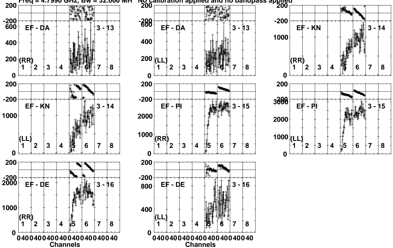
Lower frame: Micro Ampl Jy Top frame: Phas deg Vector averaged cross-power spectrum Several baselines displayed Timerange: 00/13:49:51 to 00/13:50:59
