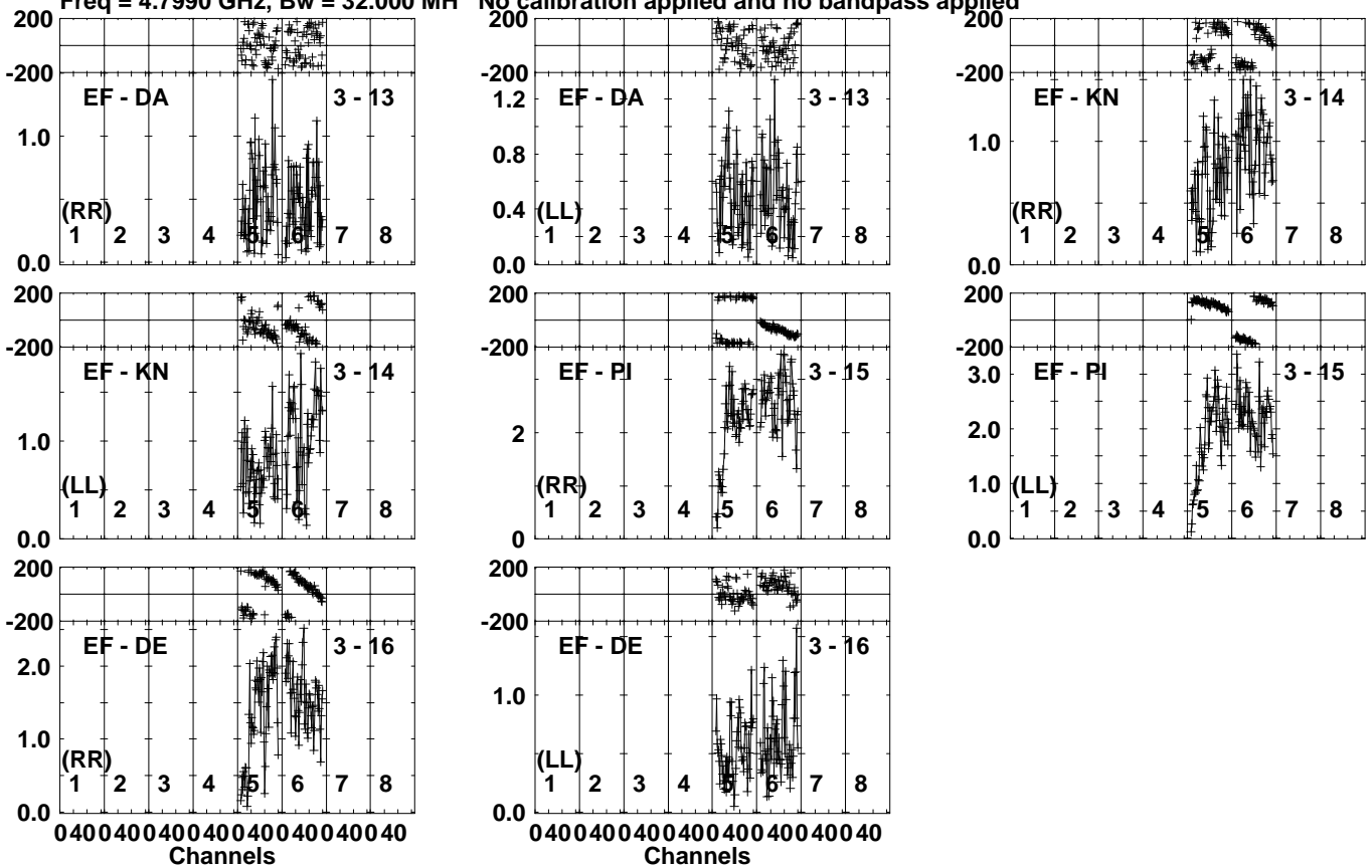
Lower frame: Milli Ampl Jy Top frame: Phas deg Vector averaged cross-power spectrum Several baselines displayed Timerange: 00/12:33:51 to 00/12:34:59
