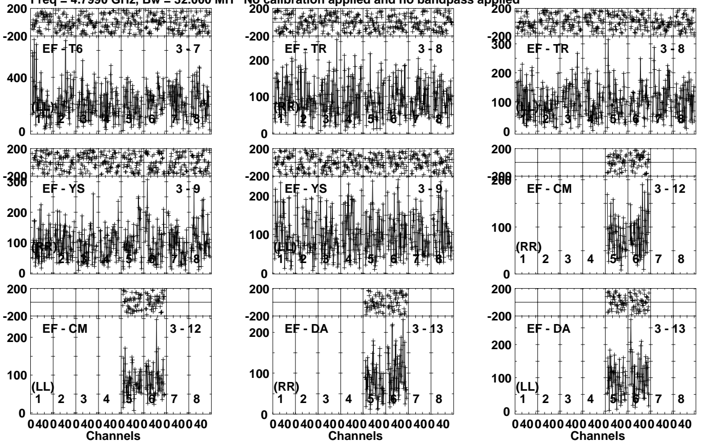
Lower frame: Micro Ampl Jy Top frame: Phas deg Vector averaged cross-power spectrum Several baselines displayed Timerange: 00/06:56:31 to 00/06:59:29
