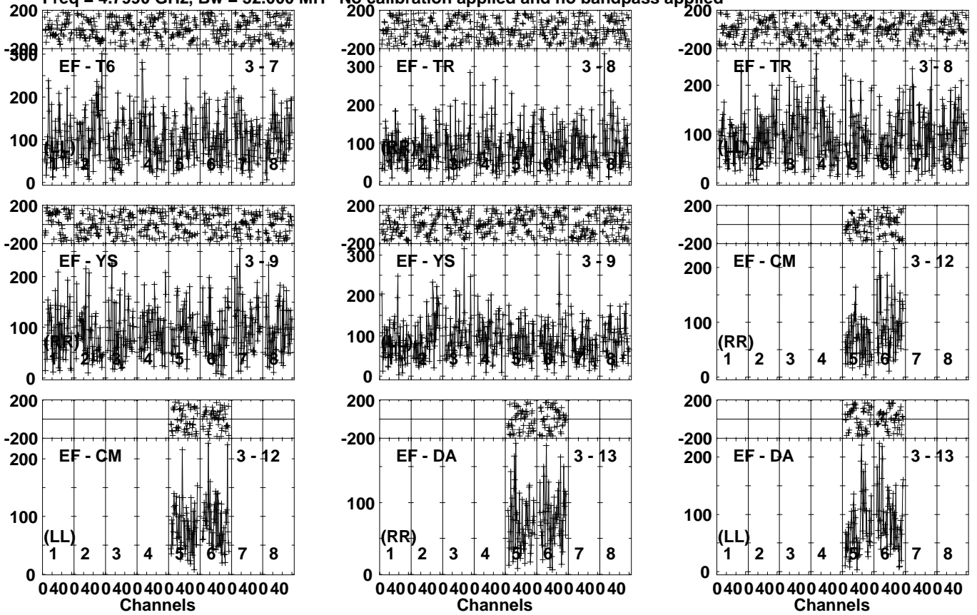
Lower frame: Micro Ampl Jy Top frame: Phas deg Vector averaged cross-power spectrum Several baselines displayed Timerange: 00/06:43:51 to 00/06:46:49
