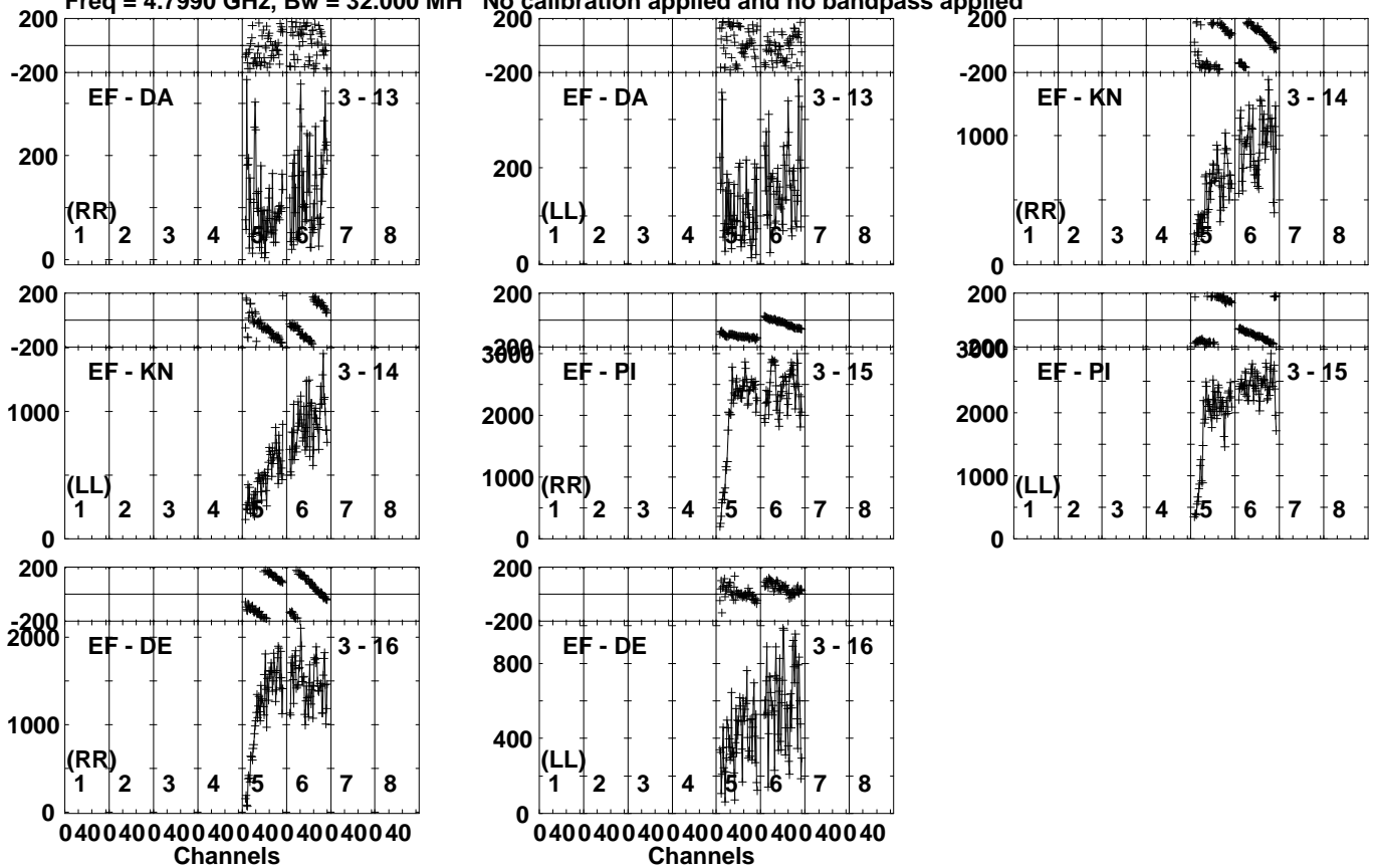
Lower frame: Micro Ampl Jy Top frame: Phas deg Vector averaged cross-power spectrum Several baselines displayed Timerange: 00/13:28:41 to 00/13:29:49
