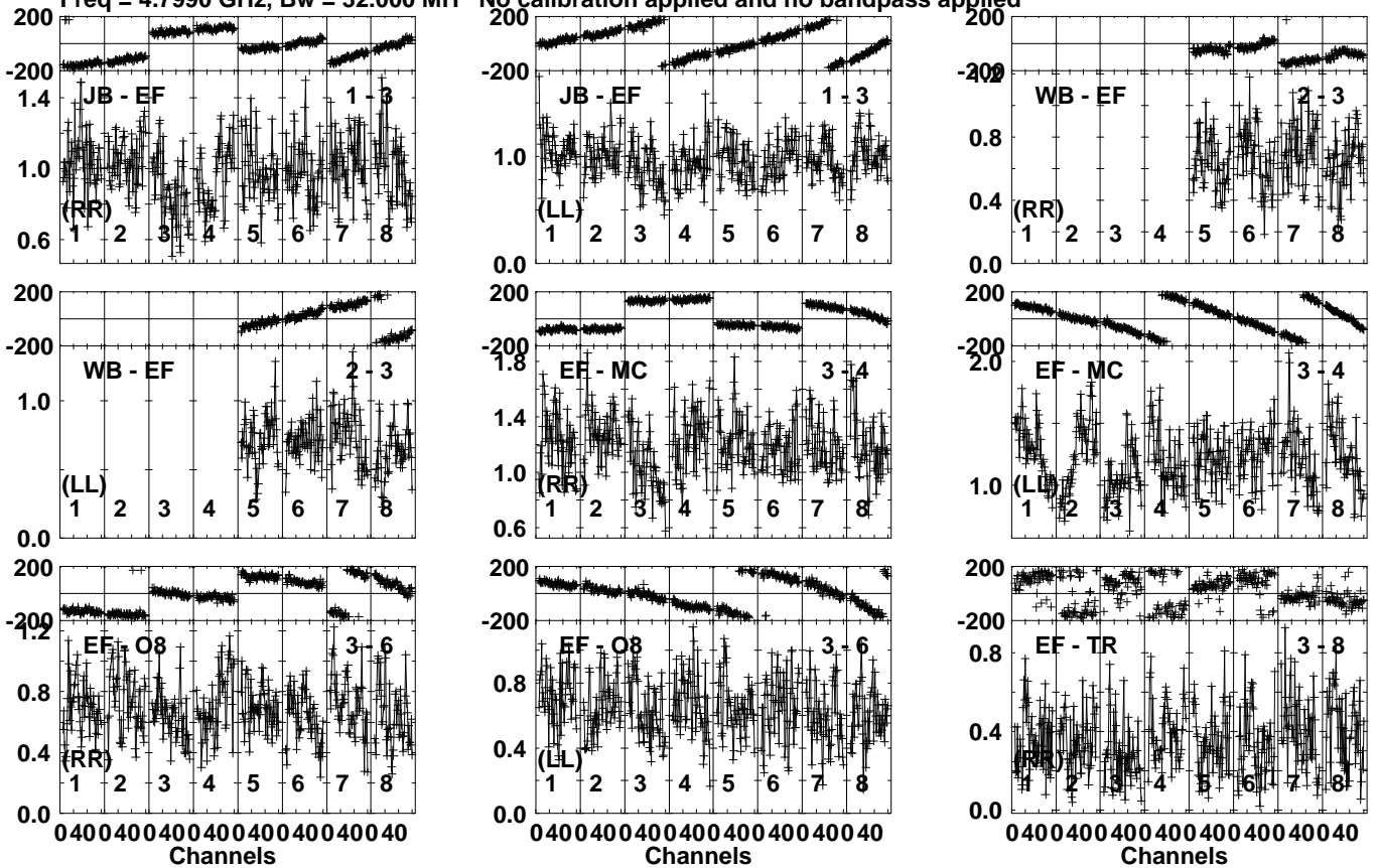
Lower frame: Milli Ampl Jy Top frame: Phas deg Vector averaged cross-power spectrum Several baselines displayed Timerange: 00/05:47:01 to 00/05:48:09
