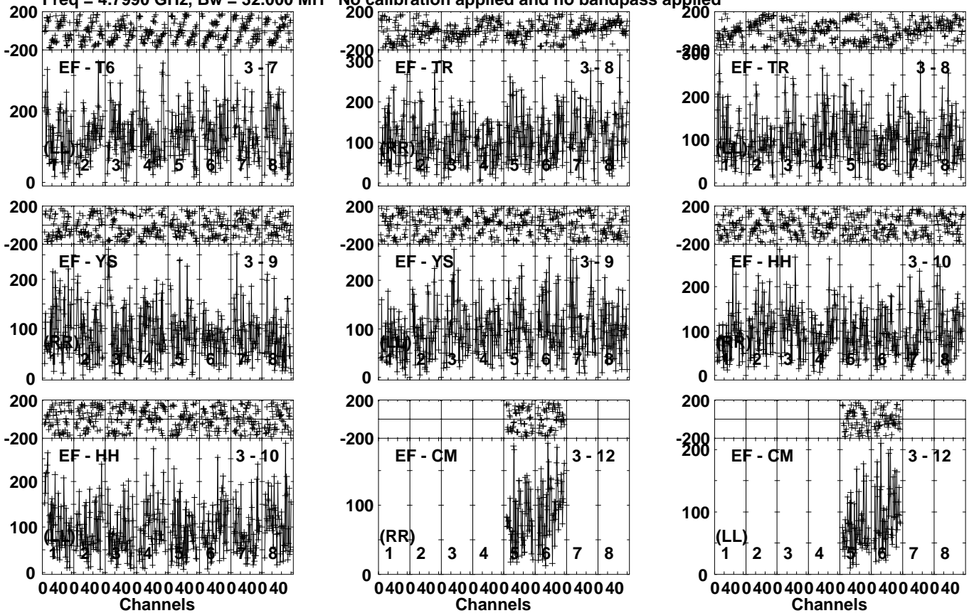
Lower frame: Micro Ampl Jy Top frame: Phas deg Vector averaged cross-power spectrum Several baselines displayed Timerange: 00/05:27:01 to 00/05:29:59
