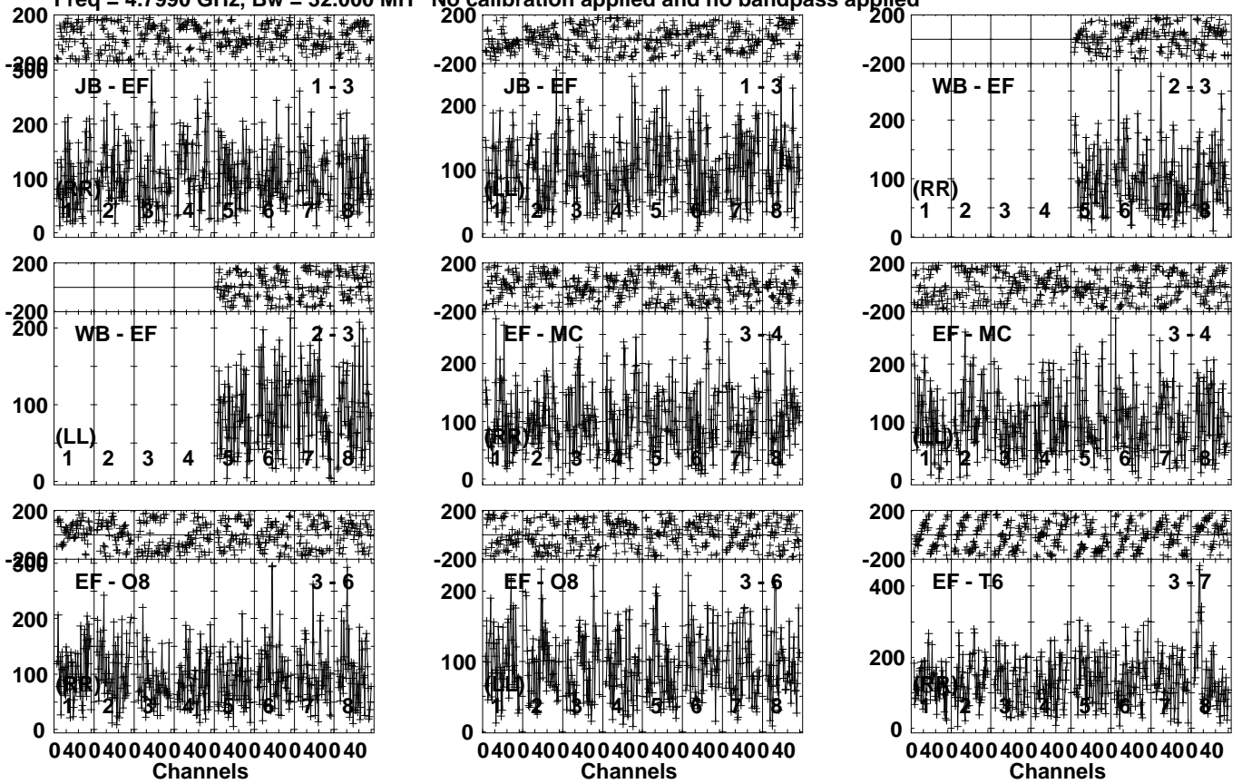
Lower frame: Micro Ampl Jy Top frame: Phas deg Vector averaged cross-power spectrum Several baselines displayed Timerange: 00/05:31:21 to 00/05:34:19
