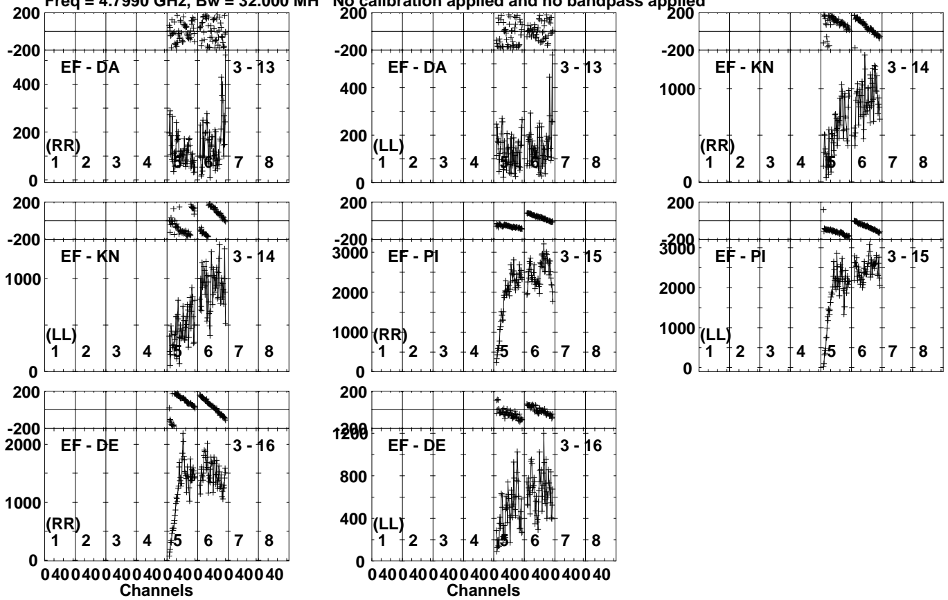
Lower frame: Micro Ampl Jy Top frame: Phas deg Vector averaged cross-power spectrum Several baselines displayed Timerange: 00/13:24:31 to 00/13:25:39
