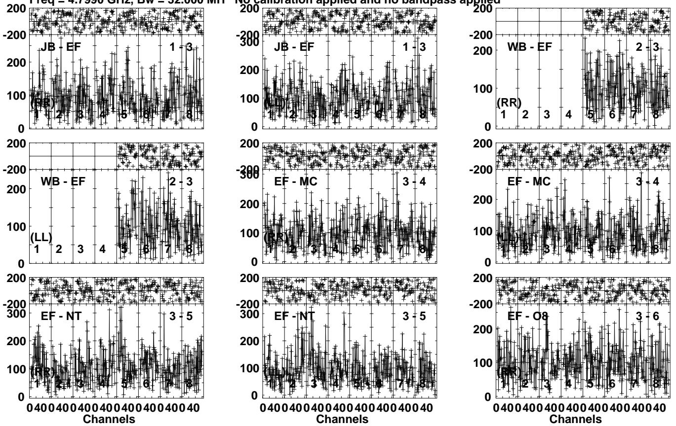
Lower frame: Micro Ampl Jy Top frame: Phas deg Vector averaged cross-power spectrum Several baselines displayed Timerange: 00/12:22:21 to 00/12:25:19
