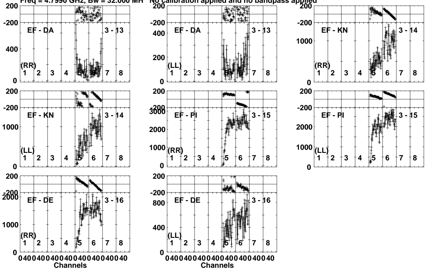
Lower frame: Micro Ampl Jy Top frame: Phas deg Vector averaged cross-power spectrum Several baselines displayed Timerange: 00/13:11:51 to 00/13:12:59
