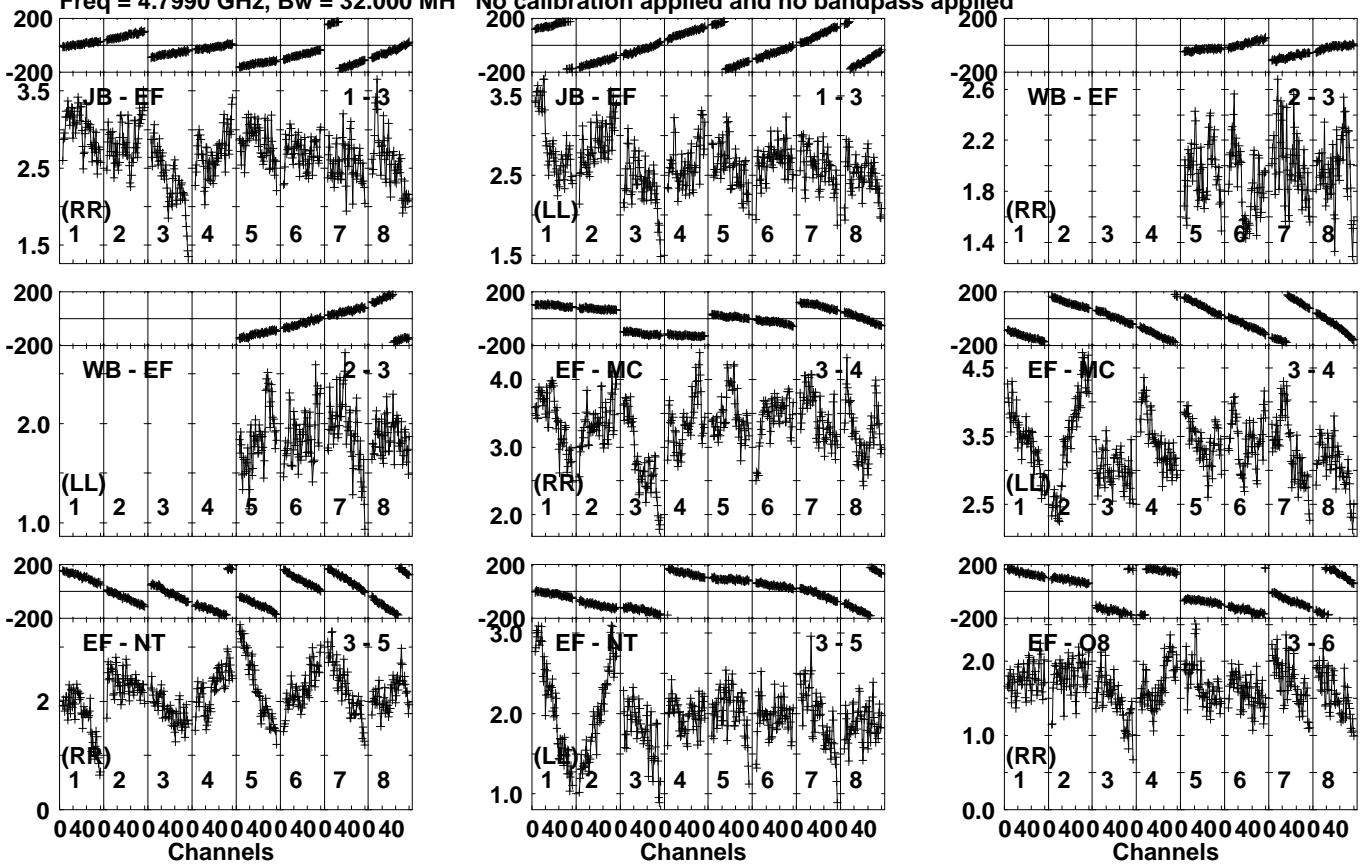
Lower frame: Milli Ampl Jy Top frame: Phas deg Vector averaged cross-power spectrum Several baselines displayed Timerange: 00/12:50:41 to 00/12:51:49
