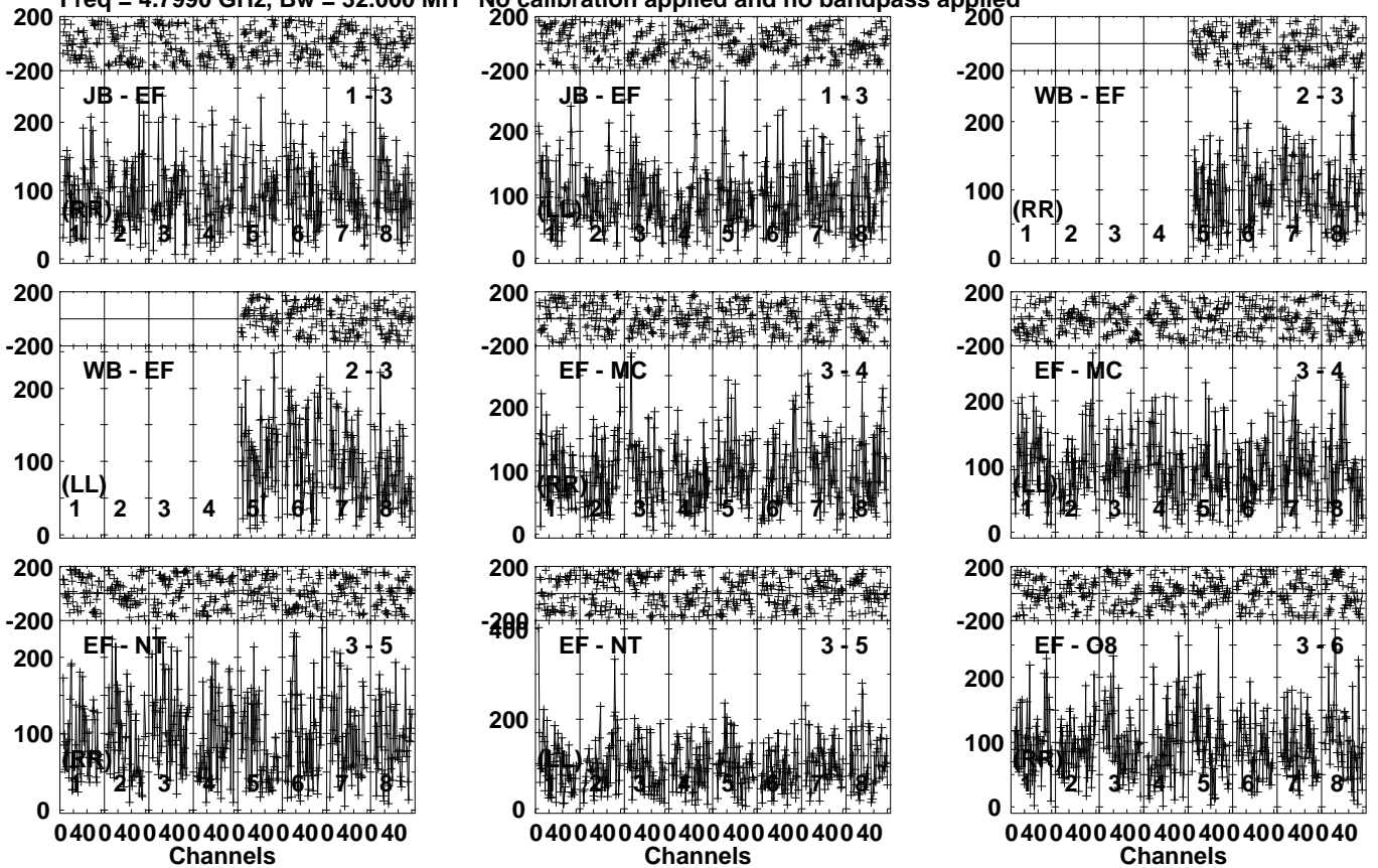
Lower frame: Micro Ampl Jy Top frame: Phas deg Vector averaged cross-power spectrum Several baselines displayed Timerange: 00/08:27:31 to 00/08:30:29
