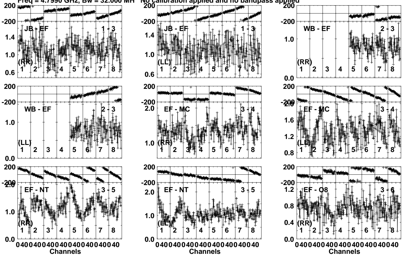
Lower frame: Milli Ampl Jy Top frame: Phas deg Vector averaged cross-power spectrum Several baselines displayed Timerange: 00/08:05:01 to 00/08:06:09
