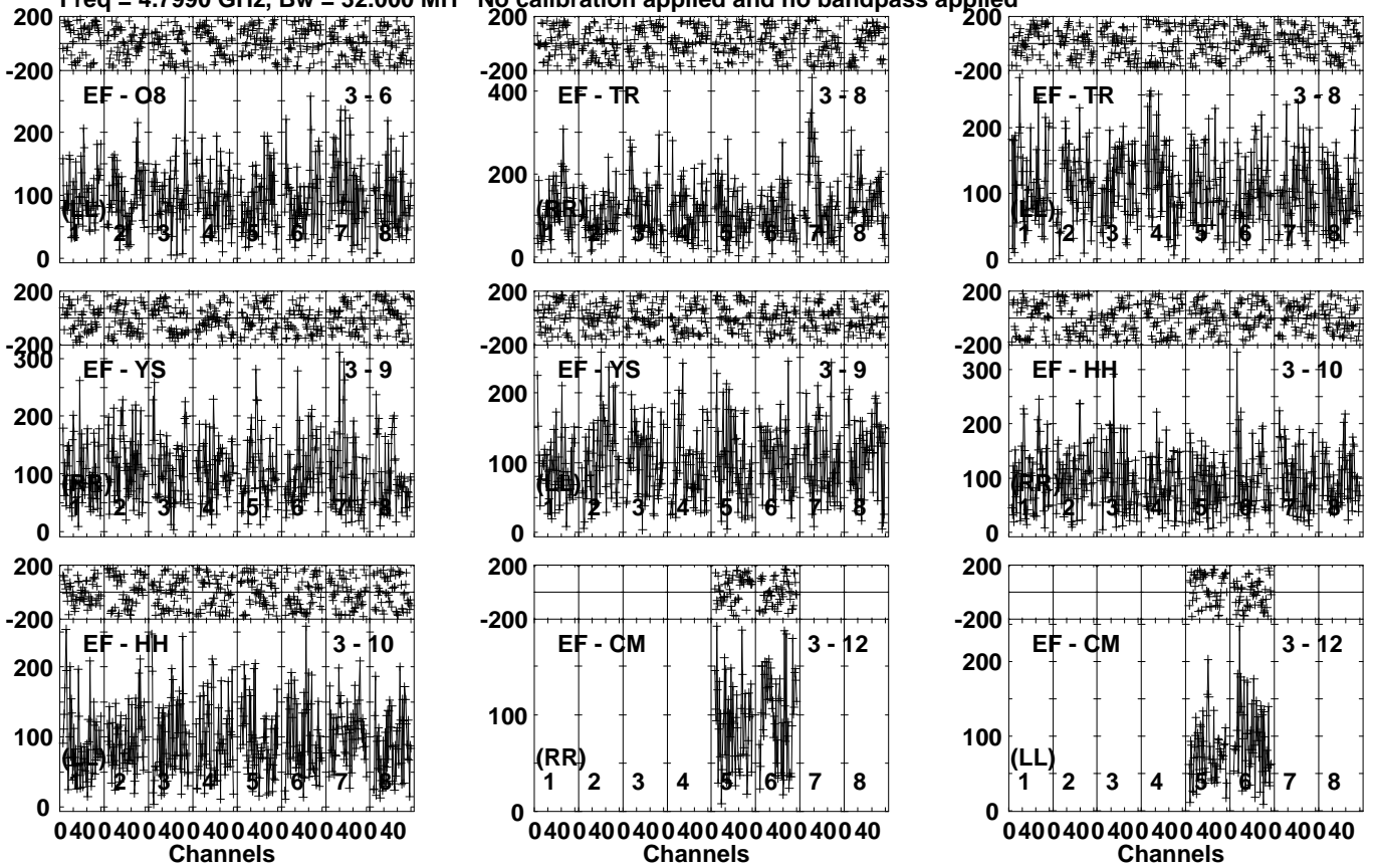
Lower frame: Micro Ampl Jy Top frame: Phas deg Vector averaged cross-power spectrum Several baselines displayed Timerange: 00/12:43:31 to 00/12:46:29
