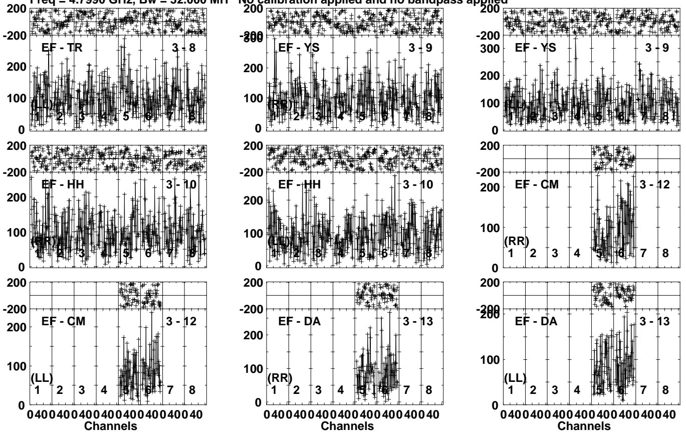
Lower frame: Micro Ampl Jy Top frame: Phas deg Vector averaged cross-power spectrum Several baselines displayed Timerange: 00/05:10:11 to 00/05:13:09
