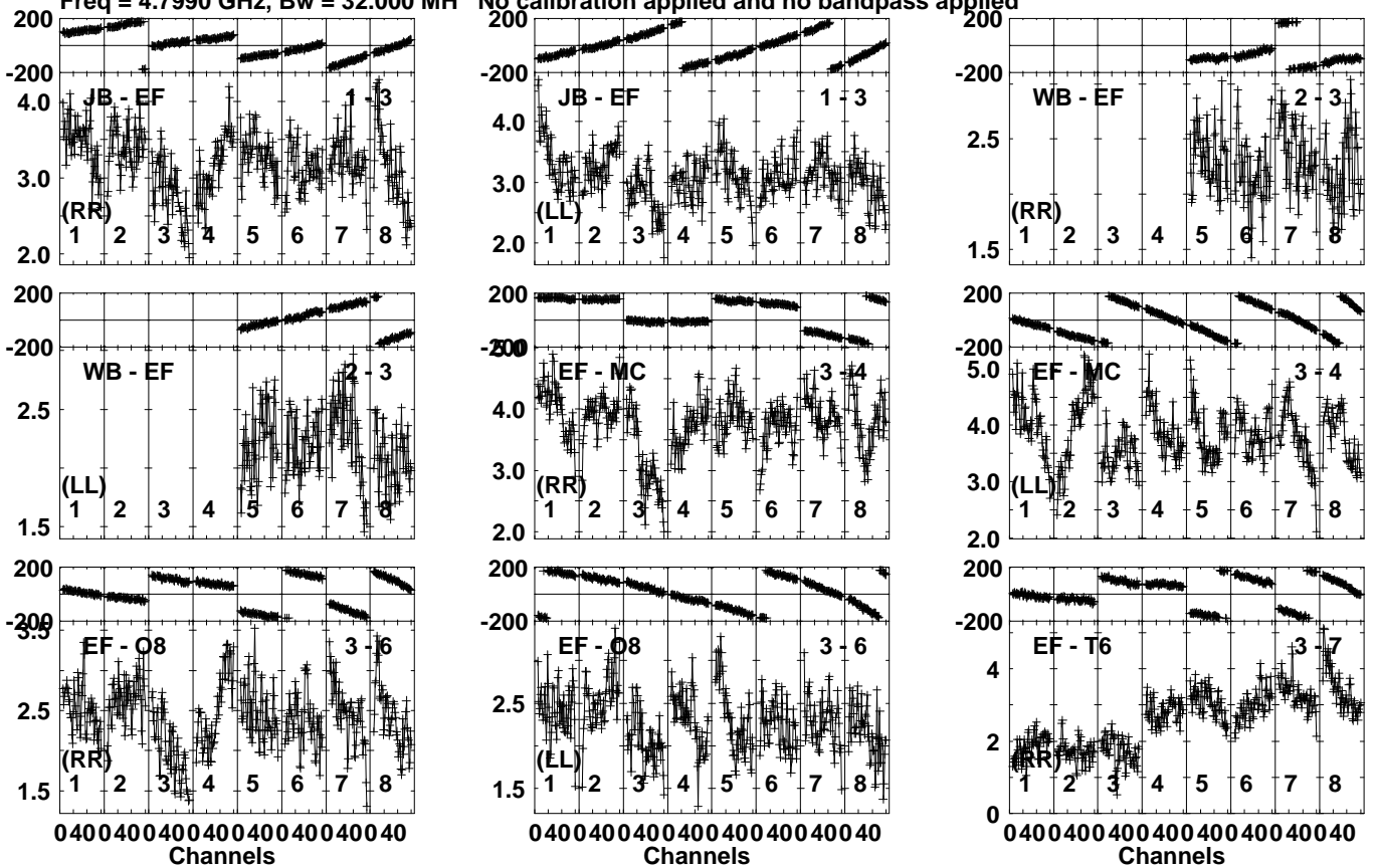
Lower frame: Milli Ampl Jy Top frame: Phas deg Vector averaged cross-power spectrum Several baselines displayed Timerange: 00/08:54:01 to 00/08:55:09
