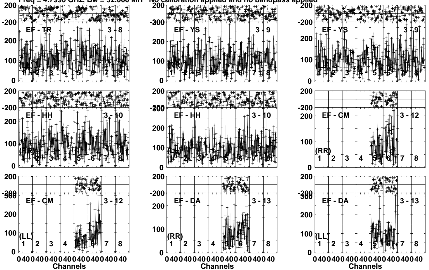
Lower frame: Micro Ampl Jy Top frame: Phas deg Vector averaged cross-power spectrum Several baselines displayed Timerange: 00/05:44:01 to 00/05:46:59
