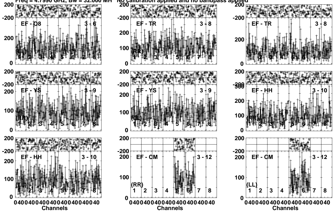
Lower frame: Micro Ampl Jy Top frame: Phas deg Vector averaged cross-power spectrum Several baselines displayed Timerange: 00/13:42:31 to 00/13:45:29
