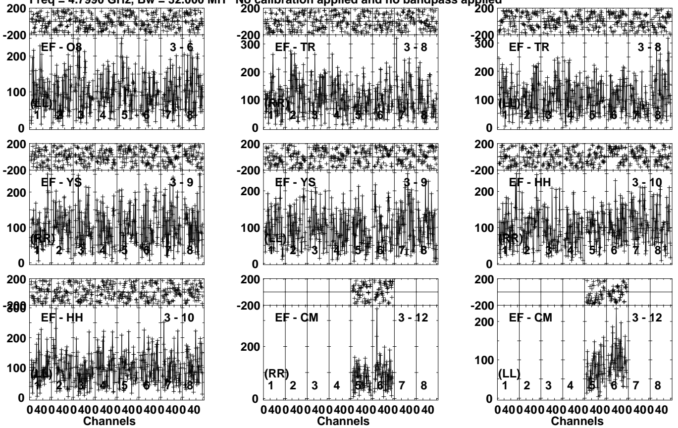
Lower frame: Micro Ampl Jy Top frame: Phas deg Vector averaged cross-power spectrum Several baselines displayed Timerange: 00/12:35:01 to 00/12:37:59
