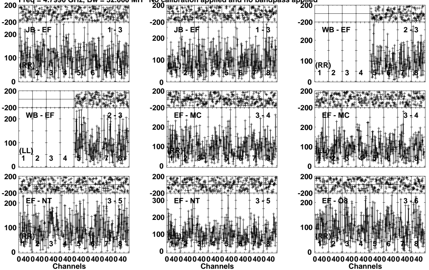
Lower frame: Micro Ampl Jy Top frame: Phas deg Vector averaged cross-power spectrum Several baselines displayed Timerange: 00/08:20:01 to 00/08:22:59
