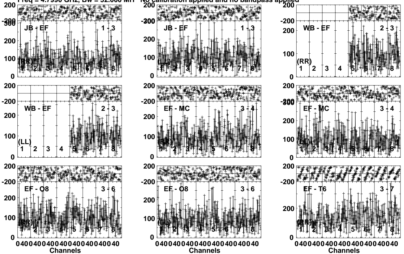
Lower frame: Micro Ampl Jy Top frame: Phas deg Vector averaged cross-power spectrum Several baselines displayed Timerange: 00/05:22:51 to 00/05:25:49
