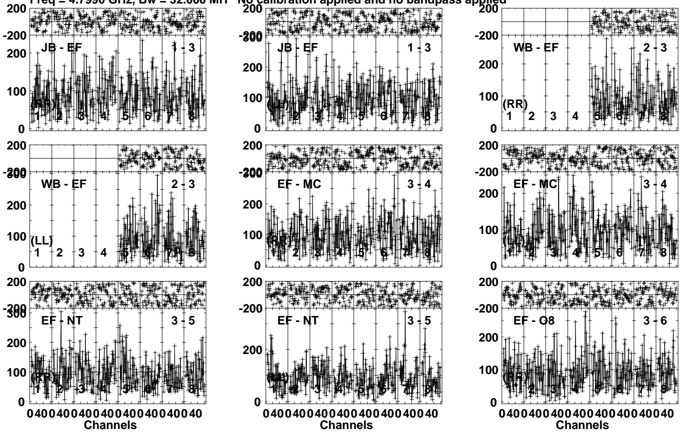
Lower frame: Micro Ampl Jy Top frame: Phas deg Vector averaged cross-power spectrum Several baselines displayed Timerange: 00/06:05:01 to 00/06:07:59
