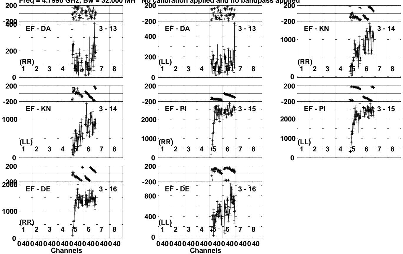
Lower frame: Micro Ampl Jy Top frame: Phas deg Vector averaged cross-power spectrum Several baselines displayed Timerange: 00/13:37:11 to 00/13:38:19
