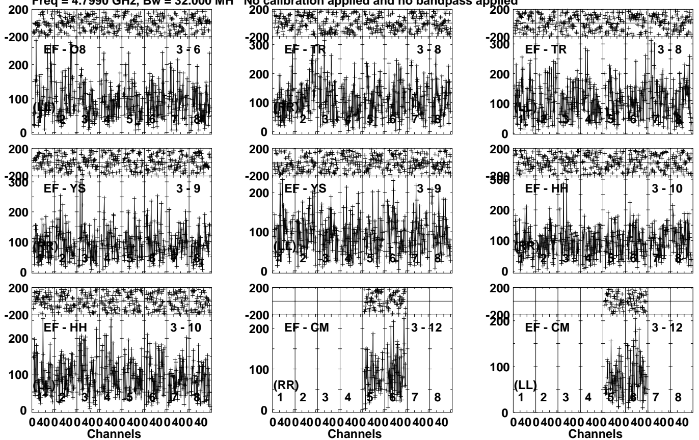
Lower frame: Micro Ampl Jy Top frame: Phas deg Vector averaged cross-power spectrum Several baselines displayed Timerange: 00/12:51:51 to 00/12:54:49
