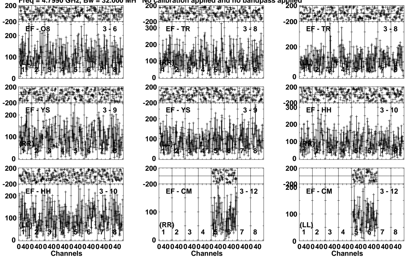
Lower frame: Micro Ampl Jy Top frame: Phas deg Vector averaged cross-power spectrum Several baselines displayed Timerange: 00/13:08:51 to 00/13:11:49
