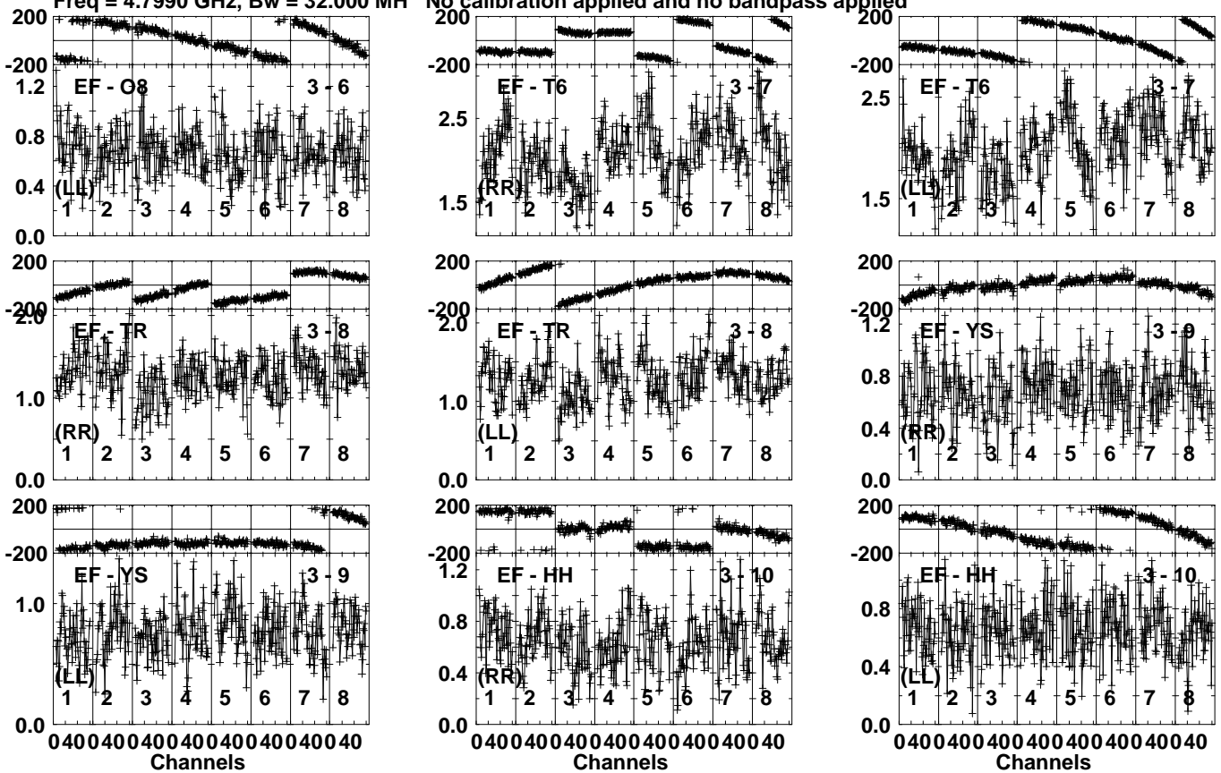
Lower frame: Milli Ampl Jy Top frame: Phas deg Vector averaged cross-power spectrum Several baselines displayed Timerange: 00/07:29:51 to 00/07:30:59
