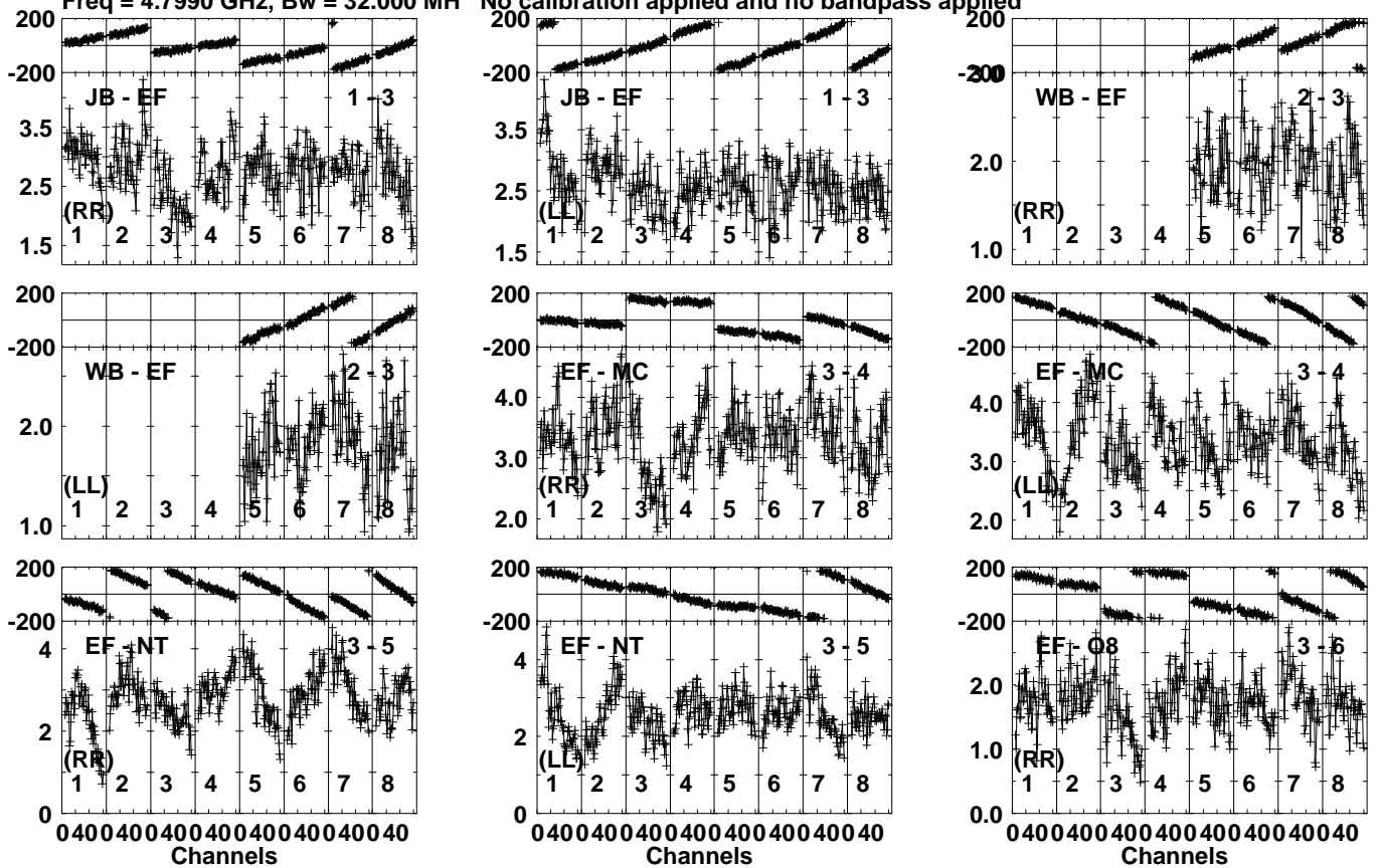
Lower frame: Milli Ampl Jy Top frame: Phas deg Vector averaged cross-power spectrum Several baselines displayed Timerange: 00/12:21:11 to 00/12:22:19
