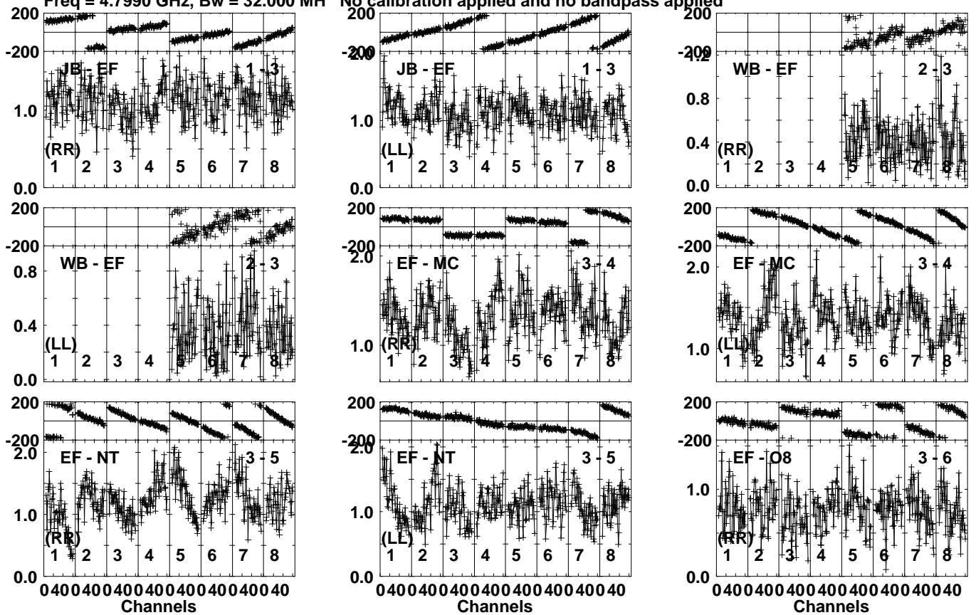
Lower frame: Milli Ampl Jy Top frame: Phas deg Vector averaged cross-power spectrum Several baselines displayed Timerange: 00/08:00:41 to 00/08:01:49
