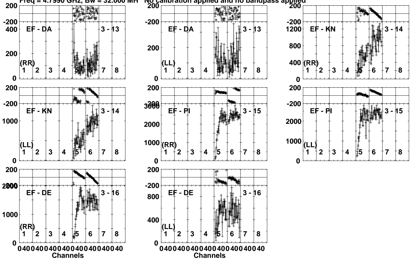
Lower frame: Micro Ampl Jy Top frame: Phas deg Vector averaged cross-power spectrum Several baselines displayed Timerange: 00/13:16:01 to 00/13:17:09
