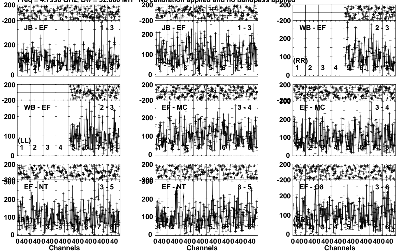
Lower frame: Micro Ampl Jy Top frame: Phas deg Vector averaged cross-power spectrum Several baselines displayed Timerange: 00/12:13:51 to 00/12:16:49
