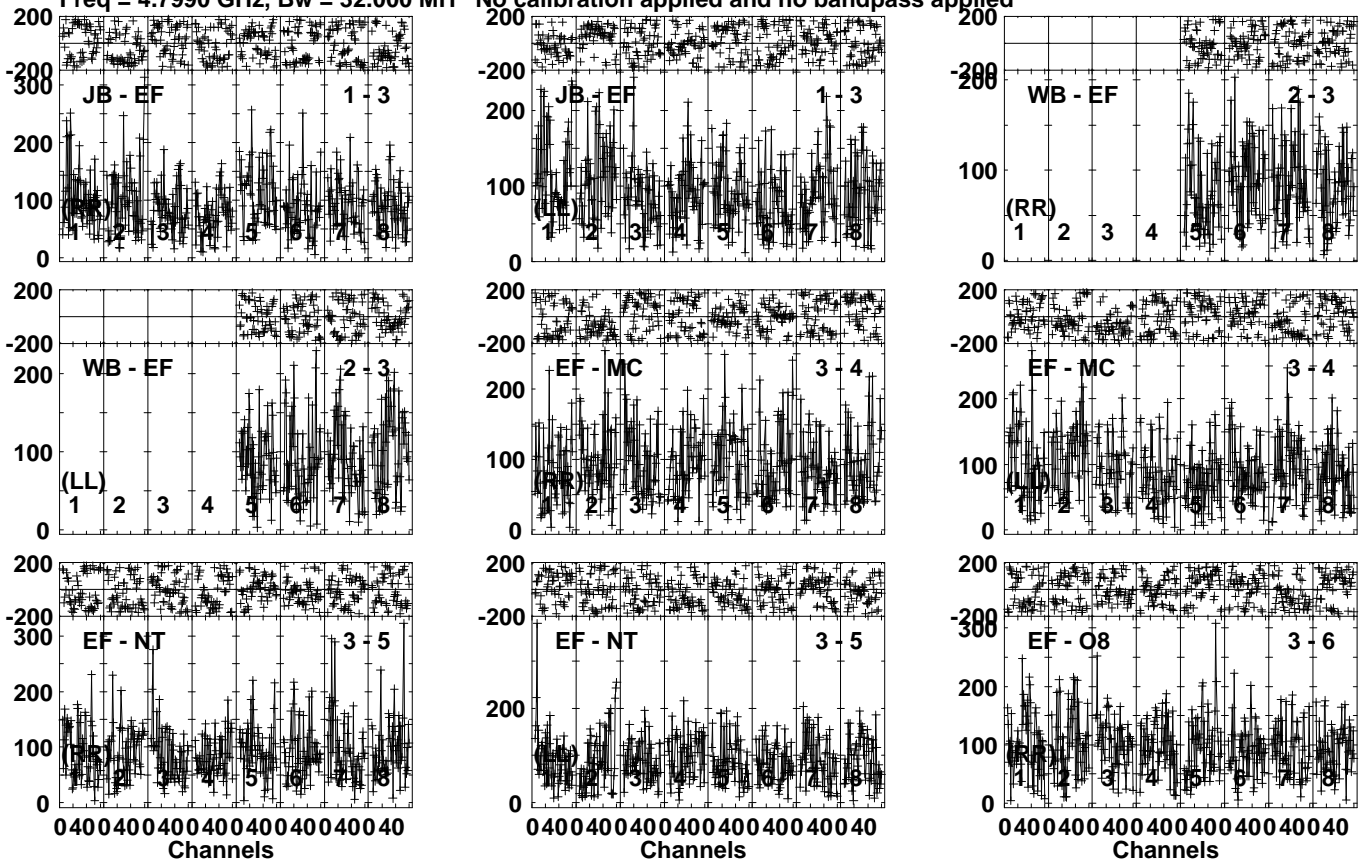
Lower frame: Micro Ampl Jy Top frame: Phas deg Vector averaged cross-power spectrum Several baselines displayed Timerange: 00/06:00:51 to 00/06:03:49
