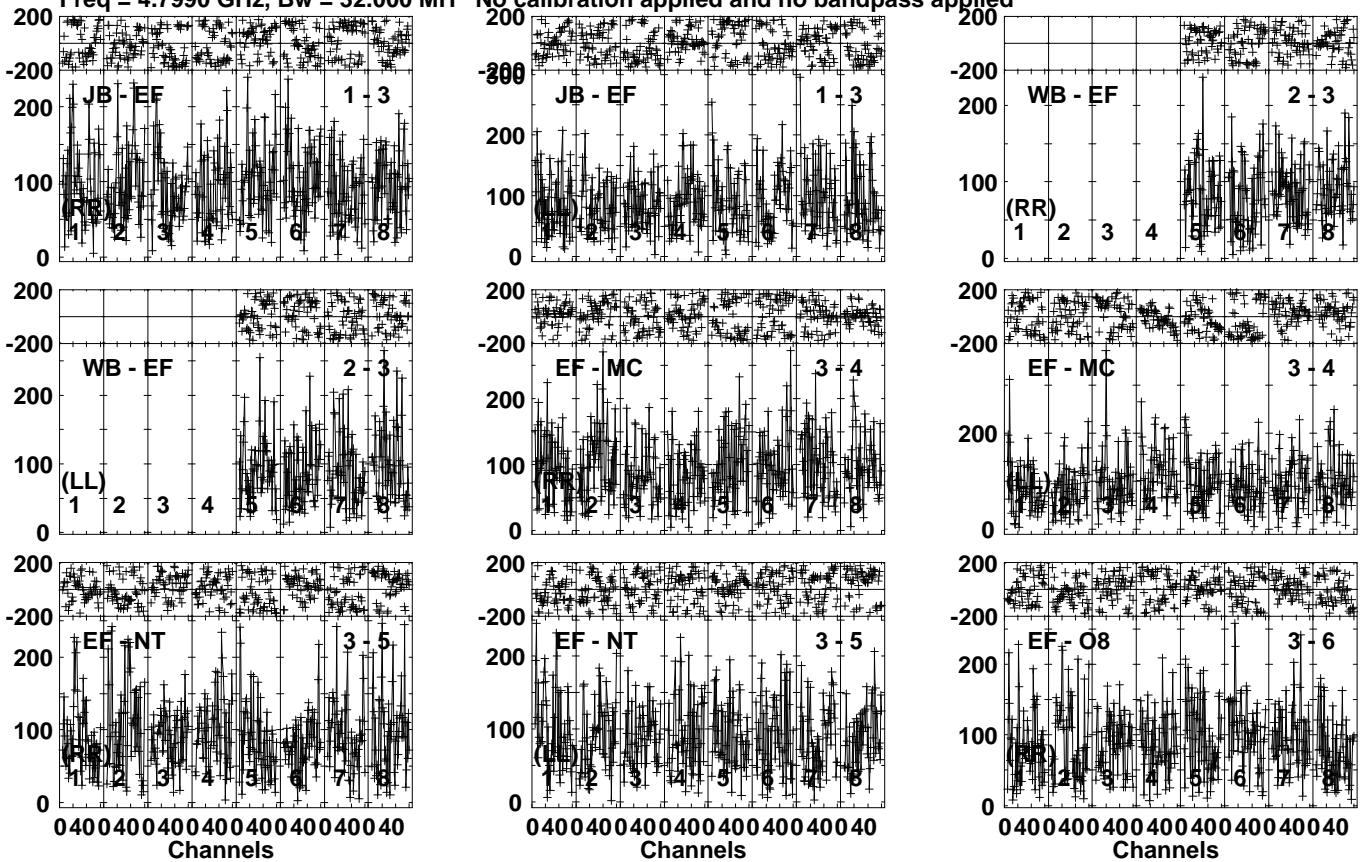
Lower frame: Micro Ampl Jy Top frame: Phas deg Vector averaged cross-power spectrum Several baselines displayed Timerange: 00/06:09:21 to 00/06:12:19
