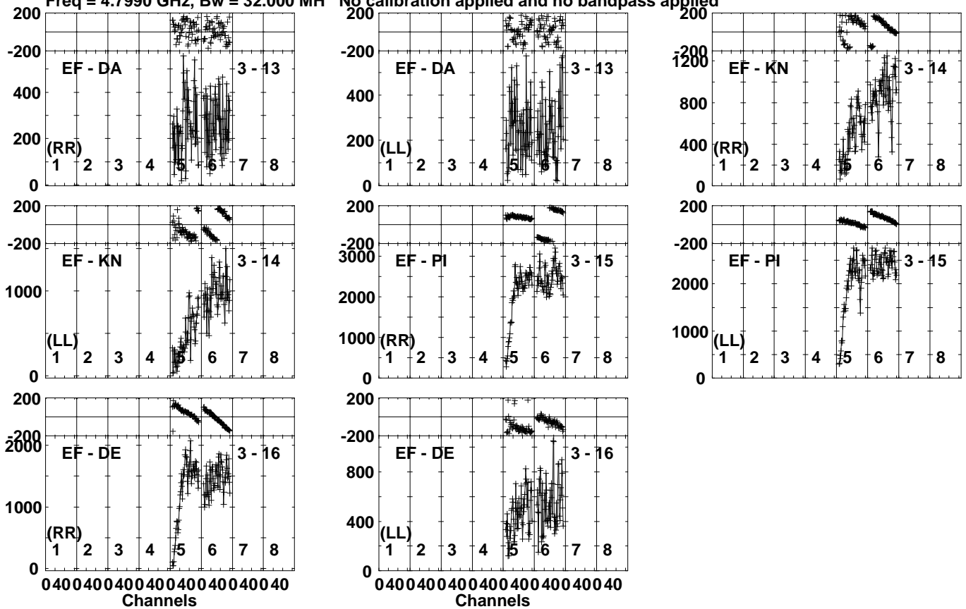
Lower frame: Micro Ampl Jy Top frame: Phas deg Vector averaged cross-power spectrum Several baselines displayed Timerange: 00/12:50:41 to 00/12:51:49
