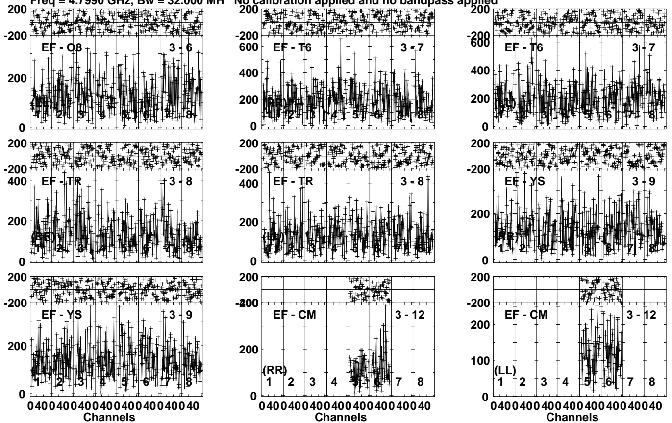
Lower frame: Micro Ampl Jy Top frame: Phas deg Vector averaged cross-power spectrum Several baselines displayed Timerange: 00/08:24:21 to 00/08:26:19
