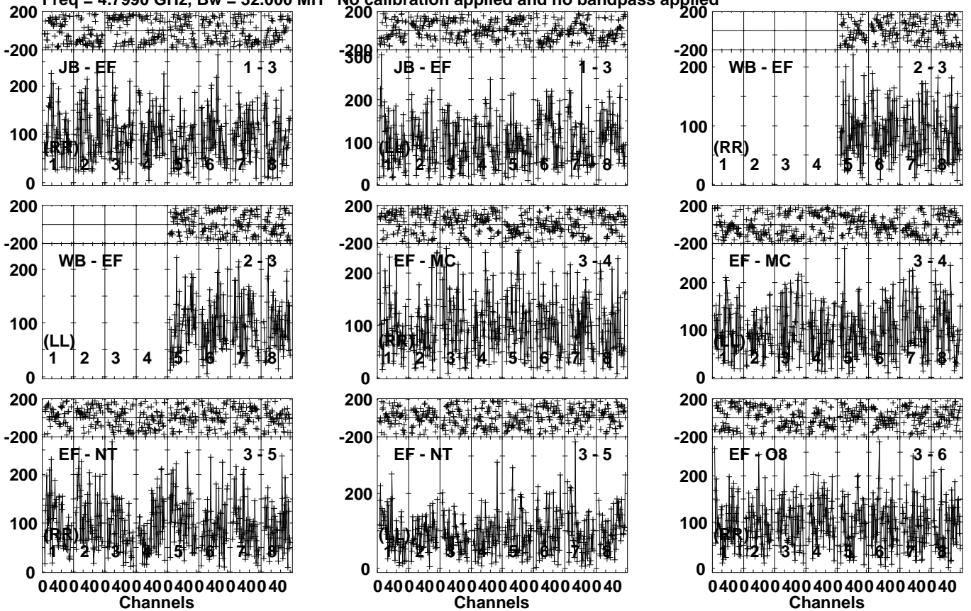
Lower frame: Micro Ampl Jy Top frame: Phas deg Vector averaged cross-power spectrum Several baselines displayed Timerange: 00/07:31:01 to 00/07:33:59
