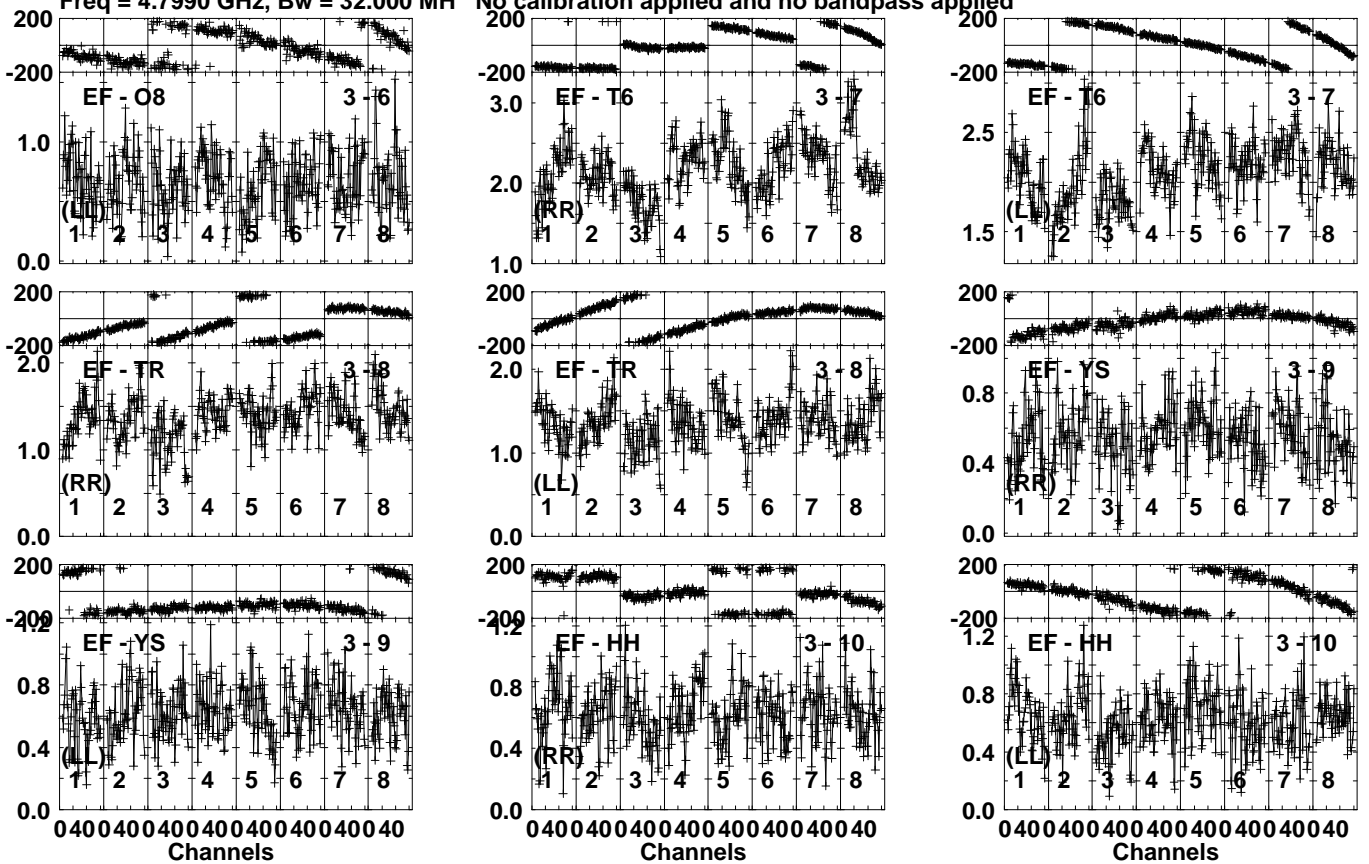
Lower frame: Milli Ampl Jy Top frame: Phas deg Vector averaged cross-power spectrum Several baselines displayed Timerange: 00/06:03:51 to 00/06:04:59
