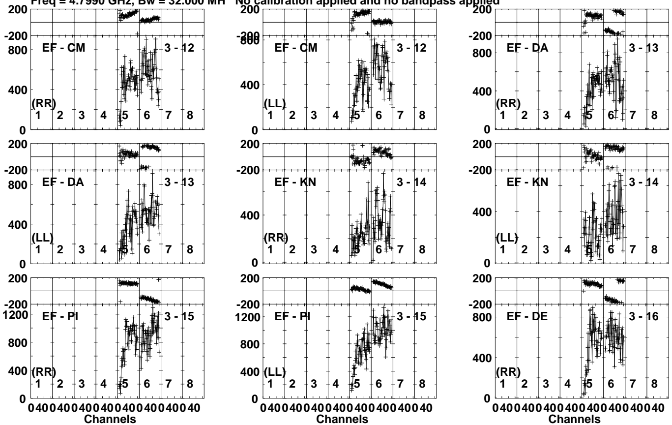
Lower frame: Micro Ampl Jy Top frame: Phas deg Vector averaged cross-power spectrum Several baselines displayed Timerange: 00/07:34:31 to 00/07:35:19
