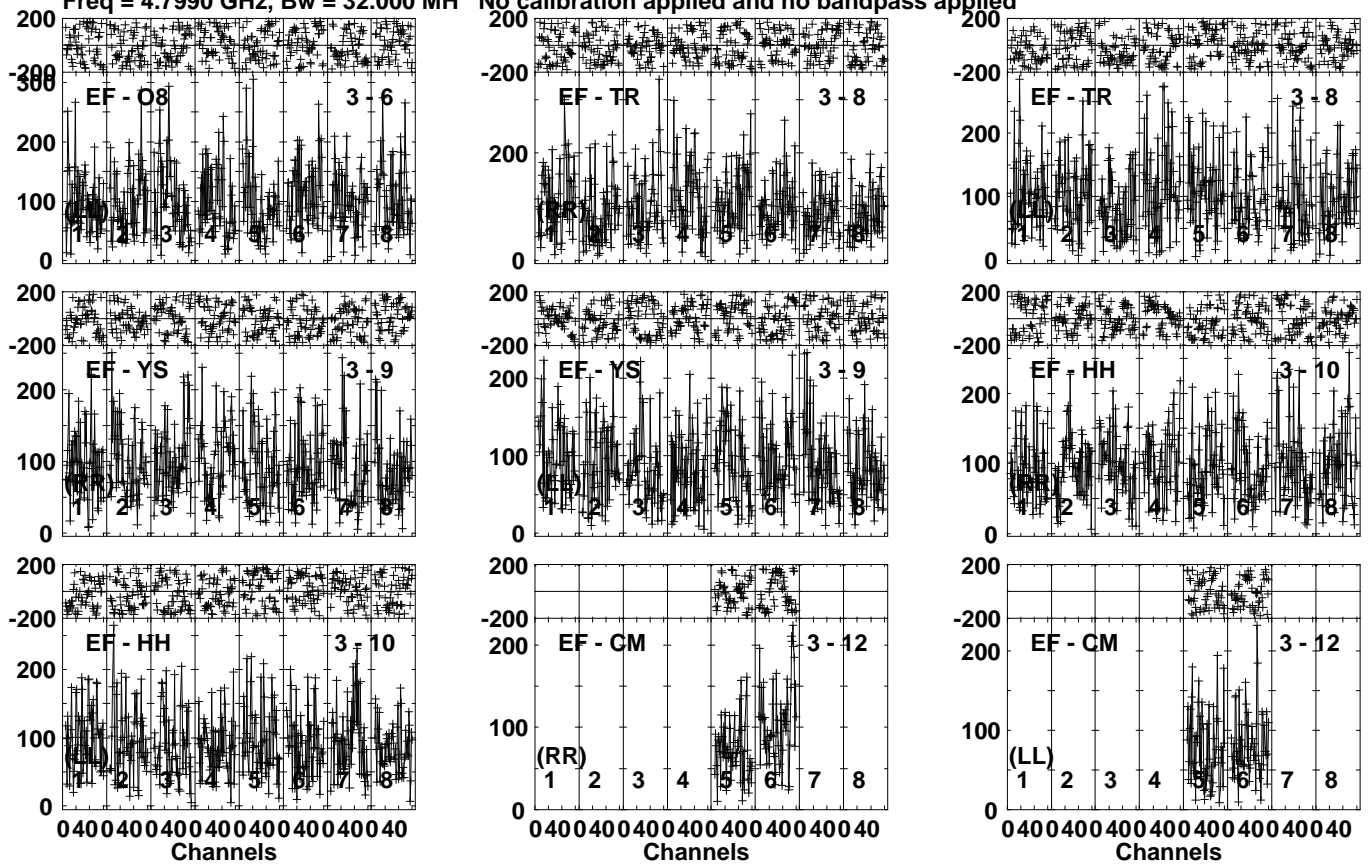
Lower frame: Micro Ampl Jy Top frame: Phas deg Vector averaged cross-power spectrum Several baselines displayed Timerange: 00/13:21:31 to 00/13:24:29
