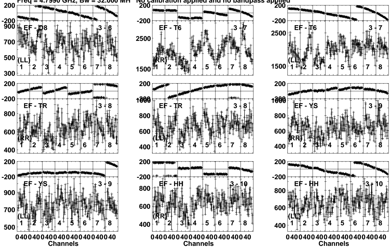
Lower frame: Micro Ampl Jy Top frame: Phas deg Vector averaged cross-power spectrum Several baselines displayed Timerange: 00/07:24:51 to 00/07:26:49
