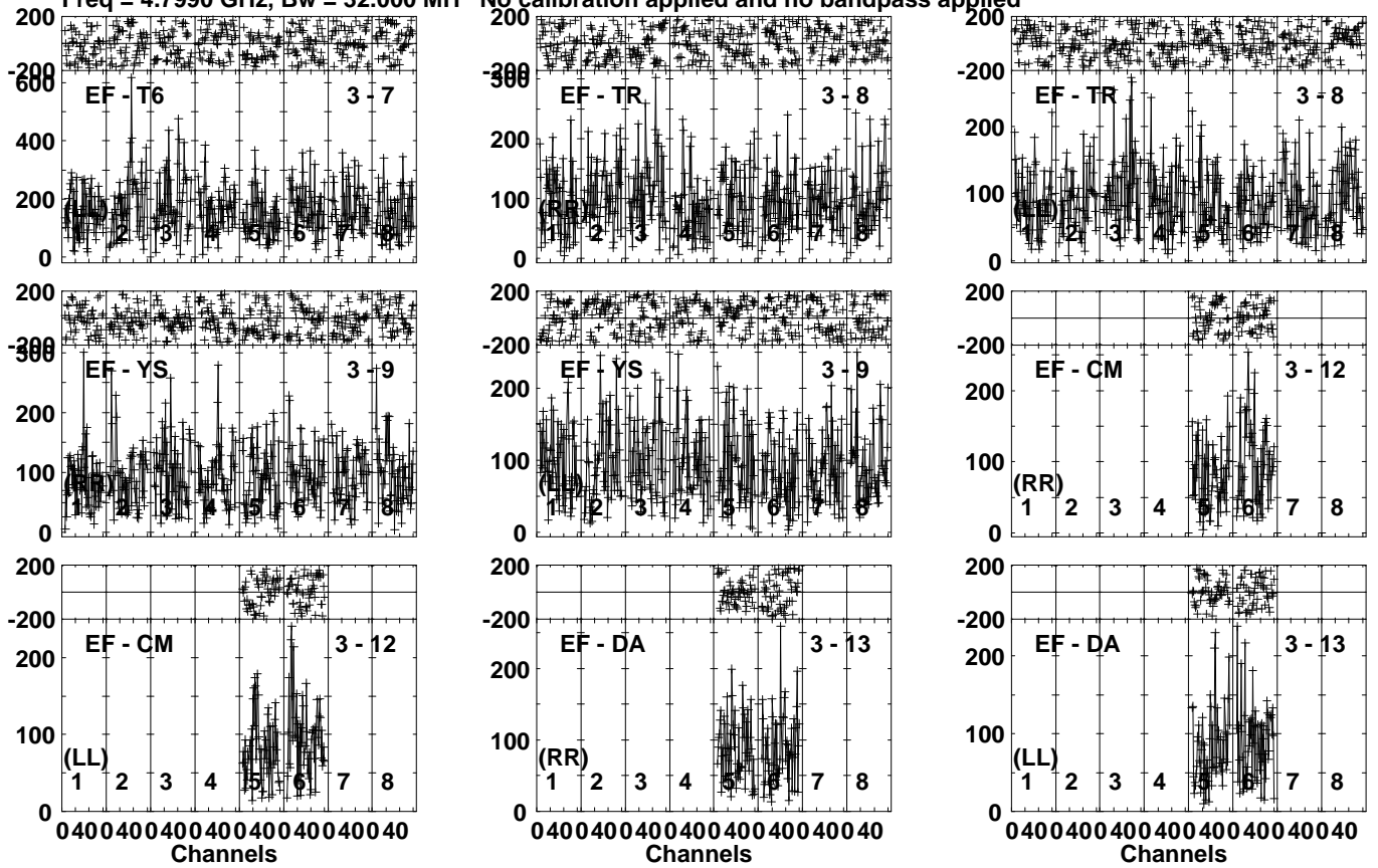
Lower frame: Micro Ampl Jy Top frame: Phas deg Vector averaged cross-power spectrum Several baselines displayed Timerange: 00/07:17:41 to 00/07:20:39
