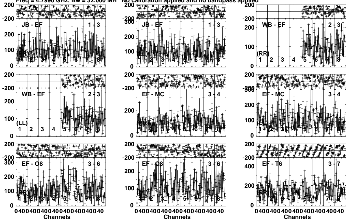
Lower frame: Micro Ampl Jy Top frame: Phas deg Vector averaged cross-power spectrum Several baselines displayed Timerange: 00/05:14:21 to 00/05:17:19
