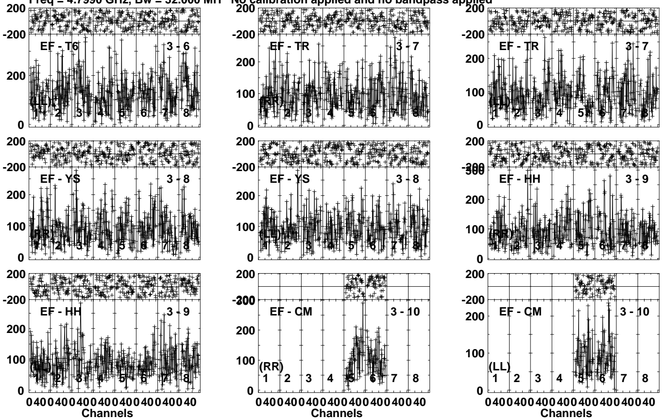
Lower frame: Micro Ampl Jy Top frame: Phas deg Vector averaged cross-power spectrum Several baselines displayed Timerange: 01/02:54:11 to 01/02:57:09
