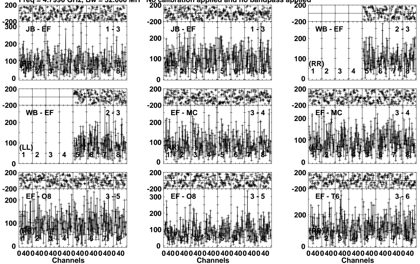
Lower frame: Micro Ampl Jy Top frame: Phas deg Vector averaged cross-power spectrum Several baselines displayed Timerange: 01/02:20:51 to 01/02:23:49
