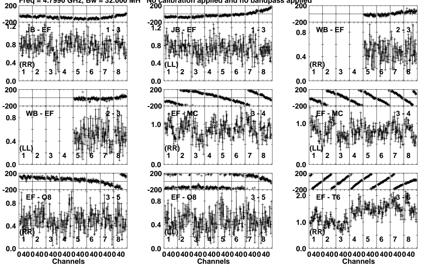
Lower frame: Milli Ampl Jy Top frame: Phas deg Vector averaged cross-power spectrum Several baselines displayed Timerange: 01/00:39:11 to 01/00:39:59
