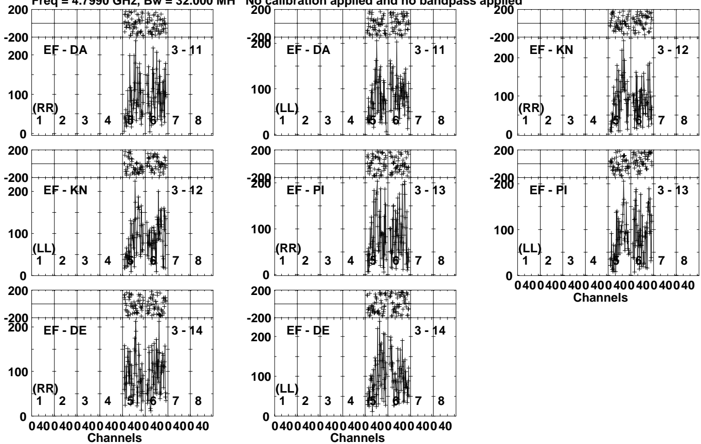
Lower frame: Micro Ampl Jy Top frame: Phas deg Vector averaged cross-power spectrum Several baselines displayed Timerange: 01/01:22:31 to 01/01:25:29
