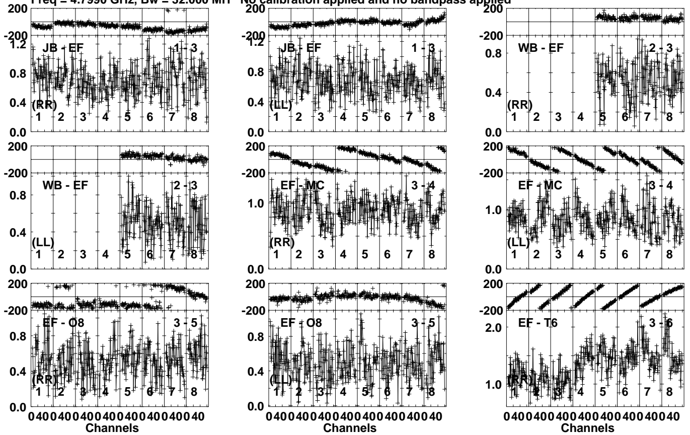
Lower frame: Milli Ampl Jy Top frame: Phas deg Vector averaged cross-power spectrum Several baselines displayed Timerange: 01/01:08:11 to 01/01:08:59
