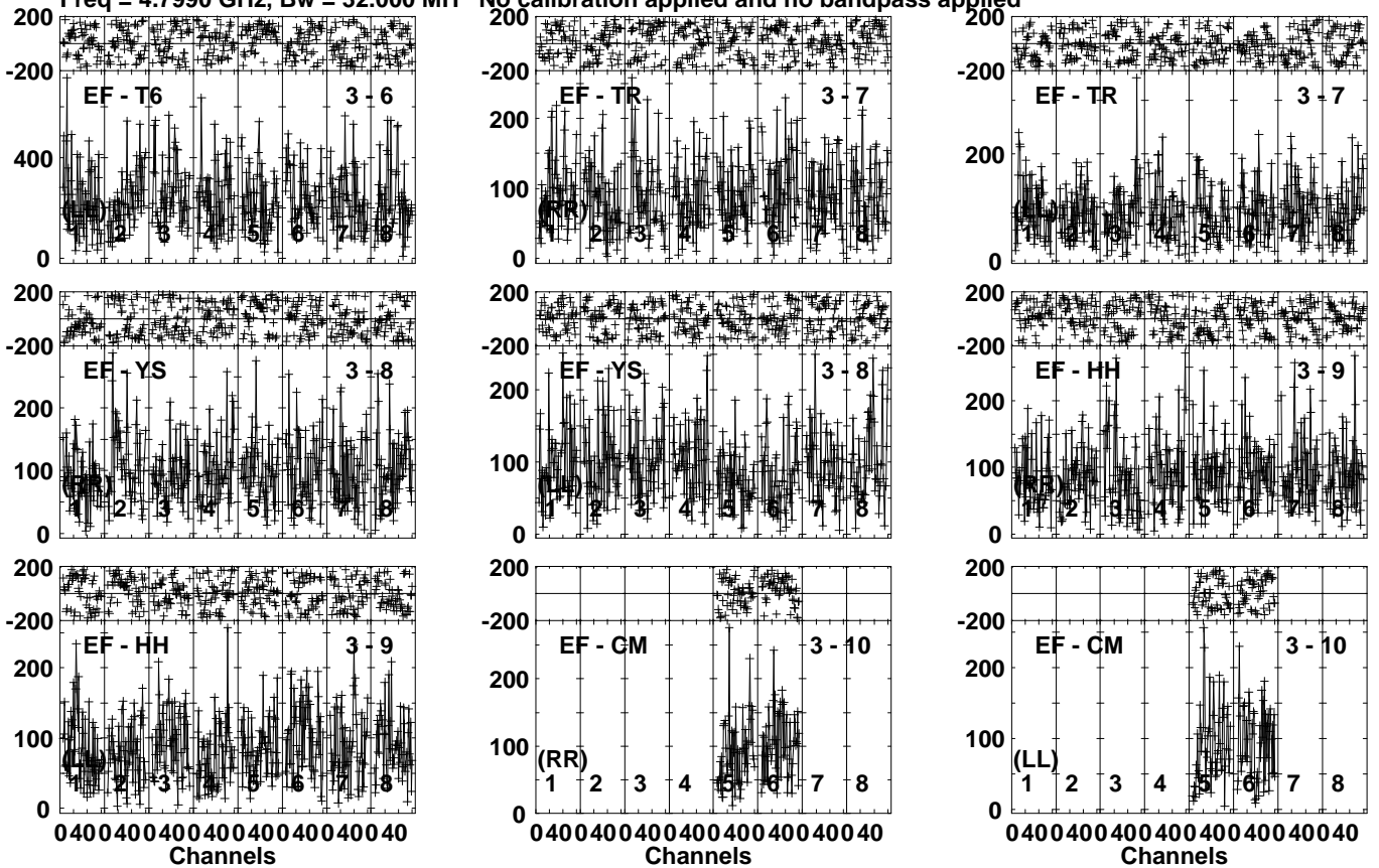
Lower frame: Micro Ampl Jy Top frame: Phas deg Vector averaged cross-power spectrum Several baselines displayed Timerange: 01/02:00:01 to 01/02:02:59
