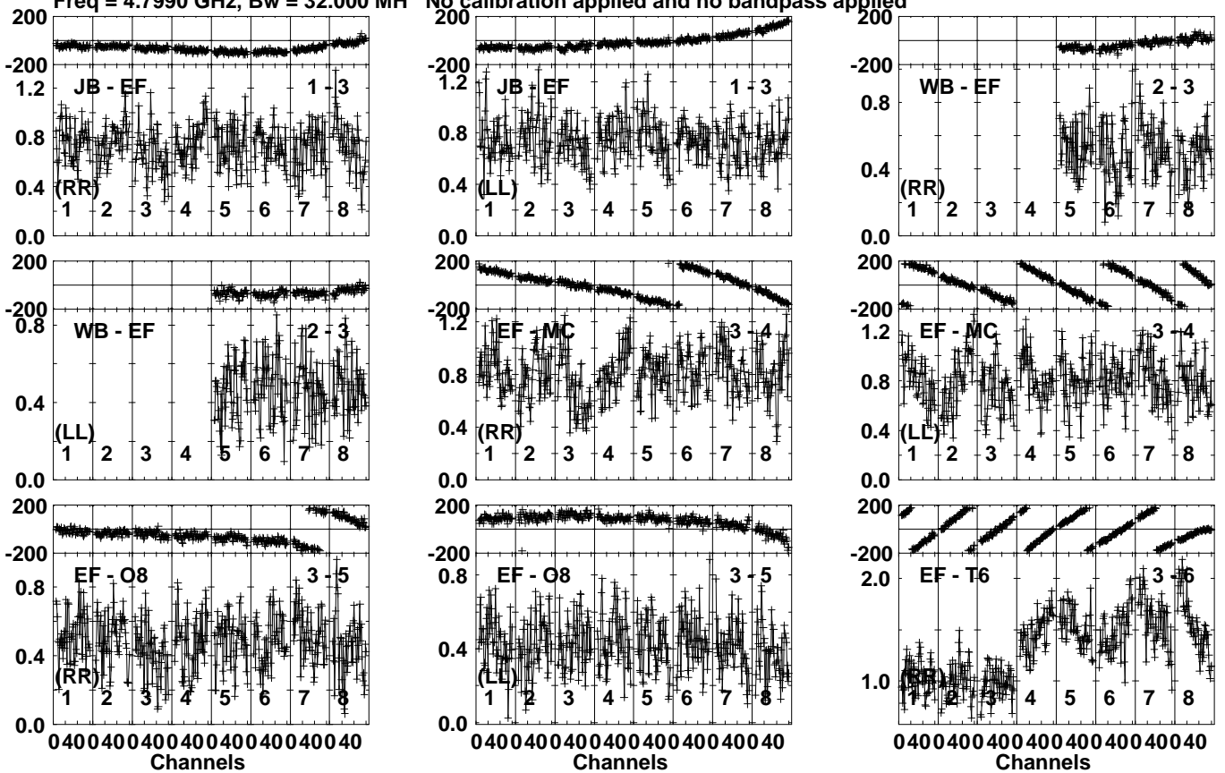
Lower frame: Milli Ampl Jy Top frame: Phas deg Vector averaged cross-power spectrum Several baselines displayed Timerange: 01/00:10:01 to 01/00:10:49
