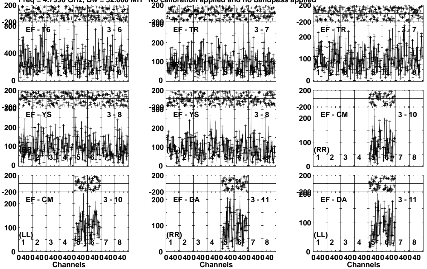
Lower frame: Micro Ampl Jy Top frame: Phas deg Vector averaged cross-power spectrum Several baselines displayed Timerange: 01/00:23:21 to 01/00:26:19
