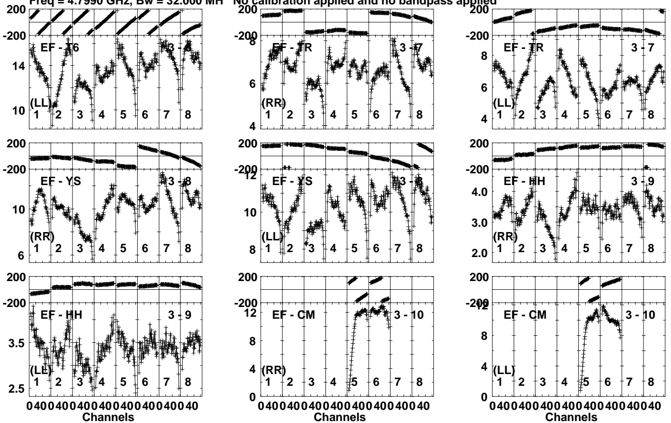
Lower frame: Milli Ampl Jy Top frame: Phas deg Vector averaged cross-power spectrum Several baselines displayed Timerange: 01/02:58:11 to 01/02:59:59
