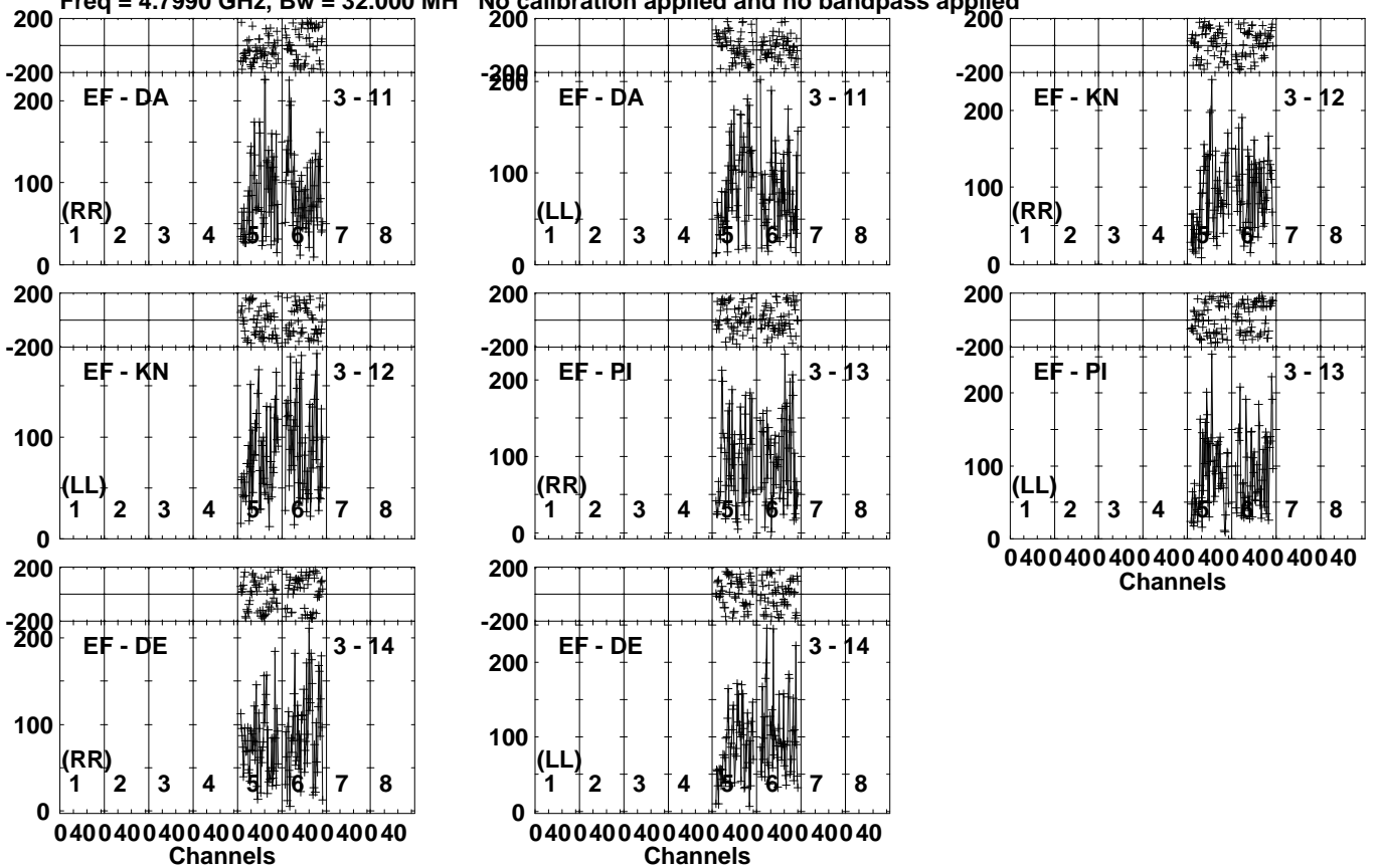
Lower frame: Micro Ampl Jy Top frame: Phas deg Vector averaged cross-power spectrum Several baselines displayed Timerange: 01/01:35:01 to 01/01:37:59
