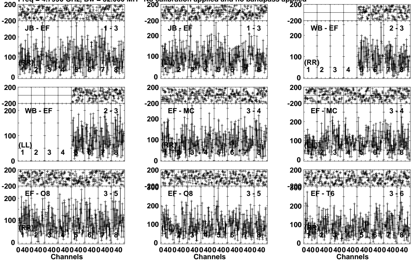
Lower frame: Micro Ampl Jy Top frame: Phas deg Vector averaged cross-power spectrum Several baselines displayed Timerange: 01/00:02:31 to 01/00:05:29
