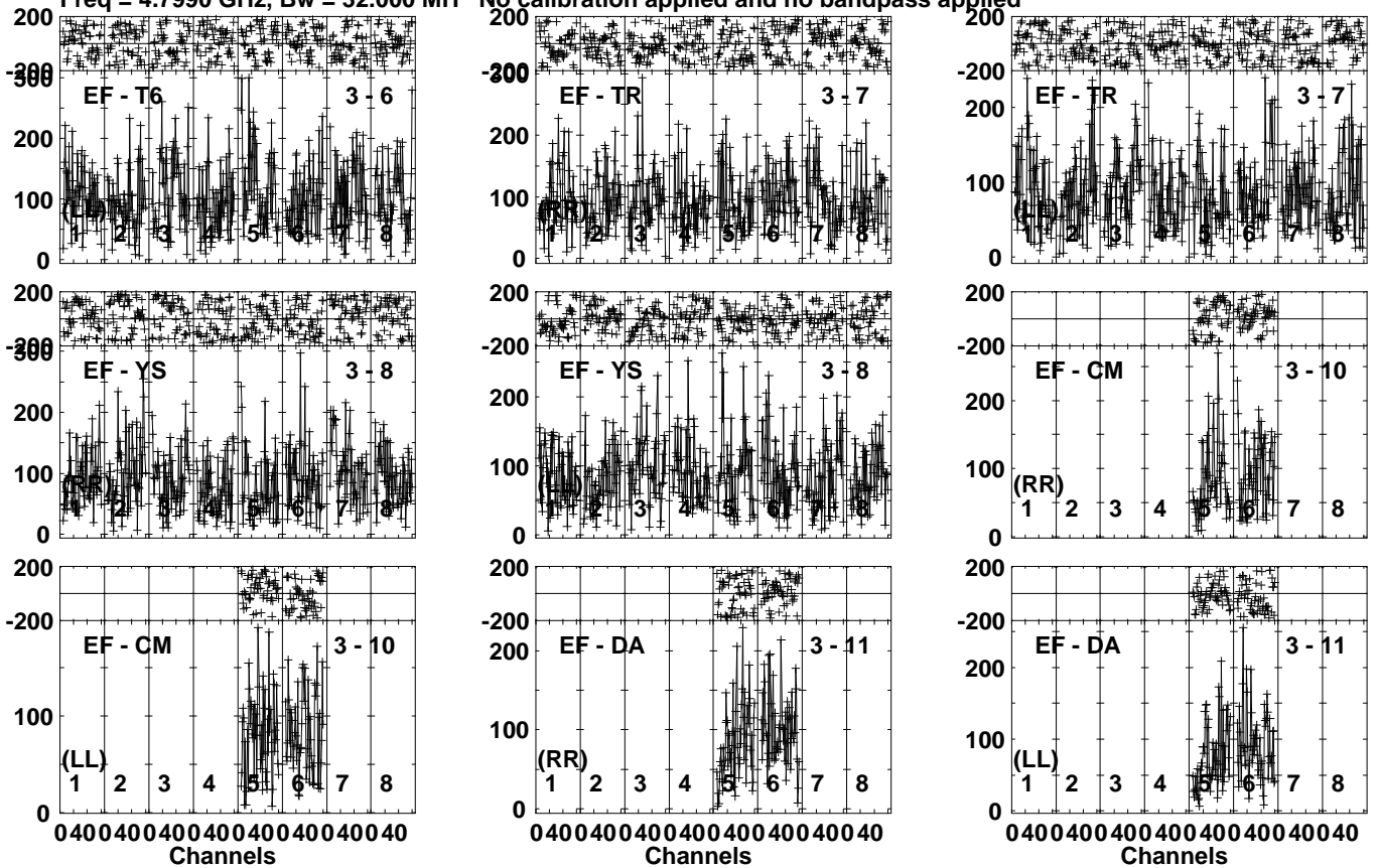
Lower frame: Micro Ampl Jy Top frame: Phas deg Vector averaged cross-power spectrum Several baselines displayed Timerange: 01/00:35:51 to 01/00:38:49
