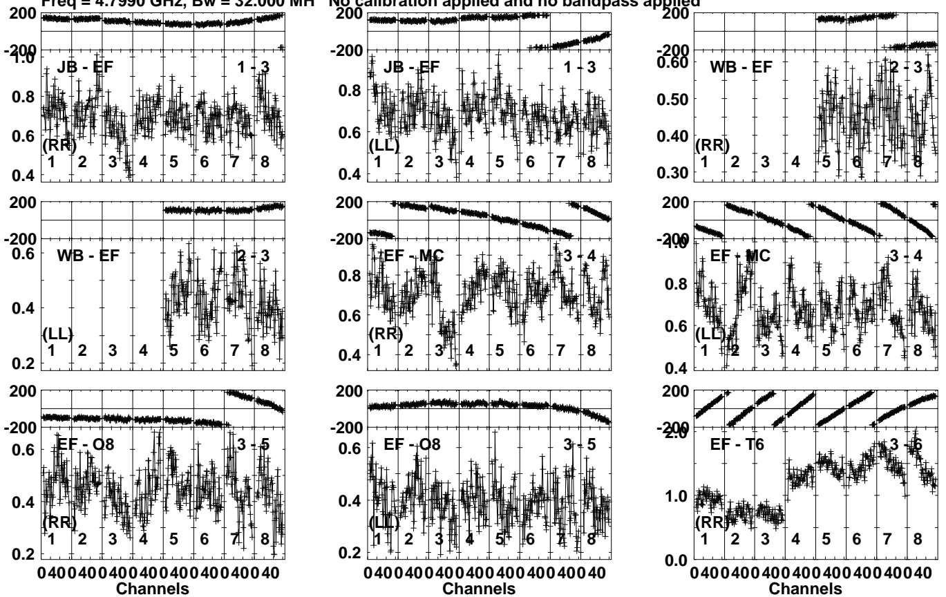
Lower frame: Milli Ampl Jy Top frame: Phas deg Vector averaged cross-power spectrum Several baselines displayed Timerange: 00/23:00:07 to 00/23:02:59
