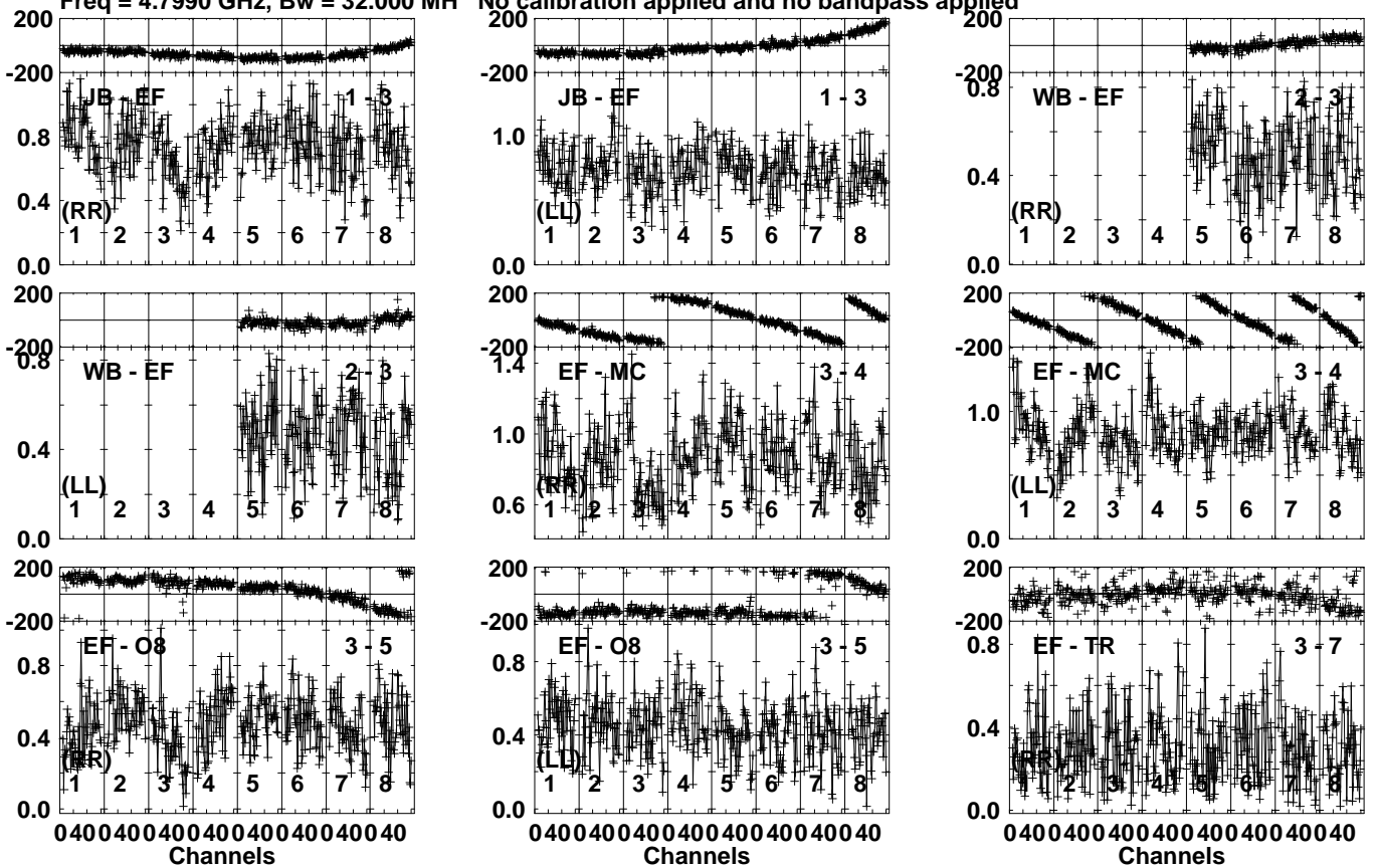
Lower frame: Milli Ampl Jy Top frame: Phas deg Vector averaged cross-power spectrum Several baselines displayed Timerange: 01/00:35:01 to 01/00:35:49
