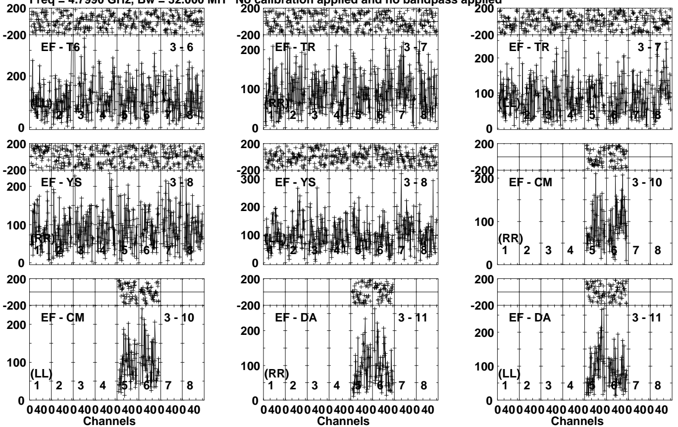
Lower frame: Micro Ampl Jy Top frame: Phas deg Vector averaged cross-power spectrum Several baselines displayed Timerange: 01/00:06:41 to 01/00:09:39
