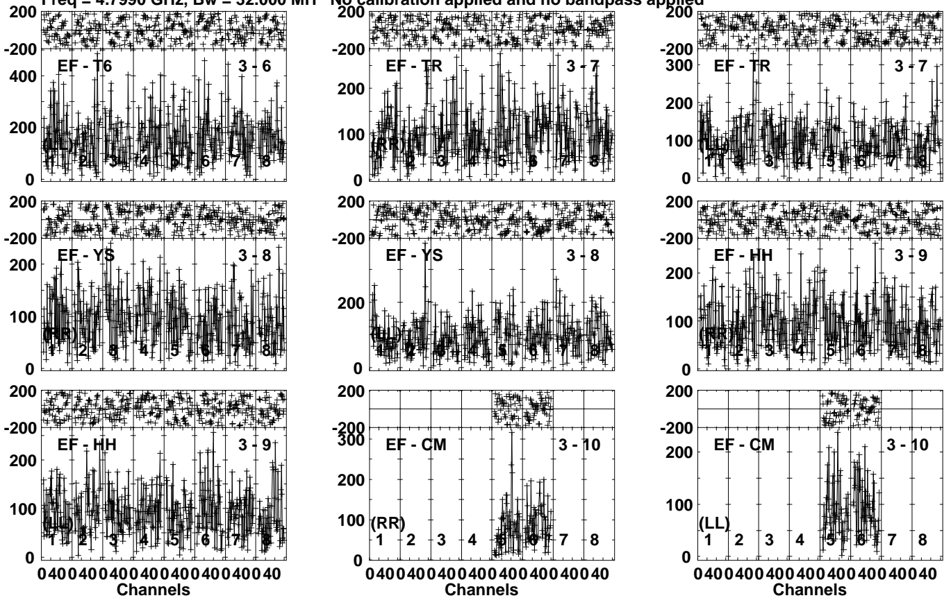
Lower frame: Micro Ampl Jy Top frame: Phas deg Vector averaged cross-power spectrum Several baselines displayed Timerange: 01/01:55:51 to 01/01:58:49
