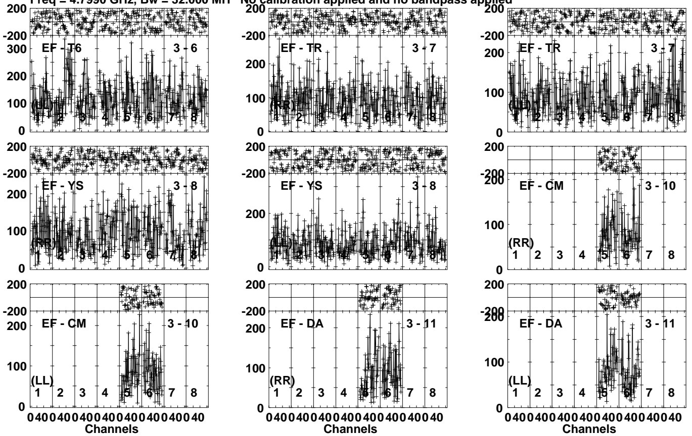
Lower frame: Micro Ampl Jy Top frame: Phas deg Vector averaged cross-power spectrum Several baselines displayed Timerange: 00/23:41:41 to 00/23:44:39
