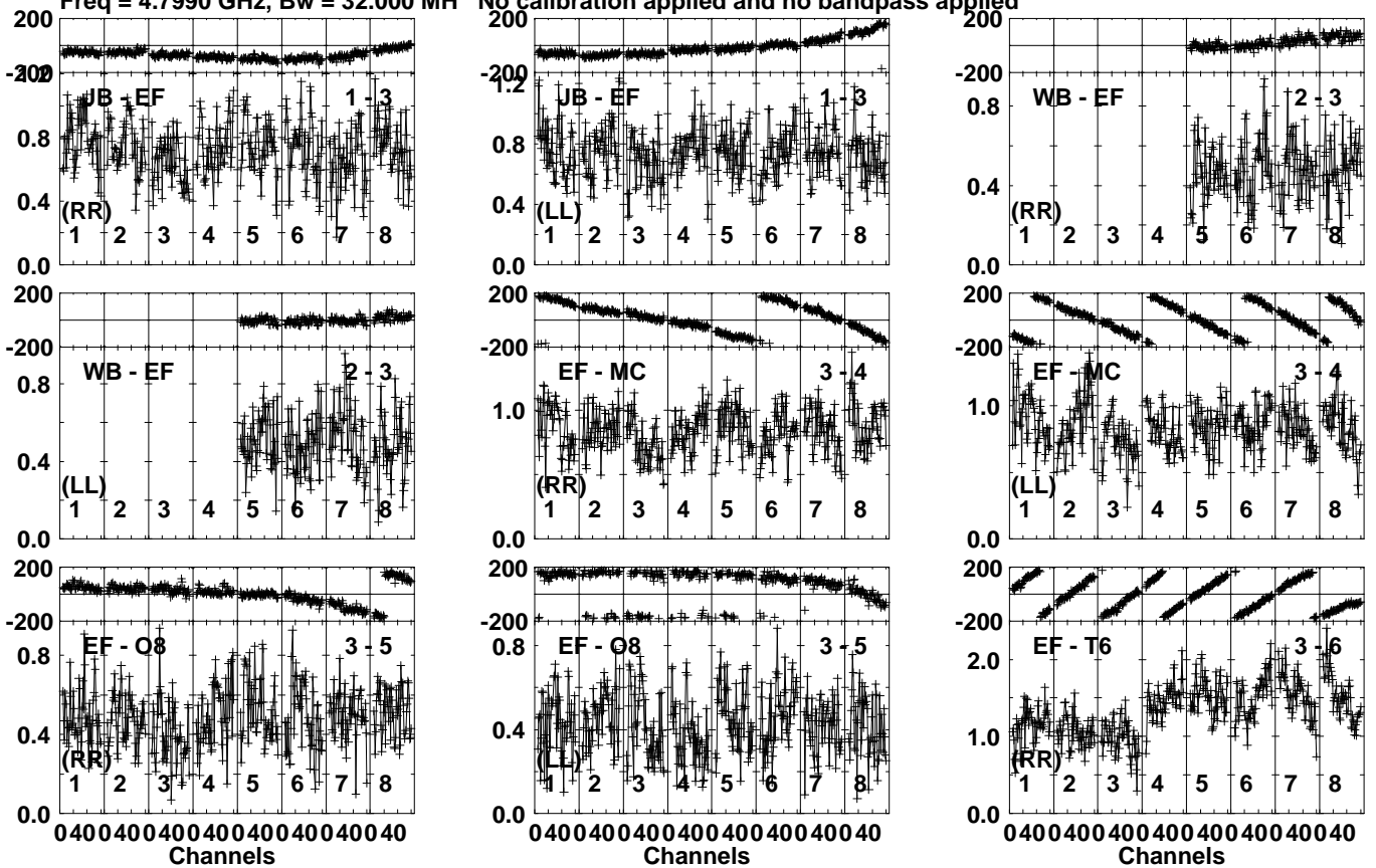
Lower frame: Milli Ampl Jy Top frame: Phas deg Vector averaged cross-power spectrum Several baselines displayed Timerange: 01/00:43:21 to 01/00:44:09
