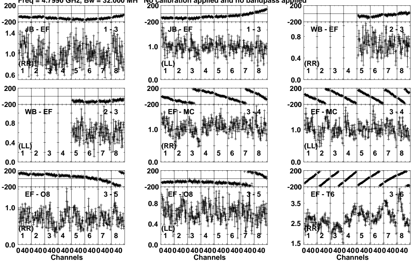
Lower frame: Milli Ampl Jy Top frame: Phas deg Vector averaged cross-power spectrum Several baselines displayed Timerange: 01/01:50:51 to 01/01:51:39
