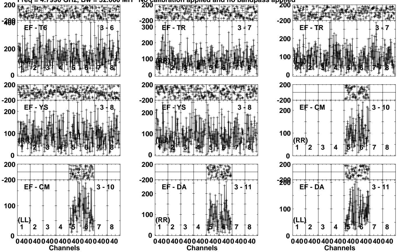
Lower frame: Micro Ampl Jy Top frame: Phas deg Vector averaged cross-power spectrum Several baselines displayed Timerange: 00/23:25:01 to 00/23:27:59
