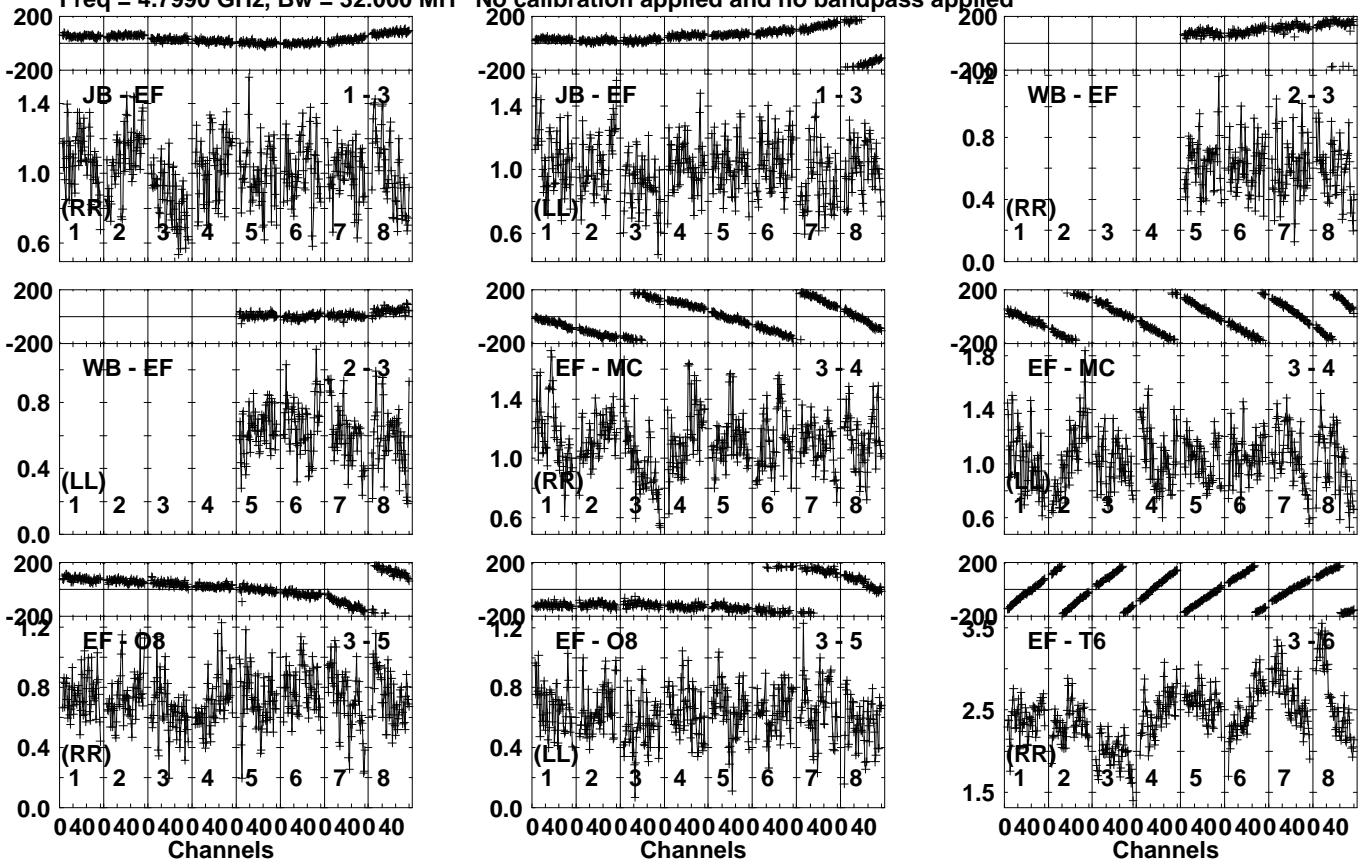
Lower frame: Milli Ampl Jy Top frame: Phas deg Vector averaged cross-power spectrum Several baselines displayed Timerange: 01/02:24:11 to 01/02:24:59
