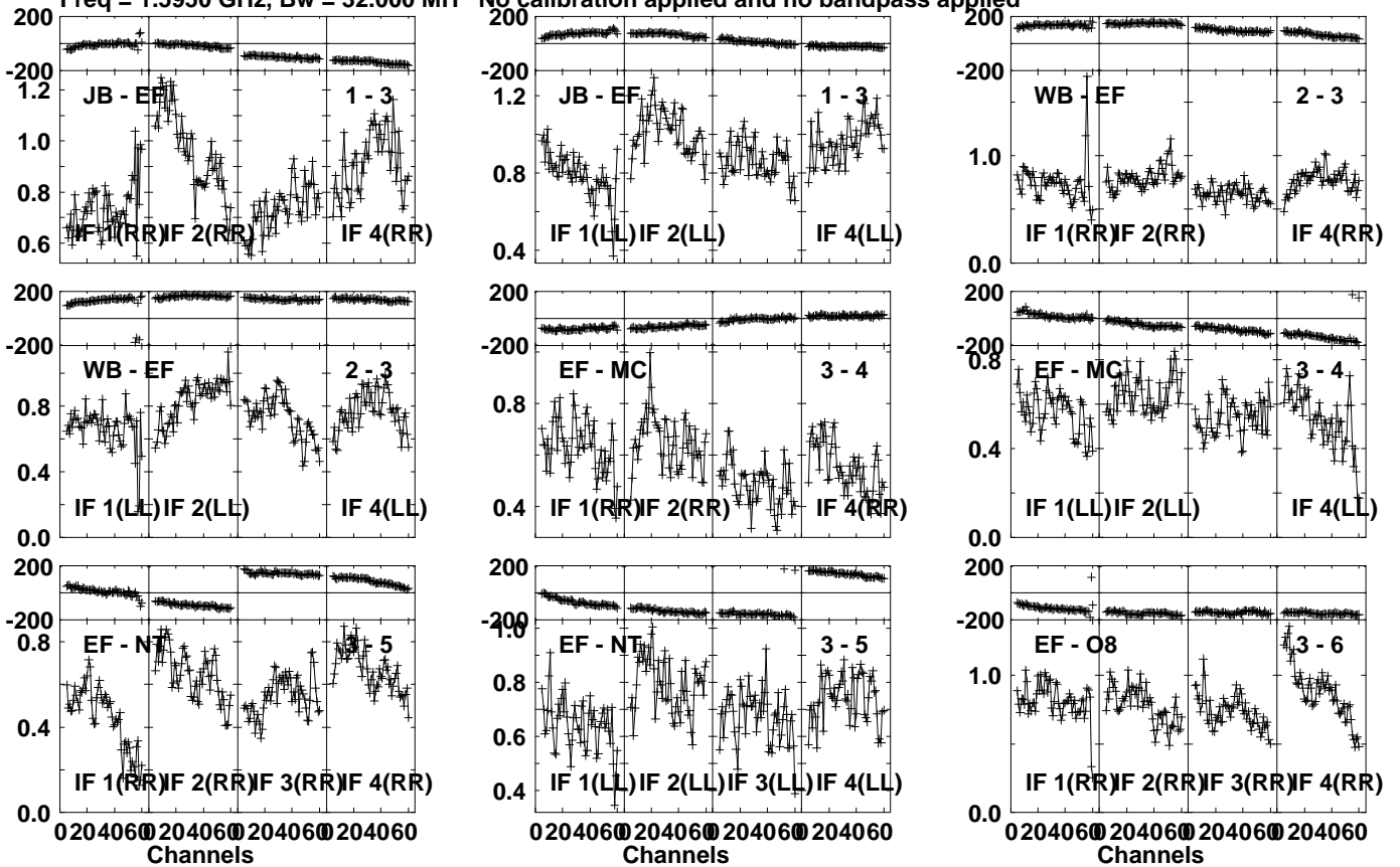
Lower frame: Milli Ampl Jy Top frame: Phas deg Vector averaged cross-power spectrum Several baselines displayed Timerange: 00/17:26:11 to 00/17:28:09
