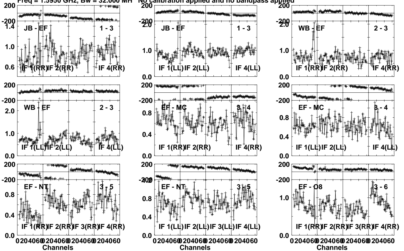
Lower frame: Milli Ampl Jy Top frame: Phas deg Vector averaged cross-power spectrum Several baselines displayed Timerange: 00/17:37:21 to 00/17:38:29
