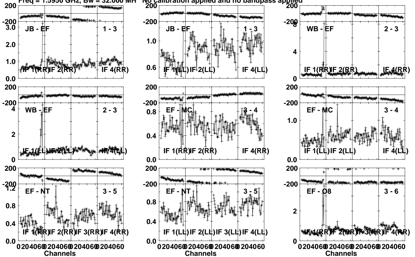
Lower frame: Milli Ampl Jy Top frame: Phas deg Vector averaged cross-power spectrum Several baselines displayed Timerange: 00/19:10:21 to 00/19:11:29
