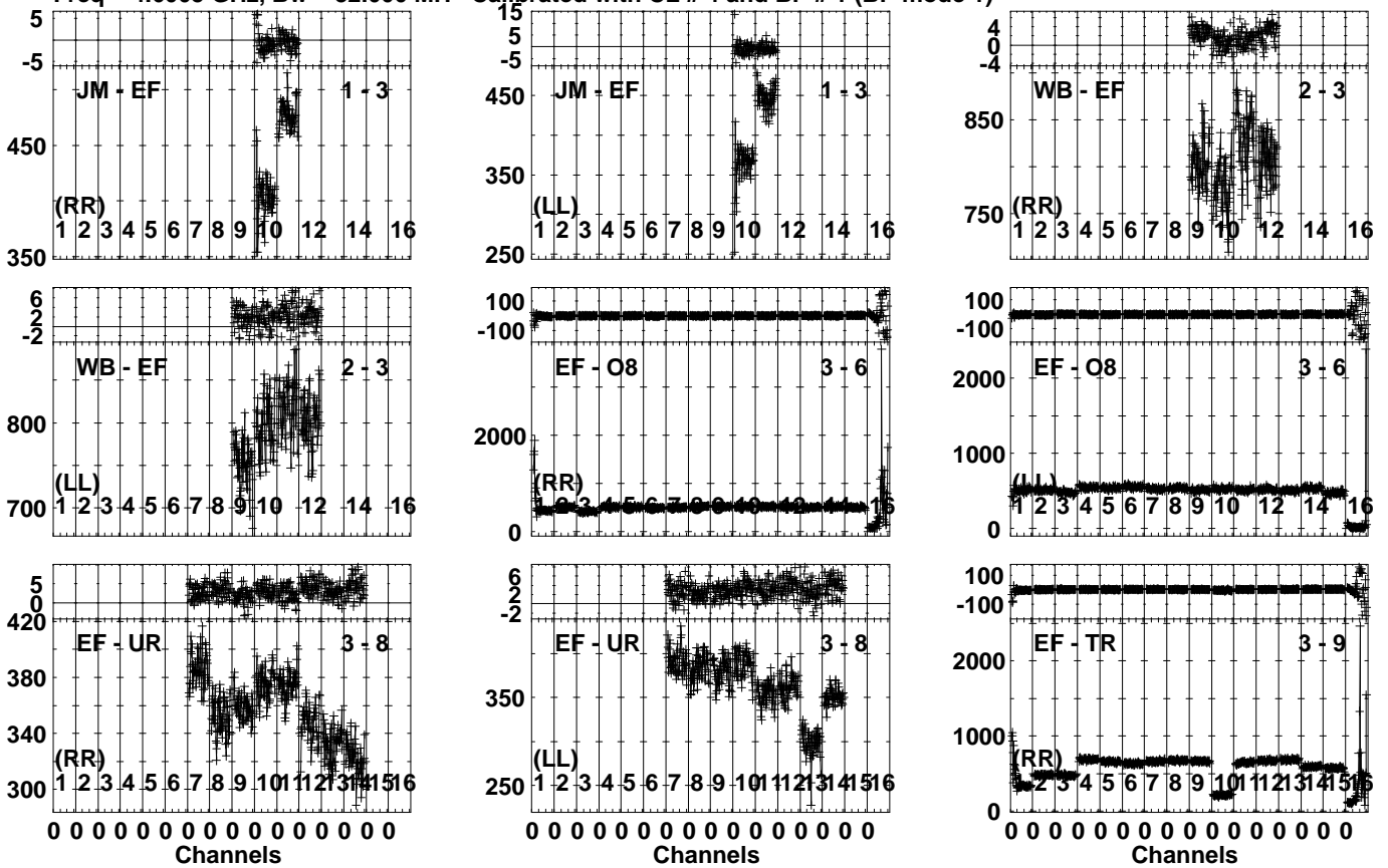
Lower frame: Milli Ampl Jy Top frame: Phas deg Vector averaged cross-power spectrum Several baselines displayed Timerange: 01/00:14:23 to 01/00:15:29
