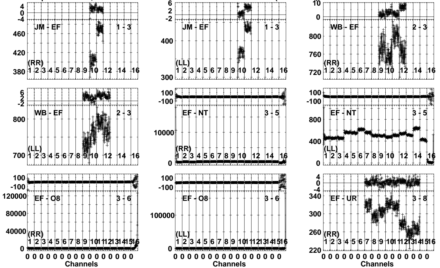
Lower frame: Milli Ampl Jy Top frame: Phas deg Vector averaged cross-power spectrum Several baselines displayed Timerange: 01/02:29:31 to 01/02:31:29
