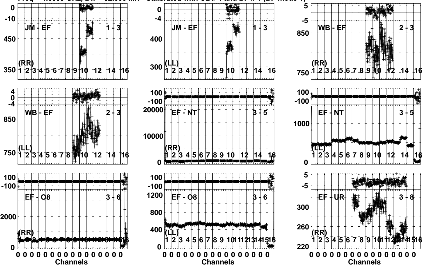
Lower frame: Milli Ampl Jy Top frame: Phas deg Vector averaged cross-power spectrum Several baselines displayed Timerange: 01/02:48:23 to 01/02:49:29
