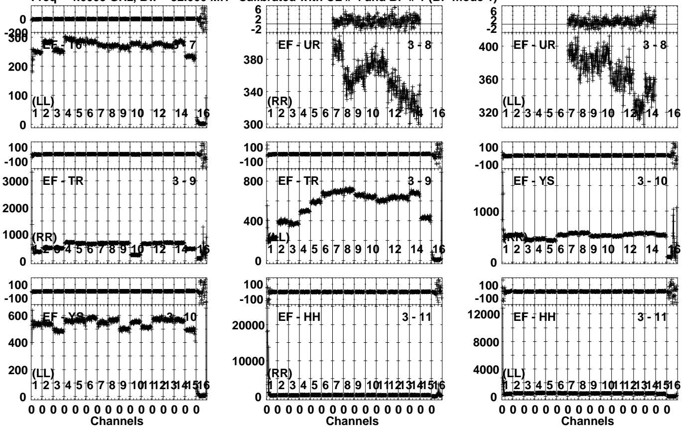
Lower frame: Milli Ampl Jy Top frame: Phas deg Vector averaged cross-power spectrum Several baselines displayed Timerange: 00/23:39:33 to 00/23:40:49
