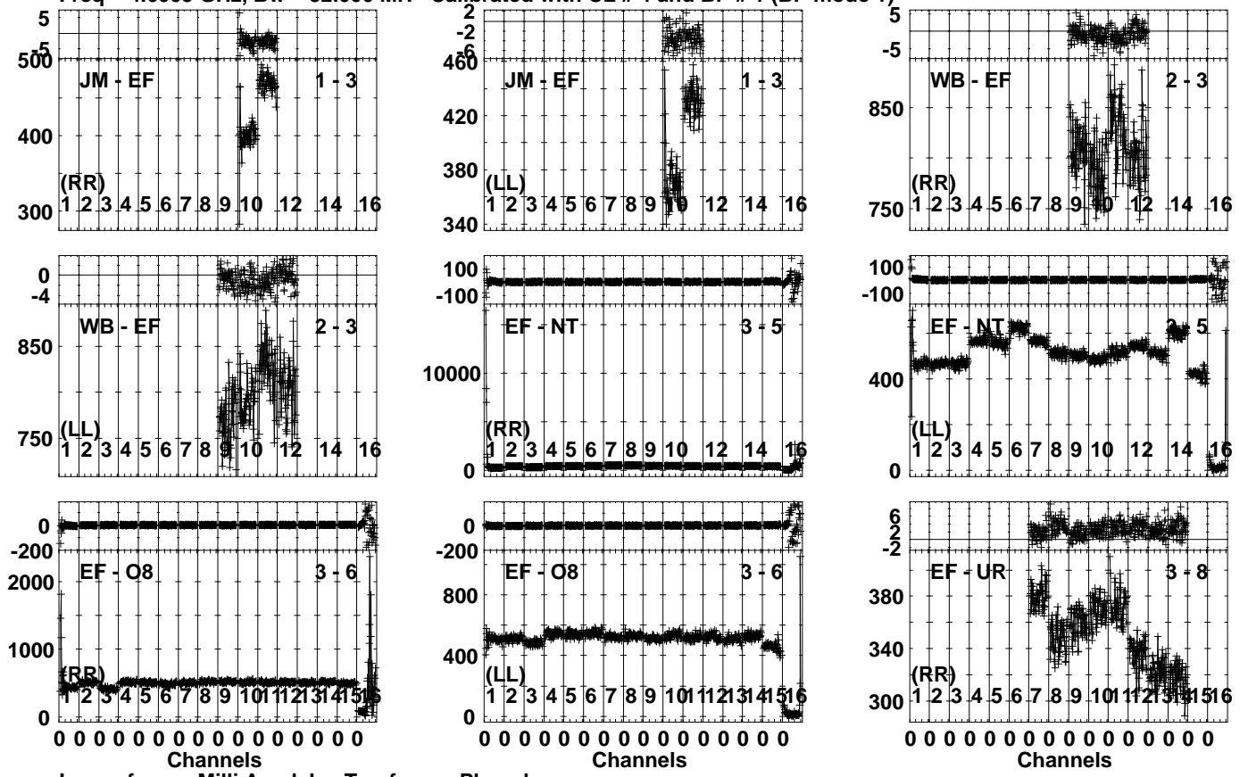
Lower frame: Milli Ampl Jy Top frame: Phas deg Vector averaged cross-power spectrum Several baselines displayed Timerange: 01/01:06:23 to 01/01:07:29
