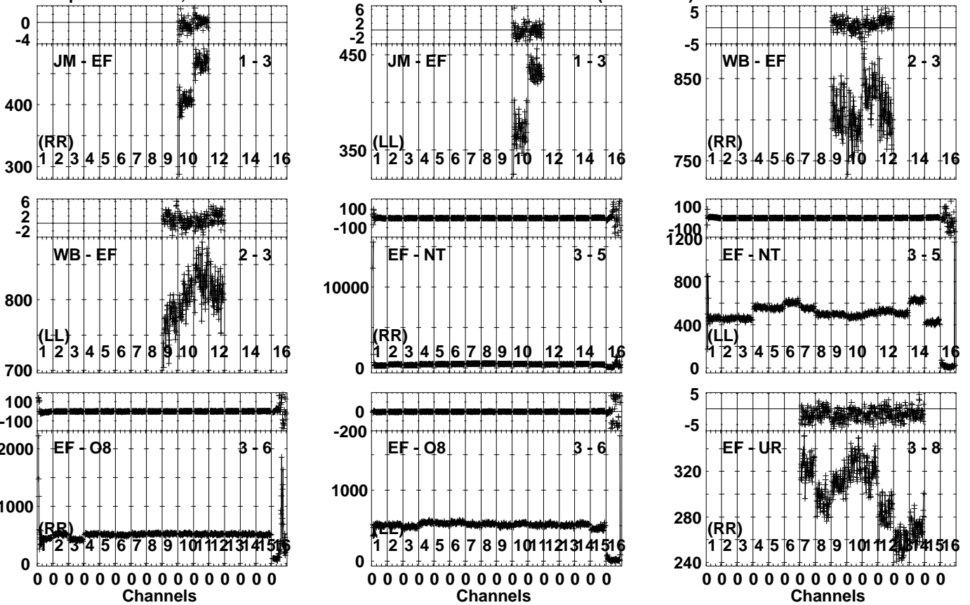
Lower frame: Milli Ampl Jy Top frame: Phas deg Vector averaged cross-power spectrum Several baselines displayed Timerange: 01/02:20:23 to 01/02:21:29
