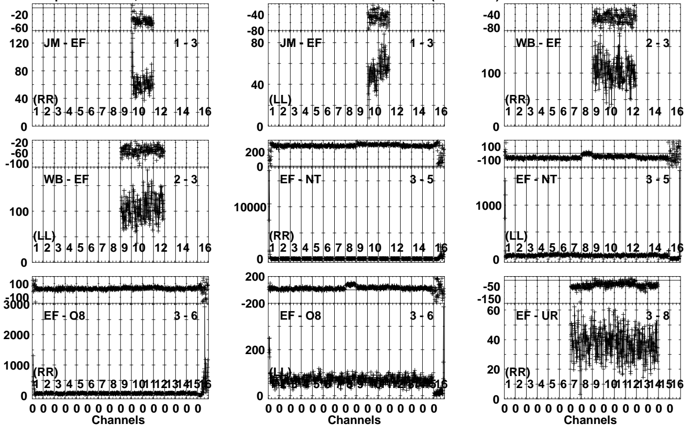
Lower frame: Milli Ampl Jy Top frame: Phas deg Vector averaged cross-power spectrum Several baselines displayed Timerange: 01/00:45:31 to 01/00:47:29
