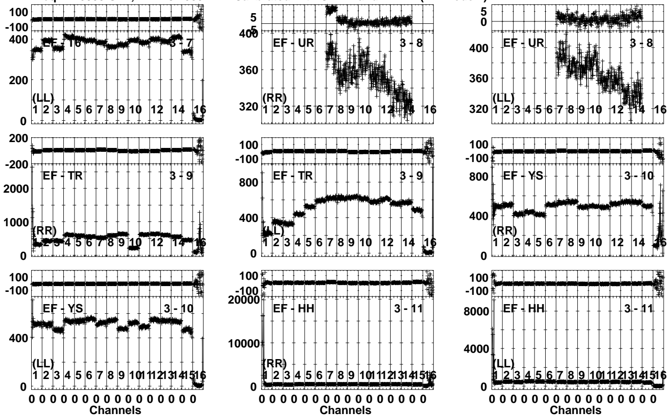
Lower frame: Milli Ampl Jy Top frame: Phas deg Vector averaged cross-power spectrum Several baselines displayed Timerange: 00/21:38:53 to 00/21:40:49
