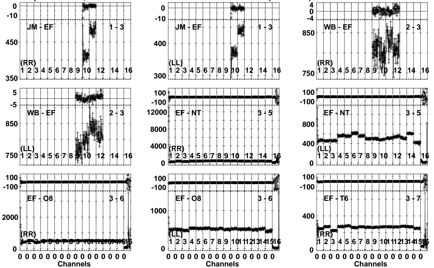
Lower frame: Milli Ampl Jy Top frame: Phas deg Vector averaged cross-power spectrum Several baselines displayed Timerange: 00/23:27:33 to 00/23:28:49
