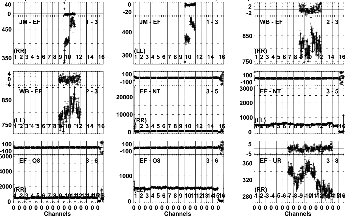
Lower frame: Milli Ampl Jy Top frame: Phas deg Vector averaged cross-power spectrum Several baselines displayed Timerange: 01/01:52:23 to 01/01:53:29
