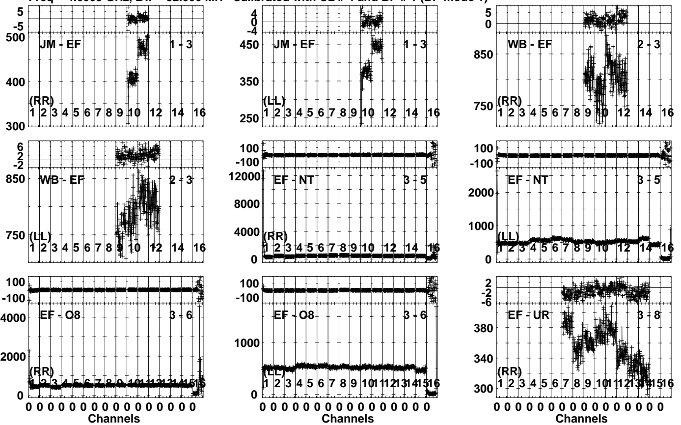
Lower frame: Milli Ampl Jy Top frame: Phas deg Vector averaged cross-power spectrum Several baselines displayed Timerange: 01/00:44:23 to 01/00:45:29
