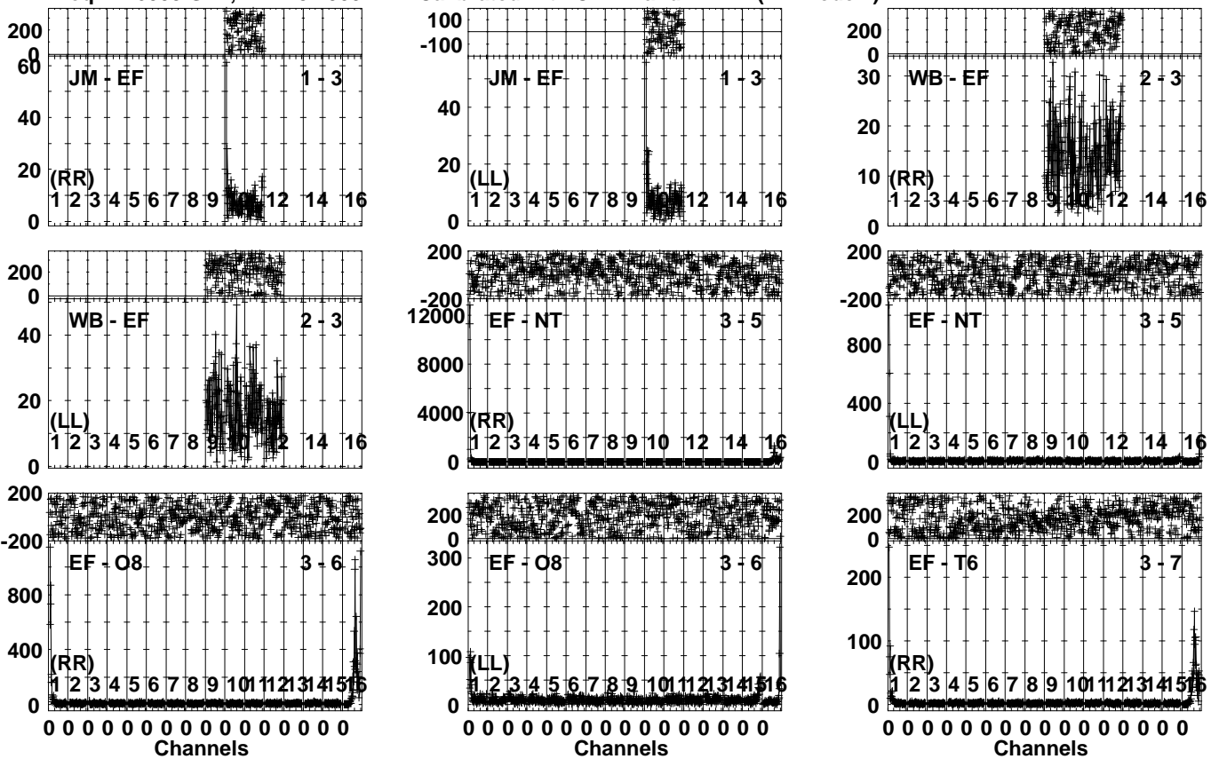
Lower frame: Milli Ampl Jy Top frame: Phas deg Vector averaged cross-power spectrum Several baselines displayed Timerange: 00/21:52:51 to 00/21:56:49
