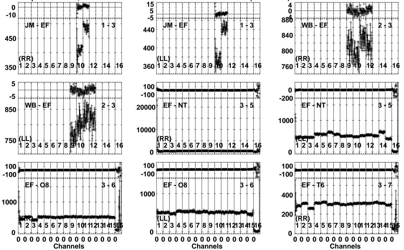
Lower frame: Milli Ampl Jy Top frame: Phas deg Vector averaged cross-power spectrum Several baselines displayed Timerange: 00/23:11:33 to 00/23:12:49
