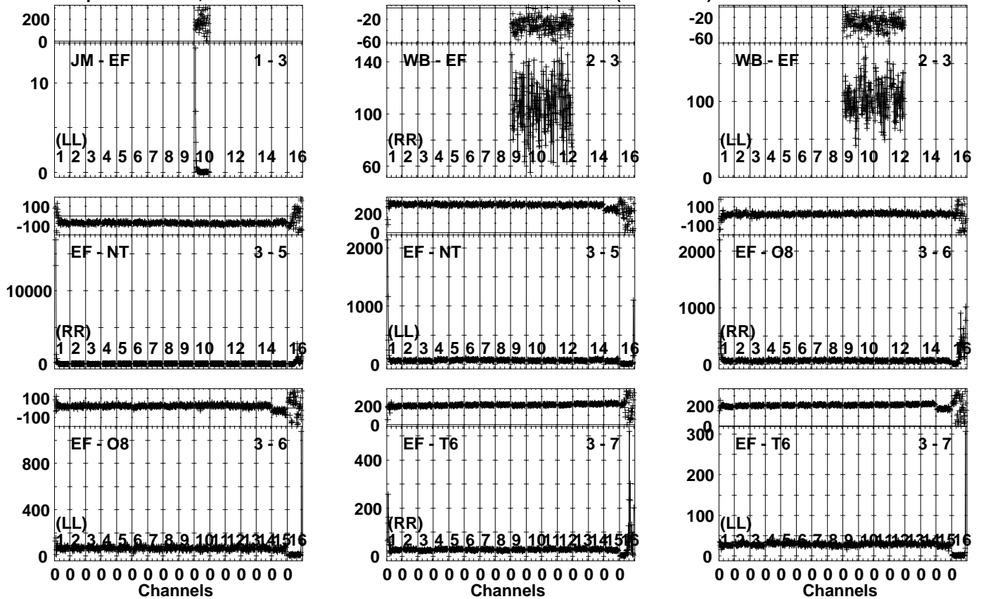
Lower frame: Milli Ampl Jy Top frame: Phas deg Vector averaged cross-power spectrum Several baselines displayed Timerange: 00/22:10:51 to 00/22:12:49
