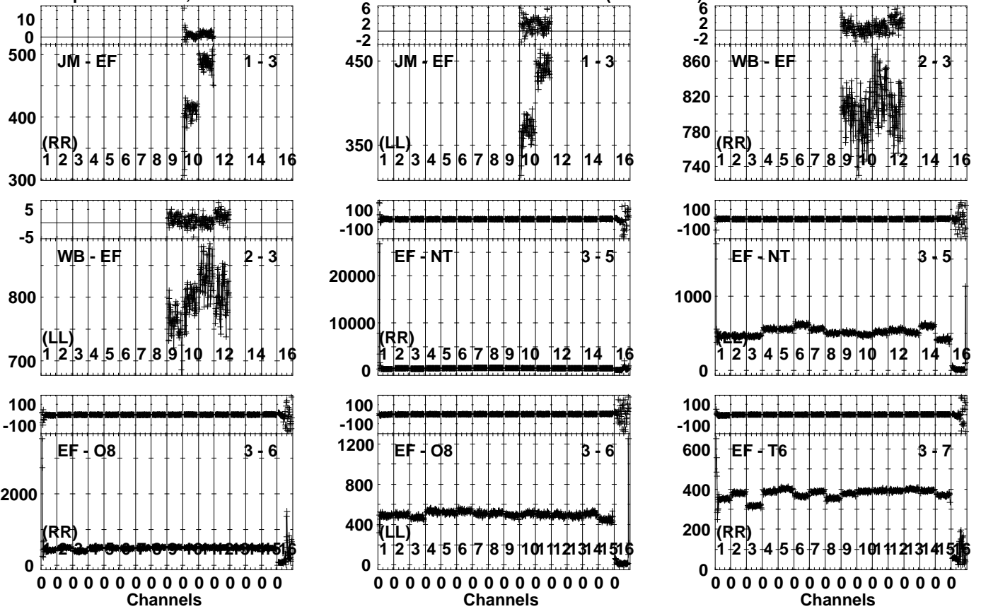
Lower frame: Milli Ampl Jy Top frame: Phas deg Vector averaged cross-power spectrum Several baselines displayed Timerange: 00/21:29:33 to 00/21:30:49
