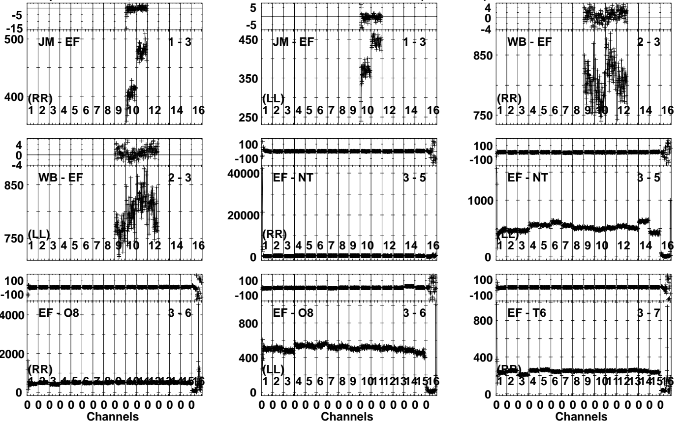
Lower frame: Milli Ampl Jy Top frame: Phas deg Vector averaged cross-power spectrum Several baselines displayed Timerange: 00/23:51:33 to 00/23:52:49
