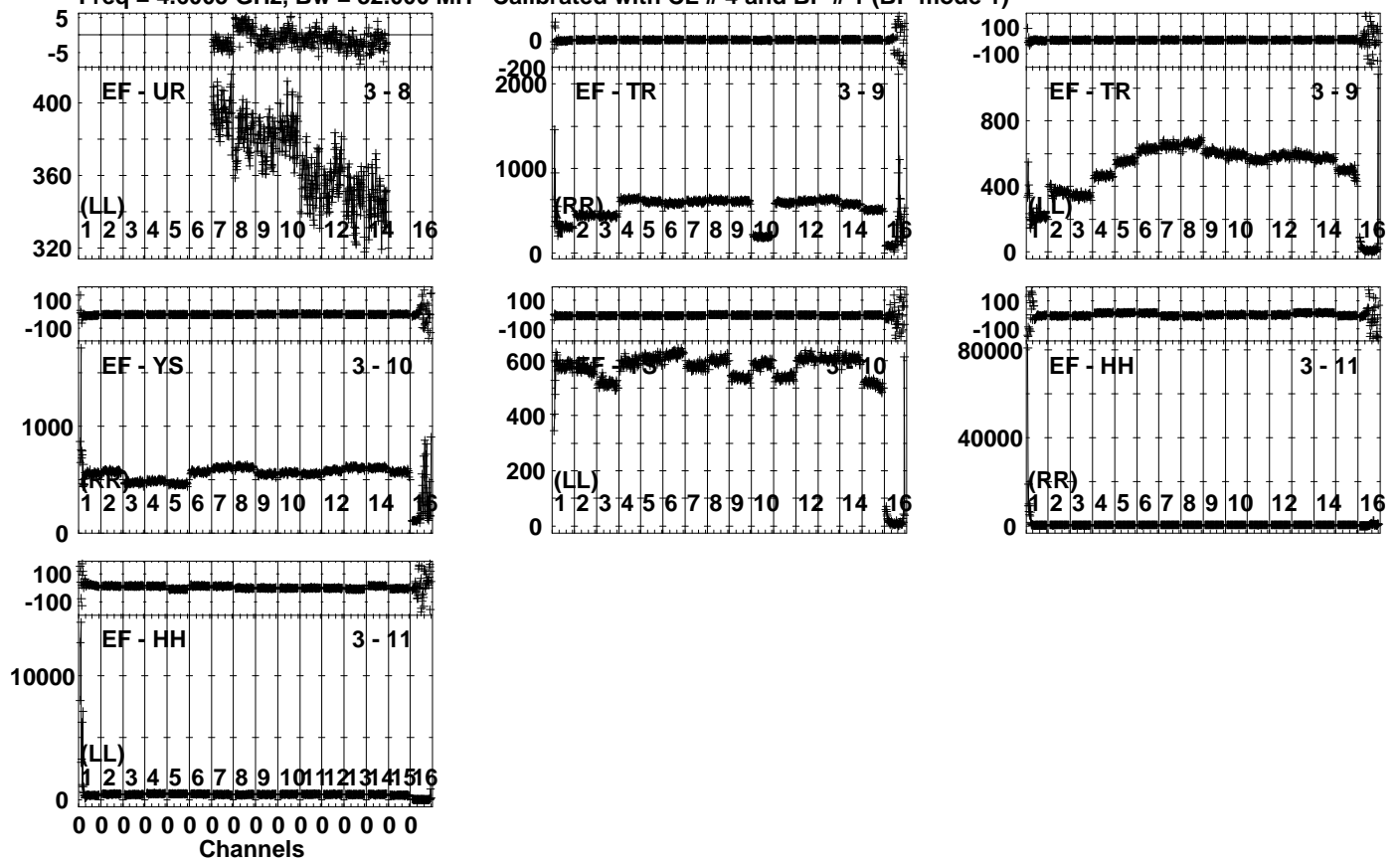
Lower frame: Milli Ampl Jy Top frame: Phas deg Vector averaged cross-power spectrum Several baselines displayed Timerange: 01/00:44:23 to 01/00:45:29
