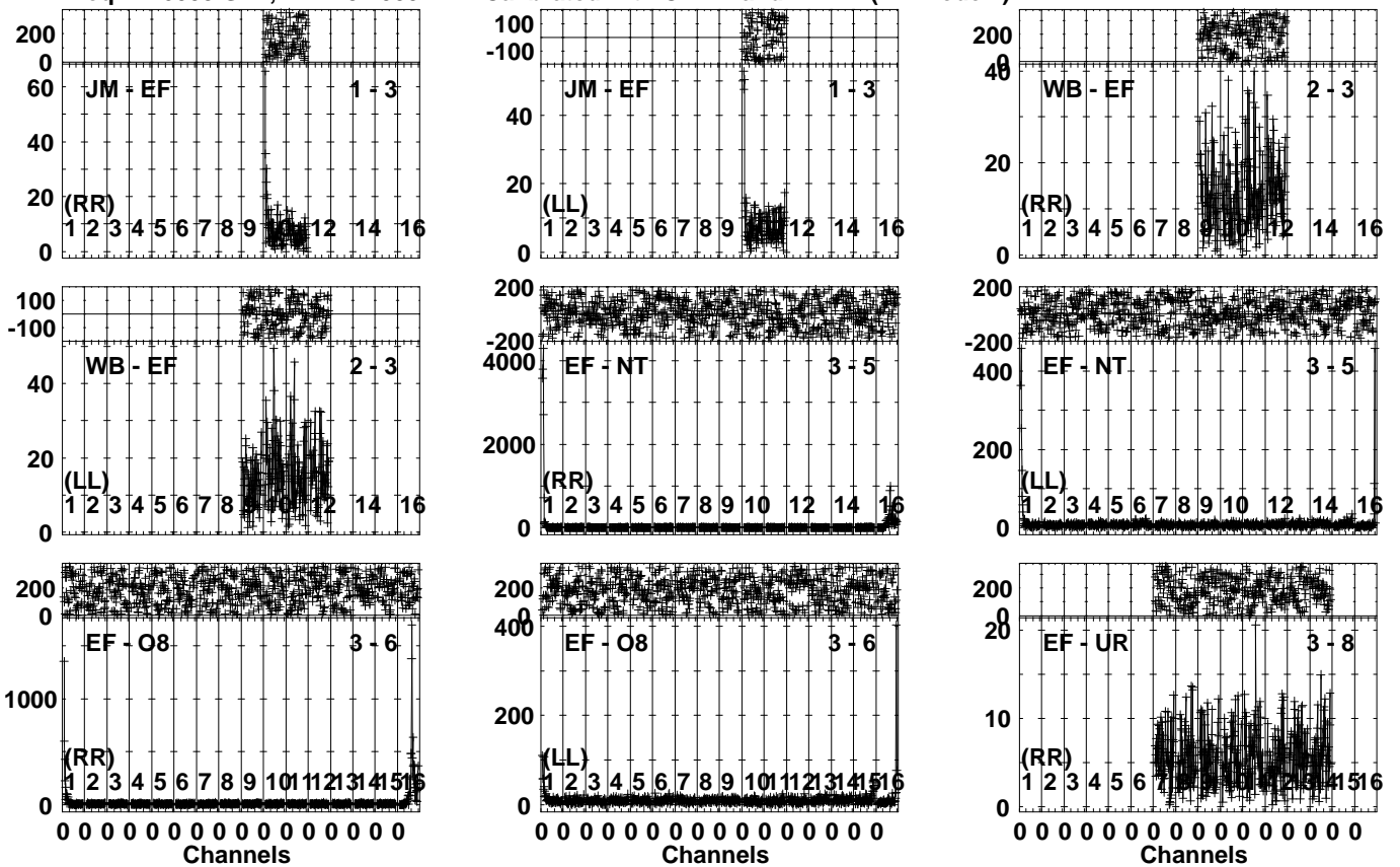
Lower frame: Milli Ampl Jy Top frame: Phas deg Vector averaged cross-power spectrum Several baselines displayed Timerange: 01/00:49:33 to 01/00:53:29
