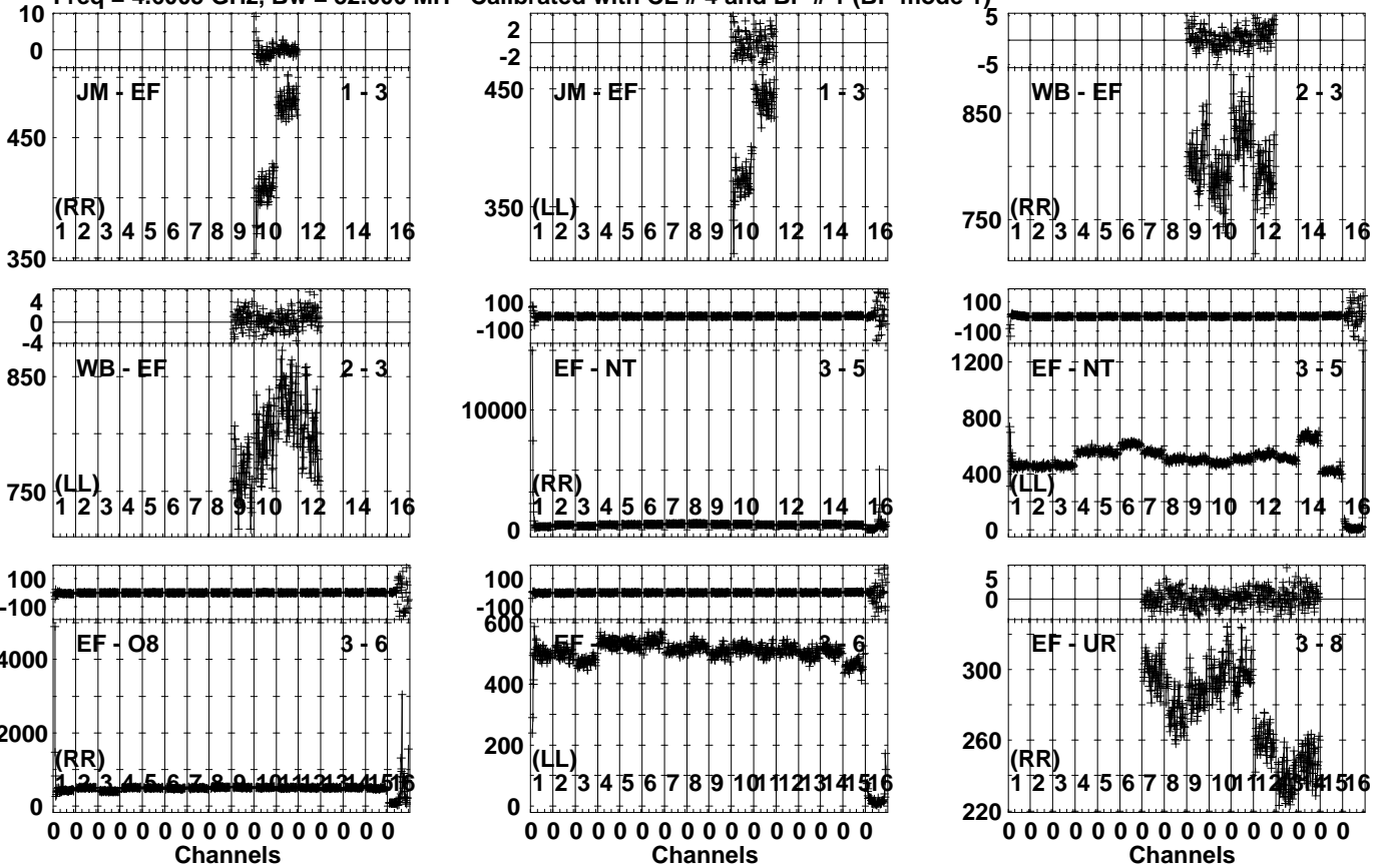
Lower frame: Milli Ampl Jy Top frame: Phas deg Vector averaged cross-power spectrum Several baselines displayed Timerange: 01/02:54:23 to 01/02:55:29
