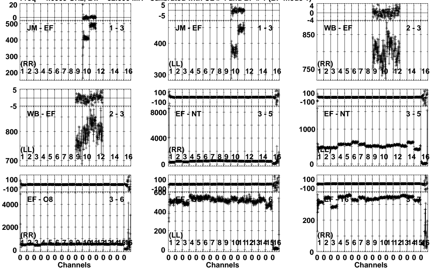
Lower frame: Milli Ampl Jy Top frame: Phas deg Vector averaged cross-power spectrum Several baselines displayed Timerange: 00/22:46:51 to 00/22:48:49
