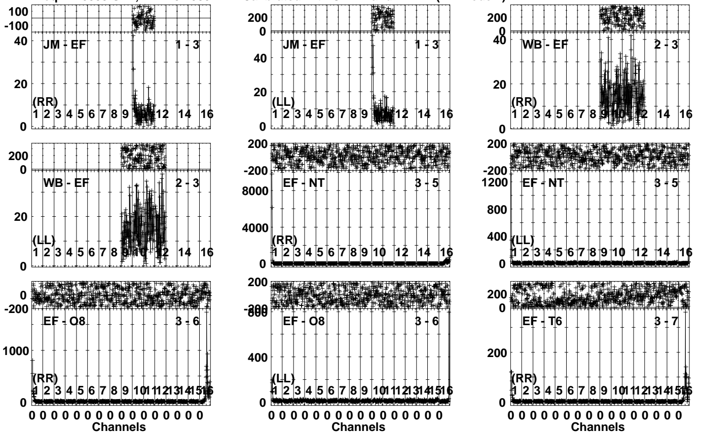
Lower frame: Milli Ampl Jy Top frame: Phas deg Vector averaged cross-power spectrum Several baselines displayed Timerange: 00/21:18:51 to 00/21:22:49
