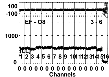
Lower frame: Milli Ampl Jy Top frame: Phas deg Vector averaged cross-power spectrum Several baselines displayed Timerange: 00/23:20:53 to 00/23:22:49
