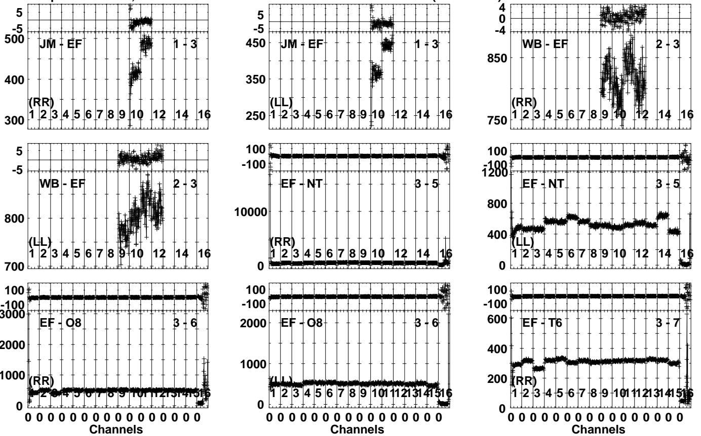
Lower frame: Milli Ampl Jy Top frame: Phas deg Vector averaged cross-power spectrum Several baselines displayed Timerange: 00/23:05:33 to 00/23:06:49
