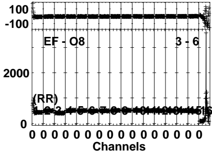
Lower frame: Milli Ampl Jy Top frame: Phas deg Vector averaged cross-power spectrum Several baselines displayed Timerange: 00/22:37:33 to 00/22:38:49
