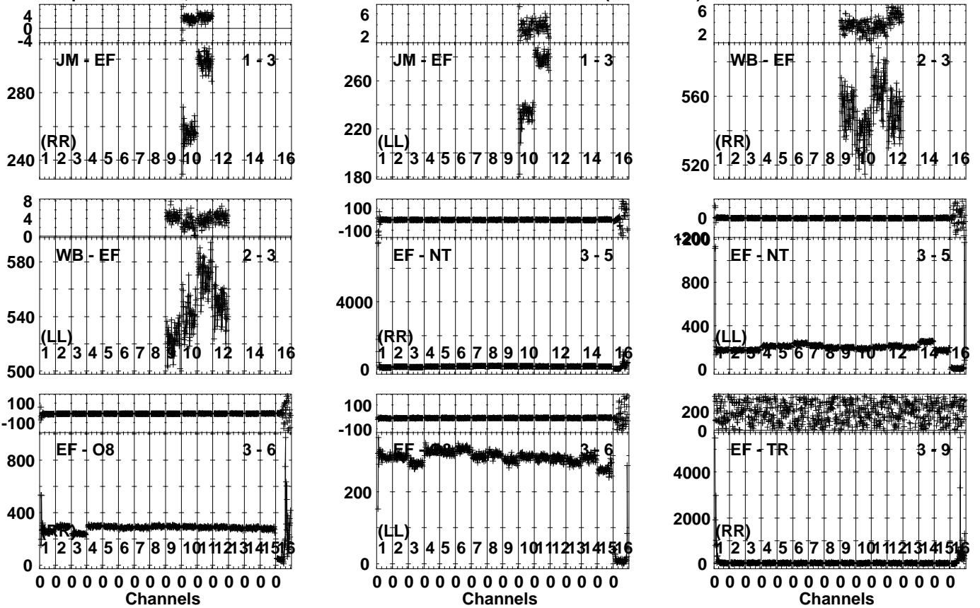
Lower frame: Milli Ampl Jy Top frame: Phas deg Vector averaged cross-power spectrum Several baselines displayed Timerange: 01/02:56:03 to 01/02:59:59
