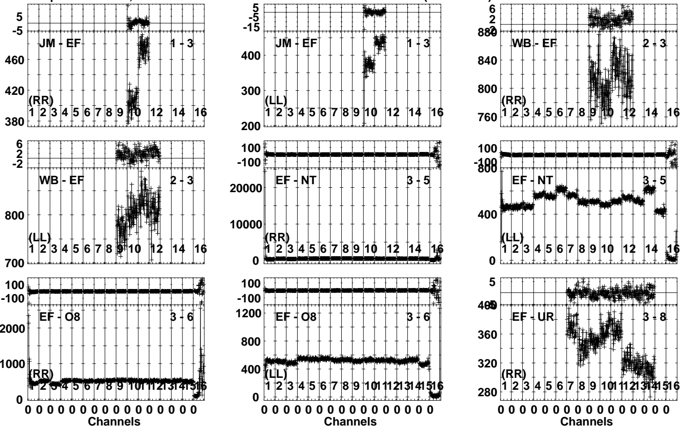
Lower frame: Milli Ampl Jy Top frame: Phas deg Vector averaged cross-power spectrum Several baselines displayed Timerange: 01/01:21:31 to 01/01:23:29
