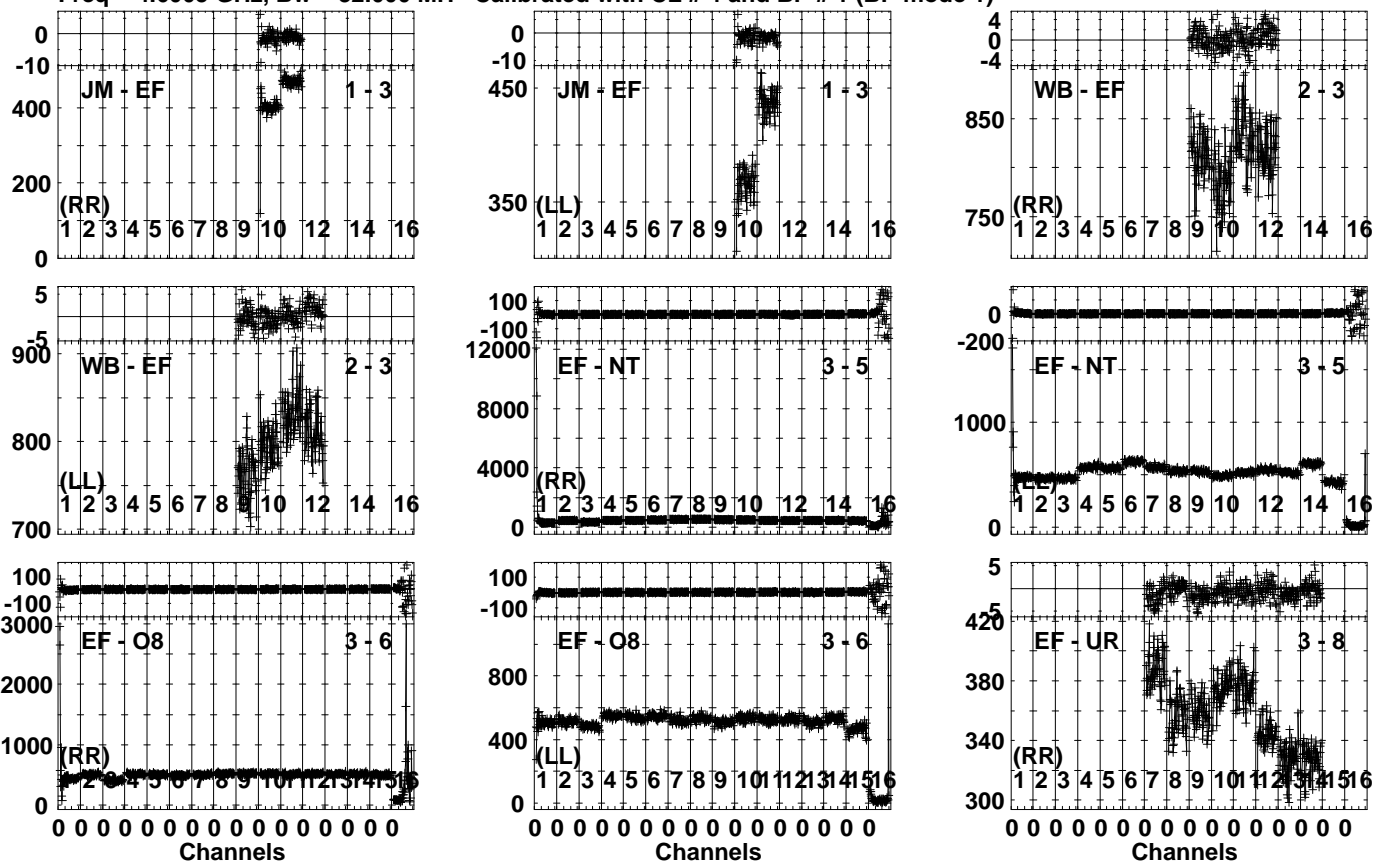
Lower frame: Milli Ampl Jy Top frame: Phas deg Vector averaged cross-power spectrum Several baselines displayed Timerange: 01/00:54:23 to 01/00:55:29
