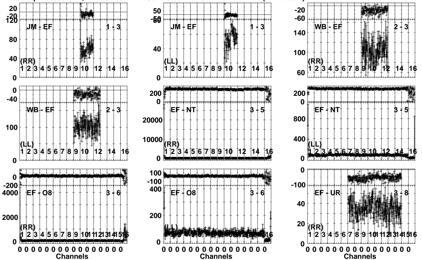
Lower frame: Milli Ampl Jy Top frame: Phas deg Vector averaged cross-power spectrum Several baselines displayed Timerange: 01/01:19:31 to 01/01:21:29
