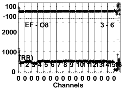
Lower frame: Milli Ampl Jy Top frame: Phas deg Vector averaged cross-power spectrum Several baselines displayed Timerange: 00/23:20:53 to 00/23:22:49
