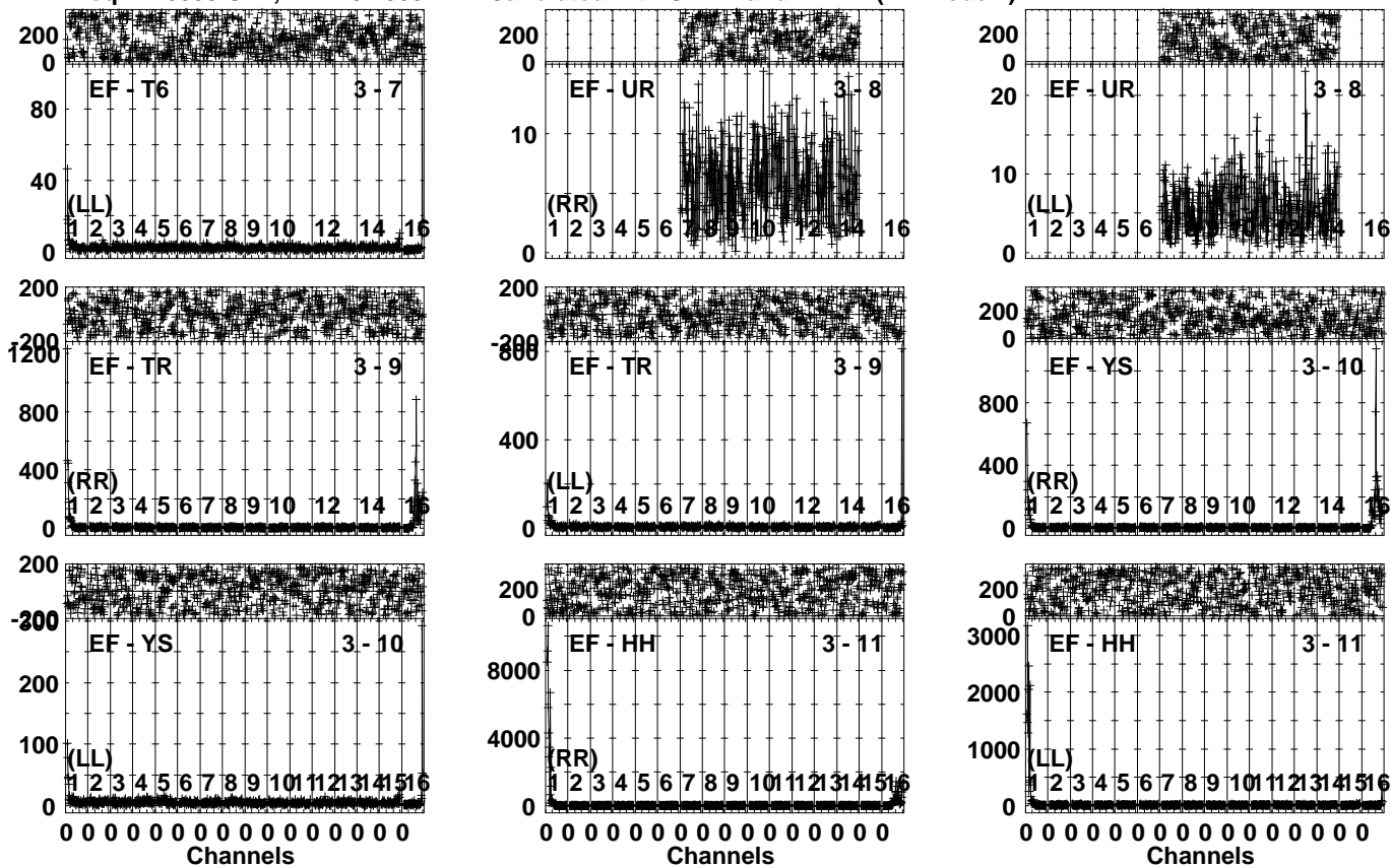
Lower frame: Milli Ampl Jy Top frame: Phas deg Vector averaged cross-power spectrum Several baselines displayed Timerange: 00/21:06:53 to 00/21:10:49
