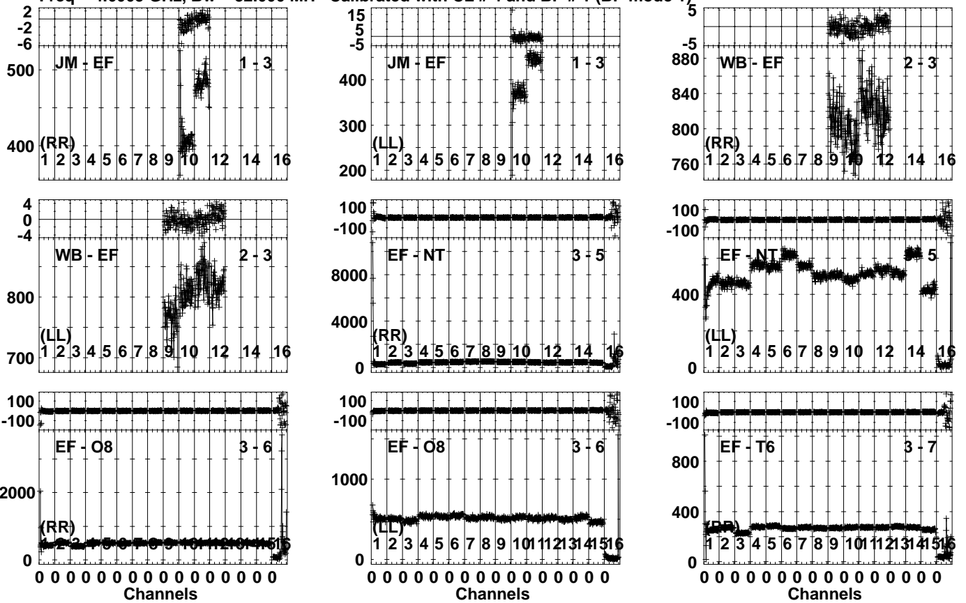
Lower frame: Milli Ampl Jy Top frame: Phas deg Vector averaged cross-power spectrum Several baselines displayed Timerange: 00/23:33:33 to 00/23:34:49
