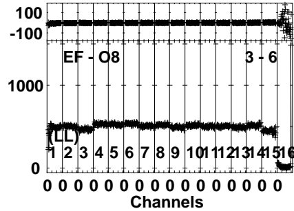
Lower frame: Milli Ampl Jy Top frame: Phas deg Vector averaged cross-power spectrum Several baselines displayed Timerange: 00/22:37:33 to 00/22:38:49
