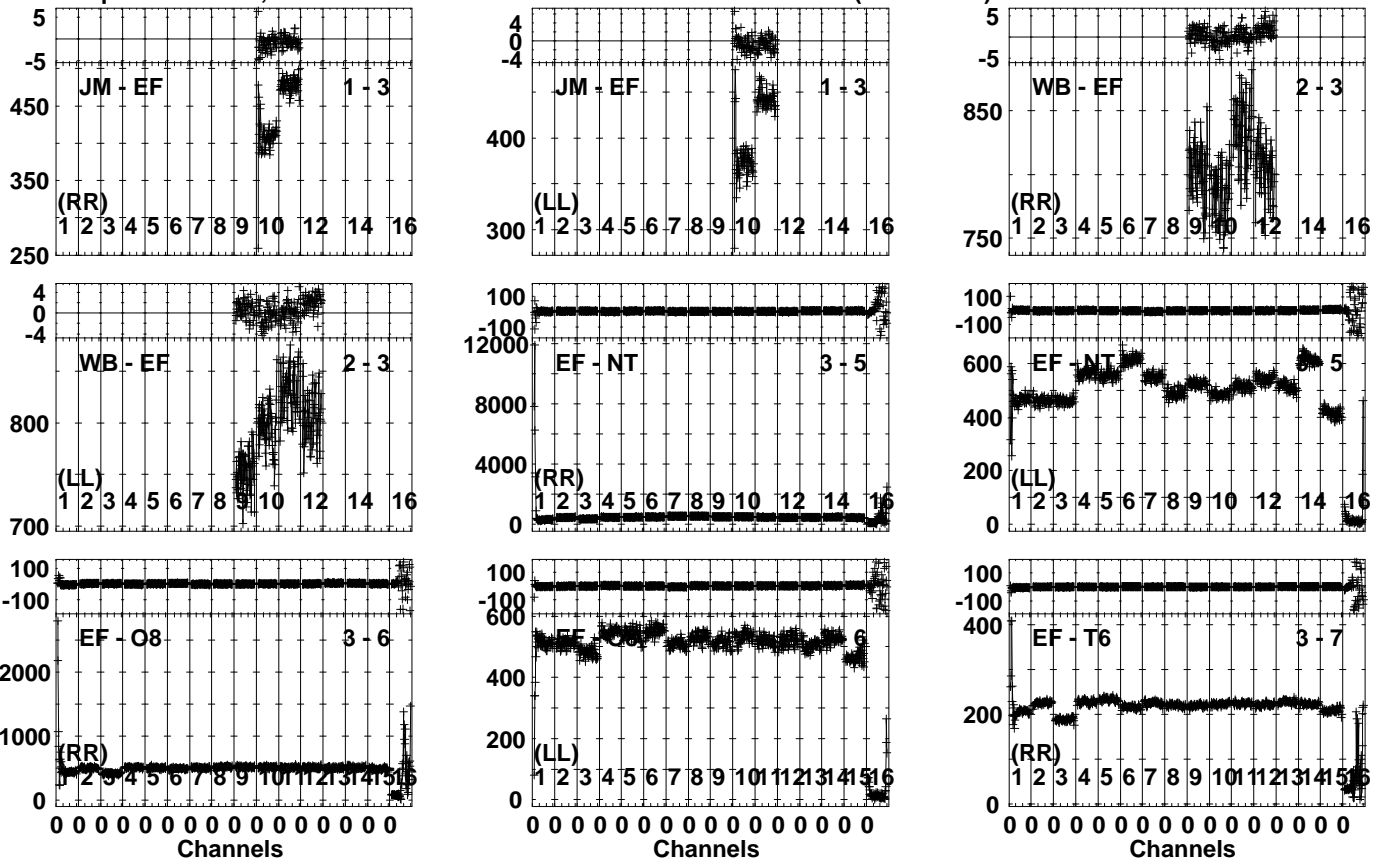
Lower frame: Milli Ampl Jy Top frame: Phas deg Vector averaged cross-power spectrum Several baselines displayed Timerange: 00/23:54:53 to 00/23:56:49
