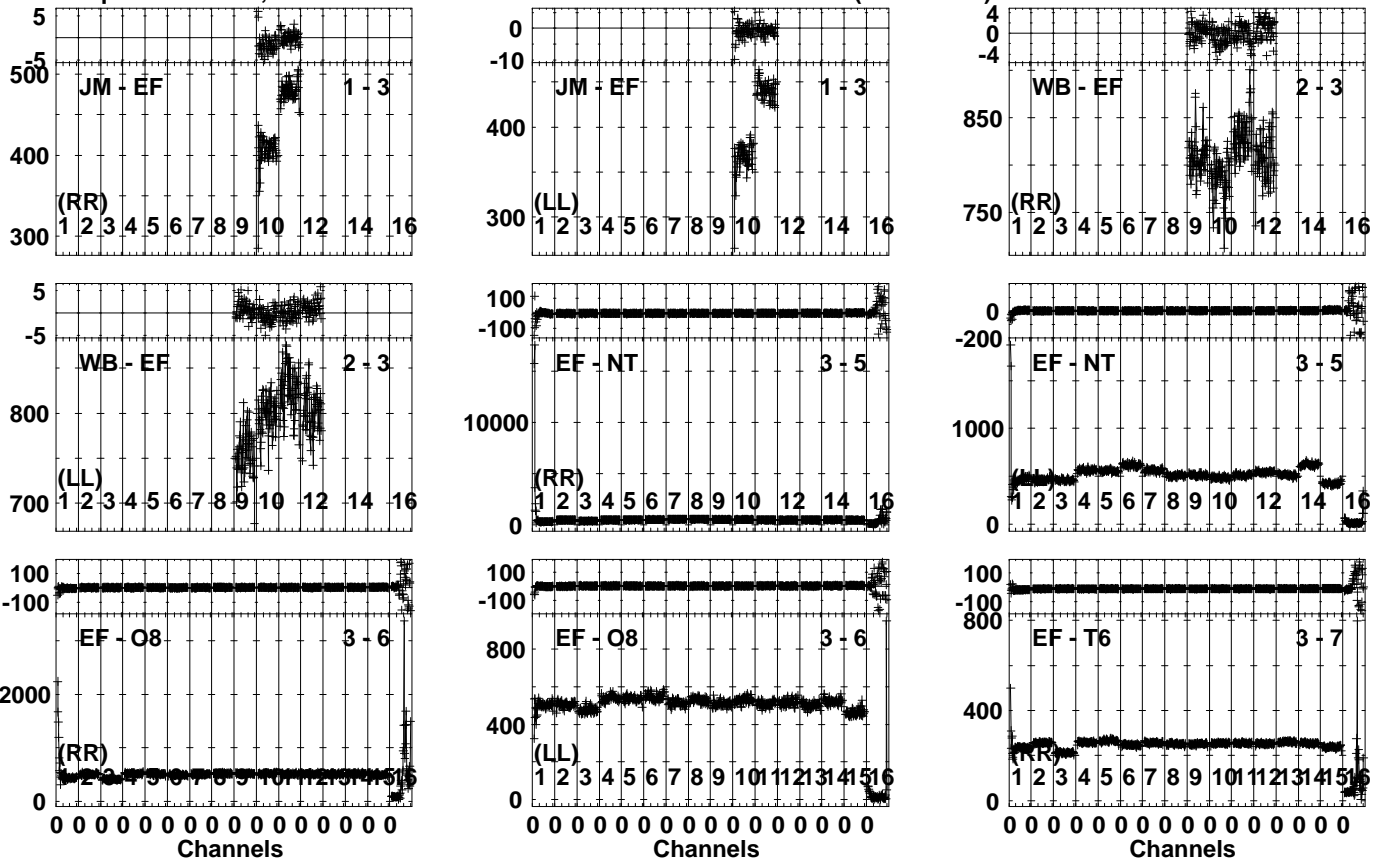
Lower frame: Milli Ampl Jy Top frame: Phas deg Vector averaged cross-power spectrum Several baselines displayed Timerange: 00/23:45:33 to 00/23:46:49
