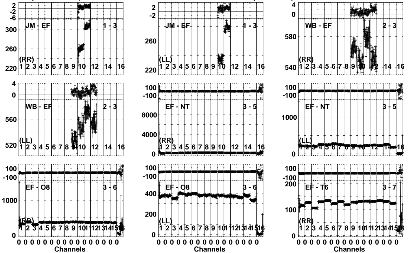
Lower frame: Milli Ampl Jy Top frame: Phas deg Vector averaged cross-power spectrum Several baselines displayed Timerange: 00/21:00:03 to 00/21:03:59
