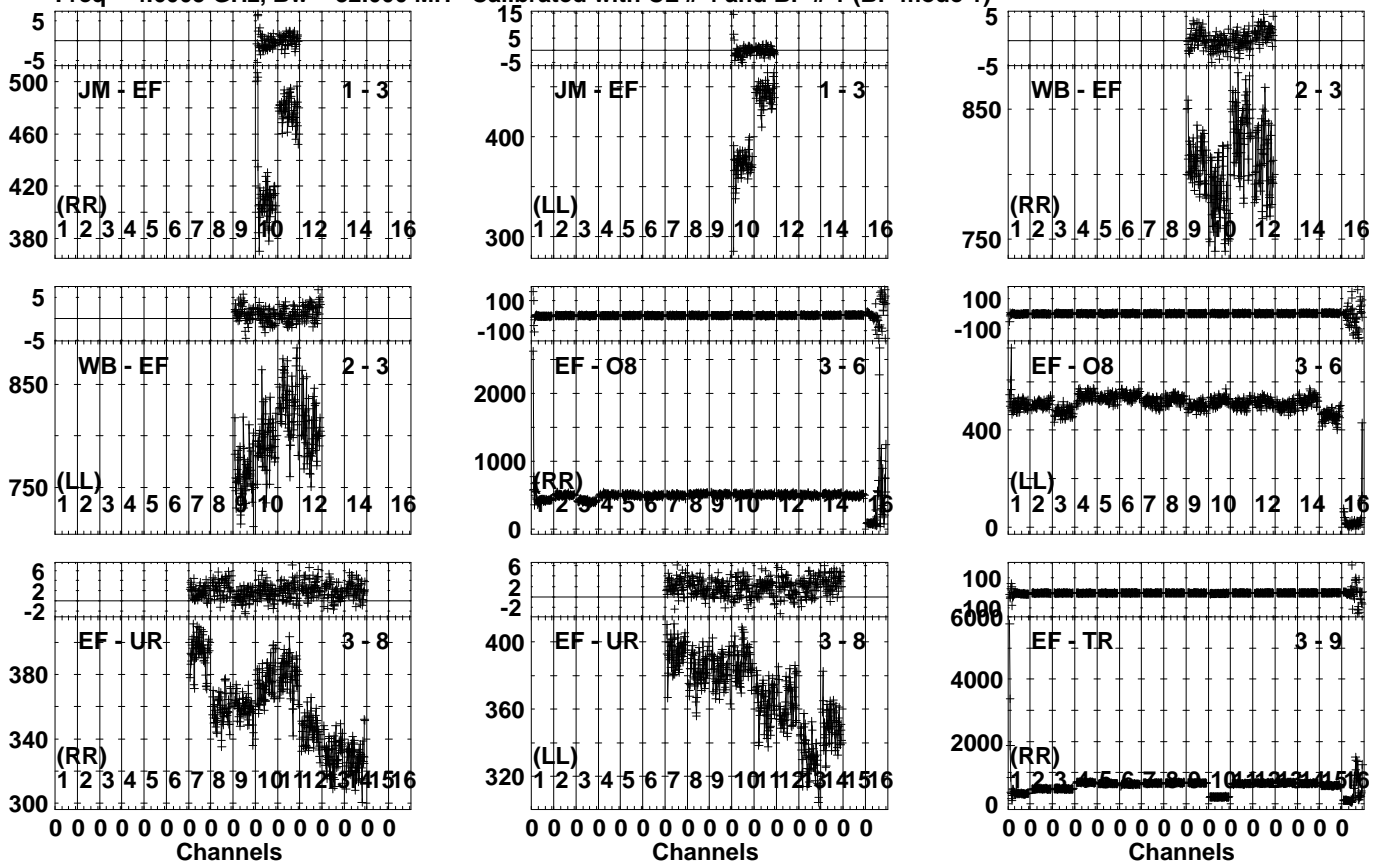
Lower frame: Milli Ampl Jy Top frame: Phas deg Vector averaged cross-power spectrum Several baselines displayed Timerange: 01/00:20:23 to 01/00:21:29
