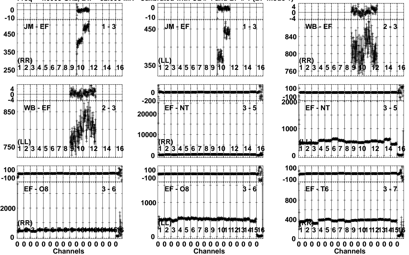
Lower frame: Milli Ampl Jy Top frame: Phas deg Vector averaged cross-power spectrum Several baselines displayed Timerange: 00/21:35:33 to 00/21:36:49
