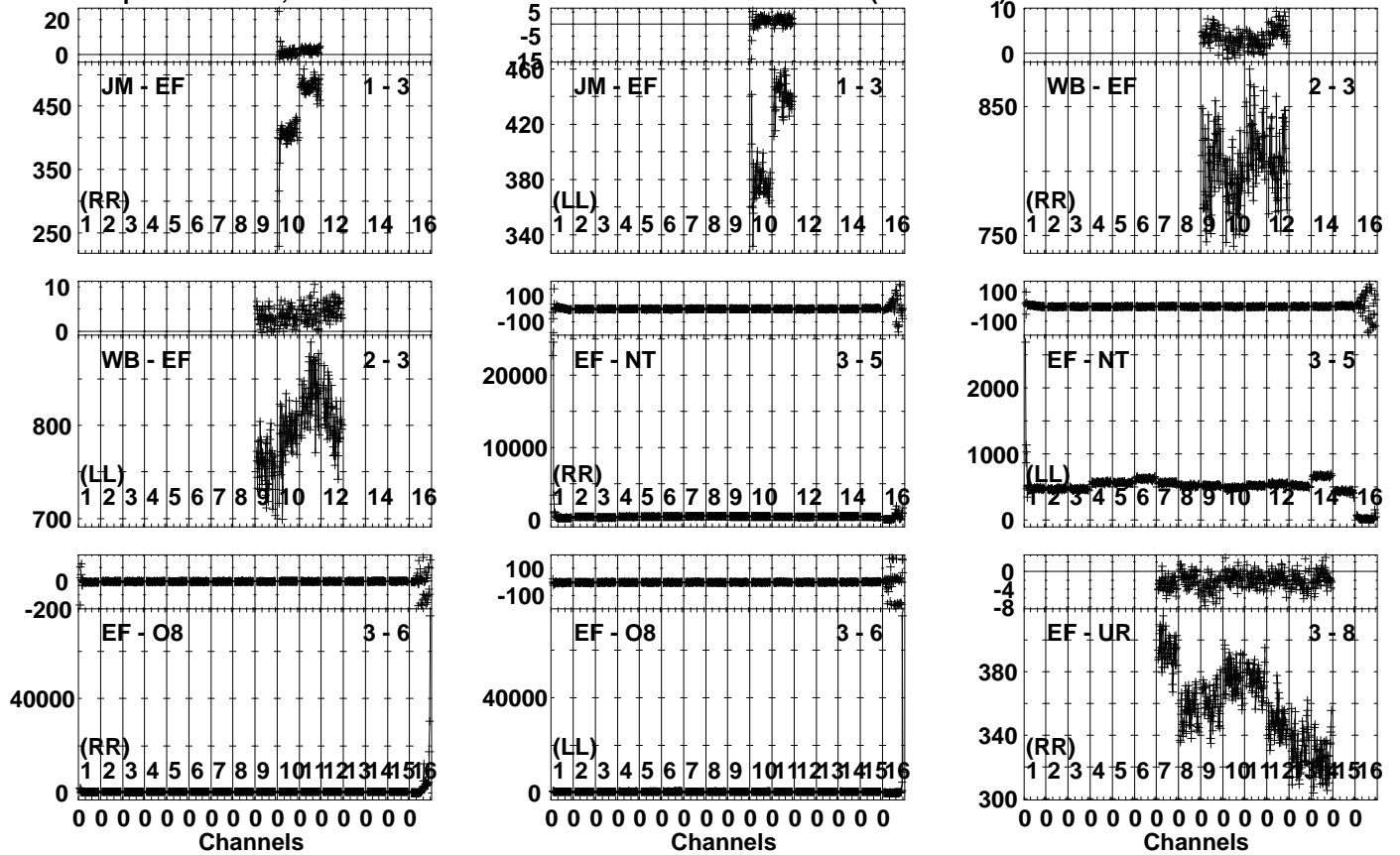
Lower frame: Milli Ampl Jy Top frame: Phas deg Vector averaged cross-power spectrum Several baselines displayed Timerange: 01/00:38:23 to 01/00:39:29
