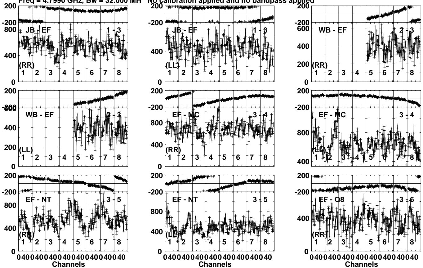
Lower frame: Micro Ampl Jy Top frame: Phas deg Vector averaged cross-power spectrum Several baselines displayed Timerange: 00/08:29:01 to 00/08:30:29
