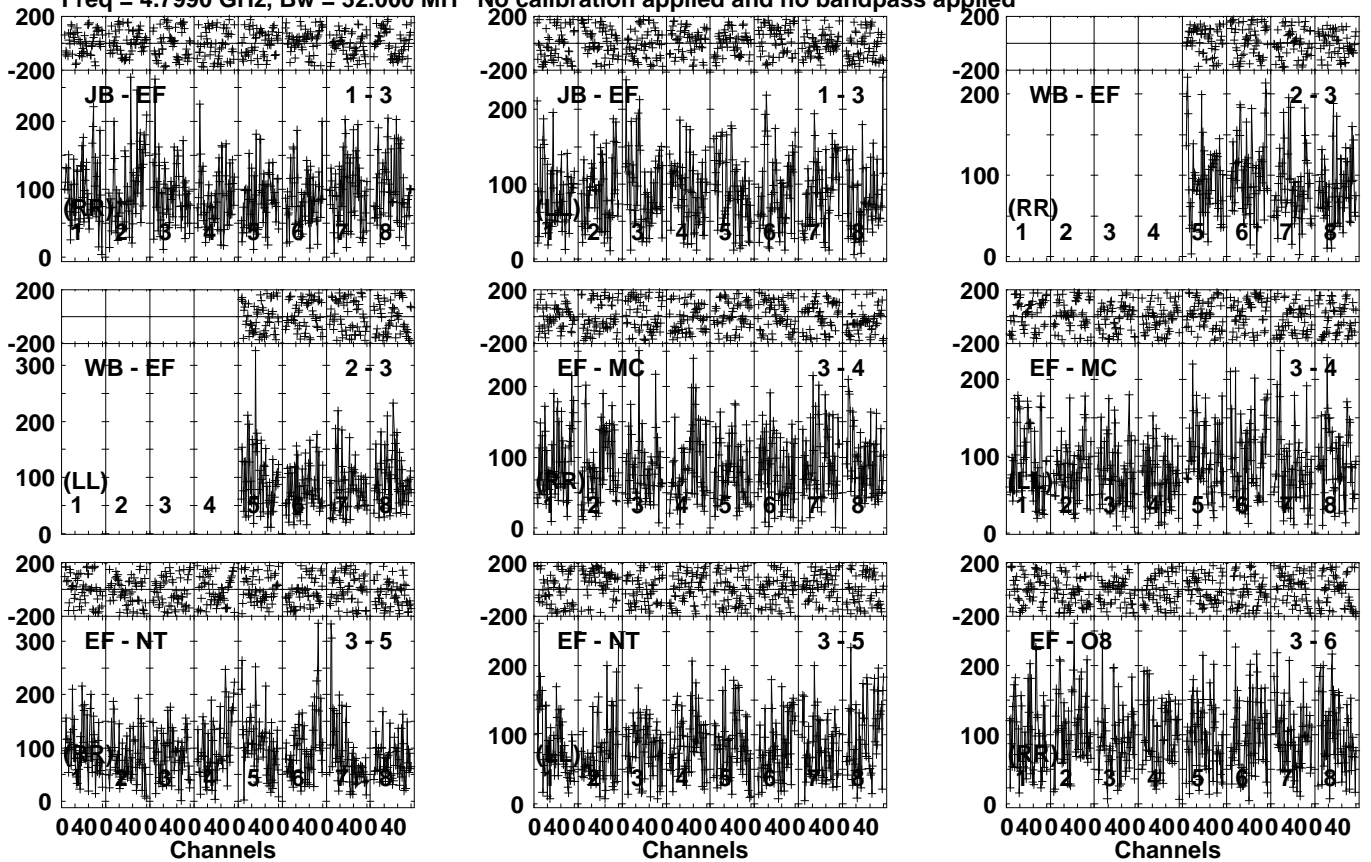
Lower frame: Micro Ampl Jy Top frame: Phas deg Vector averaged cross-power spectrum Several baselines displayed Timerange: 00/10:44:21 to 00/10:47:19
