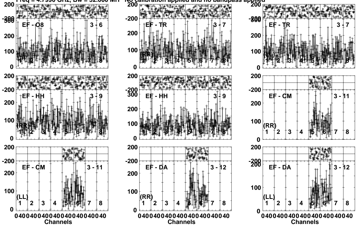
Lower frame: Micro Ampl Jy Top frame: Phas deg Vector averaged cross-power spectrum Several baselines displayed Timerange: 00/05:37:51 to 00/05:40:49
