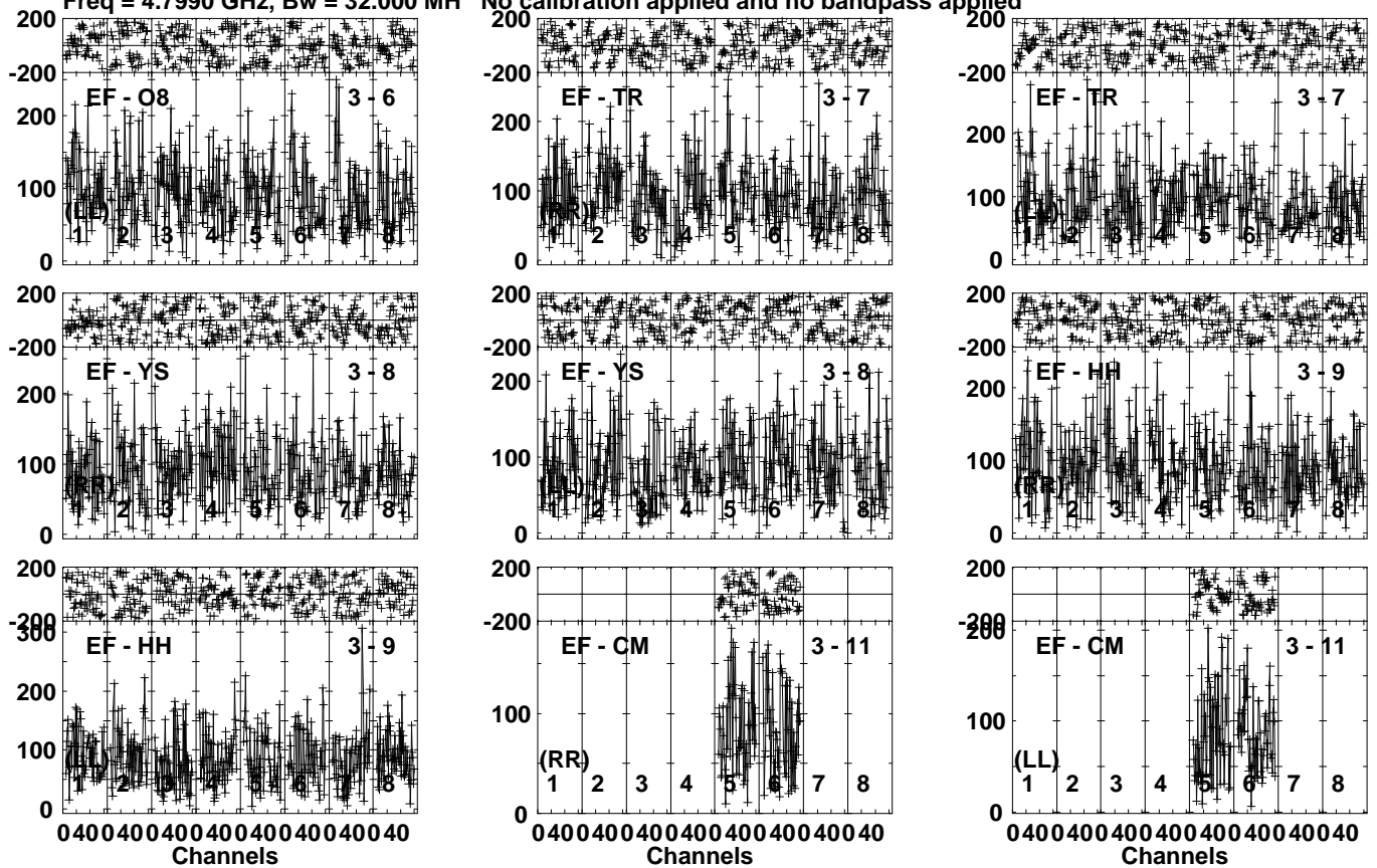
Lower frame: Micro Ampl Jy Top frame: Phas deg Vector averaged cross-power spectrum Several baselines displayed Timerange: 00/07:27:11 to 00/07:30:09
