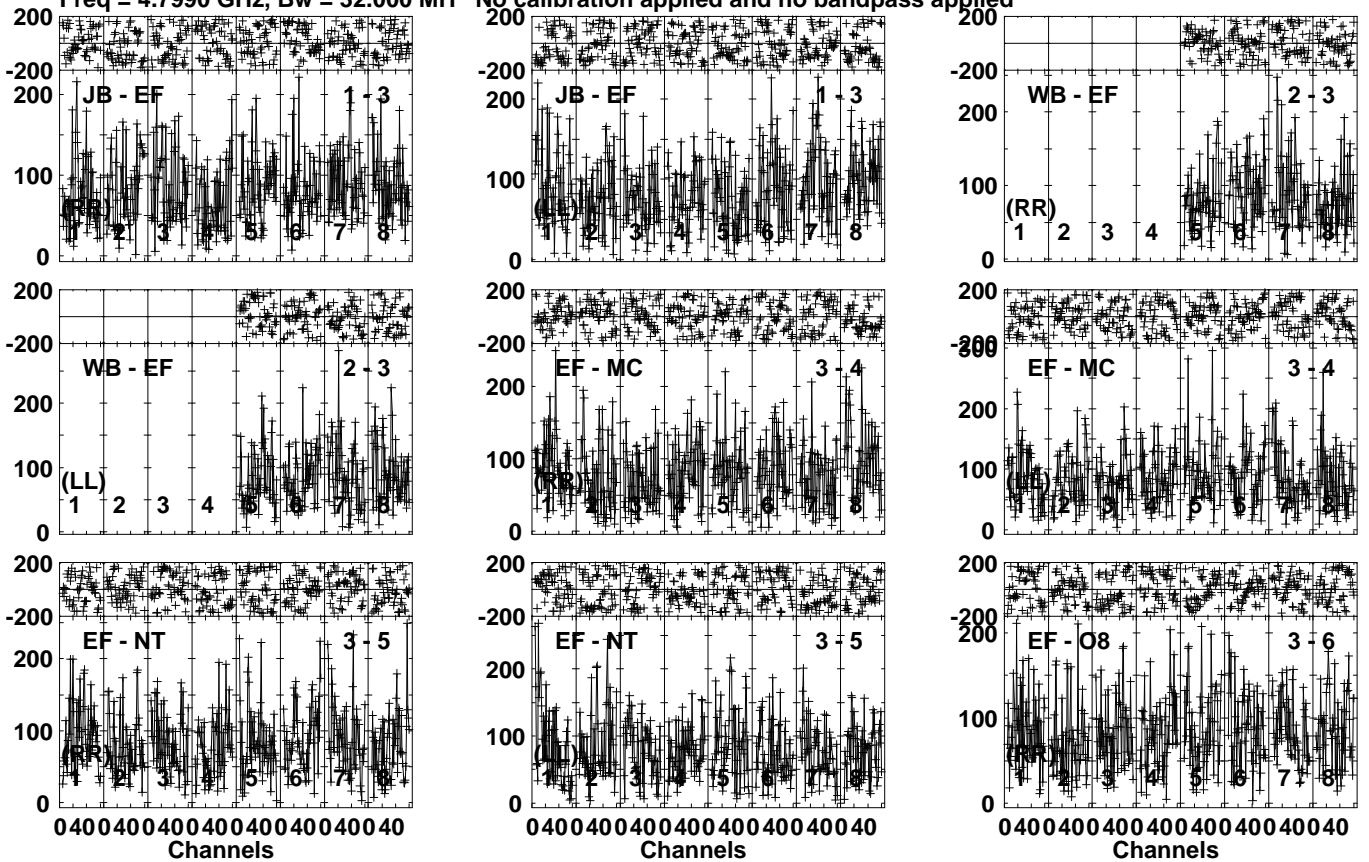
Lower frame: Micro Ampl Jy Top frame: Phas deg Vector averaged cross-power spectrum Several baselines displayed Timerange: 00/09:50:41 to 00/09:54:19
