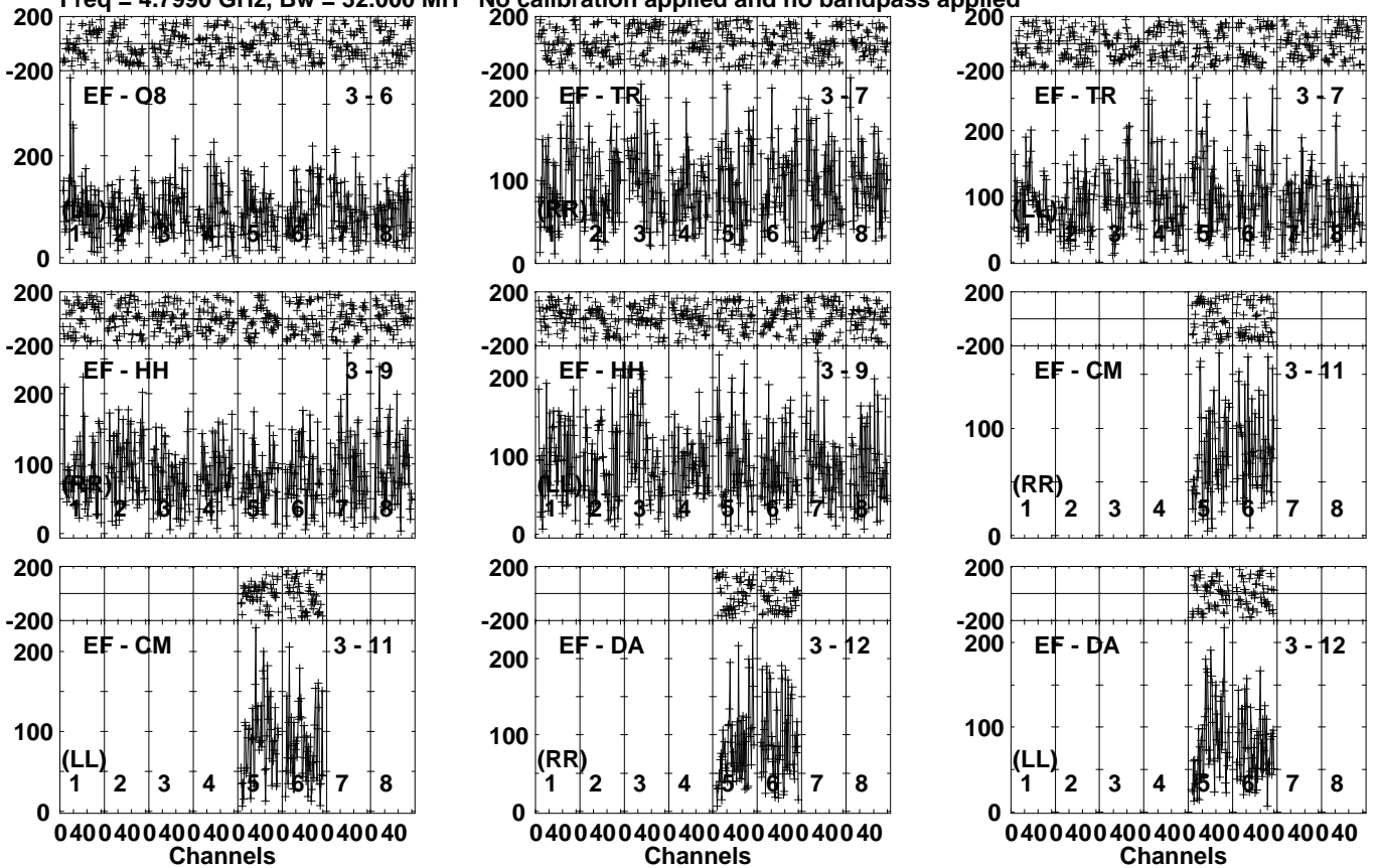
Lower frame: Micro Ampl Jy Top frame: Phas deg Vector averaged cross-power spectrum Several baselines displayed Timerange: 00/05:27:11 to 00/05:30:09
