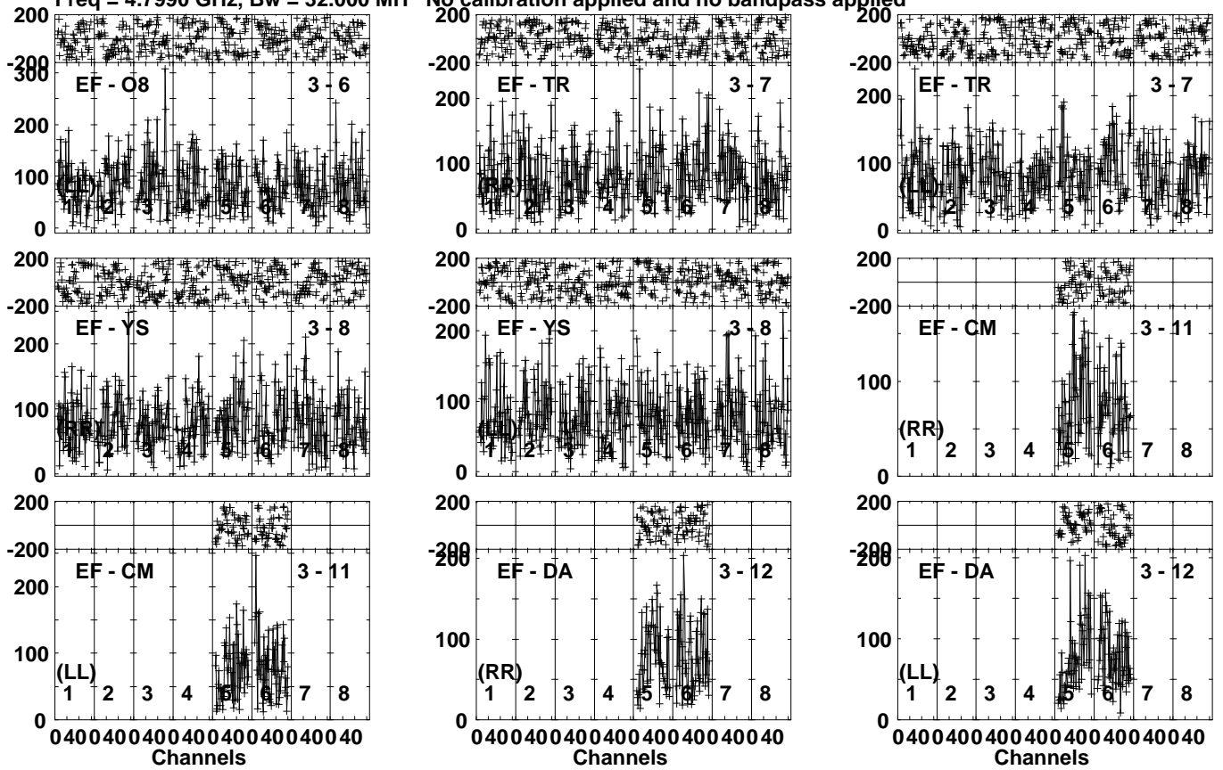
Lower frame: Micro Ampl Jy Top frame: Phas deg Vector averaged cross-power spectrum Several baselines displayed Timerange: 00/08:30:31 to 00/08:34:09
