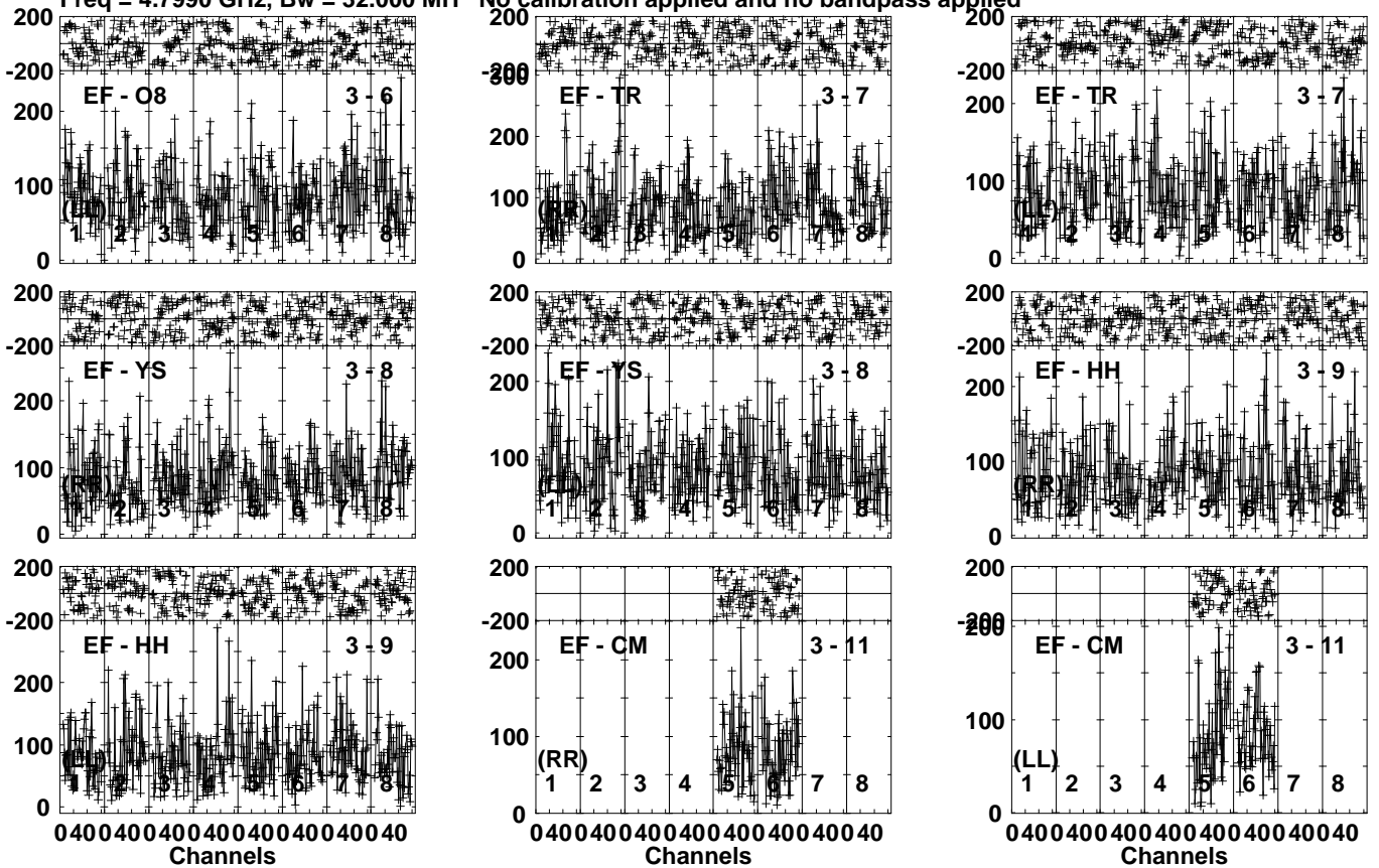
Lower frame: Micro Ampl Jy Top frame: Phas deg Vector averaged cross-power spectrum Several baselines displayed Timerange: 00/09:08:01 to 00/09:11:39
