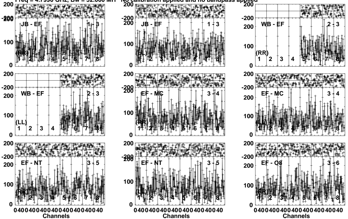
Lower frame: Micro Ampl Jy Top frame: Phas deg Vector averaged cross-power spectrum Several baselines displayed Timerange: 00/05:42:51 to 00/05:46:29
