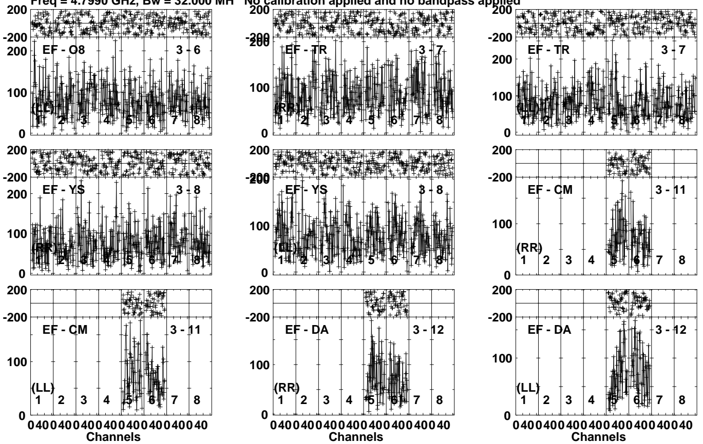
Lower frame: Micro Ampl Jy Top frame: Phas deg Vector averaged cross-power spectrum Several baselines displayed Timerange: 00/08:51:51 to 00/08:55:29
