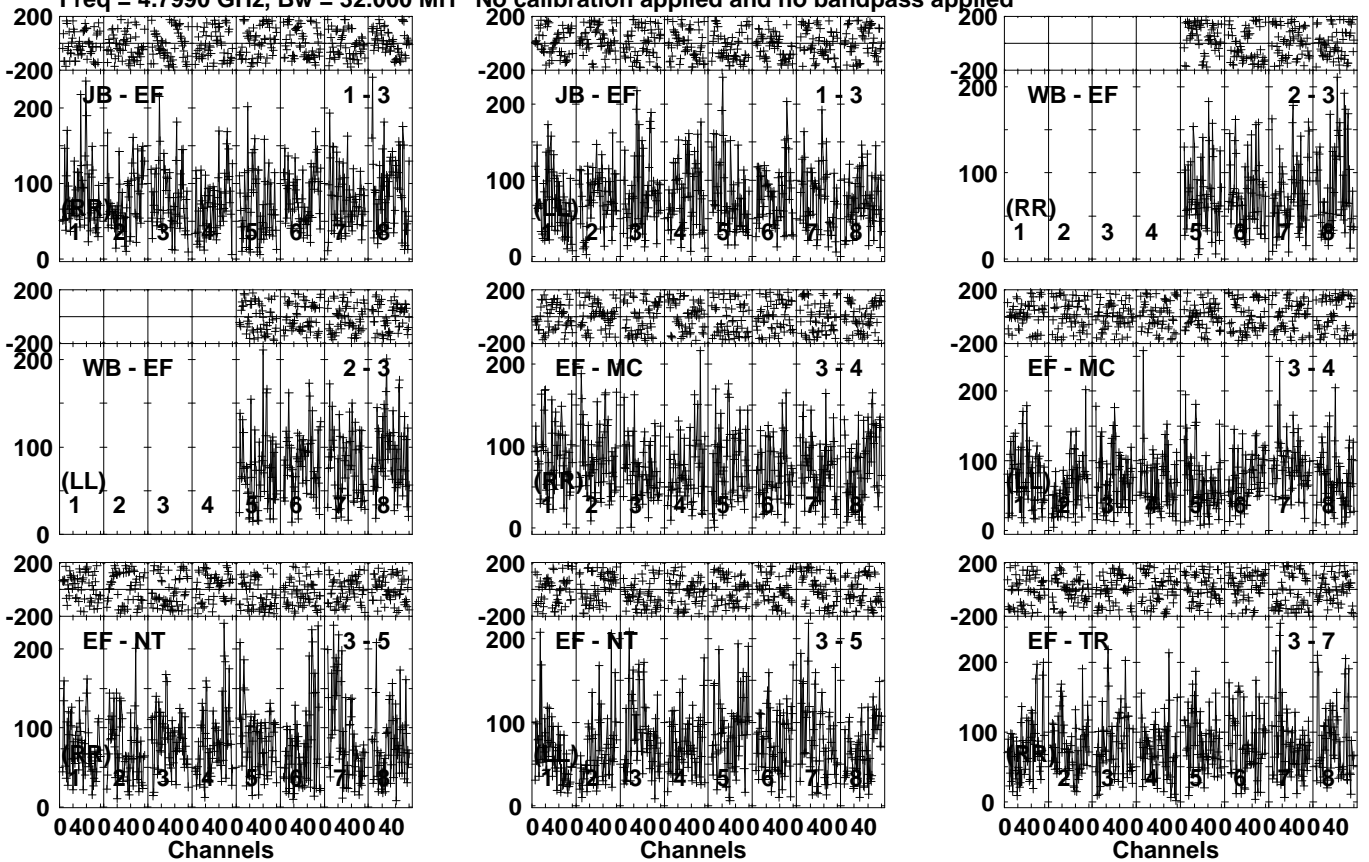
Lower frame: Micro Ampl Jy Top frame: Phas deg Vector averaged cross-power spectrum Several baselines displayed Timerange: 00/03:30:51 to 00/03:34:29
