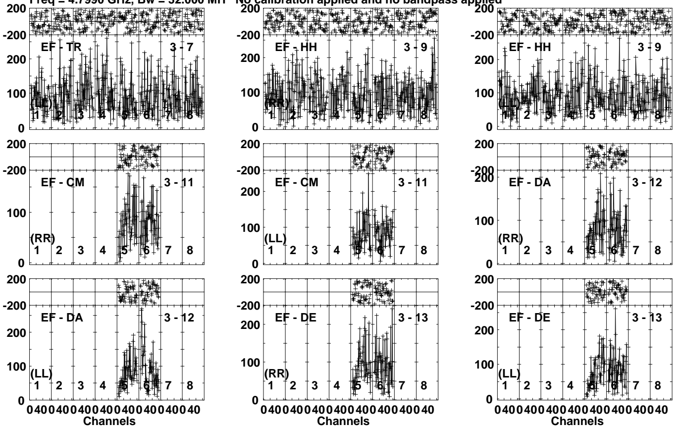
Lower frame: Micro Ampl Jy Top frame: Phas deg Vector averaged cross-power spectrum Several baselines displayed Timerange: 00/04:12:31 to 00/04:15:29
