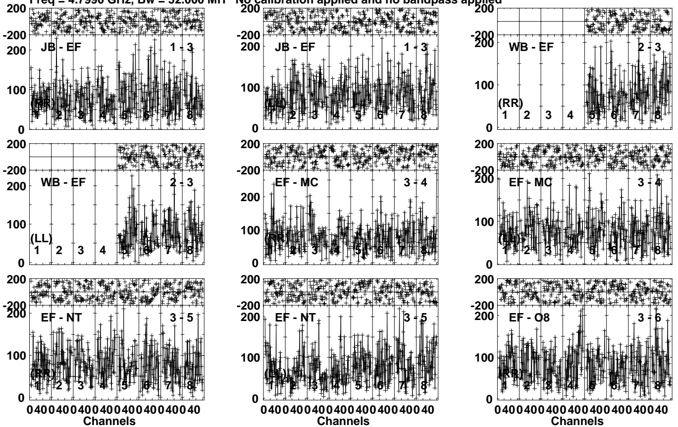
Lower frame: Micro Ampl Jy Top frame: Phas deg Vector averaged cross-power spectrum Several baselines displayed Timerange: 00/10:38:41 to 00/10:42:19
