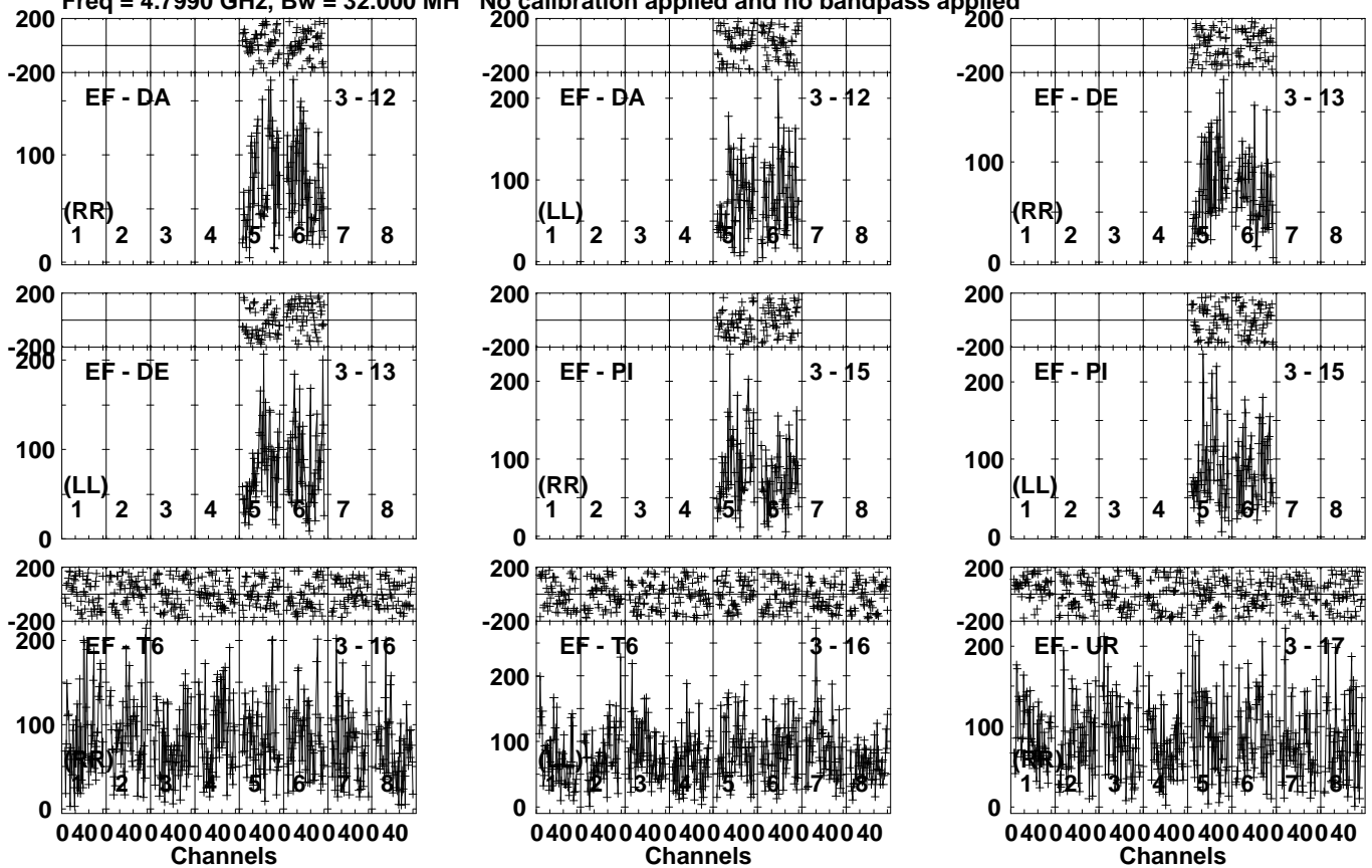
Lower frame: Micro Ampl Jy Top frame: Phas deg Vector averaged cross-power spectrum Several baselines displayed Timerange: 00/07:21:31 to 00/07:25:09
