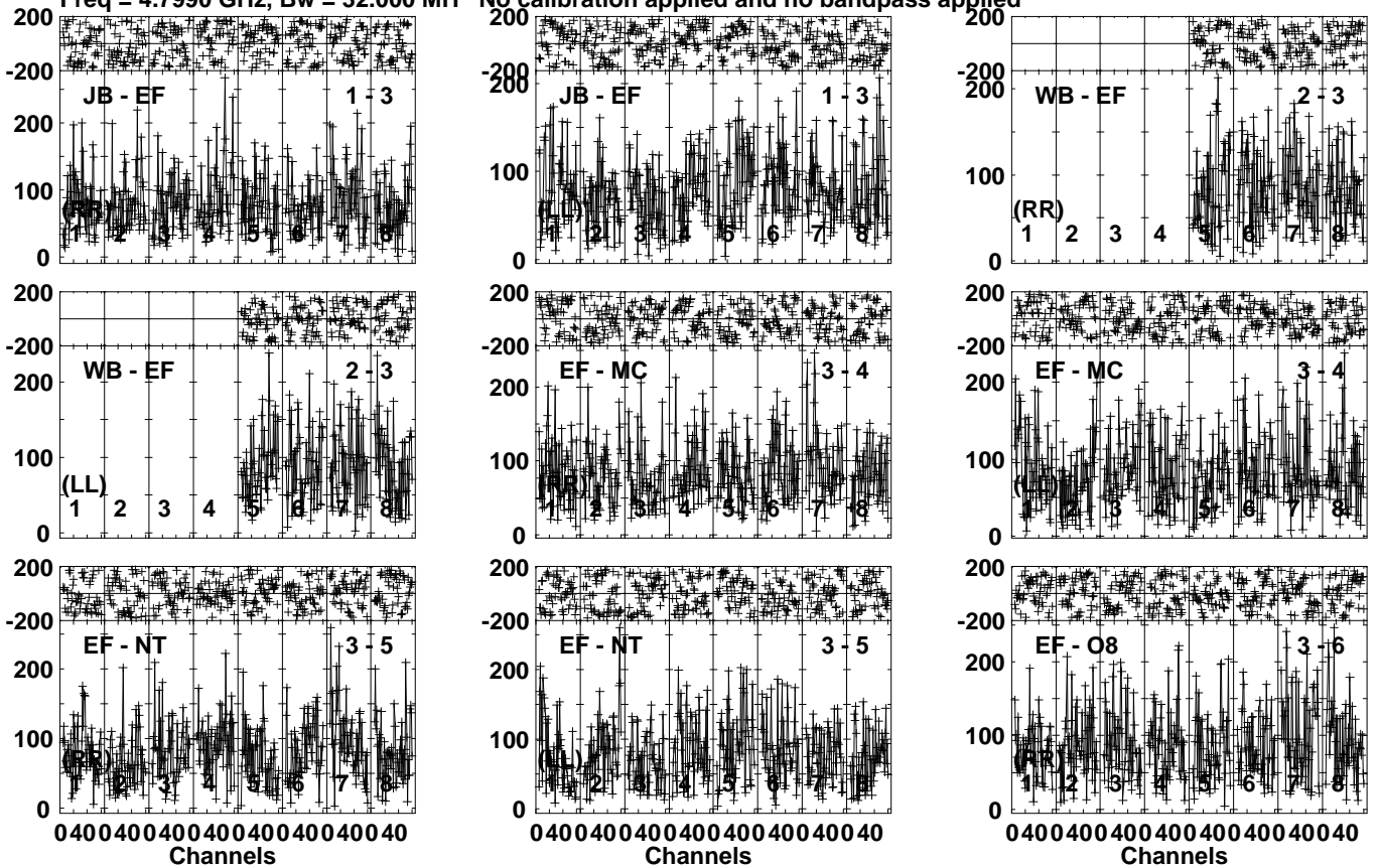
Lower frame: Micro Ampl Jy Top frame: Phas deg Vector averaged cross-power spectrum Several baselines displayed Timerange: 00/09:18:41 to 00/09:22:19
