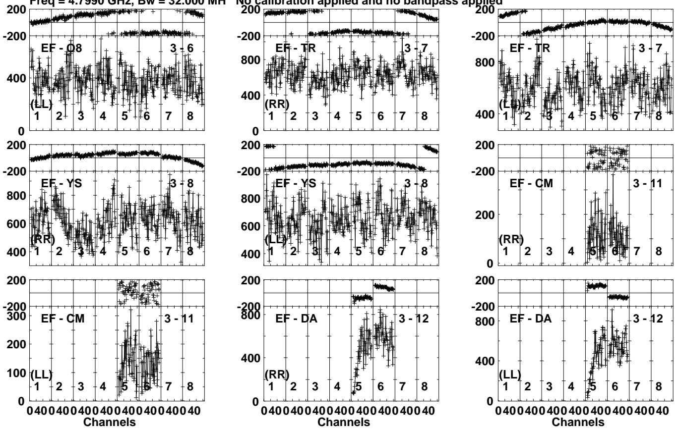
Lower frame: Micro Ampl Jy Top frame: Phas deg Vector averaged cross-power spectrum Several baselines displayed Timerange: 00/10:31:41 to 00/10:33:39
