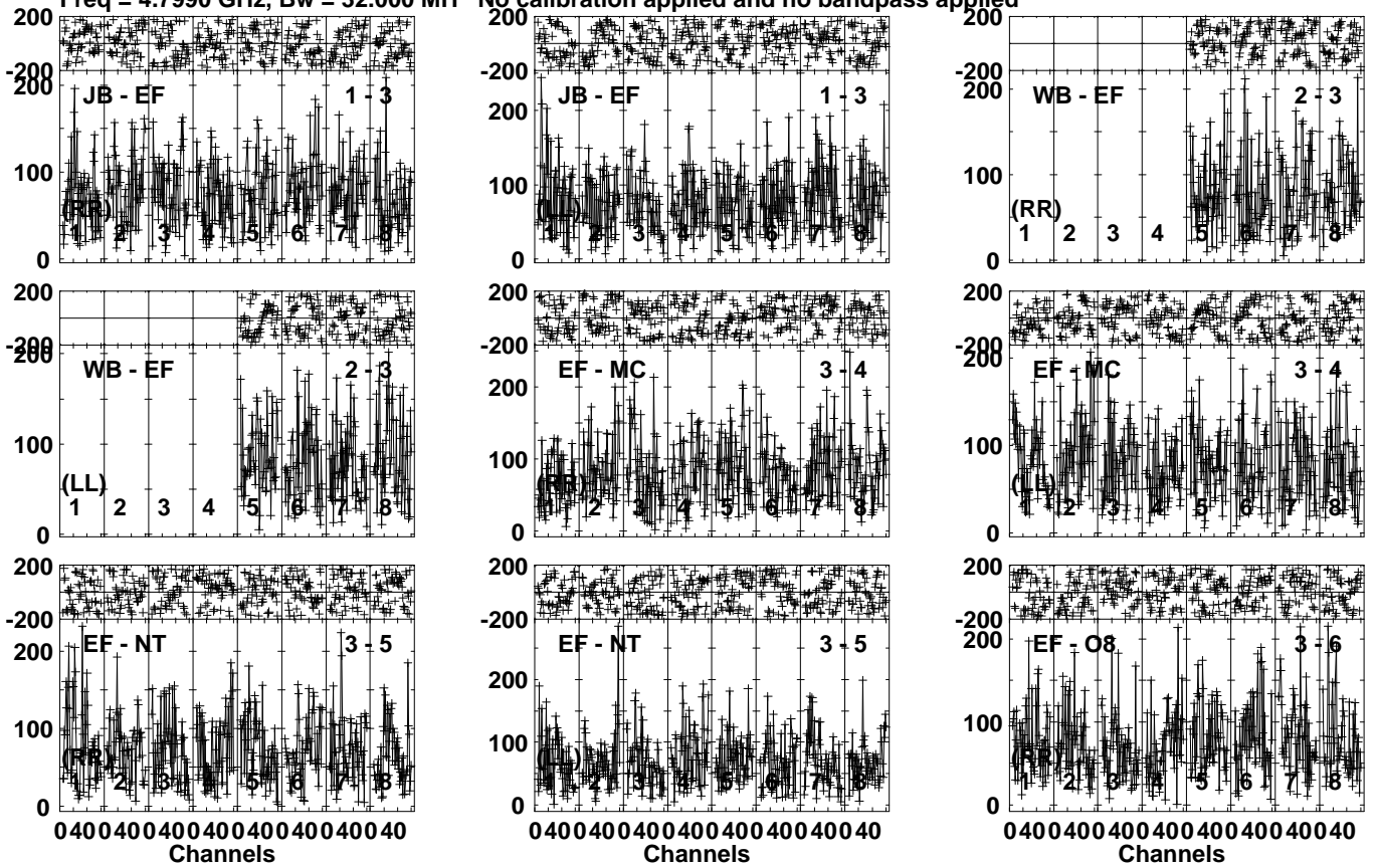
Lower frame: Micro Ampl Jy Top frame: Phas deg Vector averaged cross-power spectrum Several baselines displayed Timerange: 00/08:09:11 to 00/08:12:49
