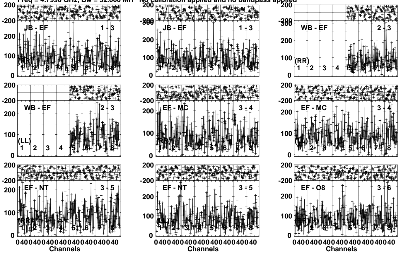
Lower frame: Micro Ampl Jy Top frame: Phas deg Vector averaged cross-power spectrum Several baselines displayed Timerange: 00/05:48:31 to 00/05:51:29
