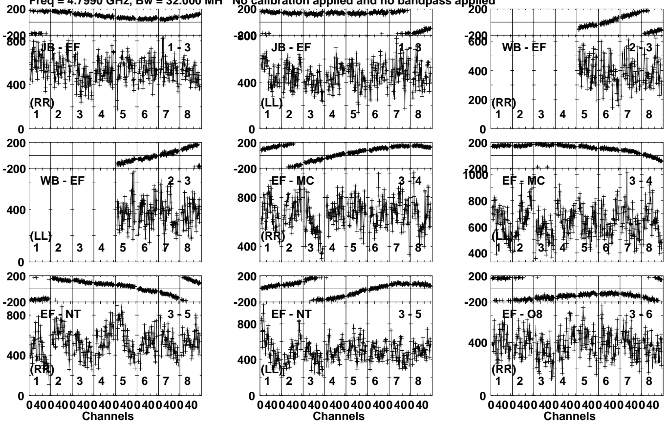
Lower frame: Micro Ampl Jy Top frame: Phas deg Vector averaged cross-power spectrum Several baselines displayed Timerange: 00/08:18:21 to 00/08:19:49
