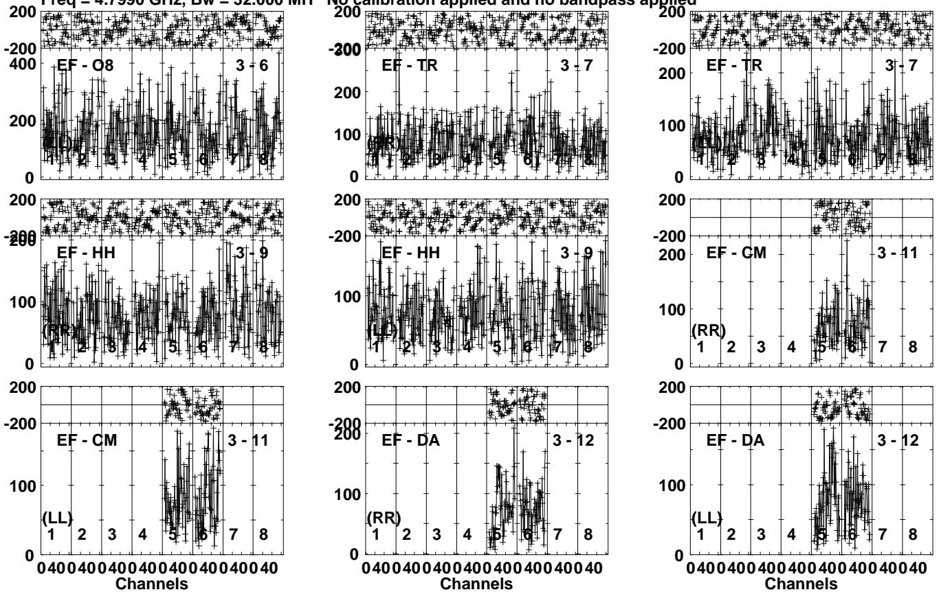
Lower frame: Micro Ampl Jy Top frame: Phas deg Vector averaged cross-power spectrum Several baselines displayed Timerange: 00/03:09:31 to 00/03:13:09
