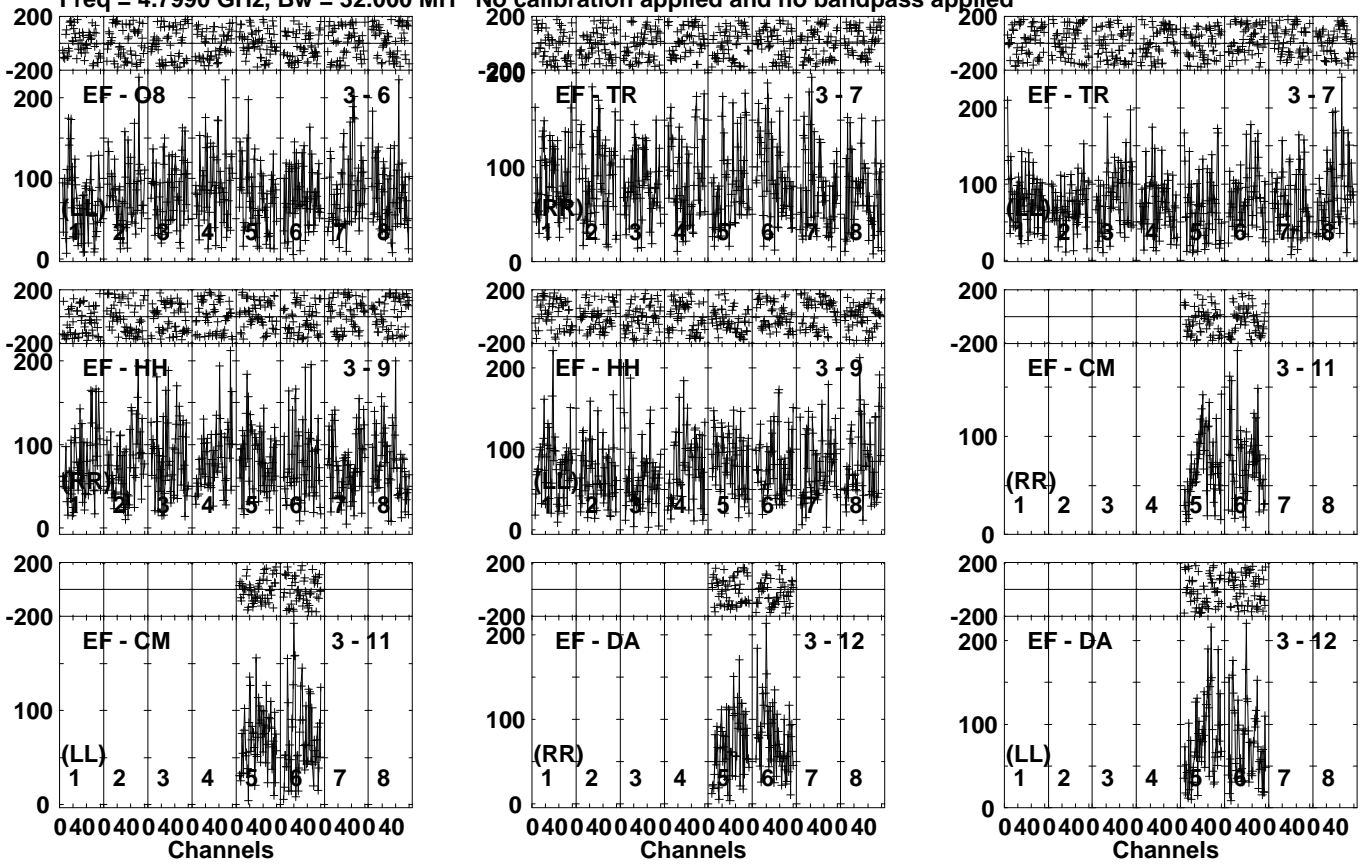
Lower frame: Micro Ampl Jy Top frame: Phas deg Vector averaged cross-power spectrum Several baselines displayed Timerange: 00/04:38:51 to 00/04:42:29
