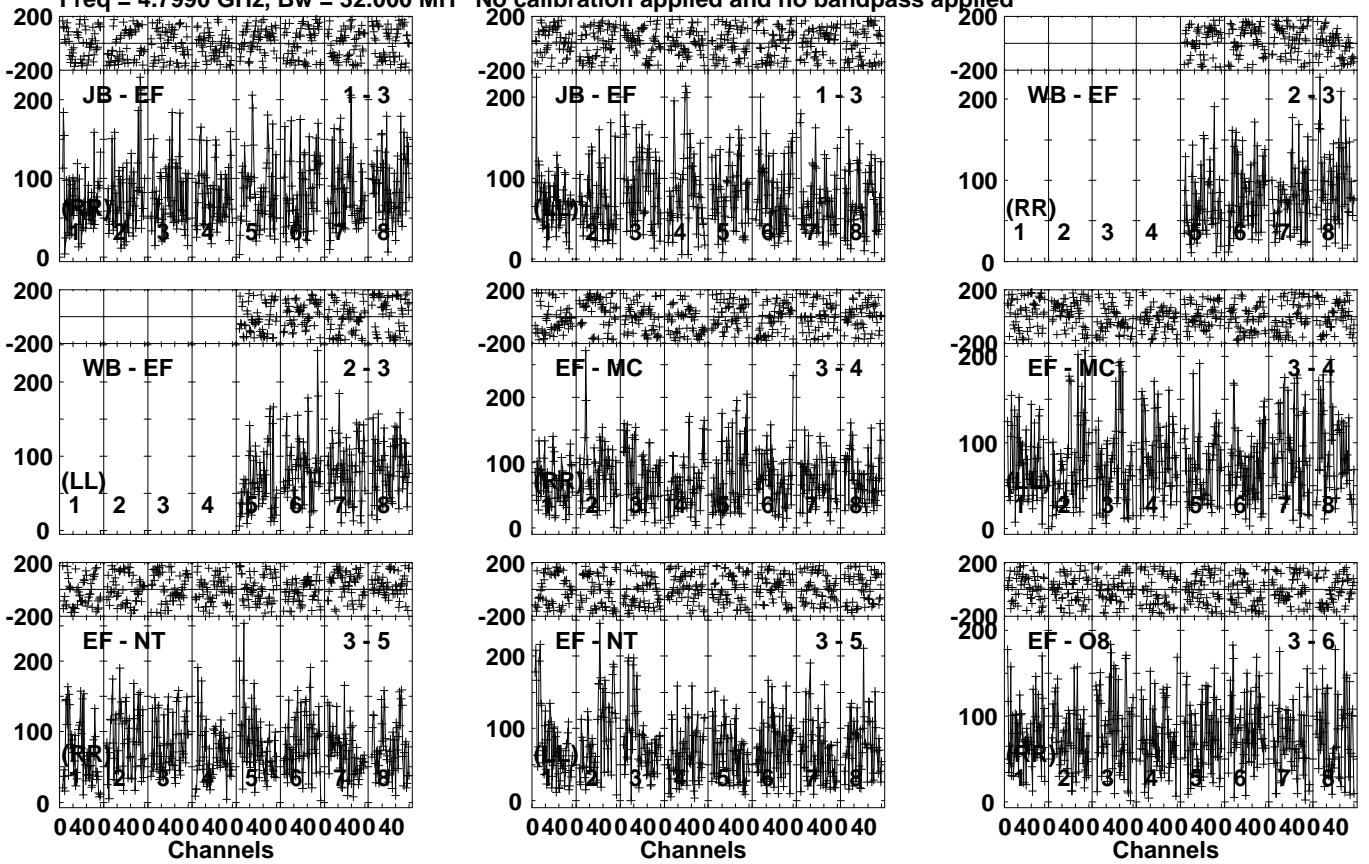
Lower frame: Micro Ampl Jy Top frame: Phas deg Vector averaged cross-power spectrum Several baselines displayed Timerange: 00/06:48:41 to 00/06:52:19
