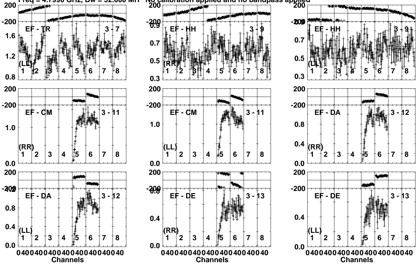
Lower frame: Milli Ampl Jy Top frame: Phas deg Vector averaged cross-power spectrum Several baselines displayed Timerange: 00/03:23:51 to 00/03:25:49
