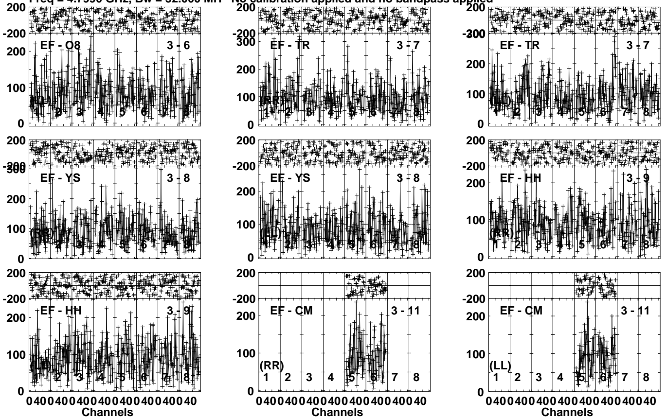
Lower frame: Micro Ampl Jy Top frame: Phas deg Vector averaged cross-power spectrum Several baselines displayed Timerange: 00/07:48:31 to 00/07:51:29
