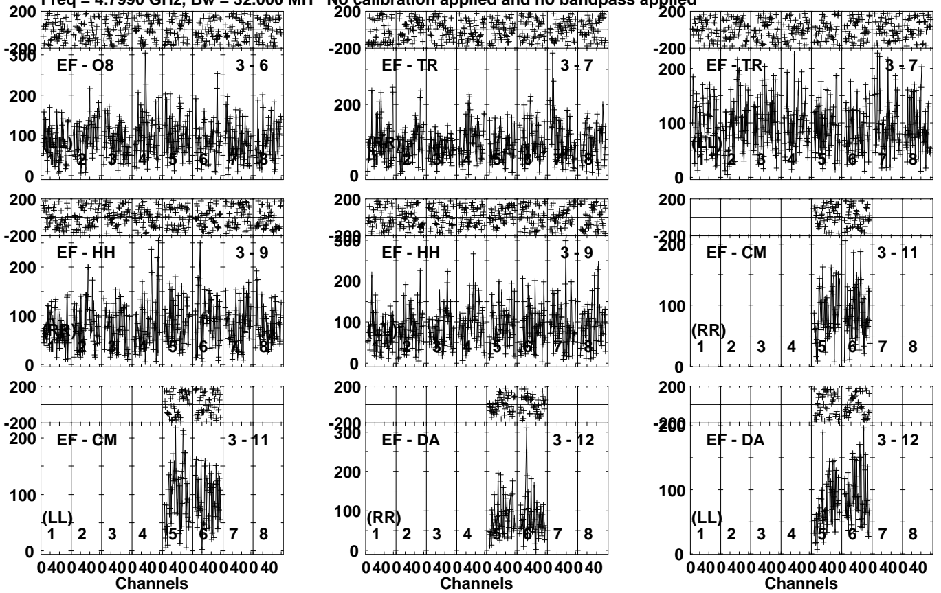
Lower frame: Micro Ampl Jy Top frame: Phas deg Vector averaged cross-power spectrum Several baselines displayed Timerange: 00/04:44:31 to 00/04:47:29
