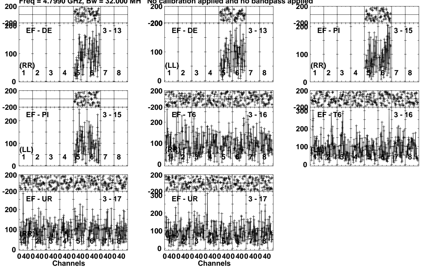
Lower frame: Micro Ampl Jy Top frame: Phas deg Vector averaged cross-power spectrum Several baselines displayed Timerange: 00/10:23:01 to 00/10:25:59
