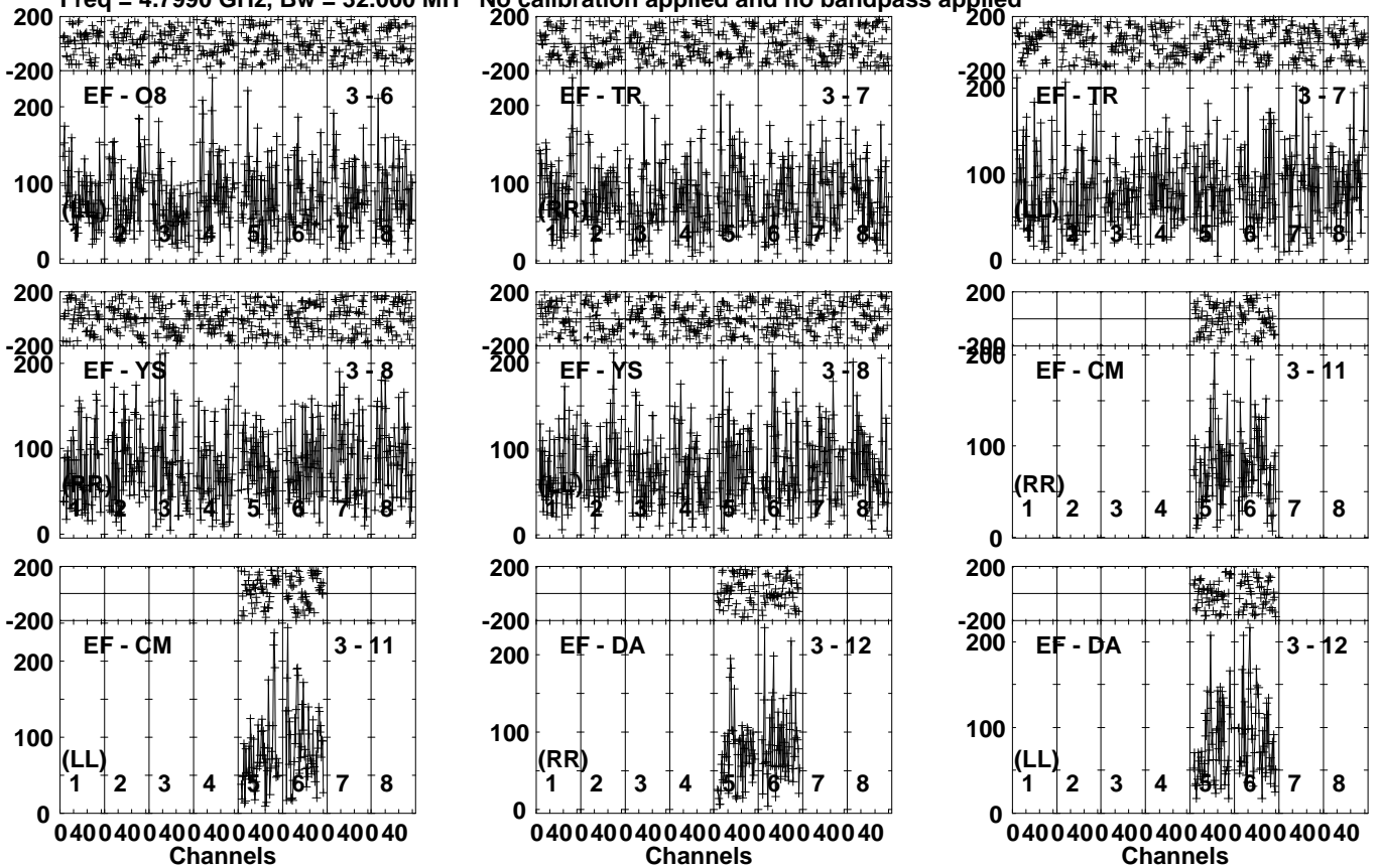
Lower frame: Micro Ampl Jy Top frame: Phas deg Vector averaged cross-power spectrum Several baselines displayed Timerange: 00/08:19:51 to 00/08:23:29
