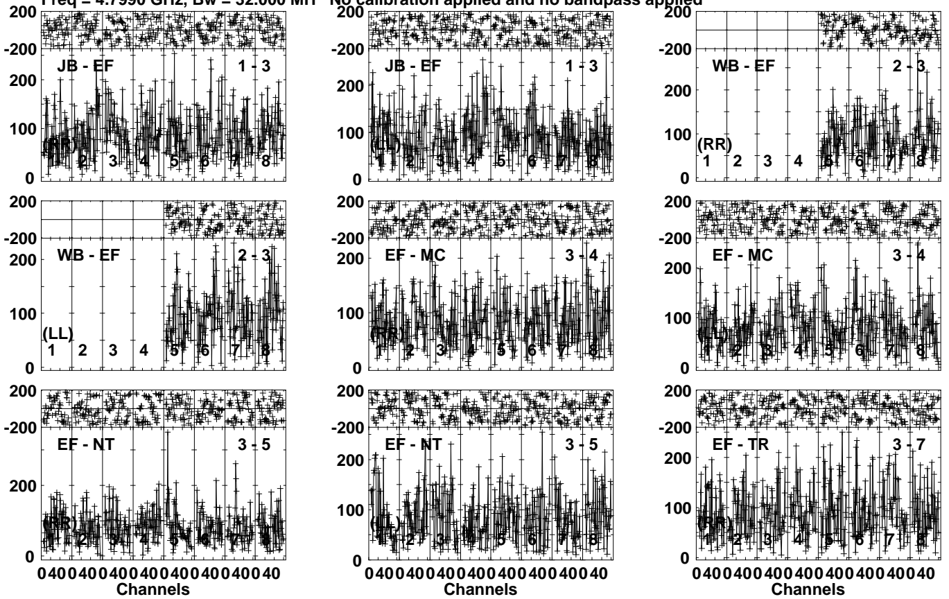
Lower frame: Micro Ampl Jy Top frame: Phas deg Vector averaged cross-power spectrum Several baselines displayed Timerange: 00/03:57:51 to 00/04:00:49
