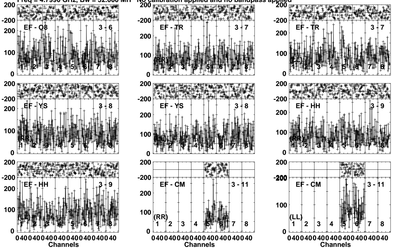
Lower frame: Micro Ampl Jy Top frame: Phas deg Vector averaged cross-power spectrum Several baselines displayed Timerange: 00/09:40:01 to 00/09:43:39
