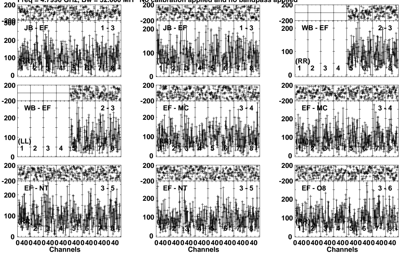
Lower frame: Micro Ampl Jy Top frame: Phas deg Vector averaged cross-power spectrum Several baselines displayed Timerange: 00/09:56:21 to 00/09:59:19
