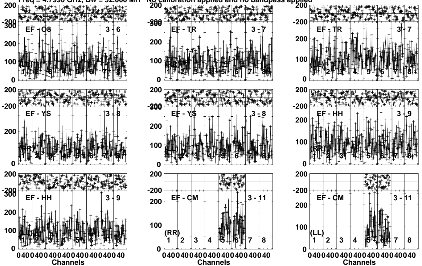
Lower frame: Micro Ampl Jy Top frame: Phas deg Vector averaged cross-power spectrum Several baselines displayed Timerange: 00/09:13:41 to 00/09:16:39
