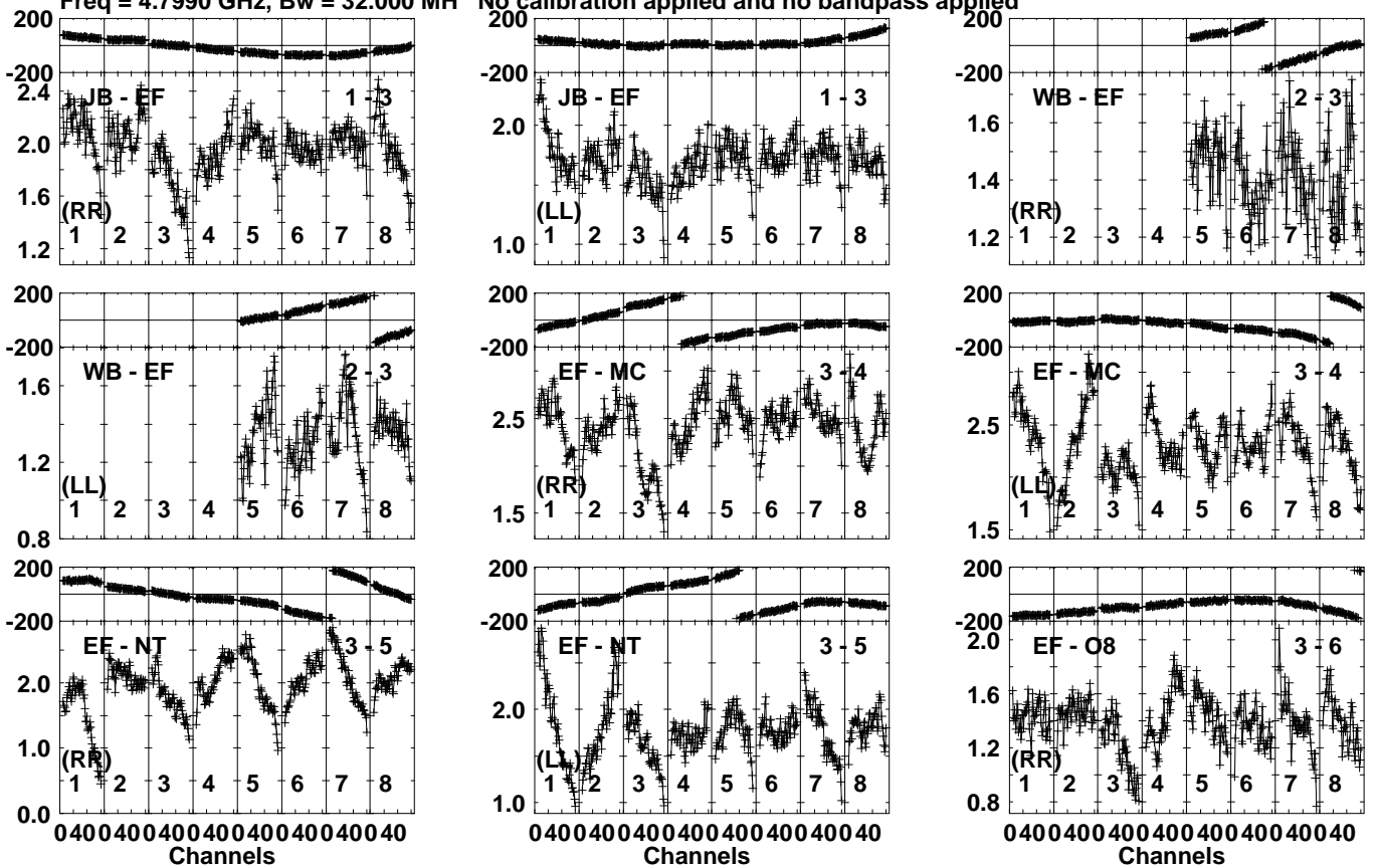
Lower frame: Milli Ampl Jy Top frame: Phas deg Vector averaged cross-power spectrum Several baselines displayed Timerange: 00/07:57:11 to 00/07:59:09
