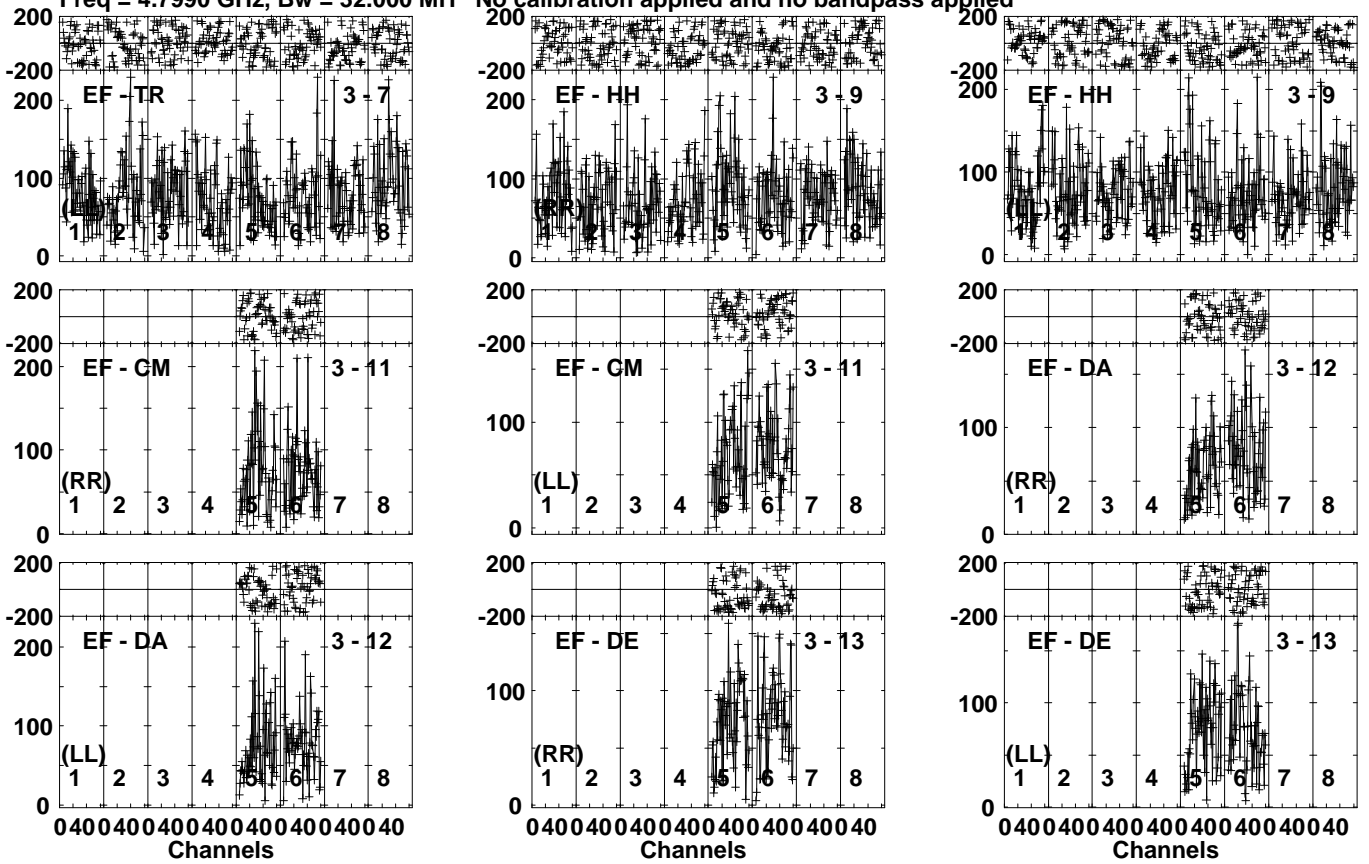
Lower frame: Micro Ampl Jy Top frame: Phas deg Vector averaged cross-power spectrum Several baselines displayed Timerange: 00/03:20:11 to 00/03:23:49
