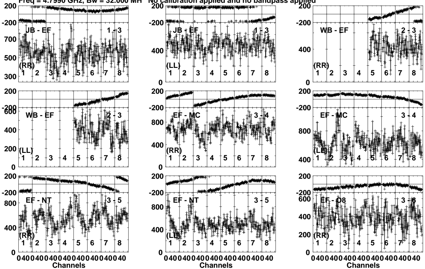
Lower frame: Micro Ampl Jy Top frame: Phas deg Vector averaged cross-power spectrum Several baselines displayed Timerange: 00/08:34:11 to 00/08:36:09
