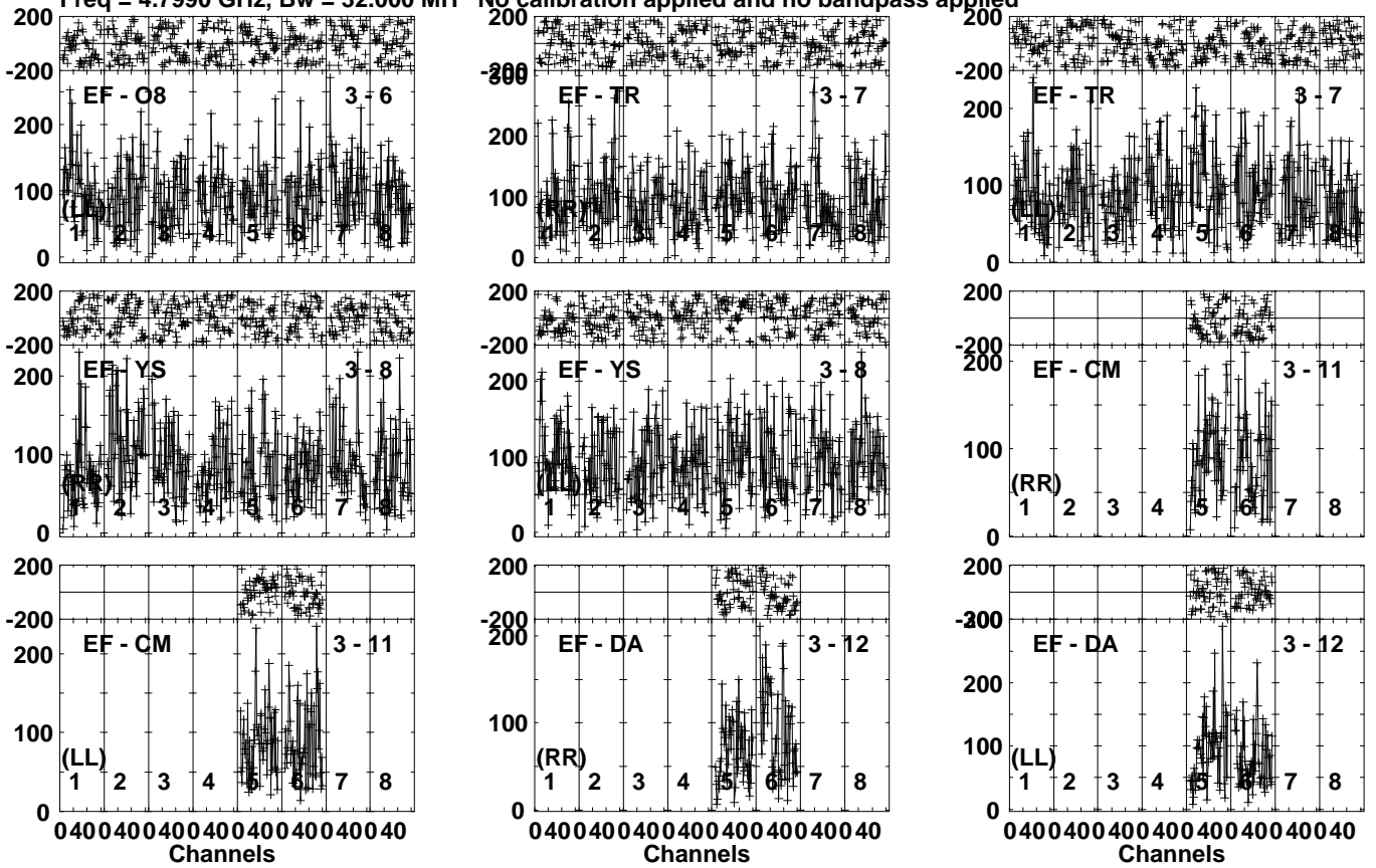
Lower frame: Micro Ampl Jy Top frame: Phas deg Vector averaged cross-power spectrum Several baselines displayed Timerange: 00/10:12:21 to 00/10:15:19
