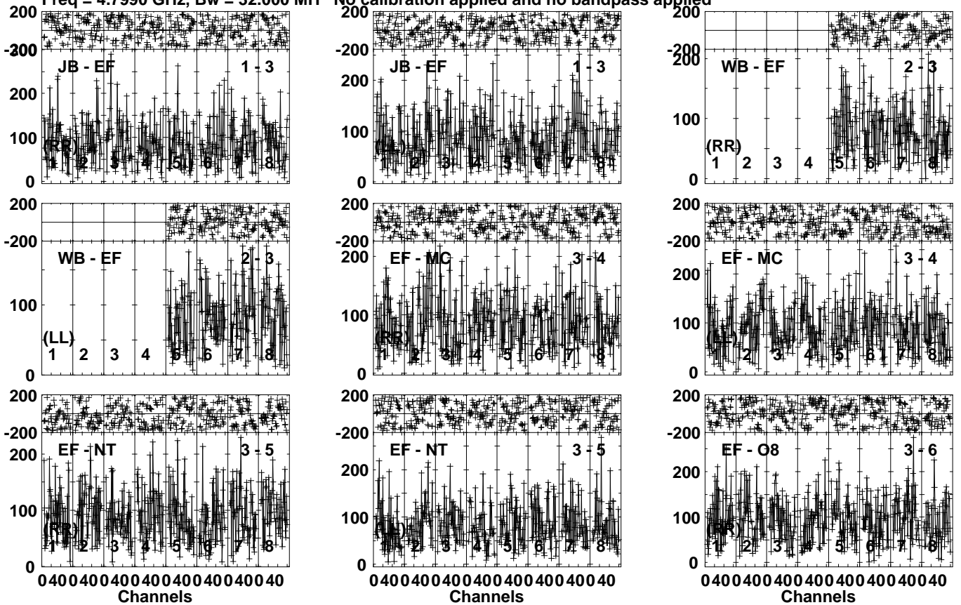
Lower frame: Micro Ampl Jy Top frame: Phas deg Vector averaged cross-power spectrum Several baselines displayed Timerange: 00/06:54:21 to 00/06:57:19
