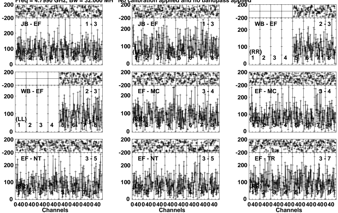
Lower frame: Micro Ampl Jy Top frame: Phas deg Vector averaged cross-power spectrum Several baselines displayed Timerange: 00/03:36:31 to 00/03:39:29
