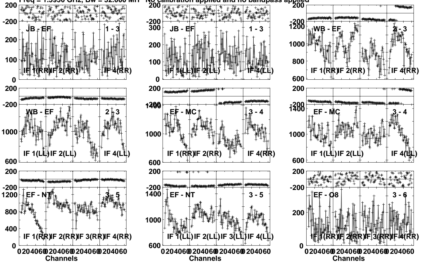
Lower frame: Micro Ampl Jy Top frame: Phas deg Vector averaged cross-power spectrum Several baselines displayed Timerange: 00/02:54:26 to 00/02:56:24
