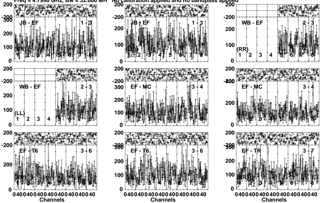
Lower frame: Micro Ampl Jy Top frame: Phas deg Vector averaged cross-power spectrum Several baselines displayed Timerange: 00/23:36:31 to 00/23:38:59
