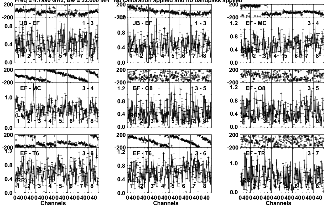
Lower frame: Milli Ampl Jy Top frame: Phas deg Vector averaged cross-power spectrum Several baselines displayed Timerange: 00/20:24:01 to 00/20:24:59
