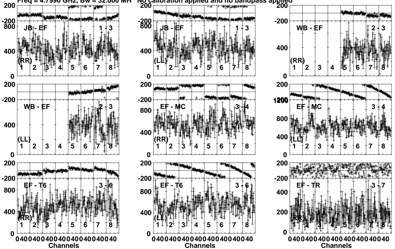
Lower frame: Micro Ampl Jy Top frame: Phas deg Vector averaged cross-power spectrum Several baselines displayed Timerange: 00/21:47:01 to 00/21:47:59
