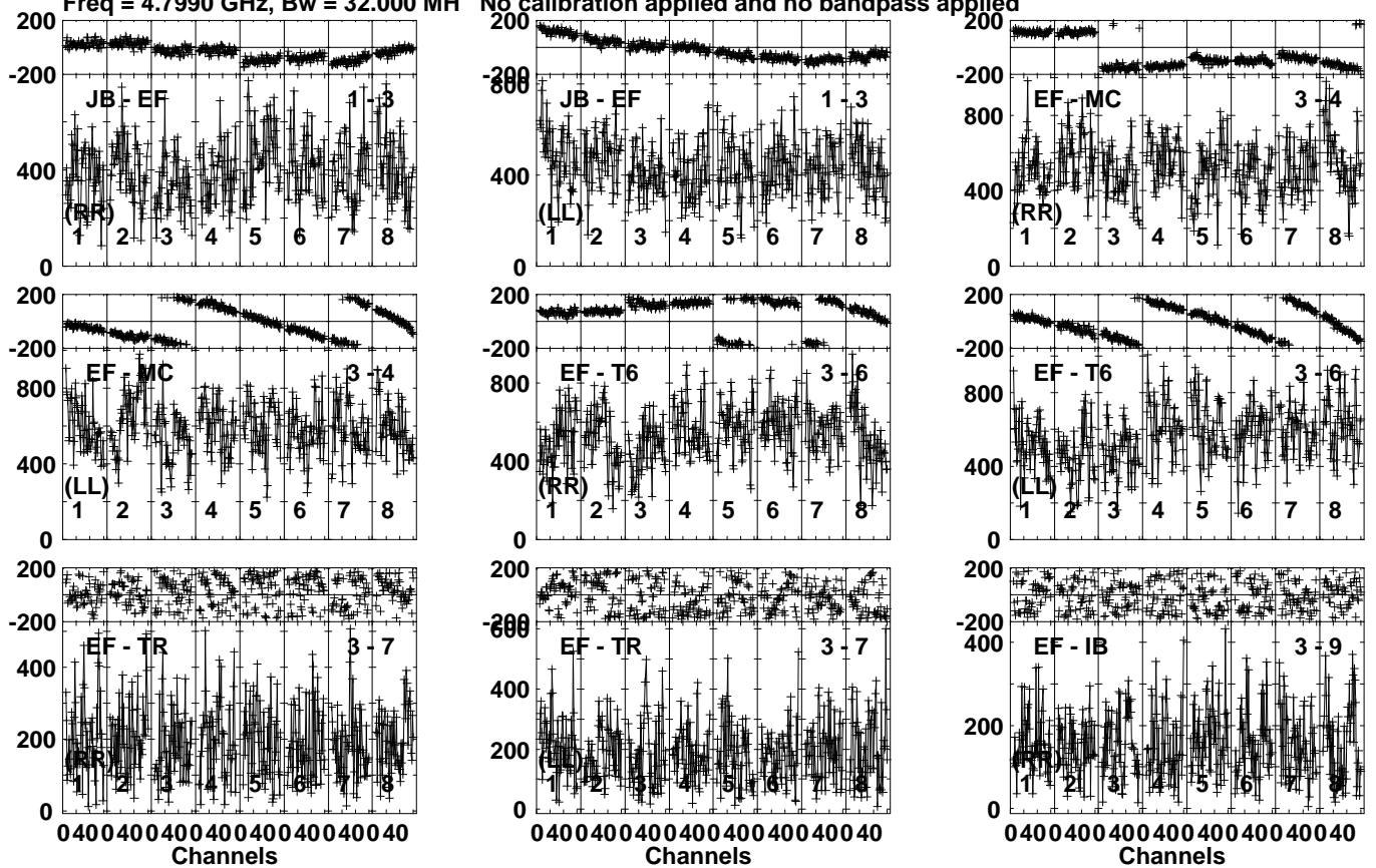
Lower frame: Micro Ampl Jy Top frame: Phas deg Vector averaged cross-power spectrum Several baselines displayed Timerange: 00/20:47:31 to 00/20:48:29
