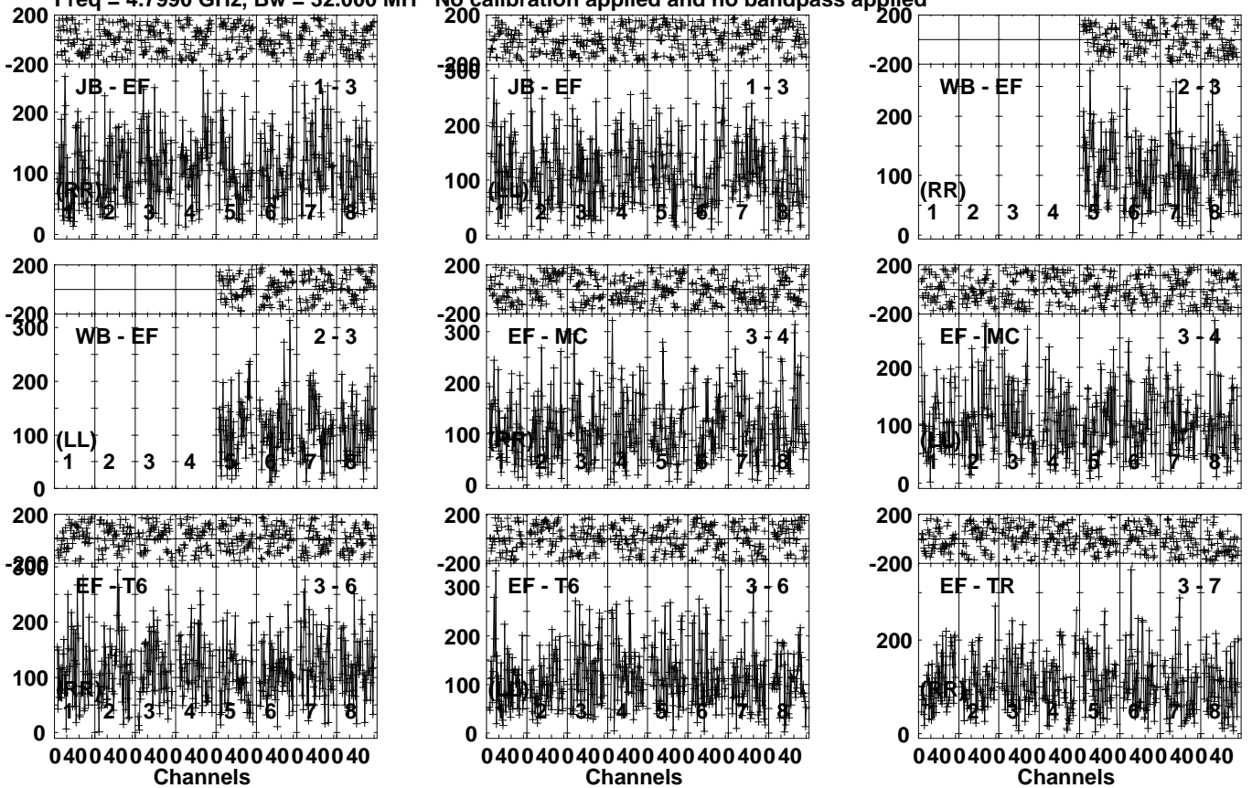
Lower frame: Micro Ampl Jy Top frame: Phas deg Vector averaged cross-power spectrum Several baselines displayed Timerange: 00/23:14:01 to 00/23:16:29
