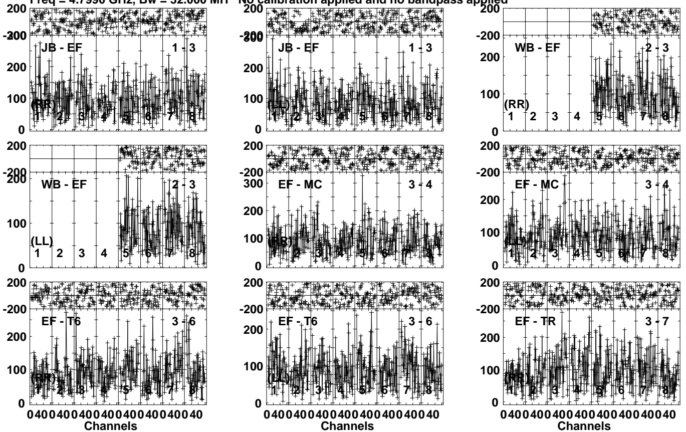
Lower frame: Micro Ampl Jy Top frame: Phas deg Vector averaged cross-power spectrum Several baselines displayed Timerange: 00/22:46:01 to 00/22:48:59
