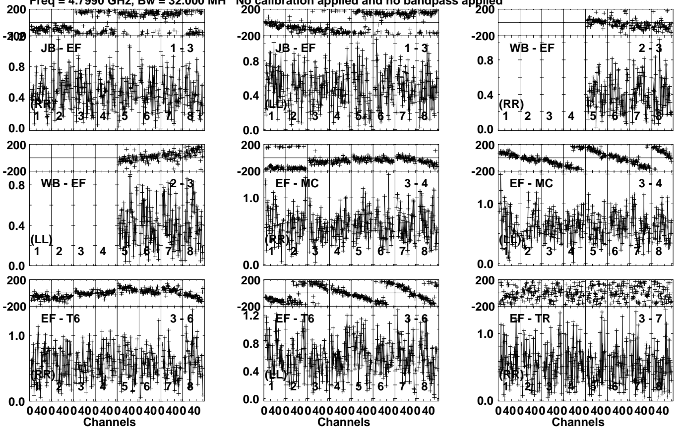
Lower frame: Milli Ampl Jy Top frame: Phas deg Vector averaged cross-power spectrum Several baselines displayed Timerange: 00/21:34:01 to 00/21:34:59
