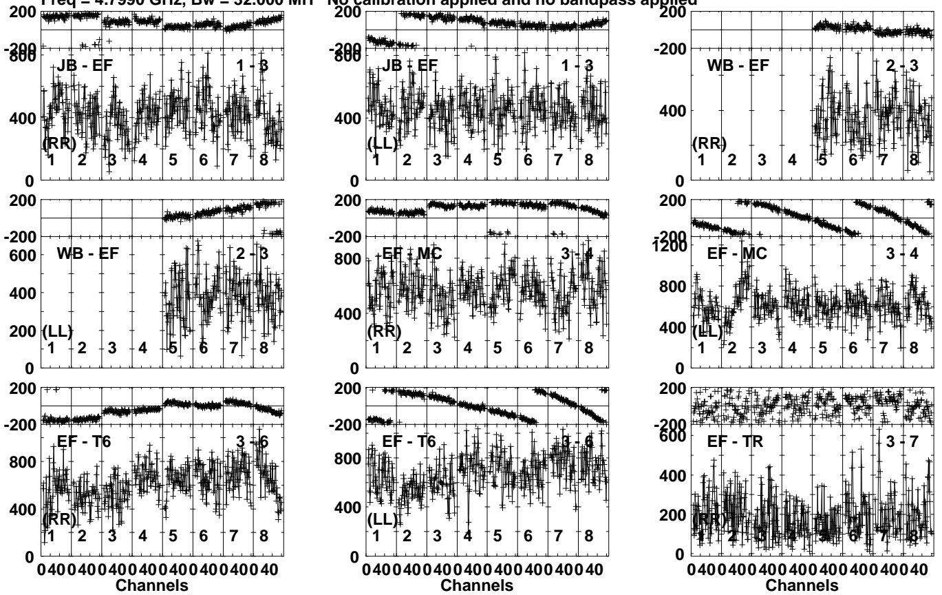
Lower frame: Micro Ampl Jy Top frame: Phas deg Vector averaged cross-power spectrum Several baselines displayed Timerange: 00/23:02:01 to 00/23:02:59
