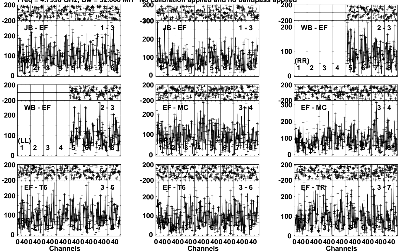
Lower frame: Micro Ampl Jy Top frame: Phas deg Vector averaged cross-power spectrum Several baselines displayed Timerange: 00/21:18:01 to 00/21:20:59
