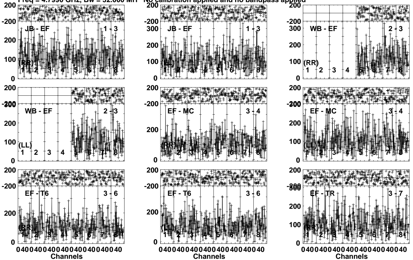
Lower frame: Micro Ampl Jy Top frame: Phas deg Vector averaged cross-power spectrum Several baselines displayed Timerange: 00/23:29:01 to 00/23:31:29
