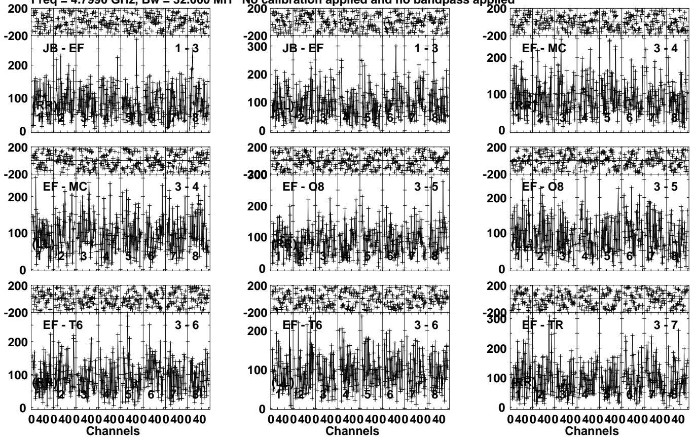
Lower frame: Micro Ampl Jy Top frame: Phas deg Vector averaged cross-power spectrum Several baselines displayed Timerange: 00/20:21:01 to 00/20:23:59
