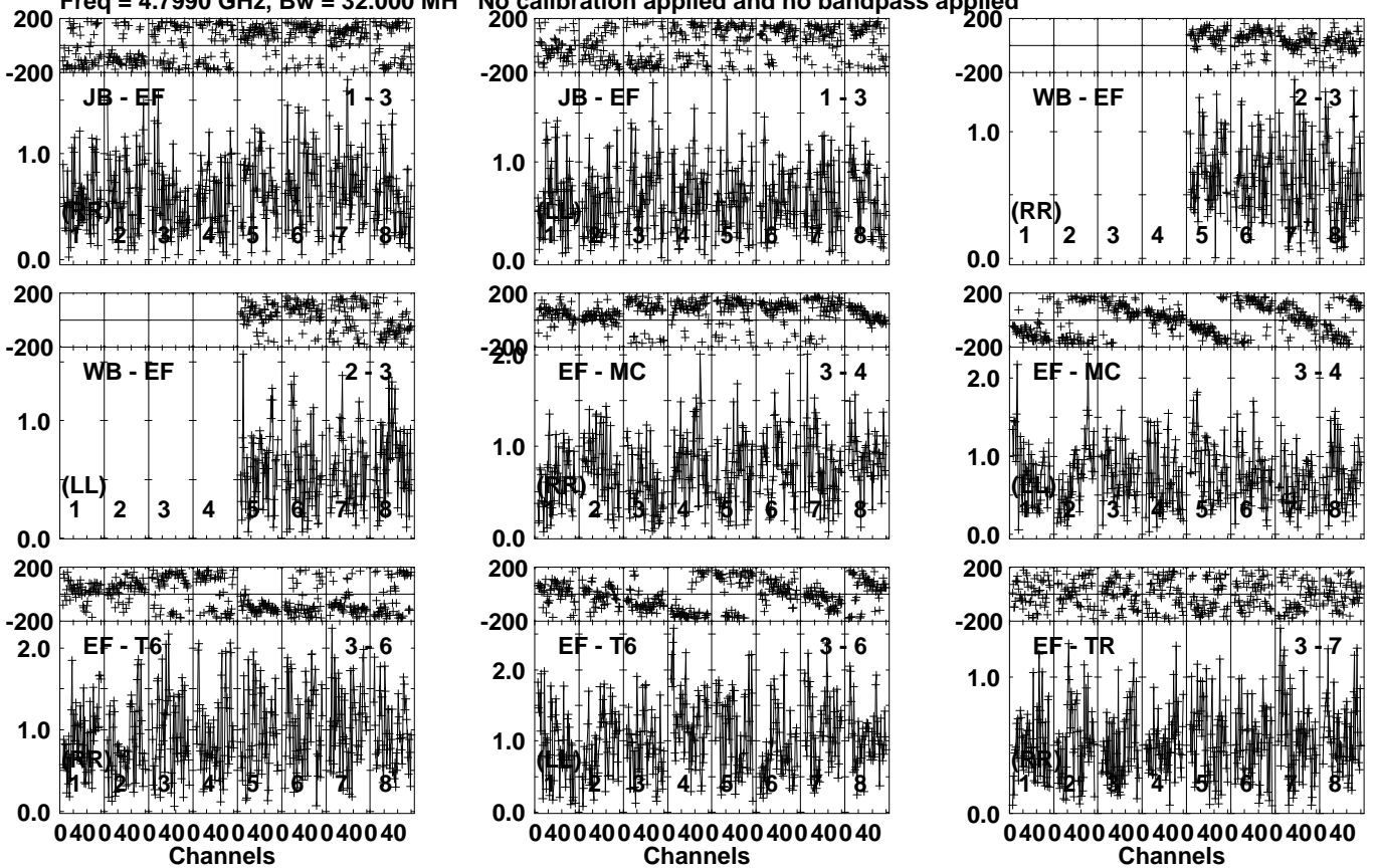
Lower frame: Milli Ampl Jy Top frame: Phas deg Vector averaged cross-power spectrum Several baselines displayed Timerange: 00/23:28:01 to 00/23:28:59
