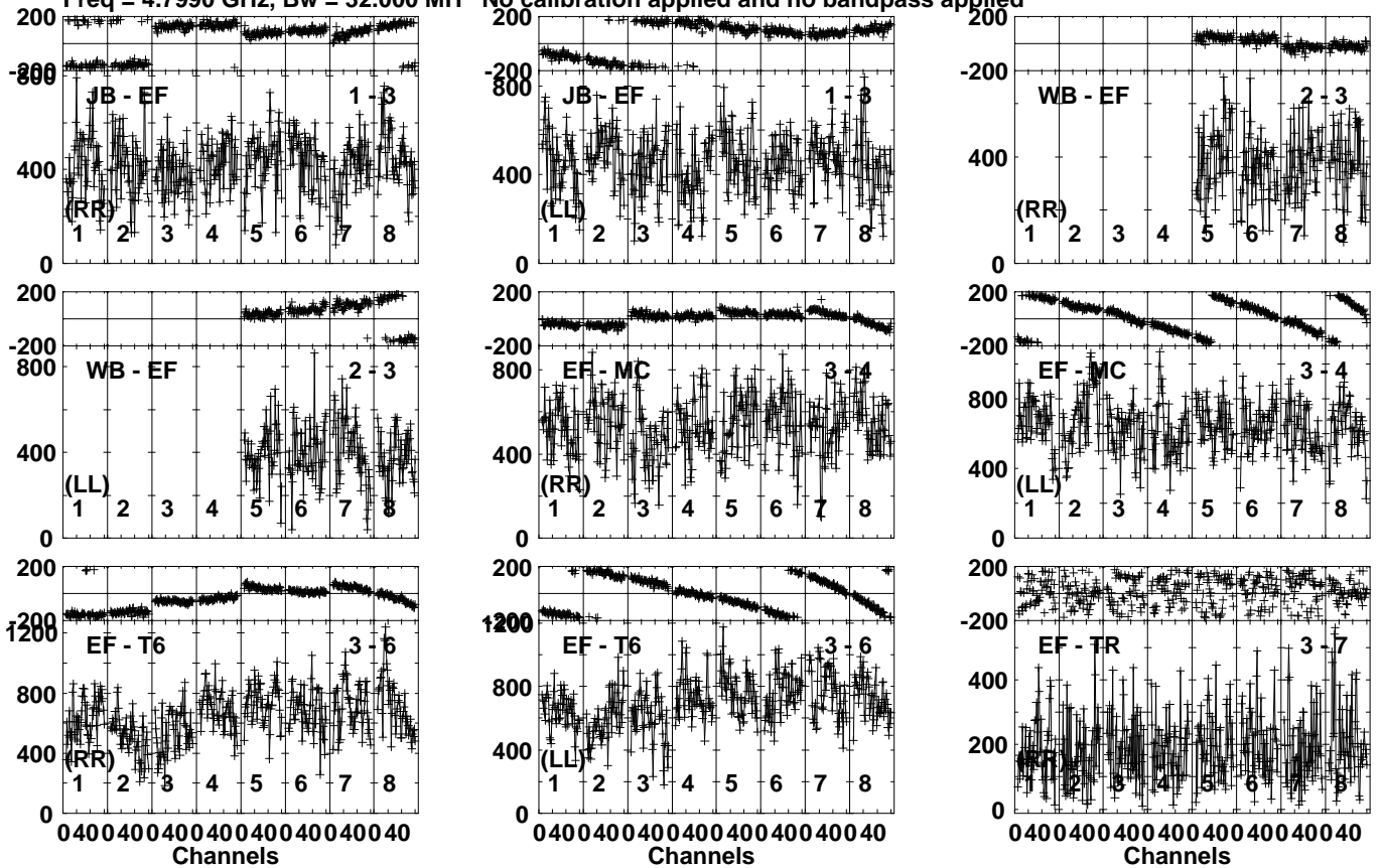
Lower frame: Micro Ampl Jy Top frame: Phas deg Vector averaged cross-power spectrum Several baselines displayed Timerange: 00/23:09:31 to 00/23:10:29
