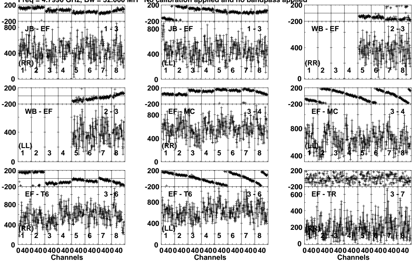
Lower frame: Micro Ampl Jy Top frame: Phas deg Vector averaged cross-power spectrum Several baselines displayed Timerange: 00/22:36:31 to 00/22:37:29
