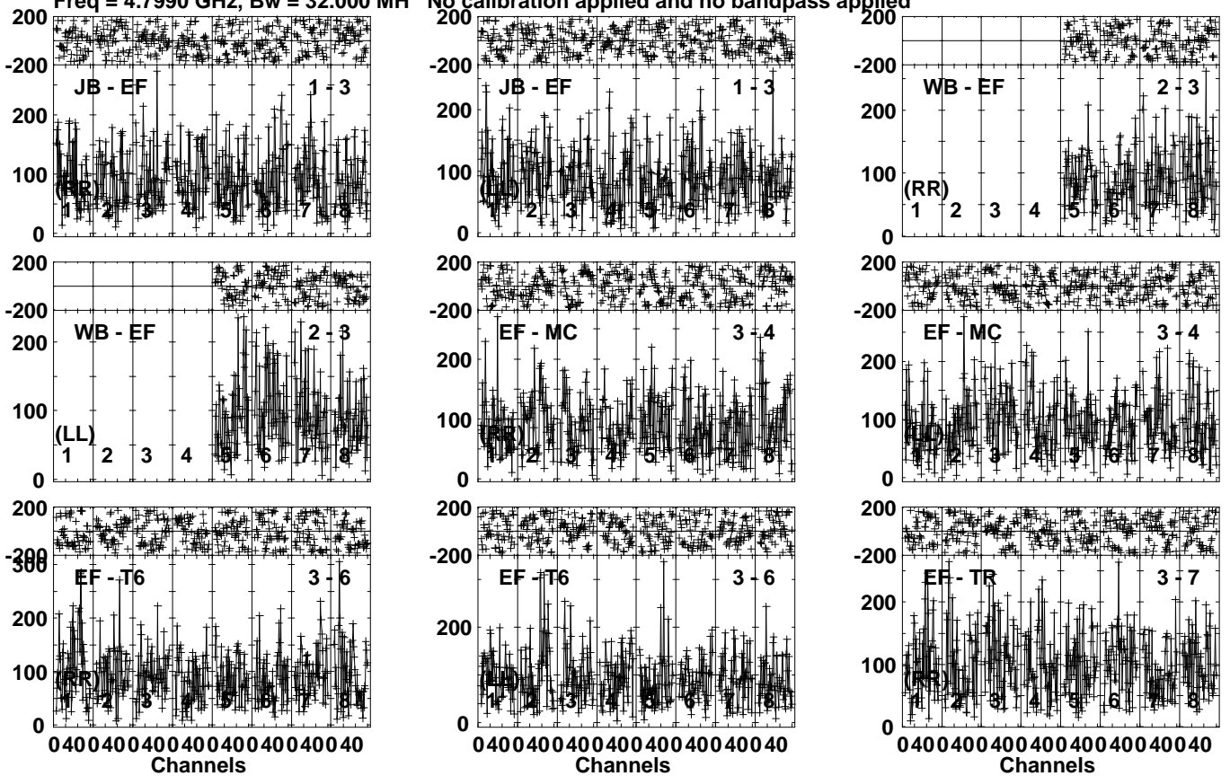
Lower frame: Micro Ampl Jy Top frame: Phas deg Vector averaged cross-power spectrum Several baselines displayed Timerange: 00/22:33:01 to 00/22:35:59
