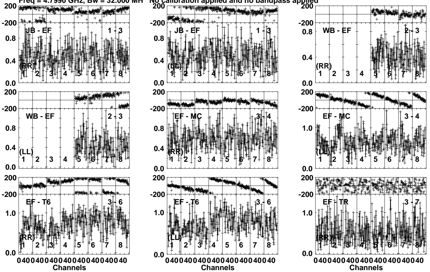
Lower frame: Milli Ampl Jy Top frame: Phas deg Vector averaged cross-power spectrum Several baselines displayed Timerange: 00/23:13:01 to 00/23:13:59
