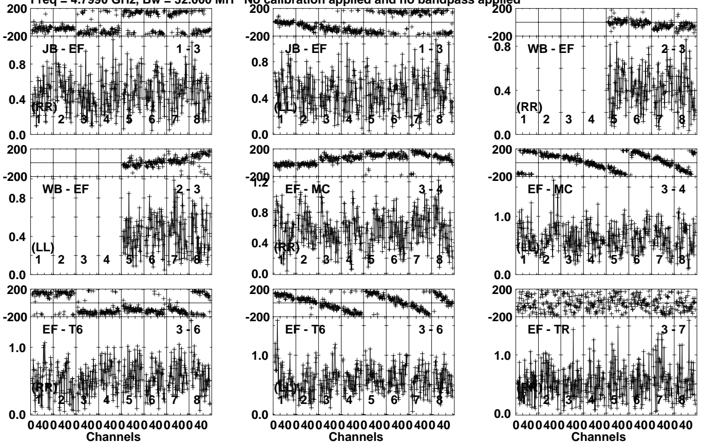
Lower frame: Milli Ampl Jy Top frame: Phas deg Vector averaged cross-power spectrum Several baselines displayed Timerange: 00/21:25:31 to 00/21:26:29
