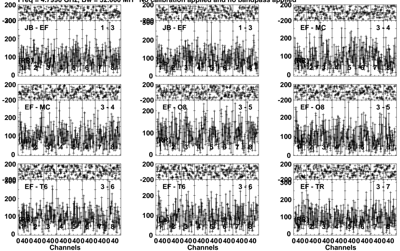
Lower frame: Micro Ampl Jy Top frame: Phas deg Vector averaged cross-power spectrum Several baselines displayed Timerange: 00/20:08:01 to 00/20:10:59
