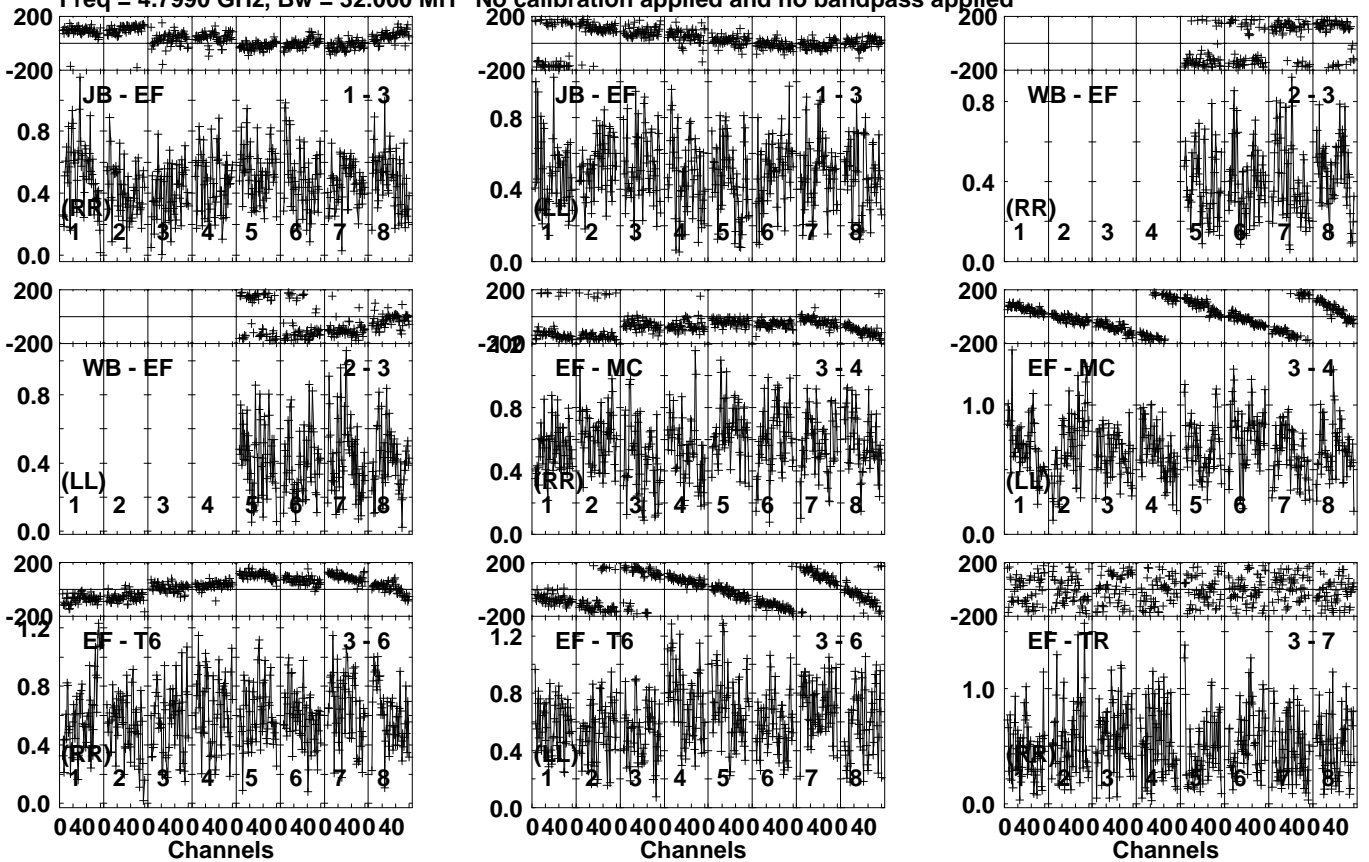
Lower frame: Milli Ampl Jy Top frame: Phas deg Vector averaged cross-power spectrum Several baselines displayed Timerange: 00/22:23:31 to 00/22:24:29
