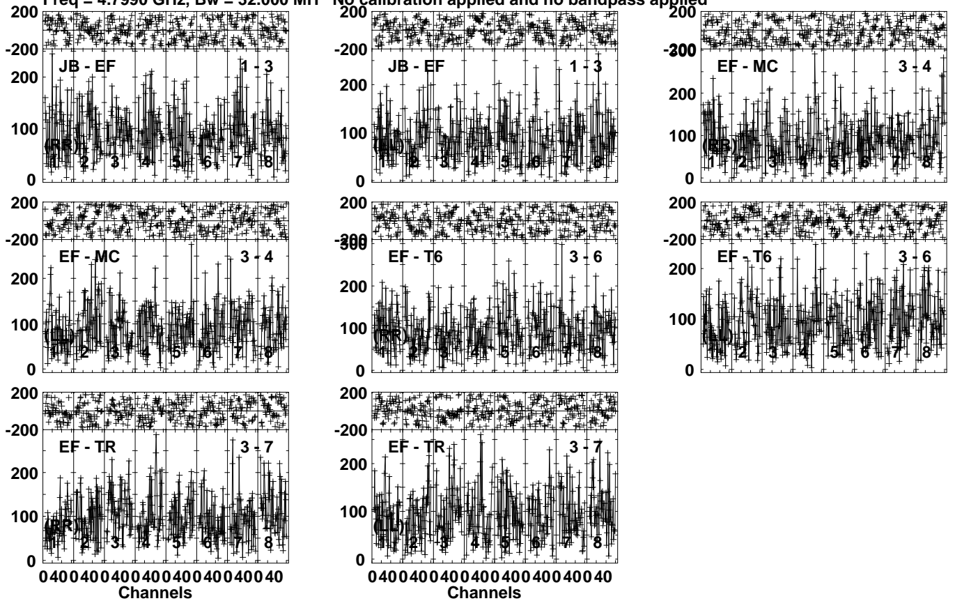
Lower frame: Micro Ampl Jy Top frame: Phas deg Vector averaged cross-power spectrum Several baselines displayed Timerange: 00/21:14:01 to 00/21:16:59
