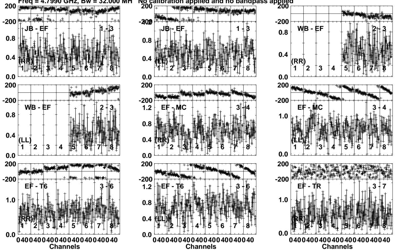
Lower frame: Milli Ampl Jy Top frame: Phas deg Vector averaged cross-power spectrum Several baselines displayed Timerange: 00/22:49:01 to 00/22:49:59
