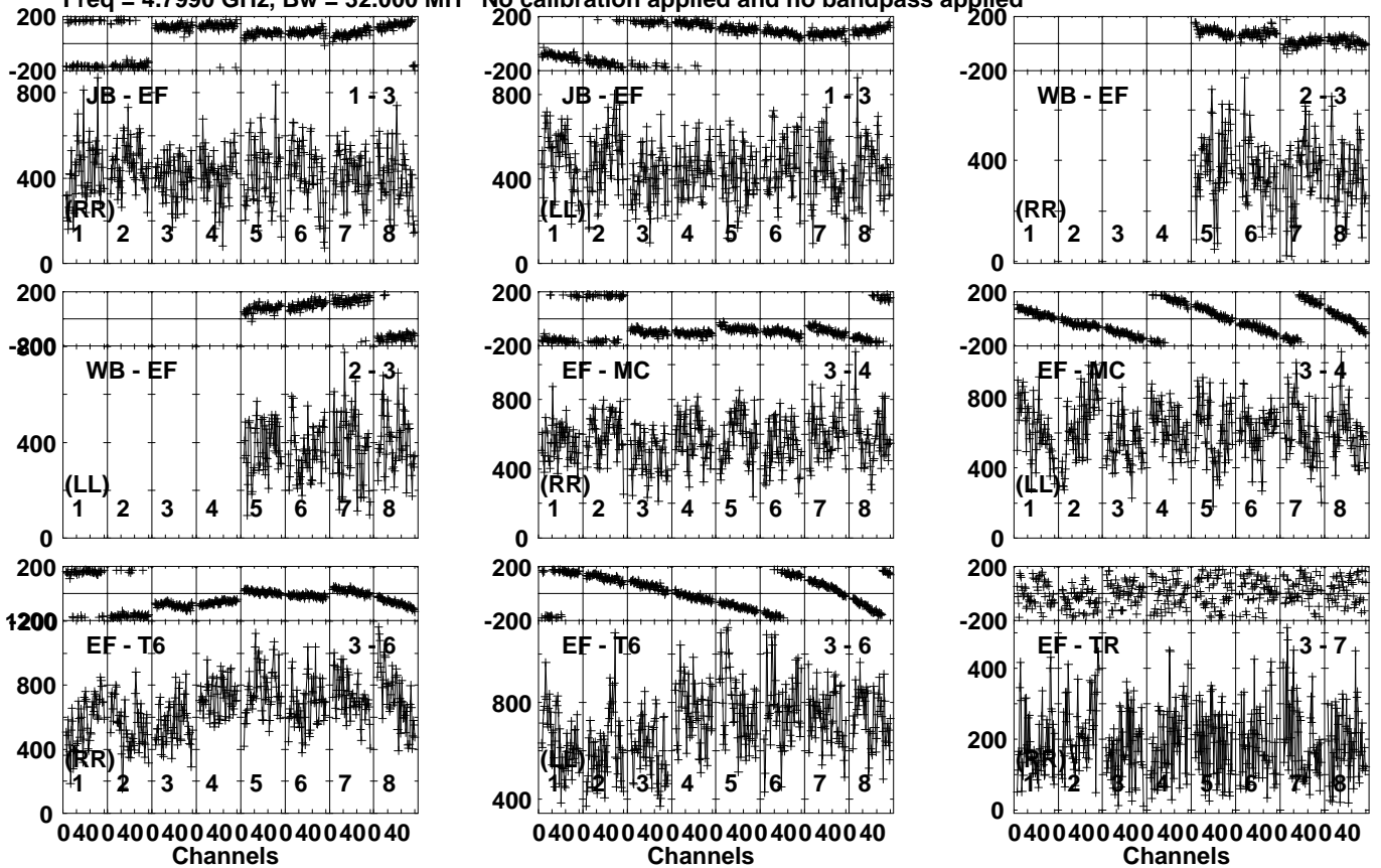
Lower frame: Micro Ampl Jy Top frame: Phas deg Vector averaged cross-power spectrum Several baselines displayed Timerange: 00/23:17:01 to 00/23:17:59
