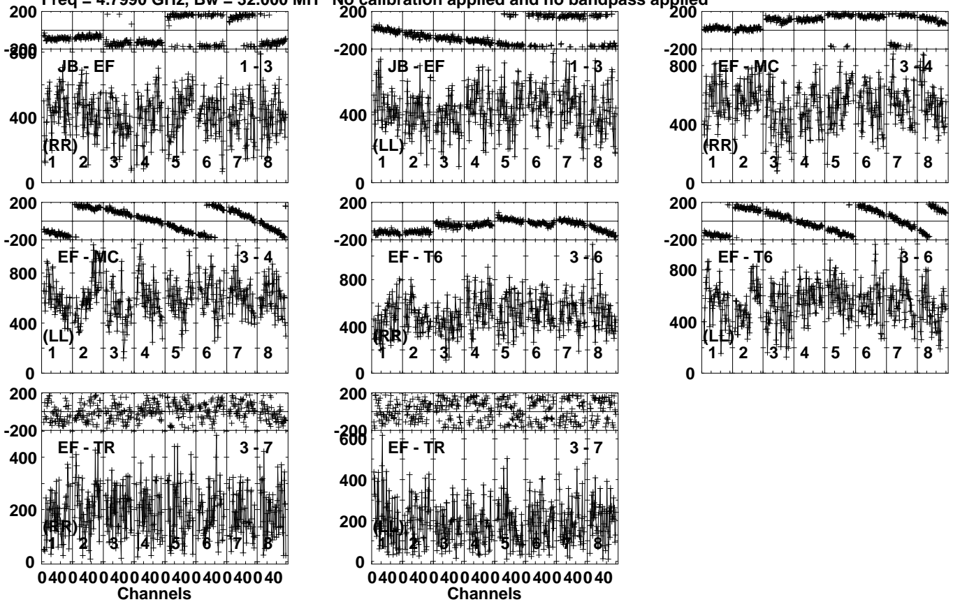
Lower frame: Micro Ampl Jy Top frame: Phas deg Vector averaged cross-power spectrum Several baselines displayed Timerange: 00/21:21:31 to 00/21:22:29
