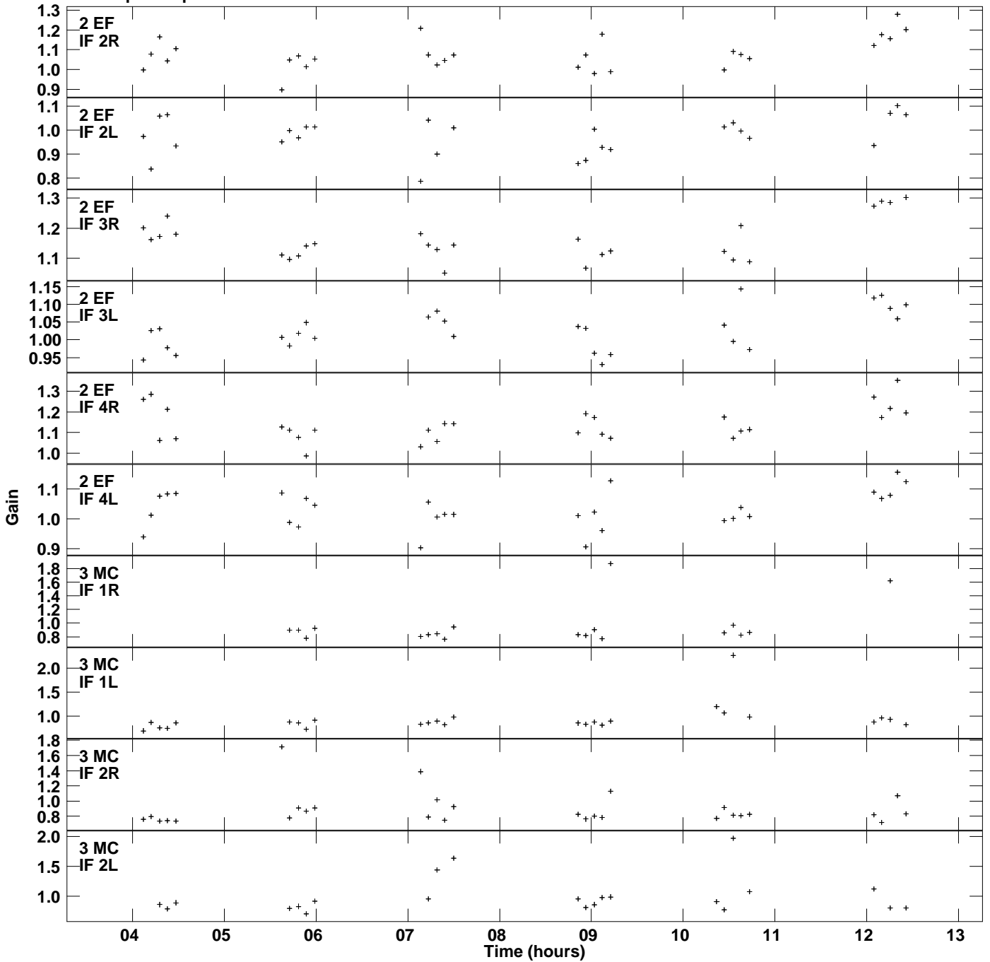
Plot file version 2 created 02-AUG-2019 11:59:10 Gain amp vs UTC time for J1848+0138.MULTI.1 SN 2 Rpol & Lpol IF 1 - 4
