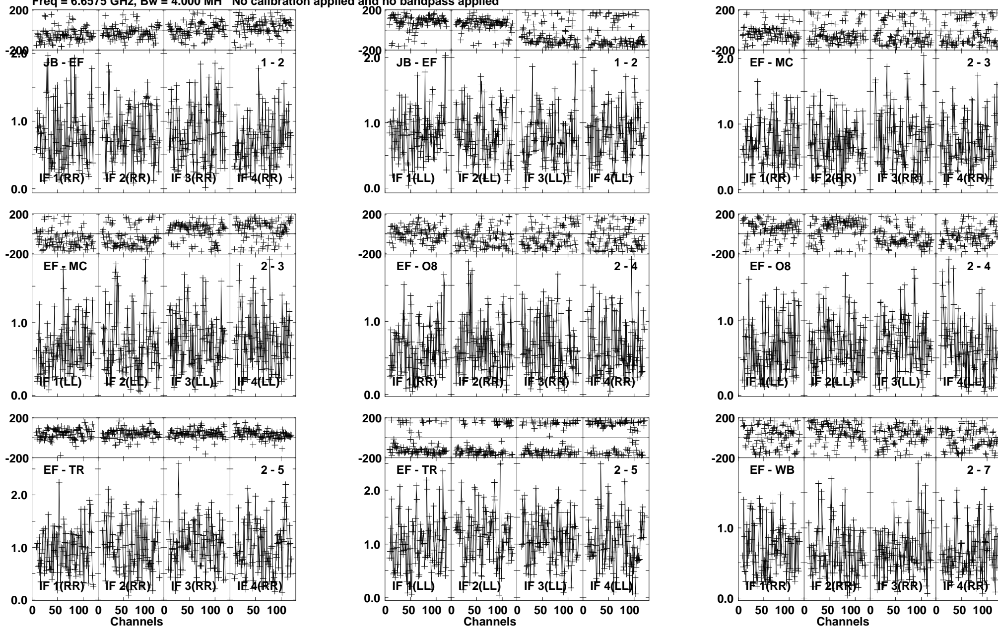
Lower frame: Milli Ampl Jy Top frame: Phas deg Vector averaged cross-power spectrum Baseline: JB (01) - EF (02) Timerange: 00/10:26:06 to 00/10:27:48
