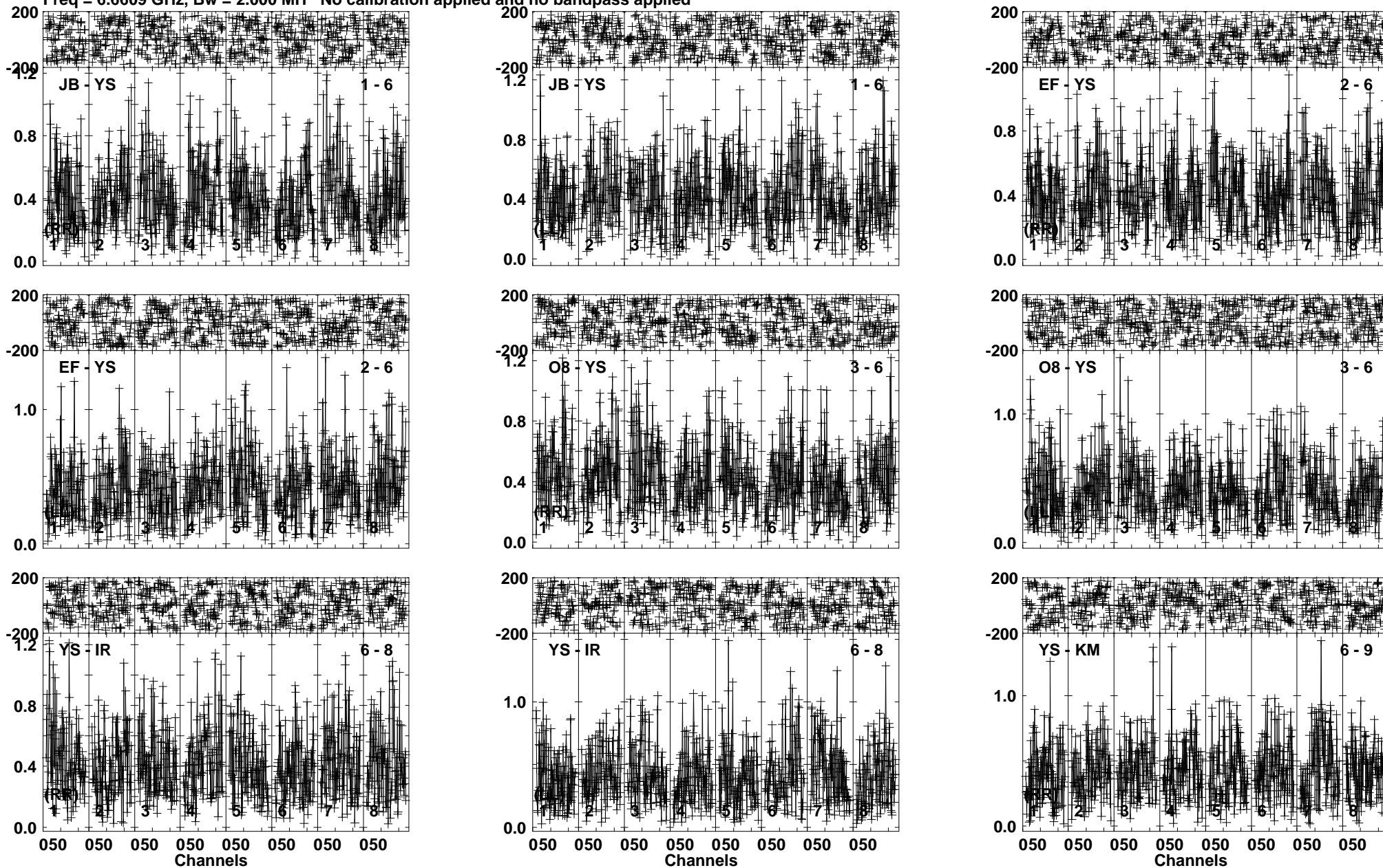
Lower frame: Milli Ampl Jy Top frame: Phas deg Vector averaged cross-power spectrum Baseline: JB (01) - YS (06) Timerange: 00/20:21:15 to 00/20:24:30
