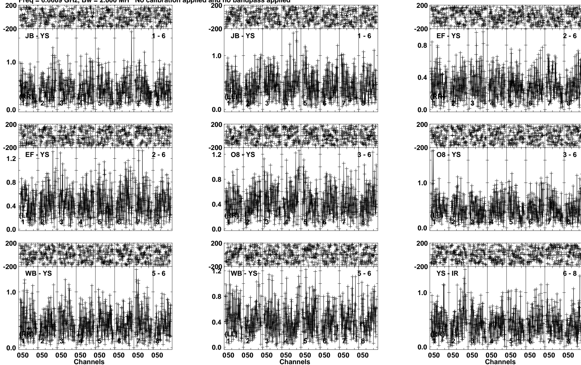
Lower frame: Milli Ampl Jy Top frame: Phas deg Vector averaged cross-power spectrum Baseline: JB (01) - YS (06) Timerange: 01/01:22:00 to 01/01:25:15
