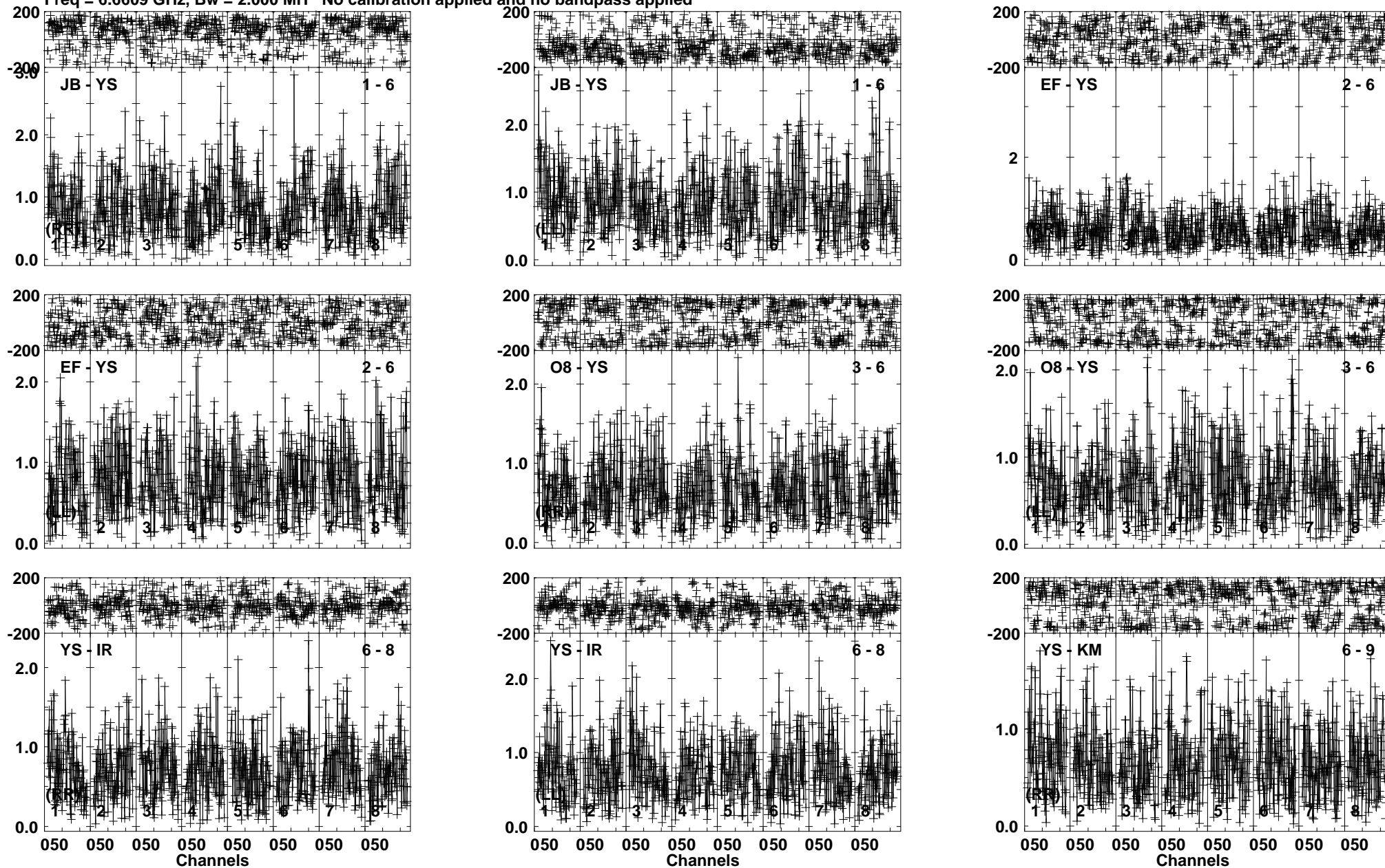
Lower frame: Milli Ampl Jy Top frame: Phas deg Vector averaged cross-power spectrum Baseline: JB (01) - YS (06) Timerange: 00/21:41:30 to 00/21:43:15
