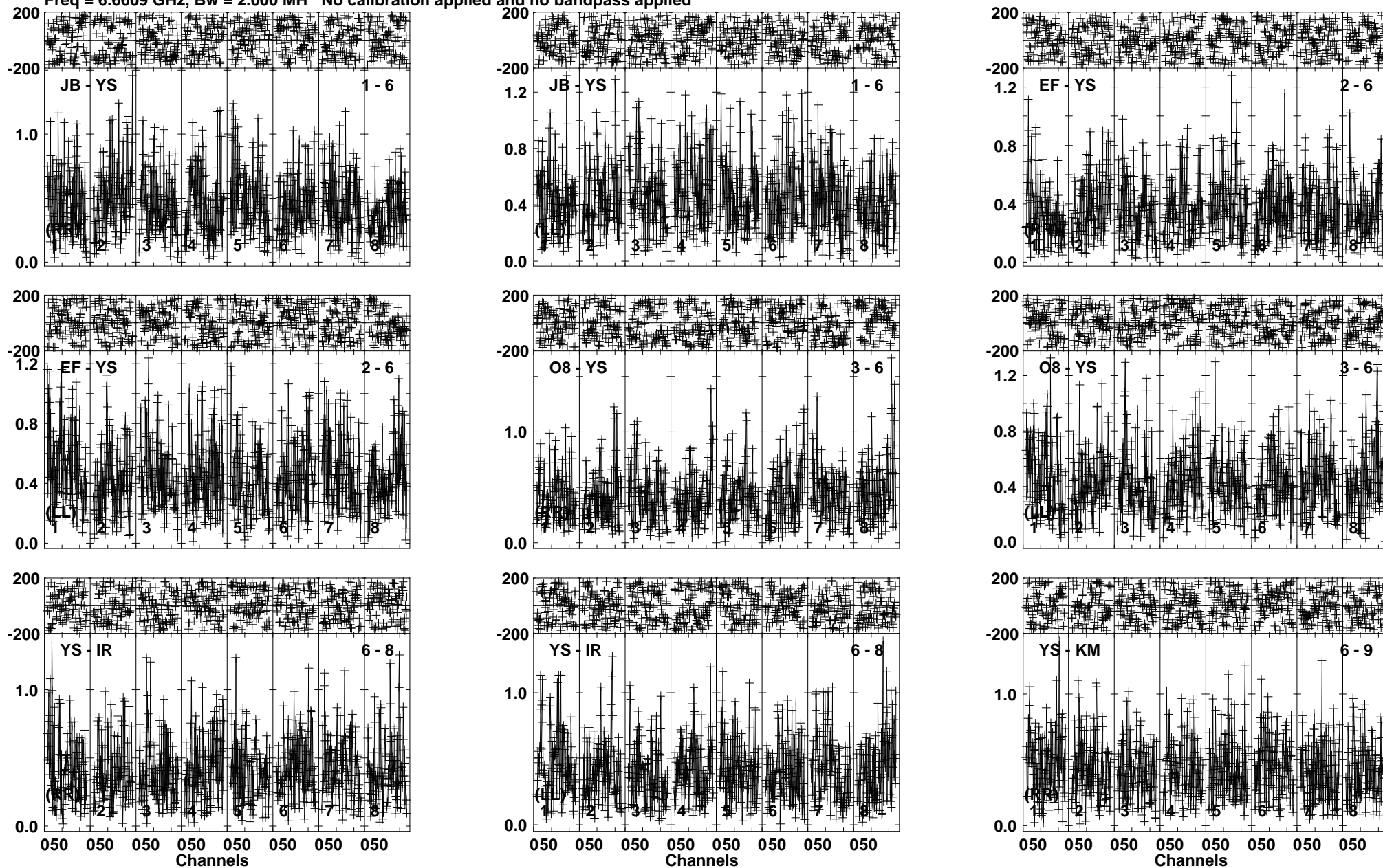
Lower frame: Milli Ampl Jy Top frame: Phas deg Vector averaged cross-power spectrum Baseline: JB (01) - YS (06) Timerange: 00/21:21:45 to 00/21:25:00
