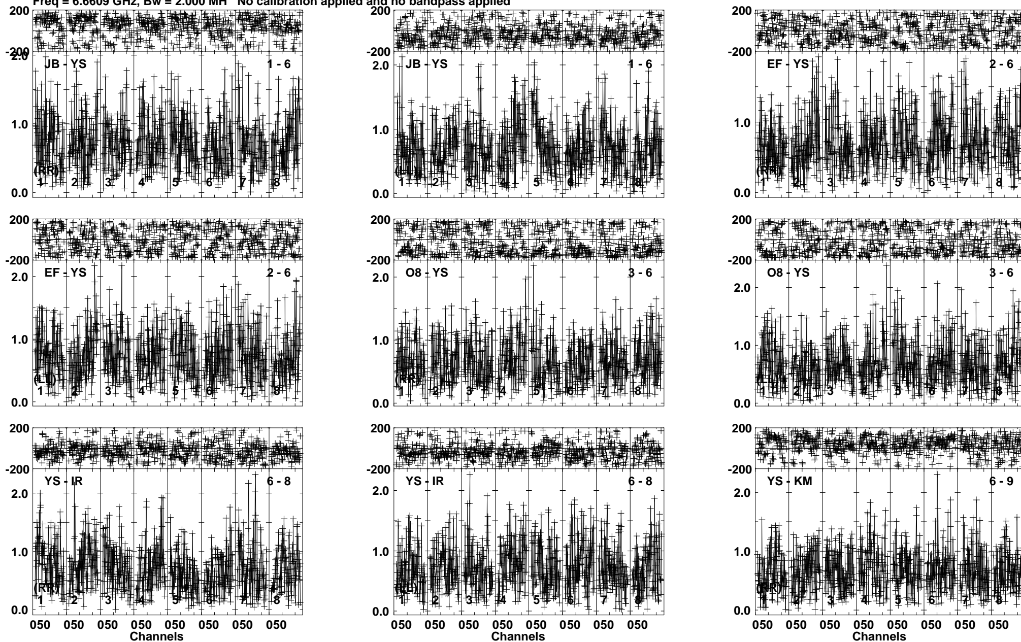
Lower frame: Milli Ampl Jy Top frame: Phas deg Vector averaged cross-power spectrum Baseline: JB (01) - YS (06) Timerange: 00/20:13:30 to 00/20:15:15
