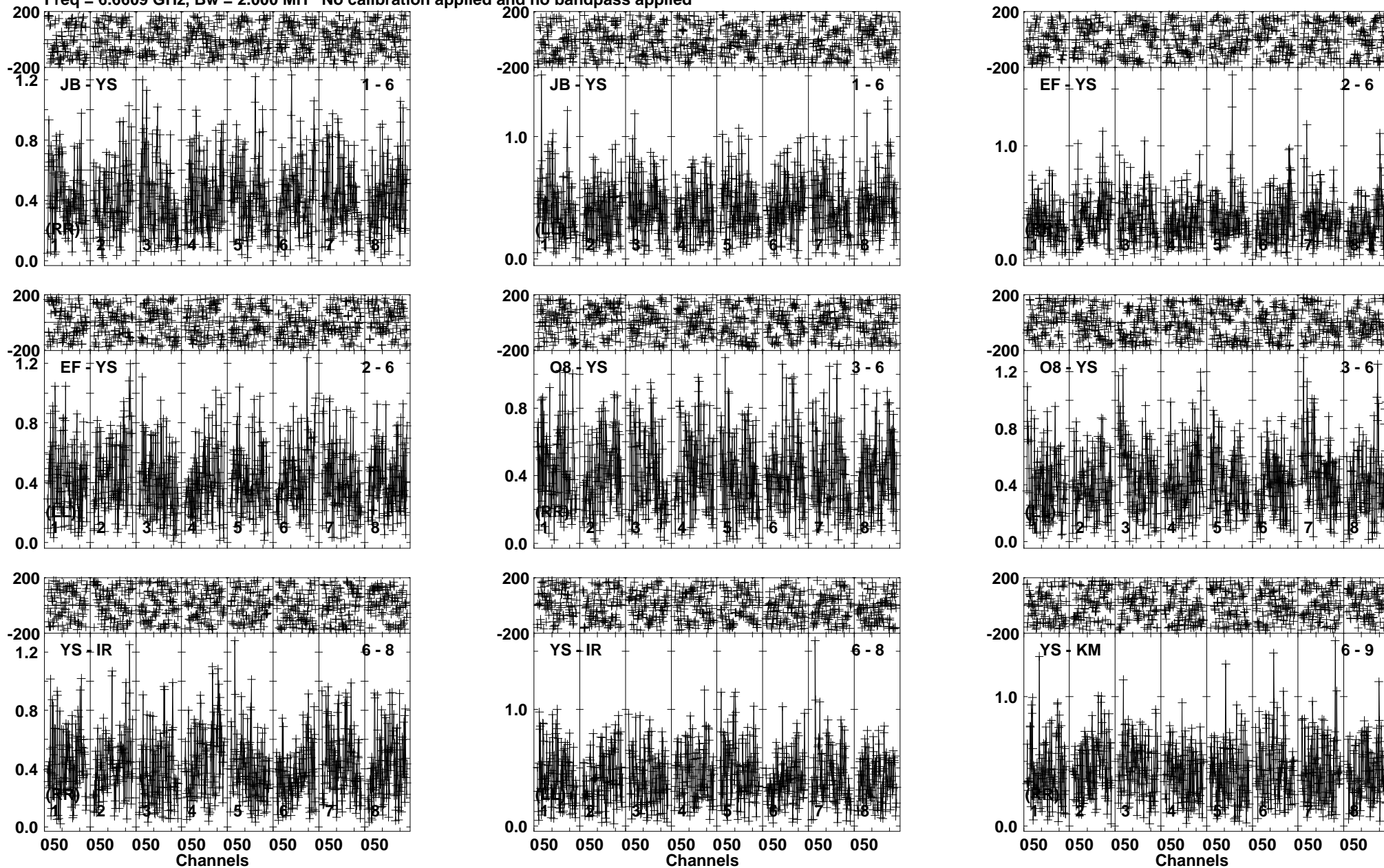
Lower frame: Milli Ampl Jy Top frame: Phas deg Vector averaged cross-power spectrum Baseline: JB (01) - YS (06) Timerange: 00/21:38:15 to 00/21:41:30
