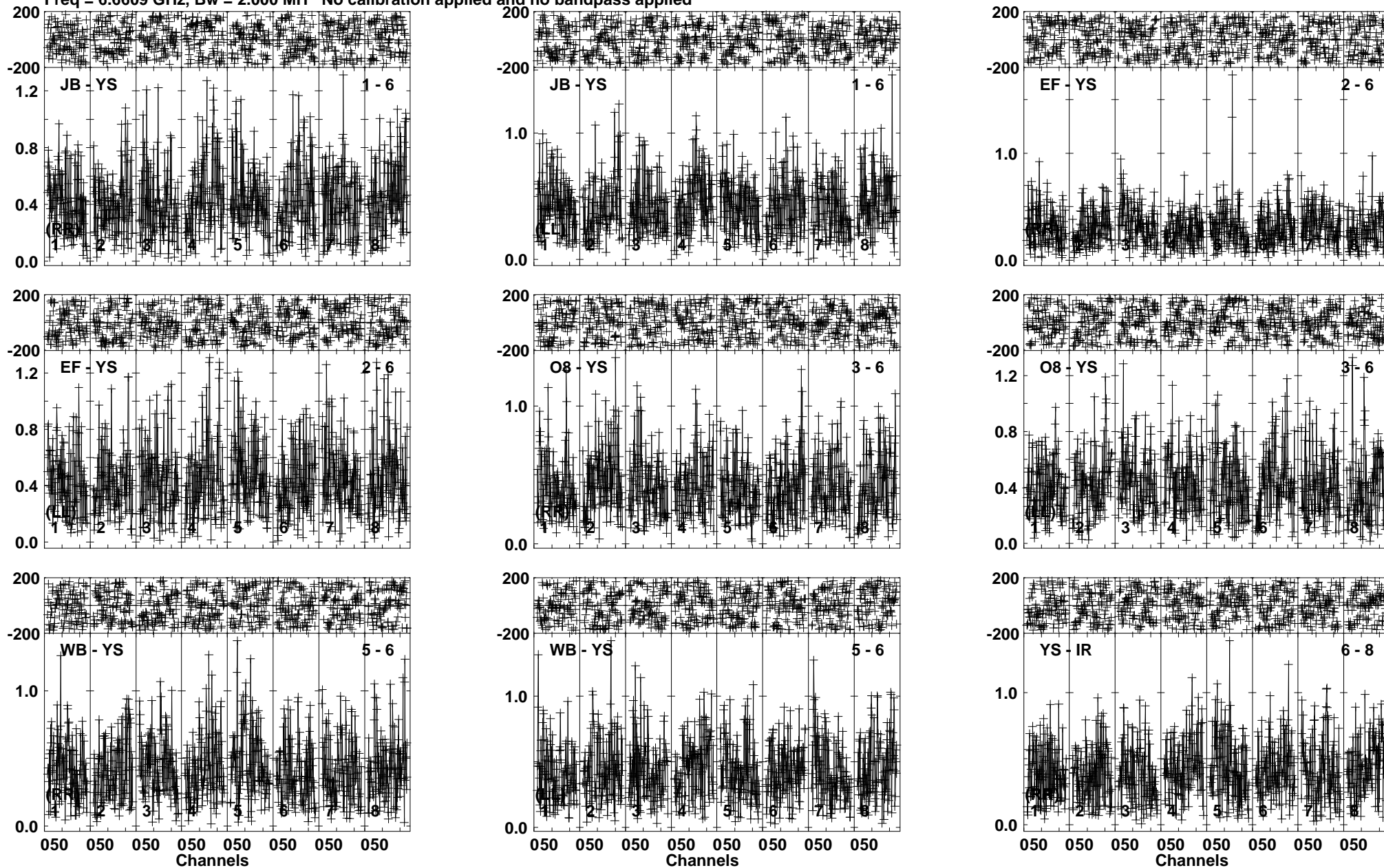
Lower frame: Milli Ampl Jy Top frame: Phas deg Vector averaged cross-power spectrum Baseline: JB (01) - YS (06) Timerange: 00/23:48:30 to 00/23:51:45
