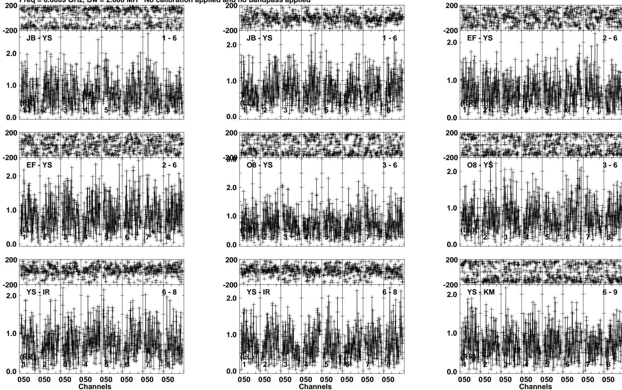
Lower frame: Milli Ampl Jy Top frame: Phas deg Vector averaged cross-power spectrum Baseline: JB (01) - YS (06) Timerange: 00:21:25:00 to 00:21:26:45
