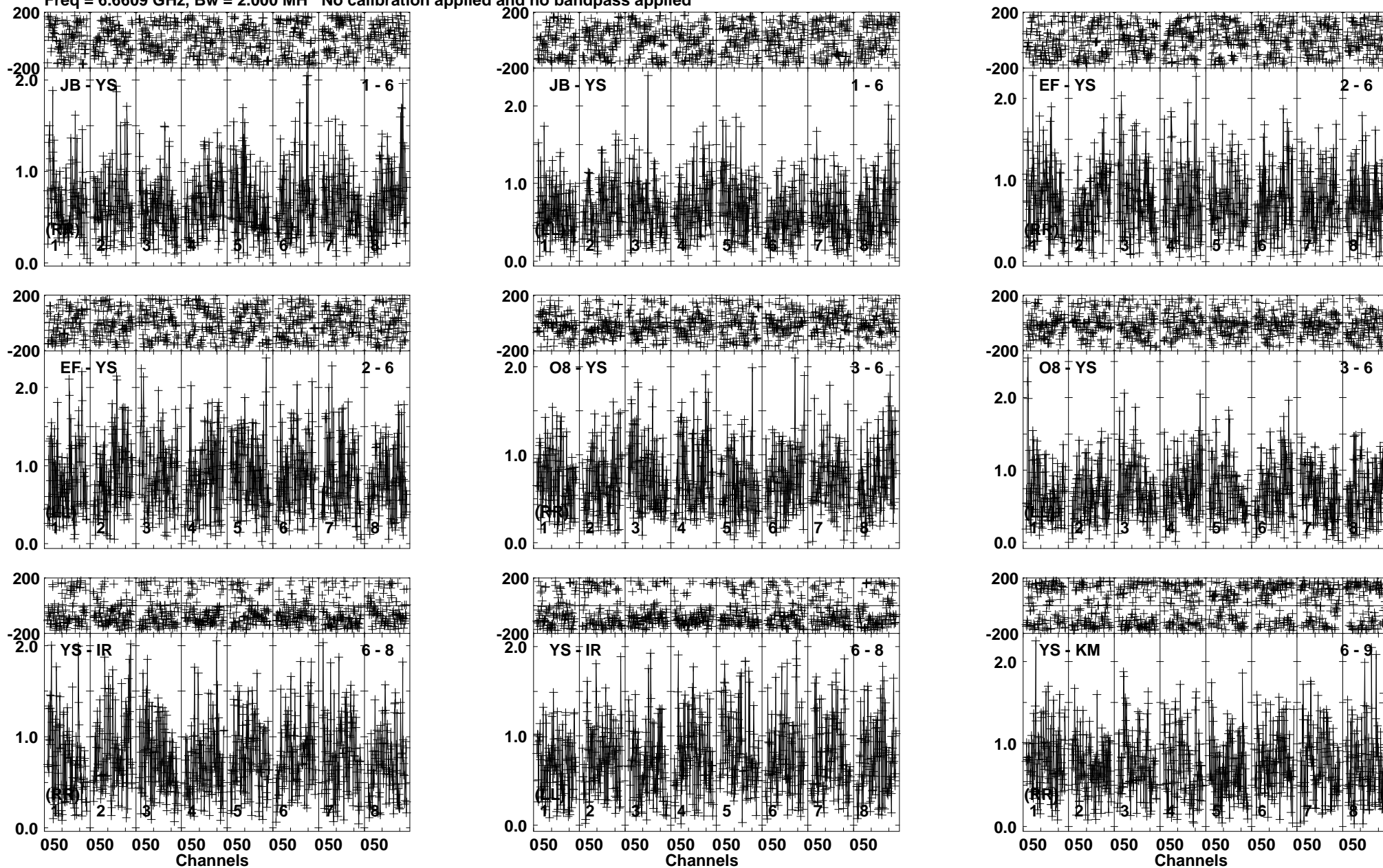
Lower frame: Milli Ampl Jy Top frame: Phas deg Vector averaged cross-power spectrum Baseline: JB (01) - YS (06) Timerange: 00/20:46:30 to 00/20:48:15
