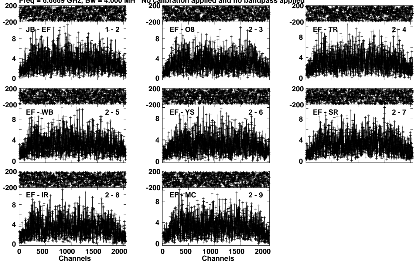
Lower frame: Milli Amp Jy Top frame: Phas deg Vector averaged cross-power spectrum Several baselines displayed Timerange: 00/17:00:45 to 00/17:02:30
