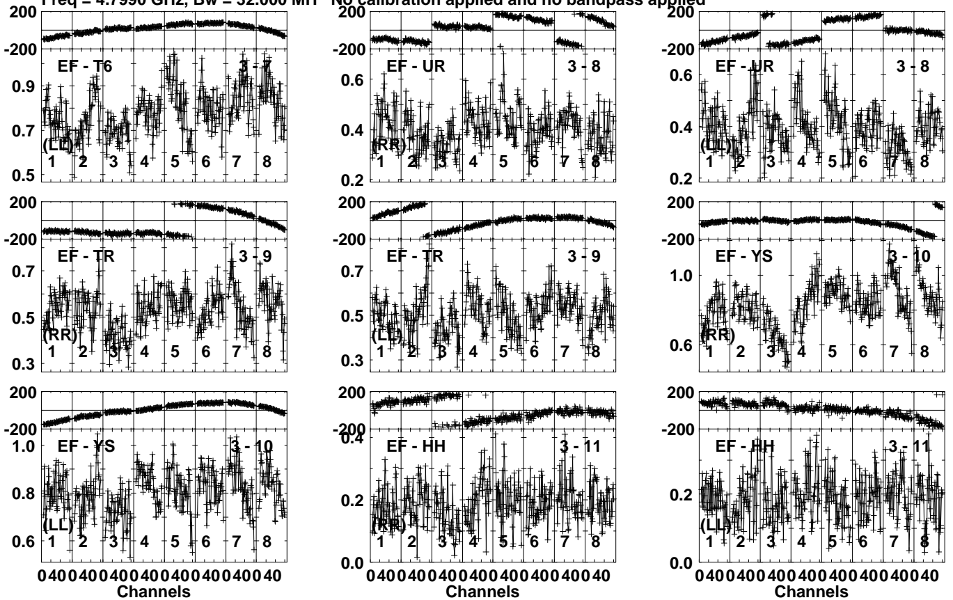
Lower frame: Milli Ampl Jy Top frame: Phas deg Vector averaged cross-power spectrum Several baselines displayed Timerange: 00/22:36:21 to 00/22:39:49
