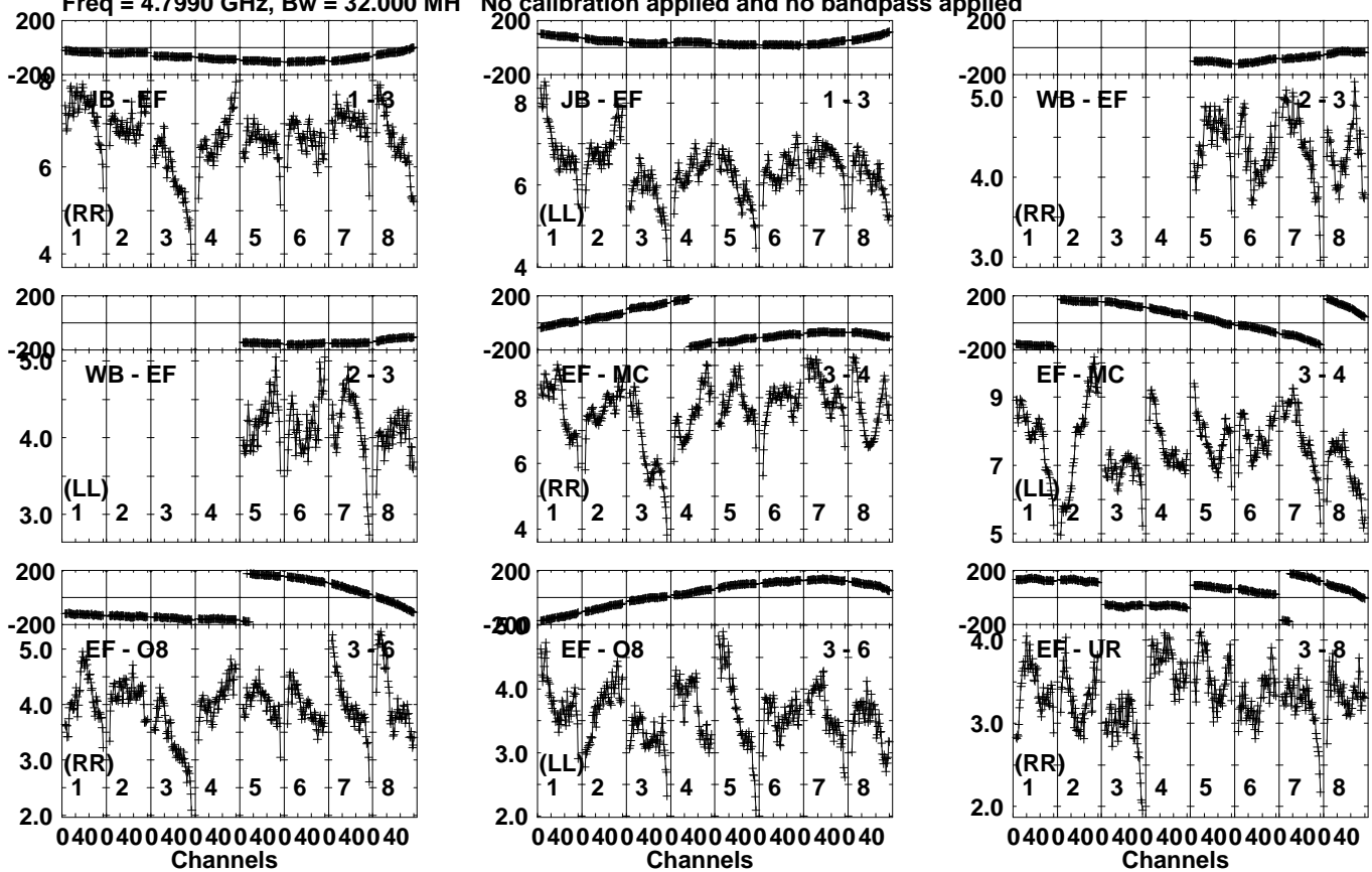
Lower frame: Milli Ampl Jy Top frame: Phas deg Vector averaged cross-power spectrum Several baselines displayed Timerange: 01/01:49:23 to 01/01:50:49
