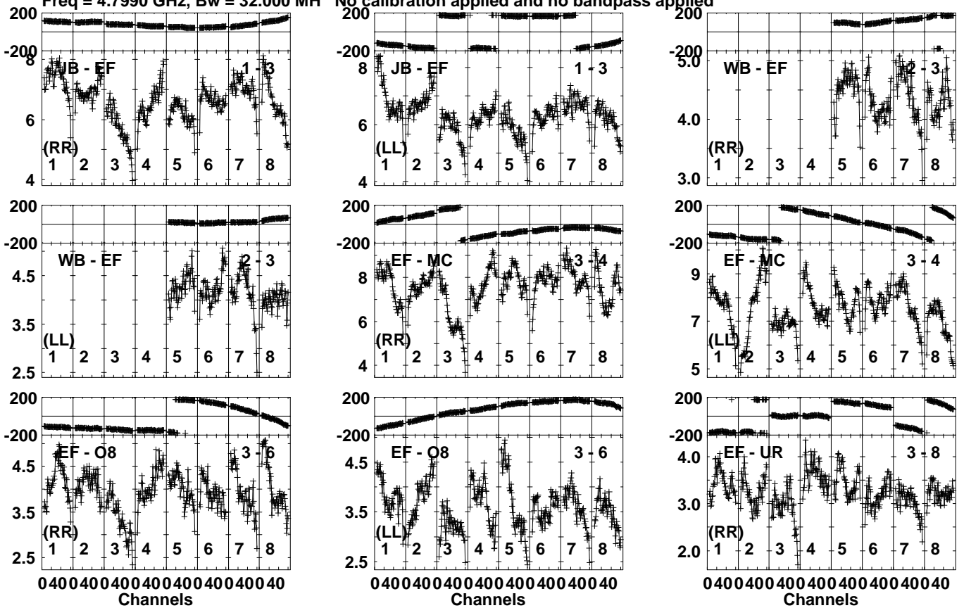
Lower frame: Milli Ampl Jy Top frame: Phas deg Vector averaged cross-power spectrum Several baselines displayed Timerange: 01/02:40:21 to 01/02:41:49
