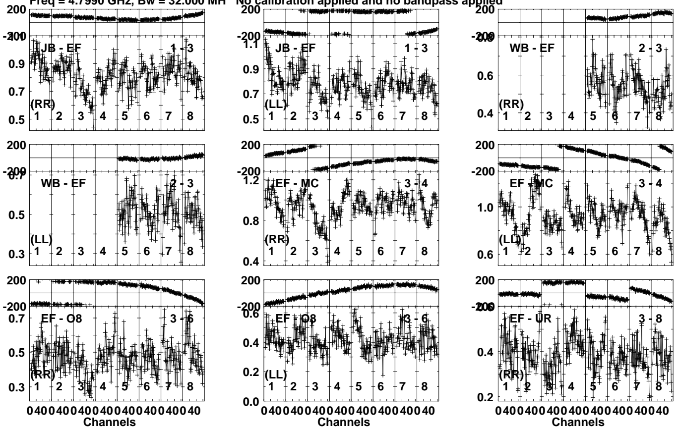
Lower frame: Milli Ampl Jy Top frame: Phas deg Vector averaged cross-power spectrum Several baselines displayed Timerange: 01/02:41:53 to 01/02:45:19
