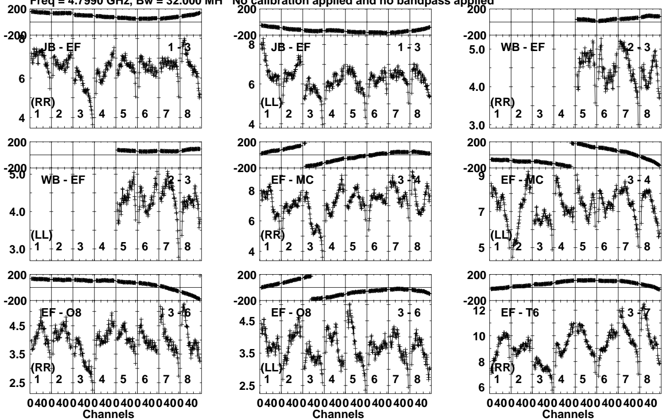
Lower frame: Milli Ampl Jy Top frame: Phas deg Vector averaged cross-power spectrum Several baselines displayed Timerange: 00/22:45:41 to 00/22:46:39
