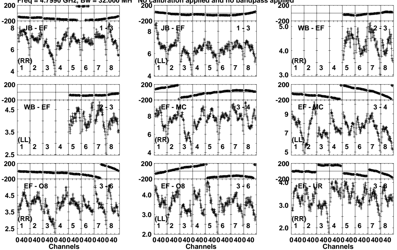
Lower frame: Milli Ampl Jy Top frame: Phas deg Vector averaged cross-power spectrum Several baselines displayed Timerange: 01/01:34:41 to 01/01:35:39
