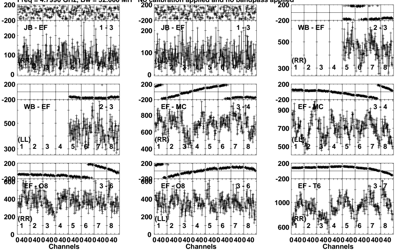
Lower frame: Micro Ampl Jy Top frame: Phas deg Vector averaged cross-power spectrum Several baselines displayed Timerange: 00/20:28:51 to 00/20:32:19
