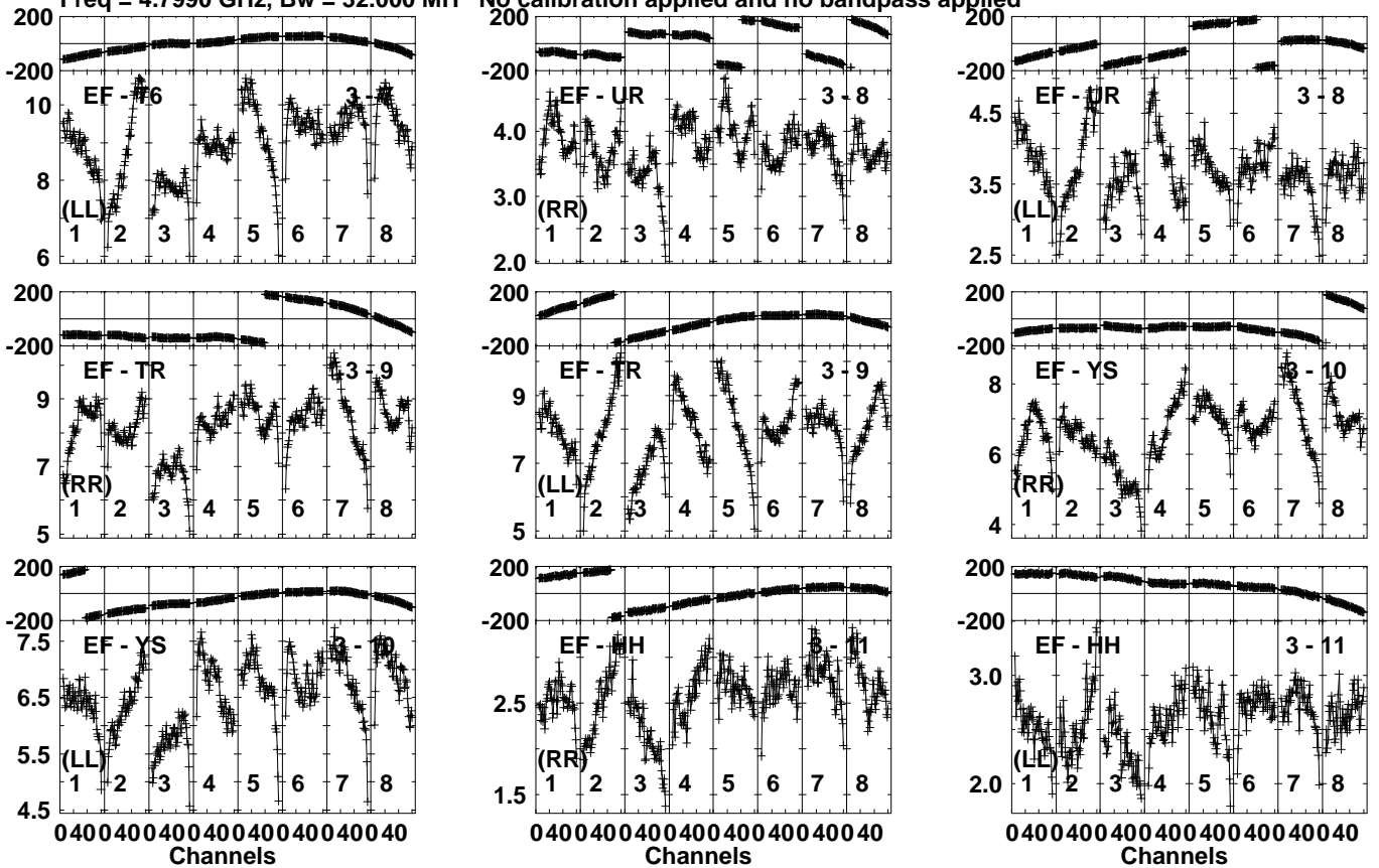
Lower frame: Milli Ampl Jy Top frame: Phas deg Vector averaged cross-power spectrum Several baselines displayed Timerange: 00/22:40:31 to 00/22:41:29
