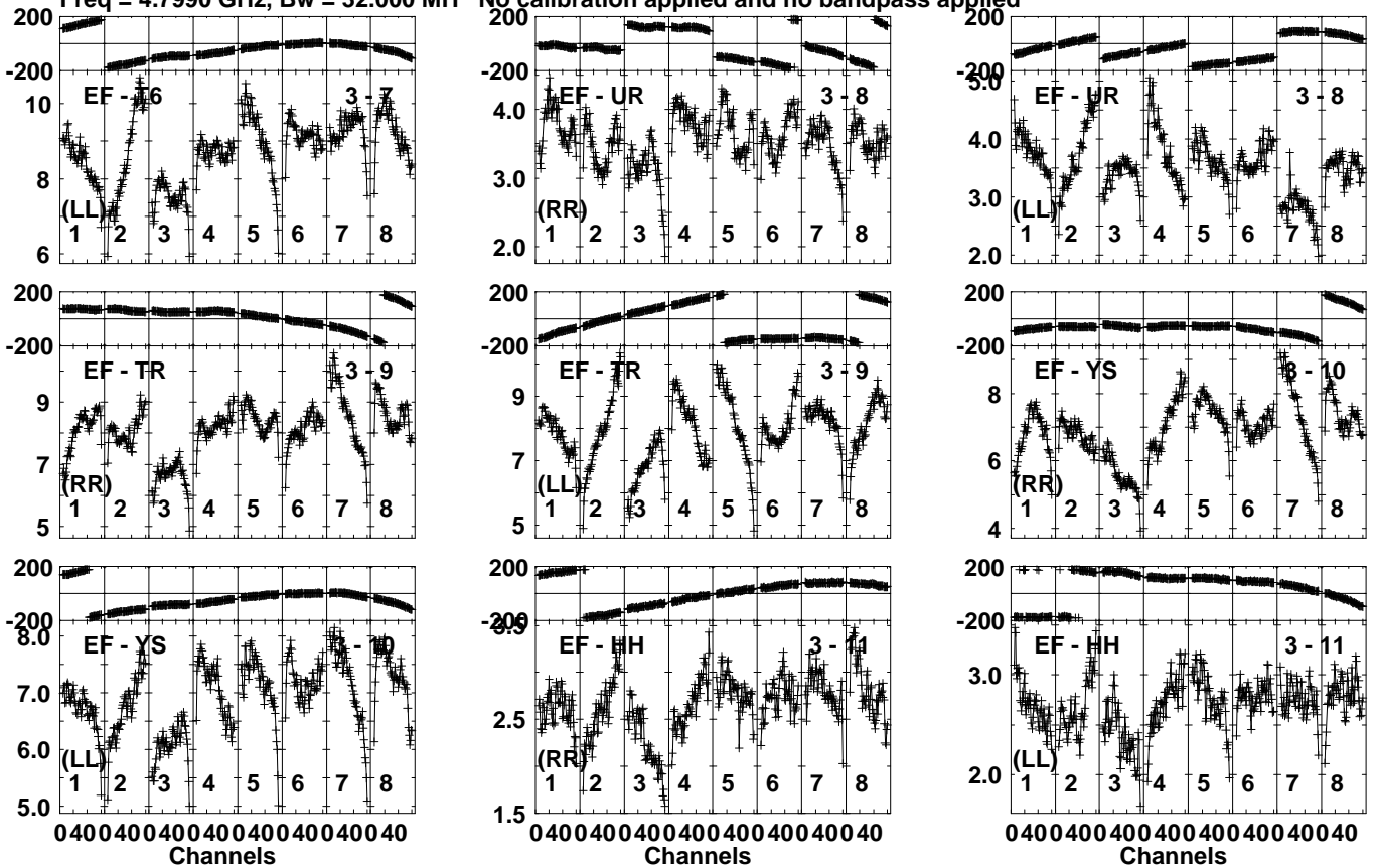
Lower frame: Milli Ampl Jy Top frame: Phas deg Vector averaged cross-power spectrum Several baselines displayed Timerange: 00/23:31:31 to 00/23:32:29
