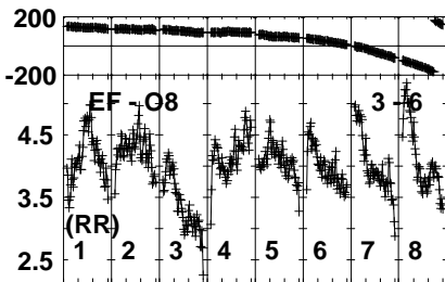
Lower frame: Milli Ampl Jy Top frame: Phas deg Vector averaged cross-power spectrum Several baselines displayed Timerange: 01/01:13:41 to 01/01:15:09
