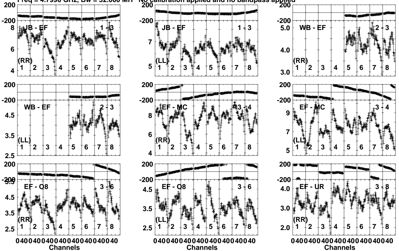
Lower frame: Milli Ampl Jy Top frame: Phas deg Vector averaged cross-power spectrum Several baselines displayed Timerange: 01/01:39:11 to 01/01:40:39
