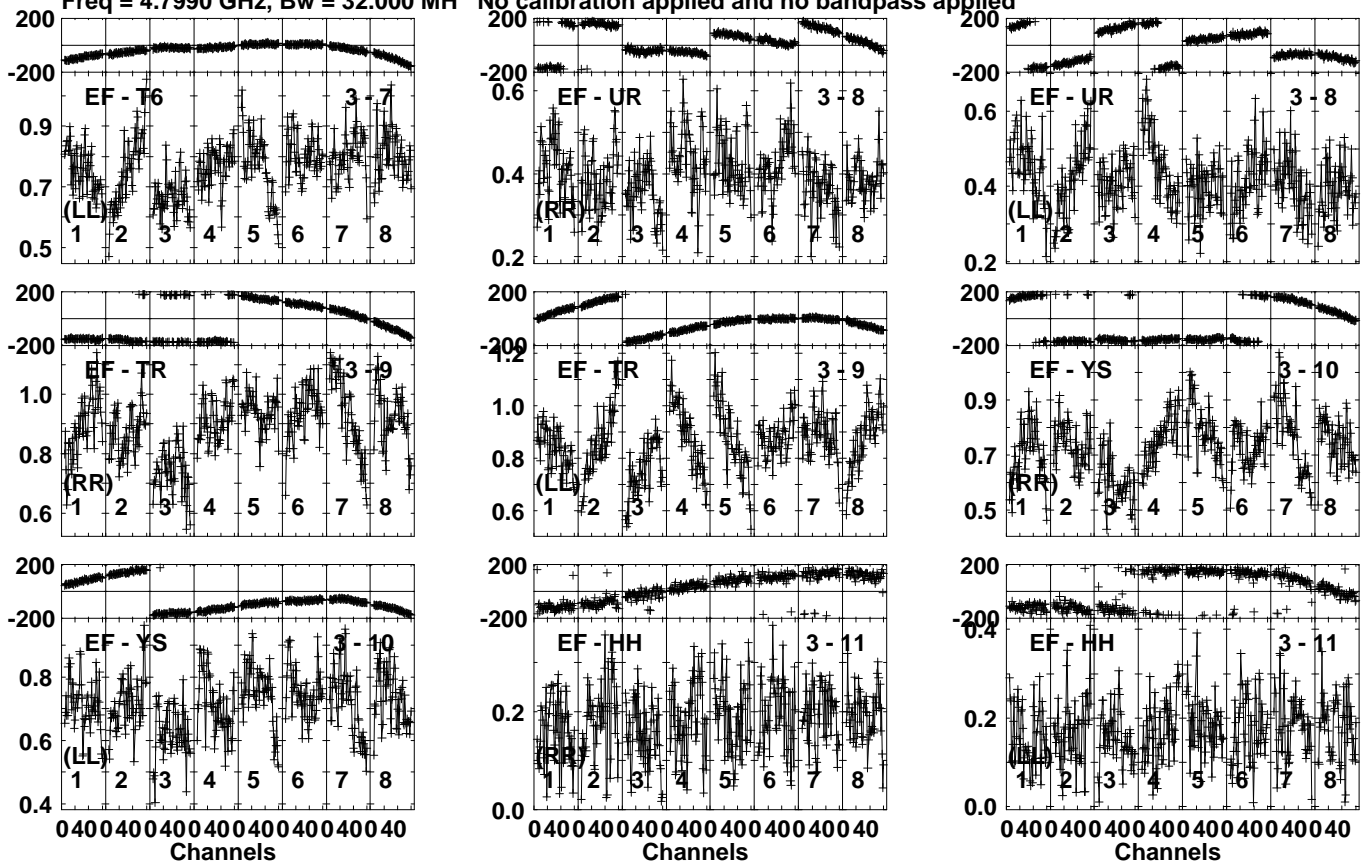
Lower frame: Milli Ampl Jy Top frame: Phas deg Vector averaged cross-power spectrum Several baselines displayed Timerange: 00/21:45:21 to 00/21:48:49
