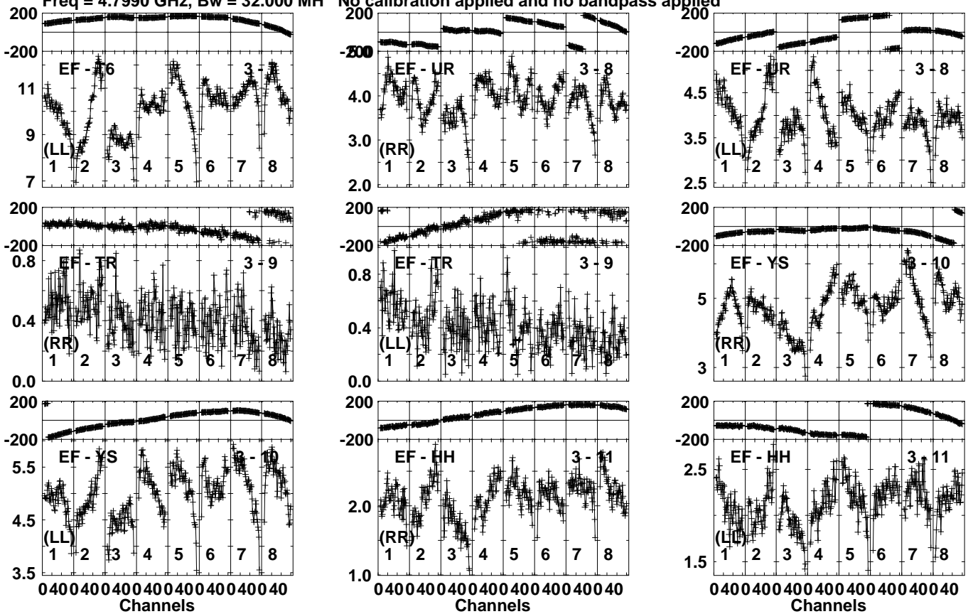
Lower frame: Milli Ampl Jy Top frame: Phas deg Vector averaged cross-power spectrum Several baselines displayed Timerange: 00/20:52:51 to 00/20:54:19
