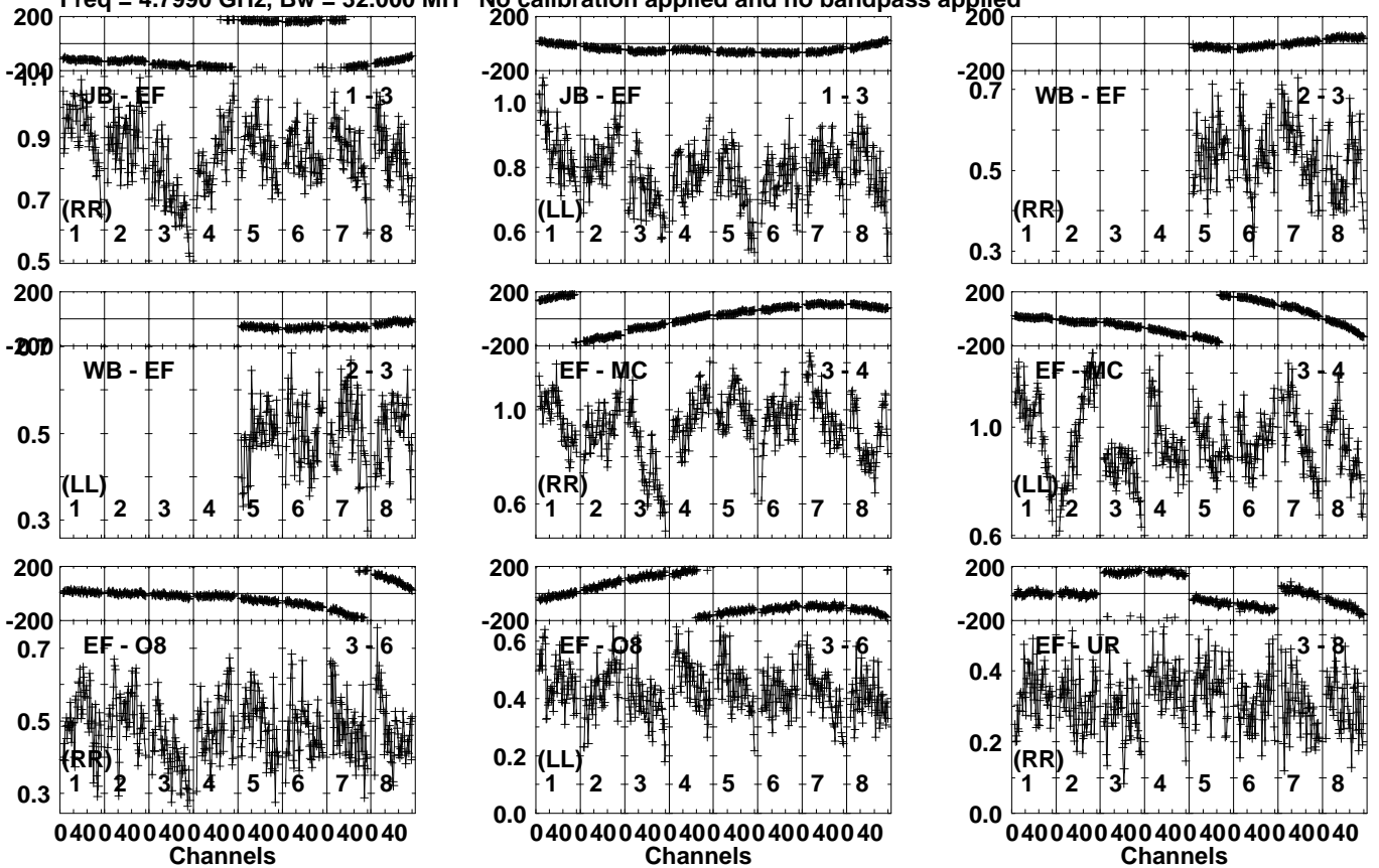
Lower frame: Milli Ampl Jy Top frame: Phas deg Vector averaged cross-power spectrum Several baselines displayed Timerange: 01/01:25:21 to 01/01:28:49
