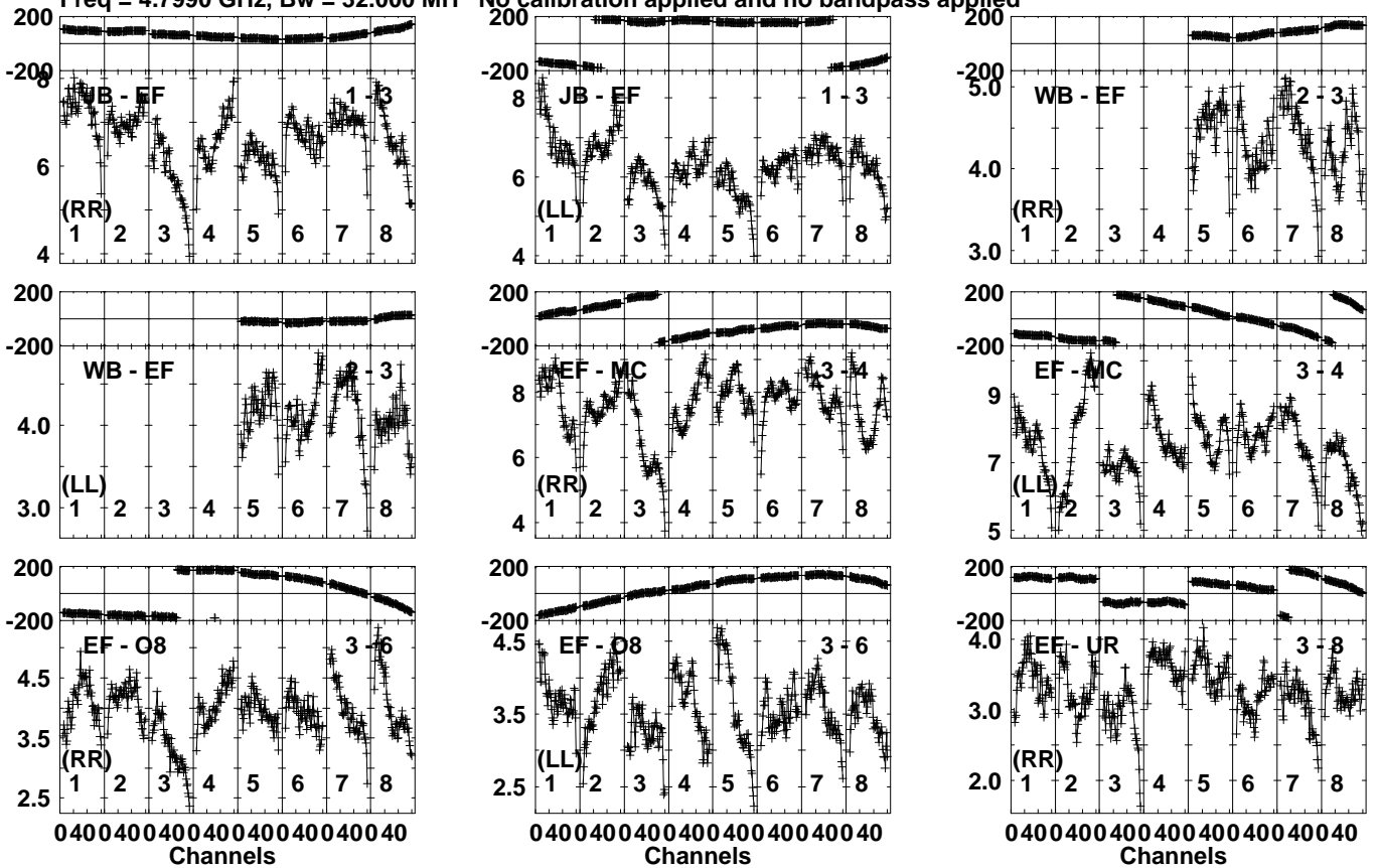
Lower frame: Milli Ampl Jy Top frame: Phas deg Vector averaged cross-power spectrum Several baselines displayed Timerange: 01/02:46:01 to 01/02:46:59
