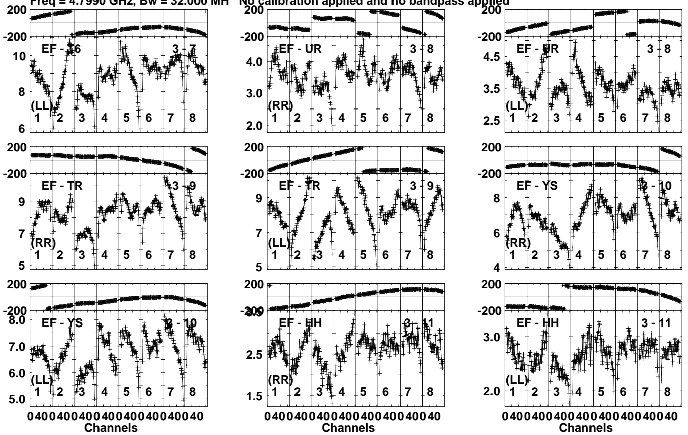
Lower frame: Milli Ampl Jy Top frame: Phas deg Vector averaged cross-power spectrum Several baselines displayed Timerange: 00/23:21:21 to 00/23:22:19
