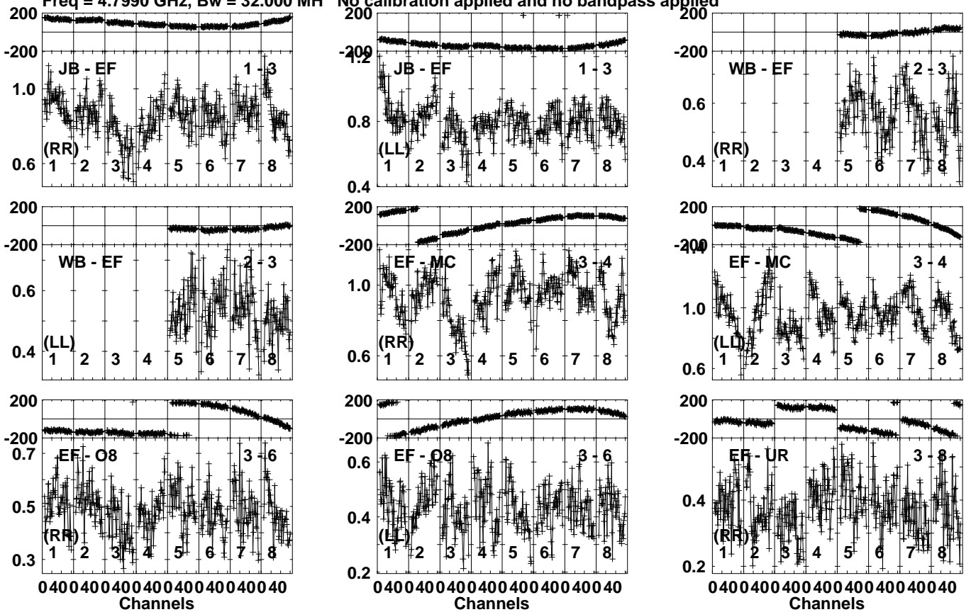
Lower frame: Milli Ampl Jy Top frame: Phas deg Vector averaged cross-power spectrum Several baselines displayed Timerange: 01/00:34:21 to 01/00:37:49
