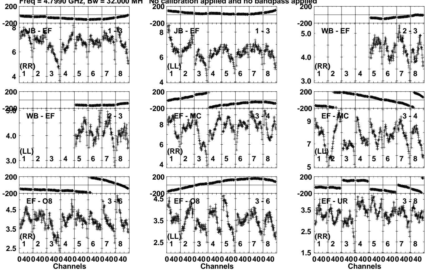
Lower frame: Milli Ampl Jy Top frame: Phas deg Vector averaged cross-power spectrum Several baselines displayed Timerange: 01/01:44:51 to 01/01:45:49
