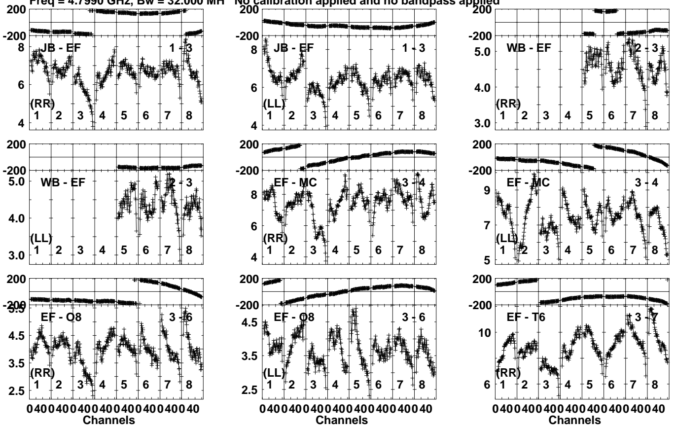
Lower frame: Milli Ampl Jy Top frame: Phas deg Vector averaged cross-power spectrum Several baselines displayed Timerange: 00/23:25:53 to 00/23:27:19
