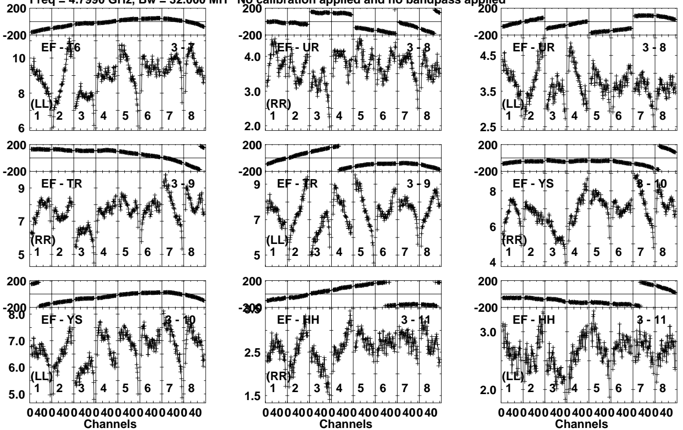
Lower frame: Milli Ampl Jy Top frame: Phas deg Vector averaged cross-power spectrum Several baselines displayed Timerange: 00/23:06:01 to 00/23:06:59
