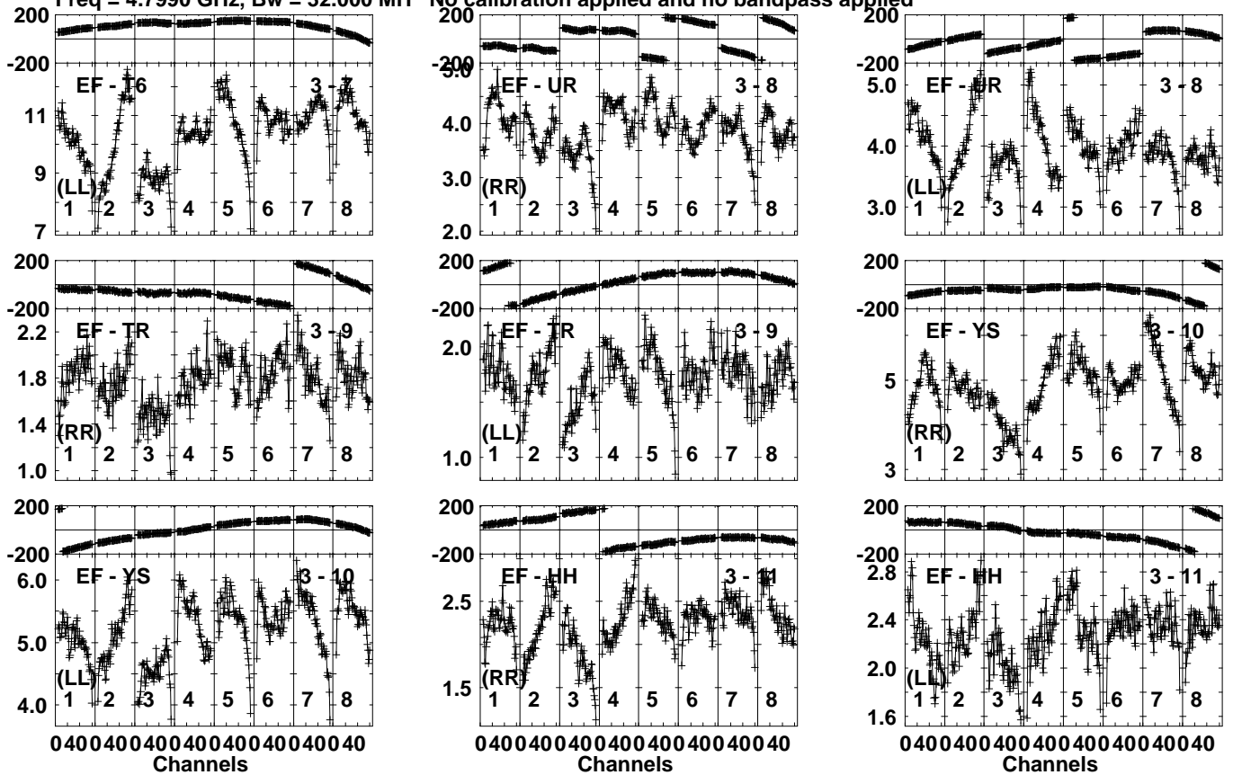
Lower frame: Milli Ampl Jy Top frame: Phas deg Vector averaged cross-power spectrum Several baselines displayed Timerange: 00/21:13:51 to 00/21:14:49
