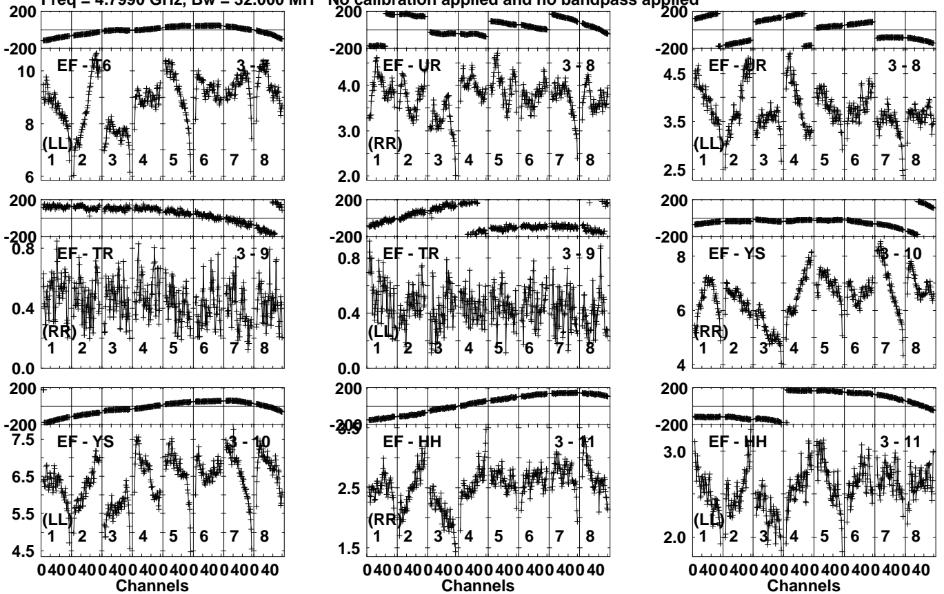
Lower frame: Milli Ampl Jy Top frame: Phas deg Vector averaged cross-power spectrum Several baselines displayed Timerange: 00/22:30:21 to 00/22:31:19
