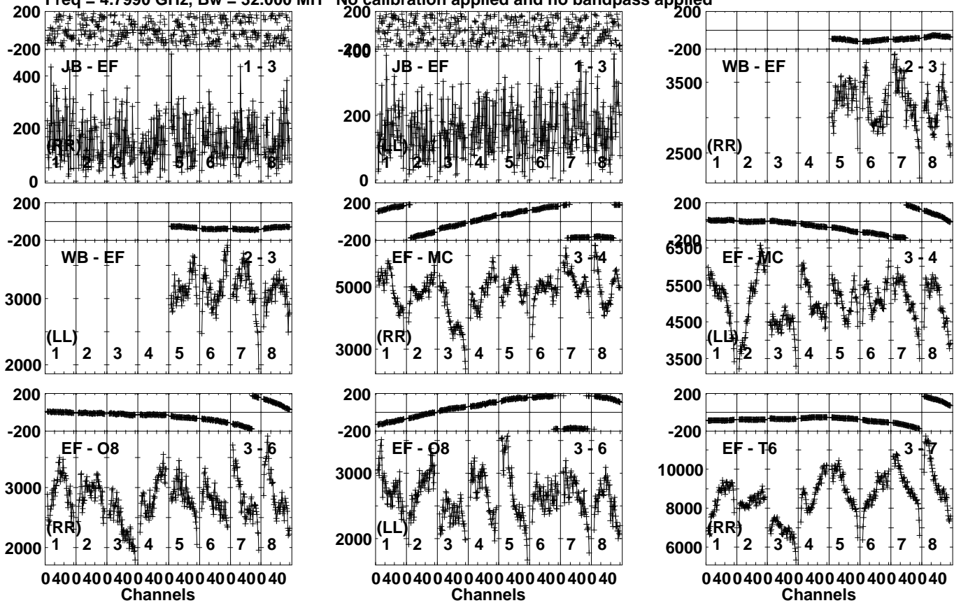
Lower frame: Micro Ampl Jy Top frame: Phas deg Vector averaged cross-power spectrum Several baselines displayed Timerange: 00/20:17:11 to 00/20:18:39
