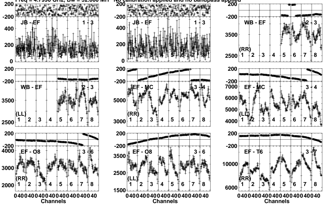
Lower frame: Micro Ampl Jy Top frame: Phas deg Vector averaged cross-power spectrum Several baselines displayed Timerange: 00/20:27:21 to 00/20:28:49
