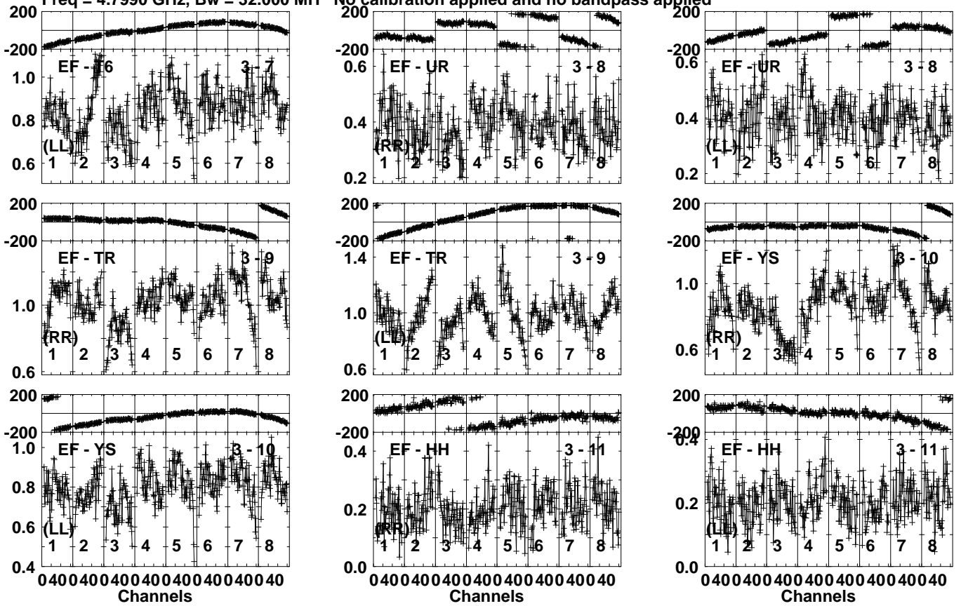
Lower frame: Milli Ampl Jy Top frame: Phas deg Vector averaged cross-power spectrum Several baselines displayed Timerange: 00/23:27:21 to 00/23:30:49
