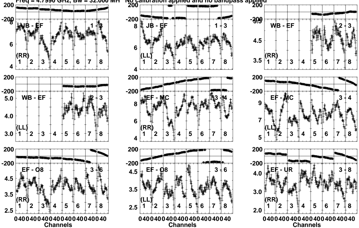
Lower frame: Milli Ampl Jy Top frame: Phas deg Vector averaged cross-power spectrum Several baselines displayed Timerange: 01/00:28:21 to 01/00:29:19
