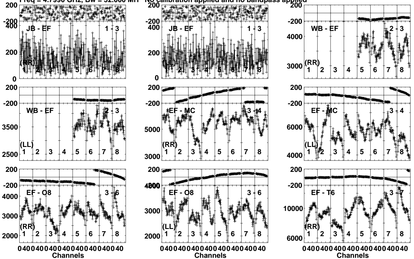
Lower frame: Micro Ampl Jy Top frame: Phas deg Vector averaged cross-power spectrum Several baselines displayed Timerange: 00/20:33:01 to 00/20:33:59
