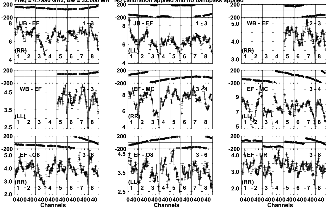
Lower frame: Milli Ampl Jy Top frame: Phas deg Vector averaged cross-power spectrum Several baselines displayed Timerange: 01/02:30:11 to 01/02:31:39
