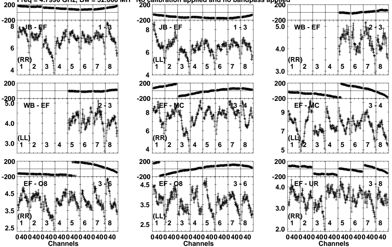
Lower frame: Milli Ampl Jy Top frame: Phas deg Vector averaged cross-power spectrum Several baselines displayed Timerange: 01/00:38:31 to 01/00:39:29
