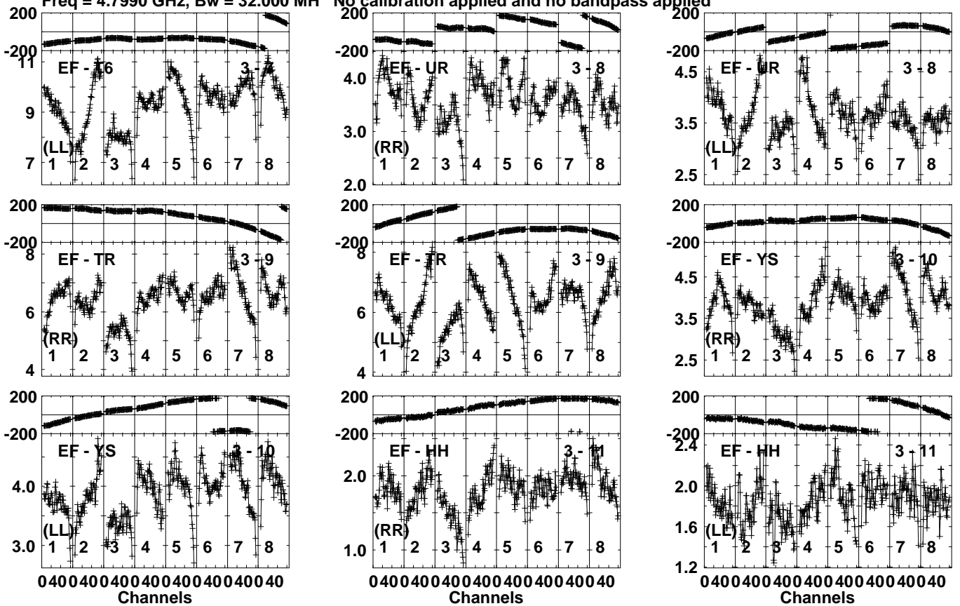
Lower frame: Milli Ampl Jy Top frame: Phas deg Vector averaged cross-power spectrum Several baselines displayed Timerange: 00/20:27:21 to 00/20:28:49
