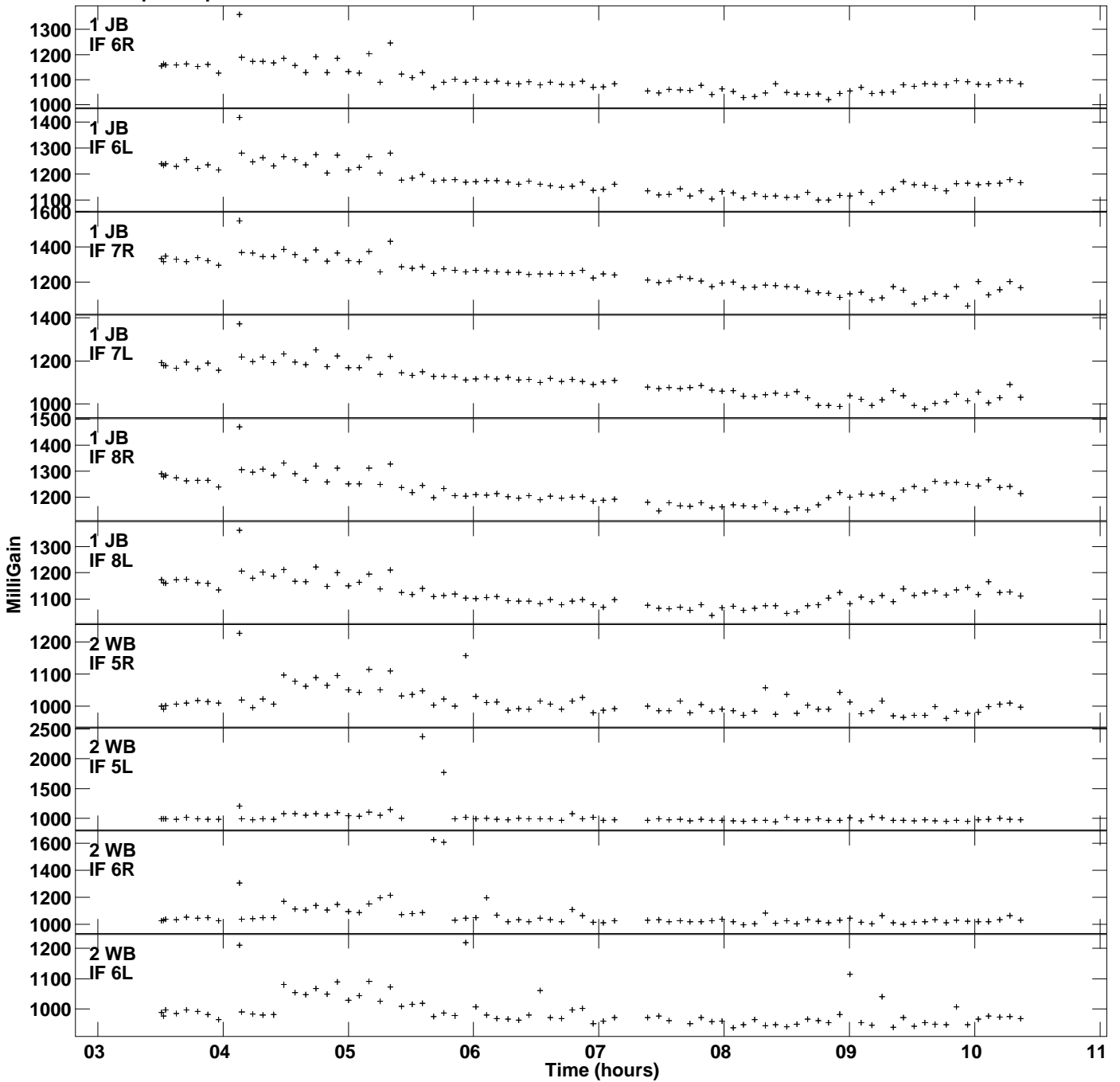
Plot file version 2 created 02-MAY-2023 14:11:43 Gain amp vs UTC time for J1935+2031.MULTI.1 SN 2 Rpol & Lpol IF 1 - 8
