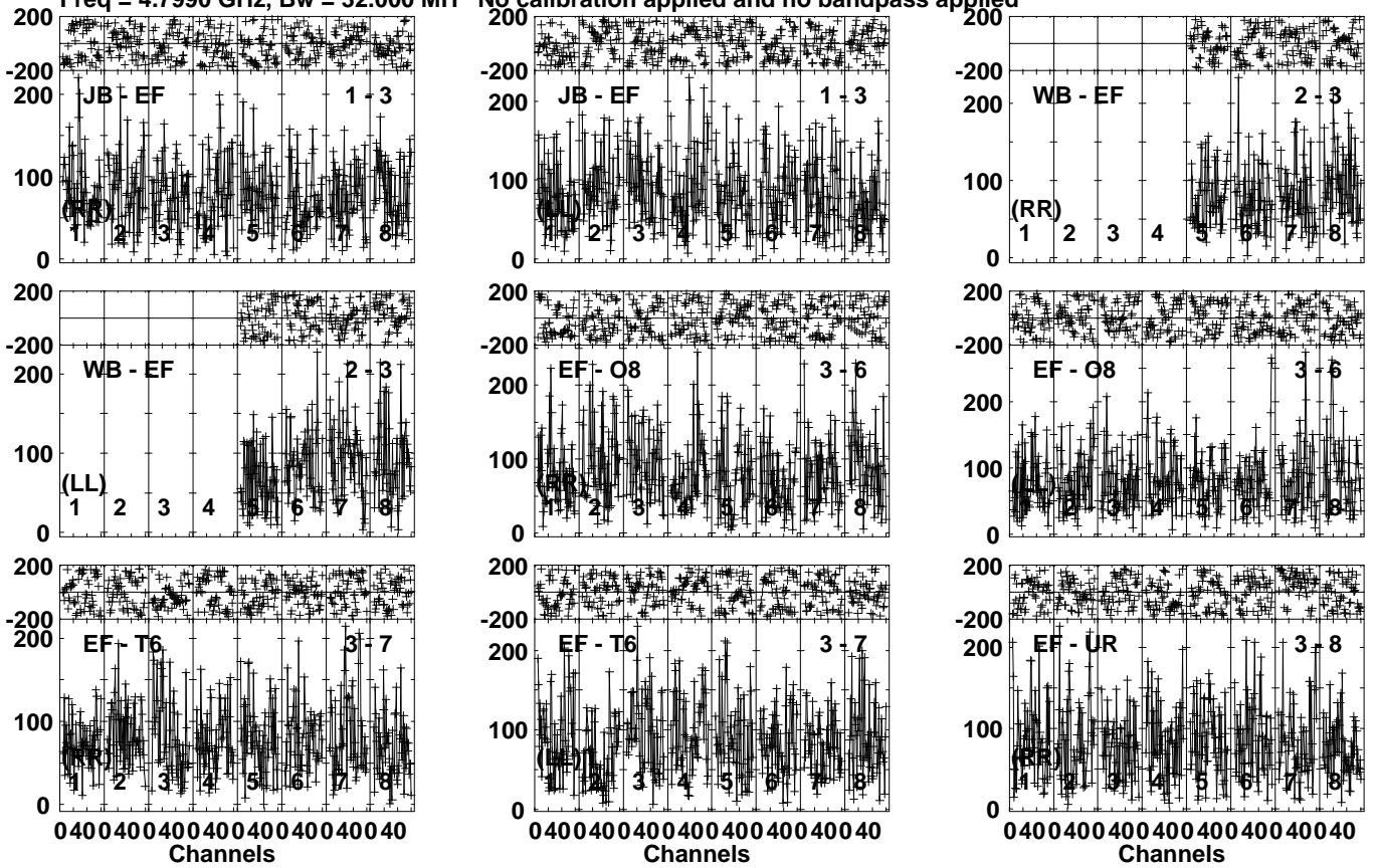
Lower frame: Micro Ampl Jy Top frame: Phas deg Vector averaged cross-power spectrum Several baselines displayed Timerange: 00/05:00:33 to 00/05:03:59
