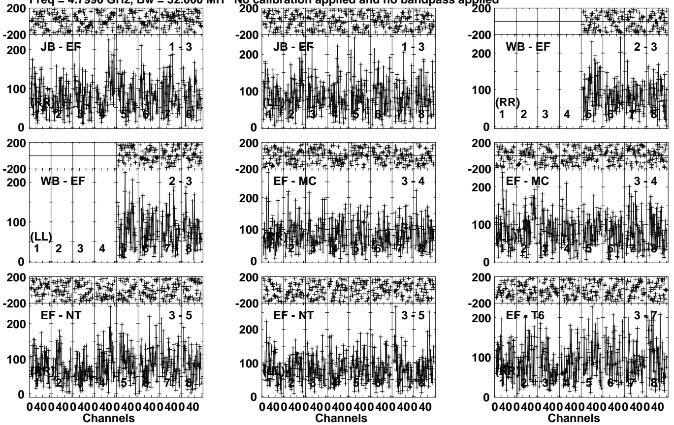
Lower frame: Micro Ampl Jy Top frame: Phas deg Vector averaged cross-power spectrum Several baselines displayed Timerange: 00/06:06:51 to 00/06:10:19
