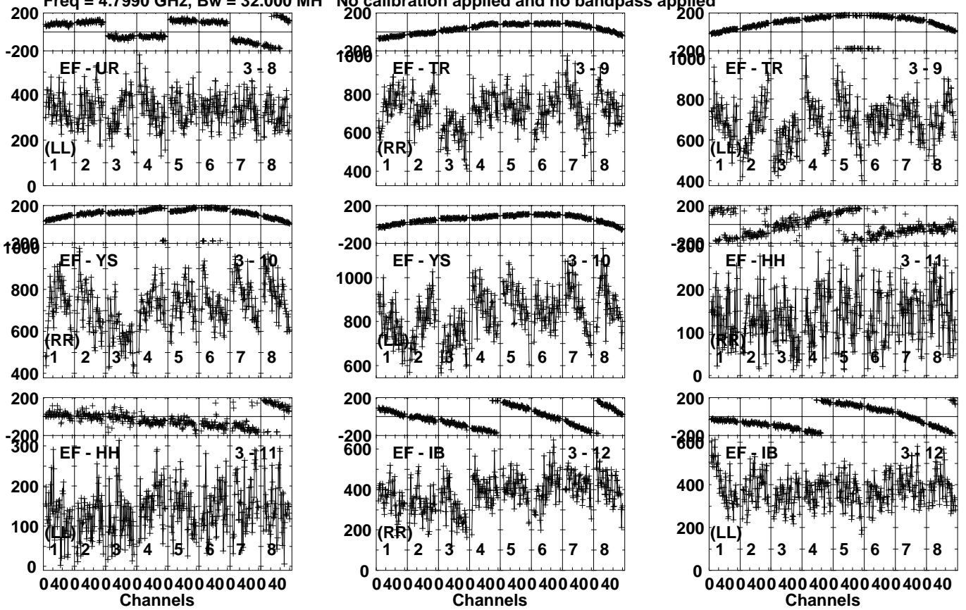
Lower frame: Micro Ampl Jy Top frame: Phas deg Vector averaged cross-power spectrum Several baselines displayed Timerange: 00/04:55:21 to 00/04:58:49
