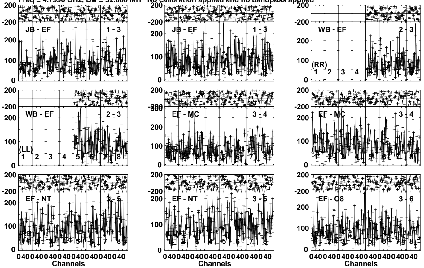
Lower frame: Micro Ampl Jy Top frame: Phas deg Vector averaged cross-power spectrum Several baselines displayed Timerange: 00/09:16:11 to 00/09:19:39
