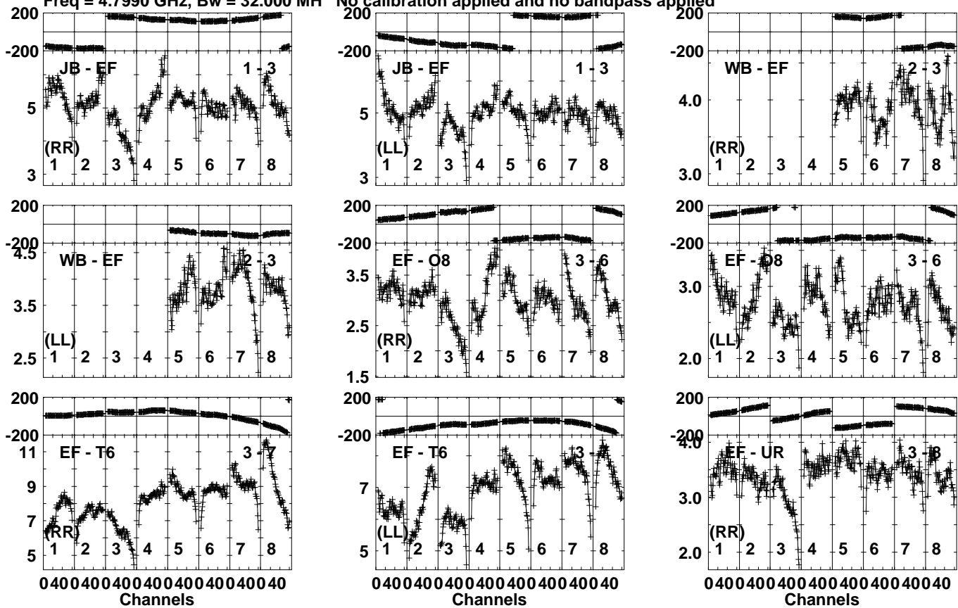
Lower frame: Milli Ampl Jy Top frame: Phas deg Vector averaged cross-power spectrum Several baselines displayed Timerange: 00/04:23:51 to 00/04:24:49
