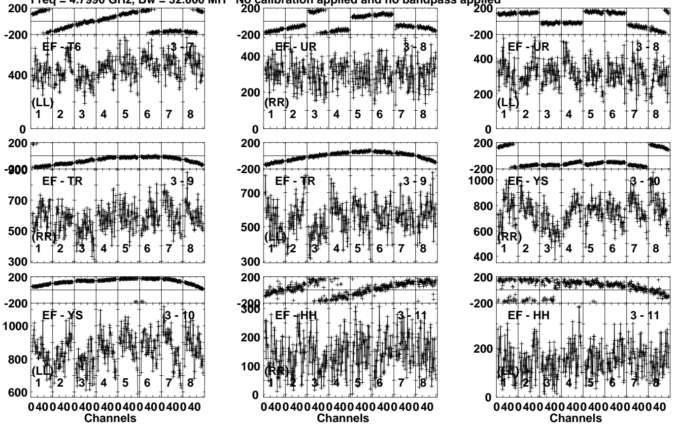
Lower frame: Micro Ampl Jy Top frame: Phas deg Vector averaged cross-power spectrum Several baselines displayed Timerange: 00/05:46:21 to 00/05:49:49
