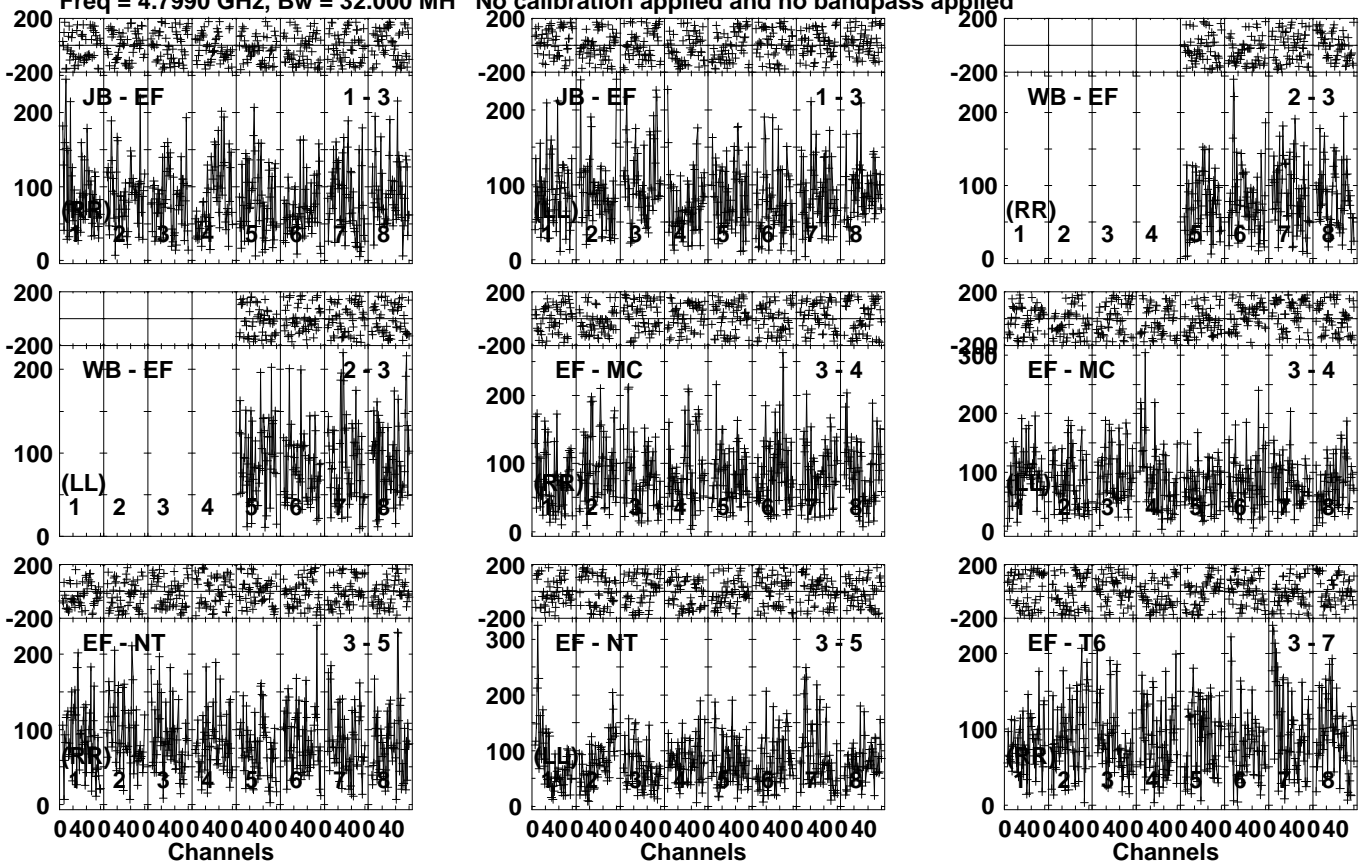
Lower frame: Micro Ampl Jy Top frame: Phas deg Vector averaged cross-power spectrum Several baselines displayed Timerange: 00/06:22:11 to 00/06:25:39
