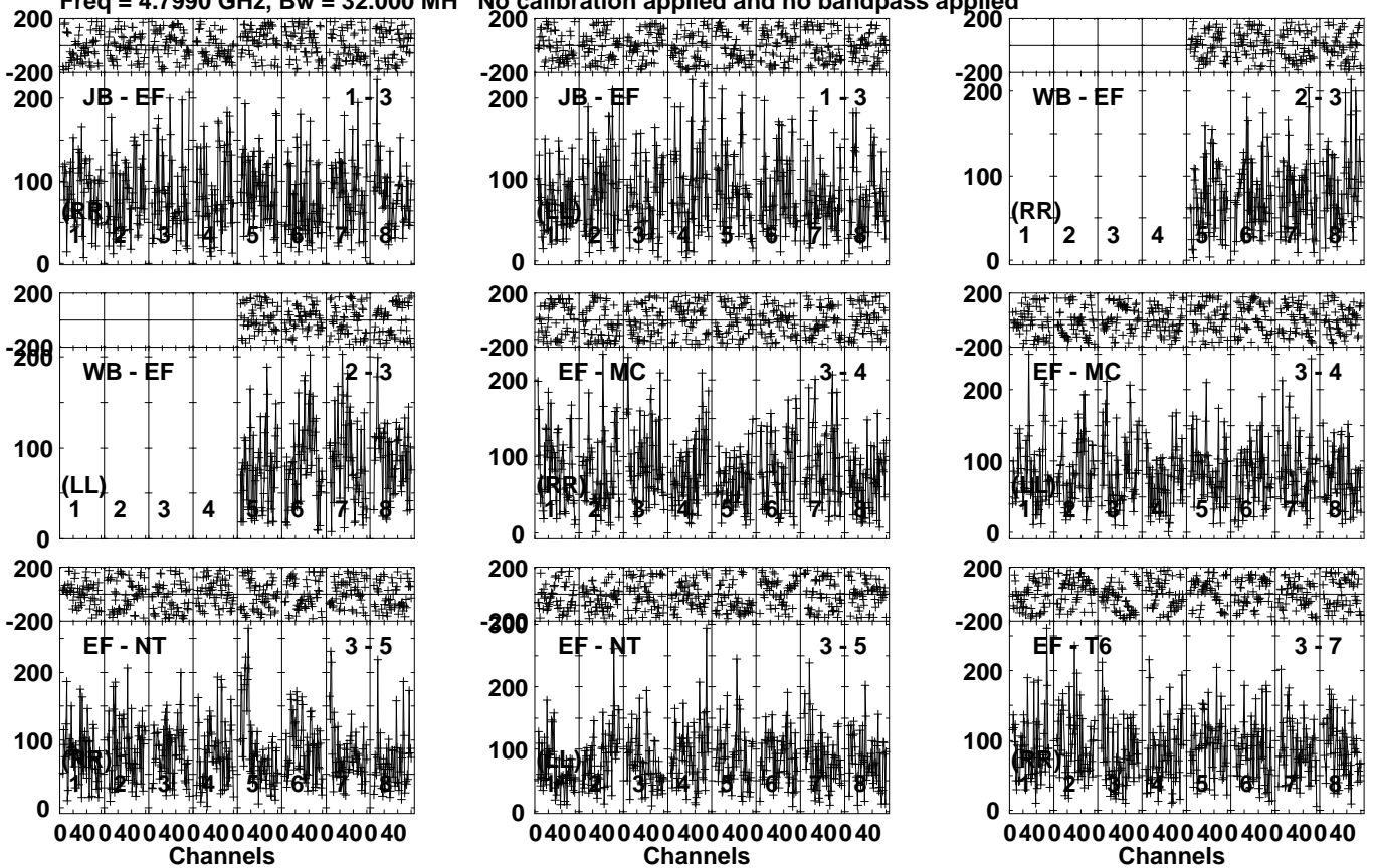
Lower frame: Micro Ampl Jy Top frame: Phas deg Vector averaged cross-power spectrum Several baselines displayed Timerange: 00/05:51:33 to 00/05:54:59
