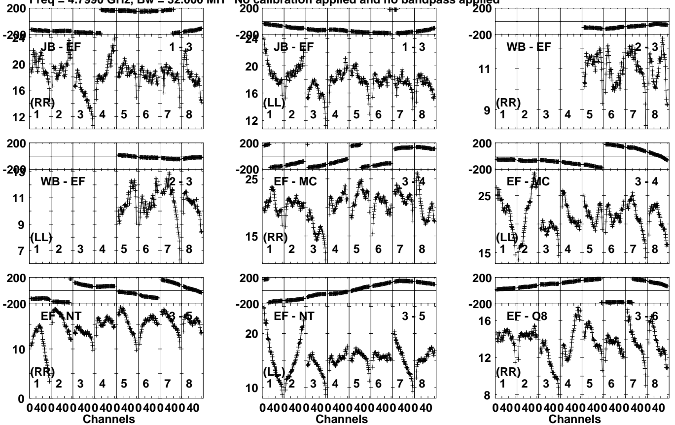
Lower frame: Milli Ampl Jy Top frame: Phas deg Vector averaged cross-power spectrum Several baselines displayed Timerange: 00/10:25:01 to 00/10:29:59
