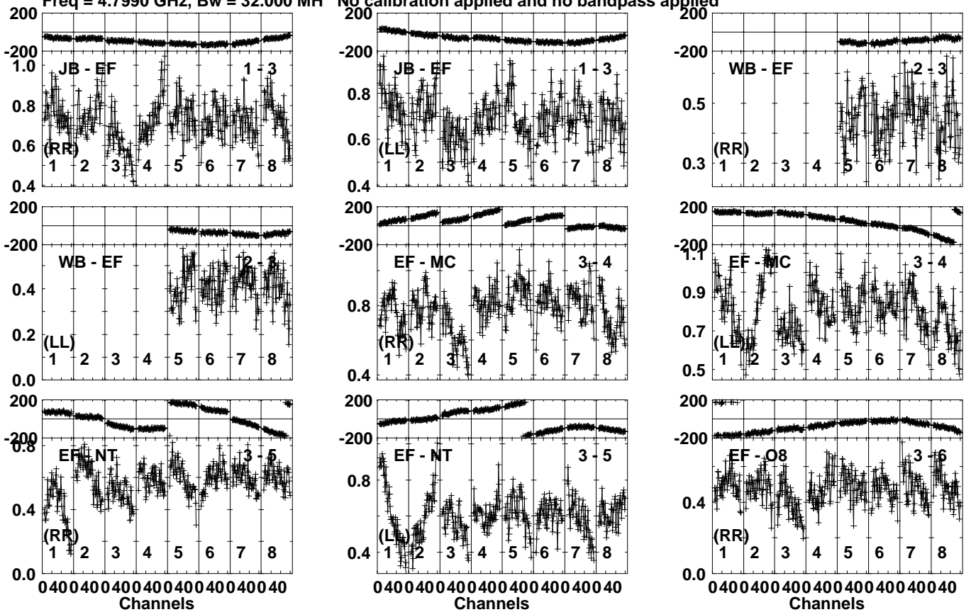
Lower frame: Milli Ampl Jy Top frame: Phas deg Vector averaged cross-power spectrum Several baselines displayed Timerange: 00/08:09:51 to 00/08:13:19
