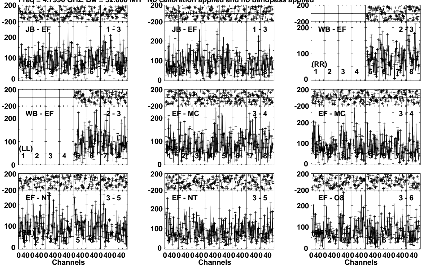
Lower frame: Micro Ampl Jy Top frame: Phas deg Vector averaged cross-power spectrum Several baselines displayed Timerange: 00/08:55:51 to 00/08:59:19
