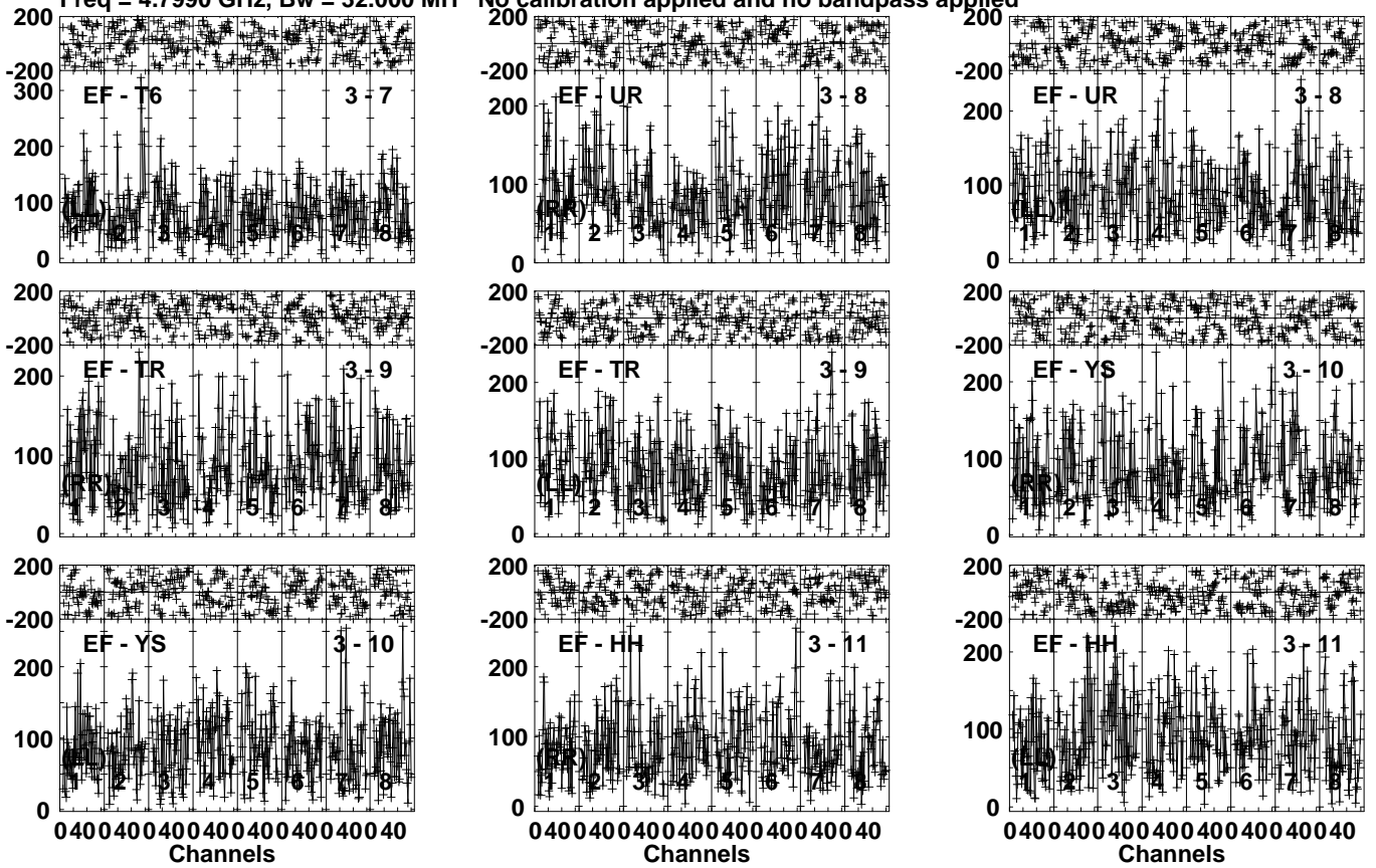
Lower frame: Micro Ampl Jy Top frame: Phas deg Vector averaged cross-power spectrum Several baselines displayed Timerange: 00/06:17:03 to 00/06:20:29
