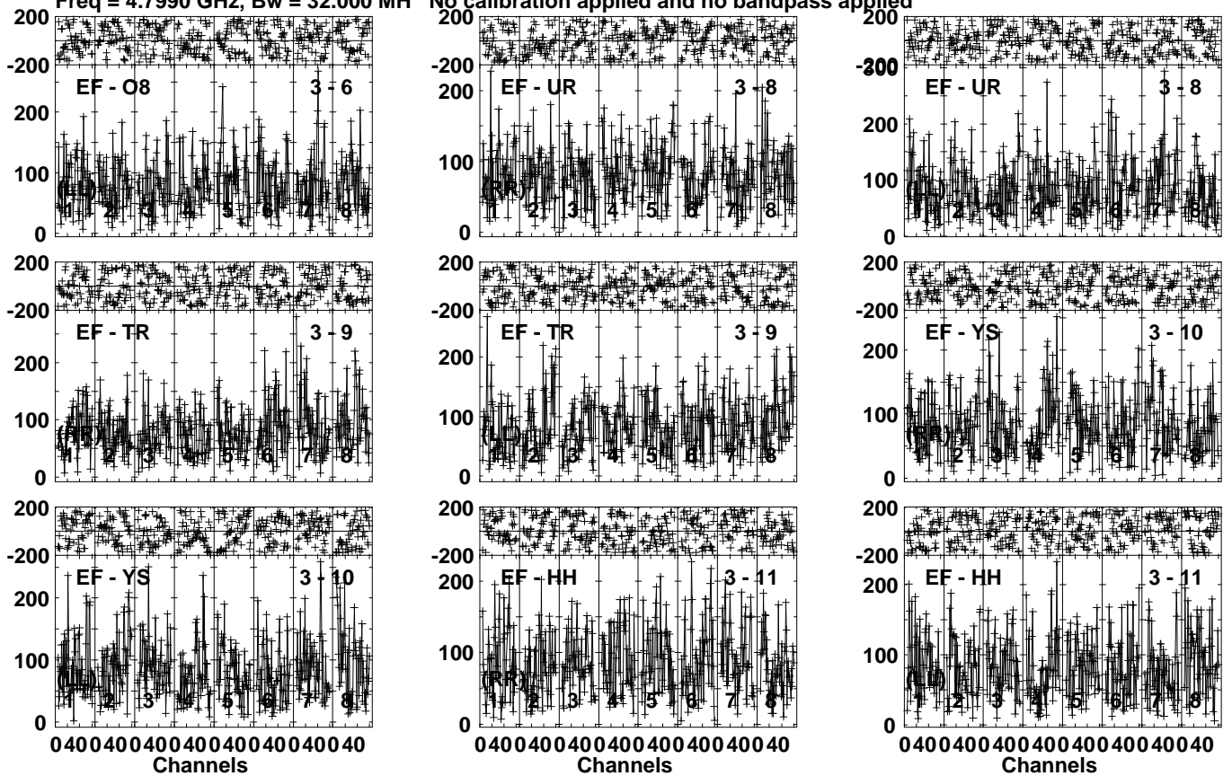
Lower frame: Micro Ampl Jy Top frame: Phas deg Vector averaged cross-power spectrum Several baselines displayed Timerange: 00/08:50:41 to 00/08:54:09
