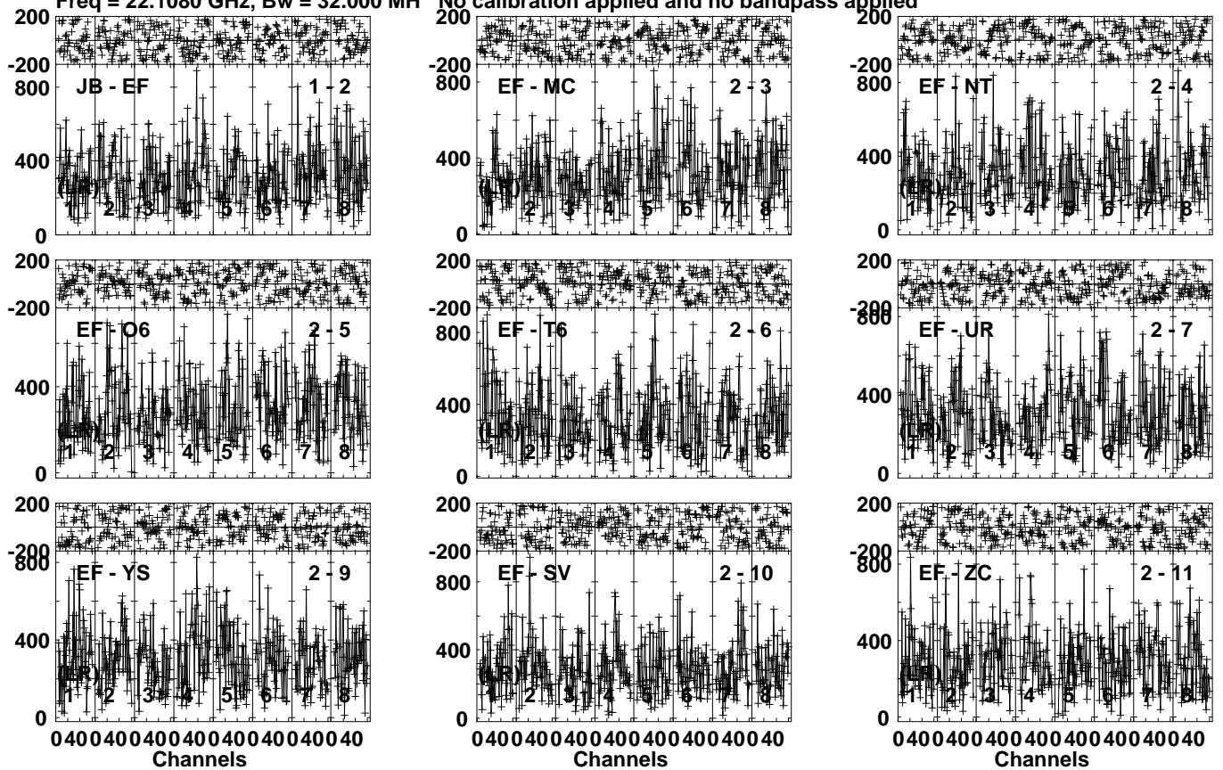
Lower frame: Micro Ampl Jy Top frame: Phas deg Vector averaged cross-power spectrum Several baselines displayed Timerange: 00/22:11:51 to 00/22:12:59
