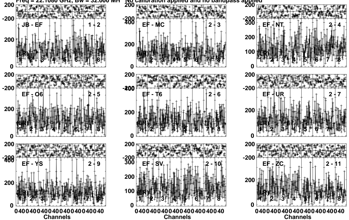
Lower frame: Micro Ampl Jy Top frame: Phas deg Vector averaged cross-power spectrum Several baselines displayed Timerange: 00/19:28:51 to 00/19:30:49
