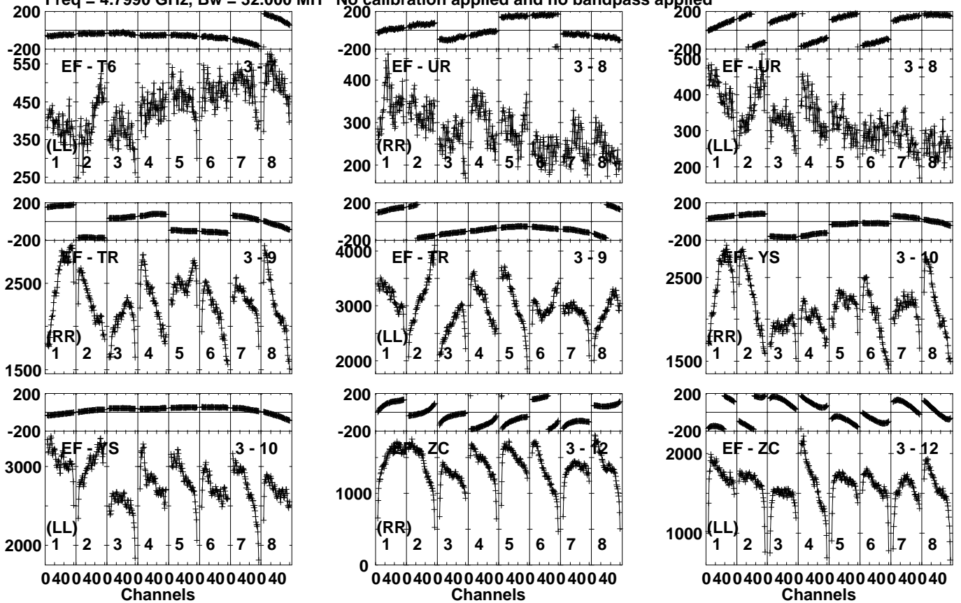
Lower frame: Micro Ampl Jy Top frame: Phas deg Vector averaged cross-power spectrum Several baselines displayed Timerange: 00/23:59:11 to 01/00:13:39
