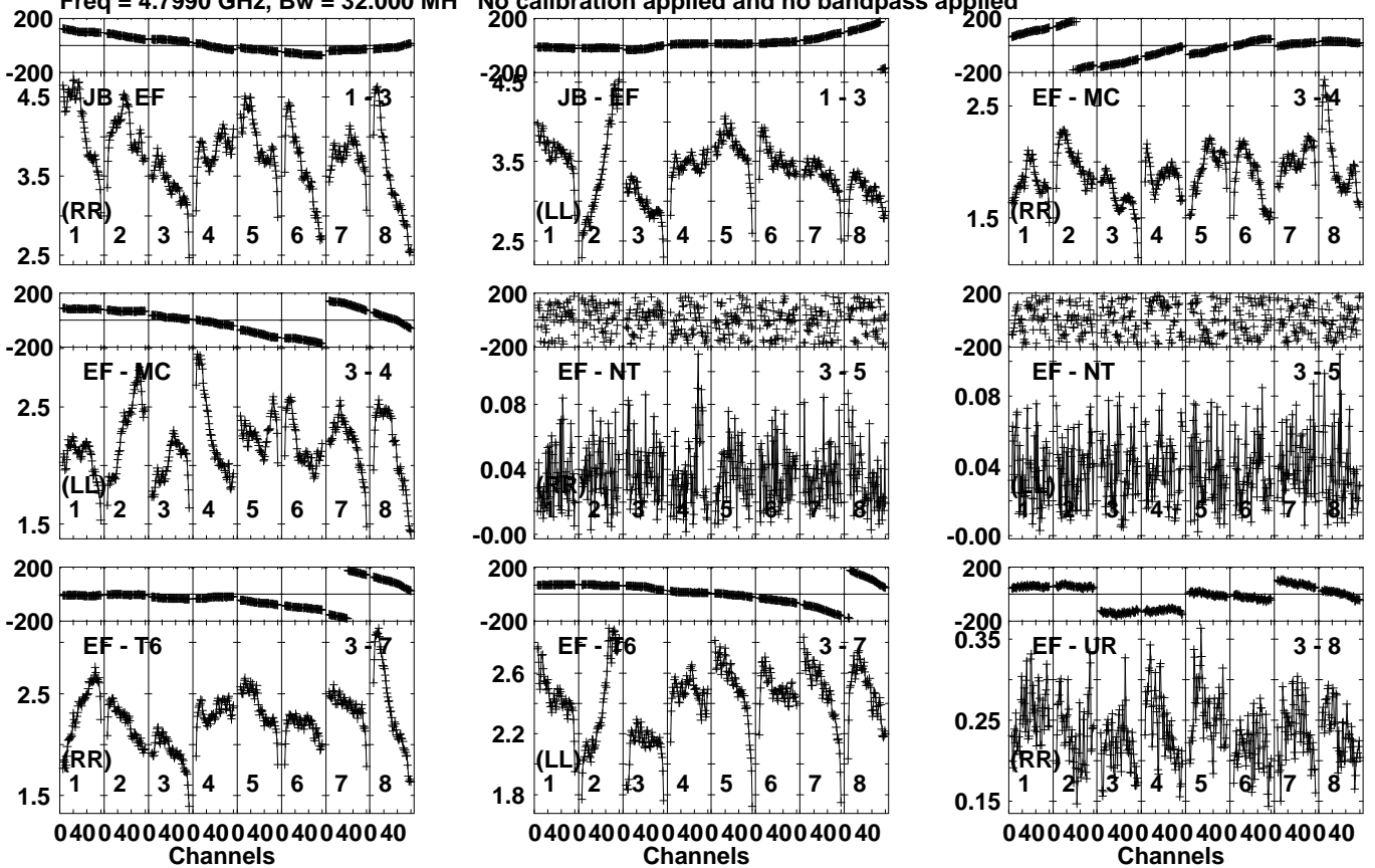
Lower frame: Milli Ampl Jy Top frame: Phas deg Vector averaged cross-power spectrum Several baselines displayed Timerange: 00/19:36:11 to 00/19:50:39
