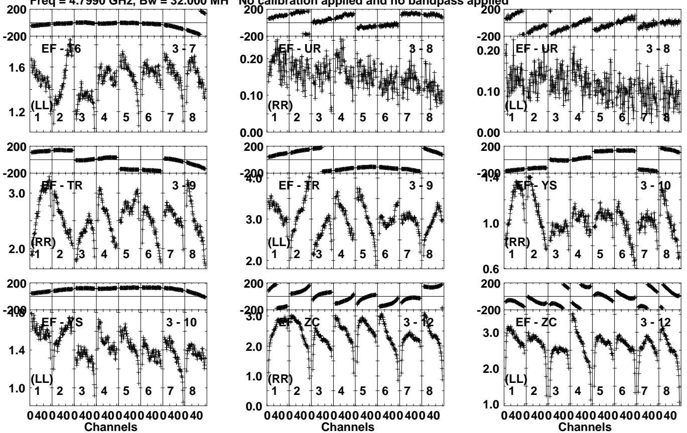
Lower frame: Milli Ampl Jy Top frame: Phas deg Vector averaged cross-power spectrum Several baselines displayed Timerange: 01/01:40:41 to 01/01:55:09
