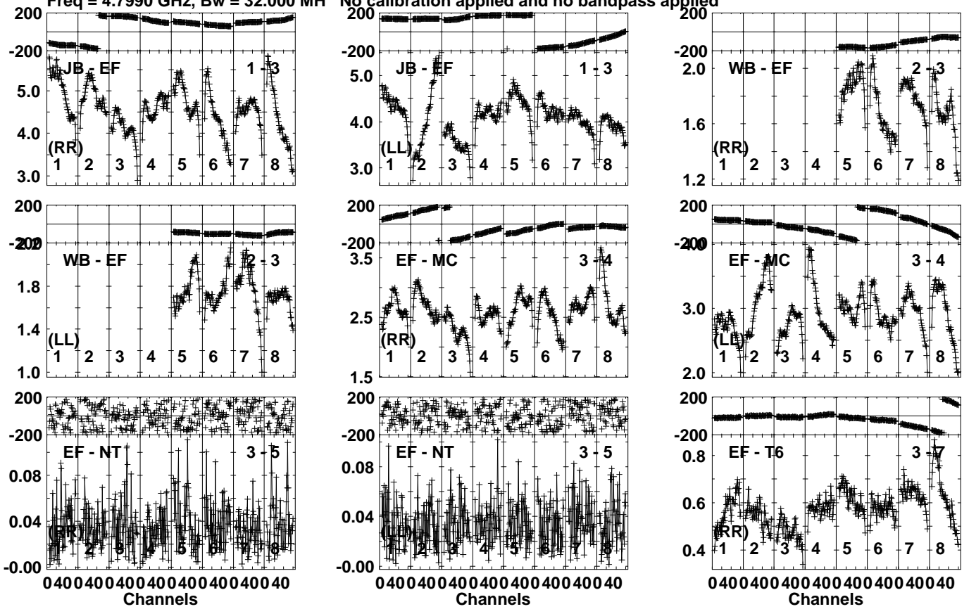
Lower frame: Milli Ampl Jy Top frame: Phas deg Vector averaged cross-power spectrum Several baselines displayed Timerange: 00/23:17:41 to 00/23:32:09
