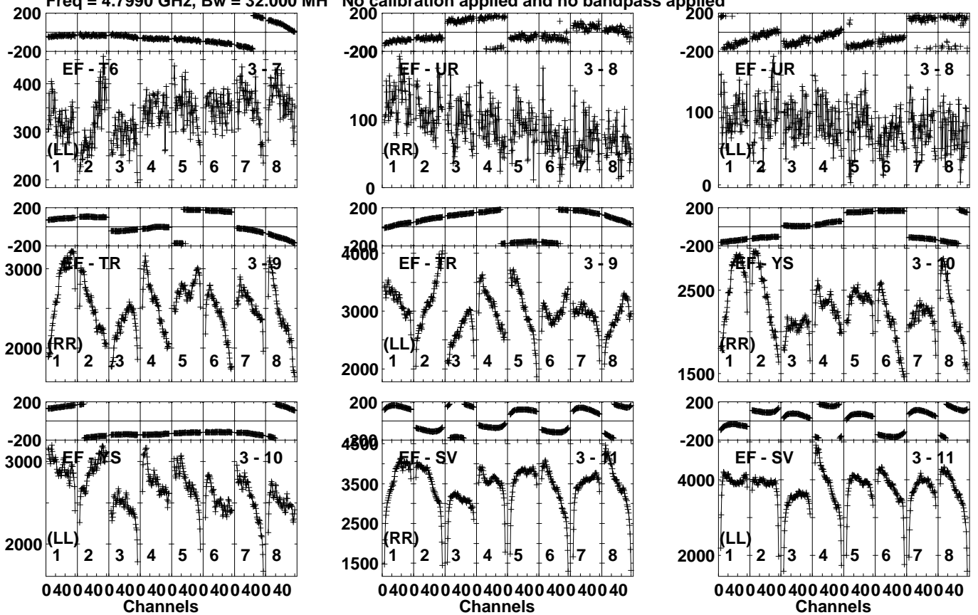
Lower frame: Micro Ampl Jy Top frame: Phas deg Vector averaged cross-power spectrum Several baselines displayed Timerange: 00/22:17:41 to 00/22:32:09
