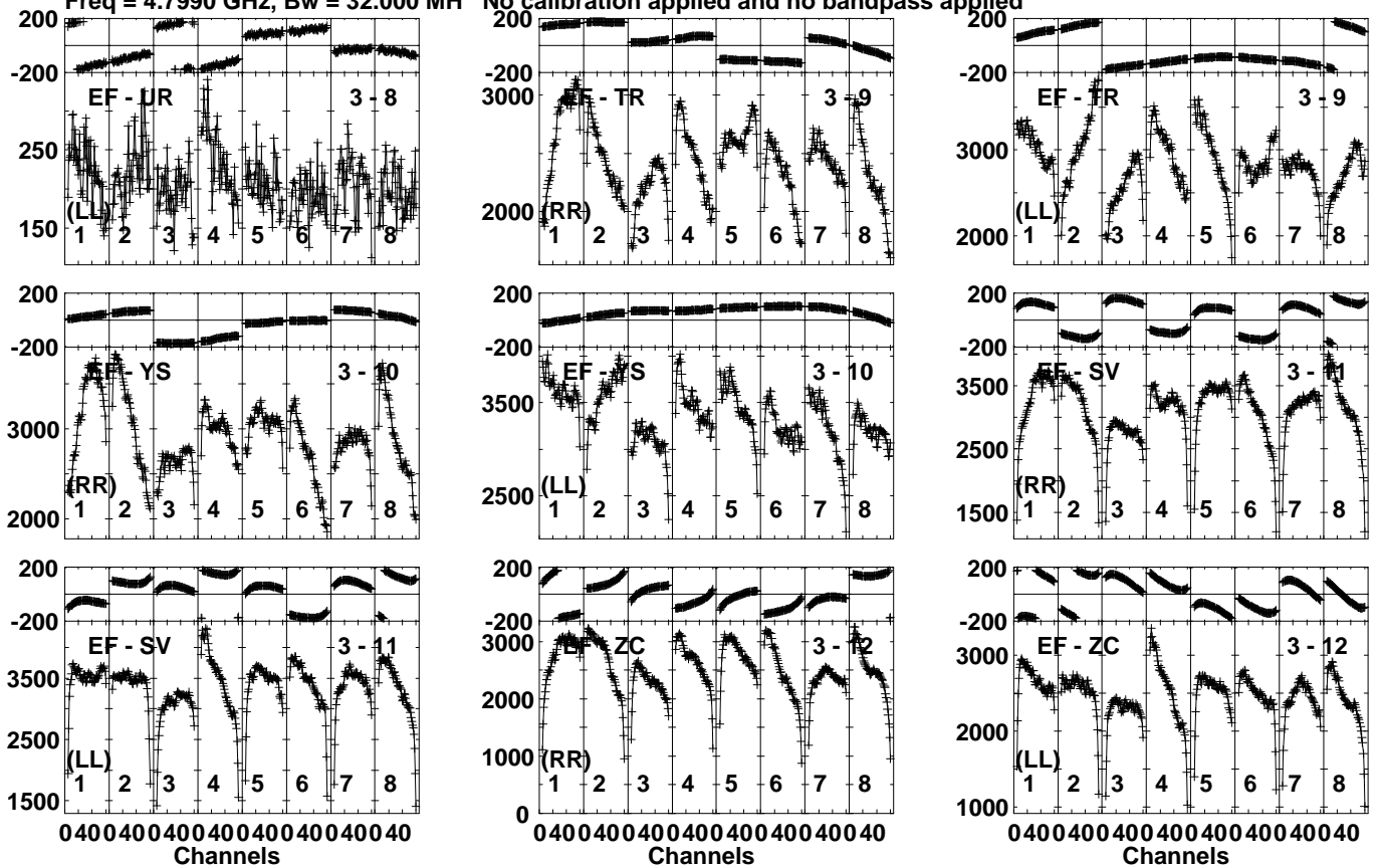
Lower frame: Micro Ampl Jy Top frame: Phas deg Vector averaged cross-power spectrum Several baselines displayed Timerange: 00/19:21:11 to 00/19:35:39
