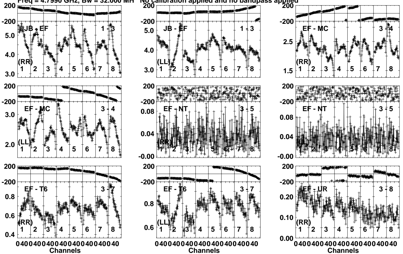
Lower frame: Milli Ampl Jy Top frame: Phas deg Vector averaged cross-power spectrum Several baselines displayed Timerange: 00/20:21:11 to 00/20:35:39
