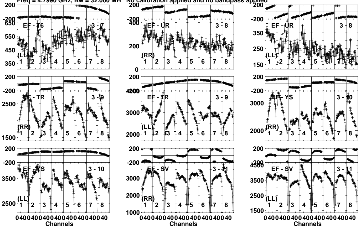
Lower frame: Micro Ampl Jy Top frame: Phas deg Vector averaged cross-power spectrum Several baselines displayed Timerange: 00/23:44:11 to 00/23:58:39
