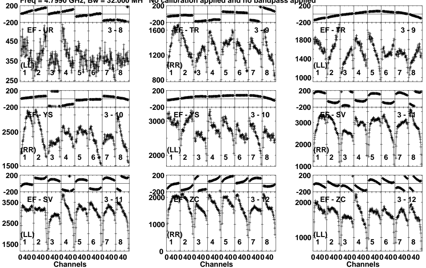
Lower frame: Micro Ampl Jy Top frame: Phas deg Vector averaged cross-power spectrum Several baselines displayed Timerange: 00/20:06:11 to 00/20:20:39
