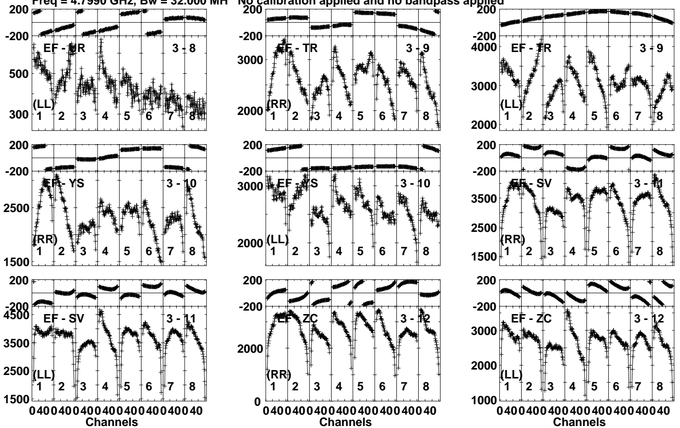
Lower frame: Micro Ampl Jy Top frame: Phas deg Vector averaged cross-power spectrum Several baselines displayed Timerange: 00/21:06:11 to 00/21:20:39
