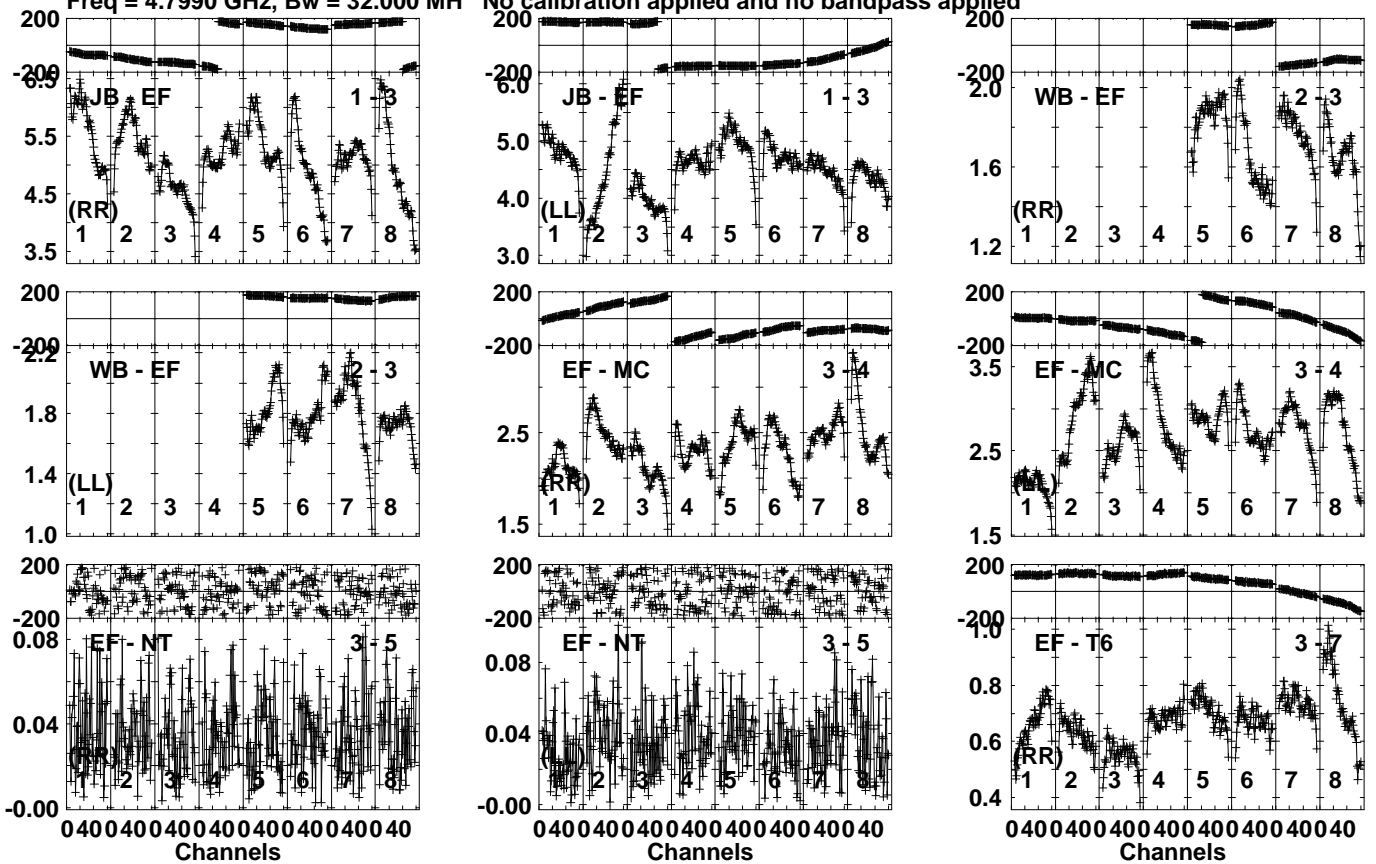
Lower frame: Milli Ampl Jy Top frame: Phas deg Vector averaged cross-power spectrum Several baselines displayed Timerange: 00/22:02:41 to 00/22:17:09
