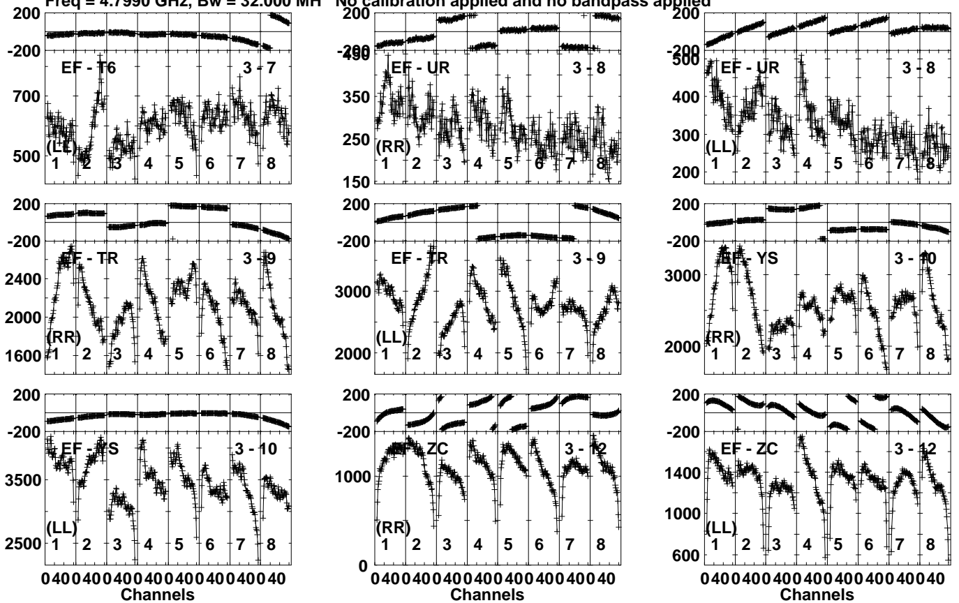
Lower frame: Micro Ampl Jy Top frame: Phas deg Vector averaged cross-power spectrum Several baselines displayed Timerange: 01/00:14:11 to 01/00:28:39
