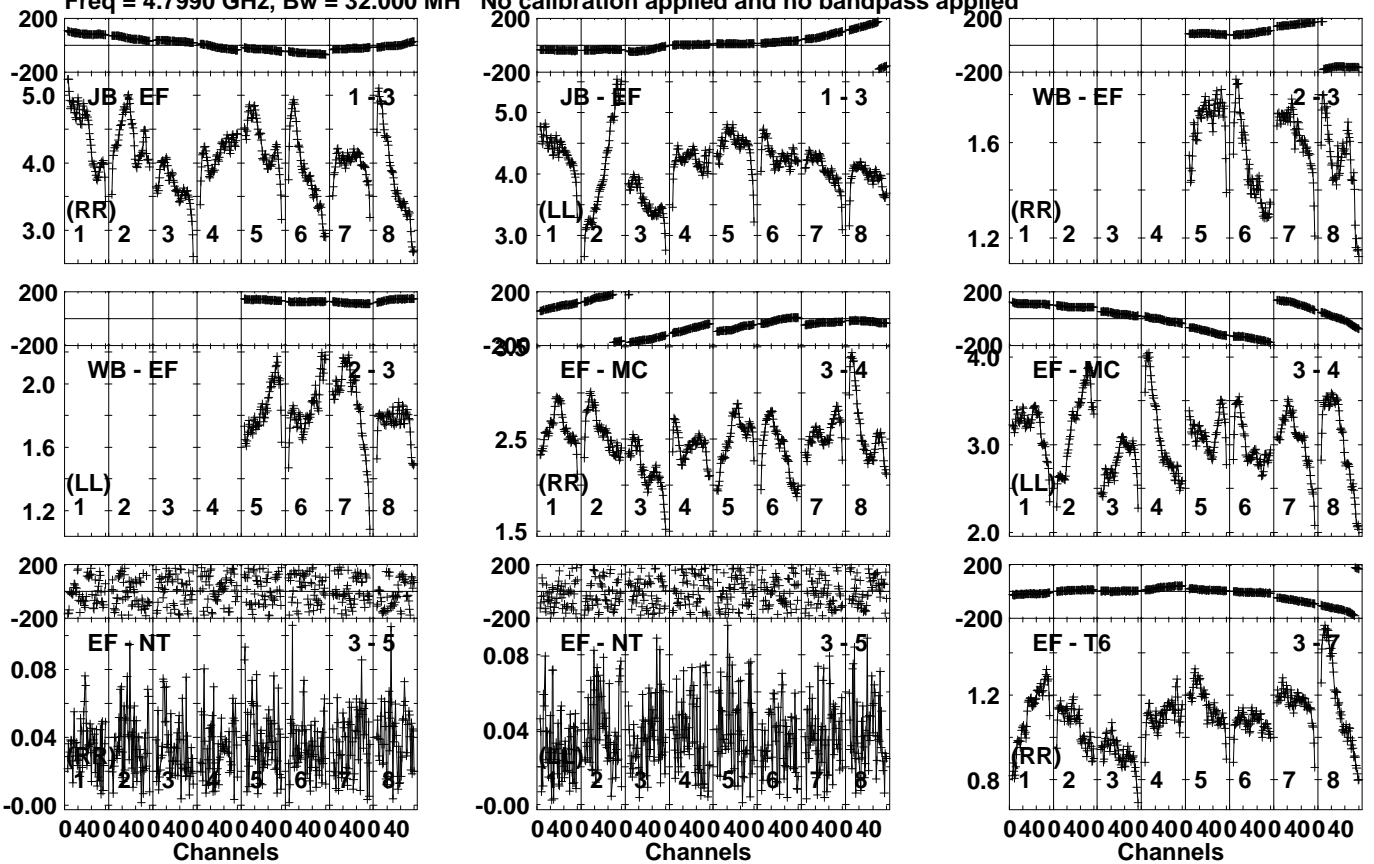
Lower frame: Milli Ampl Jy Top frame: Phas deg Vector averaged cross-power spectrum Several baselines displayed Timerange: 01/00:29:11 to 01/00:43:39
