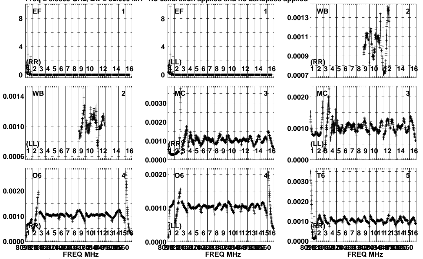
Lower frame: Kilo Real Jy Auto-corr total-power spectrum Antenna: * Timerange: 00/09:34:23 to 00/09:43:59
