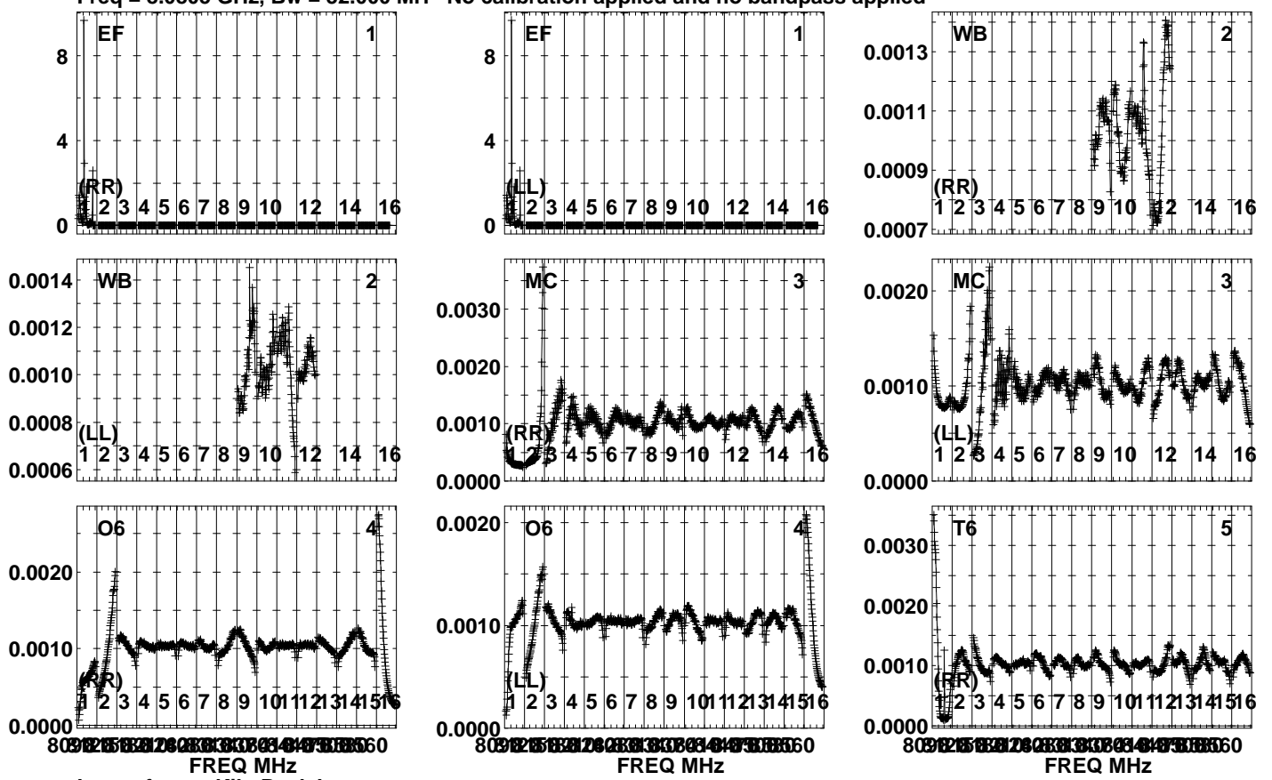
Lower frame: Kilo Real Jy Auto-corr total-power spectrum Antenna: * Timerange: 00/03:00:33 to 00/03:04:59
