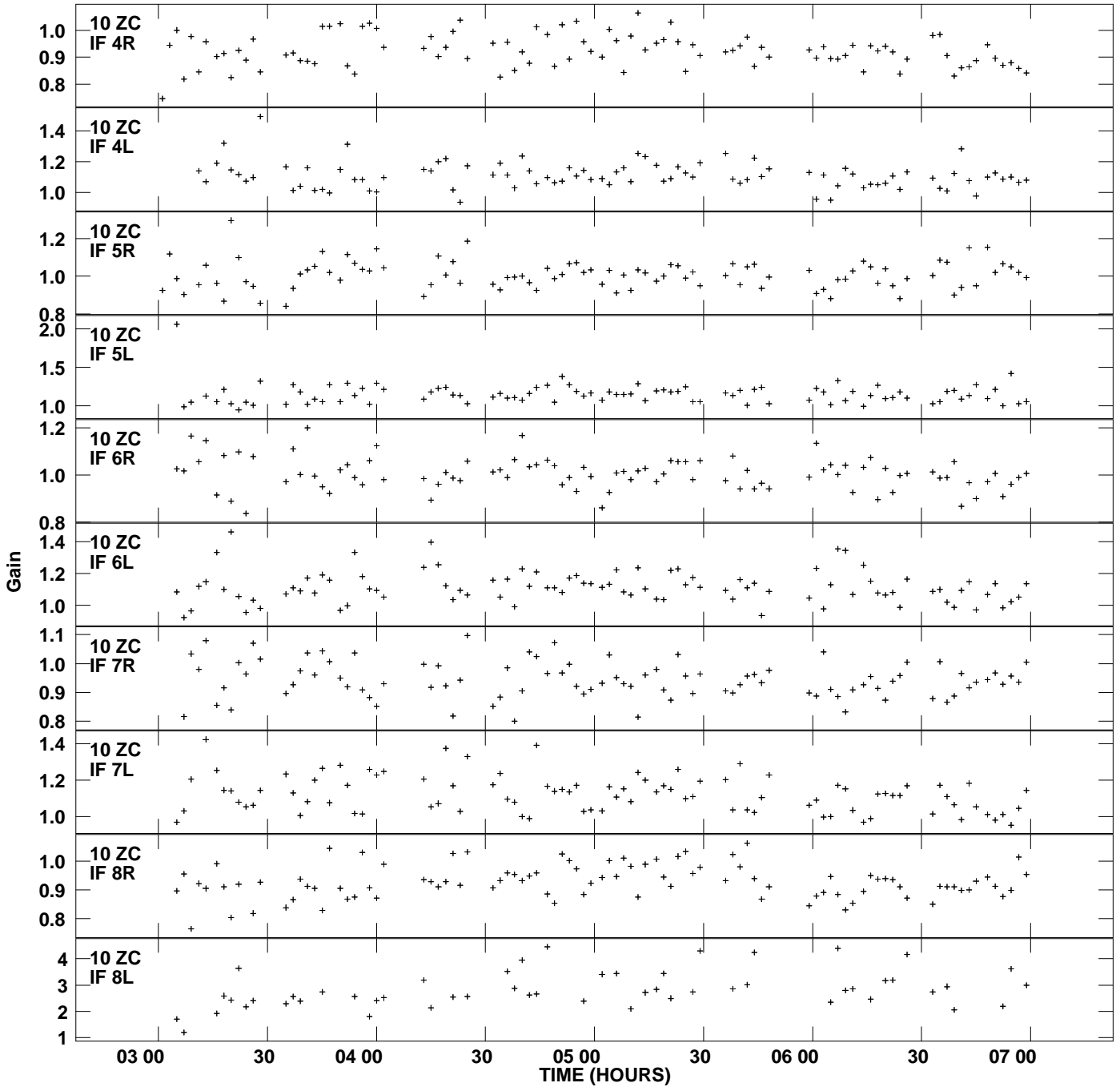
Plot file version 12 created 20-NOV-2012 13:19:06 Gain amp vs UTC time for 0229+200.MULTI.1 SN 2 Rpol & Lpol IF 1 - 8
