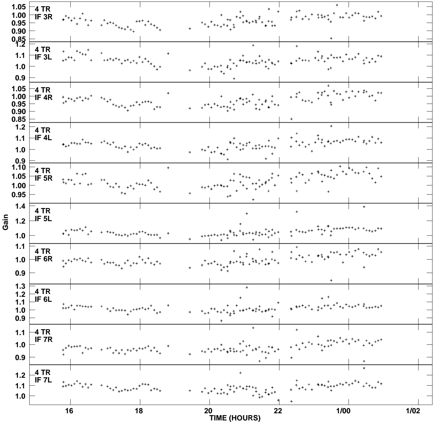
Plot file version 6 created 22-SEP-2010 15:15:30 Gain amp vs UTC time for J2102+4702.MULTI.1 SN 2 Rpol & Lpol IF 1 - 8
