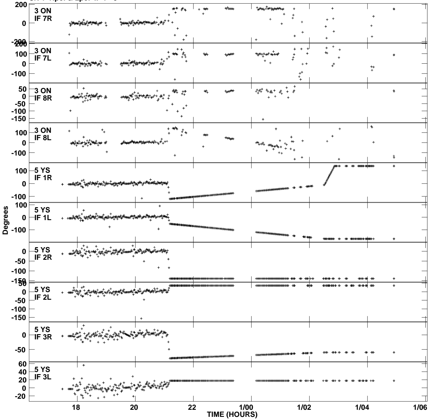
Plot file version 5 created 15-AUG-2012 16:35:10 Gain phs vs UTC time for J1638+5720.MULTI.1 SN 1 Rpol & Lpol IF 1 - 8
