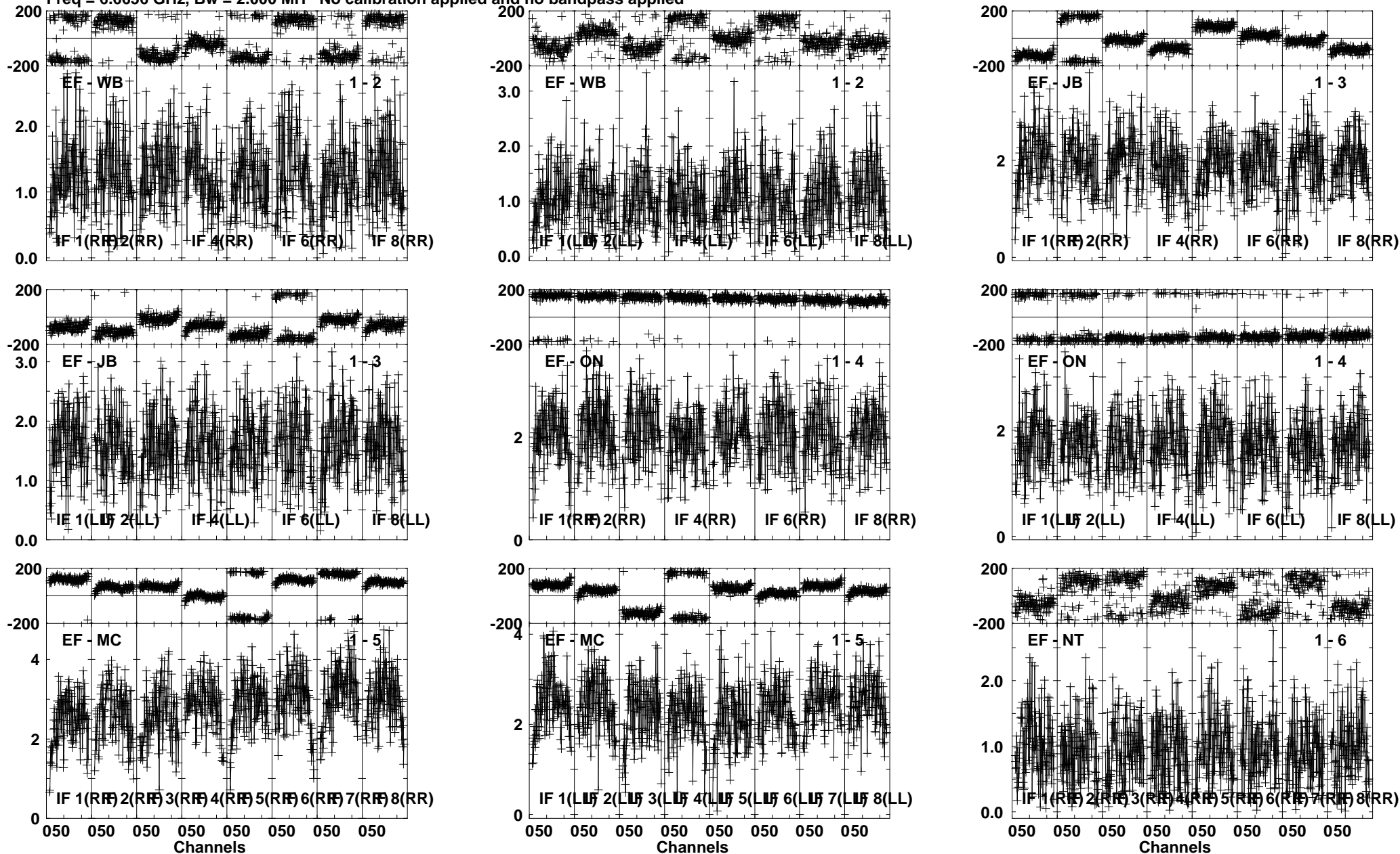
Lower frame: Milli Ampl Jy Top frame: Phas deg Vector averaged cross-power spectrum Several baselines displayed Timerange: 01/06:16:54 to 01/06:18:52
