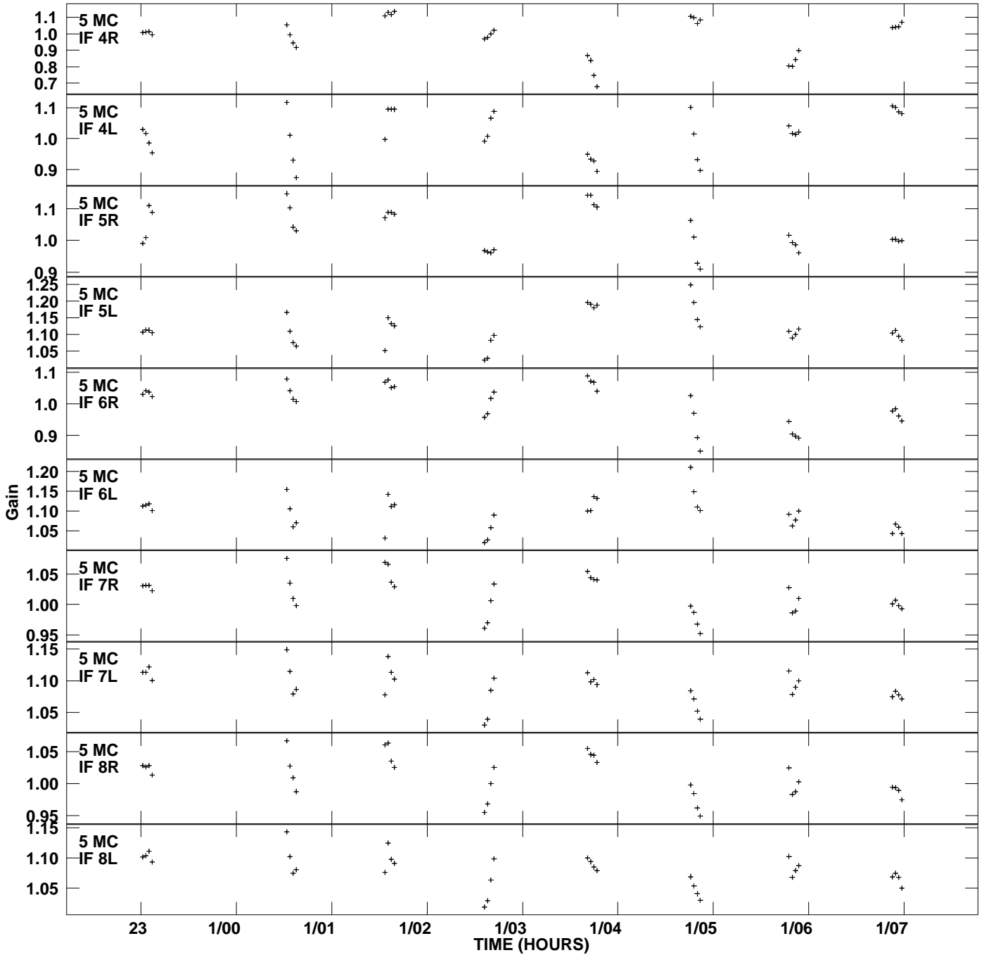
Plot file version 8 created 21-OCT-2013 17:53:46 Gain amp vs UTC time for J2202+4216.MULTI.1 SN 2 Rpol & Lpol IF 1 - 8
