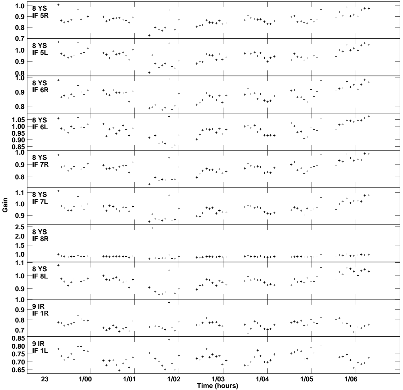
Plot file version 13 created 17-JAN-2018 18:17:55 Gain amp vs UTC time for J1930+1532.MULTI.1 SN 2 Rpol & Lpol IF 1 - 8
