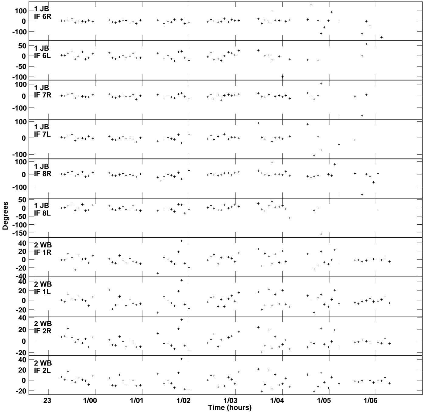
Plot file version 2 created 17-JAN-2018 18:17:43 Gain phs vs UTC time for J1930+1532.MULTI.1 SN 1 Rpol & Lpol IF 1 - 8
